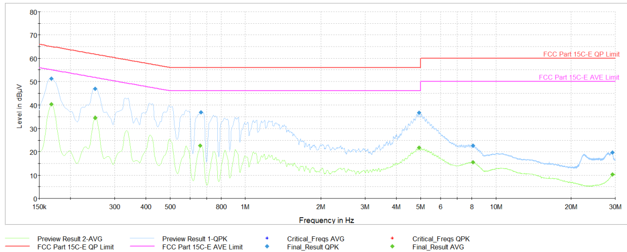
Plot 7-129. AC Line Conducted Emissions with 802.11ax (RU26) Ch.6 (N, with AC/DC Adapter)
