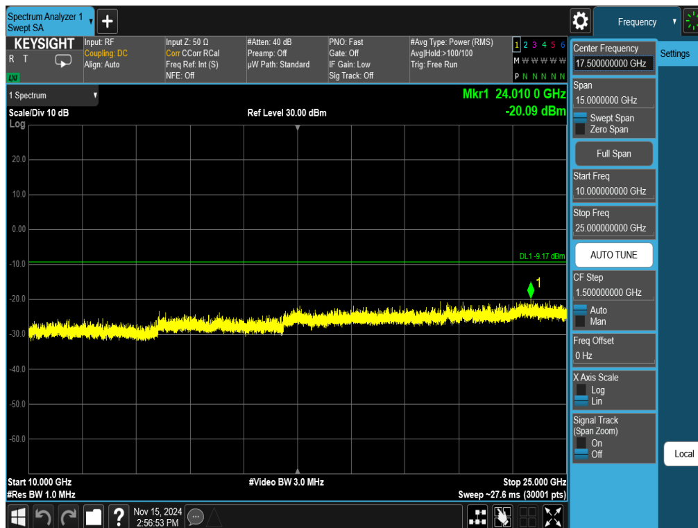
Plot 7-66. Conducted Spurious Plot Antenna 1a (802.11ax OFDMA – RU242 – Ch. 11)
