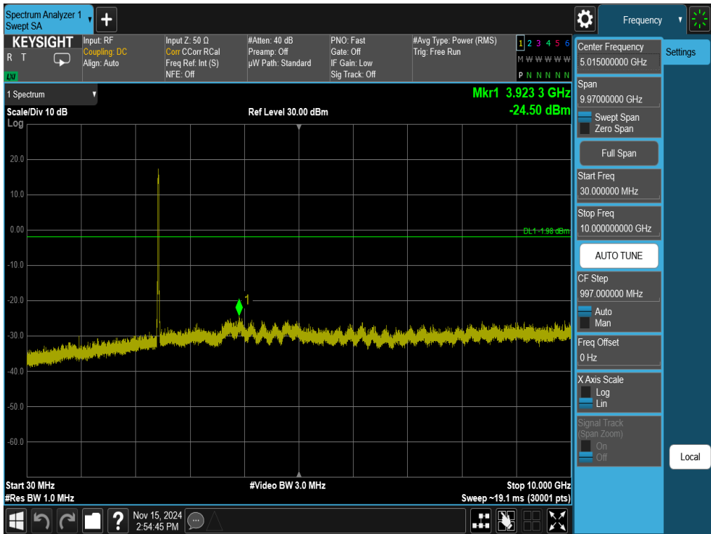
Plot 7-63. Conducted Spurious Plot Antenna 1a (802.11ax OFDMA – RU242 – Ch. 6)
