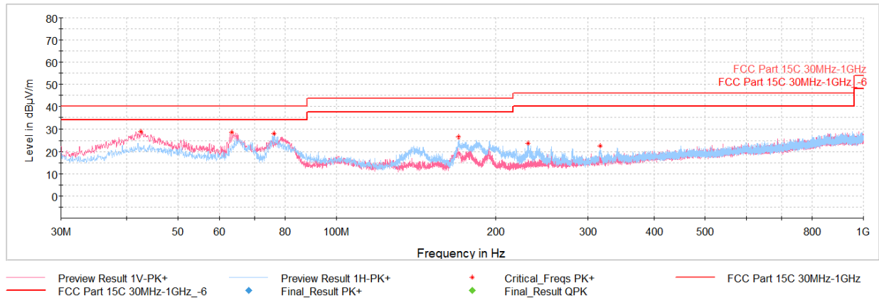
Plot 7-127. Radiated Spurious Emissions below 1GHz CDD Ch.6 (RU242), with AC/DC Adapter
