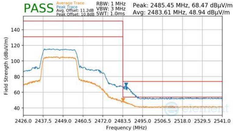
Plot 7-104 Radiated Restricted Upper Band Edge Measurement Antenna 1a (Peak & Average – RU242)
