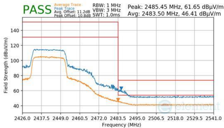
Plot 7-103 Radiated Restricted Upper Band Edge Measurement Antenna 1a (Peak & Average – RU242)
