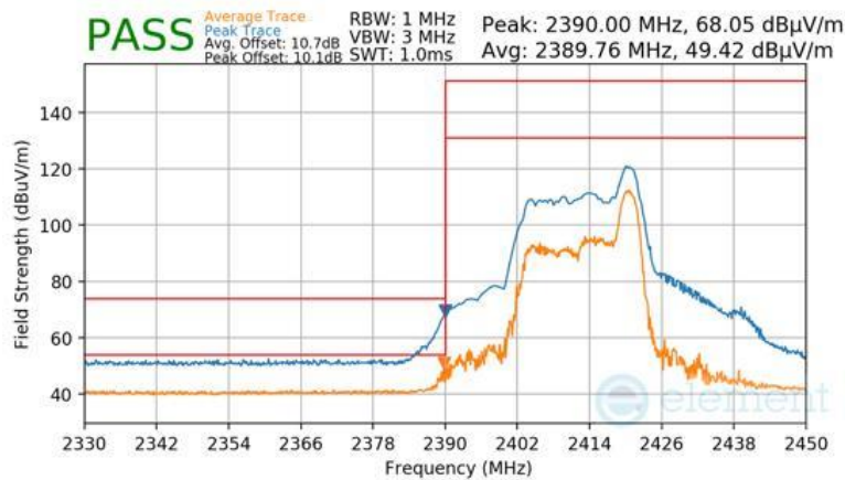
Plot 7-93 Radiated Restricted Lower Band Edge Measurement Antenna 1a (Peak & Average – RU26)
