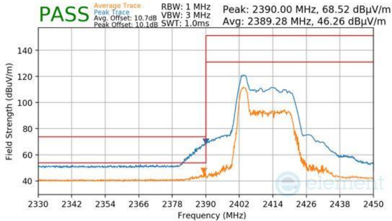
Plot 7-75 Radiated Restricted Lower Band Edge Measurement Antenna 3a (Peak & Average – RU26)
