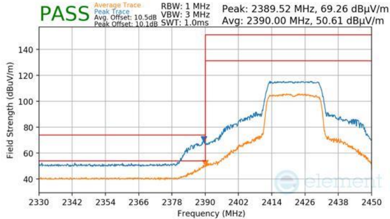
Plot 7-81 Radiated Restricted Lower Band Edge Measurement Antenna 3a (Peak & Average – RU242)
