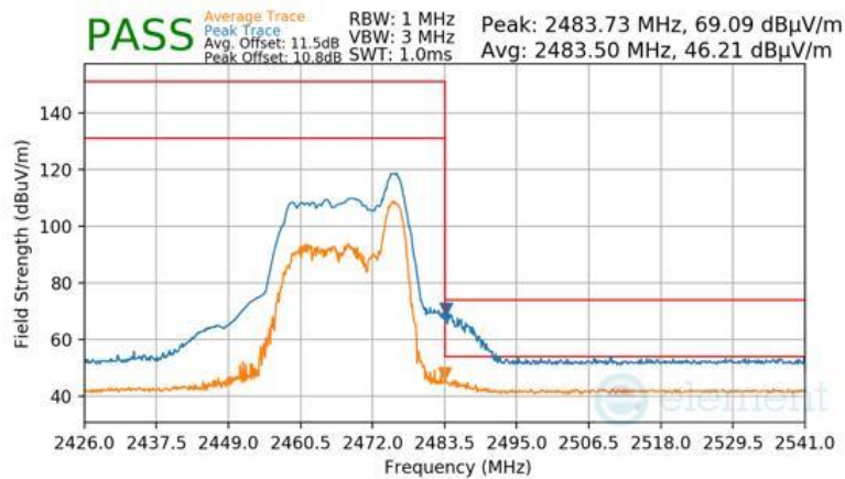
Plot 7-95 Radiated Restricted Upper Band Edge Measurement Antenna 1a (Peak & Average – RU26)
