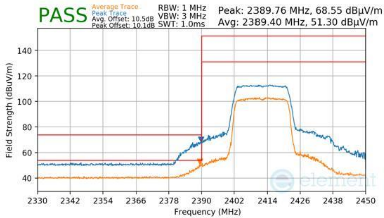
Plot 7-79 Radiated Restricted Lower Band Edge Measurement Antenna 3a (Peak & Average – RU242)
