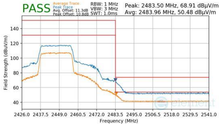
Plot 7-87 Radiated Restricted Upper Band Edge Measurement Antenna 3a (Peak & Average – RU242)
