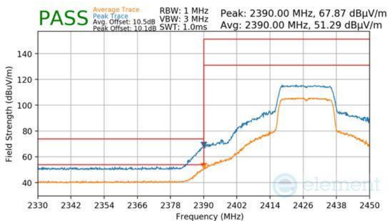
Plot 7-99 Radiated Restricted Lower Band Edge Measurement Antenna 1a (Peak & Average – RU242)
