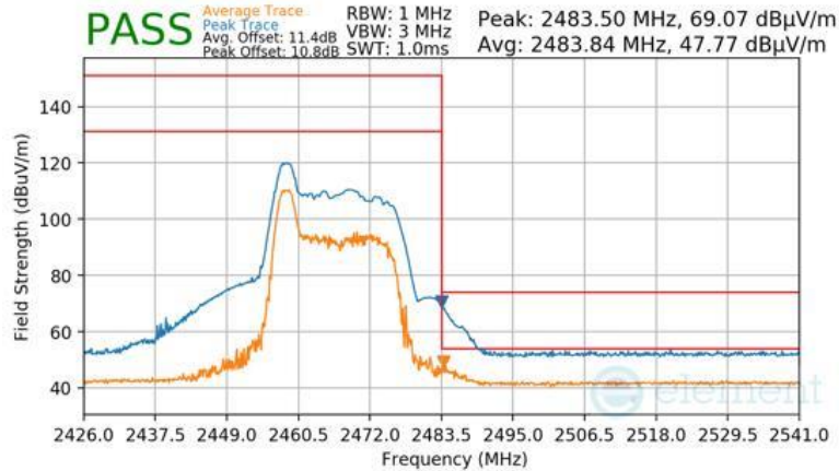
Plot 7-94 Radiated Restricted Upper Band Edge Measurement Antenna 1a (Peak & Average – RU26)
