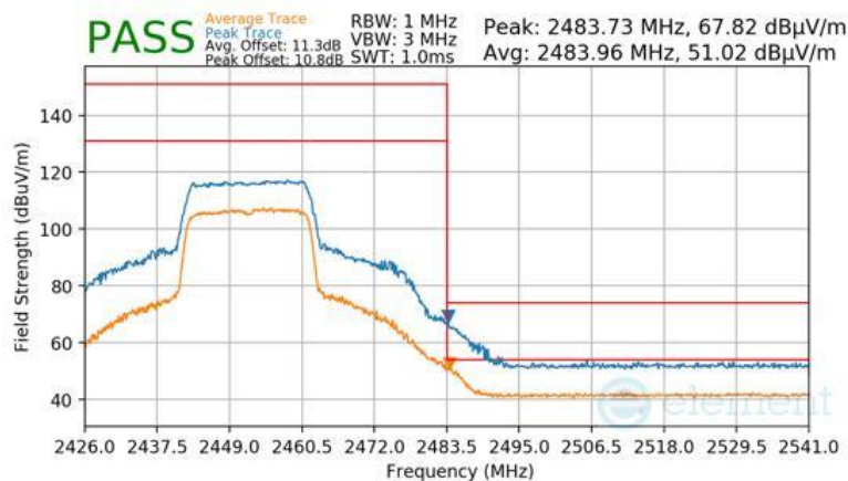
Plot 7-88 Radiated Restricted Upper Band Edge Measurement Antenna 3a (Peak & Average – RU242)
