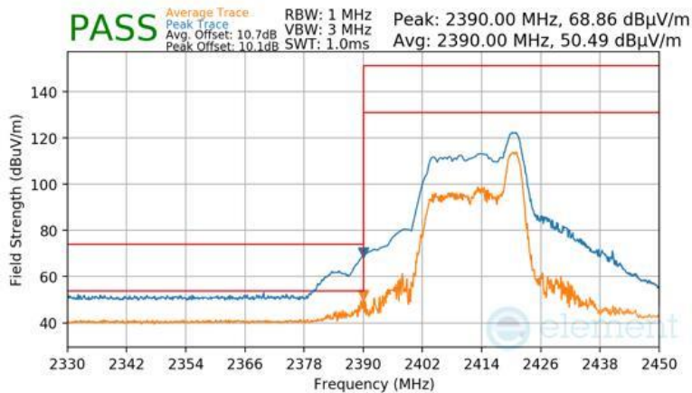
Plot 7-76 Radiated Restricted Lower Band Edge Measurement Antenna 3a (Peak & Average – RU26)
