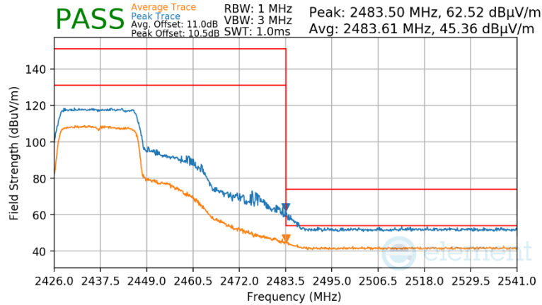
Plot 7-85 Radiated Restricted Upper Band Edge Measurement Antenna 3a (Peak & Average – RU242)
