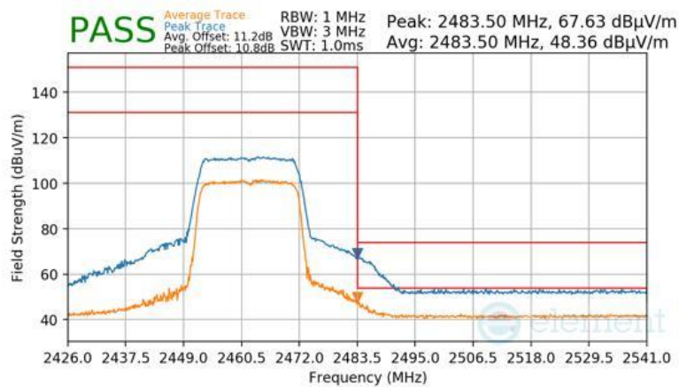
Plot 7-107 Radiated Restricted Upper Band Edge Measurement Antenna 1a (Peak & Average – RU242)
