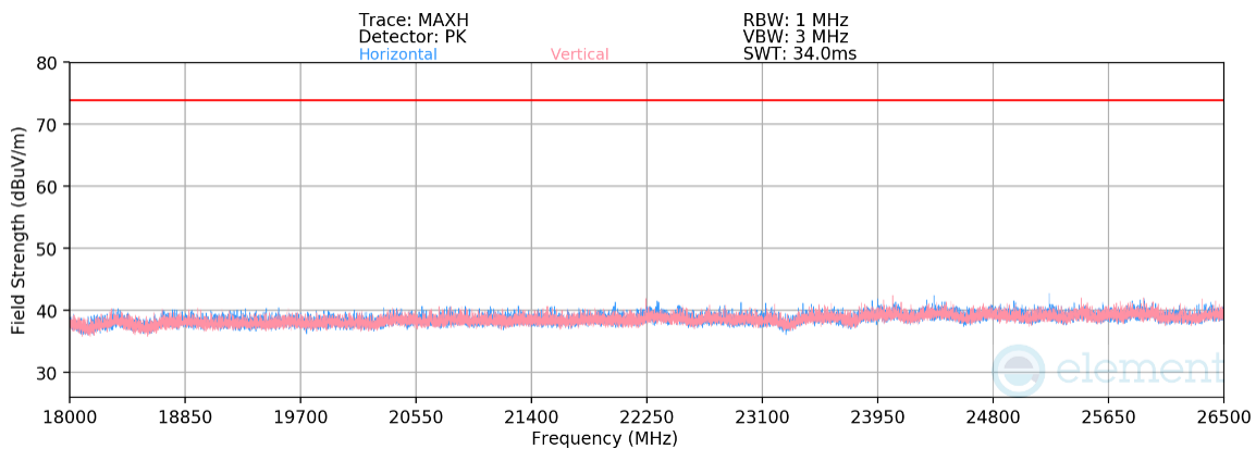
Plot 7-73. Radiated Spurious Emissions above 18GHz CDD (802.11ax OFDMA – RU242 – Ch. 6)
