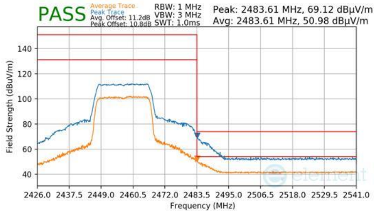
Plot 7-106 Radiated Restricted Upper Band Edge Measurement Antenna 1a (Peak & Average – RU242)
