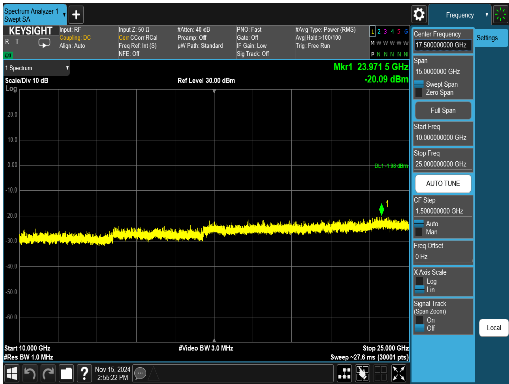
Plot 7-64. Conducted Spurious Plot Antenna 1a (802.11ax OFDMA – RU242 – Ch. 6)
