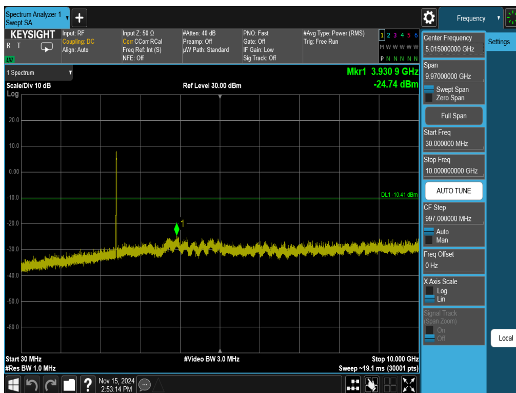
Plot 7-61. Conducted Spurious Plot Antenna 1a (802.11ax OFDMA – RU242 – Ch. 1)
