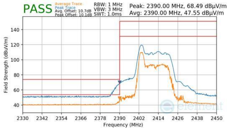
Plot 7-92 Radiated Restricted Lower Band Edge Measurement Antenna 1a (Peak & Average – RU26)
