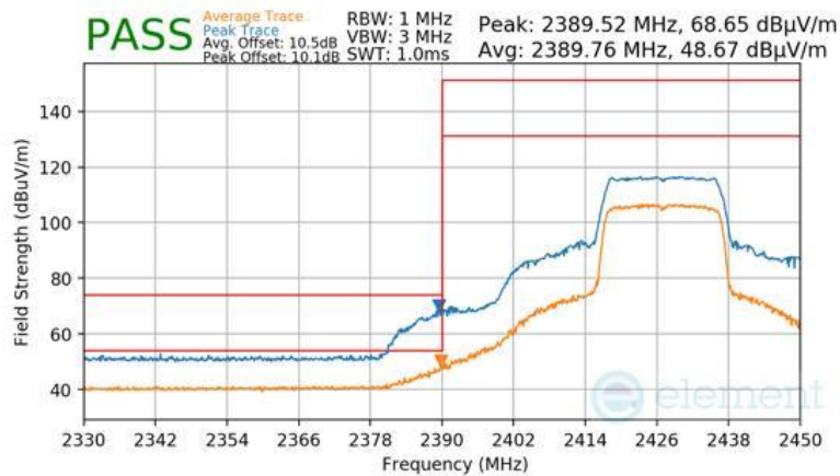
Plot 7-82 Radiated Restricted Lower Band Edge Measurement Antenna 3a (Peak & Average – RU242)
