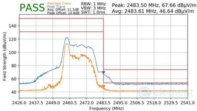
Plot 7-77 Radiated Restricted Upper Band Edge Measurement Antenna 3a (Peak & Average – RU26)
