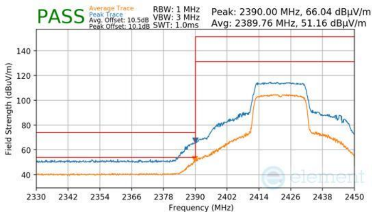
Plot 7-98 Radiated Restricted Lower Band Edge Measurement Antenna 1a (Peak & Average – RU242)
