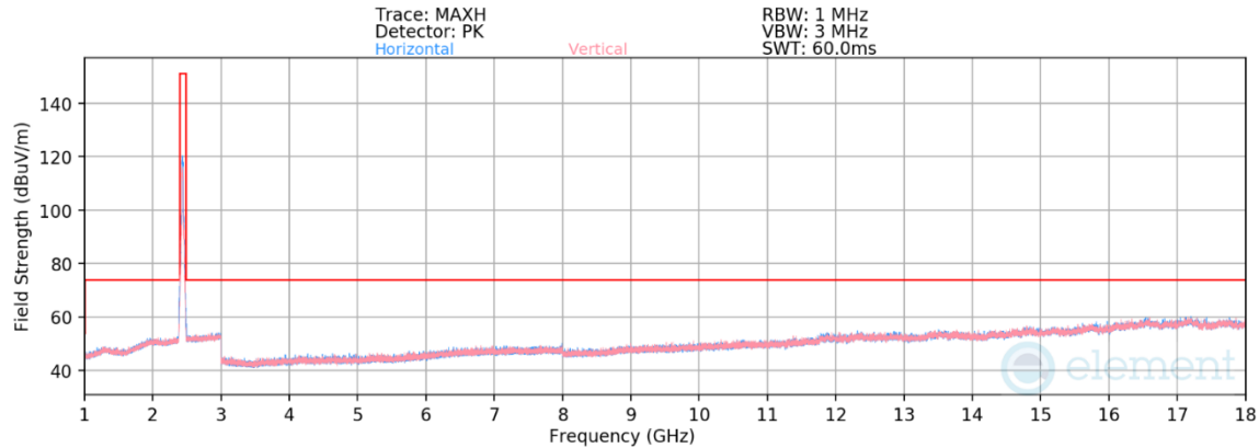
Plot 7-72. Radiated Spurious Emissions above 1GHz CDD (802.11ax OFDMA – RU242 – Ch. 6)
