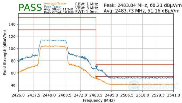
Plot 7-105 Radiated Restricted Upper Band Edge Measurement Antenna 1a (Peak & Average – RU242)
