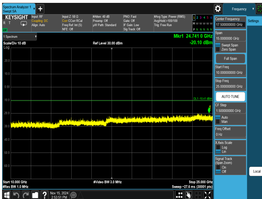
Plot 7-62. Conducted Spurious Plot Antenna 1a (802.11ax OFDMA – RU242 – Ch. 1)
