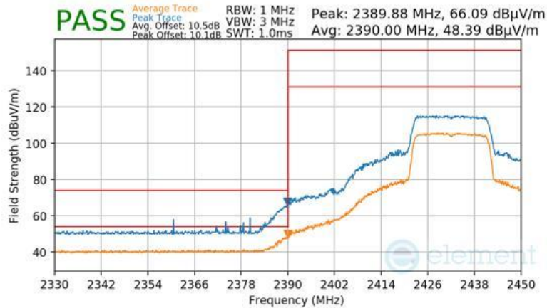
Plot 7-100 Radiated Restricted Lower Band Edge Measurement Antenna 1a (Peak & Average – RU242)
