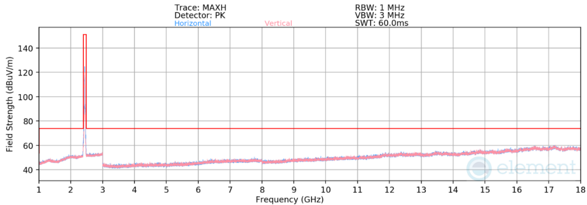
Plot 7-68. Radiated Spurious Emissions above 1GHz CDD (802.11ax OFDMA – RU26 – Ch. 6)
