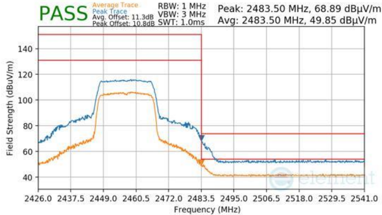
Plot 7-89 Radiated Restricted Upper Band Edge Measurement Antenna 3a (Peak & Average – RU242)
