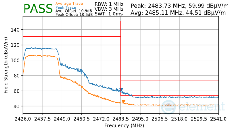
Plot 7-102 Radiated Restricted Upper Band Edge Measurement Antenna 1a (Peak & Average – RU242)
