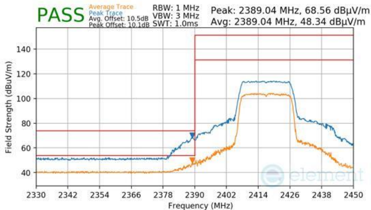
Plot 7-80 Radiated Restricted Lower Band Edge Measurement Antenna 3a (Peak & Average – RU242)
