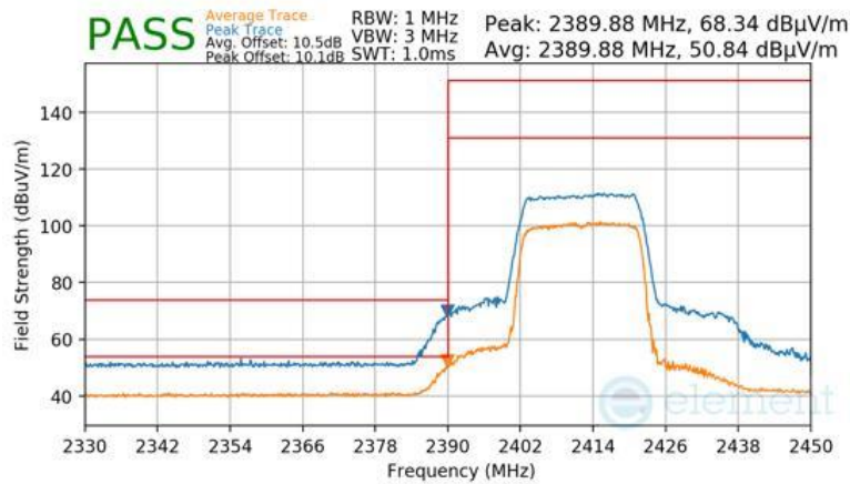
Plot 7-96 Radiated Restricted Lower Band Edge Measurement Antenna 1a (Peak & Average – RU242)
