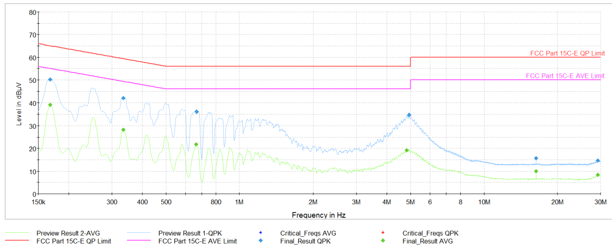
Plot 7-128. AC Line Conducted Emissions with 802.11ax (RU26) Ch.6 (L1, with AC/DC Adapter)
