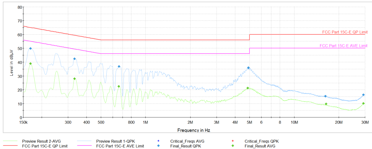
Plot 7-131. AC Line Conducted Emissions with 802.11ax (RU242) Ch.6 (N, with AC/DC Adapter)
