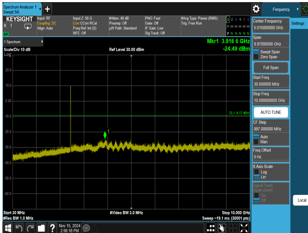
Plot 7-65. Conducted Spurious Plot Antenna 1a (802.11ax OFDMA – RU242 – Ch. 11)
