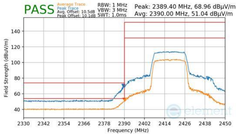
Plot 7-97 Radiated Restricted Lower Band Edge Measurement Antenna 1a (Peak & Average – RU242)
