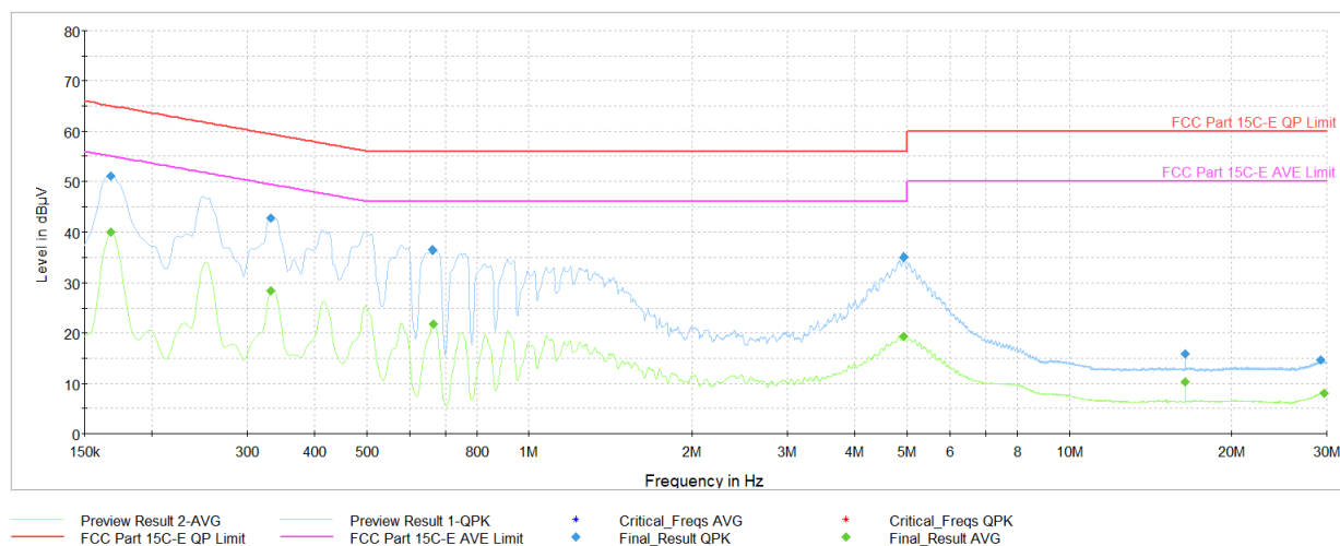
Plot 7-130. AC Line Conducted Emissions with 802.11ax (RU242) Ch.6 (L1, with AC/DC Adapter)
