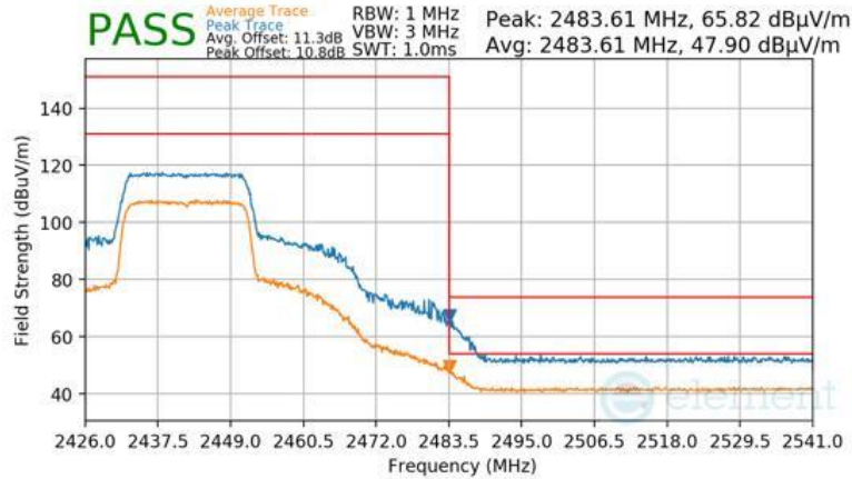
Plot 7-86 Radiated Restricted Upper Band Edge Measurement Antenna 3a (Peak & Average – RU242)
