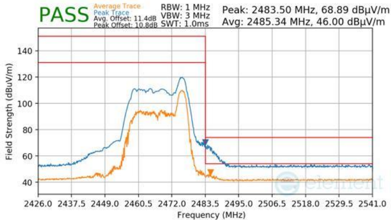
Plot 7-78 Radiated Restricted Upper Band Edge Measurement Antenna 3a (Peak & Average – RU26)
