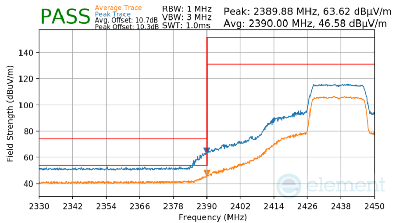
Plot 7-101 Radiated Restricted Lower Band Edge Measurement Antenna 1a (Peak & Average – RU242)
