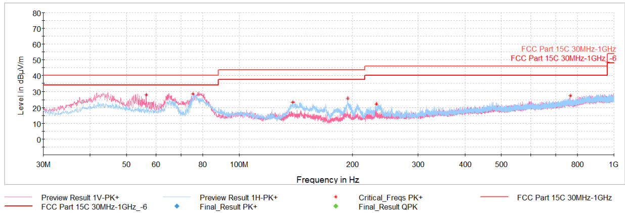
Plot 7-126. Radiated Spurious Emissions below 1GHz CDD Ch.6 (RU26), with AC/DC Adapter
