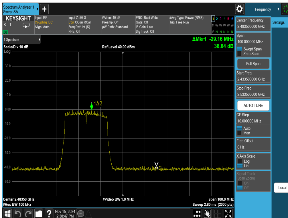
Plot 7-42. Band Edge Antenna 1a (802.11ax OFDMA – RU242 – Ch. 12)
