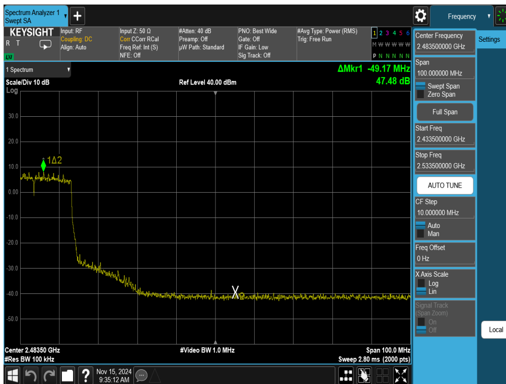
Plot 7-21. Band Edge Antenna 3a (802.11ax OFDMA – RU242 – Ch. 6(High Channel))
