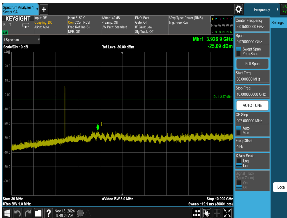
Plot 7-45. Conducted Spurious Plot Antenna 3a (802.11ax OFDMA – RU26 – Ch. 6)
