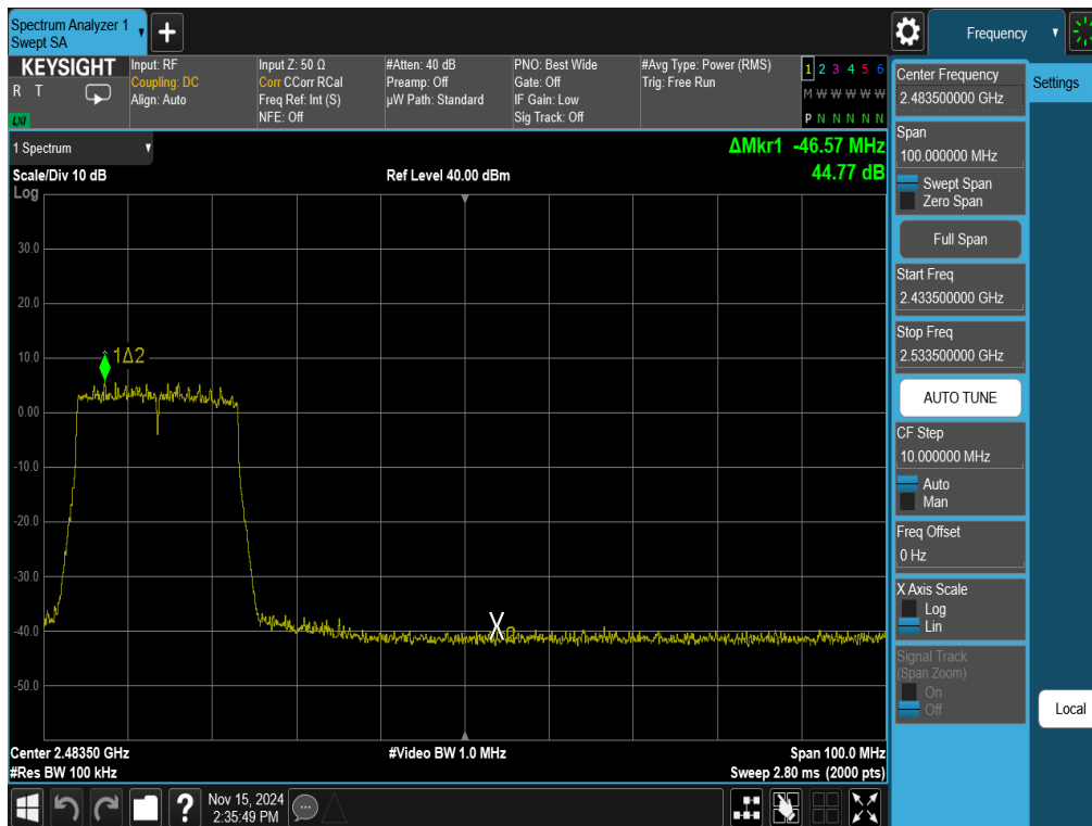
Plot 7-38. Band Edge Antenna 1a (802.11ax OFDMA – RU242 – Ch. 8)
