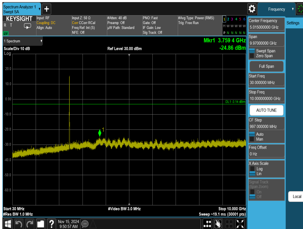
Plot 7-47. Conducted Spurious Plot Antenna 3a (802.11ax OFDMA – RU26 – Ch. 11)
