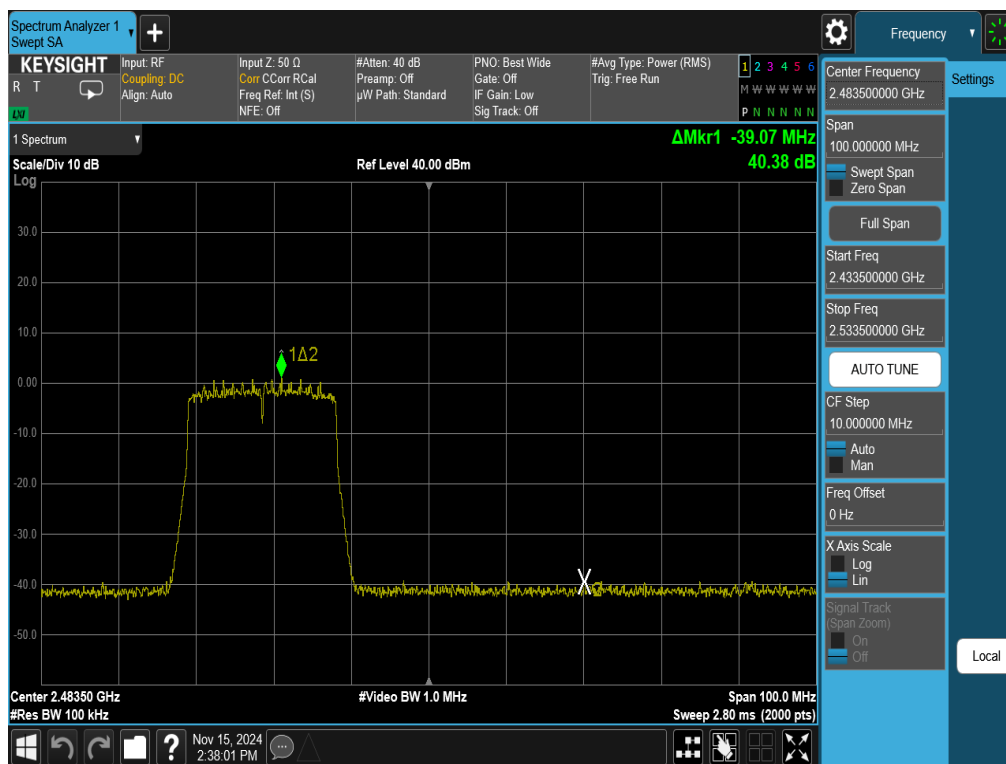
Plot 7-41. Band Edge Antenna 1a (802.11ax OFDMA – RU242 – Ch. 11)
