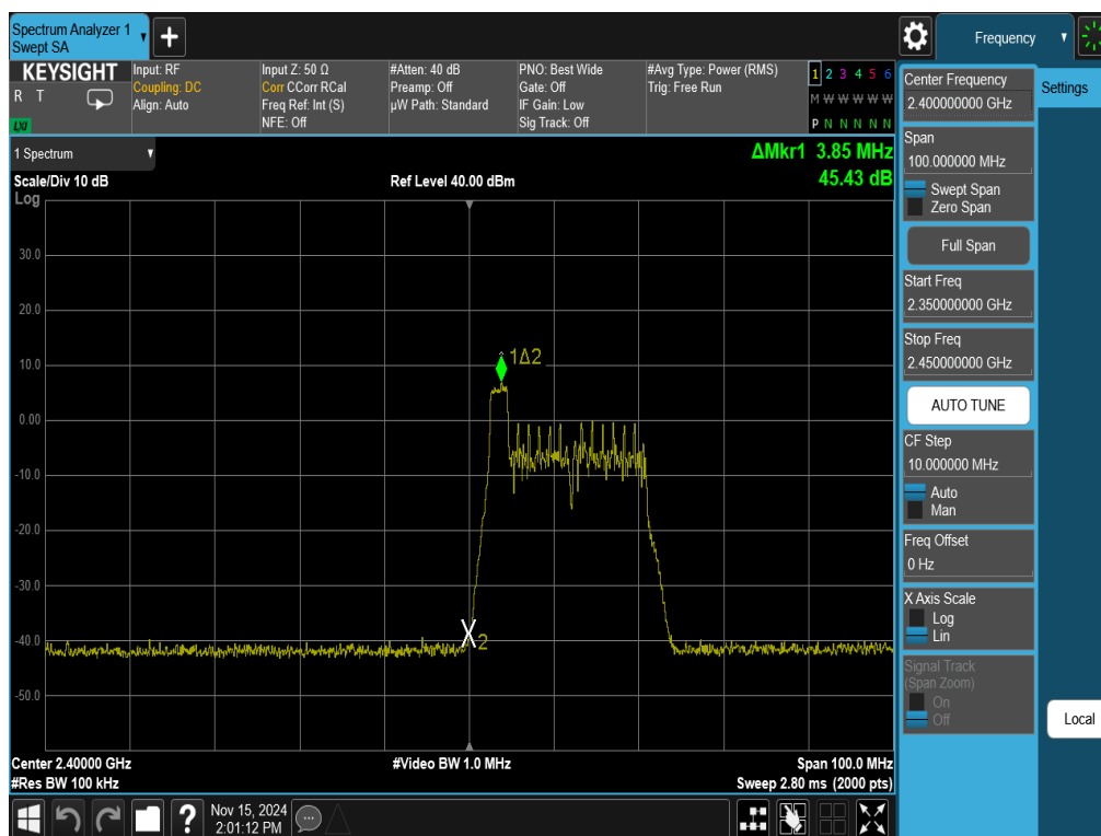
Plot 7-28. Band Edge Antenna 1a (802.11ax OFDMA – RU26 Index 0 – Ch. 1)
