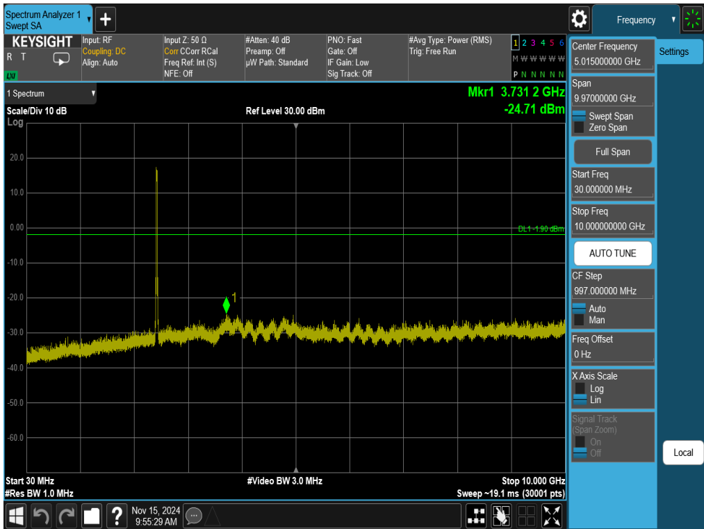
Plot 7-51. Conducted Spurious Plot Antenna 3a (802.11ax OFDMA – RU242 – Ch. 6)
