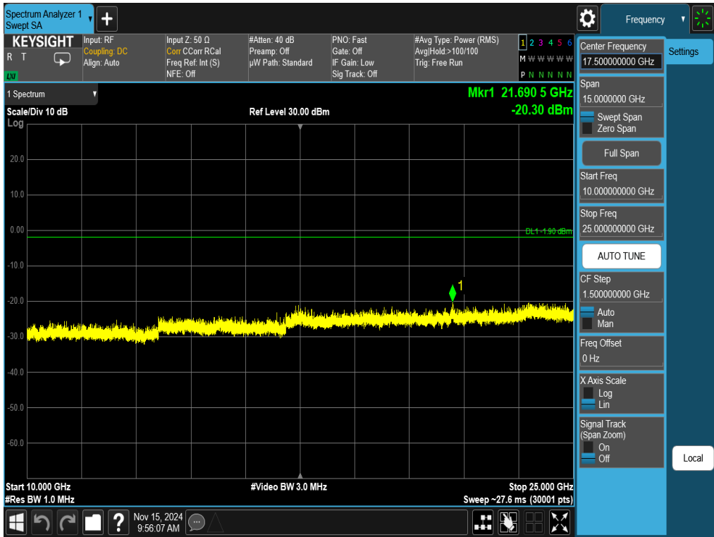
Plot 7-52. Conducted Spurious Plot Antenna 3a (802.11ax OFDMA – RU242 – Ch. 6)
