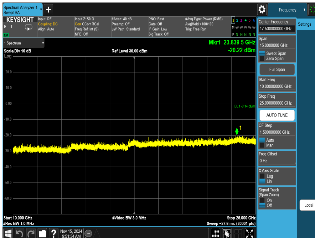
Plot 7-48. Conducted Spurious Plot Antenna 3a (802.11ax OFDMA – RU26 – Ch. 11)
