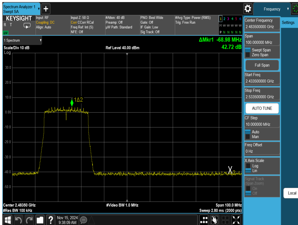
Plot 7-25. Band Edge Antenna 3a (802.11ax OFDMA – RU242 – Ch. 10)
