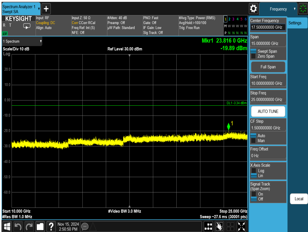
Plot 7-60. Conducted Spurious Plot Antenna 1a (802.11ax OFDMA – RU26 – Ch. 11)
