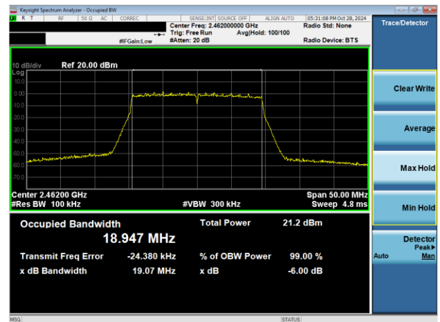
Plot 7-2. 6dB BW & 99% OBW Plot Antenna 3a (802.11ax OFDMA – RU242 – Ch. 11)
