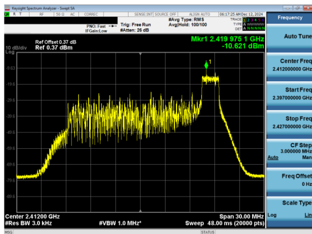
Plot 7-7. Power Spectral Density Plot Antenna 1a (802.11ax OFDMA – RU26 Index 8 – Ch. 1)
