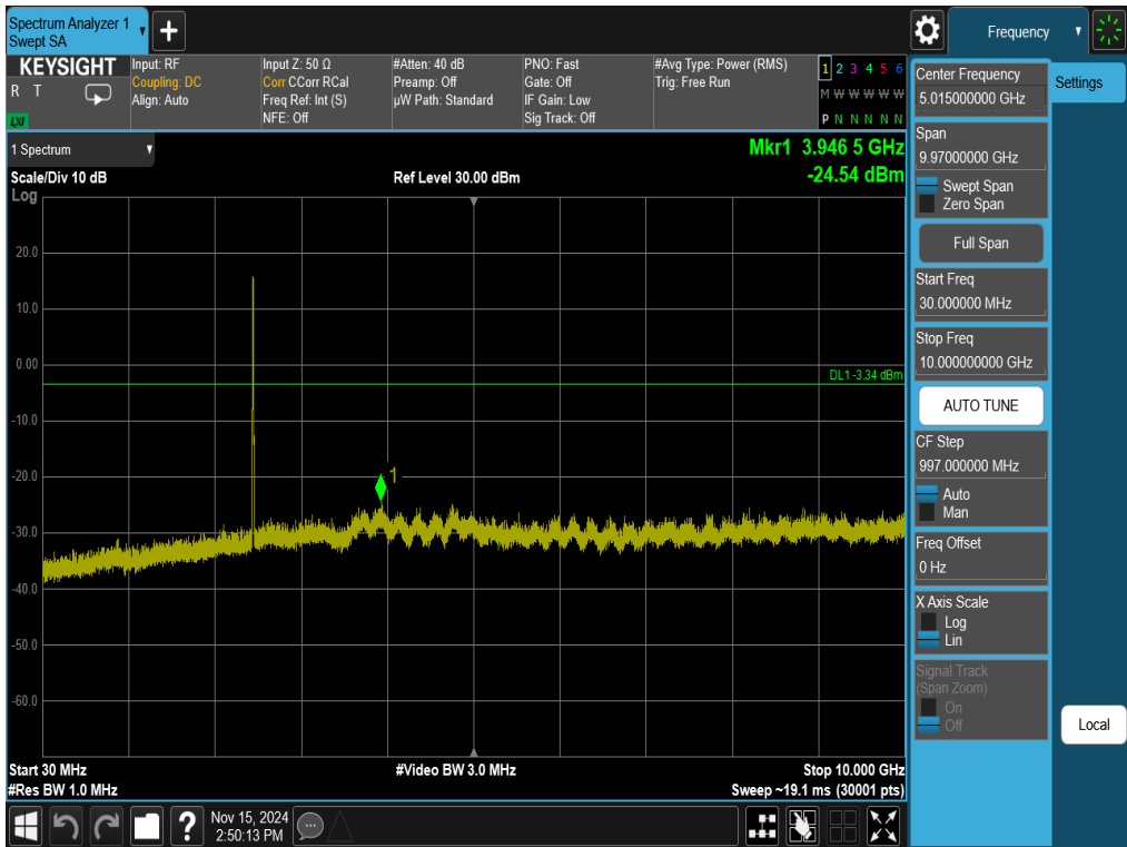
Plot 7-59. Conducted Spurious Plot Antenna 1a (802.11ax OFDMA – RU26 – Ch. 11)
