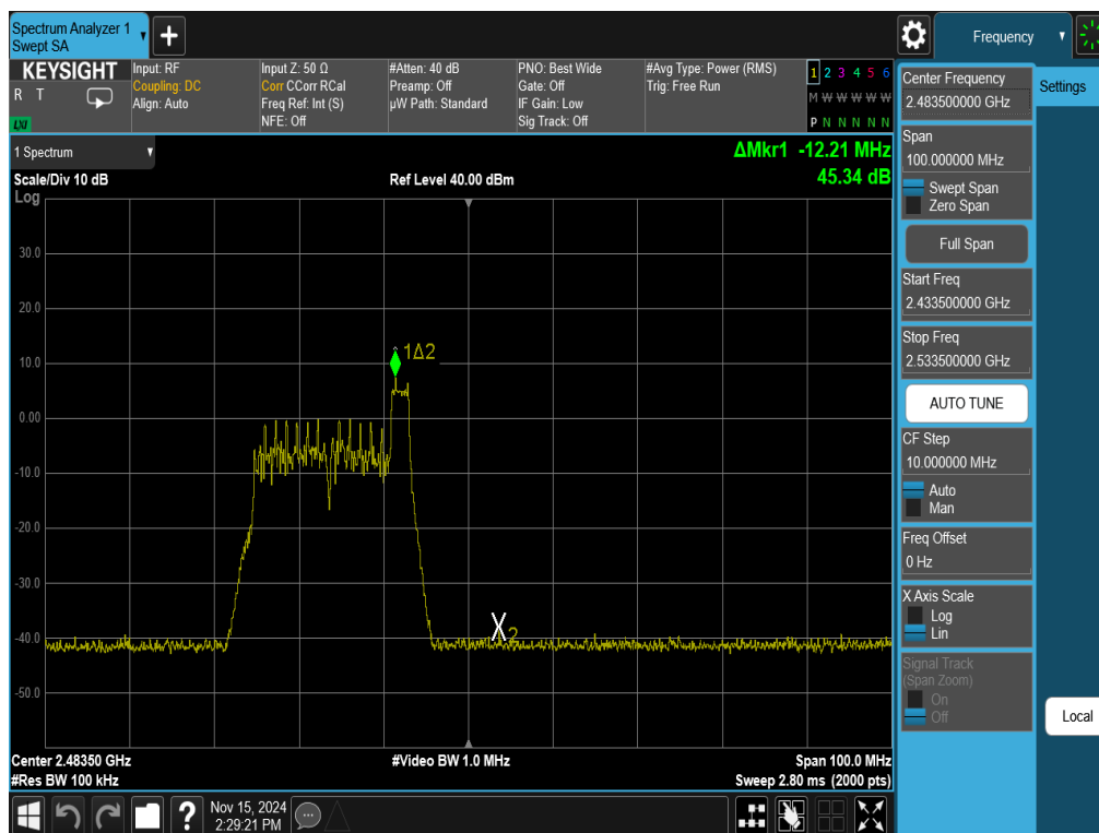
Plot 7-29. Band Edge Antenna 1a (802.11ax OFDMA – RU26 Index 8 – Ch. 12)
