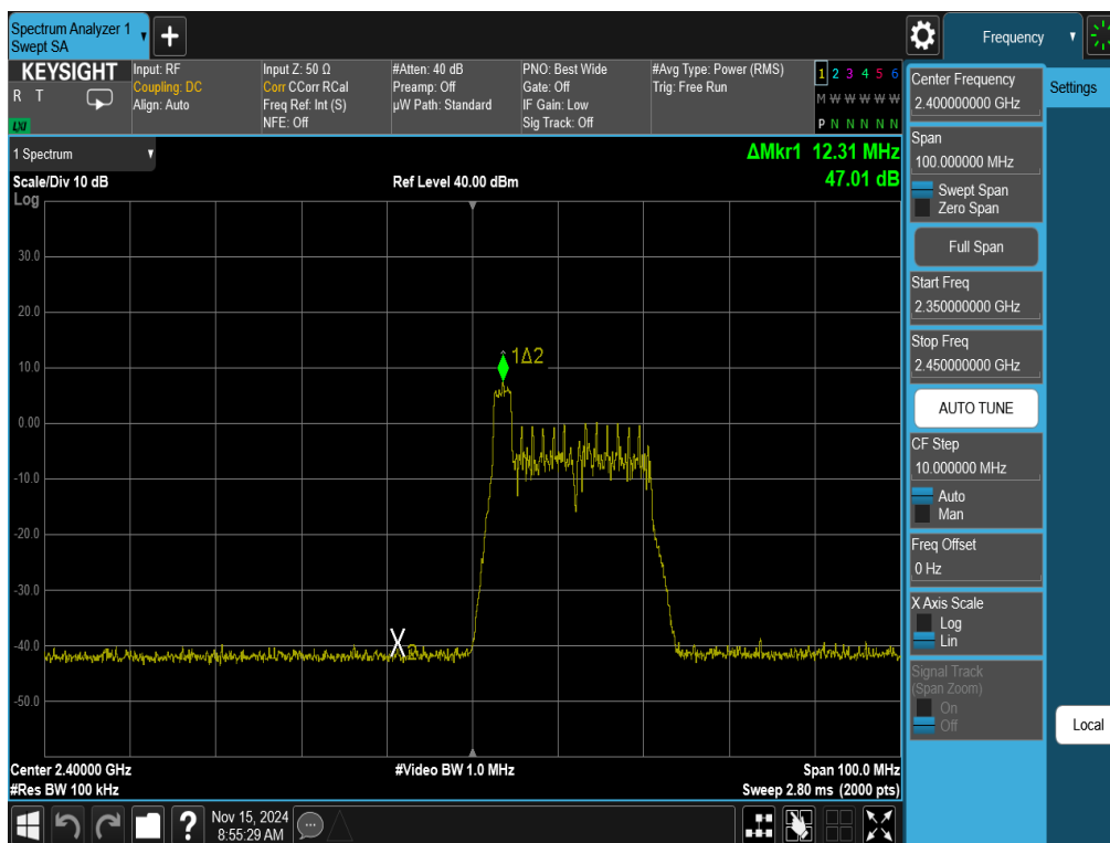
Plot 7-13. Band Edge Antenna 3a (802.11ax OFDMA – RU26 Index 0 – Ch. 1)
