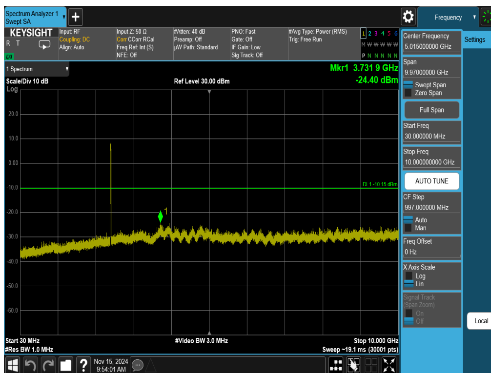
Plot 7-49. Conducted Spurious Plot Antenna 3a (802.11ax OFDMA – RU242 – Ch. 1)
