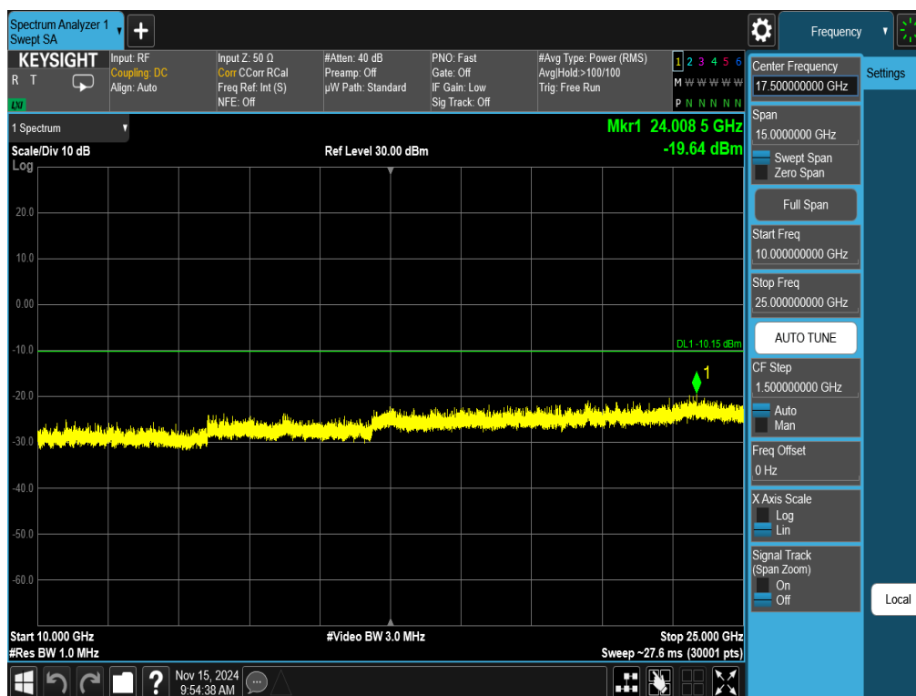
Plot 7-50. Conducted Spurious Plot Antenna 3a (802.11ax OFDMA – RU242 – Ch. 1)
