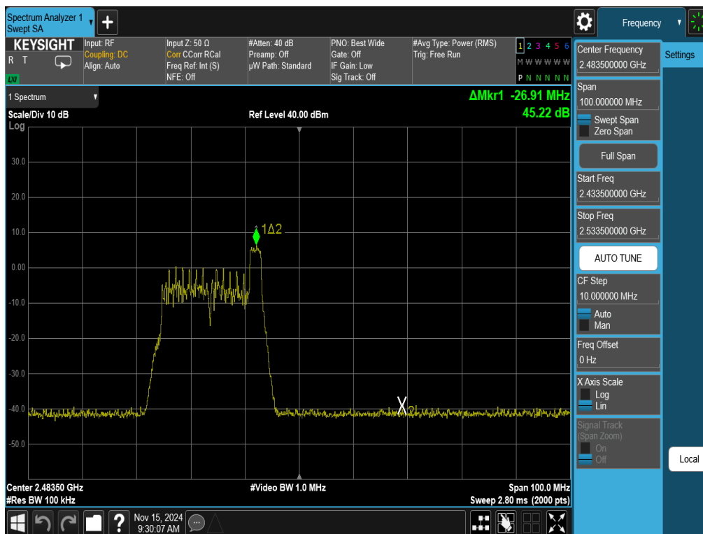
Plot 7-14. Band Edge Antenna 3a (802.11ax OFDMA – RU26 Index 8 – Ch. 12)
