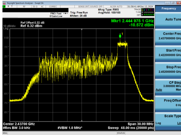
Plot 7-9. Power Spectral Density Plot Antenna 3a (802.11ax OFDMA – RU26 Index 8 – Ch. 6)
