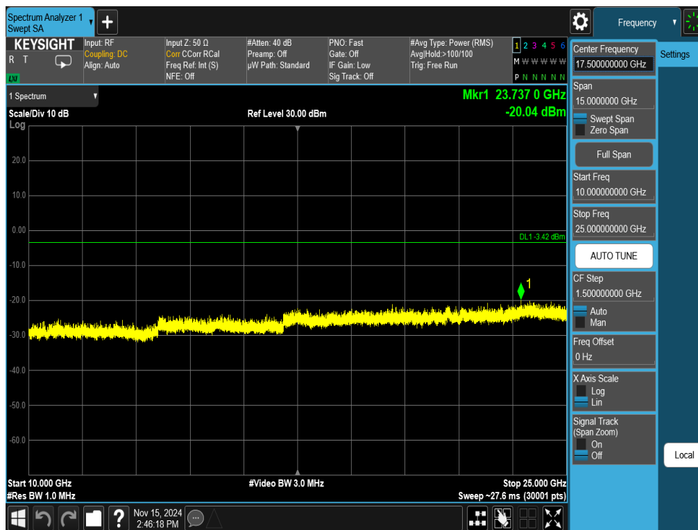
Plot 7-58. Conducted Spurious Plot Antenna 1a (802.11ax OFDMA – RU26 – Ch. 6)
