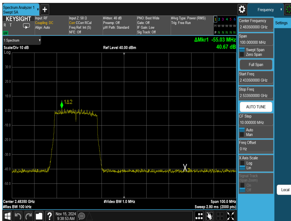
Plot 7-26. Band Edge Antenna 3a (802.11ax OFDMA – RU242 – Ch. 11)
