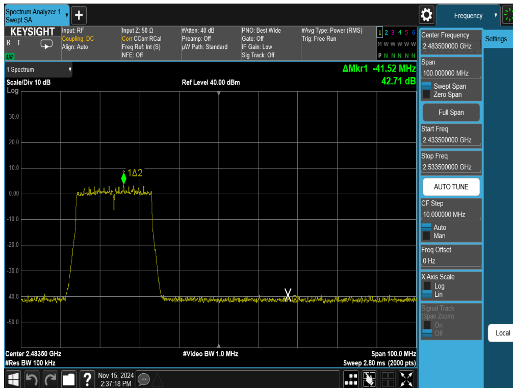
Plot 7-40. Band Edge Antenna 1a (802.11ax OFDMA – RU242 – Ch. 10)
