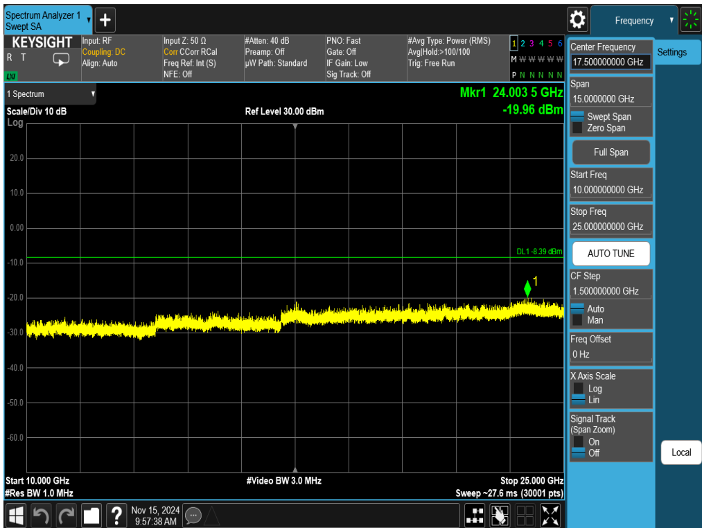
Plot 7-54. Conducted Spurious Plot Antenna 3a (802.11ax OFDMA – RU242 – Ch. 11)
