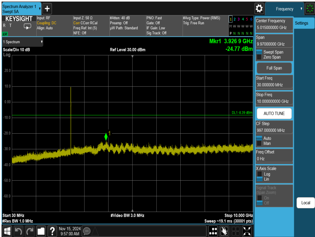
Plot 7-53. Conducted Spurious Plot Antenna 3a (802.11ax OFDMA – RU242 – Ch. 11)
