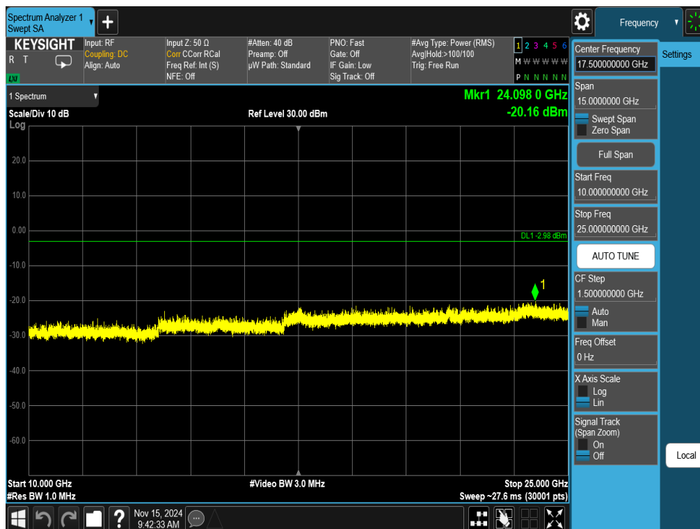
Plot 7-44. Conducted Spurious Plot Antenna 3a (802.11ax OFDMA – RU26 – Ch. 1)
