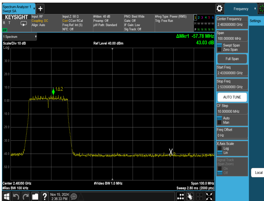
Plot 7-39. Band Edge Antenna 1a (802.11ax OFDMA – RU242 – Ch. 9)
