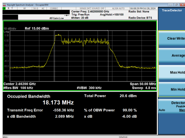
Plot 7-3. 6dB BW & 99% OBW Antenna 1a (802.11ax OFDMA – RU26 Index 0 – Ch. 11)
