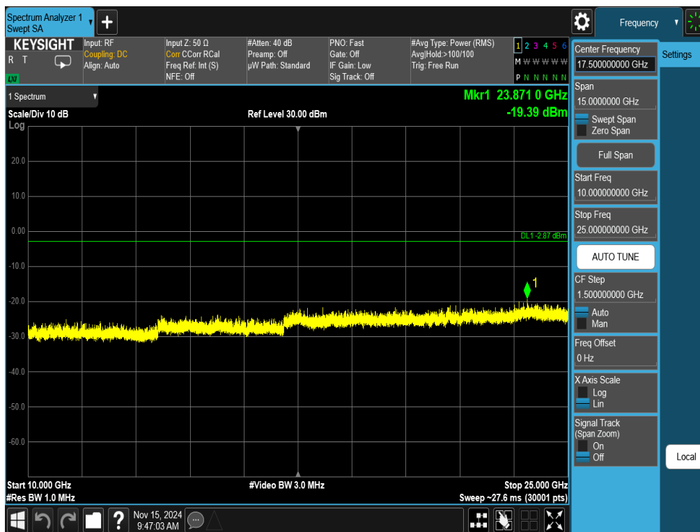
Plot 7-46. Conducted Spurious Plot Antenna 3a (802.11ax OFDMA – RU26 – Ch. 6)
