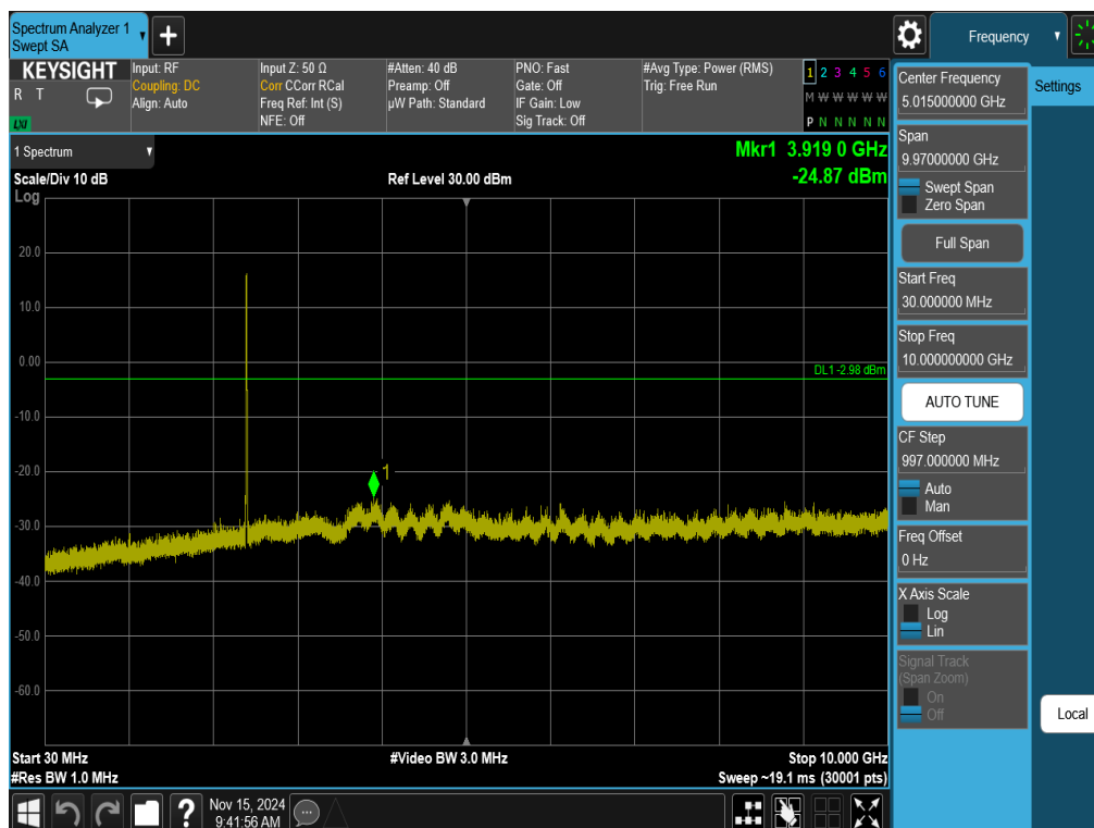
Plot 7-43. Conducted Spurious Plot Antenna 3a (802.11ax OFDMA – RU26 – Ch. 1)
