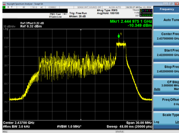
Plot 7-10. Power Spectral Density Plot Antenna 1a (802.11ax OFDMA – RU26 Index 8 – Ch. 6)
