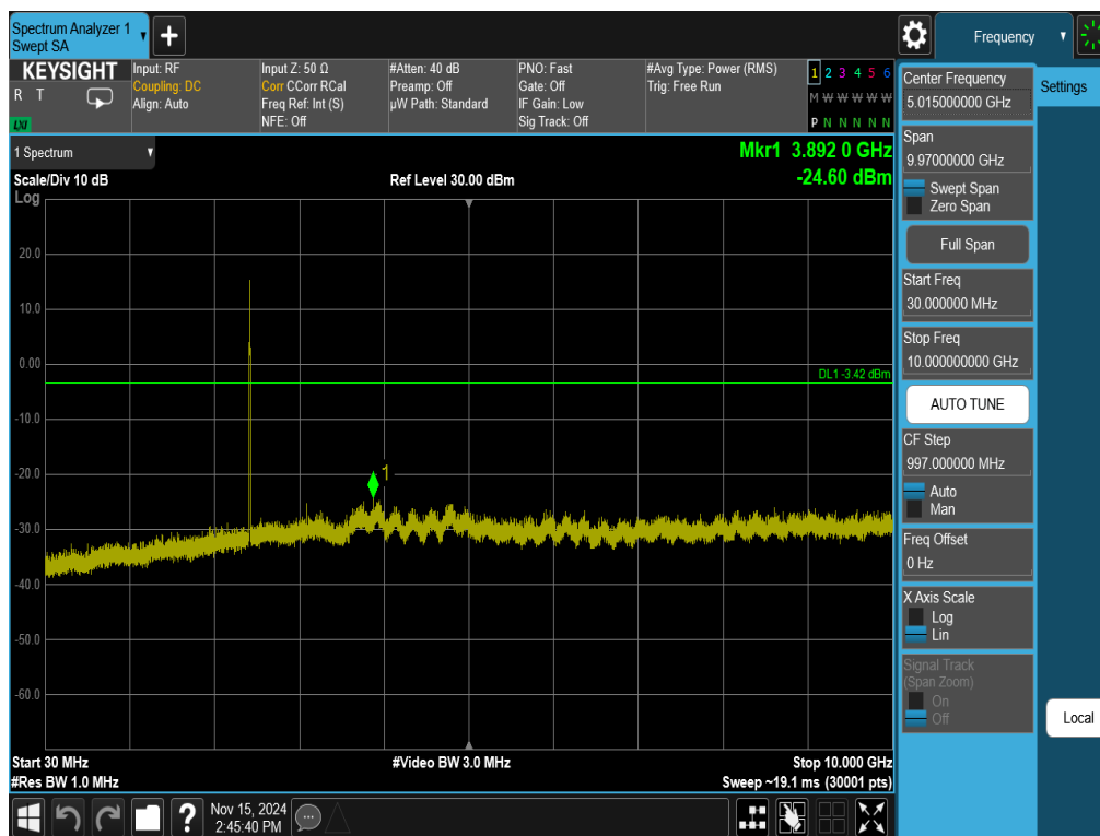
Plot 7-57. Conducted Spurious Plot Antenna 1a (802.11ax OFDMA – RU26 – Ch. 6)
