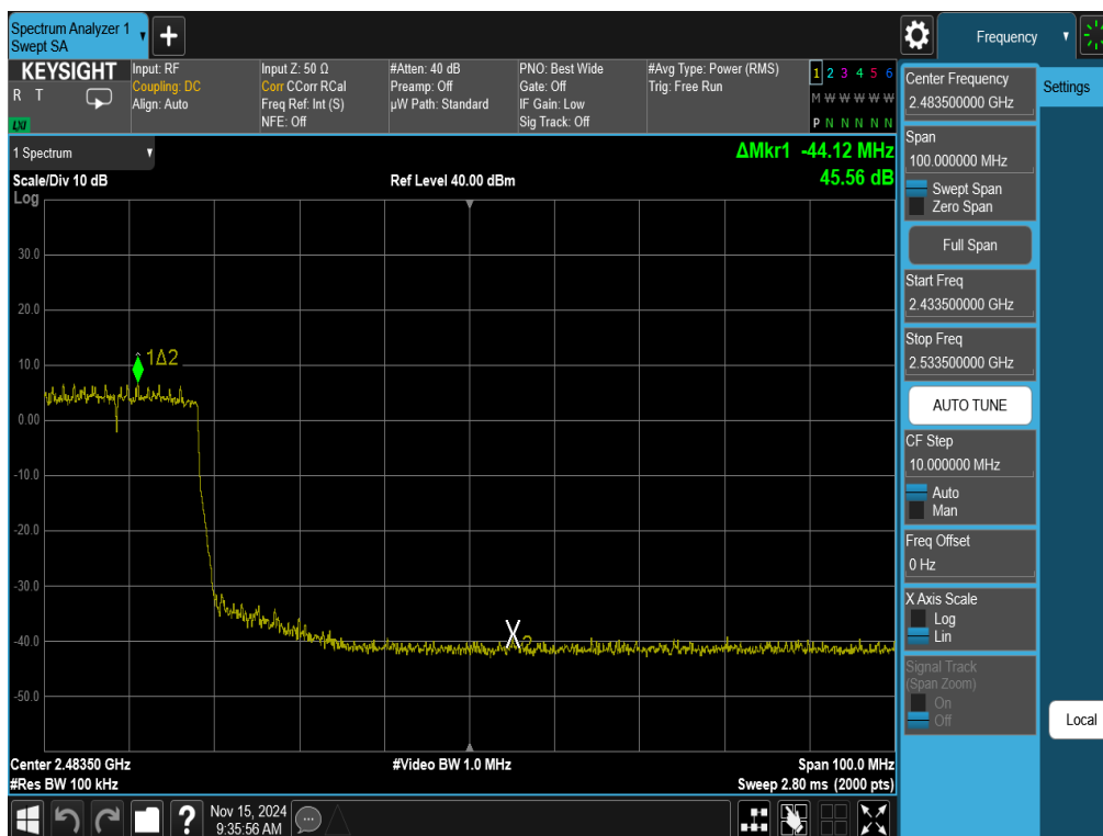
Plot 7-22. Band Edge Antenna 3a (802.11ax OFDMA – RU242 – Ch. 7)
