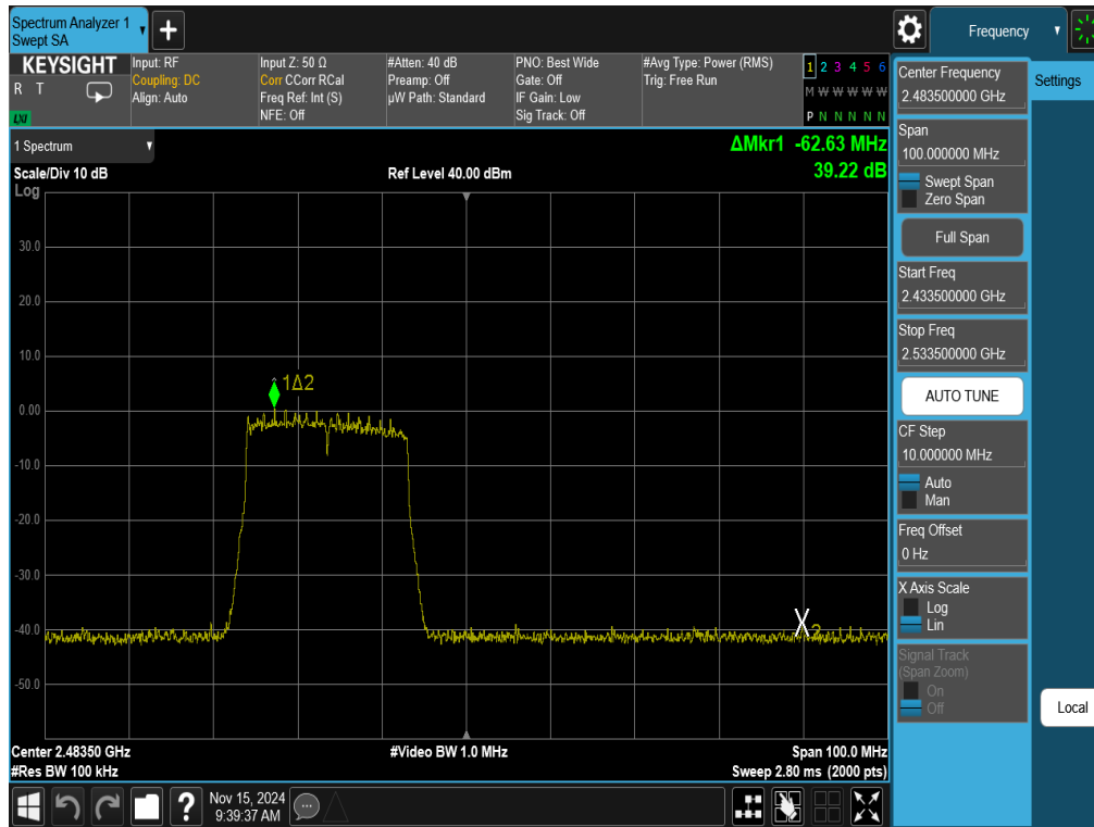
Plot 7-27. Band Edge Antenna 3a (802.11ax OFDMA – RU242 – Ch. 12)
