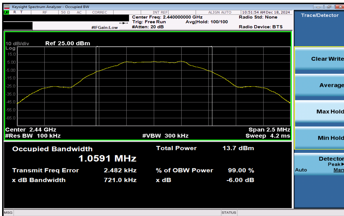
Plot 7-8. 6dB BW & 99% OBW Plot Antenna 1a (Bluetooth (LE), 1Mbps, ePA – Ch. 19)
