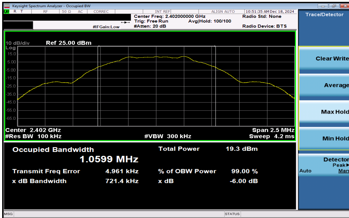
Plot 7-7. 6dB BW & 99% OBW Plot Antenna 1a (Bluetooth (LE), 1Mbps, ePA – Ch. 0)
