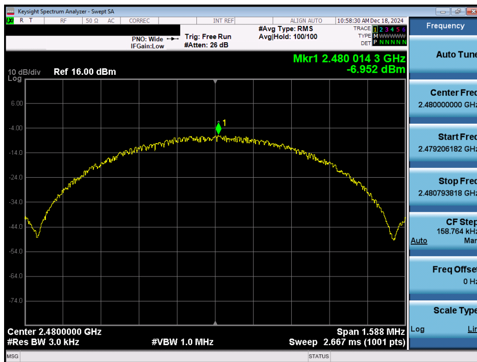
Plot 7-30. Power Spectral Density Plot Antenna 1a (Bluetooth (LE), 1Mbps, iPA – Ch. 39)
