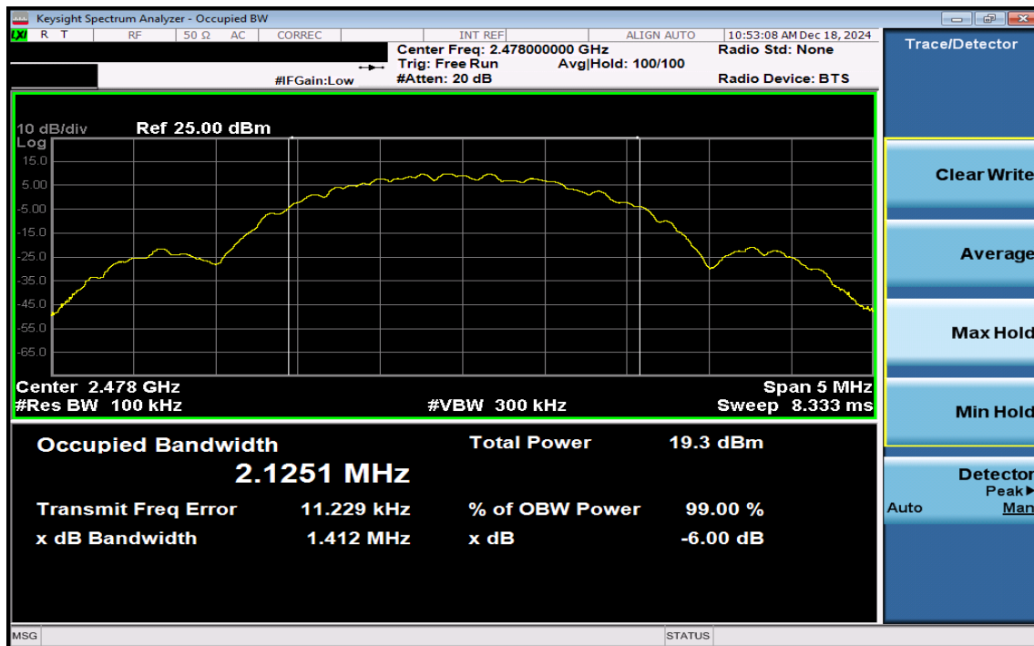
Plot 7-12. 6dB BW & 99% OBW Plot Antenna 1a (Bluetooth (LE), 2Mbps, ePA – Ch. 38)
