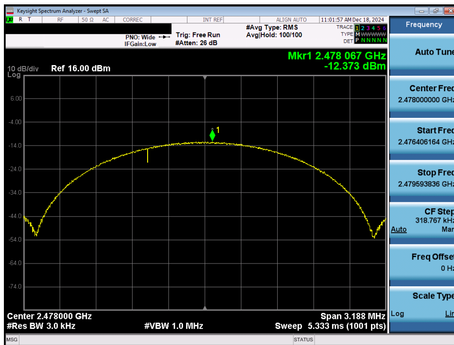
Plot 7-36. Power Spectral Density Plot Antenna 1a (Bluetooth (LE), 2Mbps, iPA – Ch. 38)
