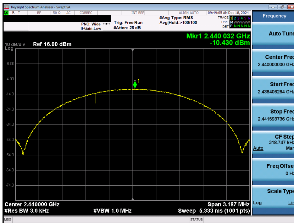
Plot 7-20. Power Spectral Density Plot Antenna 3a (Bluetooth (LE), 2Mbps, ePA – Ch. 19)
