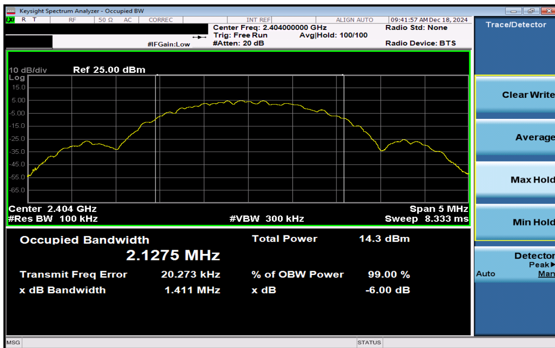
Plot 7-4. 6dB BW & 99% OBW Plot Antenna 3a (Bluetooth (LE), 2Mbps, ePA – Ch. 1)
