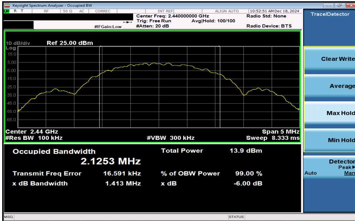
Plot 7-11. 6dB BW & 99% OBW Plot Antenna 1a (Bluetooth (LE), 2Mbps, ePA – Ch. 19)
