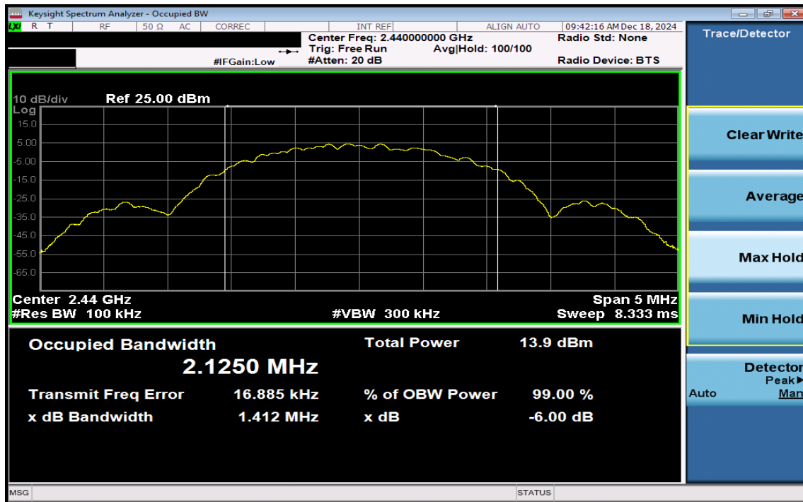
Plot 7-5. 6dB BW & 99% OBW Plot Antenna 3a (Bluetooth (LE), 2Mbps, ePA – Ch. 19)
