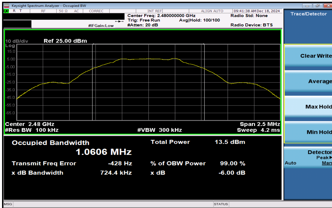
Plot 7-3. 6dB BW & 99% OBW Plot Antenna 3a (Bluetooth (LE), 1Mbps, ePA – Ch. 39)
