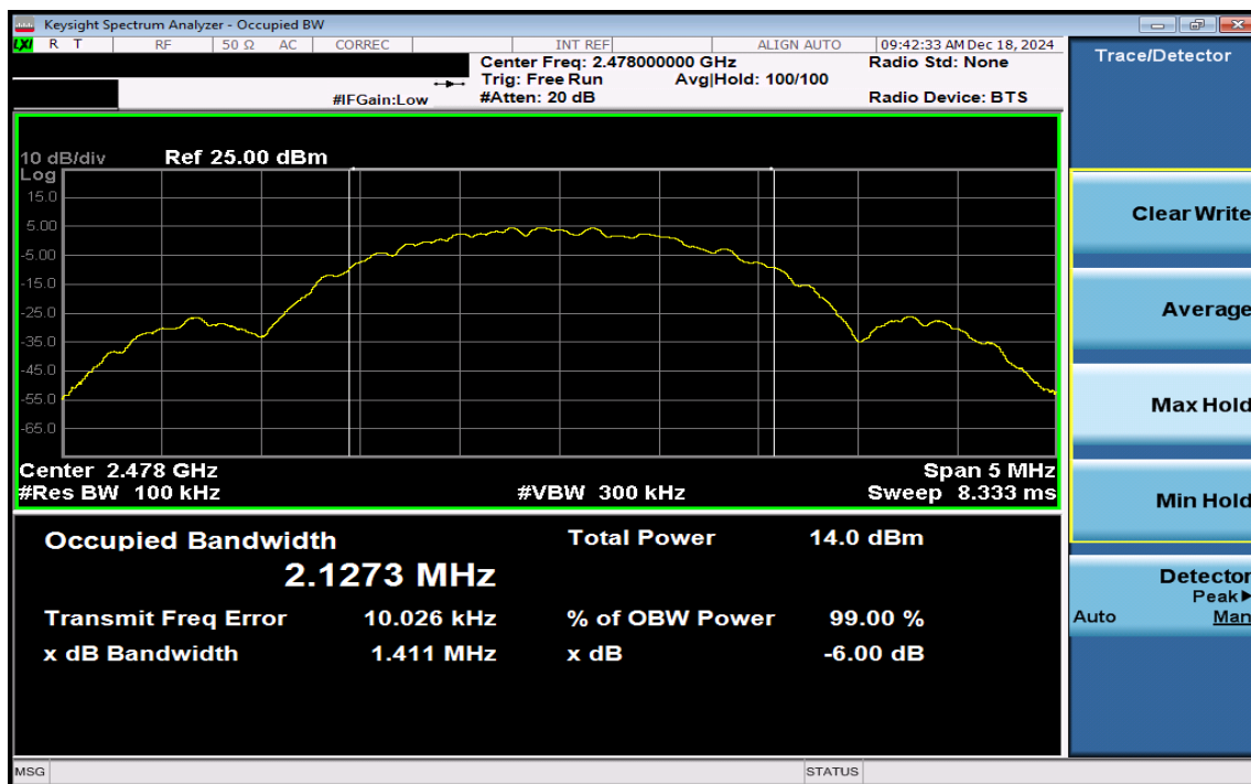
Plot 7-6. 6dB BW & 99% OBW Plot Antenna 3a (Bluetooth (LE), 2Mbps, ePA – Ch. 38)
