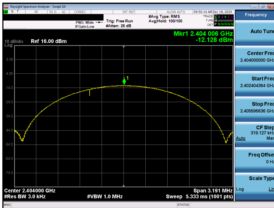
Plot 7-22. Power Spectral Density Plot Antenna 3a (Bluetooth (LE), 2Mbps, iPA – Ch. 1)
