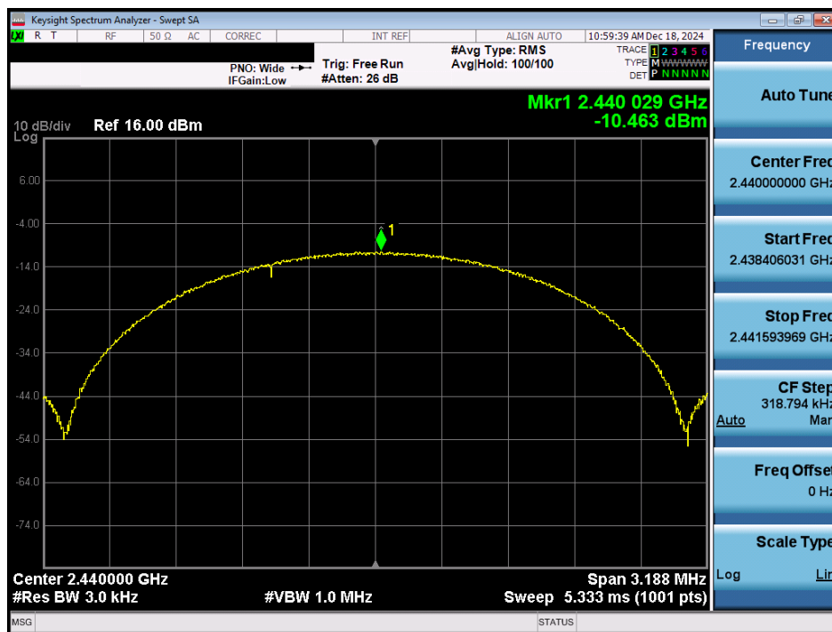
Plot 7-32. Power Spectral Density Plot Antenna 1a (Bluetooth (LE), 2Mbps, ePA – Ch. 19)
