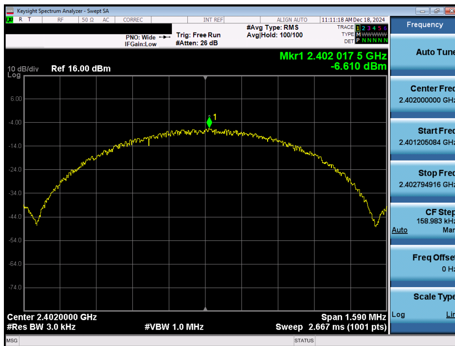
Plot 7-44. Power Spectral Density Plot Antenna 1a (Bluetooth (LE), 1Mbps, iPA – Ch. 0)
