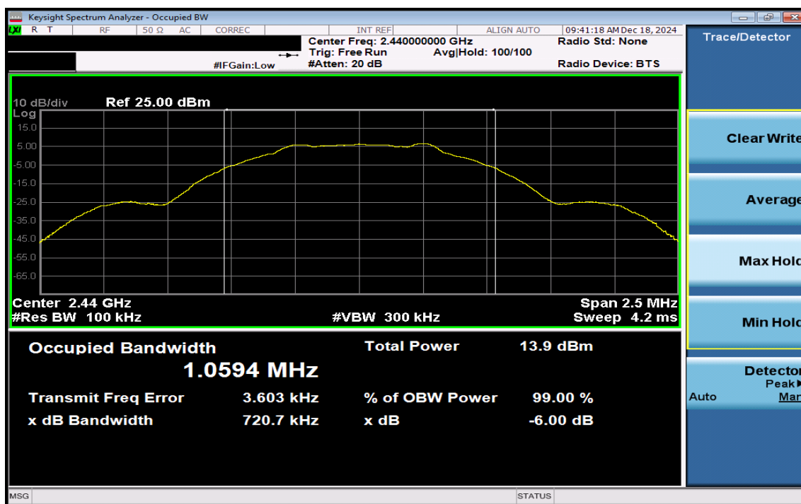
Plot 7-2. 6dB BW & 99% OBW Plot Antenna 3a (Bluetooth (LE), 1Mbps, ePA – Ch. 19)
