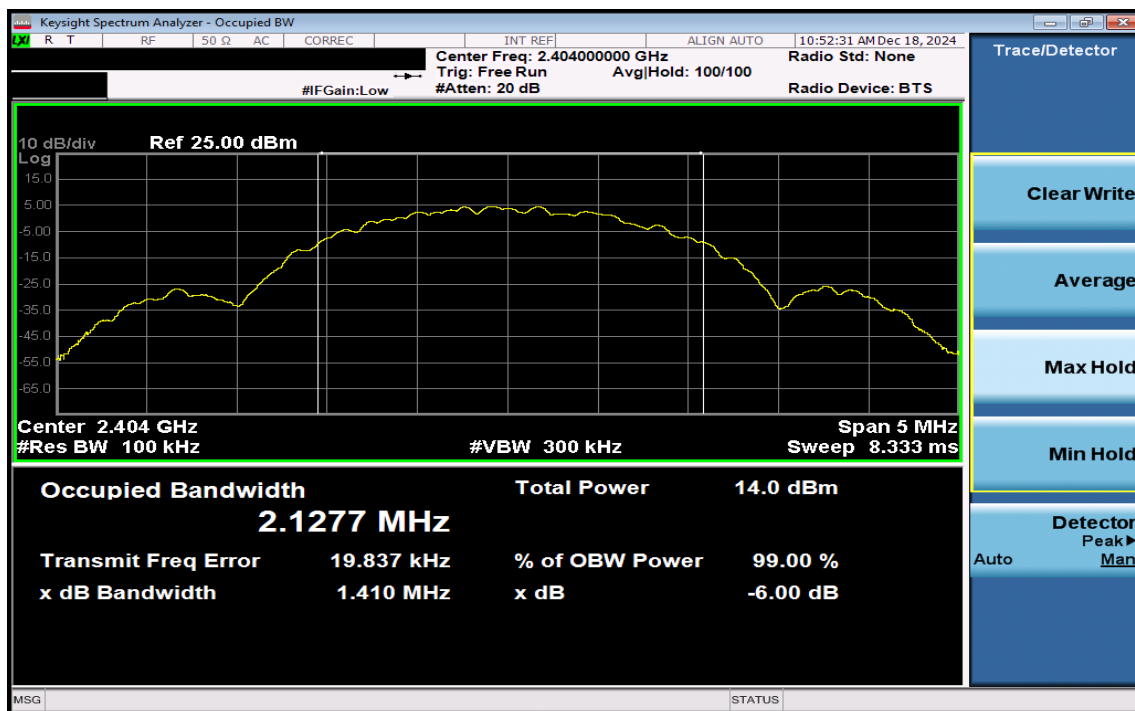
Plot 7-10. 6dB BW & 99% OBW Plot Antenna 1a (Bluetooth (LE), 2Mbps, ePA – Ch. 1)
