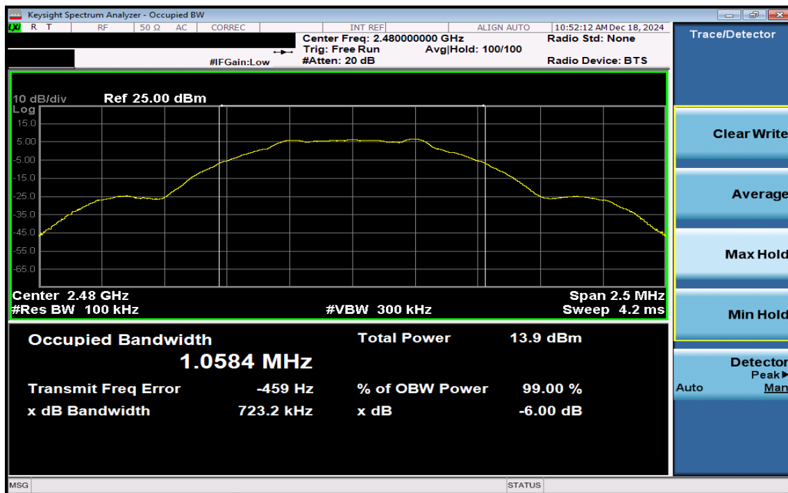
Plot 7-9. 6dB BW & 99% OBW Plot Antenna 1a (Bluetooth (LE), 1Mbps, ePA – Ch. 39)
