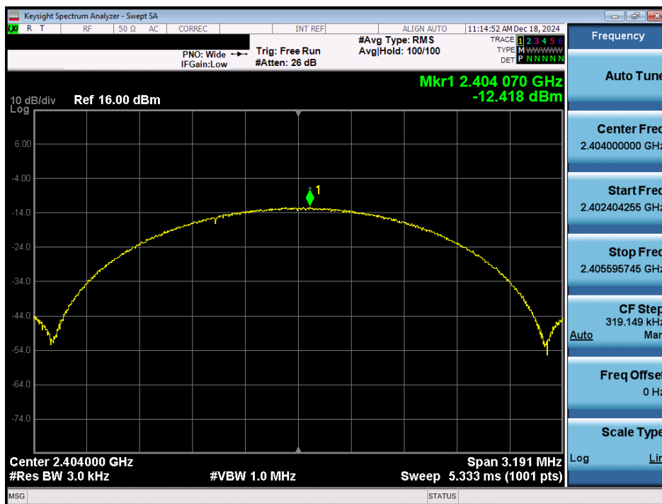
Plot 7-56. Power Spectral Density Plot Antenna 1a (Bluetooth (LE), 2Mbps, iPA – Ch. 1)
