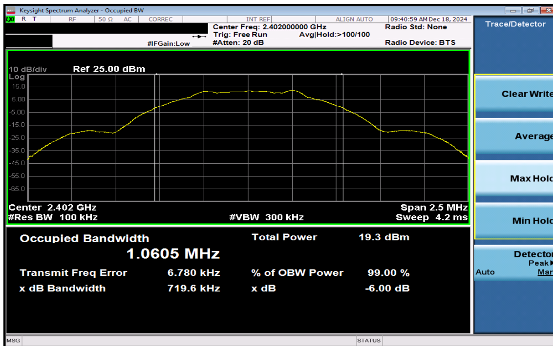
Plot 7-1. 6dB BW & 99% OBW Plot Antenna 3a (Bluetooth (LE), 1Mbps, ePA – Ch. 0)
