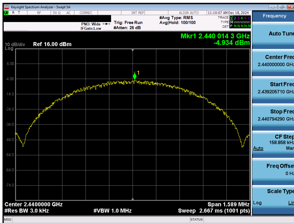
Plot 7-40. Power Spectral Density Plot Antenna 1a (Bluetooth (LE), 1Mbps, ePA – Ch. 19)
