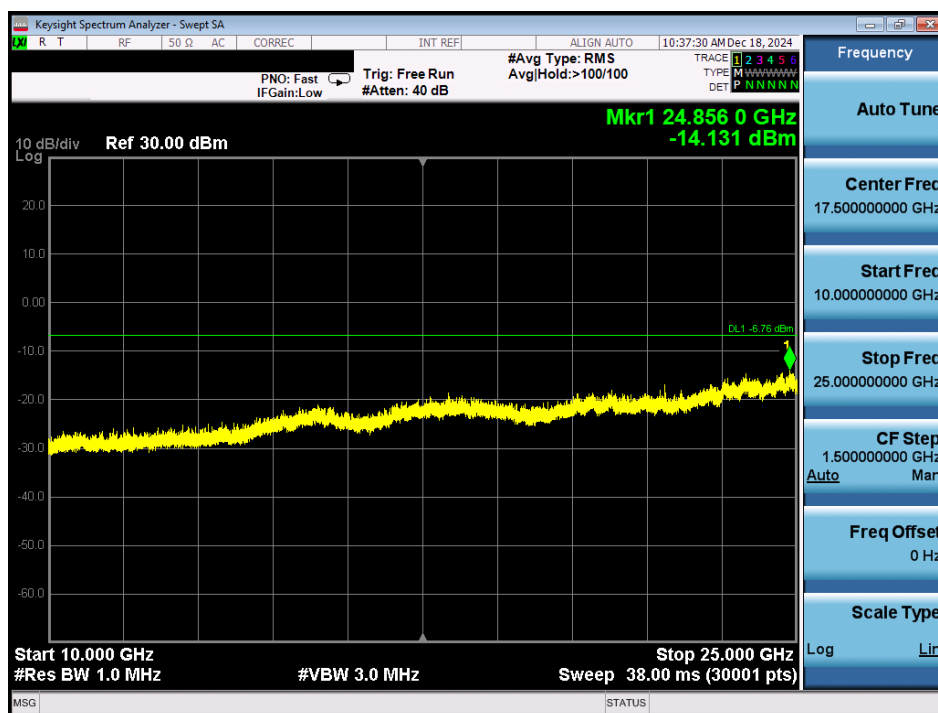
Plot 7-72. Conducted Spurious Plot Antenna 3a (Bluetooth (HDR4), 4 Mbps, ePA – Ch. 38)
