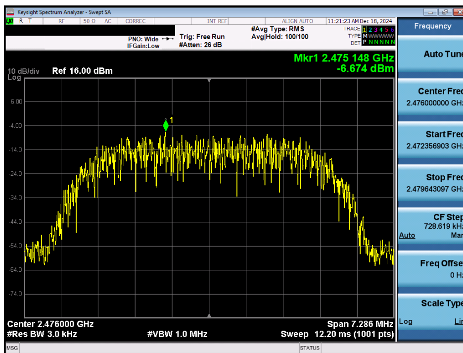
Plot 7-54. Power Spectral Density Plot TxBF Antenna 1a (Bluetooth (HDR8), 8Mbps, ePA – Ch. 73)
