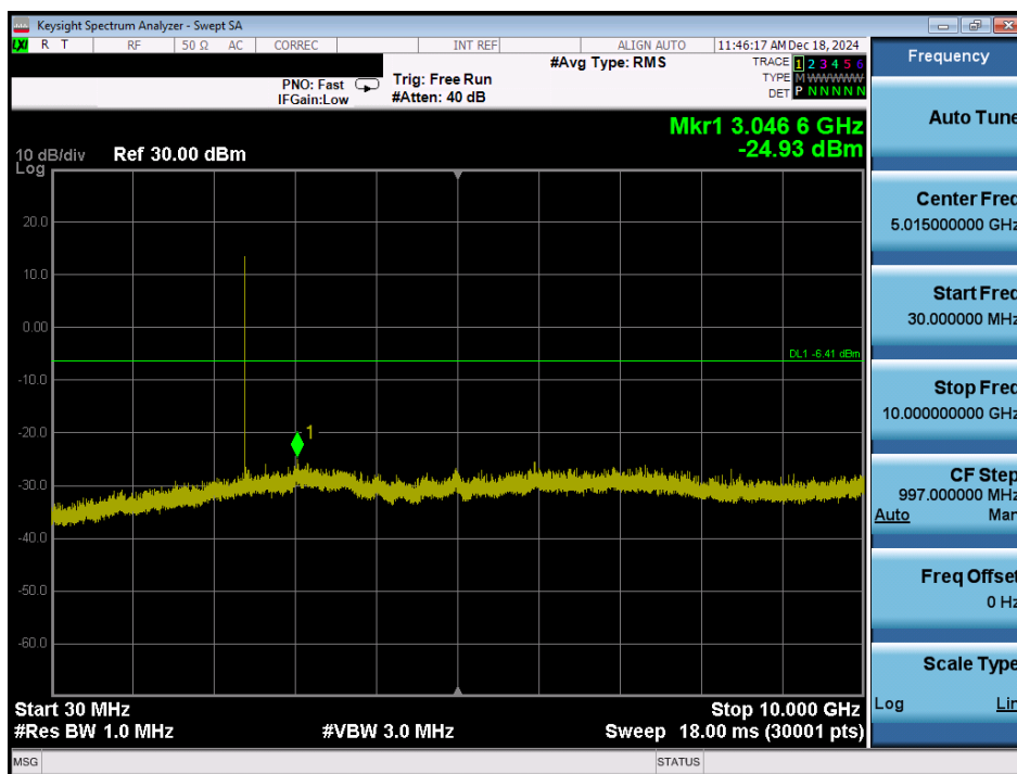
Plot 7-75. Conducted Spurious Plot Antenna 1a (Bluetooth (HDR4), 4 Mbps, ePA – Ch. 1)
