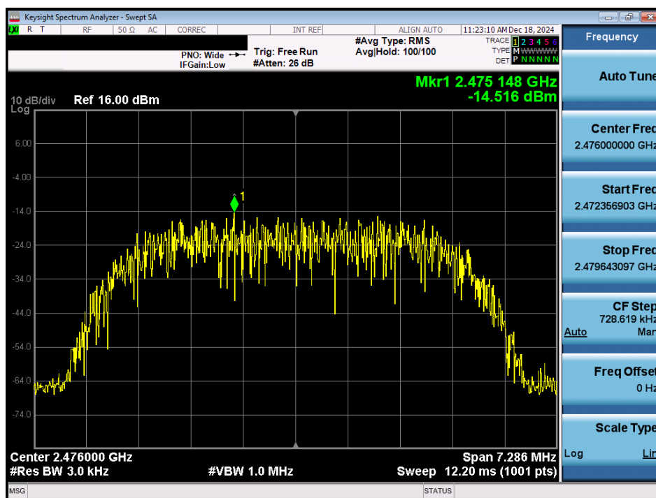
Plot 7-60. Power Spectral Density Plot TxBF Antenna 1a (Bluetooth (HDR8), 8Mbps, iPA – Ch. 73)
