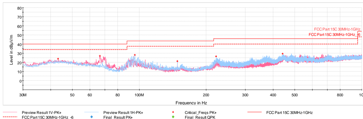
Plot 7-97. Radiated Spurious Emissions Below 1GHz TxBF (4Mbps, ePA – Ch.38 with AC/DC Adapter)
