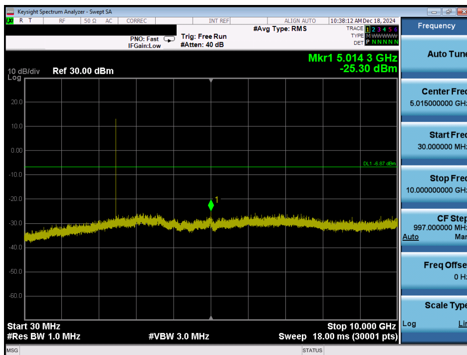
Plot 7-73. Conducted Spurious Plot Antenna 3a (Bluetooth (HDR4), 4 Mbps, ePA – Ch. 73)
