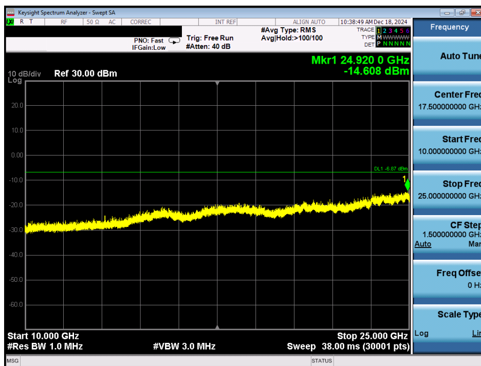
Plot 7-74. Conducted Spurious Plot Antenna 3a (Bluetooth (HDR4), 4 Mbps, ePA – Ch. 73)
