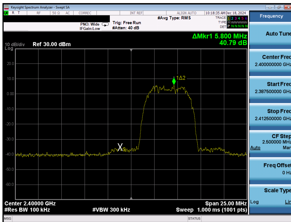
Plot 7-63. Band Edge Plot Antenna 3a (Bluetooth (HDR8), ePA – Ch. 1)
