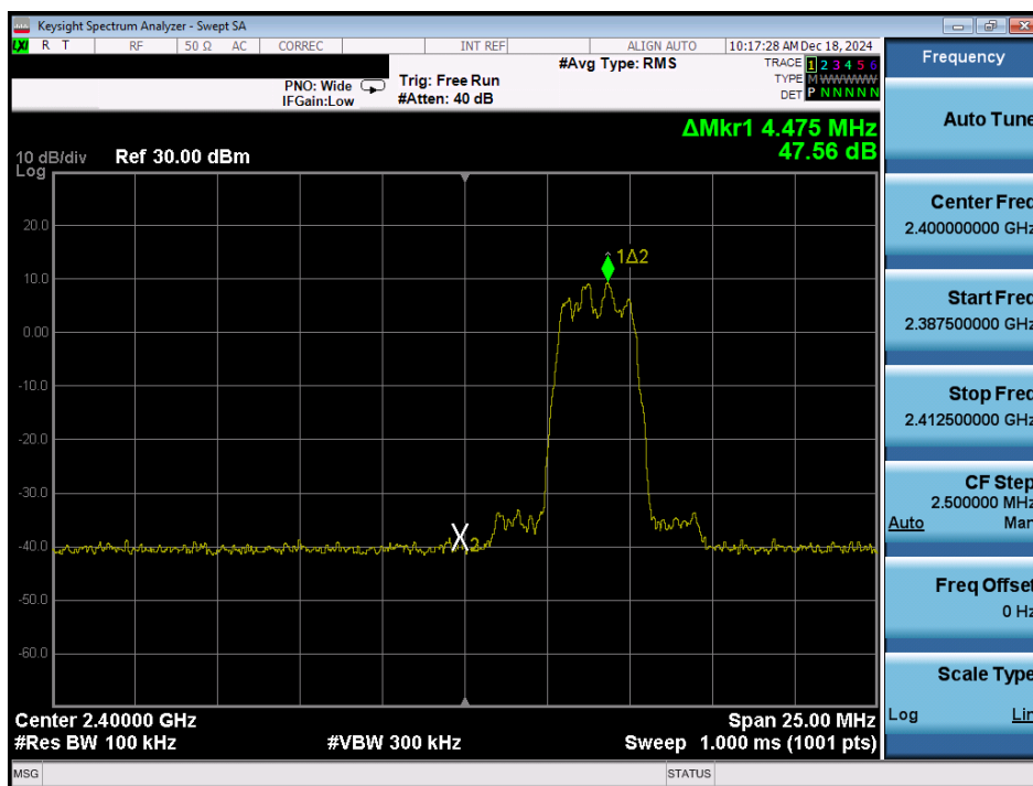
Plot 7-61. Band Edge Plot Antenna 3a (Bluetooth (HDR4), ePA – Ch. 1)
