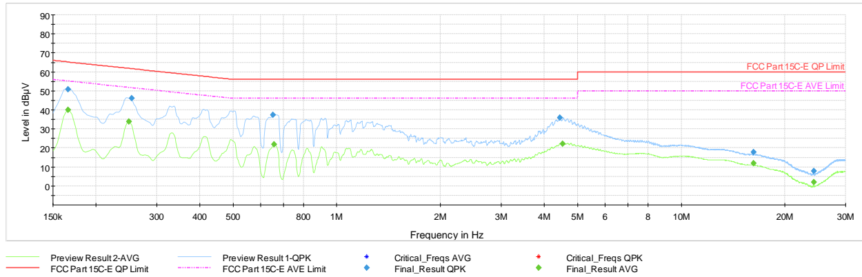
Plot 7-99. AC Line Conducted Plot with Bluetooth HDR (N, 4Mbps ePA - Ch.38 with AC/DC Adapter)
