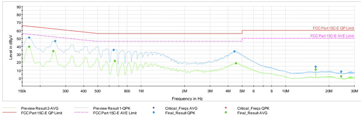
Plot 7-98. AC Line Conducted Plot with Bluetooth HDR Tx BF (L1, 4Mbps ePA - Ch.38 with AC/DC Adapter)
