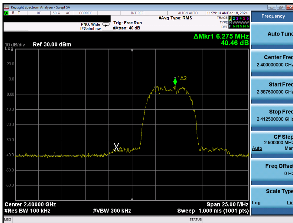
Plot 7-67. Band Edge Plot Antenna 1a (Bluetooth (HDR8), ePA – Ch. 1)
