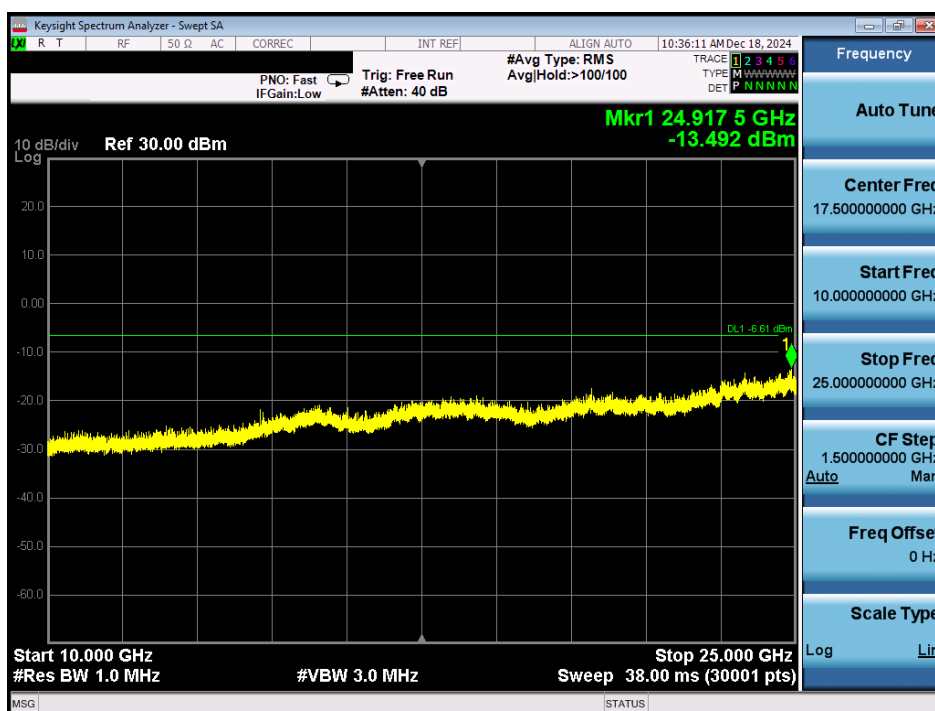
Plot 7-70. Conducted Spurious Plot Antenna 3a (Bluetooth (HDR4), 4 Mbps, ePA – Ch. 1)
