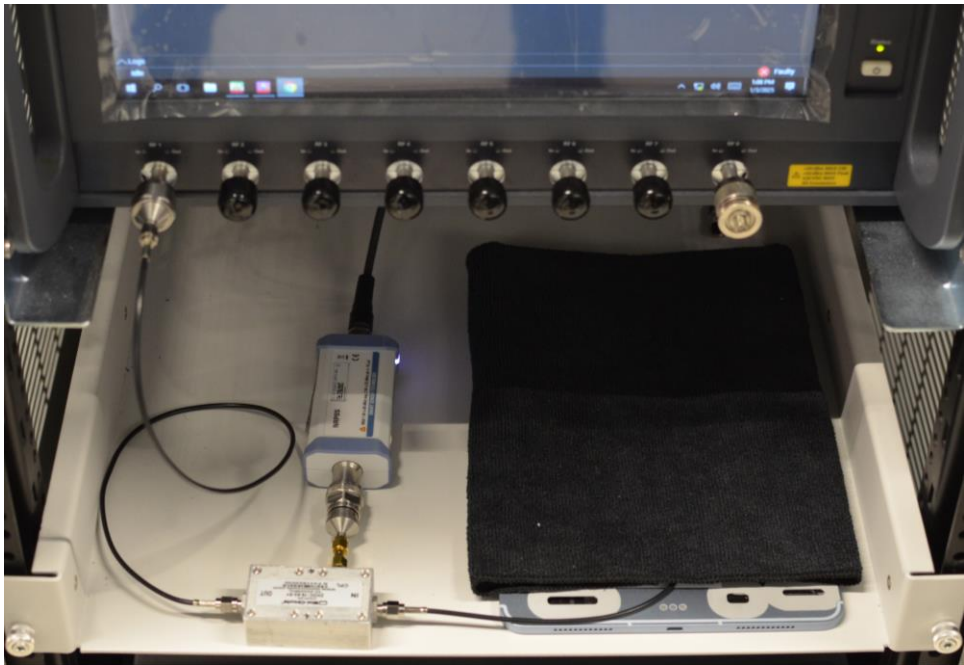
Test Setup Photo 2 – Conducted Test Setup (Figure 5-1a)
