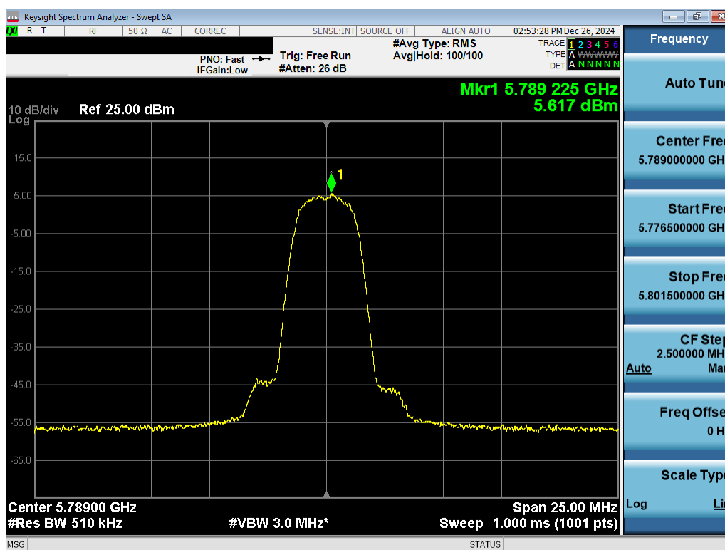
Plot 7-72. PSD TxBF Antenna 3a (NB UNII HDR4, ePA 5789MHz)
