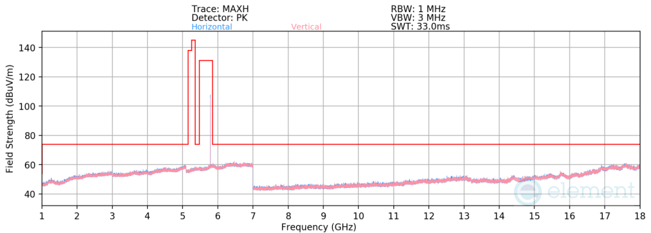
Plot 7-81. Radiated Spurious Emissions 1-18GHz Antenna 1b (NB UNII BDR ePA – 5789MHz)
