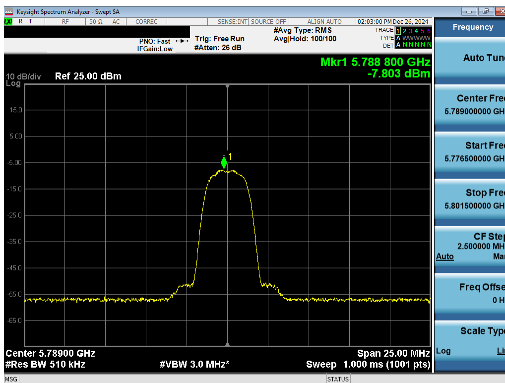
Plot 7-28. PSD Antenna 3c (NB UNII HDR4, iPA – 5789MHz)
