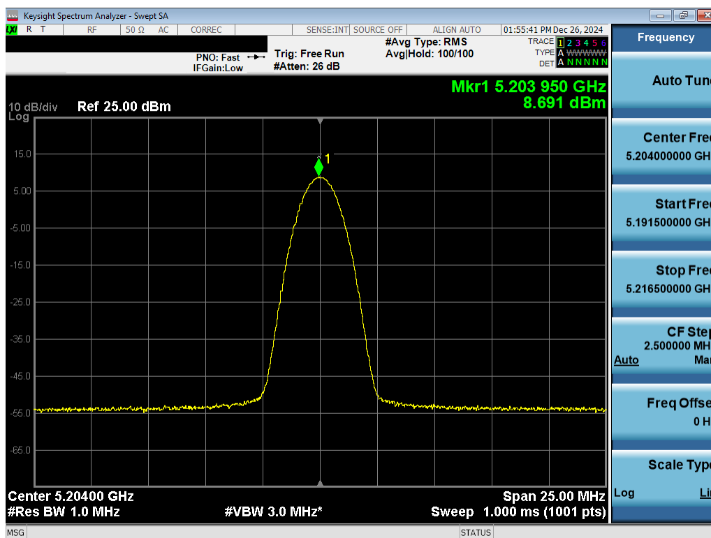
Plot 7-19. PSD Antenna 3c (NB UNII BDR, ePA – 5204MHz)
