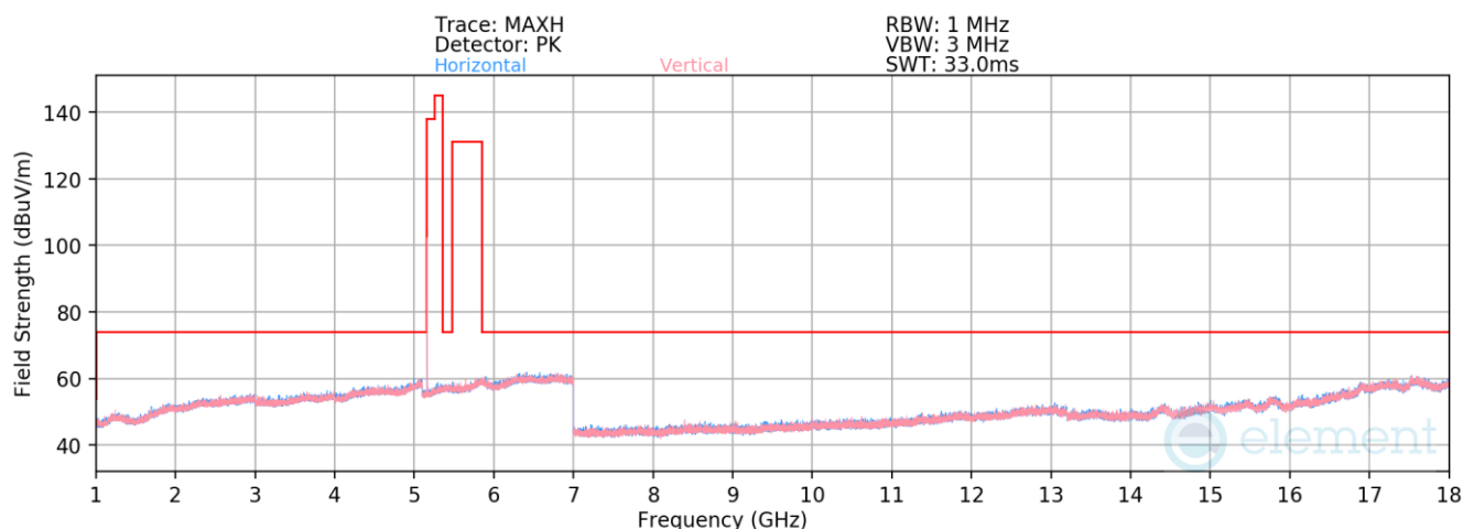
Plot 7-83. Radiated Spurious Emissions 1-18GHz Antenna 1b (NB UNII HDR4, ePA – 5162MHz)
