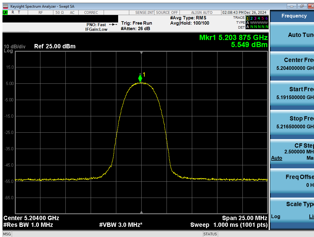
Plot 7-59. PSD TxBF Antenna 3c (NB UNII HDR4, ePA – 5204MHz)
