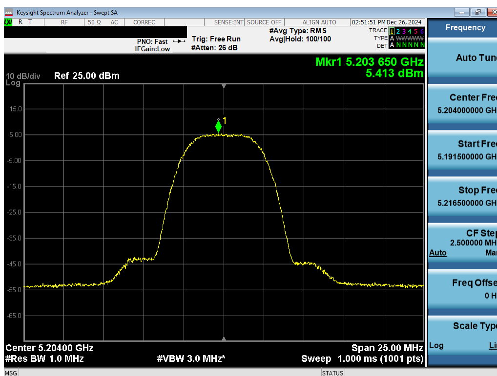
Plot 7-64. PSD Tx BF Antenna 3a (NB UNII HDR8, ePA – 5204MHz)
