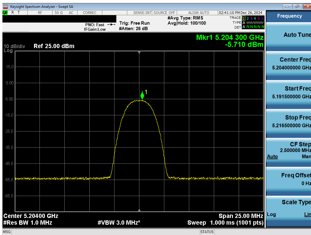
Plot 7-34. PSD Antenna 3a (NB UNII HDR4, iPA – 5204MHz)
