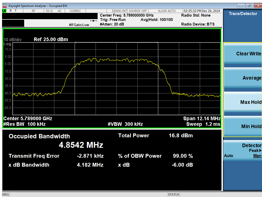
Plot 7-15. 6dB BW & 99% OBW Antenna 3a (NB UNII HDR8, ePA – 5789MHz)
