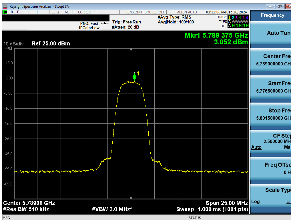
Plot 7-51. PSD Antenna 1b (NB UNII HDR4, ePA – 5789MHz)
