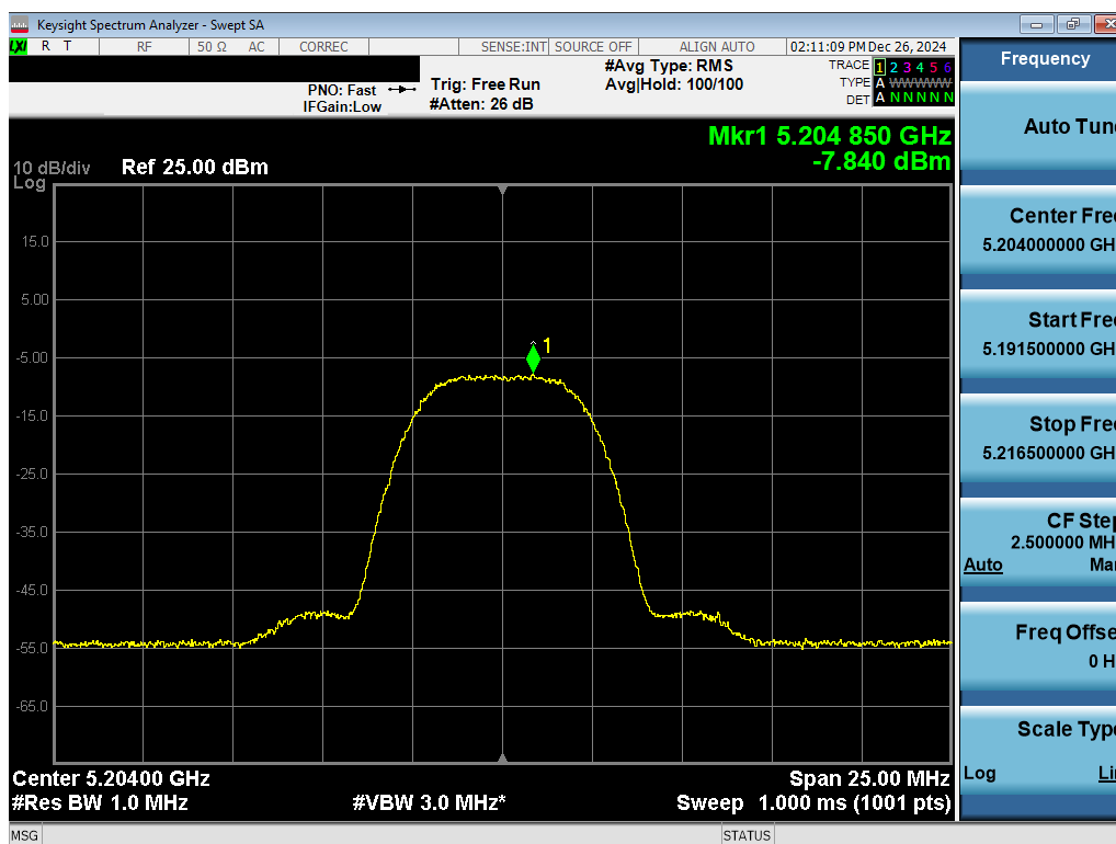
Plot 7-65. PSD TxBF Antenna 3c (NB UNII HDR8, iPA – 5204MHz)
