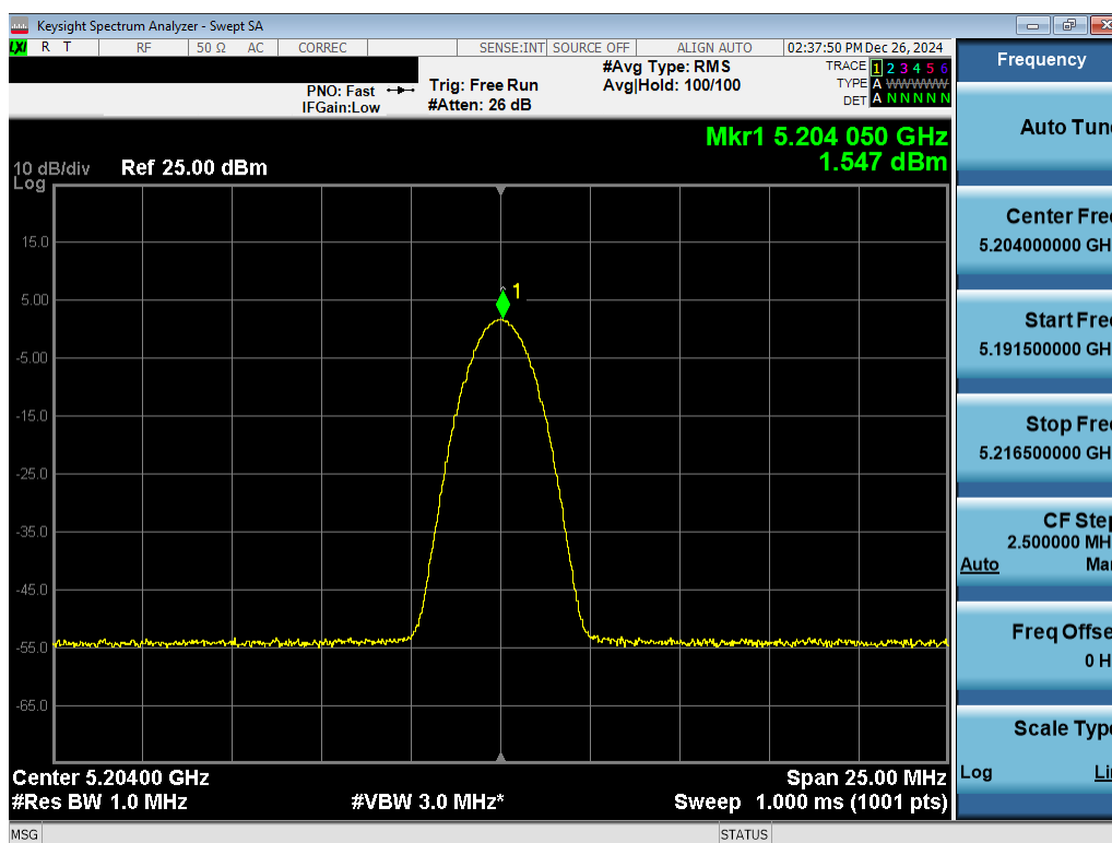
Plot 7-32. PSD Antenna 3a (NB UNII BDR, iPA – 5204MHz)
