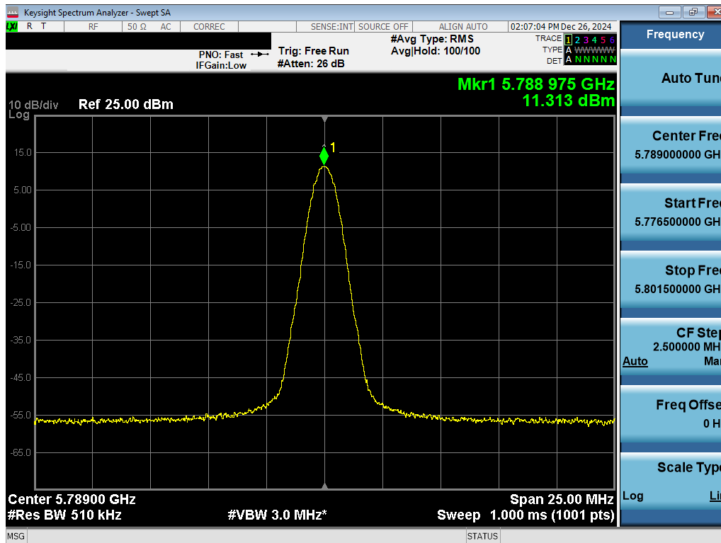
Plot 7-67. PSD TxBF Antenna 3c (NB UNII BDR, ePA 5789MHz)
