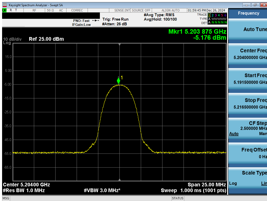
Plot 7-22. PSD Antenna 3c (NB UNII HDR4, iPA – 5204MHz)
