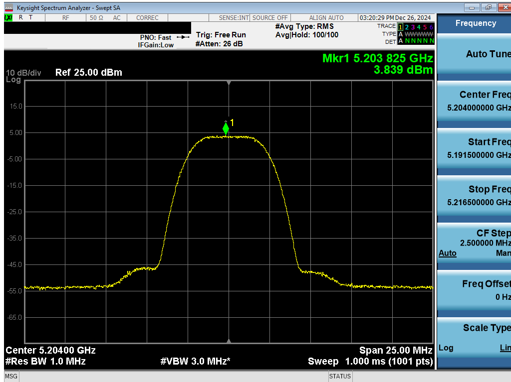
Plot 7-47. PSD Antenna 1b (NB UNII HDR8, ePA – 5204MHz)
