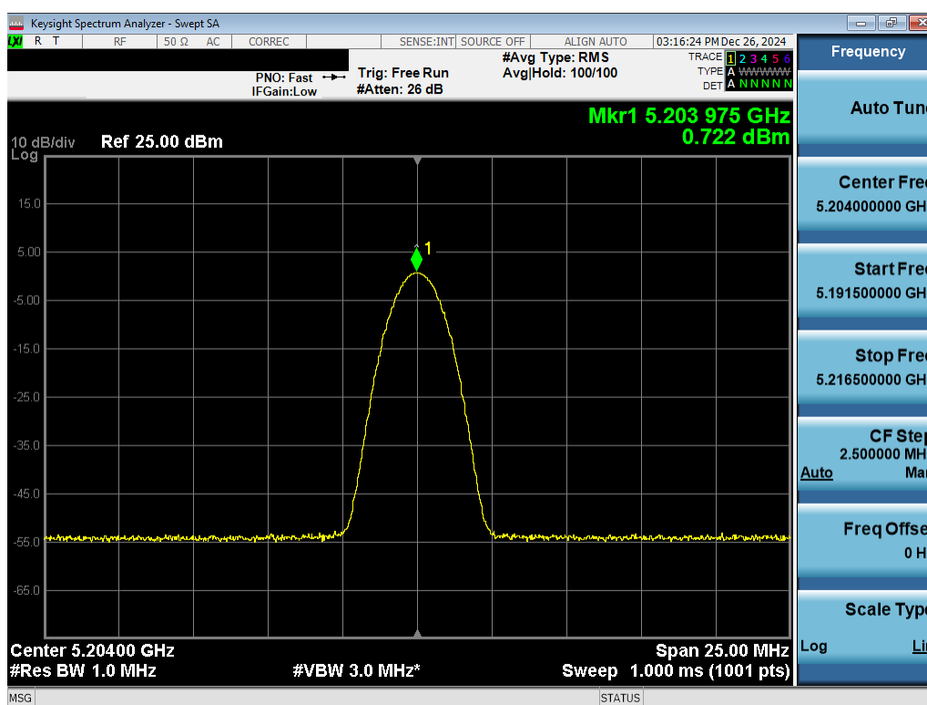
Plot 7-44. PSD Antenna 1b (NB UNII BDR, iPA – 5204MHz)
