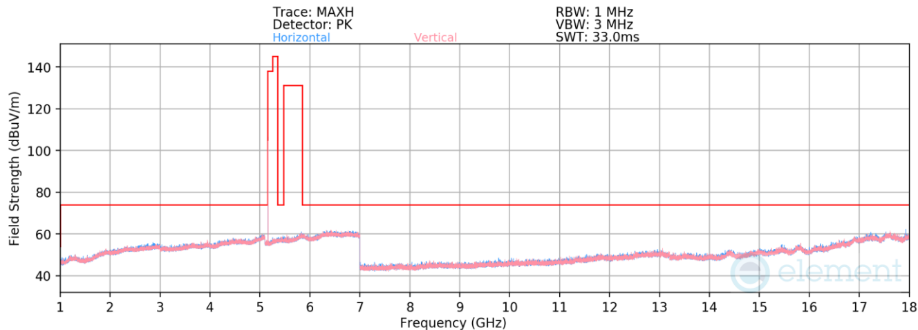
Plot 7-77. Radiated Spurious Emissions 1-18GHz Antenna 1b (NB UNII BDR ePA – 5162MHz)
