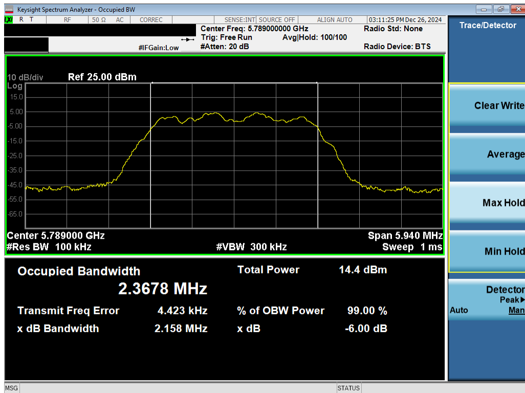
Plot 7-17. 6dB BW & 99% OBW Antenna 1b (NB UNII HDR4, ePA – 5789MHz)
