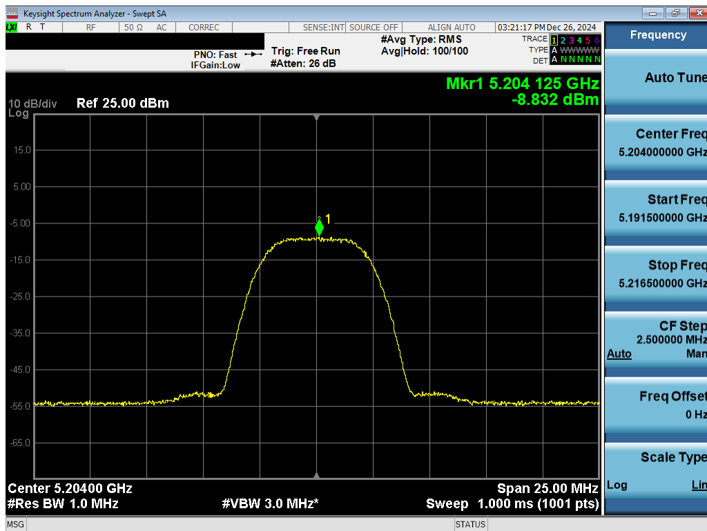
Plot 7-48. PSD Antenna 1b (NB UNII HDR8, iPA – 5204MHz)
