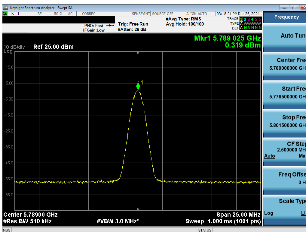
Plot 7-50. PSD Antenna 1b (NB UNII BDR, iPA – 5789MHz)
