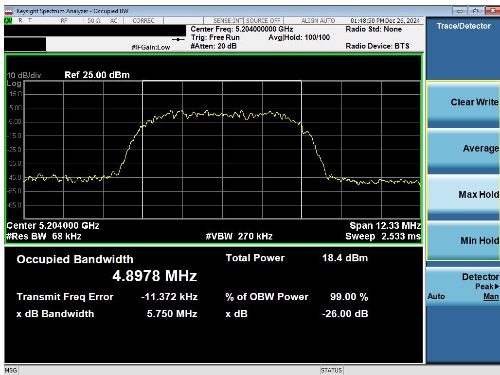
Plot 7-3. 26dB BW & 99% OBW Antenna 3c (NB UNII HDR8, ePA- 5204MHz)
