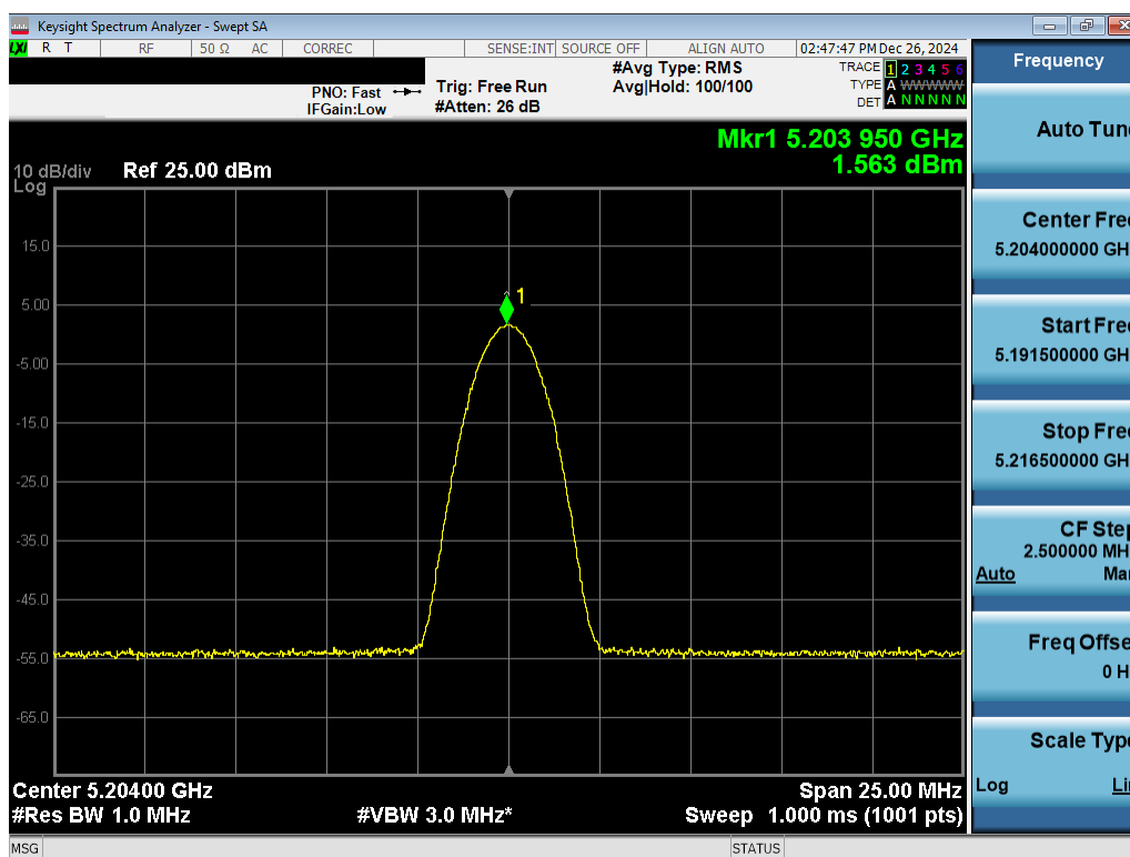
Plot 7-58. PSD TxBF Antenna 3a (NB UNII BDR, iPA – 5204MHz)
