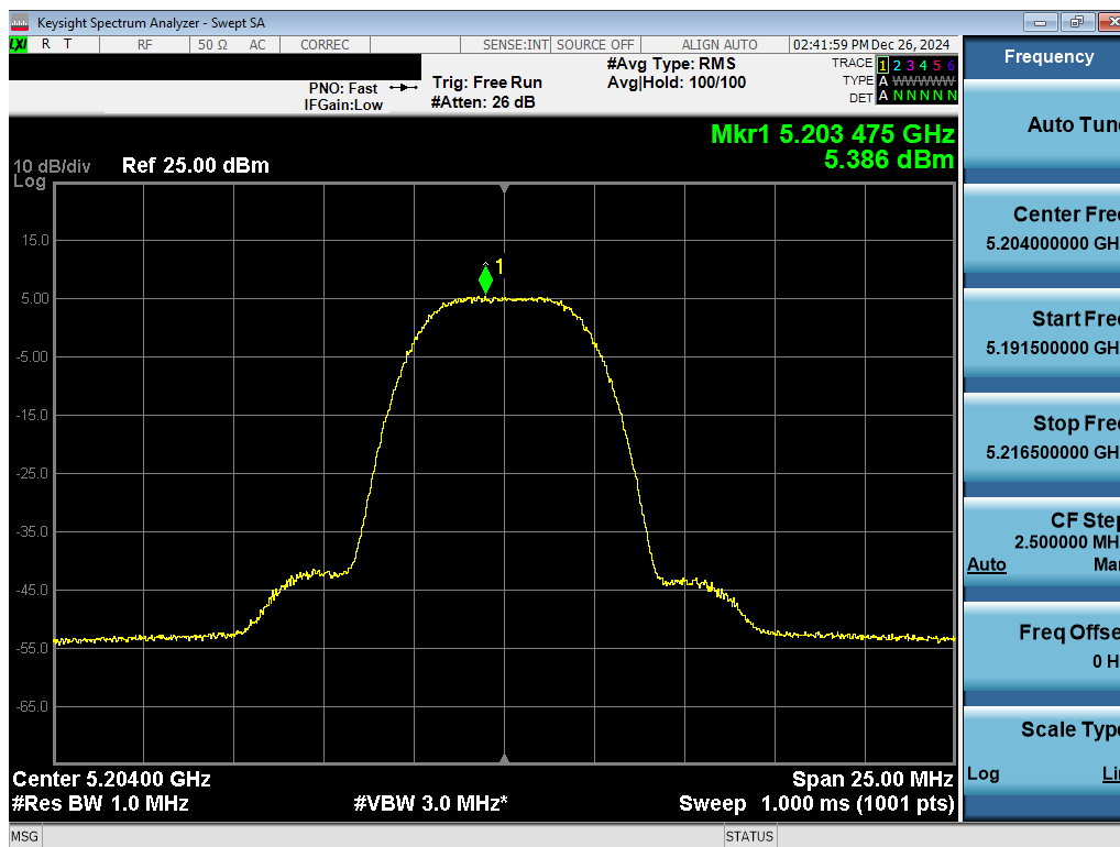
Plot 7-35. PSD Antenna 3a (NB UNII HDR8, ePA - 5204MHz)
