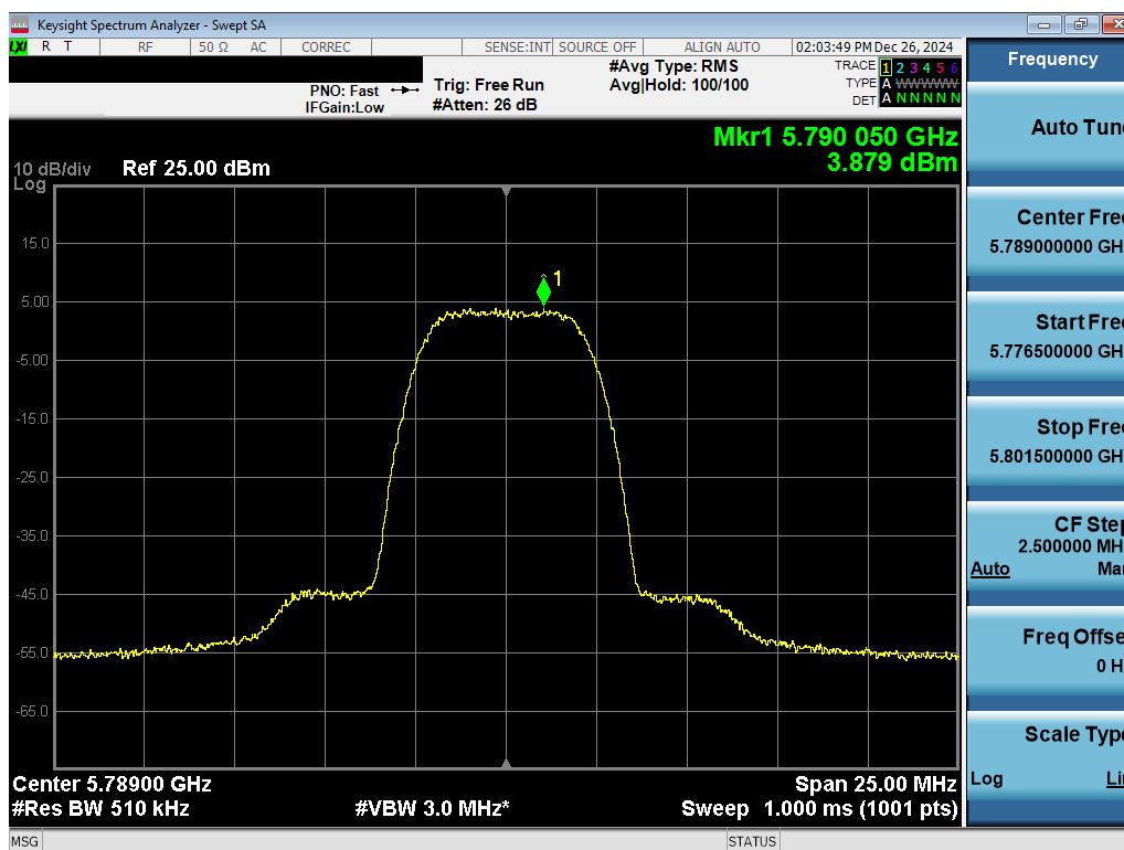
Plot 7-29. PSD Antenna 3c (NB UNII HDR8, ePA – 5789MHz)
