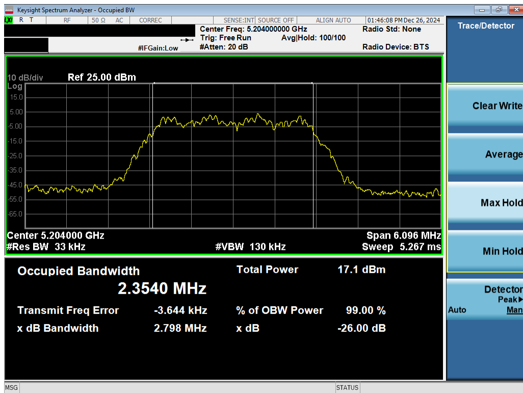
Plot 7-2. 26dB BW & 99% OBW Antenna 3c (NB UNII HDR4, ePA- 5204MHz)
