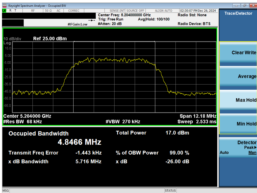
Plot 7-6. 26dB BW & 99% OBW Antenna 3a (NB UNII HDR8, ePA- 5204MHz)
