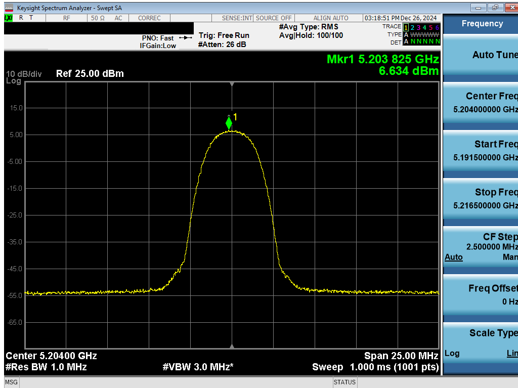
Plot 7-45. PSD Antenna 1b (NB UNII HDR4, ePA – 5204MHz)
