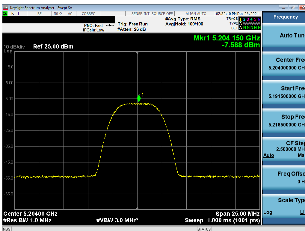
Plot 7-66. PSD TxBF Antenna 3a (NB UNII HDR8, iPA – 5204MHz)
