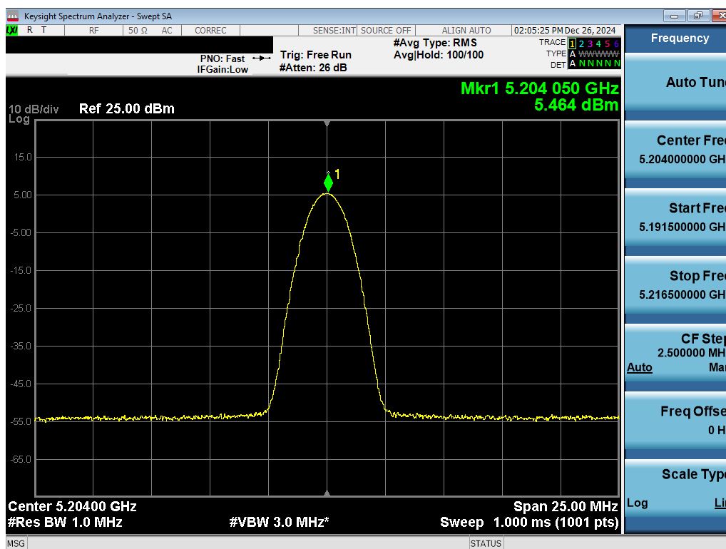
Plot 7-55. PSD TxBF Antenna 3c (NB UNII BDR, ePA – 5204MHz)
