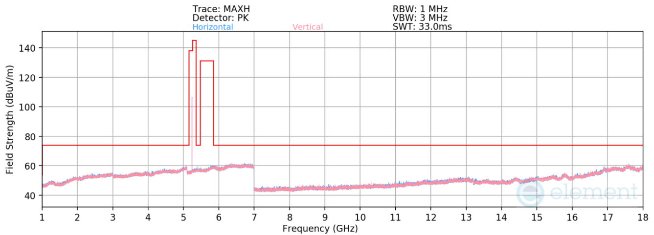
Plot 7-79. Radiated Spurious Emissions 1-18GHz Antenna 1b (NB UNII BDR ePA – 5245MHz)
