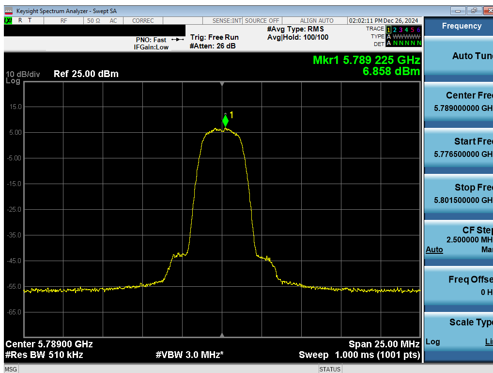
Plot 7-27. PSD Antenna 3c (NB UNII HDR4, ePA – 5789MHz)
