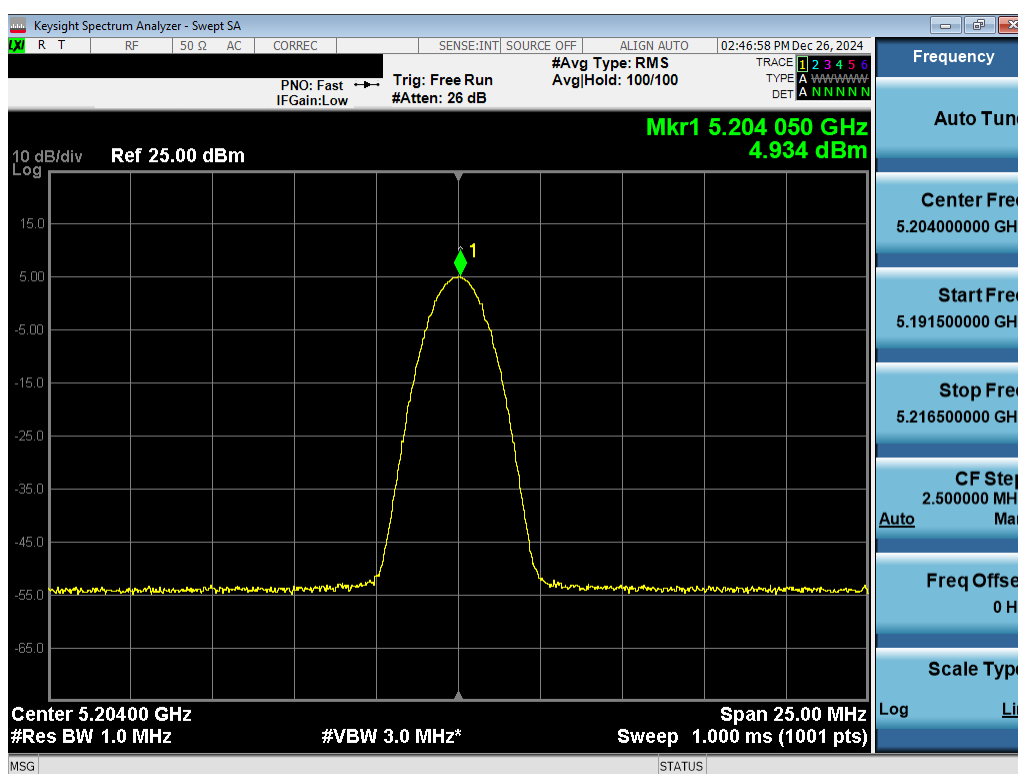
Plot 7-56. PSD TxBF Antenna 3a (NB UNII BDR, ePA – 5204MHz)
