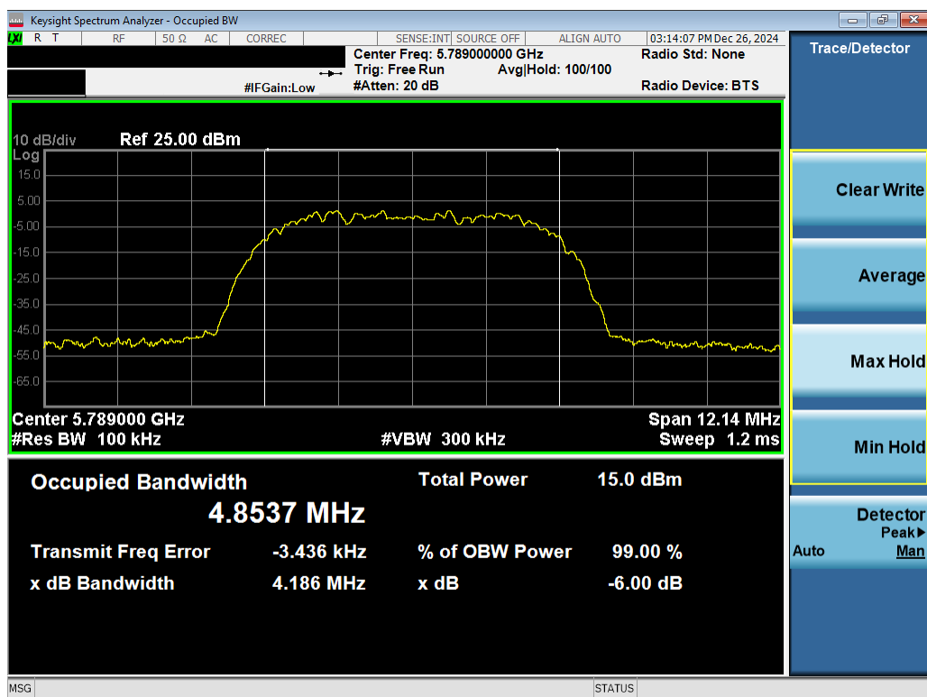
Plot 7-18. 6dB BW & 99% OBW Antenna 1b (NB UNII HDR8, ePA – 5789MHz)
