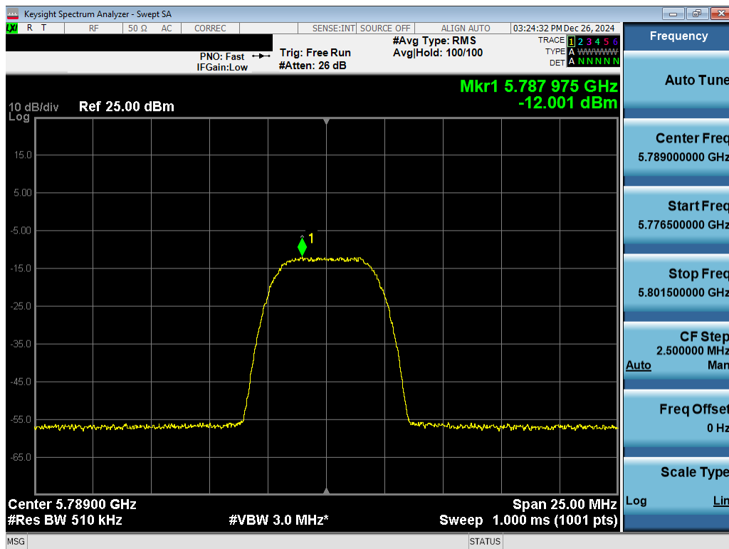
Plot 7-54. PSD Antenna 1b (NB UNII HDR8, iPA – 5789MHz)
