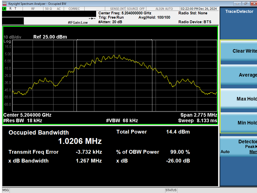
Plot 7-4. 26dB BW & 99% OBW Antenna 3a (NB UNII BDR, ePA- 5204MHz)
