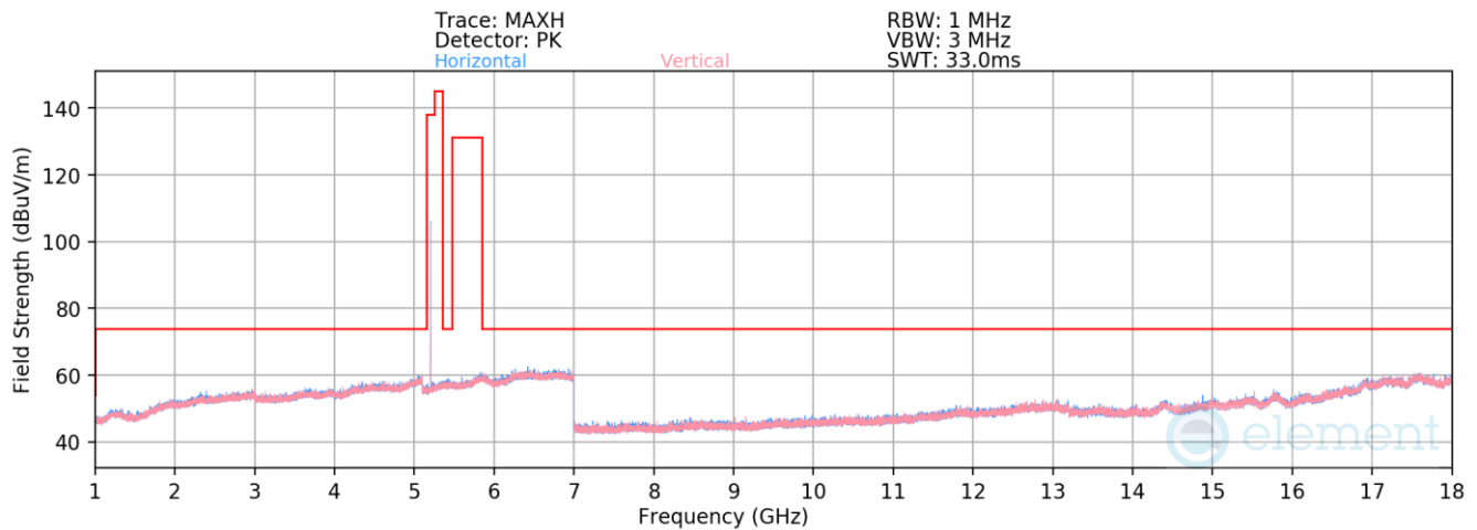
Plot 7-78. Radiated Spurious Emissions 1-18GHz Antenna 1b (NB UNII BDR ePA – 5204MHz)
