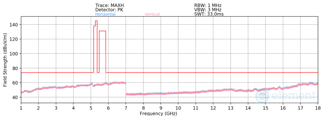
Plot 7-82. Radiated Spurious Emissions 1-18GHz Antenna 1b (NB UNII BDR ePA – 5844MHz)
