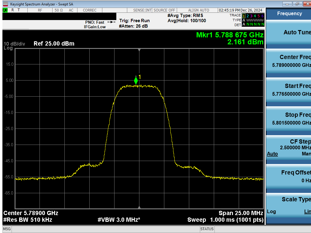
Plot 7-41. PSD Antenna 3a (NB UNII HDR8, ePA – 5789MHz)
