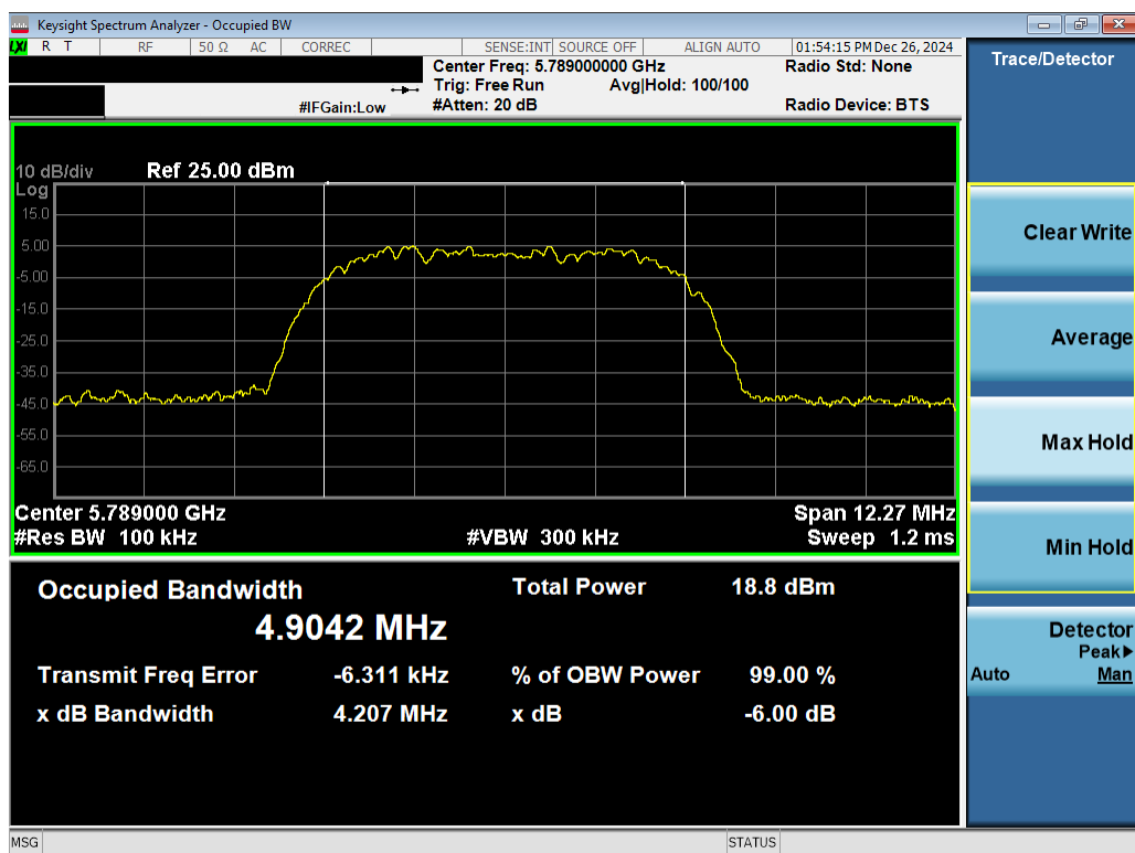
Plot 7-12. 6dB BW & 99% OBW Antenna 3c (NB UNII HDR8, ePA – 5789MHz)
