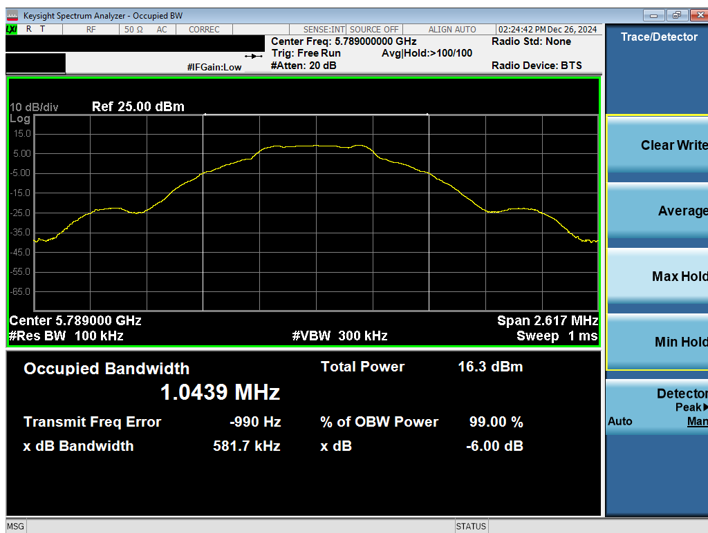
Plot 7-13. 6dB BW & 99% OBW Antenna 3a (NB UNII BDR, ePA – 5789MHz)
