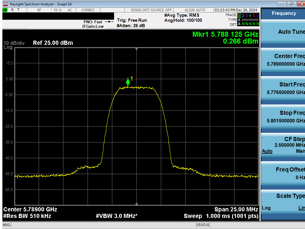
Plot 7-53. PSD Antenna 1b (NB UNII HDR8, ePA – 5789MHz)
