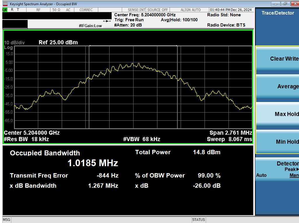
Plot 7-1. 26dB BW & 99% OBW Antenna 3c (NB UNII BDR, ePA- 5204MHz)
