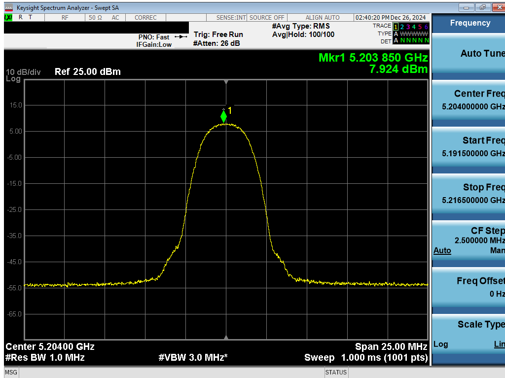
Plot 7-33. PSD Antenna 3a (NB UNII HDR4, ePA – 5204MHz)
