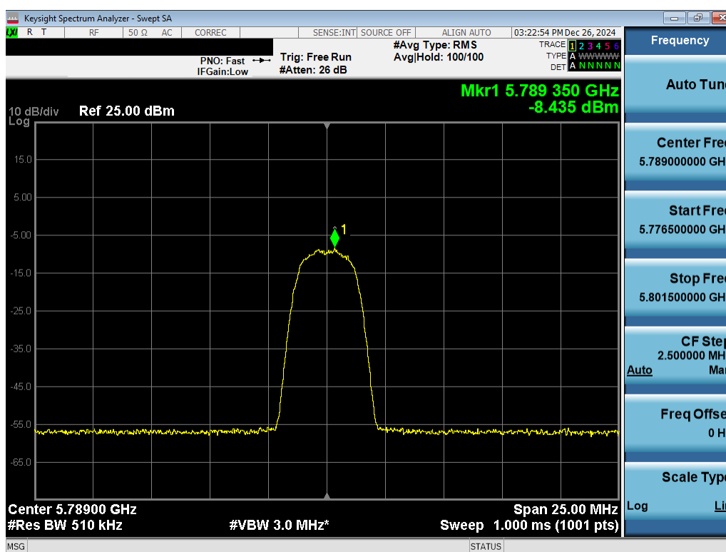
Plot 7-52. PSD Antenna 1b (NB UNII HDR4, iPA – 5789MHz)
