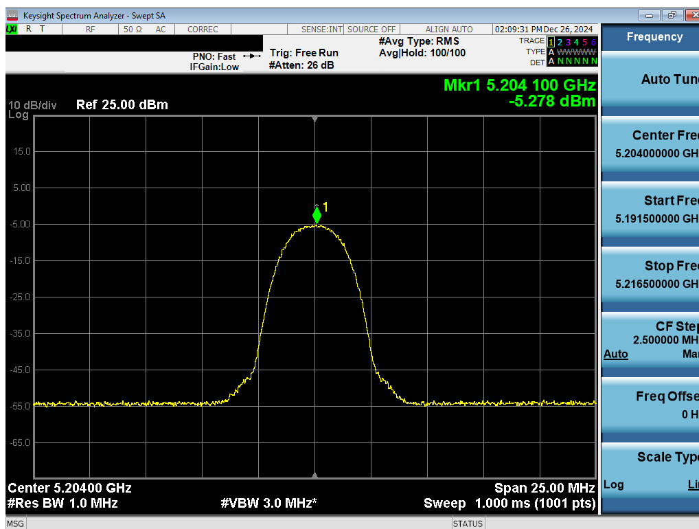
Plot 7-61. PSD TxBF Antenna 3c (NB UNII HDR4, iPA – 5204MHz)
