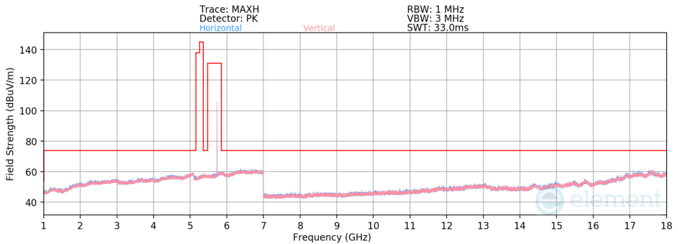
Plot 7-86. Radiated Spurious Emissions 1-18GHz Antenna 1b (NB UNII HDR4, ePA – 5733MHz)
