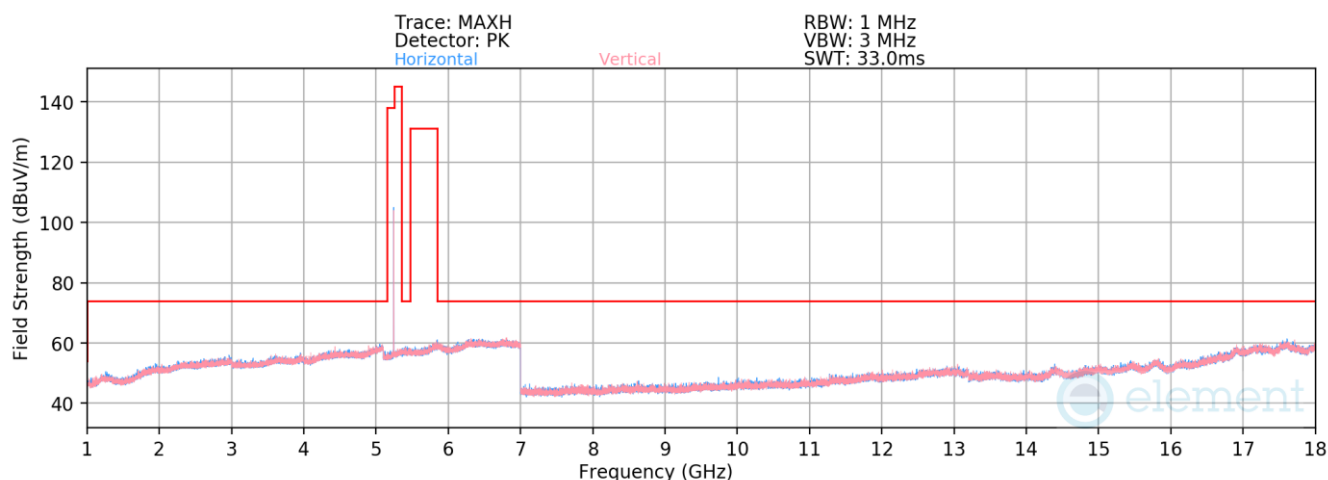
Plot 7-85. Radiated Spurious Emissions 1-18GHz Antenna 1b (NB UNII HDR4, ePA – 5245MHz)
