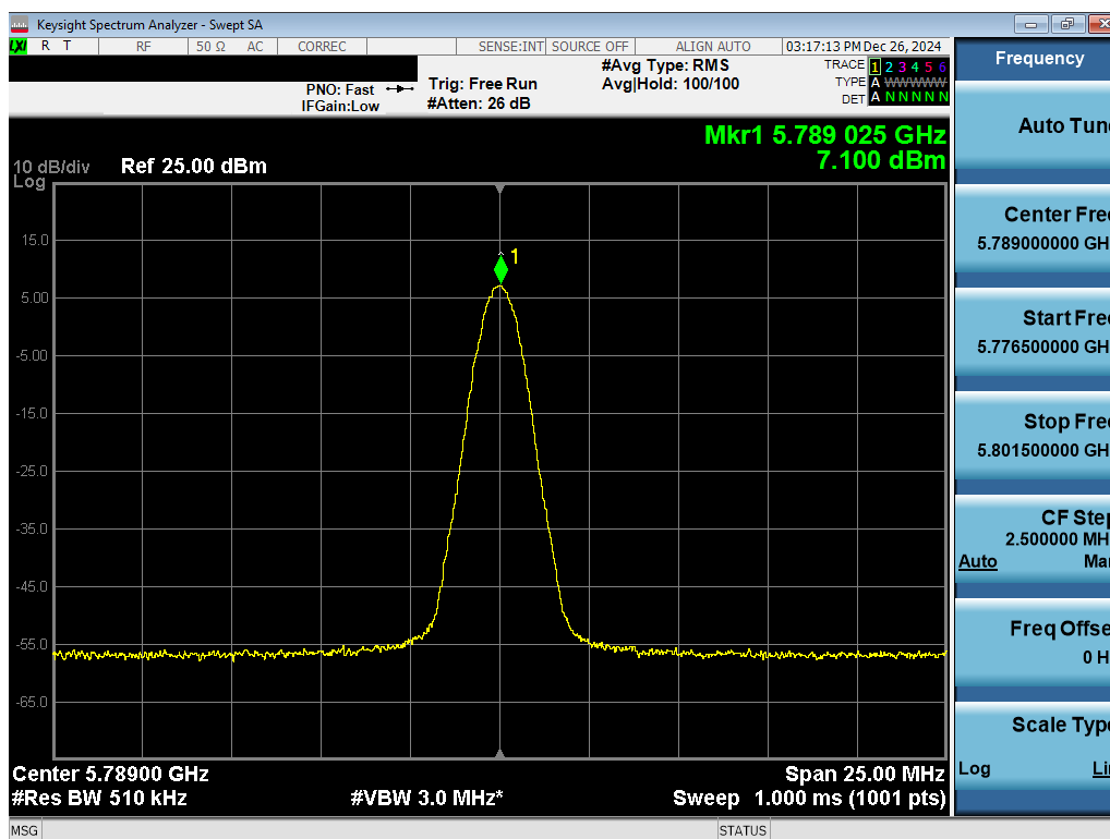
Plot 7-49. PSD Antenna 1b (NB UNII BDR, ePA – 5789MHz)
