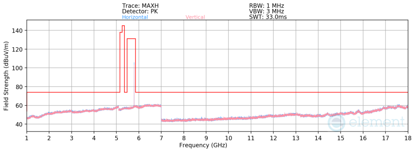
Plot 7-87. Radiated Spurious Emissions 1-18GHz Antenna 1b (NB UNII HDR4, ePA – 5789MHz)
