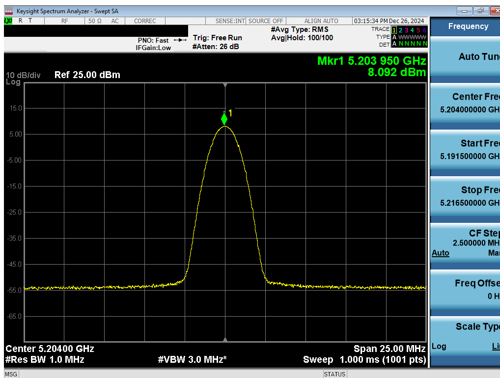
Plot 7-43. PSD Antenna 1b (NB UNII BDR, ePA – 5204MHz)
