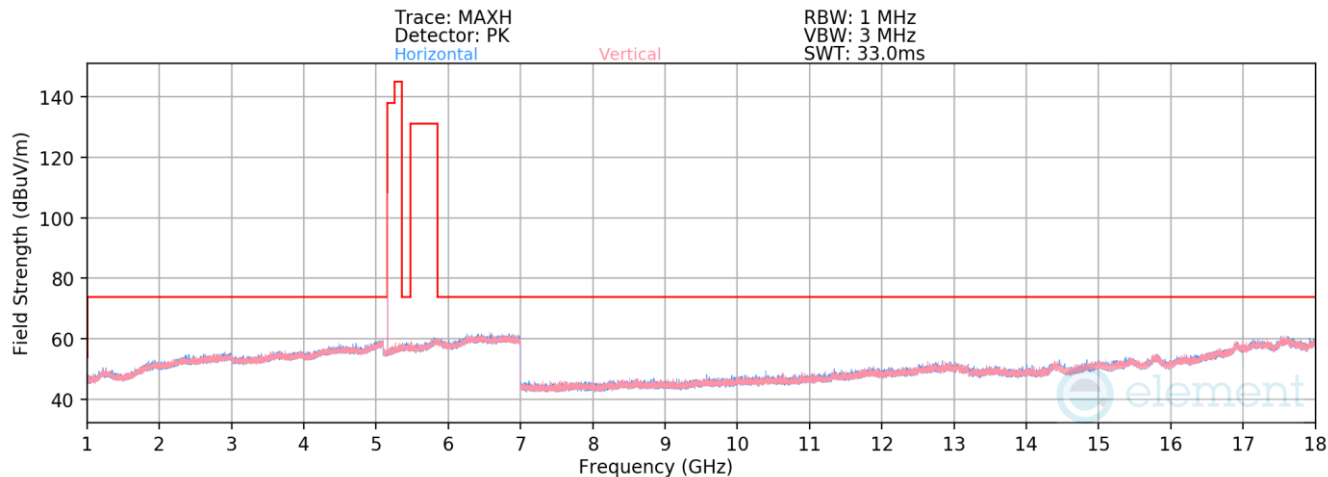
Plot 7-89. Radiated Spurious Emissions 1-18GHz TxBF (NB UNII BDR ePA – 5162MHz)
