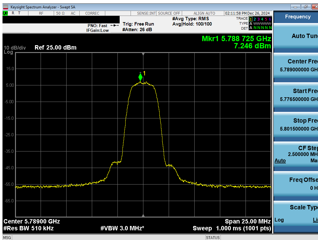
Plot 7-71. PSD TxBF Antenna 3c (NB UNII HDR4, ePA 5789MHz)
