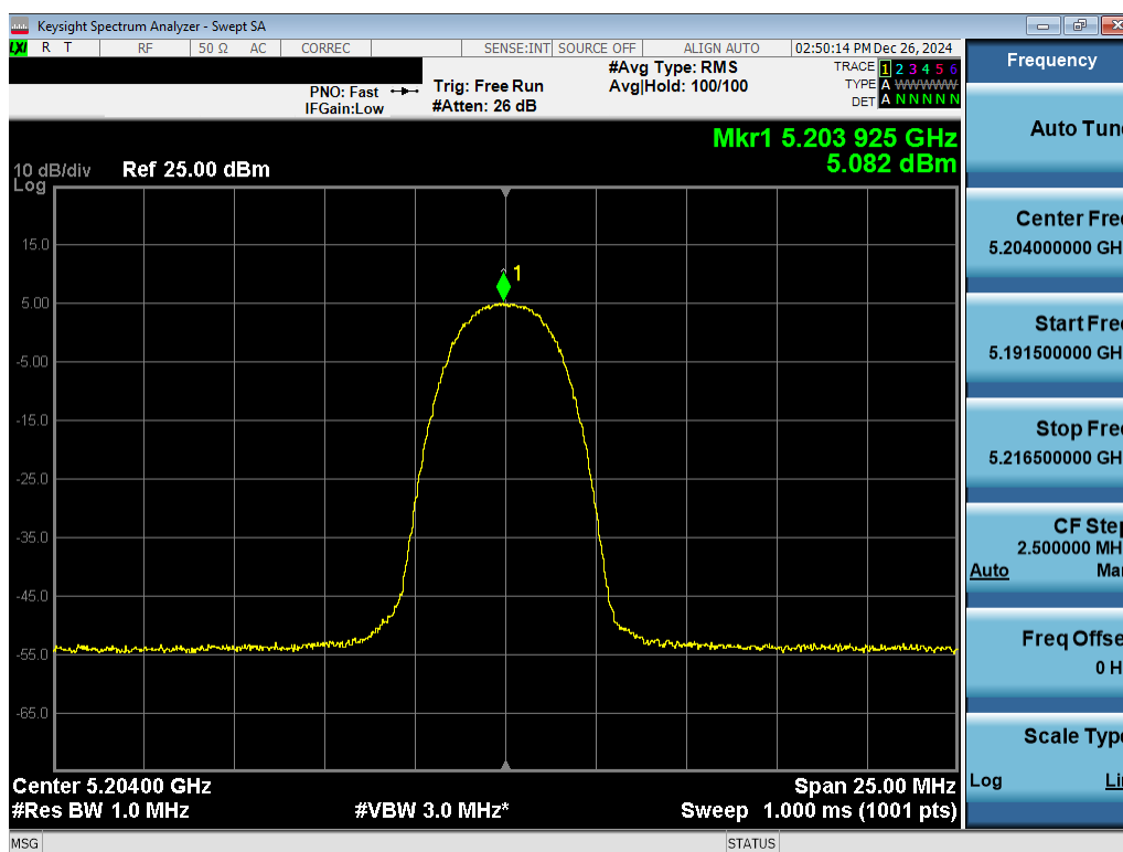
Plot 7-60. PSD TxBF Antenna 3a (NB UNII HDR4, ePA – 5204MHz)
