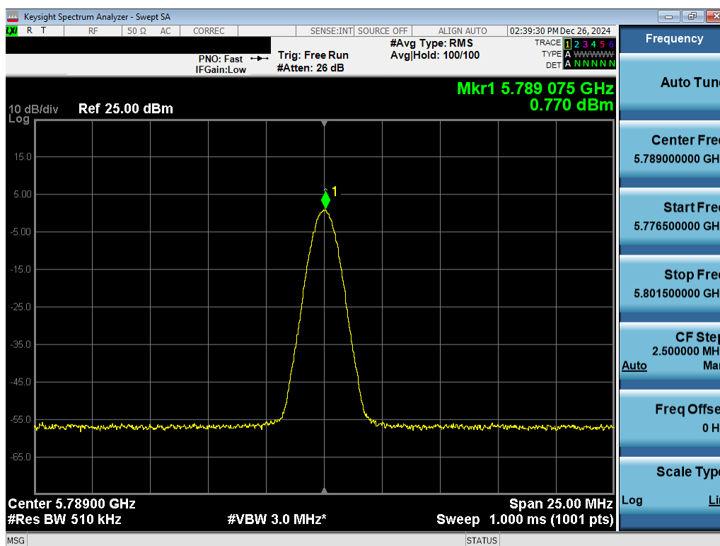
Plot 7-38. PSD Antenna 3a (NB UNII BDR, iPA – 5789MHz)
