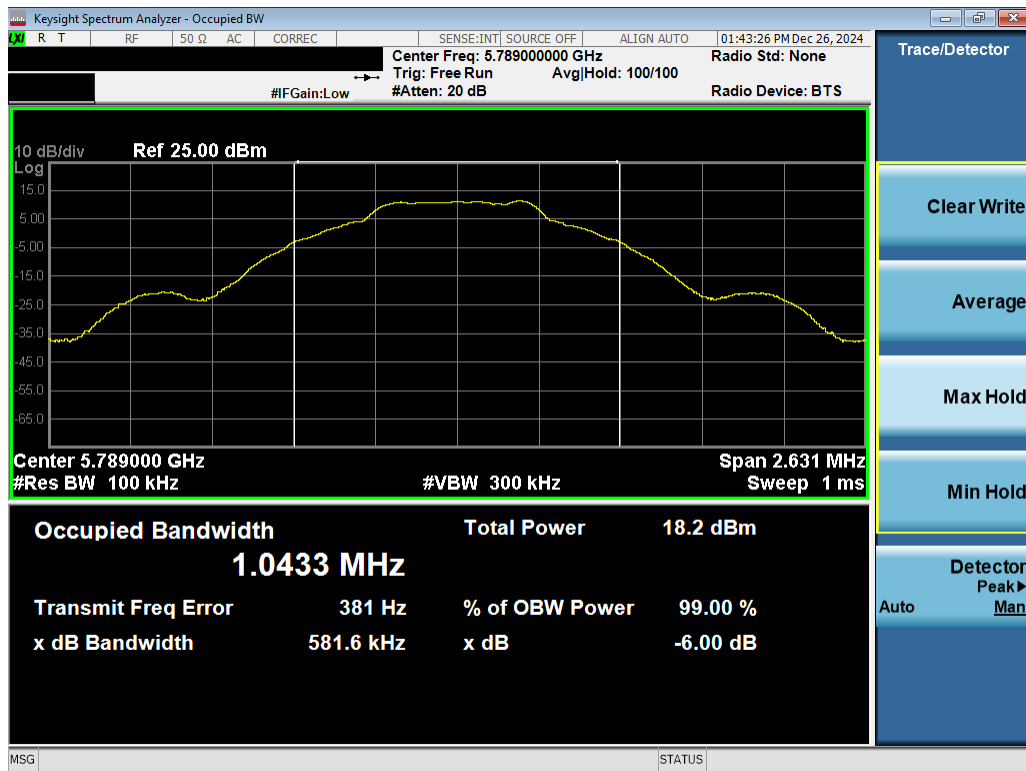
Plot 7-10. 6dB BW & 99% OBW Antenna 3c (NB UNII BDR, ePA – 5789MHz)
