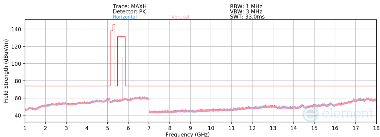
Plot 7-80. Radiated Spurious Emissions 1-18GHz Antenna 1b (NB UNII BDR ePA – 5733MHz)
