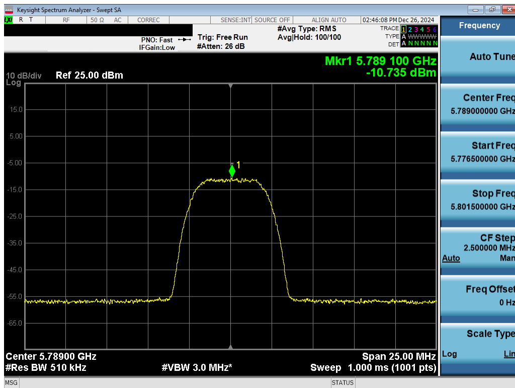
Plot 7-42. PSD Antenna 3a (NB UNII HDR8, iPA – 5789MHz)
