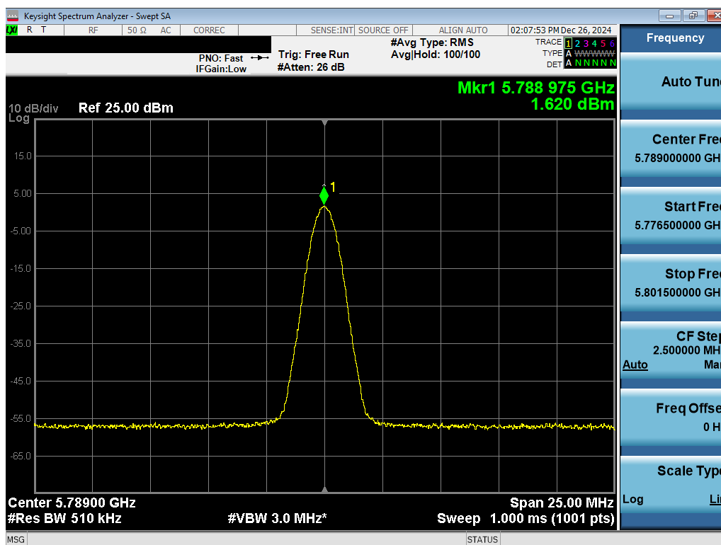
Plot 7-69. PSD TxBF Antenna 3c (NB UNII BDR, iPA 5789MHz)
