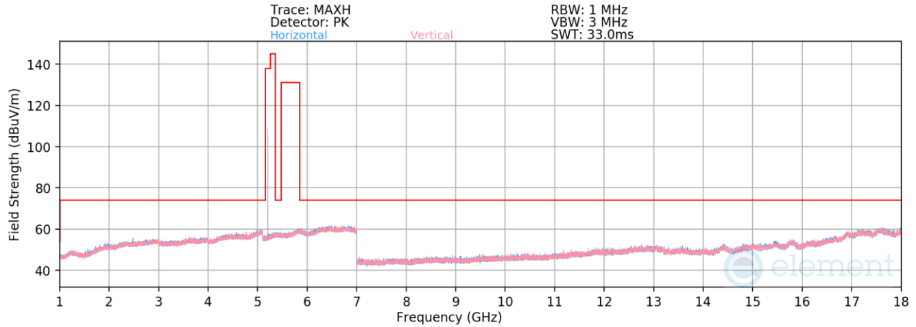
Plot 7-90. Radiated Spurious Emissions 1-18GHz TxBF (NB UNII BDR ePA – 5204MHz)
