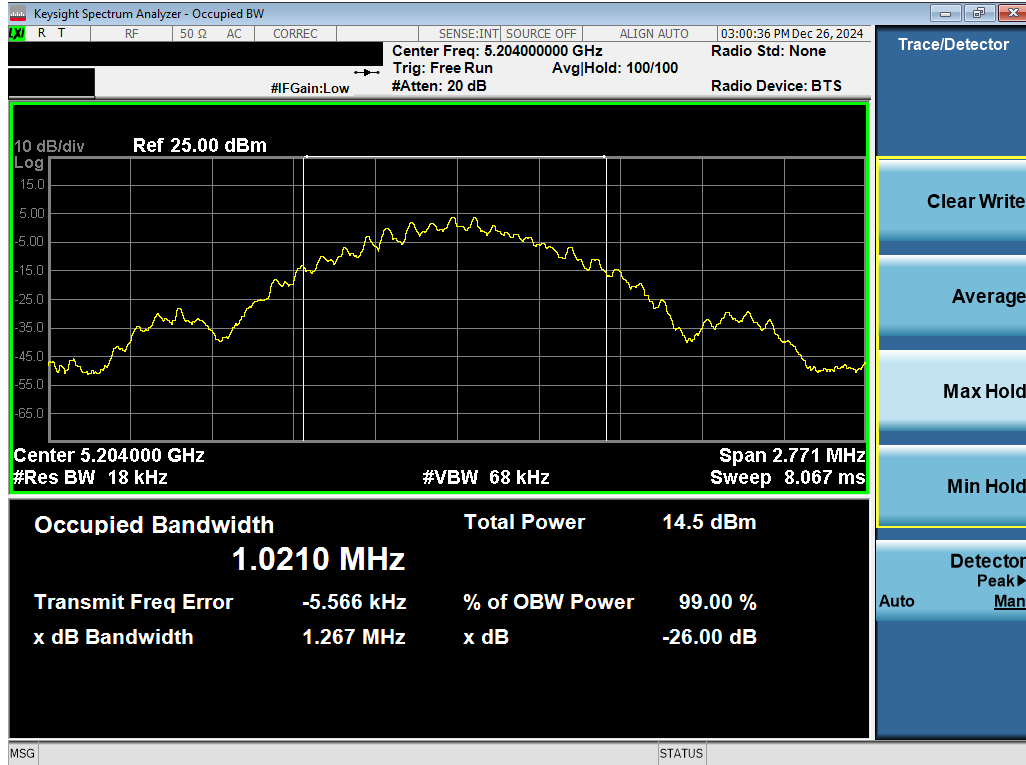
Plot 7-7. 26dB BW & 99% OBW Antenna 1b (NB UNII BDR, ePA- 5204MHz)
