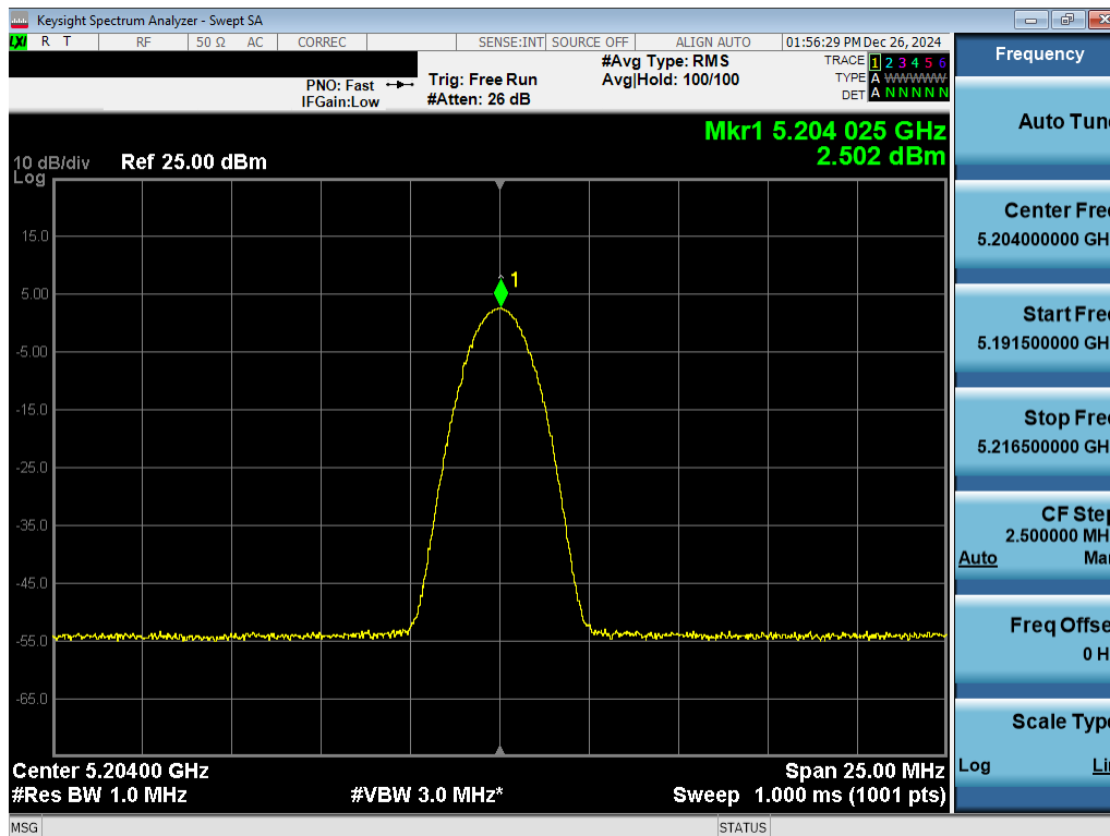
Plot 7-20. PSD Antenna 3c (NB UNII BDR, iPA – 5204MHz)
