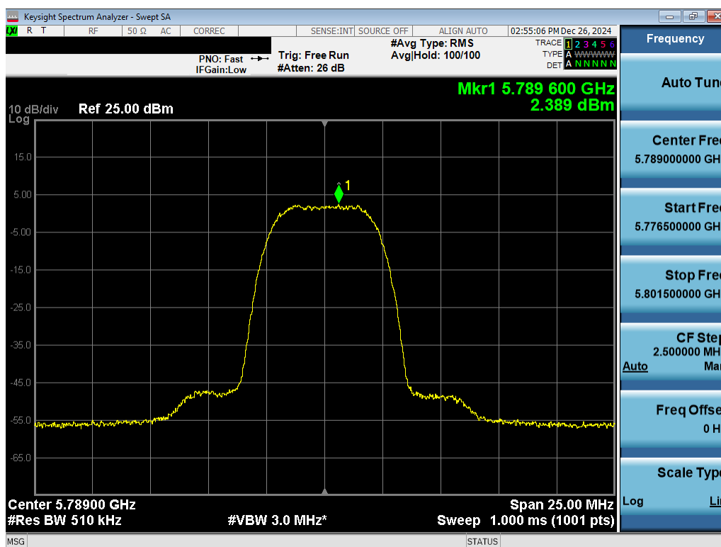
Plot 7-74. PSD TxBF Antenna 3a (NB UNII HDR8, ePA 5789MHz)
