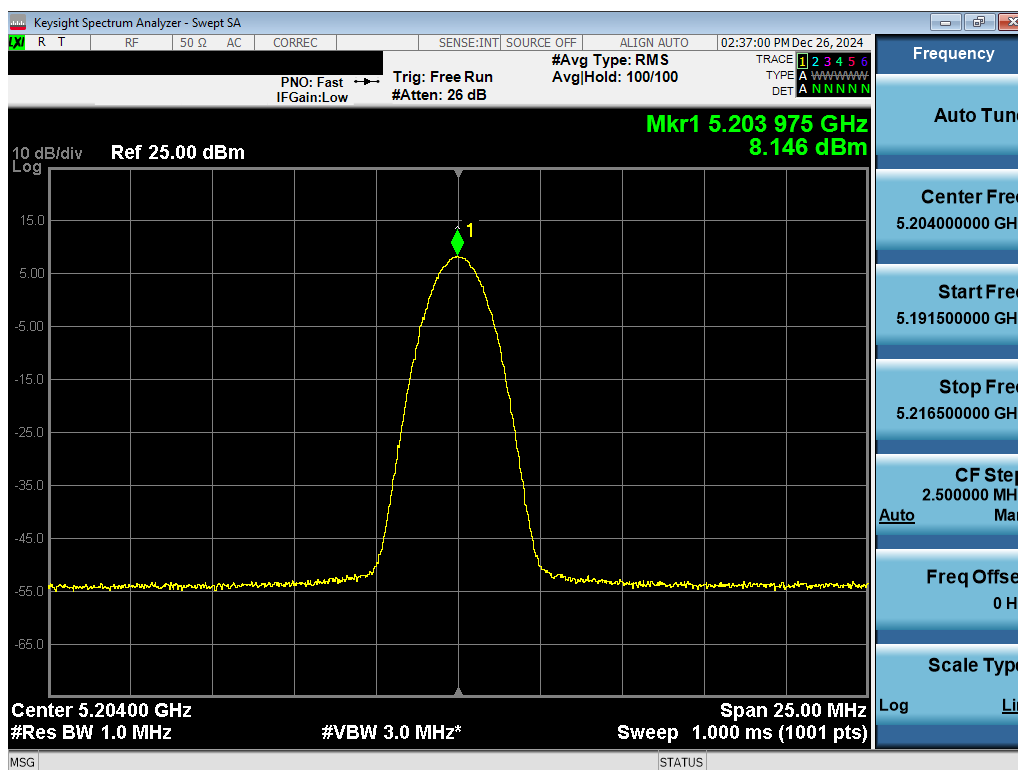
Plot 7-31. PSD Antenna 3a (NB UNII BDR, ePA – 5204MHz)
