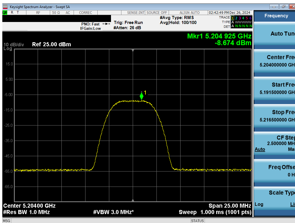
Plot 7-36. PSD Antenna 3a (NB UNII HDR8, iPA - 5204MHz)
