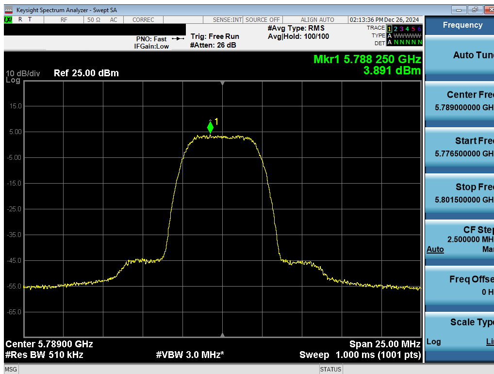
Plot 7-73. PSD TxBF Antenna 3c (NB UNII HDR8, ePA 5789MHz)
