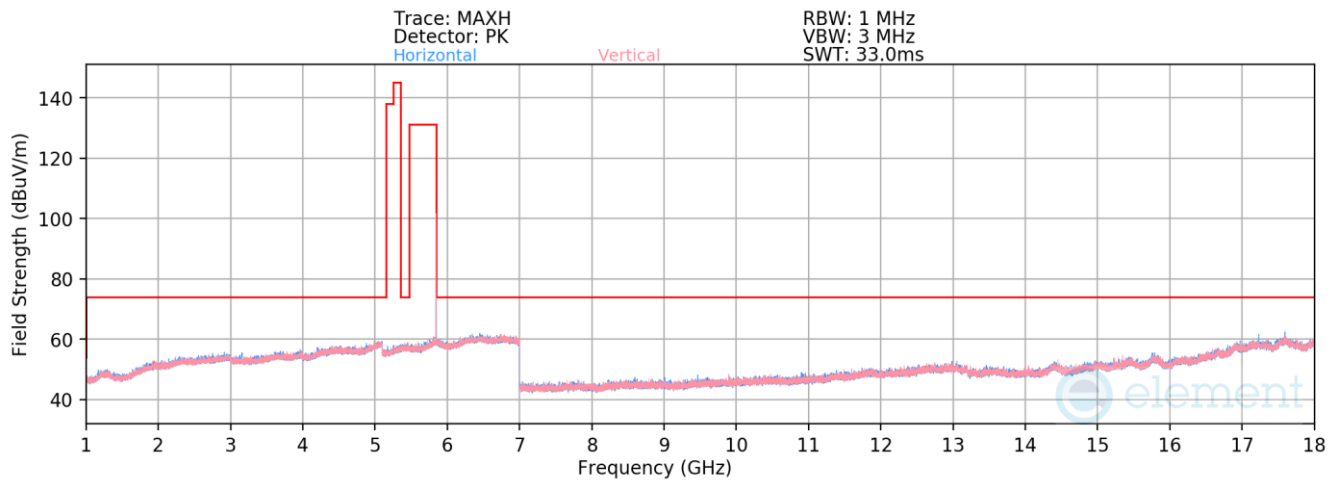
Plot 7-88. Radiated Spurious Emissions 1-18GHz Antenna 1b (NB UNII HDR4, ePA – 5844MHz)
