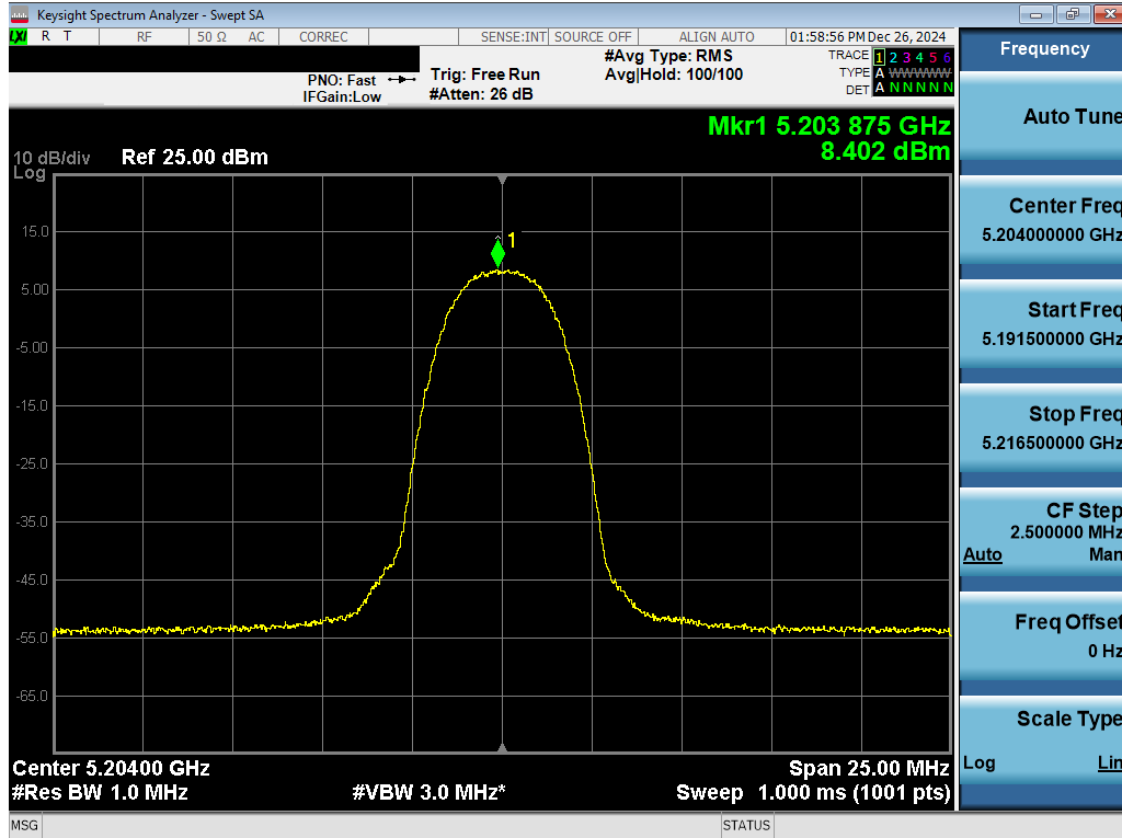
Plot 7-21. PSD Antenna 3c (NB UNII HDR4, ePA – 5204MHz)
