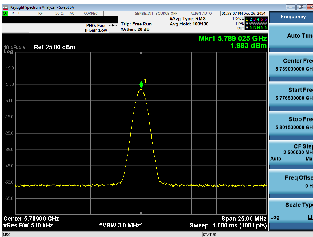
Plot 7-26. PSD Antenna 3c (NB UNII BDR, iPA – 5789MHz)
