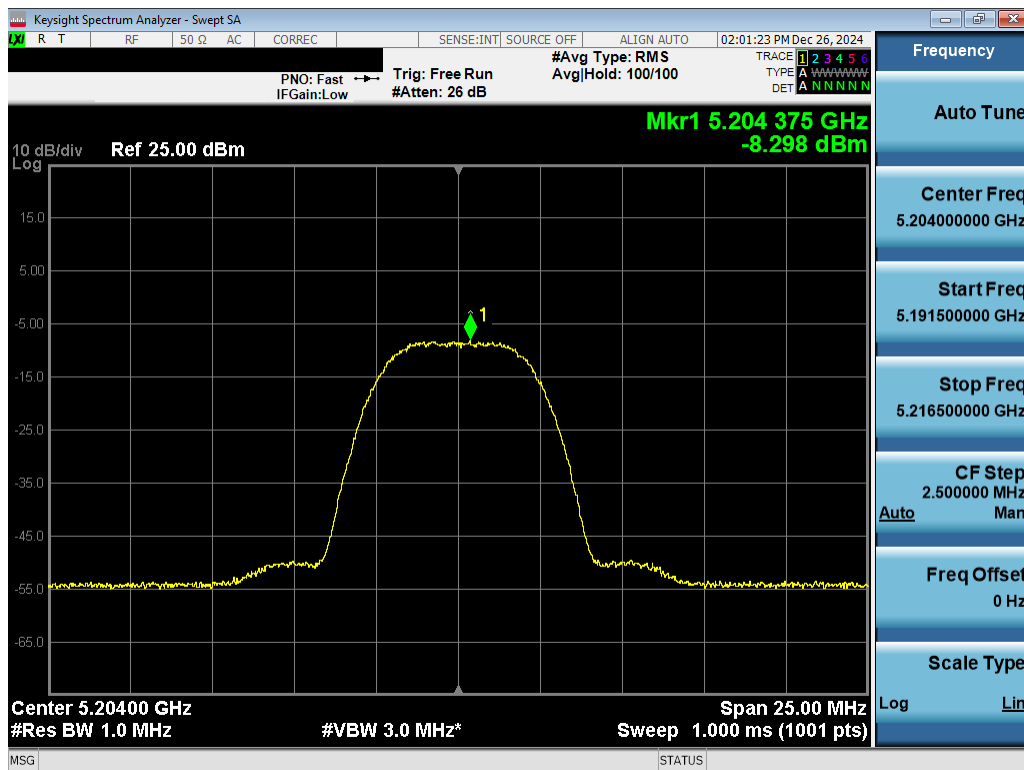
Plot 7-24. PSD Antenna 3c (NB UNII HDR8, iPA – 5204MHz)
