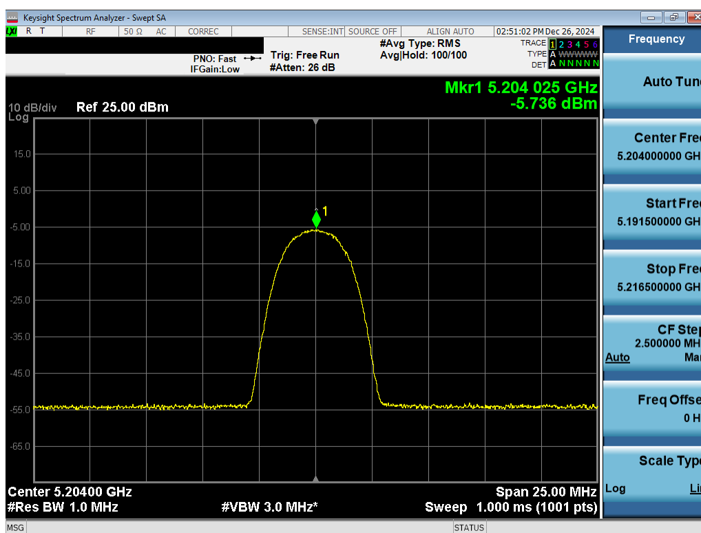
Plot 7-62. PSD TxBF Antenna 3a (NB UNII HDR4, iPA – 5204MHz)
