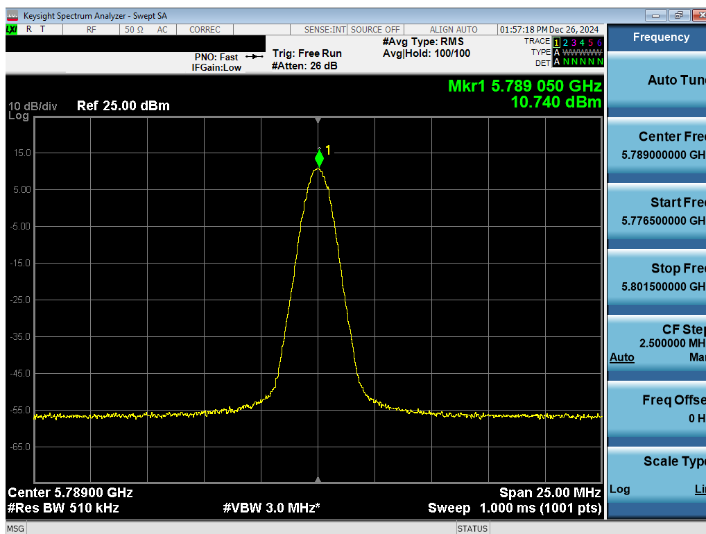
Plot 7-25. PSD Antenna 3c (NB UNII BDR, ePA – 5789MHz)
