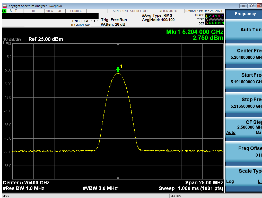
Plot 7-57. PSD TxBF Antenna 3c (NB UNII BDR, iPA – 5204MHz)
