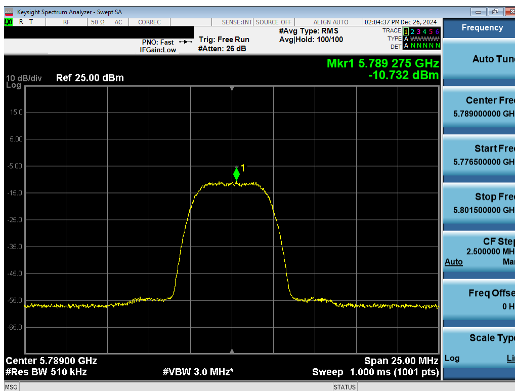
Plot 7-30. PSD Antenna 3c (NB UNII HDR8, iPA – 5789MHz)
