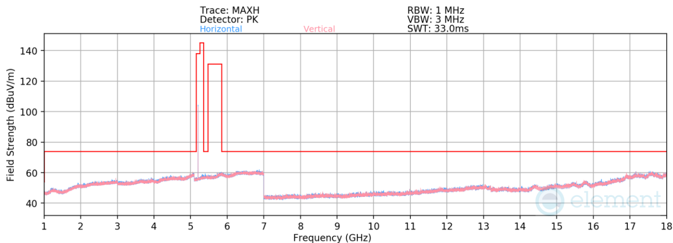
Plot 7-84. Radiated Spurious Emissions 1-18GHz Antenna 1b (NB UNII HDR4, ePA – 5204MHz)
