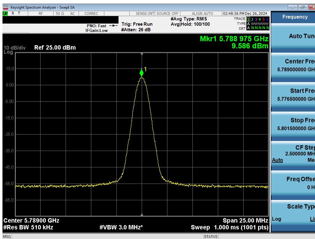
Plot 7-68. PSD TxBF Antenna 3a (NB UNII BDR, ePA 5789MHz)
