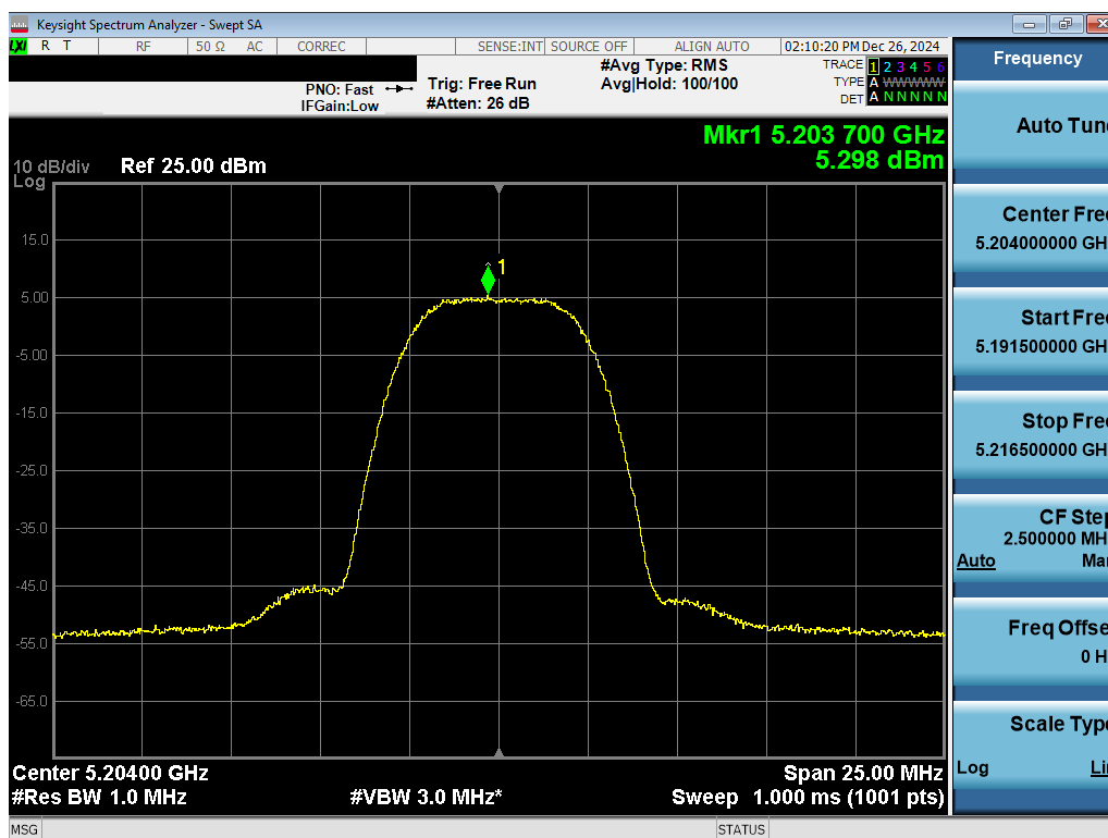
Plot 7-63. PSD Tx BF Antenna 3c (NB UNII HDR8, ePA – 5204MHz)
