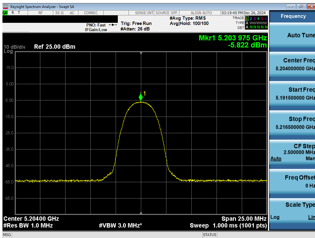
Plot 7-46. PSD Antenna 1b (NB UNII HDR4, iPA – 5204MHz)
