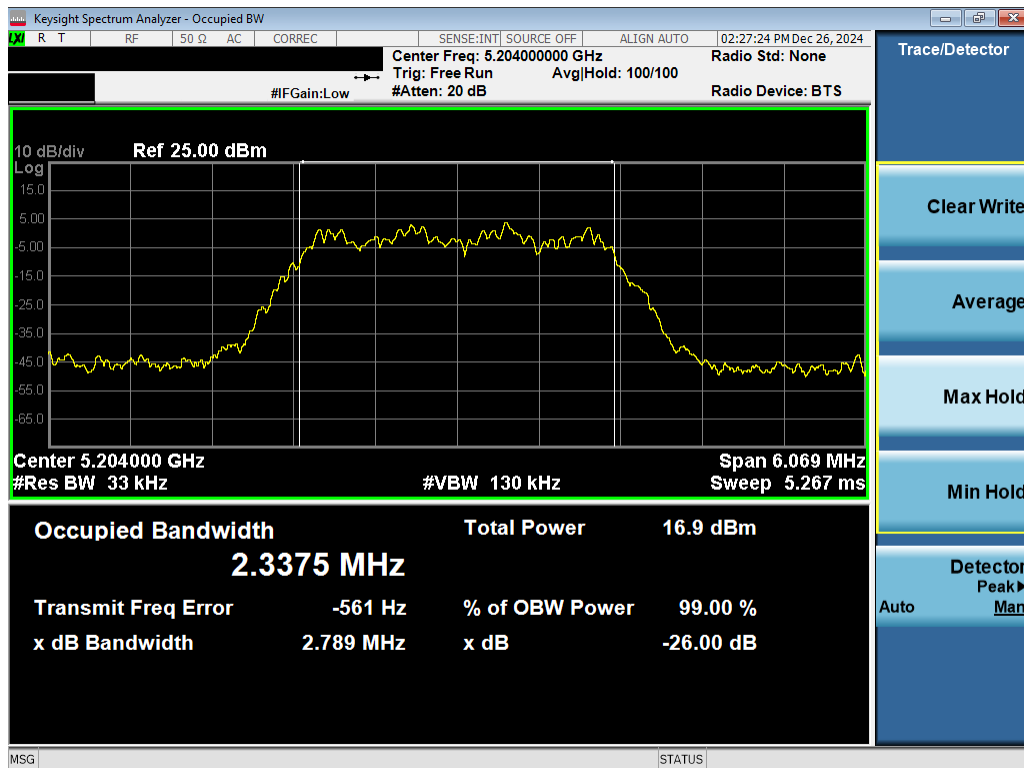
Plot 7-5. 26dB BW & 99% OBW Antenna 3a (NB UNII HDR4, ePA- 5204MHz)
