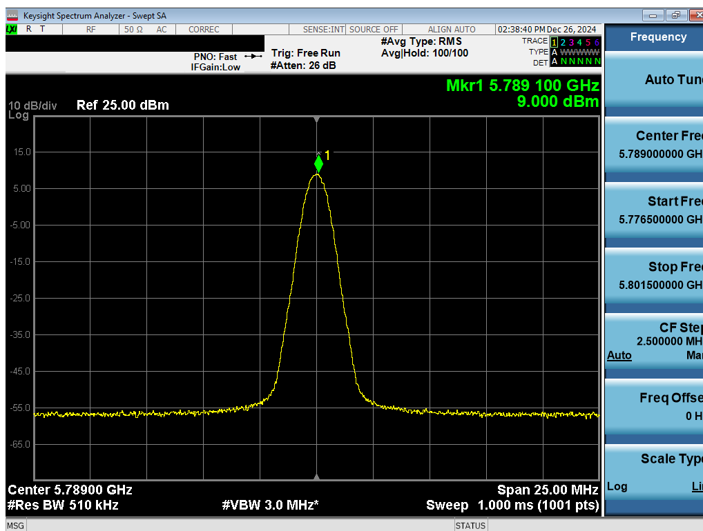
Plot 7-37. PSD Antenna 3a (NB UNII BDR, ePA – 5789MHz)
