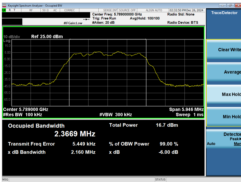
Plot 7-14. 6dB BW & 99% OBW Antenna 3a (NB UNII HDR4, ePA – 5789MHz)
