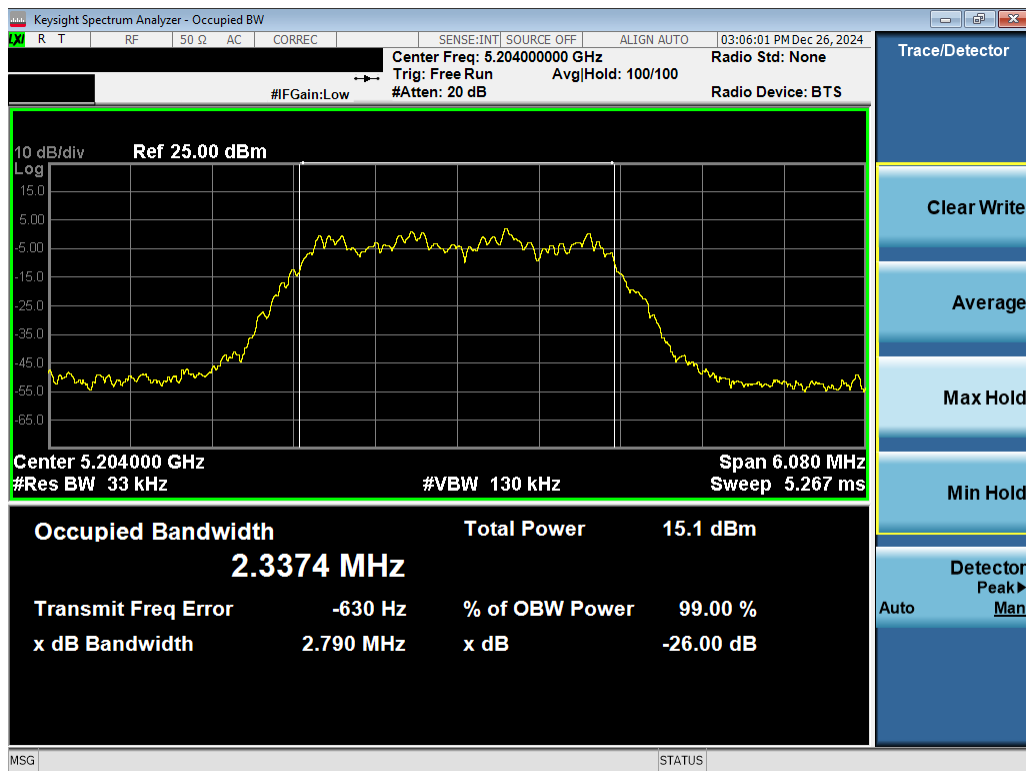
Plot 7-8. 26dB BW & 99% OBW Antenna 1b (NB UNII HDR4, ePA- 5204MHz)
