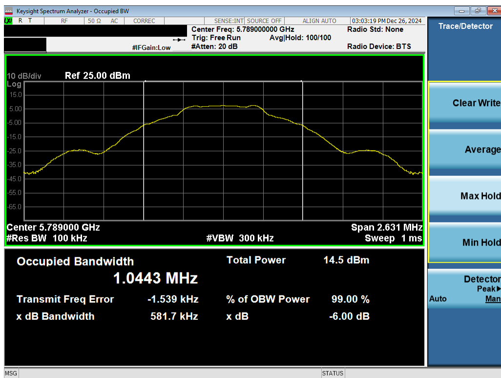
Plot 7-16. 6dB BW & 99% OBW Antenna 1b (NB UNII BDR, ePA – 5789MHz)
