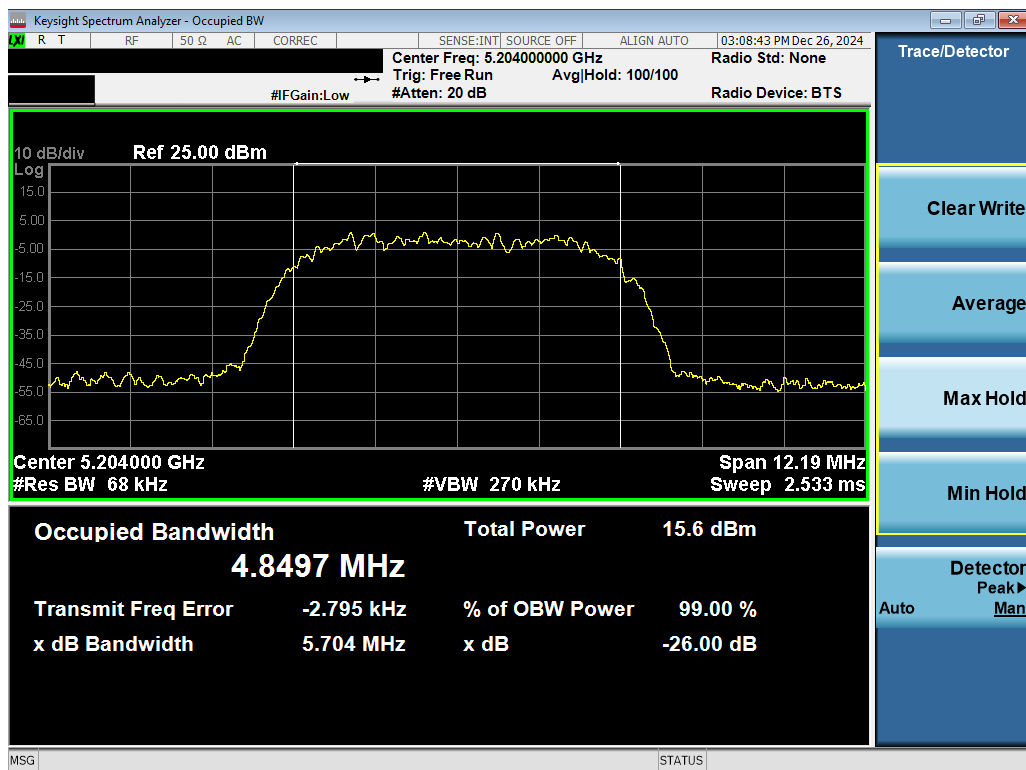
Plot 7-9. 26dB BW & 99% OBW Antenna 1b (NB UNII HDR8, ePA- 5204MHz)
