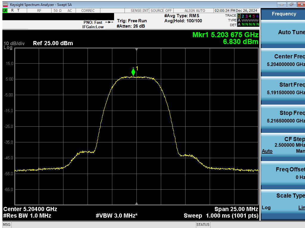
Plot 7-23. PSD Antenna 3c (NB UNII HDR8, ePA – 5204MHz)
