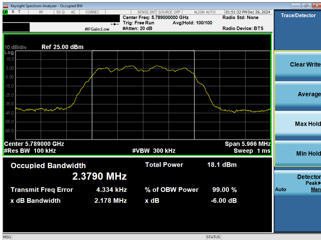
Plot 7-11. 6dB BW & 99% OBW Antenna 3c (NB UNII HDR4, ePA – 5789MHz)
