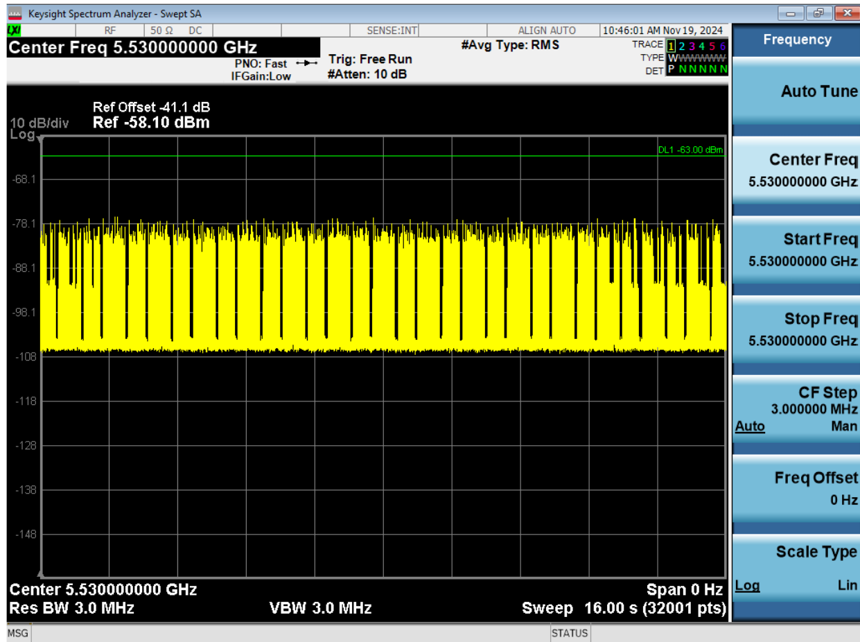
Figure 9-7. 5530MHz - Channel Loading - Mode 3 (80MHz)
