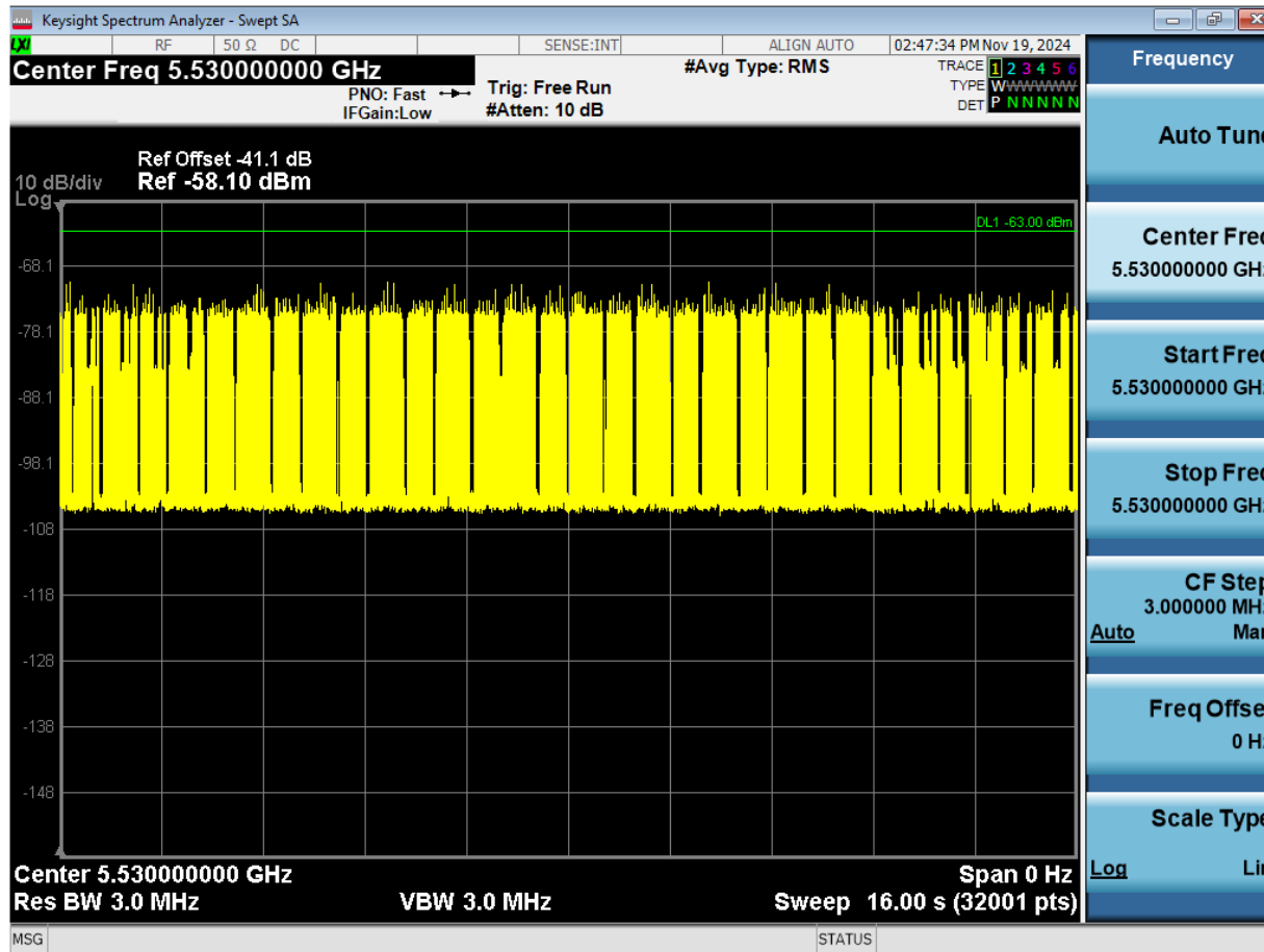
Figure 9-9. 5530 MHz - Channel Loading - Mode 4 (80MHz)
