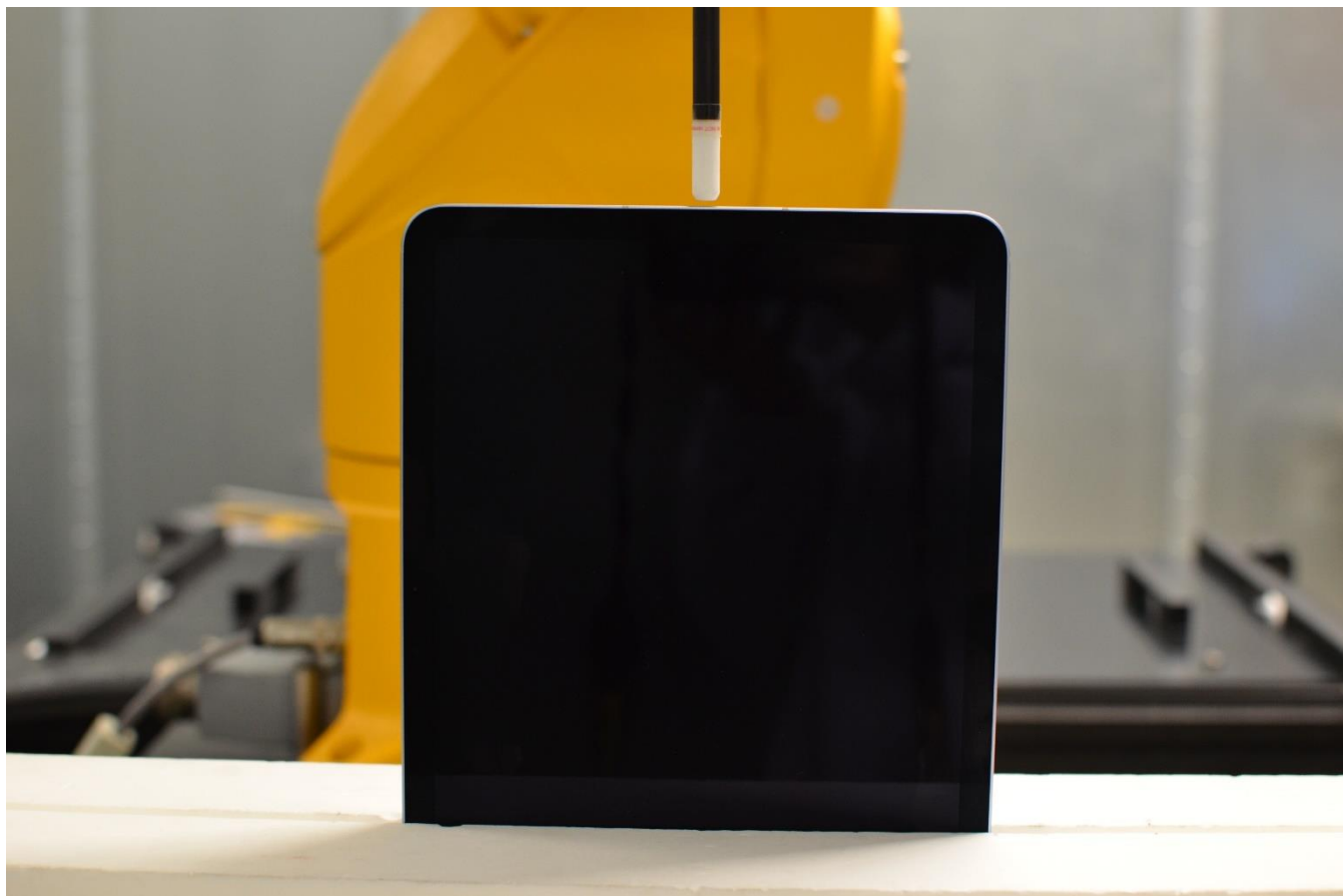
Near Field Power Density Test Setup 18: Bottom Edge at 2mm – Antenna 1b/3a/3c
