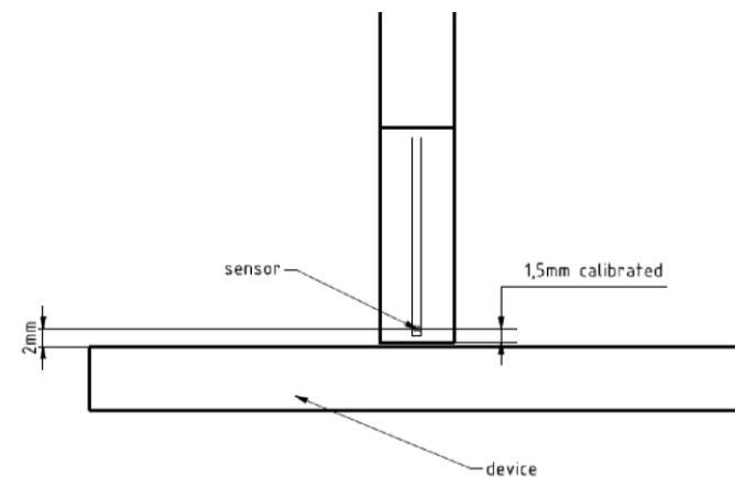
Figure J-2 EUMmWVx Probe
