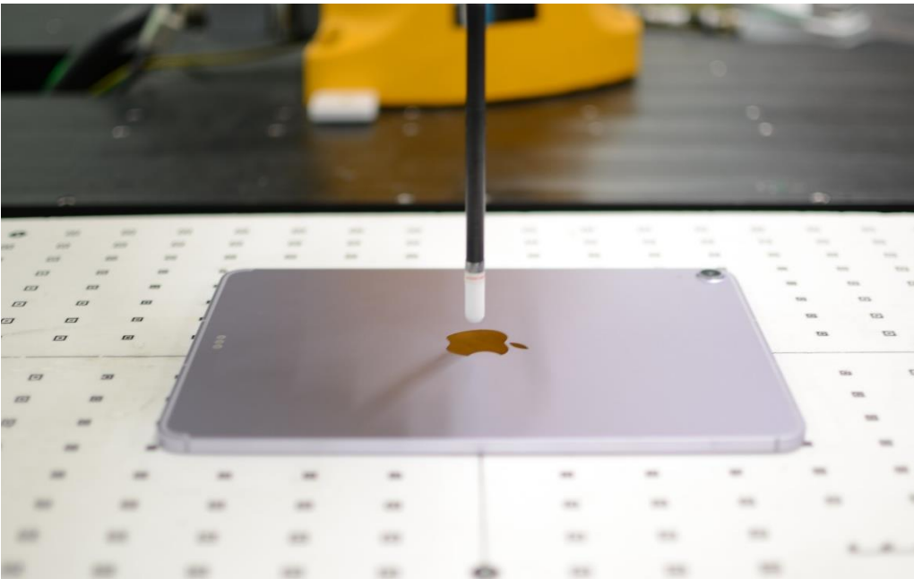
Near Field Power Density Test Setup 15: Back Side at 8.58mm – Antenna 1b/3a
