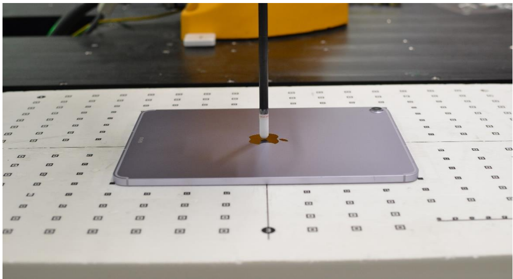
Near Field Power Density Test Setup 14: Back Side at 2mm – Antenna 1b/3a/3c
