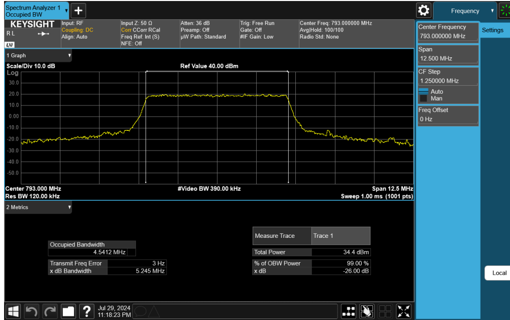
Plot 7-17. Occupied Bandwidth Plot (LTE Band 14 - 5MHz QPSK - Full RB)
