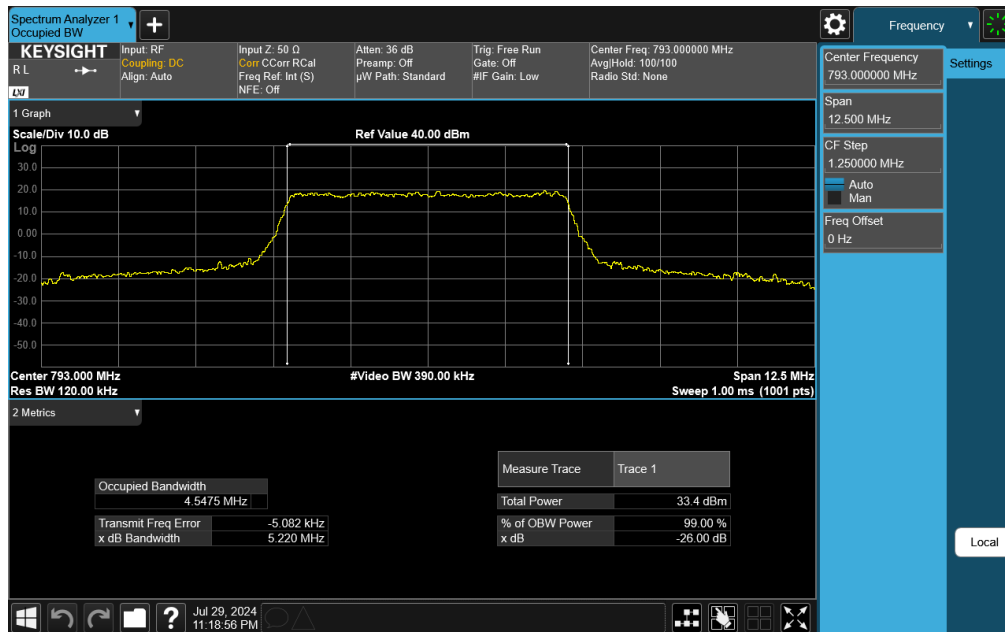
Plot 7-18. Occupied Bandwidth Plot (LTE Band 14 - 5MHz 16-QAM - Full RB)
