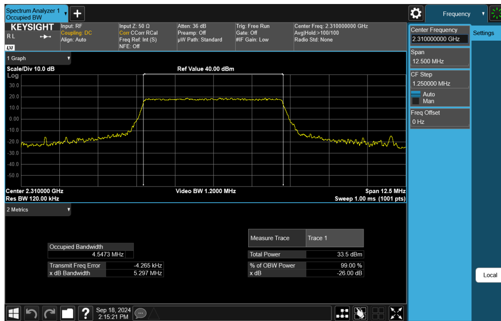
Plot 7-1. Occupied Bandwidth Plot (LTE Band 30 - 5MHz QPSK - Full RB)
