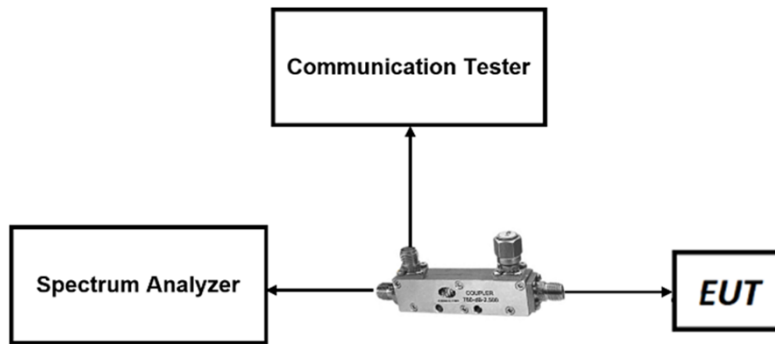
Figure 7-1. LTE Test Instrument & Measurement Setup
