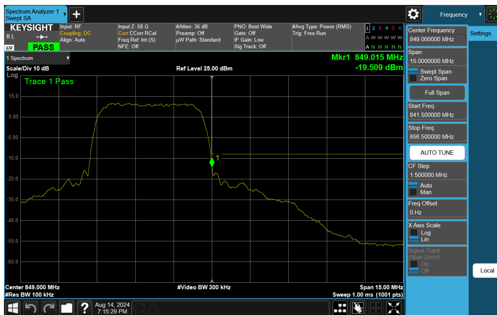
Plot 7-113. Upper BE Plot (WCDMA Cell – Ch. 4233)
