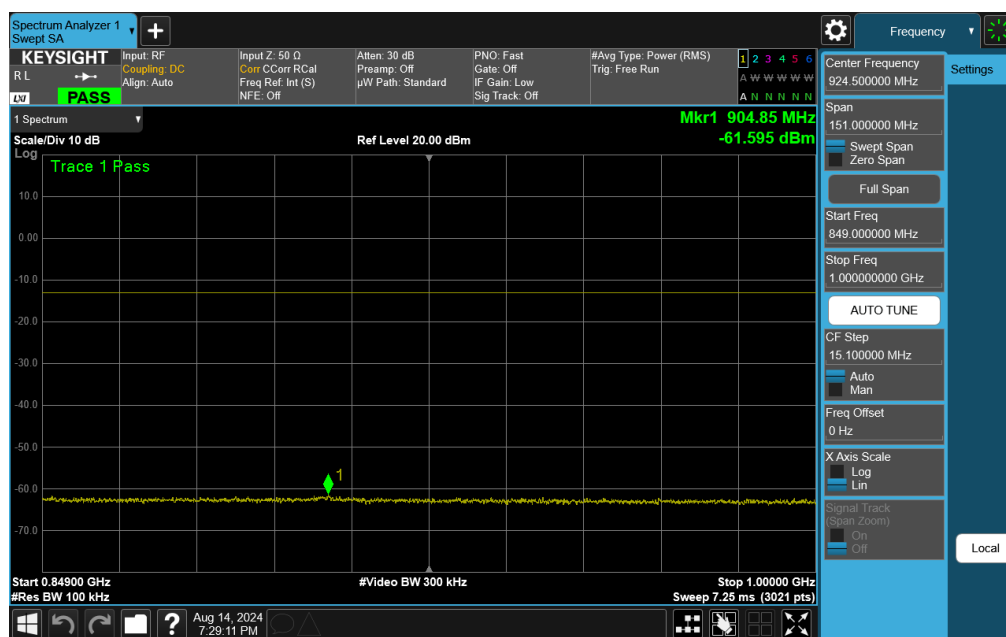
Plot 7-70. Conducted Spurious Plot (WCDMA Ch. 4132)
