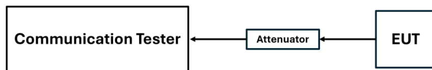
Figure 7-7. LTE Test Instrument & Measurement Setup
