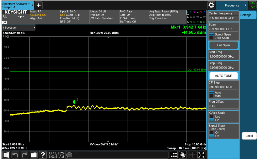
Plot 7-68. Conducted Spurious Plot (NR Band n26/n5 - 20.0MHz DFT-s-OFDM QPSK - RB Size 1, RB Offset 0 - High Channel)
