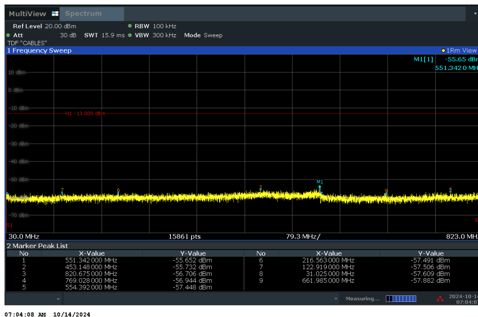
Plot 7-42. Conducted Spurious Plot (LTE Band 26/5 - 10MHz QPSK - RB Size 1, RB Offset 0 - Low Channel)
