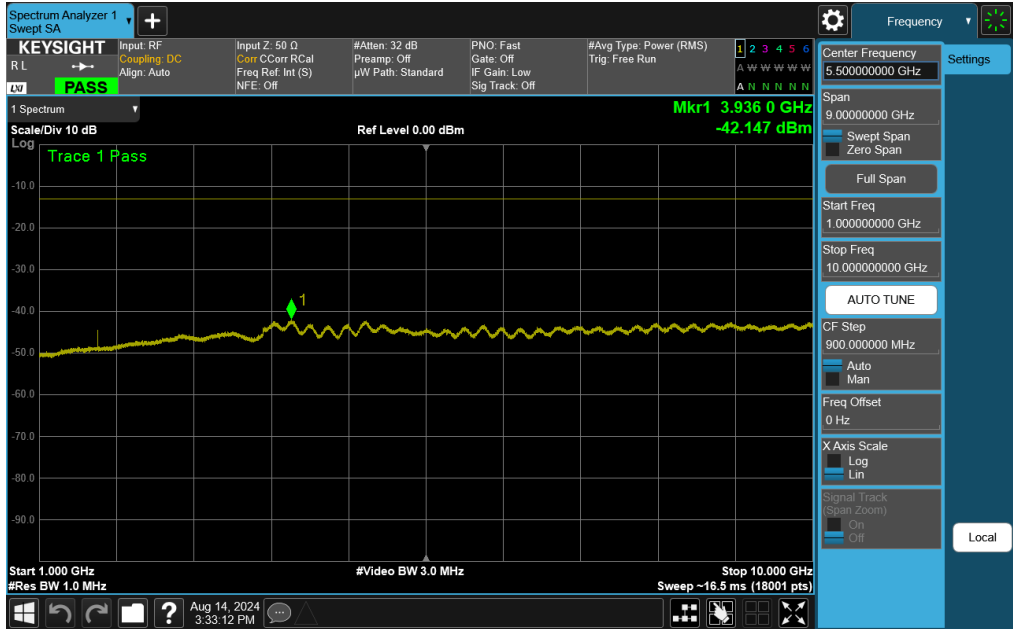
Plot 7-59. Conducted Spurious Plot (ULCA LTE Band 5 – (10 + 10)MHz QPSK – PCC 1/0 SCC 1/49 - High Channel)
