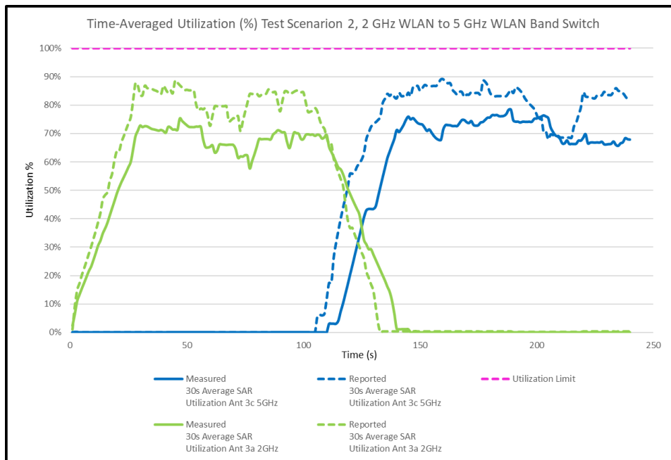
Figure K-7 30s Average Utilization vs. Time during Band Switch
