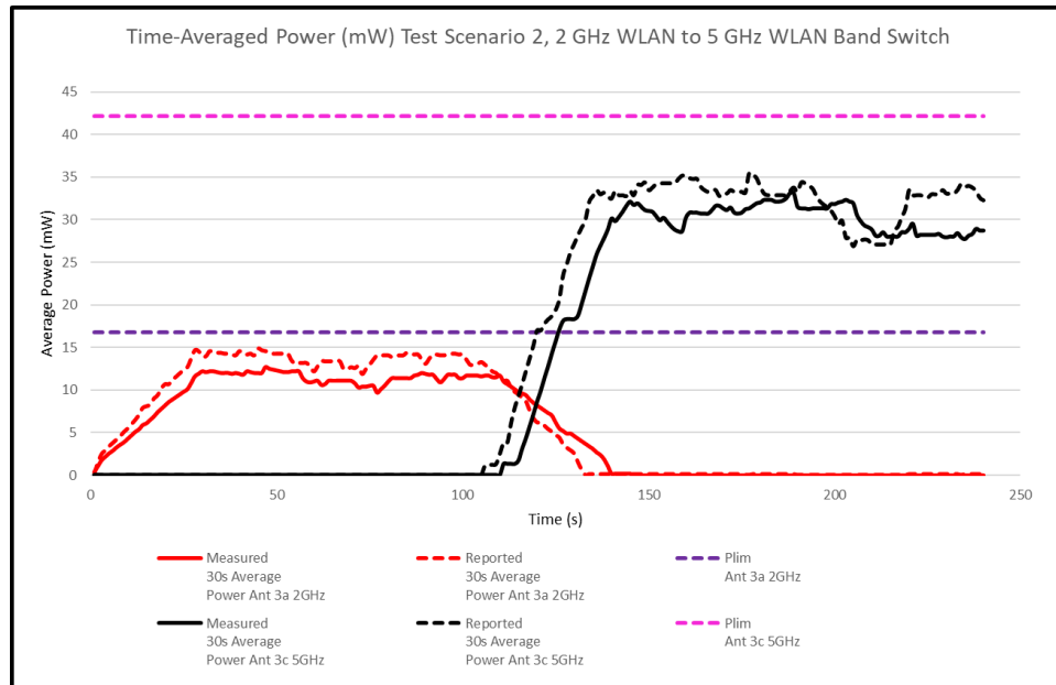
Figure K-8 30s Average Power vs. Time during Band Switch
