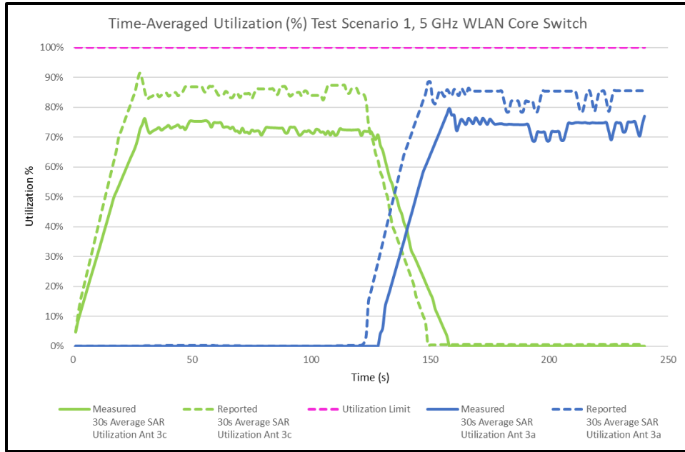
Figure K-3 30s Average SAR Utilization vs. Time, 5 GHz
