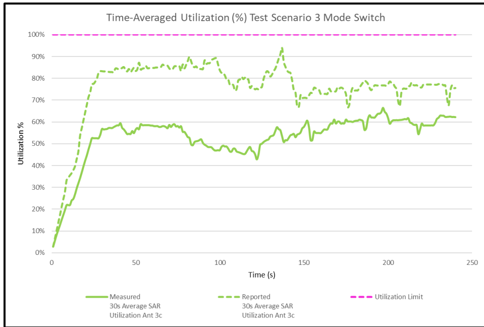
Figure K-9 30s Average Utilization vs. Time during Mode Switch
