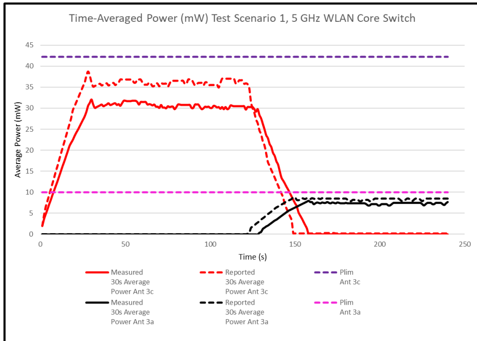
Figure K-4 30s Average Power vs. Time, 5 GHz
