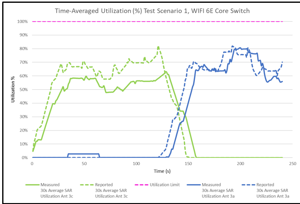
Figure K-5 30s Average SAR Utilization vs. Time, 6 GHz
