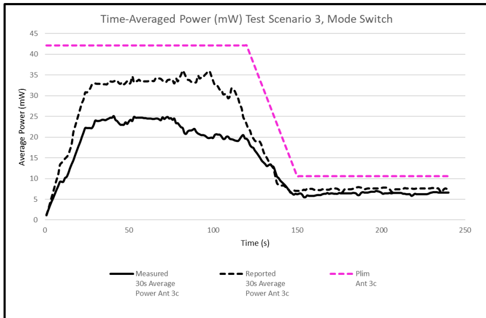
Figure K-10 30s Average Power vs. Time during Mode Switch
