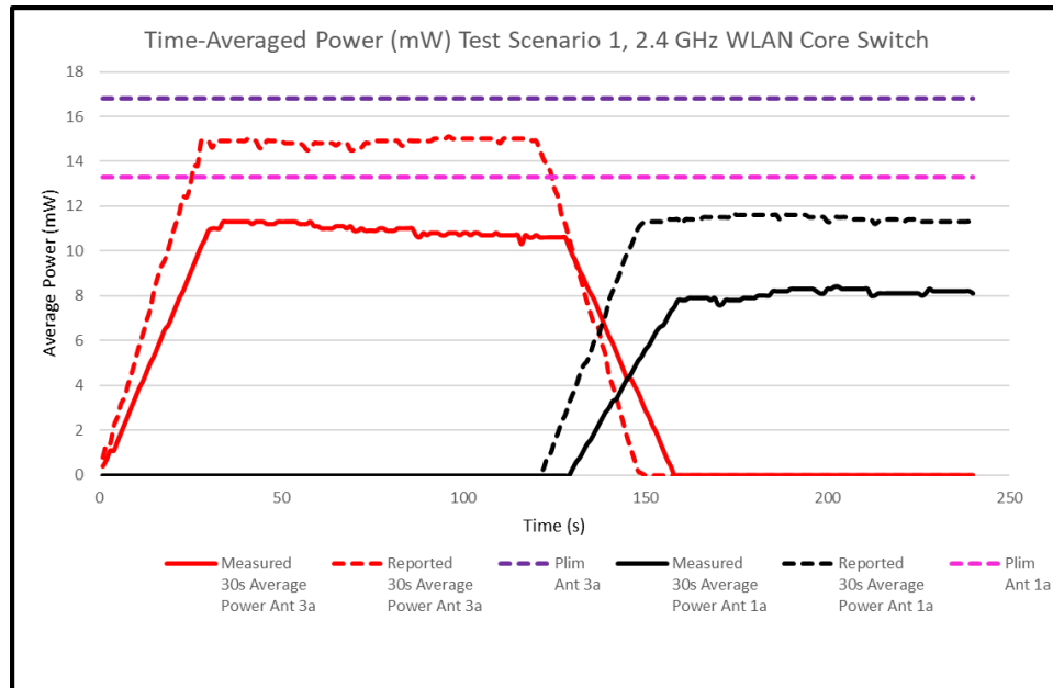
Figure K-2 30s Average Power vs. Time, 2.4 GHz
