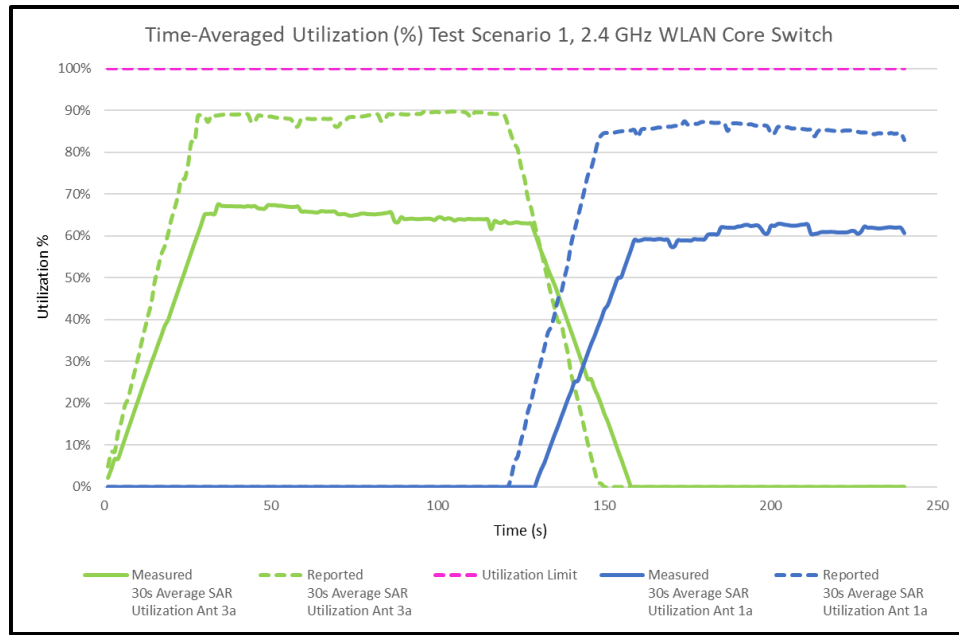
Figure K-1 30s Average SAR Utilization vs. Time, 2.4 GHz
