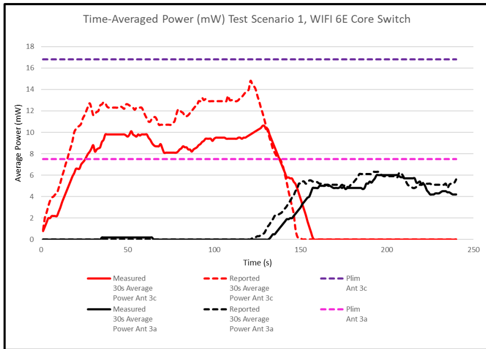
Figure K-6 30s Average Power vs. Time, 6 GHz
