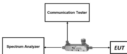
Figure 7-5. LTE Test Instrument & Measurement Setup
