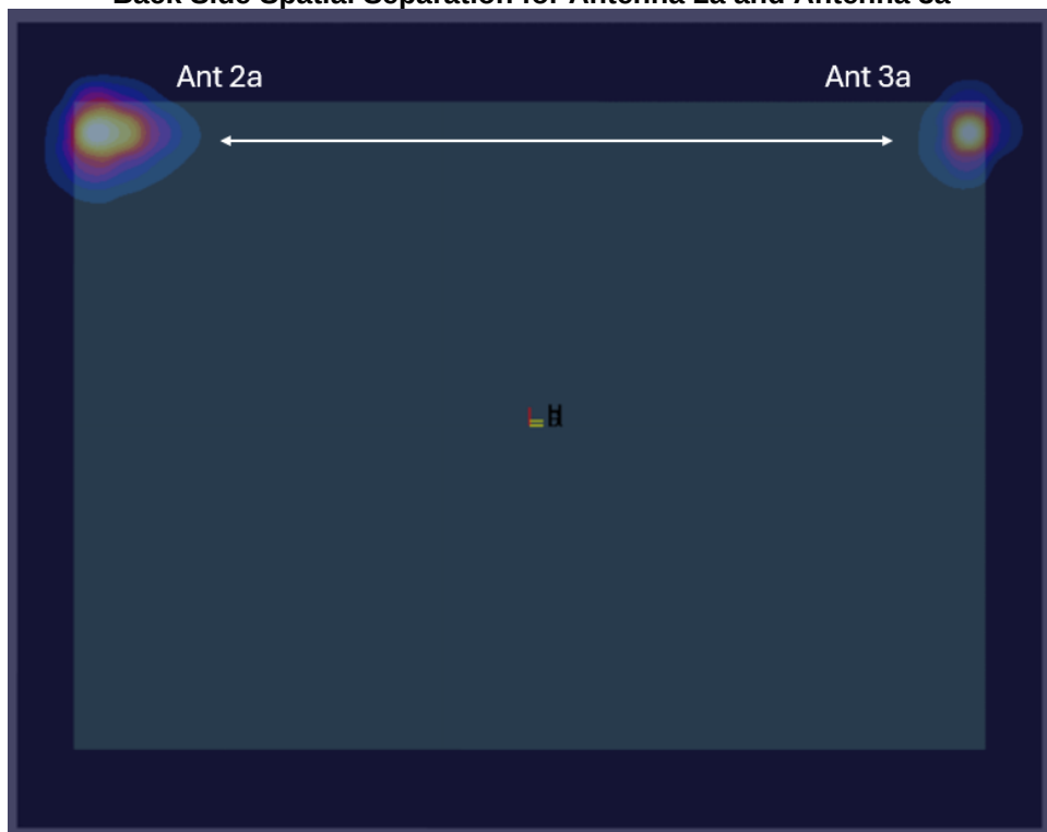
Figure E-15 Back Side Spatial Separation for Antenna 2a and Antenna 3a
