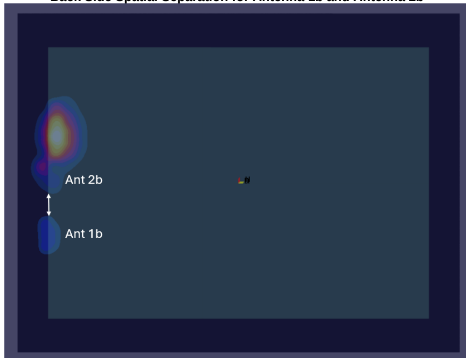
Figure E-9 Back Side Spatial Separation for Antenna 1b and Antenna 2b
