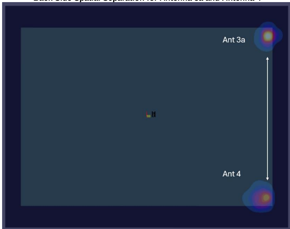
Figure E-21 Back Side Spatial Separation for Antenna 3a and Antenna 4
