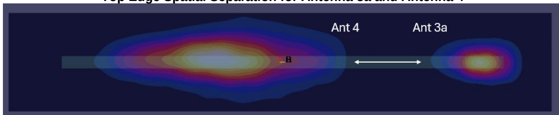
Figure E-28 Top Edge Spatial Separation for Antenna 3a and Antenna 4
