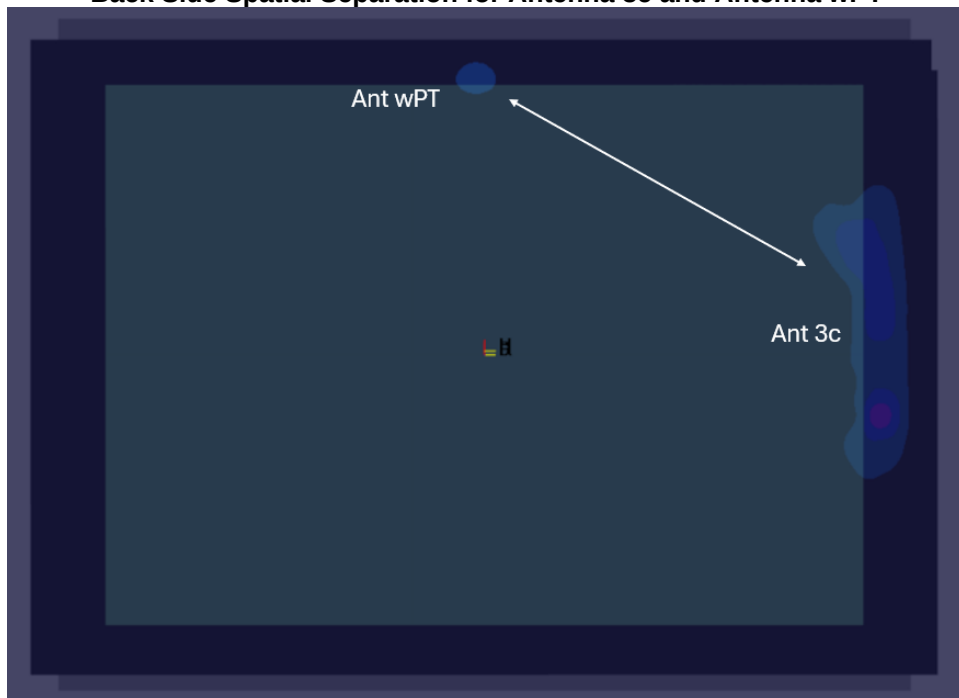
Figure E-25 Back Side Spatial Separation for Antenna 3c and Antenna wPT
