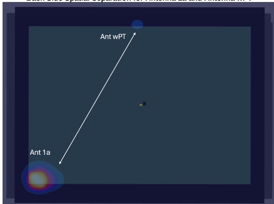
Figure E-7 Back Side Spatial Separation for Antenna 1a and Antenna wPT
