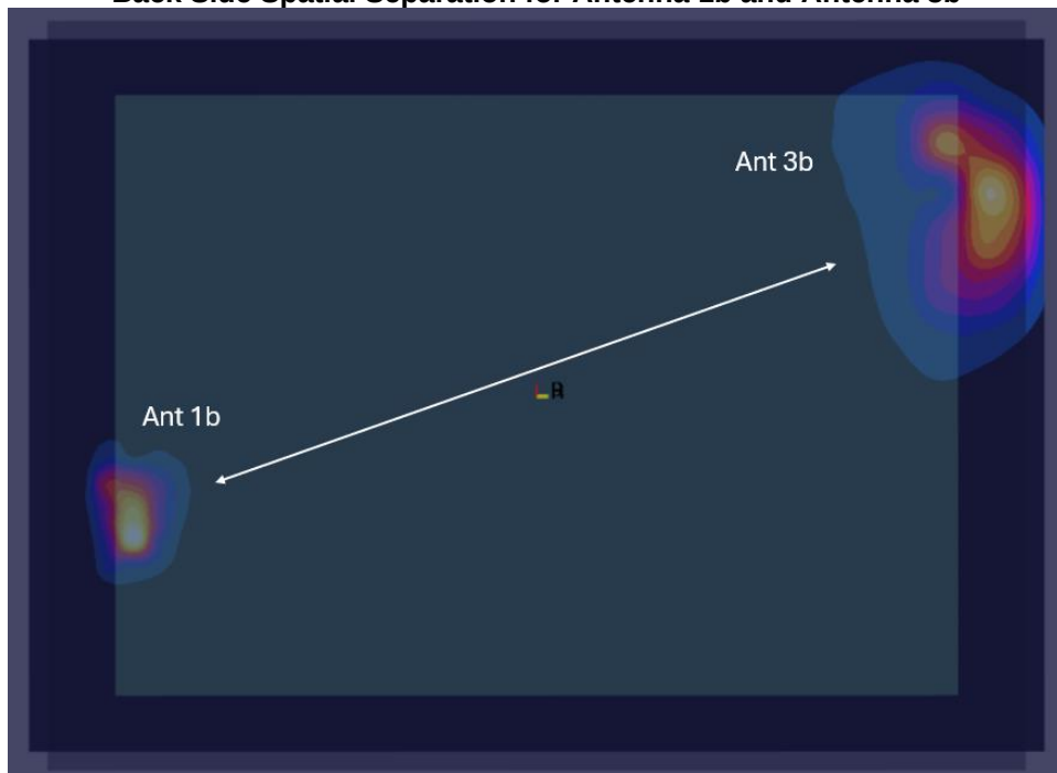
Figure E-11 Back Side Spatial Separation for Antenna 1b and Antenna 3b
