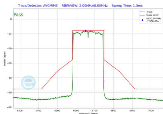
Plot 7-58. In-Band Emission Plot Antenna WF8 (160MHz 802.11ax (UNII Band 7) – Ch. 143)
