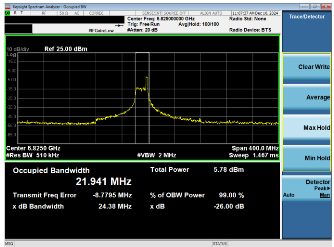
Plot 7-44. 26dB & 99% Bandwidth Plot Antenna WF8 (160MHz 802.11ax RU26 (UNII Band 7) – Ch. 175)
