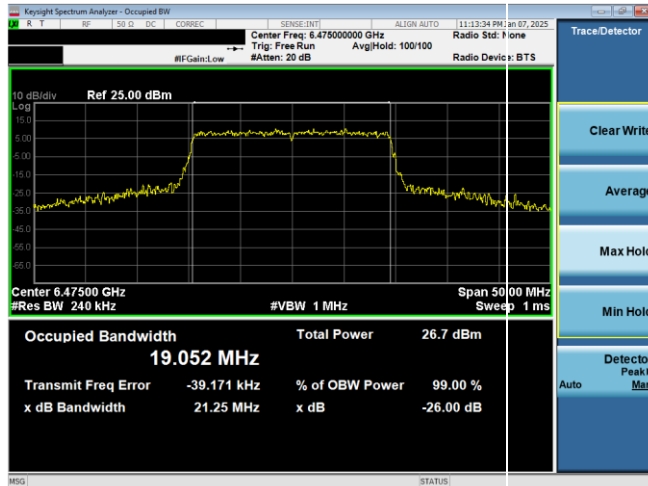
Plot 7-13. 26dB & 99% Bandwidth Plot Antenna WF8 (20MHz 802.11ax RU242 (UNII Band 6) – Ch. 105)
