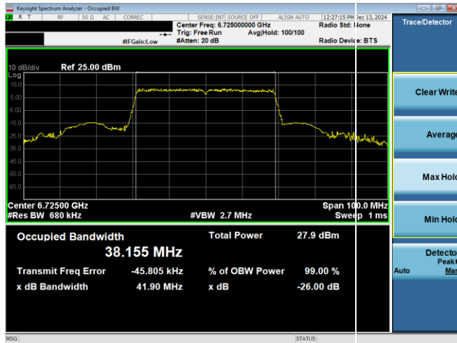
Plot 7-22. 26dB & 99% Bandwidth Plot Antenna WF8 (40MHz 802.11ax RU484 (UNII Band 7) – Ch. 155)
