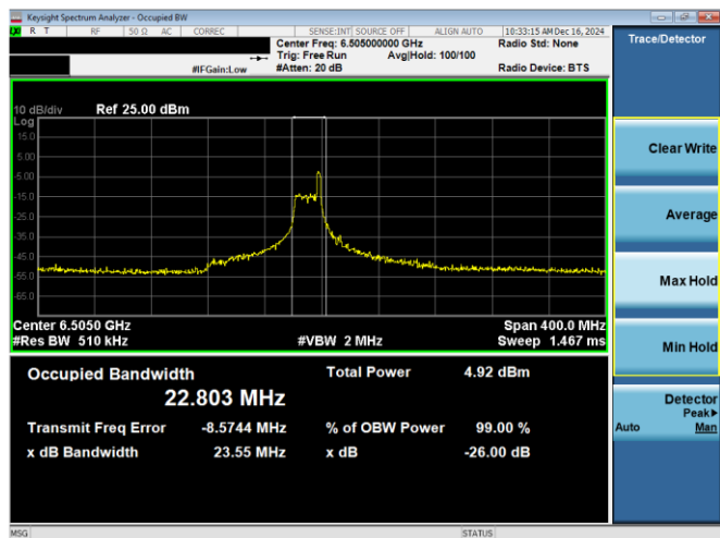
Plot 7-36. 26dB & 99% Bandwidth Plot Antenna WF8 (160MHz 802.11ax RU26 (UNII Band 6) – Ch. 111)
