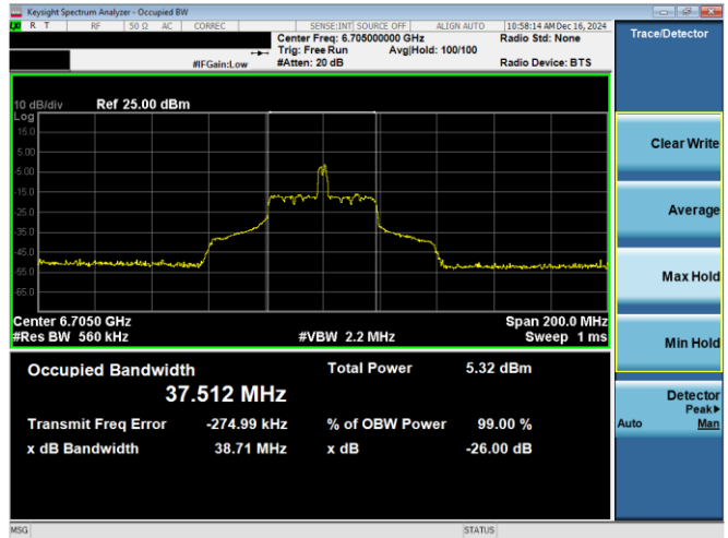
Plot 7-43. 26dB & 99% Bandwidth Plot Antenna WF8 (80MHz 802.11ax RU26 (UNII Band 7) – Ch. 151)
