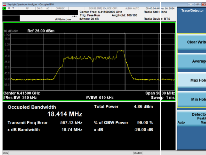
Plot 7-25. 26dB & 99% Bandwidth Plot Antenna WF8 (20MHz 802.11ax RU26 (UNII Band 5) – Ch. 93)
