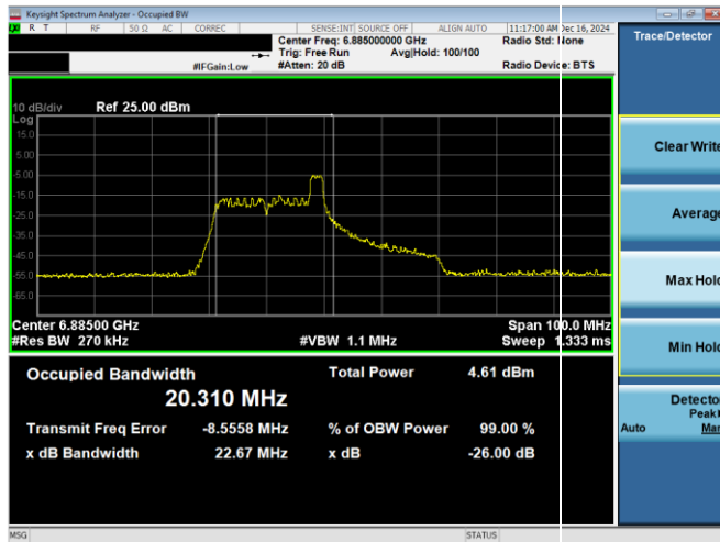
Plot 7-50. 26dB & 99% Bandwidth Plot Antenna WF8 (40MHz 802.11ax RU26 (UNII Band 8) – Ch. 187)
