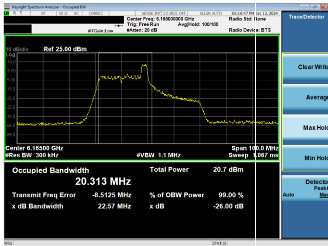
Plot 7-58. 26dB & 99% Bandwidth Plot Antenna WF7a (40MHz 802.11ax RU26 (UNII Band 5) – Ch. 43)
