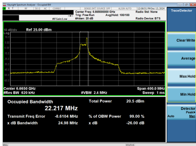
Plot 7-20. 26dB & 99% Bandwidth Plot Antenna WF8 (160MHz 802.11ax RU26 (UNII Band 7) – Ch. 143)
