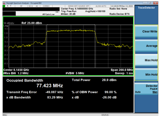
Plot 7-7. 26dB & 99% Bandwidth Plot Antenna WF8 (80MHz 802.11ax RU996 (UNII Band 5) – Ch. 39)
