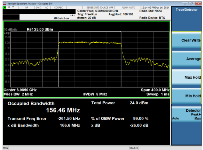
Plot 7-56. 26dB & 99% Bandwidth Plot Antenna WF8 (160MHz 802.11ax RU996x2 (UNII Band 8) – Ch. 207)
