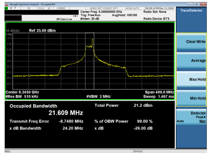
Plot 7-60. 26dB & 99% Bandwidth Plot Antenna WF7a (160MHz 802.11ax RU26 (UNII Band 5) – Ch. 79)
