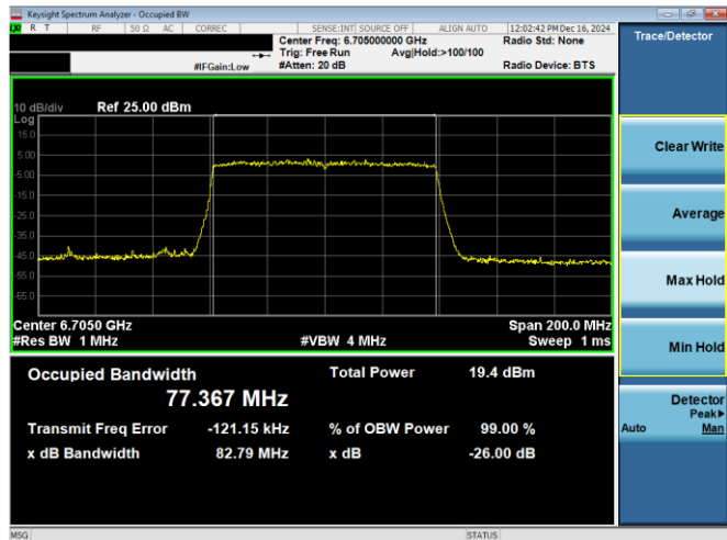
Plot 7-47. 26dB & 99% Bandwidth Plot Antenna WF8 (80MHz 802.11ax RU996 (UNII Band 7) – Ch. 151)
