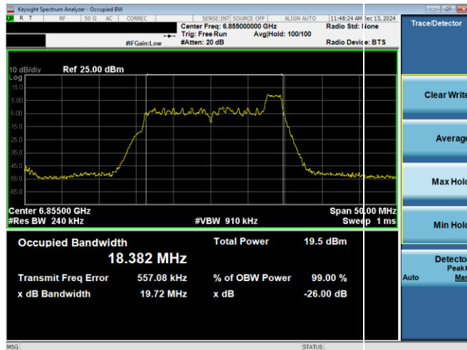
Plot 7-17. 26dB & 99% Bandwidth Plot Antenna WF8 (20MHz 802.11ax RU26 (UNII Band 7) – Ch. 181)
