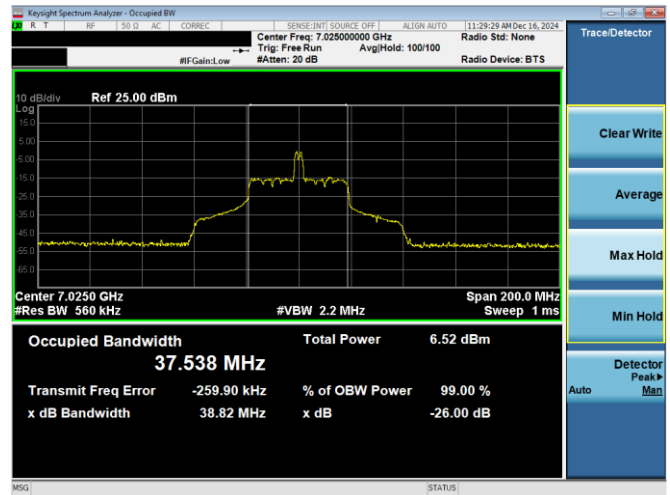
Plot 7-51. 26dB & 99% Bandwidth Plot Antenna WF8 (80MHz 802.11ax RU26 (UNII Band 8) – Ch. 215)
