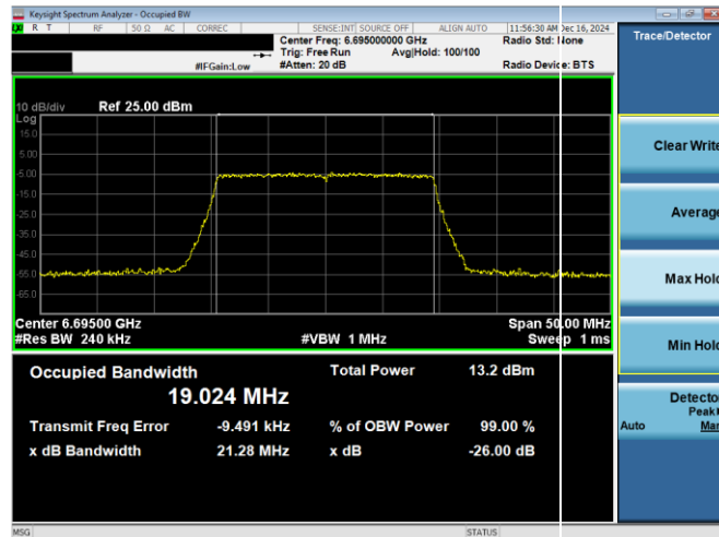
Plot 7-45. 26dB & 99% Bandwidth Plot Antenna WF8 (20MHz 802.11ax RU242 (UNII Band 7) – Ch. 149)
