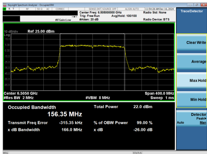
Plot 7-40. 26dB & 99% Bandwidth Plot Antenna WF8 (160MHz 802.11ax RU996x2 (UNII Band 6) – Ch. 111)
