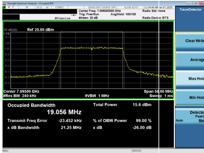
Plot 7-53. 26dB & 99% Bandwidth Plot Antenna WF8 (20MHz 802.11ax RU242 (UNII Band 8) – Ch. 229)
