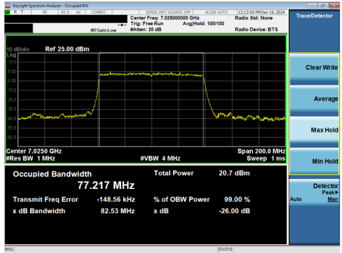
Plot 7-55. 26dB & 99% Bandwidth Plot Antenna WF8 (80MHz 802.11ax RU996 (UNII Band 8) – Ch. 215)
