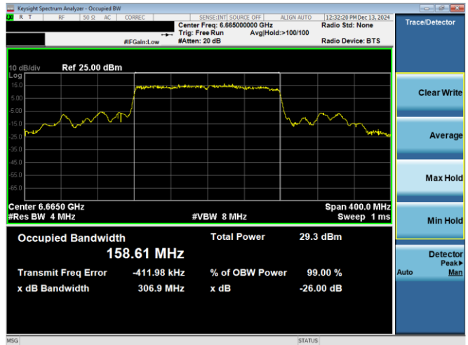
Plot 7-24. 26dB & 99% Bandwidth Plot Antenna WF8 (160MHz 802.11ax RU996x2 (UNII Band 7) – Ch. 143)
