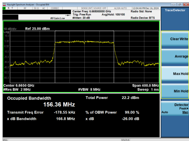
Plot 7-48. 26dB & 99% Bandwidth Plot Antenna WF8 (160MHz 802.11ax RU996x2 (UNII Band 7) – Ch. 143)
