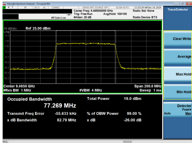
Plot 7-39. 26dB & 99% Bandwidth Plot Antenna WF8 (80MHz 802.11ax RU996 (UNII Band 6) – Ch. 103)
