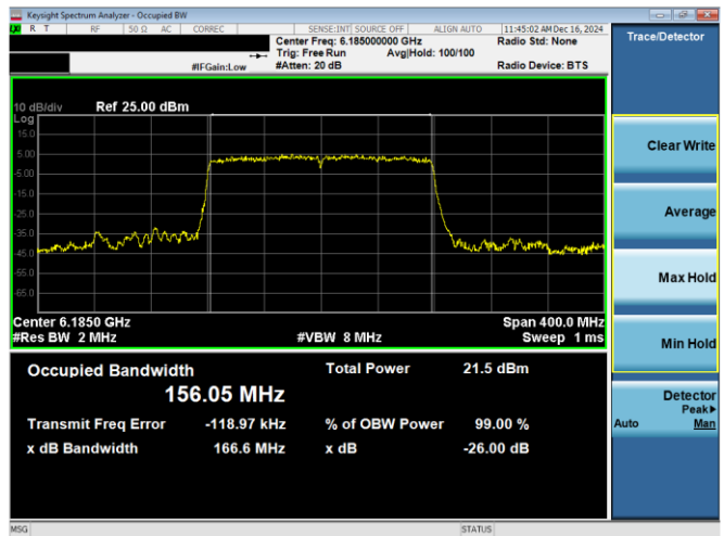
Plot 7-32. 26dB & 99% Bandwidth Plot Antenna WF8 (160MHz 802.11ax RU996x2 (UNII Band 5) – Ch. 47)
