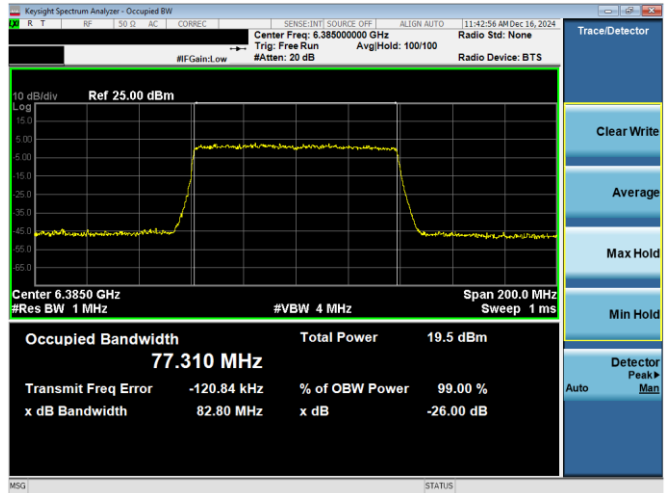
Plot 7-31. 26dB & 99% Bandwidth Plot Antenna WF8 (80MHz 802.11ax RU996 (UNII Band 5) – Ch. 87)
