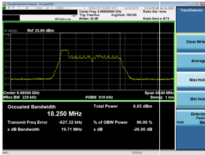
Plot 7-49. 26dB & 99% Bandwidth Plot Antenna WF8 (20MHz 802.11ax RU26 (UNII Band 8) – Ch. 209)
