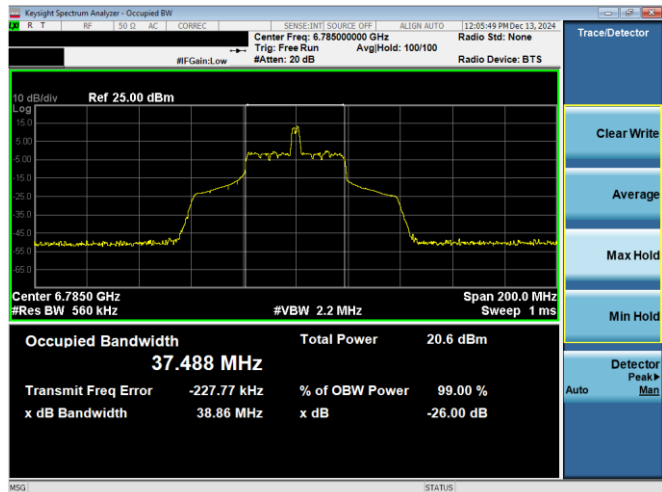
Plot 7-19. 26dB & 99% Bandwidth Plot Antenna WF8 (80MHz 802.11ax RU26 (UNII Band 7) – Ch. 167)
