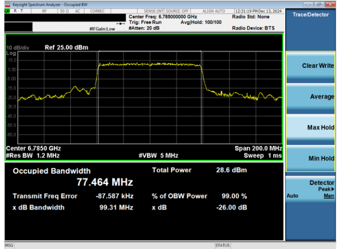
Plot 7-23. 26dB & 99% Bandwidth Plot Antenna WF8 (80MHz 802.11ax RU996 (UNII Band 7) – Ch. 167)
