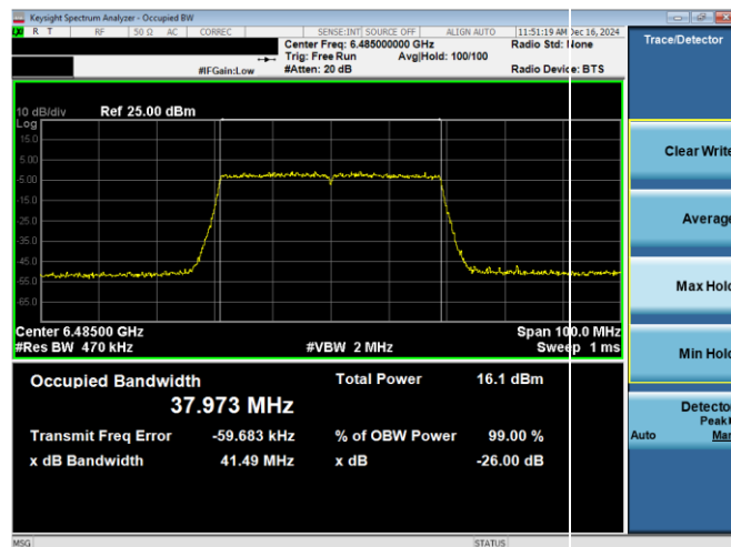
Plot 7-38. 26dB & 99% Bandwidth Plot Antenna WF8 (40MHz 802.11ax RU484 (UNII Band 6) – Ch. 107)
