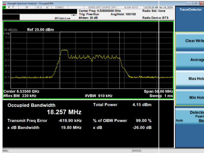
Plot 7-41. 26dB & 99% Bandwidth Plot Antenna WF8 (20MHz 802.11ax RU26 (UNII Band 7) – Ch. 117)
