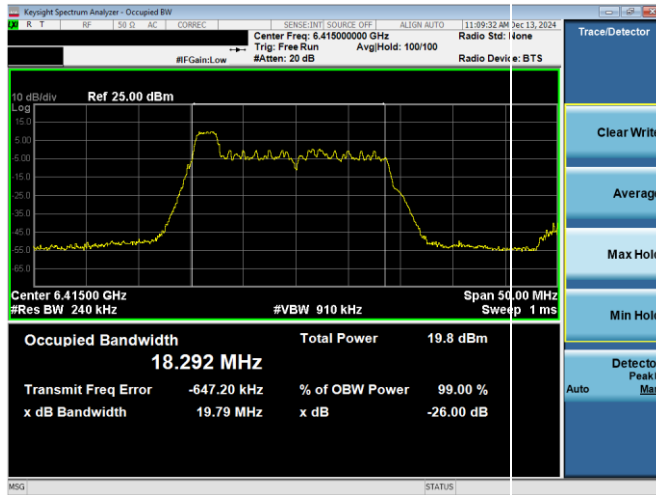
Plot 7-1. 26dB & 99% Bandwidth Plot Antenna WF8 (20MHz 802.11ax RU26 (UNII Band 5) – Ch. 93)
