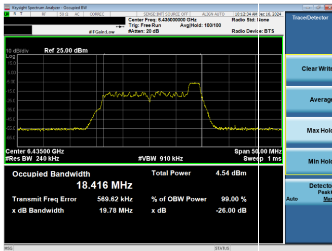
Plot 7-33. 26dB & 99% Bandwidth Plot Antenna WF8 (20MHz 802.11ax RU26 (UNII Band 6) – Ch. 97)
