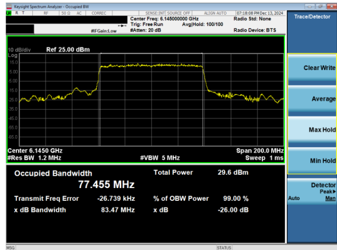
Plot 7-63. 26dB & 99% Bandwidth Plot Antenna WF7a (80MHz 802.11ax RU996 (UNII Band 5) – Ch. 39)
