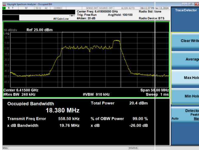
Plot 7-57. 26dB & 99% Bandwidth Plot Antenna WF7a (20MHz 802.11ax RU26 (UNII Band 5) – Ch. 93)
