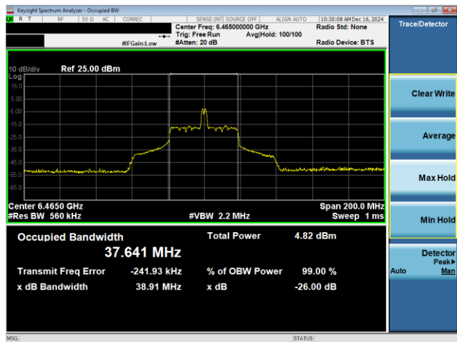
Plot 7-35. 26dB & 99% Bandwidth Plot Antenna WF8 (80MHz 802.11ax RU26 (UNII Band 6) – Ch. 103)
