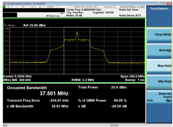
Plot 7-59. 26dB & 99% Bandwidth Plot Antenna WF7a (80MHz 802.11ax RU26 (UNII Band 5) – Ch. 87)
