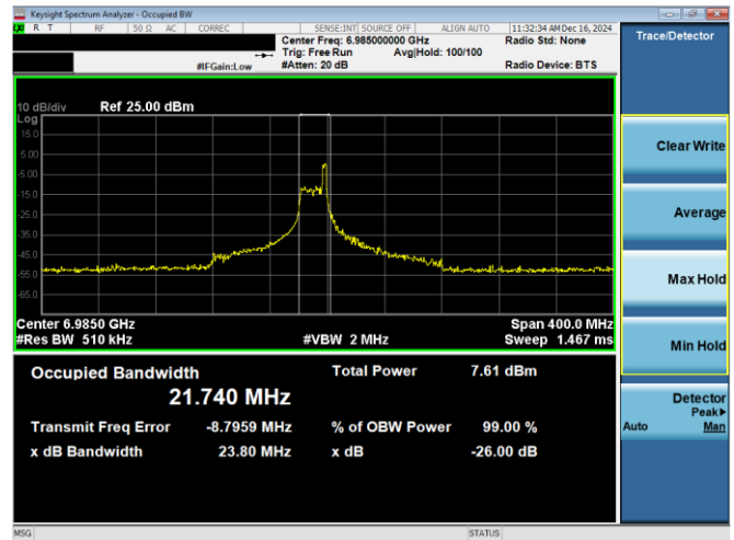
Plot 7-52. 26dB & 99% Bandwidth Plot Antenna WF8 (160MHz 802.11ax RU26 (UNII Band 8) – Ch. 207)
