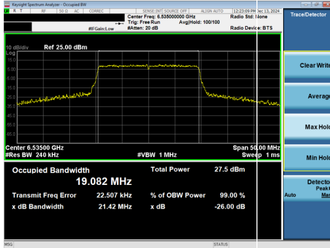
Plot 7-21. 26dB & 99% Bandwidth Plot Antenna WF8 (20MHz 802.11ax RU242 (UNII Band 7) – Ch. 117)
