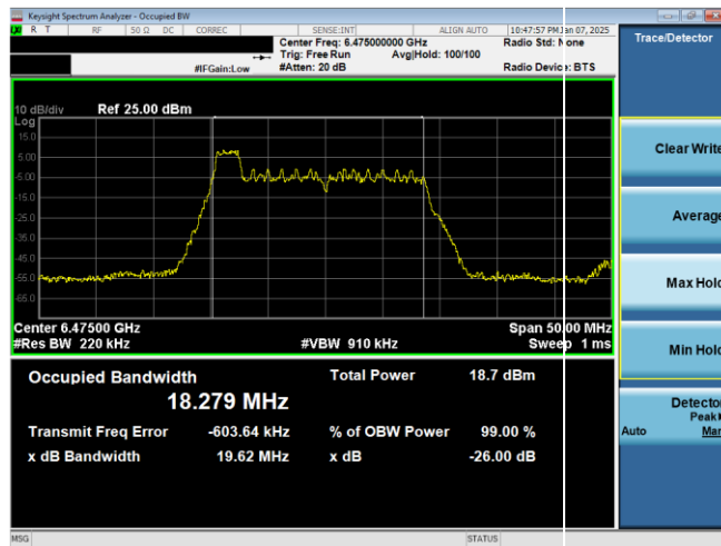
Plot 7-9. 26dB & 99% Bandwidth Plot Antenna WF8 (20MHz 802.11ax RU26 (UNII Band 6) – Ch. 105)
