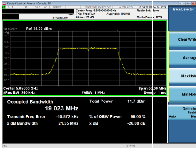
Plot 7-29. 26dB & 99% Bandwidth Plot Antenna WF8 (20MHz 802.11ax RU242 (UNII Band 5) – Ch. 1)
