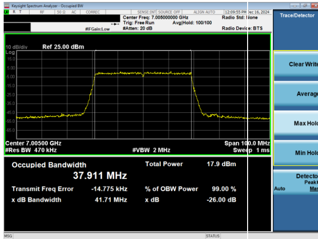
Plot 7-54. 26dB & 99% Bandwidth Plot Antenna WF8 (40MHz 802.11ax RU484 (UNII Band 8) – Ch. 211)
