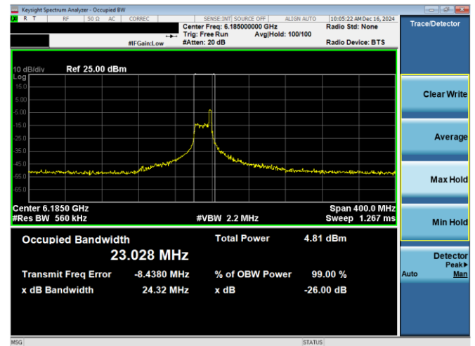
Plot 7-28. 26dB & 99% Bandwidth Plot Antenna WF8 (160MHz 802.11ax RU26 (UNII Band 5) – Ch. 47)
