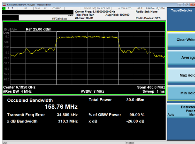
Plot 7-64. 26dB & 99% Bandwidth Plot Antenna WF7a (160MHz 802.11ax RU996x2 (UNII Band 5) – Ch. 47)
