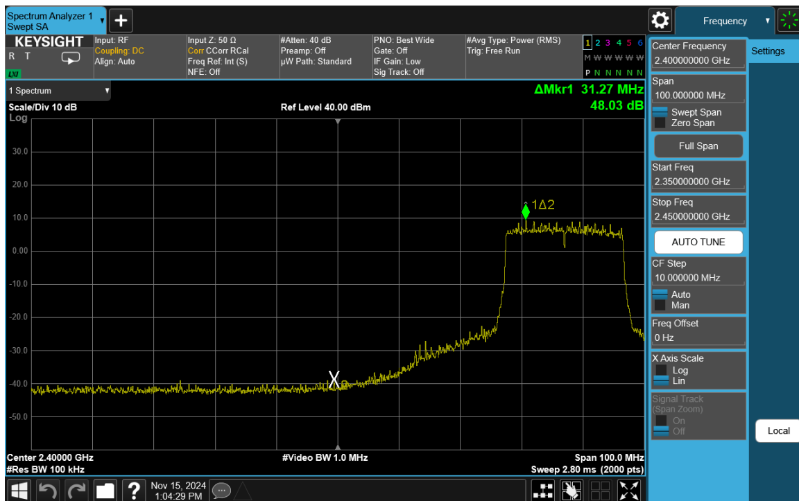
Plot 7-60. Band Edge Plot Antenna WF8 (802.11ax (SU - 2.4GHz) – Ch. 6-Low)
