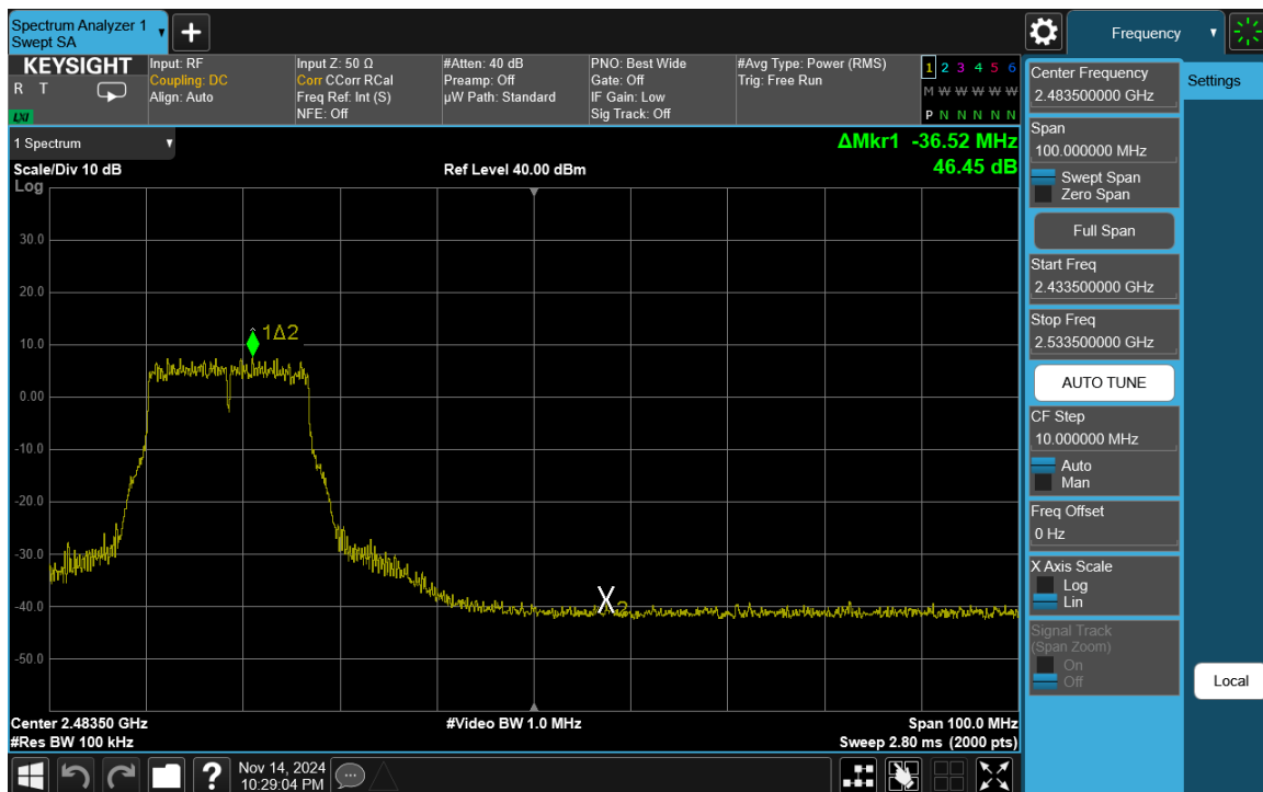
Plot 7-36. Band Edge Plot Antenna WF8 (802.11g – Ch. 9)
