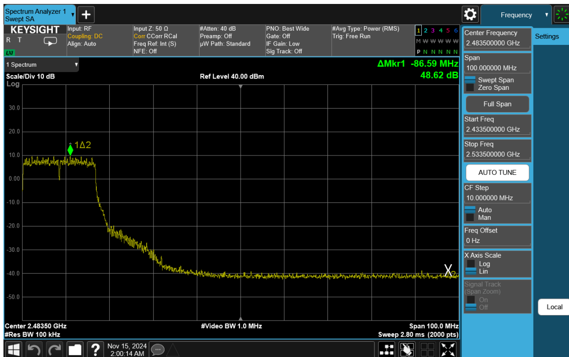
Plot 7-79. Band Edge Plot Antenna WF7b (802.11g – Ch. 7)
