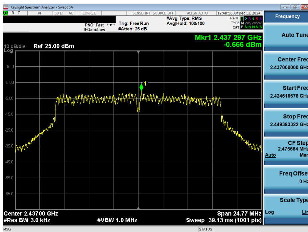
Plot 7-18. Power Spectral Density Plot CDD Antenna WF7b (802.11g – Ch. 6)
