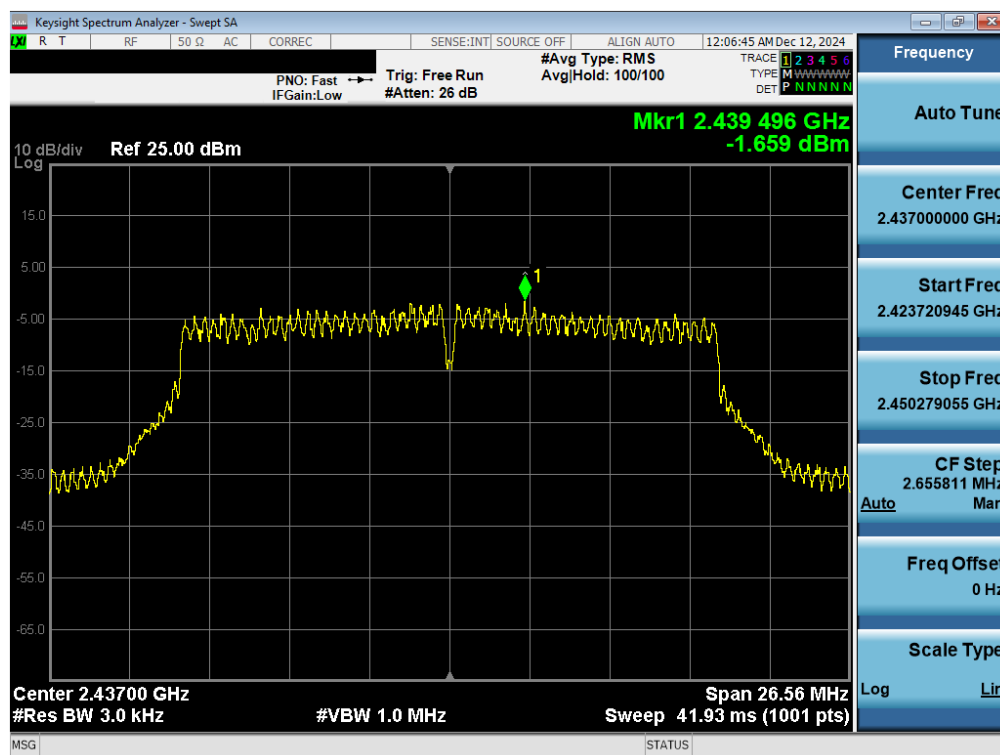
Plot 7-15. Power Spectral Density Plot Antenna WF7b (802.11n – Ch. 6)
