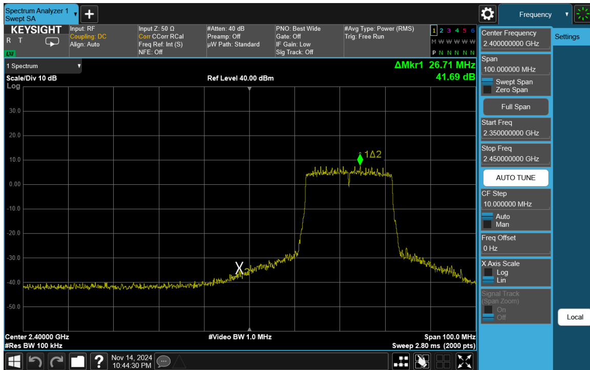
Plot 7-57. Band Edge Plot Antenna WF8 (802.11ax (SU - 2.4GHz) – Ch. 3)
