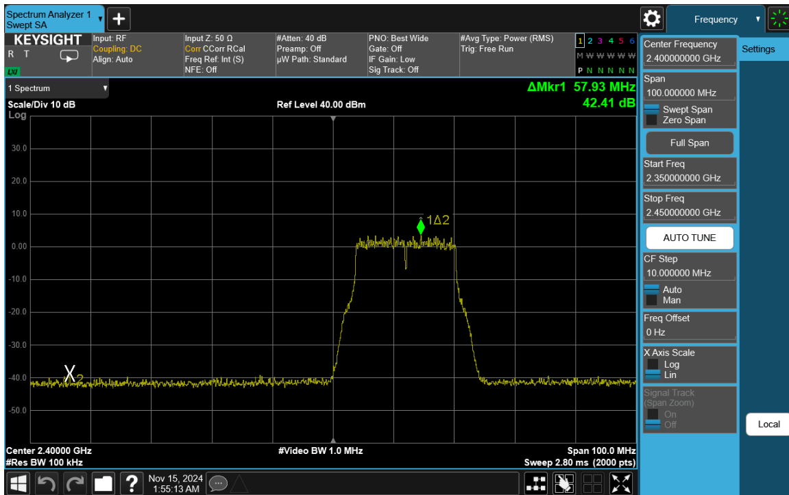
Plot 7-72. Band Edge Plot Antenna WF7b (802.11g – Ch. 1)
