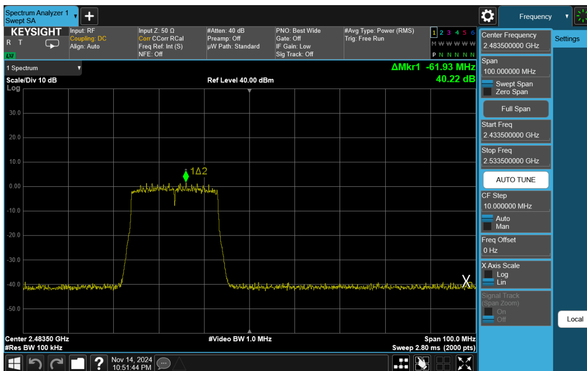
Plot 7-67. Band Edge Plot Antenna WF8 (802.11ax (SU - 2.4GHz) – Ch. 12)
