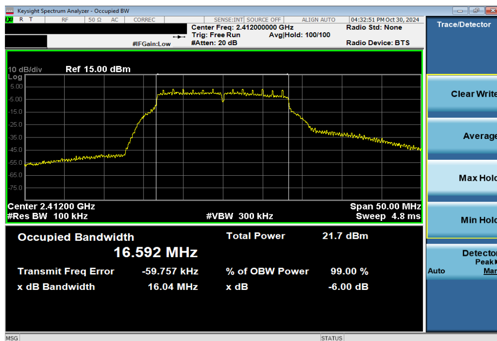
Plot 7-2. 6 dB BW and 99% OBW Plot Antenna WF8 (802.11g – Ch. 1)
