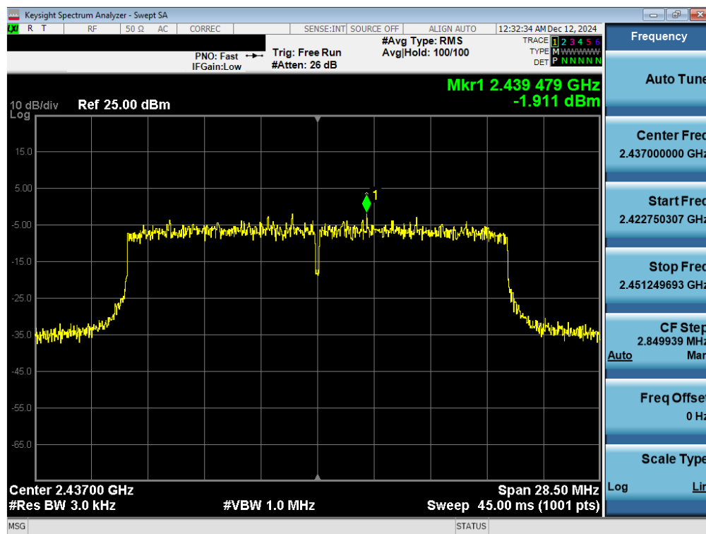
Plot 7-16. Power Spectral Density Plot Antenna WF7b (802.11axSU – Ch. 6)
