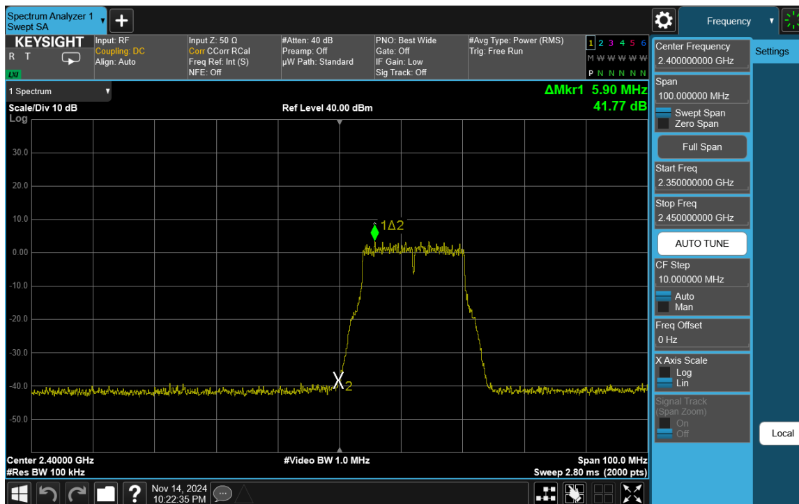
Plot 7-27. Band Edge Plot Antenna WF8 (802.11g – Ch. 1)
