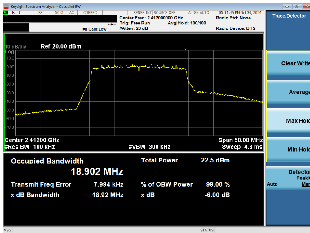
Plot 7-8. 6 dB BW and 99% OBW Plot Antenna WF7b (802.11axSU – Ch. 1)
