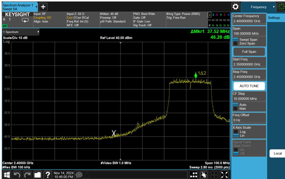
Plot 7-59. Band Edge Plot Antenna WF8 (802.11ax (SU - 2.4GHz) – Ch. 5)
