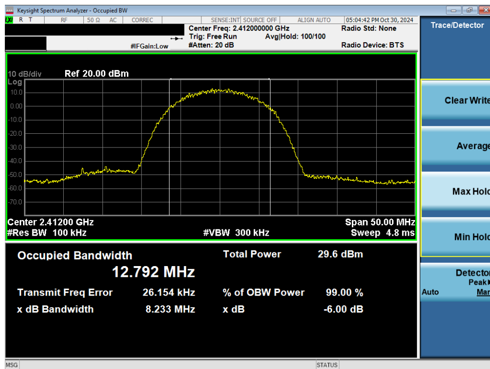
Plot 7-5. 6 dB BW and 99% OBW Plot Antenna WF7b (802.11b – Ch. 1)
