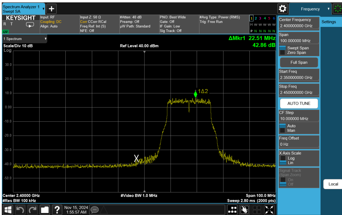
Plot 7-73. Band Edge Plot Antenna WF7b (802.11g – Ch. 2)
