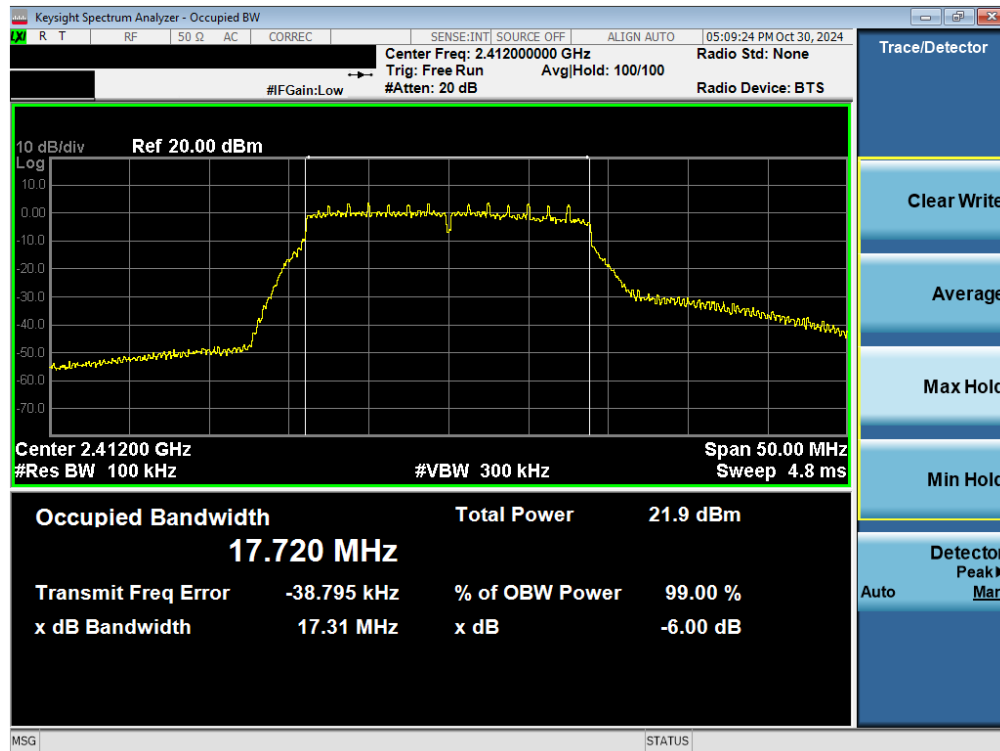
Plot 7-7. 6 dB BW and 99% OBW Plot Antenna WF7b (802.11n – Ch. 1)
