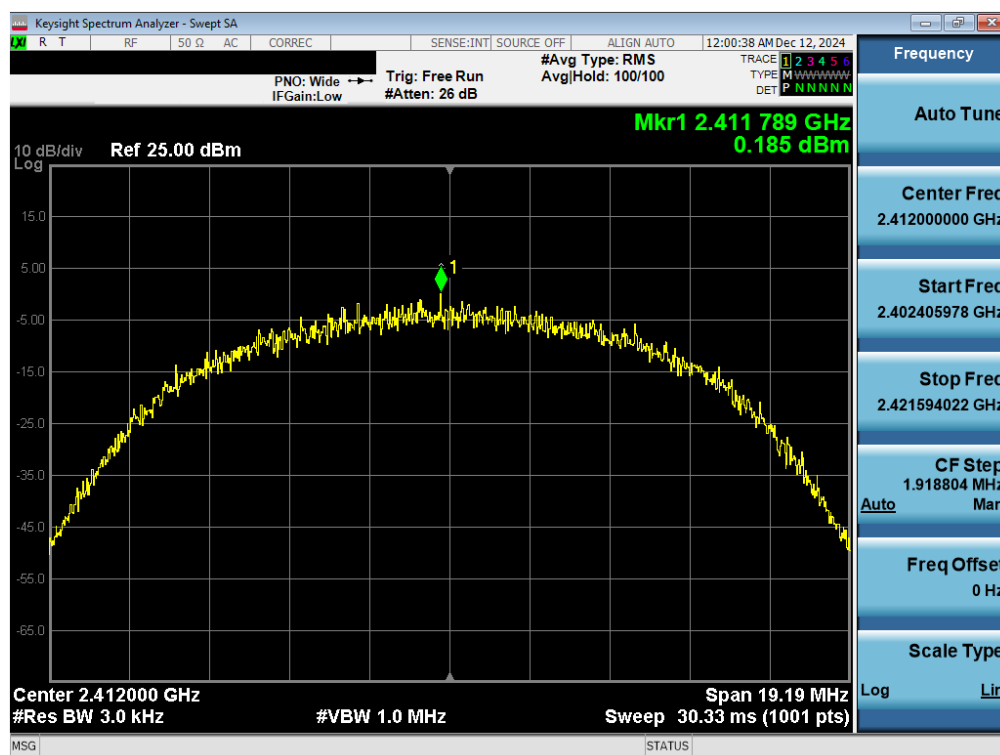
Plot 7-13. Power Spectral Density Plot Antenna WF7b (802.11b – Ch. 1)
