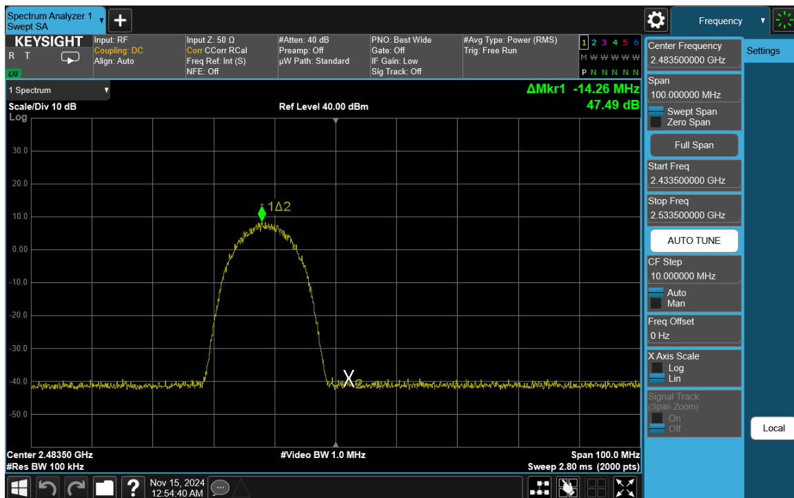
Plot 7-71. Band Edge Plot Antenna WF7b (802.11b – Ch. 13)
