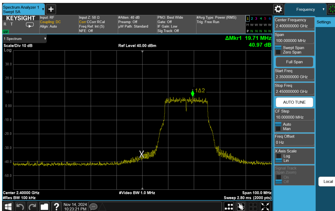
Plot 7-28. Band Edge Plot Antenna WF8 (802.11g – Ch. 2)
