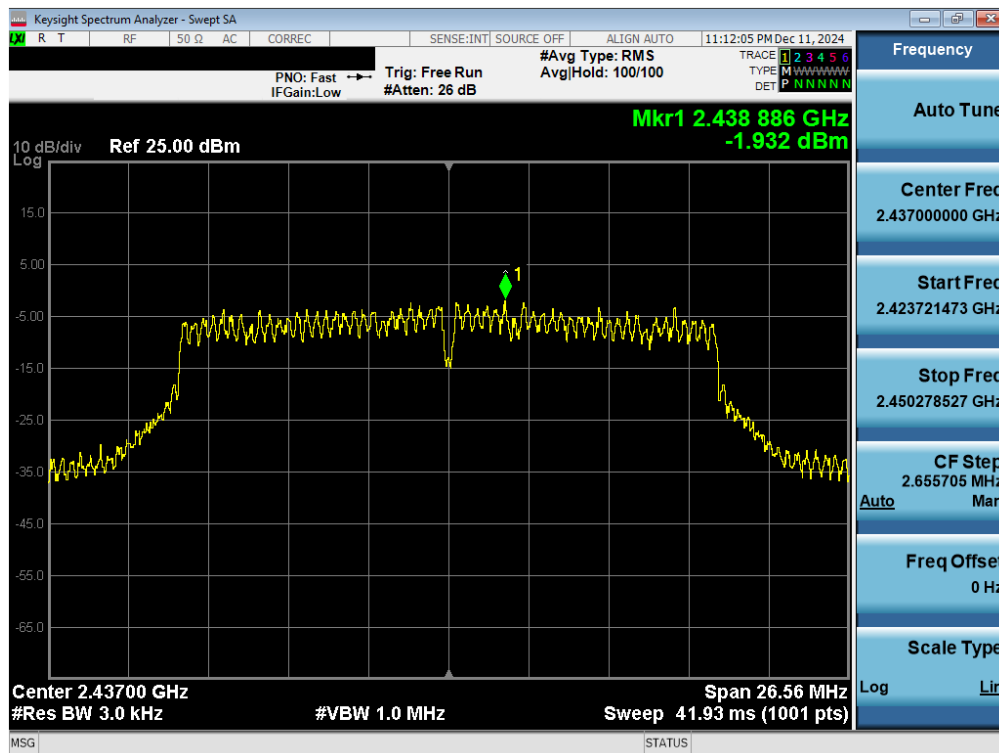
Plot 7-11. Power Spectral Density Plot Antenna WF8 (802.11n – Ch. 6)
