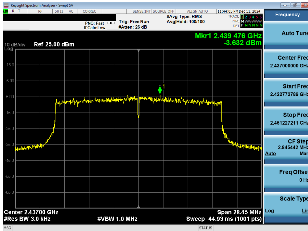
Plot 7-21. Power Spectral Density Plot CDD Antenna WF8 (802.11axSU – Ch. 6)
