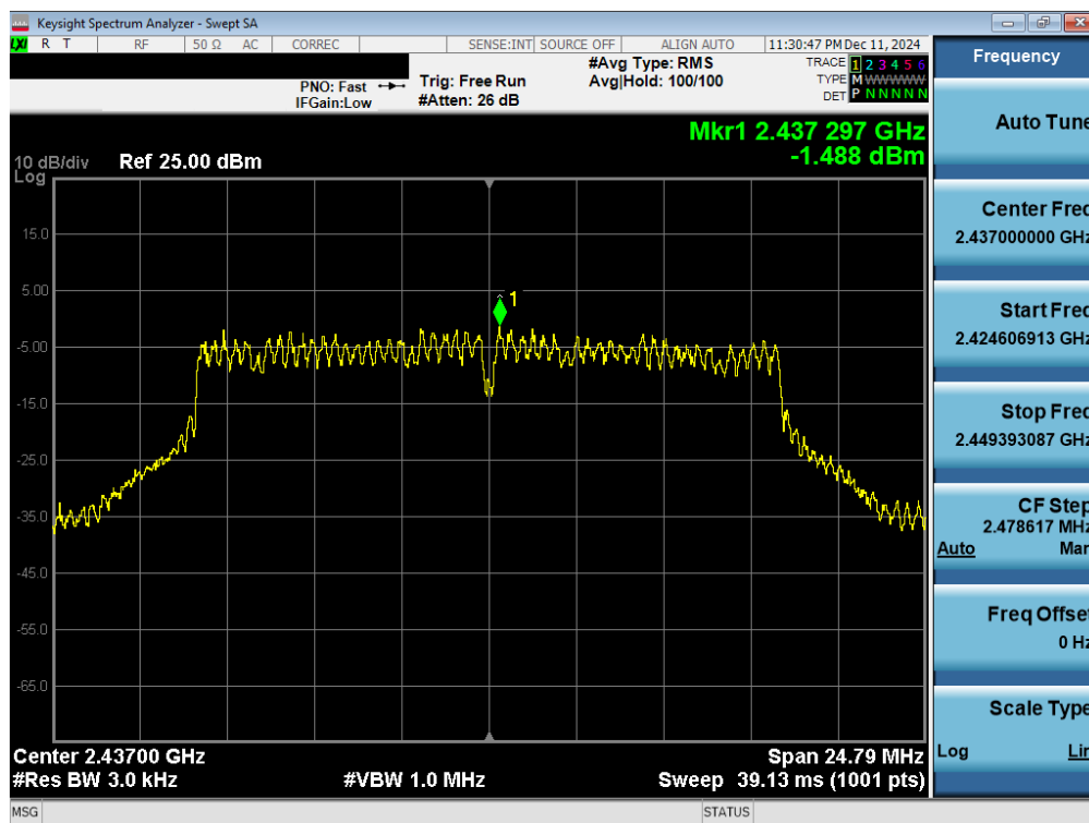
Plot 7-17. Power Spectral Density Plot CDD Antenna WF8 (802.11g – Ch. 6)
