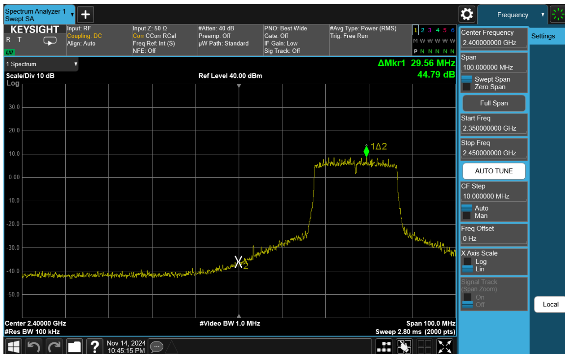
Plot 7-58. Band Edge Plot Antenna WF8 (802.11ax (SU - 2.4GHz) – Ch. 4)
