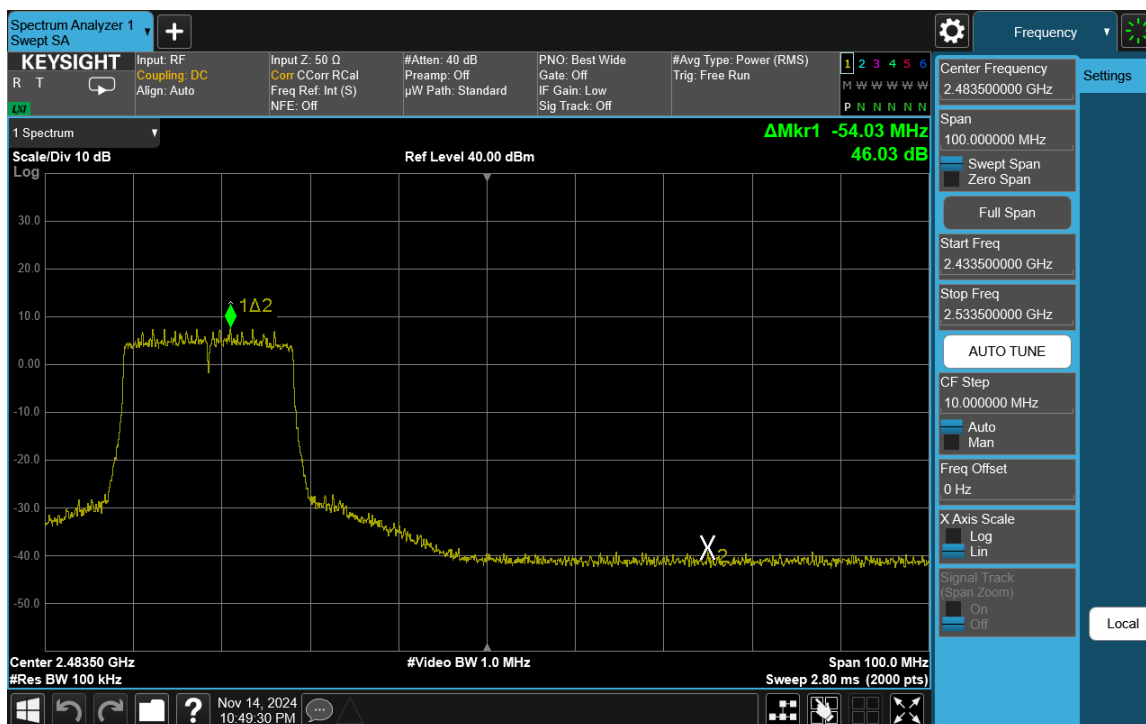
Plot 7-64. Band Edge Plot Antenna WF8 (802.11ax (SU - 2.4GHz) – Ch. 9)
