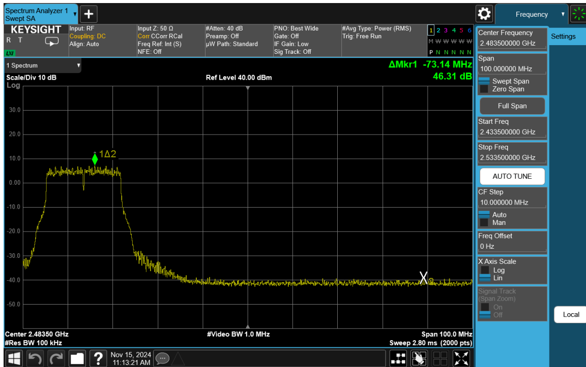
Plot 7-35. Band Edge Plot Antenna WF8 (802.11g – Ch. 8)
