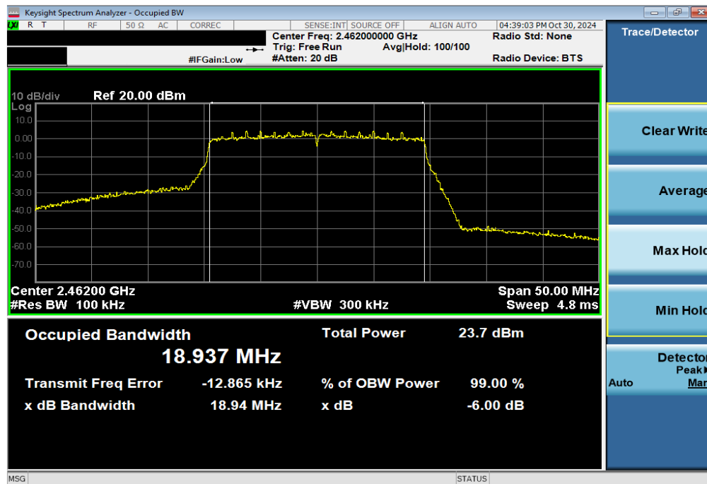
Plot 7-4. 6 dB BW and 99% OBW Plot Antenna WF8 (802.11axSU – Ch. 11)
