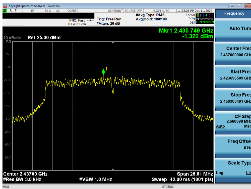
Plot 7-19. Power Spectral Density Plot CDD Antenna WF8 (802.11n – Ch. 6)
