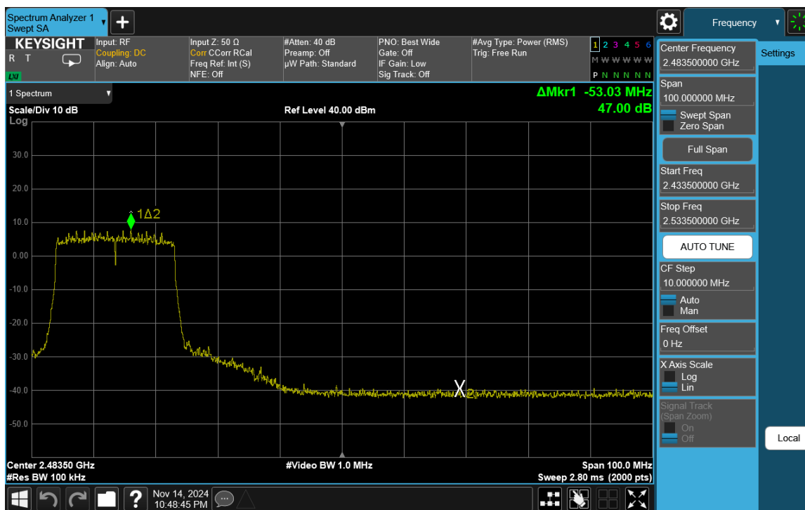
Plot 7-63. Band Edge Plot Antenna WF8 (802.11ax (SU - 2.4GHz) – Ch. 8)
