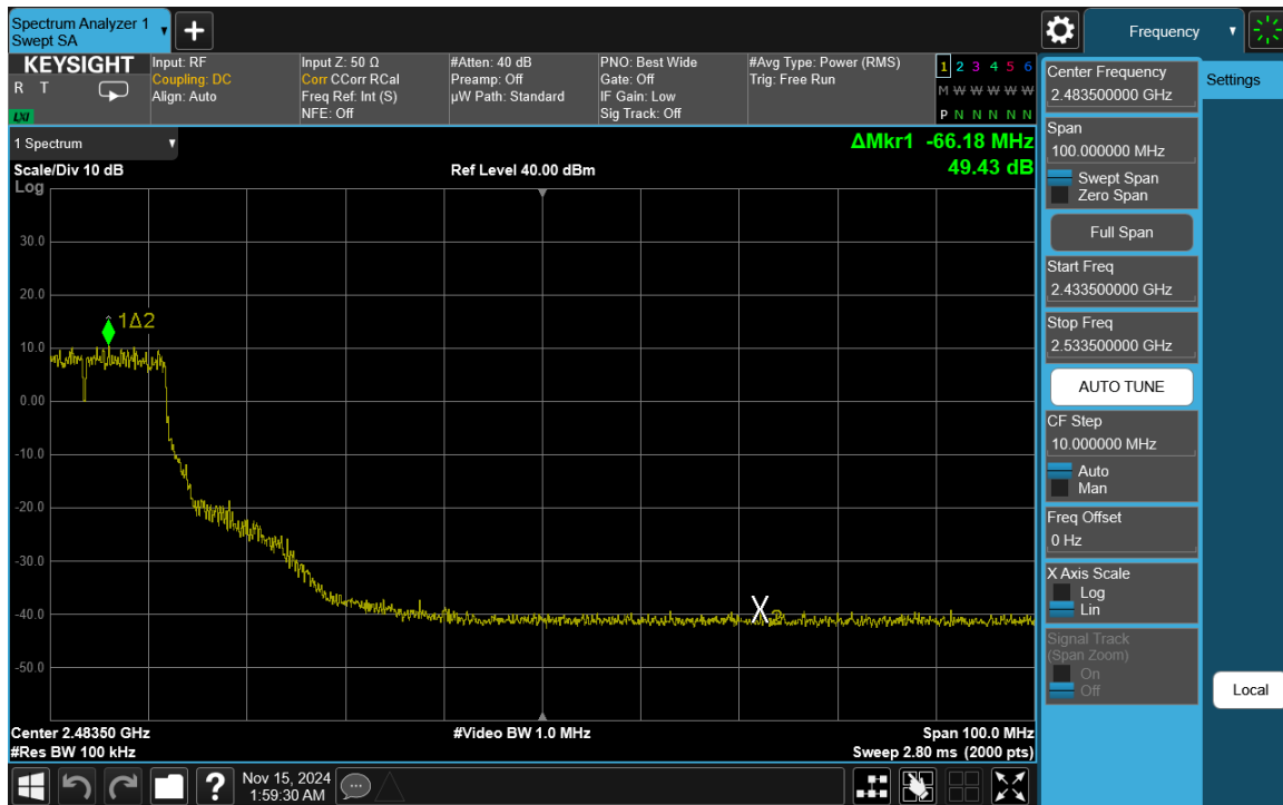
Plot 7-78. Band Edge Plot Antenna WF7b (802.11g – Ch. 6-High)
