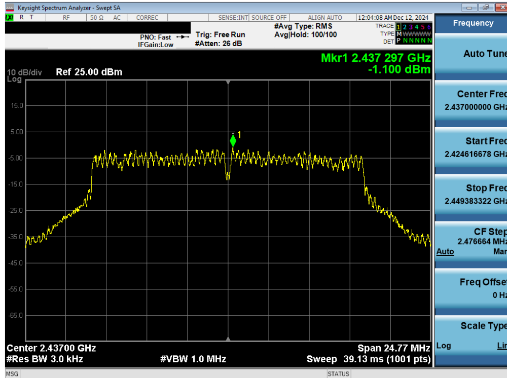
Plot 7-14. Power Spectral Density Plot Antenna WF7b (802.11g – Ch. 6)
