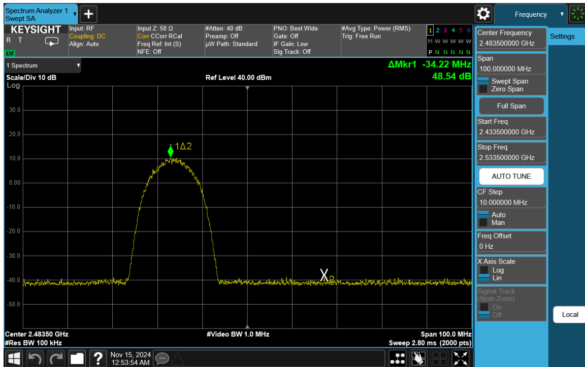
Plot 7-70. Band Edge Plot Antenna WF7b (802.11b – Ch. 12)
