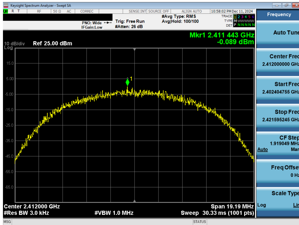
Plot 7-9. Power Spectral Density Plot Antenna WF8 (802.11b – Ch. 1)
