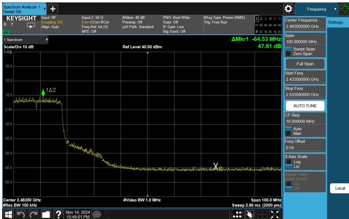
Plot 7-62. Band Edge Plot Antenna WF8 (802.11ax (SU - 2.4GHz) – Ch. 7)
