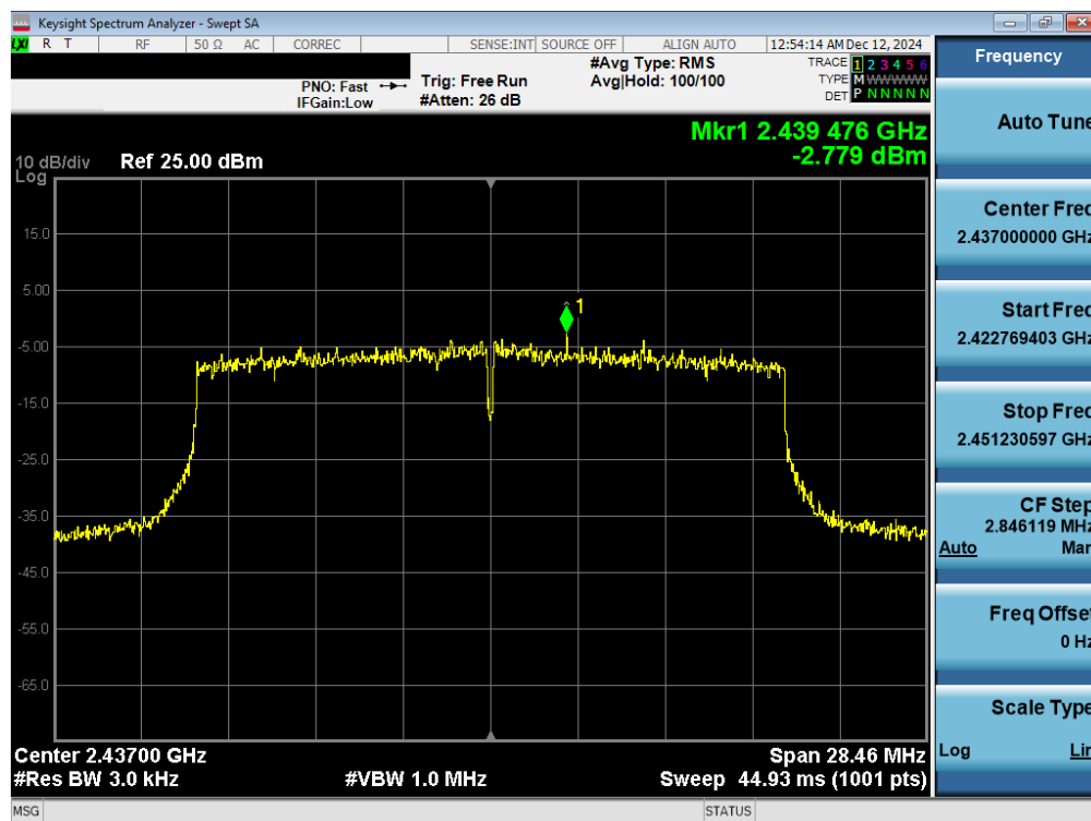
Plot 7-22. Power Spectral Density Plot CDD Antenna WF7b (802.11axSU – Ch. 6)
