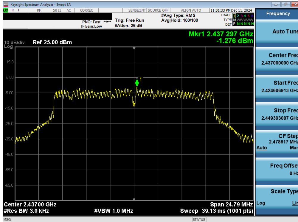
Plot 7-10. Power Spectral Density Plot Antenna WF8 (802.11g – Ch. 6)
