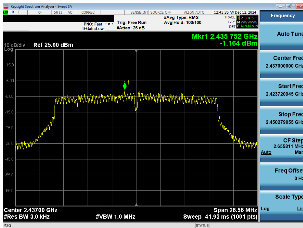
Plot 7-20. Power Spectral Density Plot CDD Antenna WF7b (802.11n – Ch. 6)
