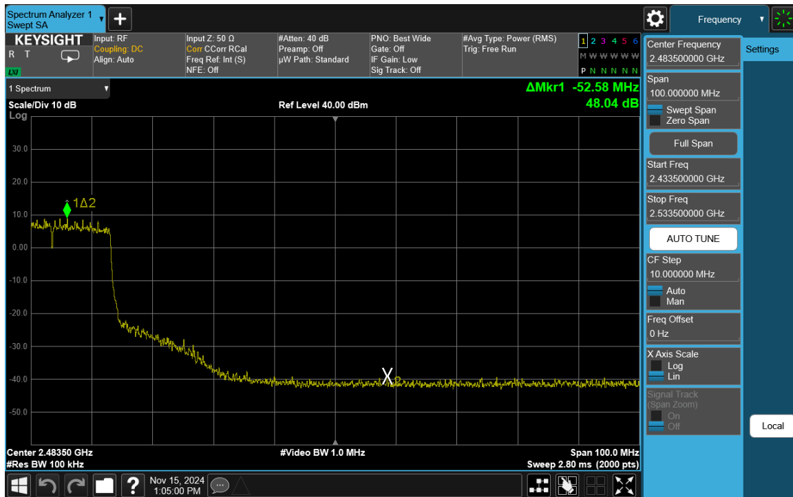
Plot 7-61. Band Edge Plot Antenna WF8 (802.11ax (SU - 2.4GHz) – Ch. 6-High)
