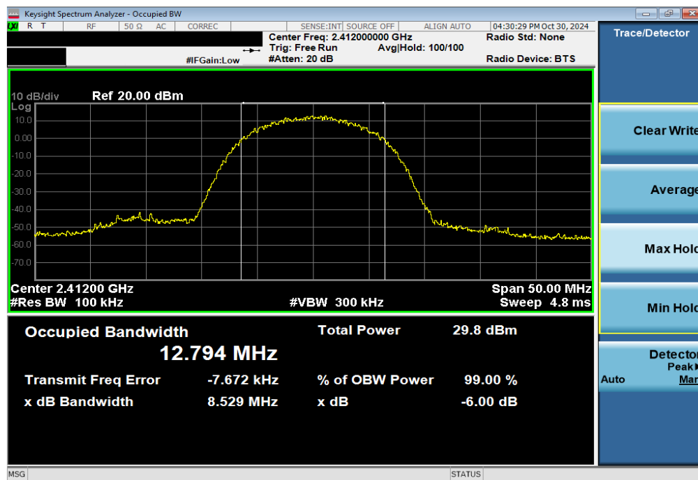
Plot 7-1. 6 dB BW and 99% OBW Plot Antenna WF8 (802.11b – Ch. 1)
