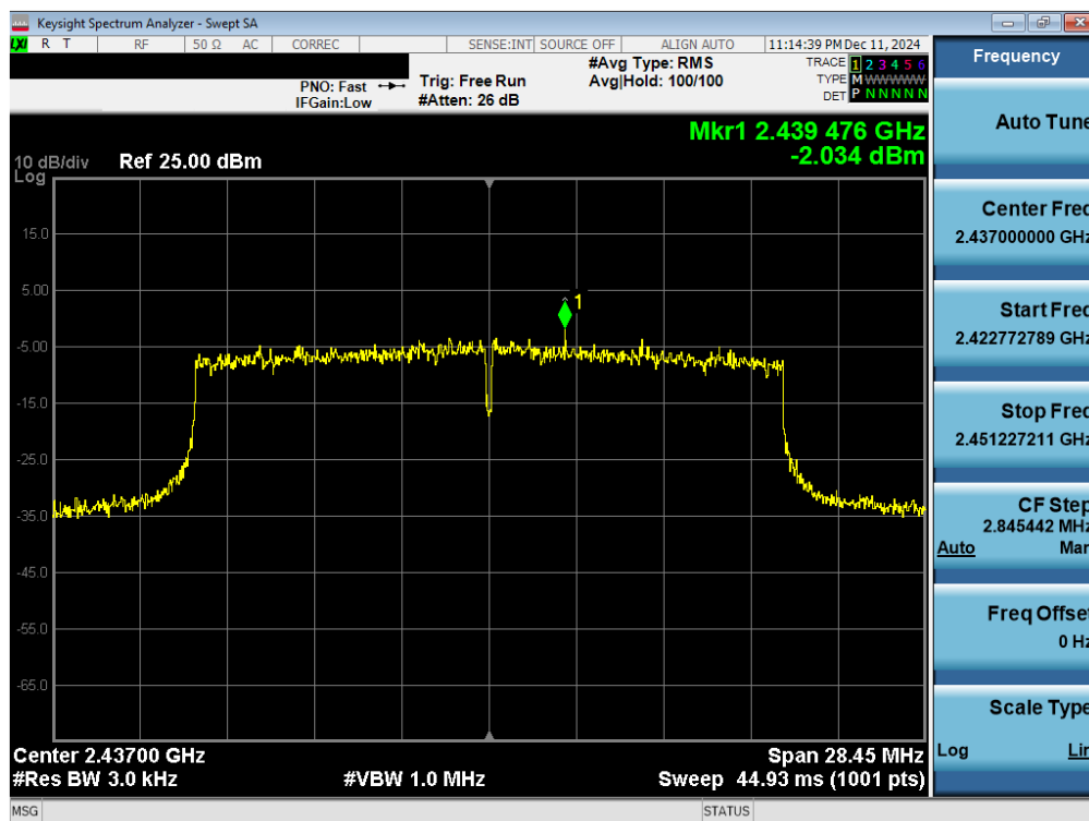
Plot 7-12. Power Spectral Density Plot Antenna WF8 (802.11axSU – Ch. 6)
