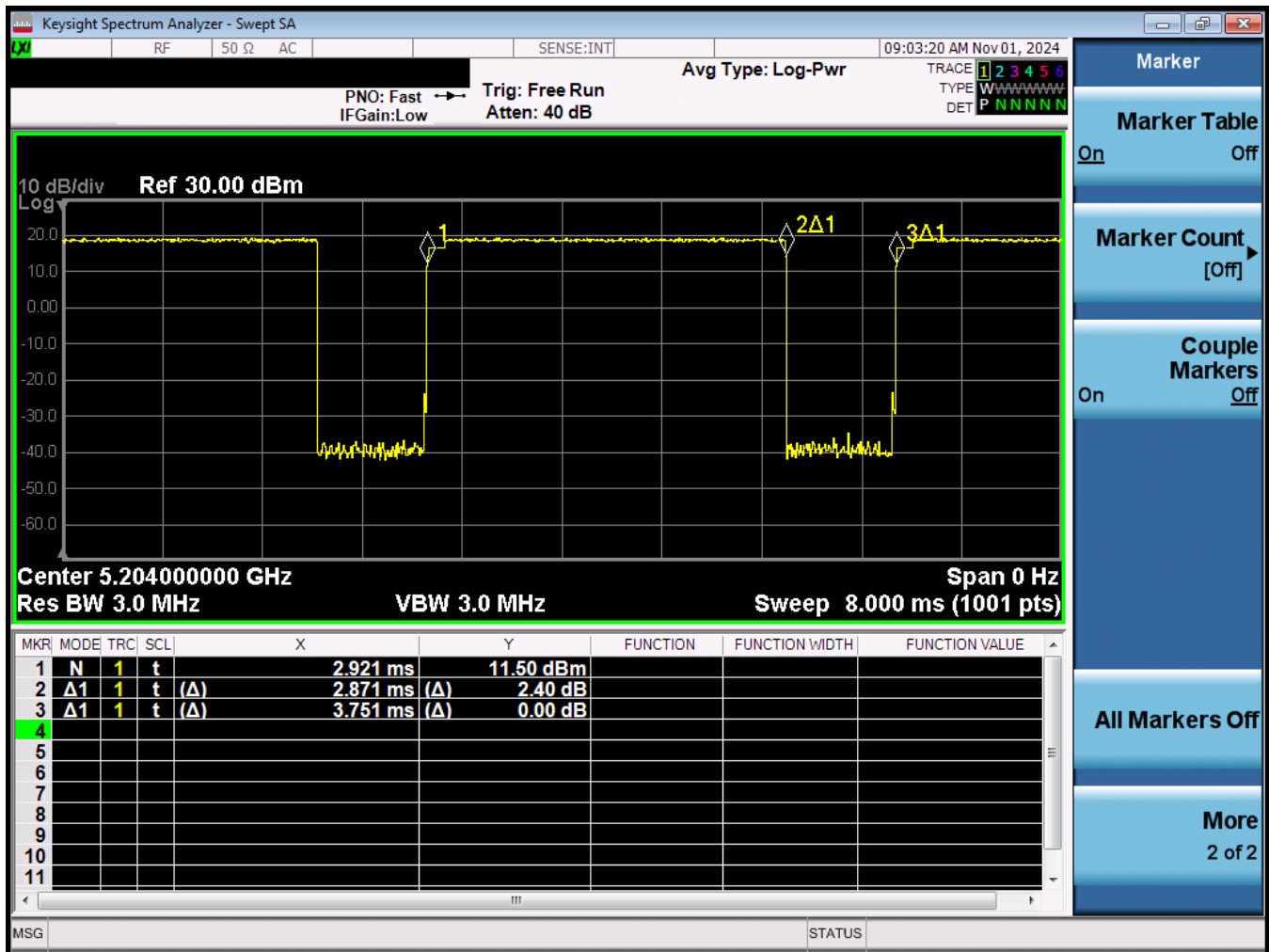
Figure 7-12 NB UNII 1 (HDR4) Transmission Plot – Antenna WF8, Variant 1
