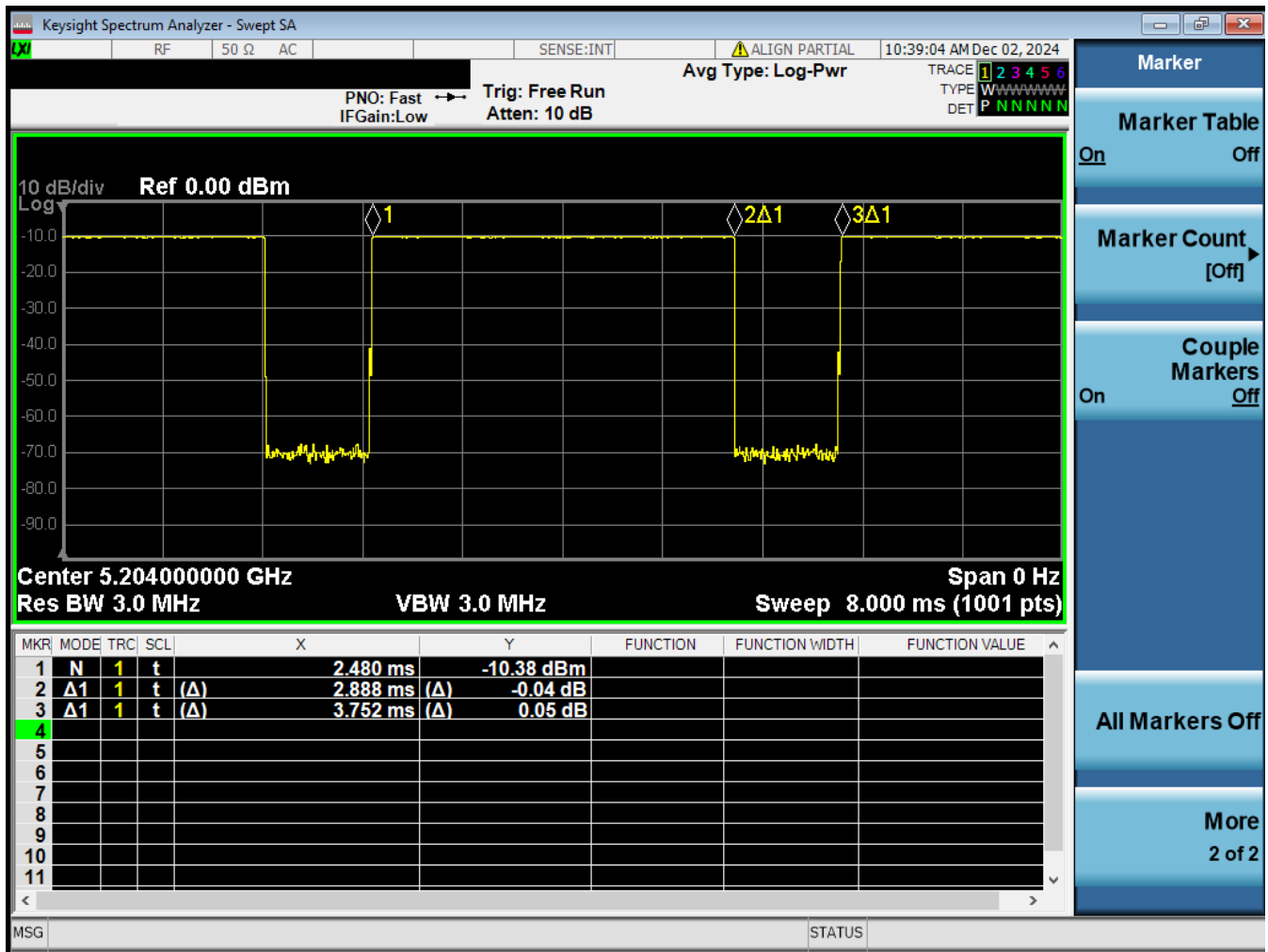
Figure 7-18 NB UNII 1 (BDR) Transmission Plot – Antenna WF7a, Variant 1
