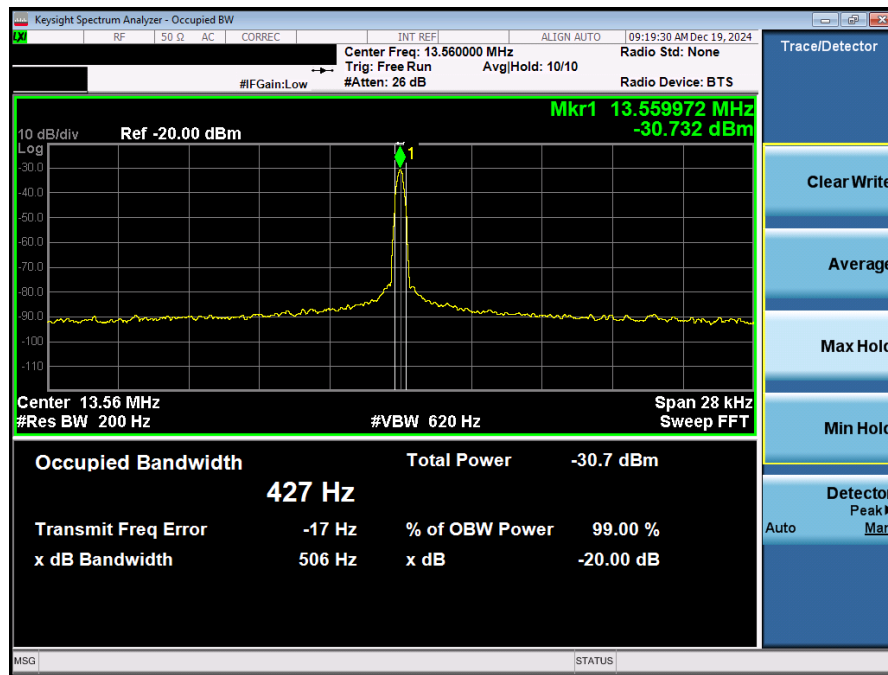
Figure 7-2. 20dB and 99% Bandwidth WPT Plot (Charging Rate 2.6C)
