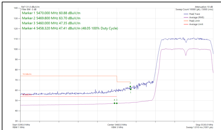
Figure 494 - 802.11n HT40, SDM, Core 0 - Core 1 - 5510 MHz Band Edge Frequency 5470 MHz
