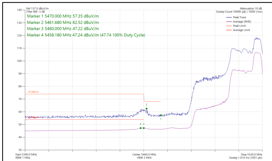
Figure 498 - 802.11ax HE40, RU 52-44, SDM, Core 0 - Core 1 - 5510 MHz Band Edge Frequency 5470 MHz
