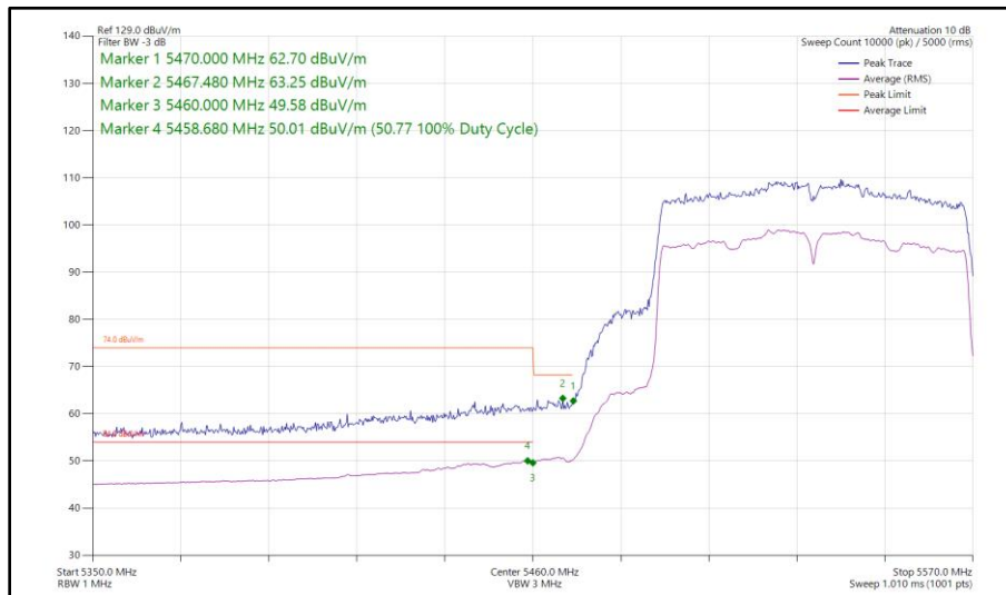
Figure 523 - 802.11ac VHT80, SISO, Core 0 - 5530 MHz Band Edge Frequency 5470 MHz
