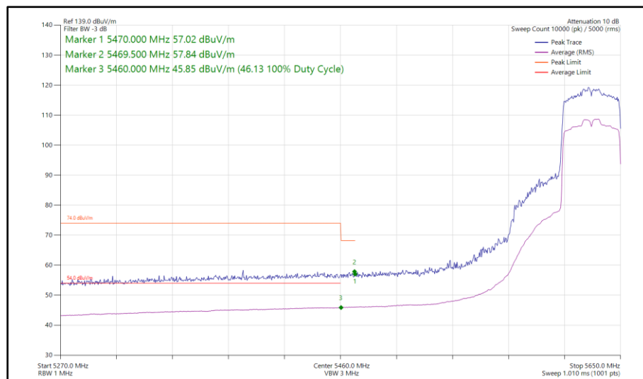
Figure 501 - 802.11ax HE40, SU, SDM, Core 0 - Core 1 - 5630 MHz Band Edge Frequency 5470 MHz
