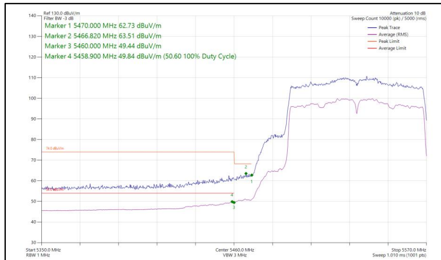
Figure 553 - 802.11ac VHT80, CDD, Core 0 - Core 1 - 5530 MHz Band Edge Frequency 5470 MHz
