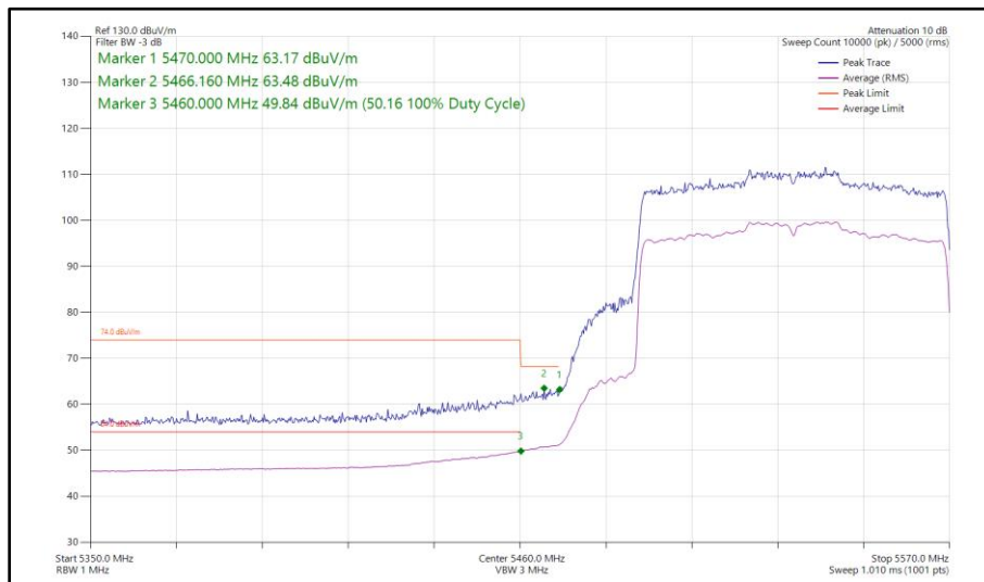
Figure 554 - 802.11ax HE80, SU, CDD, Core 0 - Core 1 - 5530 MHz Band Edge Frequency 5470 MHz
