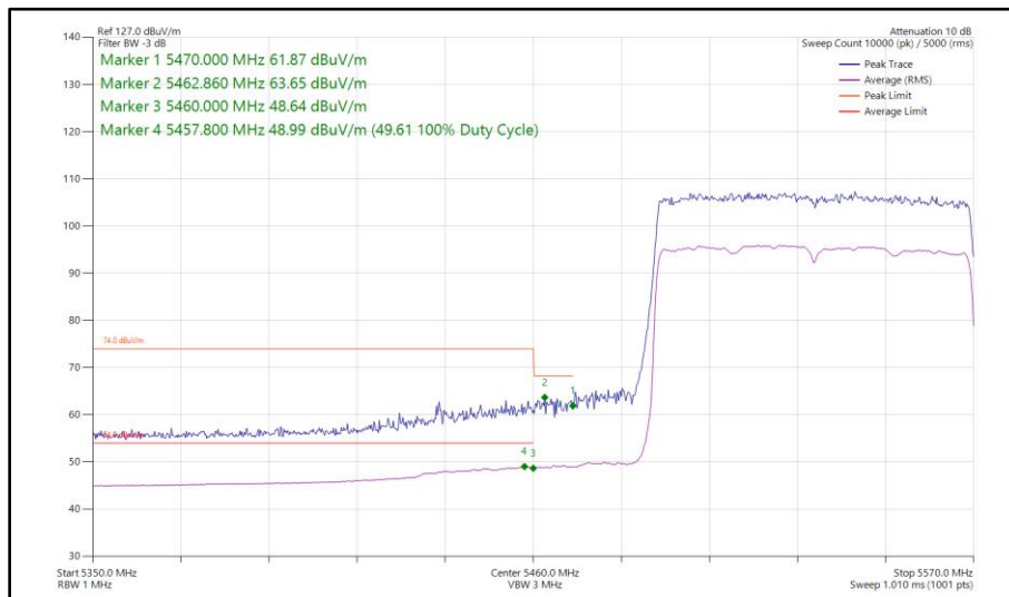
Figure 524 - 802.11ax HE80, SU, SISO, Core 0 - 5530 MHz Band Edge Frequency 5470 MHz
