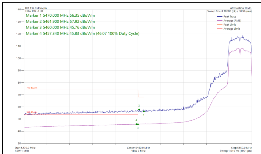
Figure 496 - 802.11n HT40, SDM, Core 0 - Core 1 - 5630 MHz Band Edge Frequency 5470 MHz
