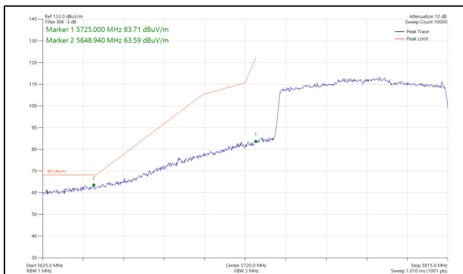
Figure 527 - 802.11ax HE80, SU, SISO, Core 0 - 5775 MHz Band Edge Frequency 5725 MHz
