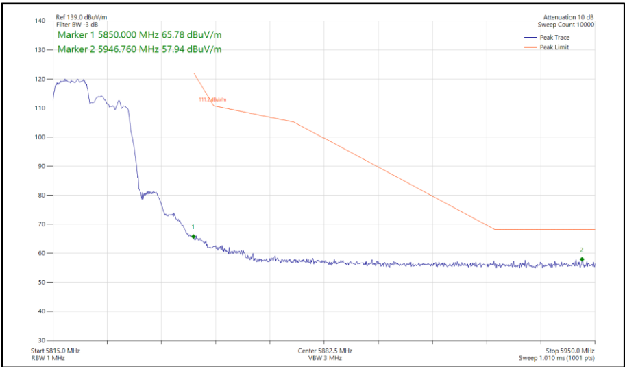
Figure 417 - 802.11ax HE20, RU 106-53, SDM, Core 0 - Core 1 - 5825 MHz Band Edge Frequency 5850 MHz
