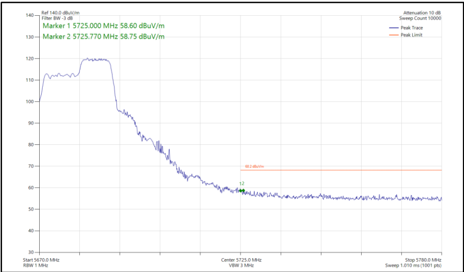
Figure 345 - 802.11ax HE20, RU 106-54, SISO, Core 0 - 5680 MHz Band Edge Frequency 5725 MHz
