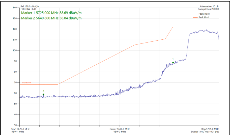
Figure 403 - 802.11ax HE20, SU, SDM, Core 0 - Core 1 - 5745 MHz Band Edge Frequency 5725 MHz
