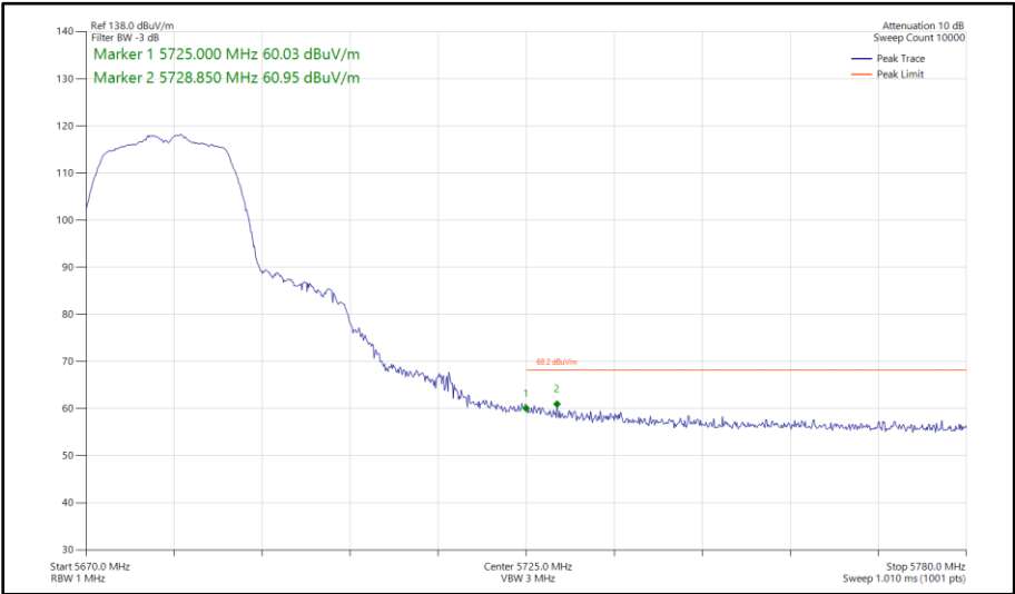
Figure 340 - 802.11a, SISO, Core 0 - 5680 MHz Band Edge Frequency 5725 MHz
