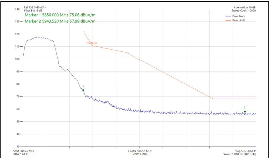
Figure 349 - 802.11a, SISO, Core 0 - 5825 MHz Band Edge Frequency 5850 MHz
