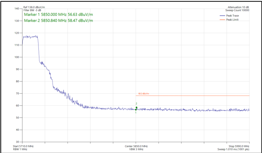
Figure 413 - 802.11ax HE20, SU, SDM, Core 0 - Core 1 - 5720 MHz Band Edge Frequency 5850 MHz
