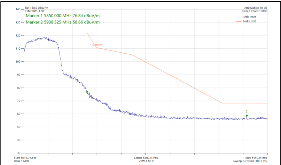
Figure 379 - 802.11n HT20, SISO, Core 1 - 5825 MHz Band Edge Frequency 5850 MHz
