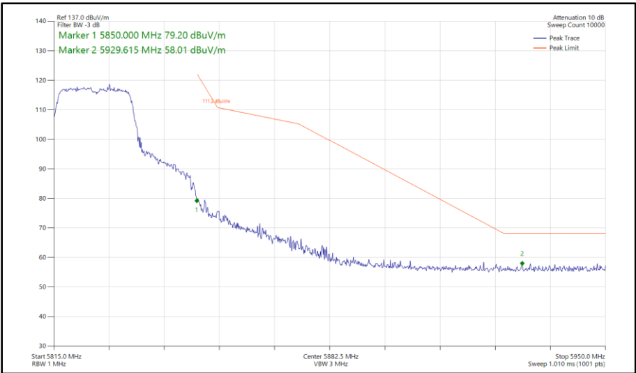
Figure 394 - 802.11n HT20, CDD, Core 0 - Core 1 - 5825 MHz Band Edge Frequency 5850 MHz
