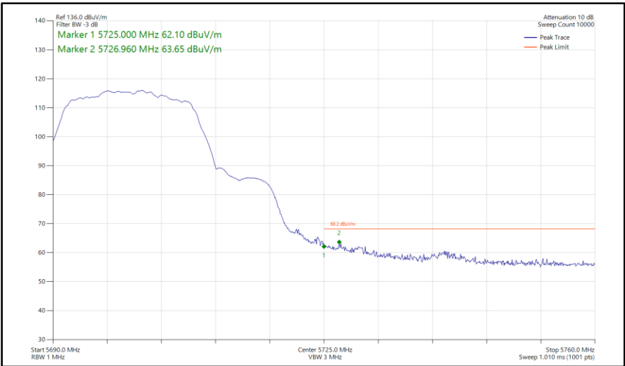
Figure 369 - 802.11a, SISO, Core 1 - 5700 MHz Band Edge Frequency 5725 MHz
