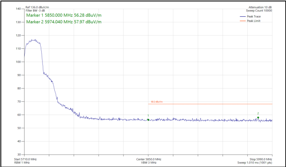
Figure 350 - 802.11n HT20, SISO, Core 0 - 5720 MHz Band Edge Frequency 5850 MHz
