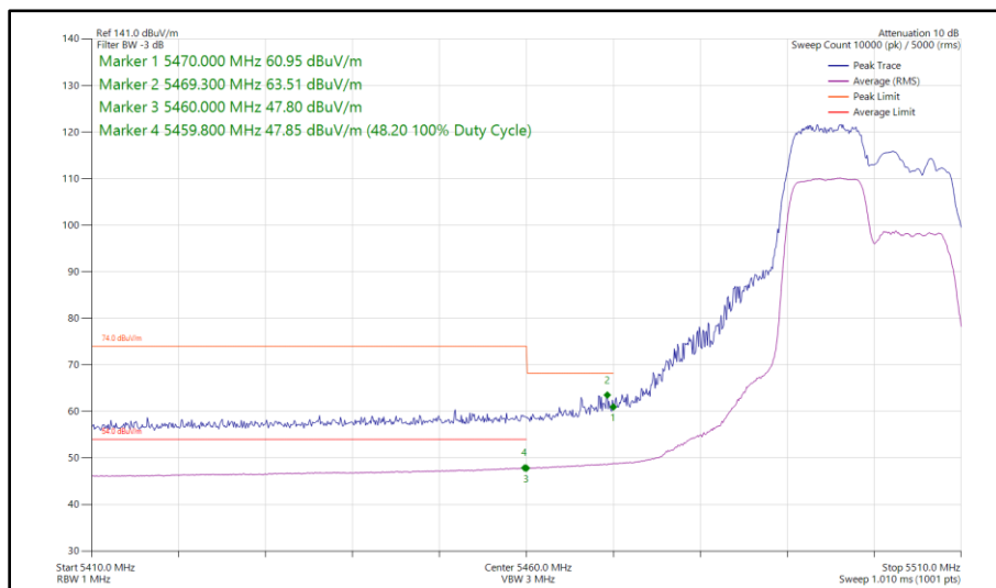
Figure 386 - 802.11ax HE20, RU 106-53, CDD, Core 0 - Core 1 - 5500 MHz Band Edge Frequency 5470 MHz
