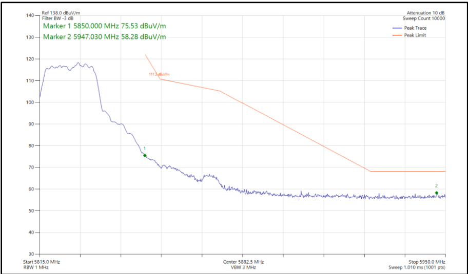
Figure 377 - 802.11a, SISO, Core 1 - 5825 MHz Band Edge Frequency 5850 MHz
