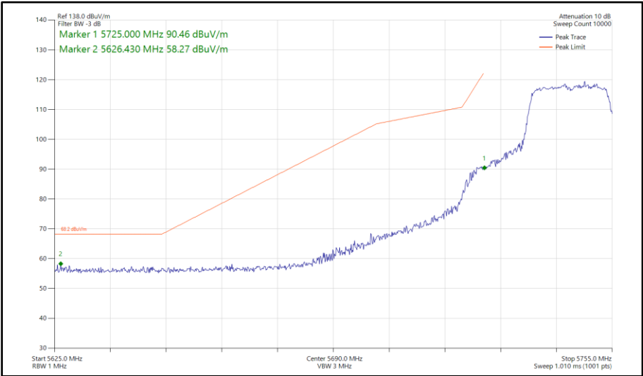
Figure 387 - 802.11n HT20, CDD, Core 0 - Core 1 - 5745 MHz Band Edge Frequency 5725 MHz
