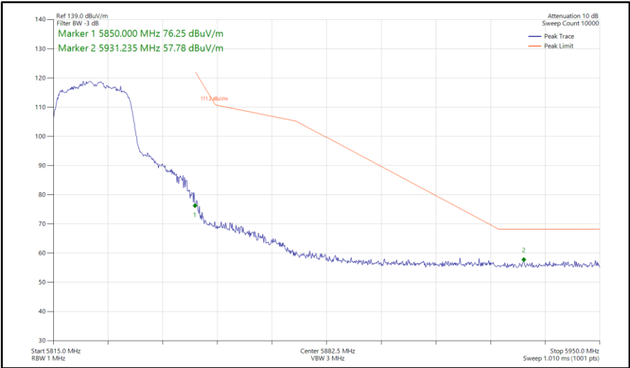
Figure 412 - 802.11n HT20, SDM, Core 0 - Core 1 - 5825 MHz Band Edge Frequency 5850 MHz
