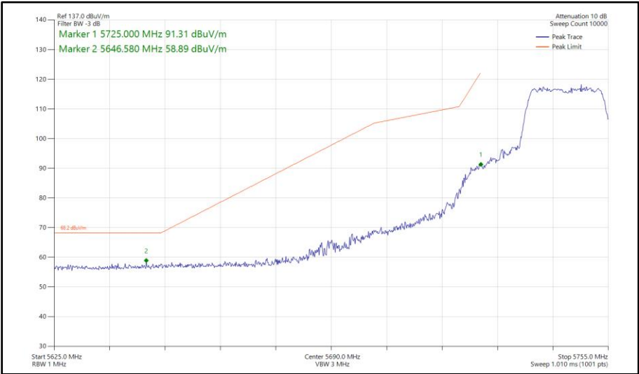
Figure 402 - 802.11n HT20, SDM, Core 0 - Core 1 - 5745 MHz Band Edge Frequency 5725 MHz
