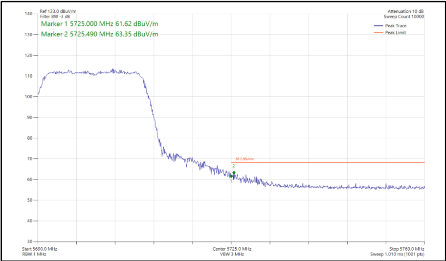
Figure 406 - 802.11n HT20, SDM, Core 0 - Core 1 - 5700 MHz Band Edge Frequency 5725 MHz
