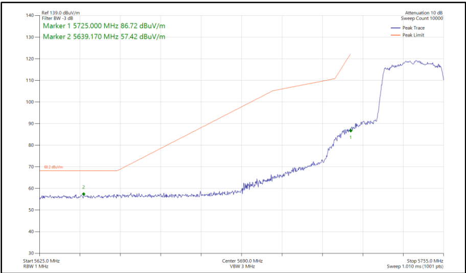
Figure 388 - 802.11ax HE20, SU, CDD, Core 0 - Core 1 - 5745 MHz Band Edge Frequency 5725 MHz
