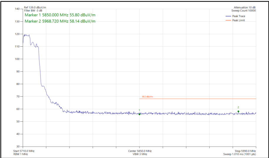
Figure 381 - 802.11ax HE20, RU 106-53, SISO, Core 1 - 5720 MHz Band Edge Frequency 5850 MHz
