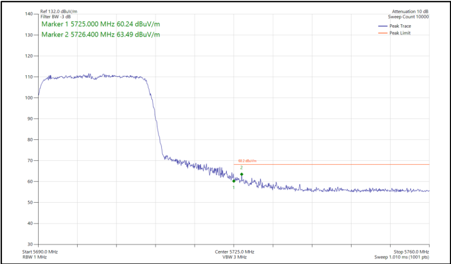
Figure 346 - 802.11ax HE20, SU, SISO, Core 0 - 5700 MHz Band Edge Frequency 5725 MHz
