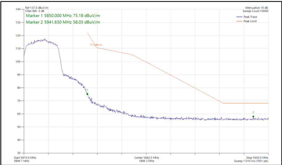
Figure 351 - 802.11n HT20, SISO, Core 0 - 5825 MHz Band Edge Frequency 5850 MHz
