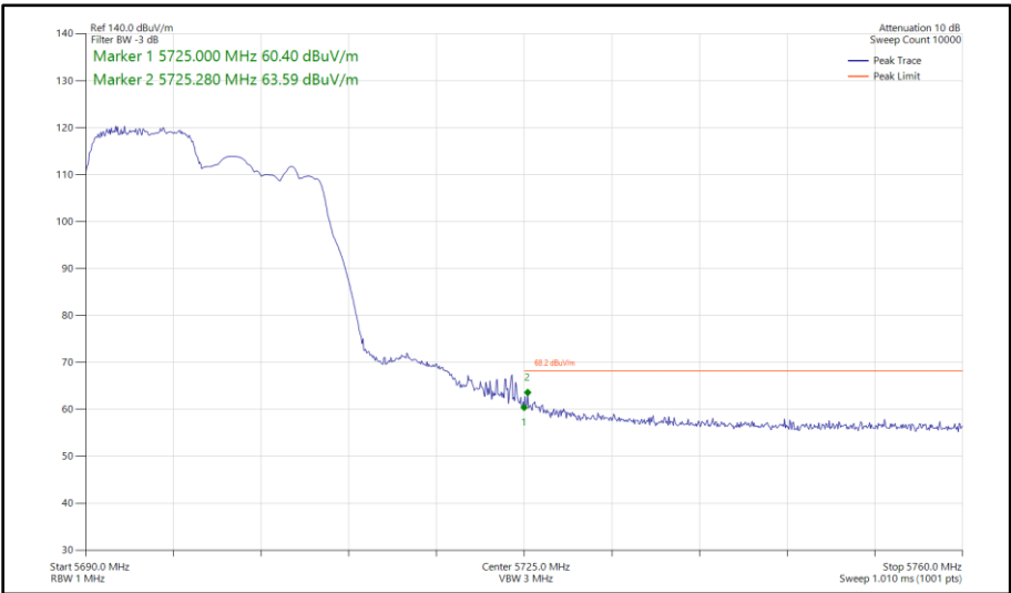
Figure 375 - 802.11ax HE20, RU 106-53, SISO, Core 1 - 5700 MHz Band Edge Frequency 5725 MHz
