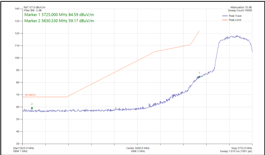
Figure 365 - 802.11n HT20, SISO, Core 1 - 5745 MHz Band Edge Frequency 5725 MHz
