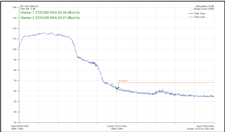
Figure 390 - 802.11n HT20, CDD, Core 0 - Core 1 - 5700 MHz Band Edge Frequency 5725 MHz
