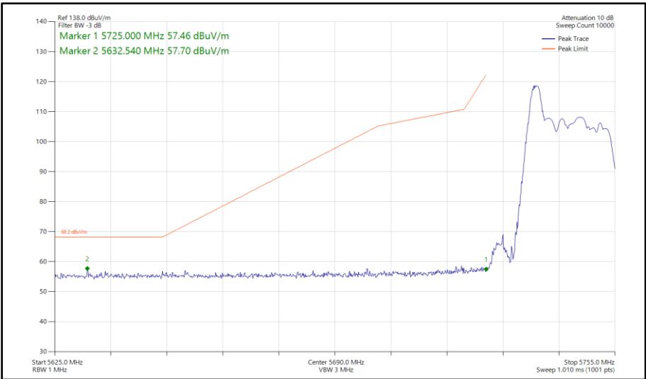
Figure 339 - 802.11ax HE20, RU 26-0, SISO, Core 0 - 5745 MHz Band Edge Frequency 5725 MHz
