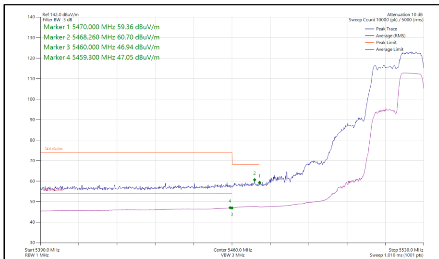
Figure 363 - 802.11ax HE20, RU 106-54, SISO, Core 1 - 5520 MHz Band Edge Frequency 5470 MHz
