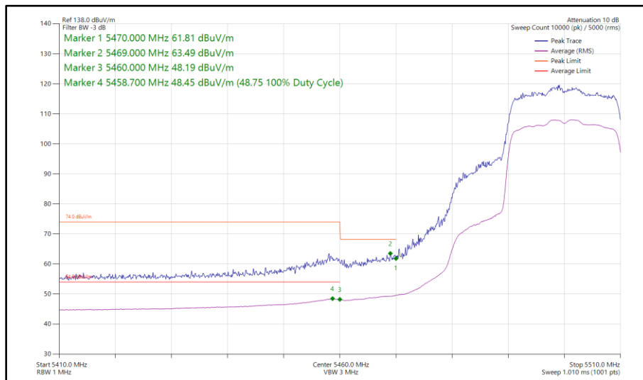
Figure 385 - 802.11ax HE20, SU, CDD, Core 0 - Core 1 - 5500 MHz Band Edge Frequency 5470 MHz
