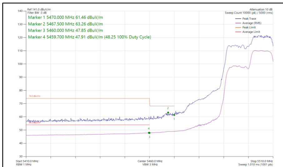
Figure 401 - 802.11ax HE20, RU 106-54, SDM, Core 0 - Core 1 - 5500 MHz Band Edge Frequency 5470 MHz
