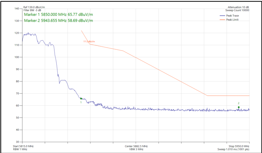
Figure 398 - 802.11ax HE20, RU 106-53, CDD, Core 0 - Core 1 - 5825 MHz Band Edge Frequency 5850 MHz
