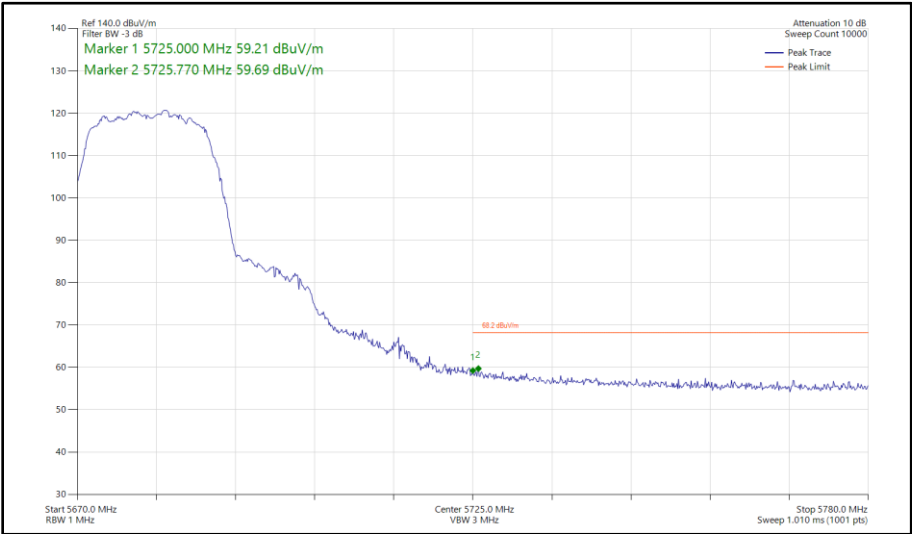
Figure 368 - 802.11a, SISO, Core 1 - 5680 MHz Band Edge Frequency 5725 MHz
