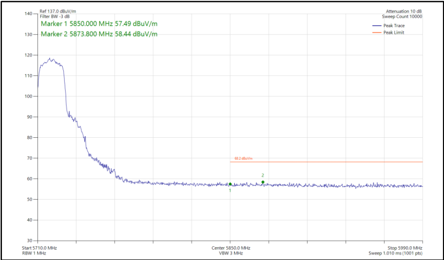
Figure 378 - 802.11n HT20, SISO, Core 1 - 5720 MHz Band Edge Frequency 5850 MHz
