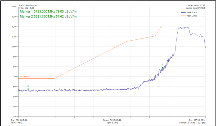
Figure 404 - 802.11ax HE20, RU 106-53, SDM, Core 0 - Core 1 - 5745 MHz Band Edge Frequency 5725 MHz
