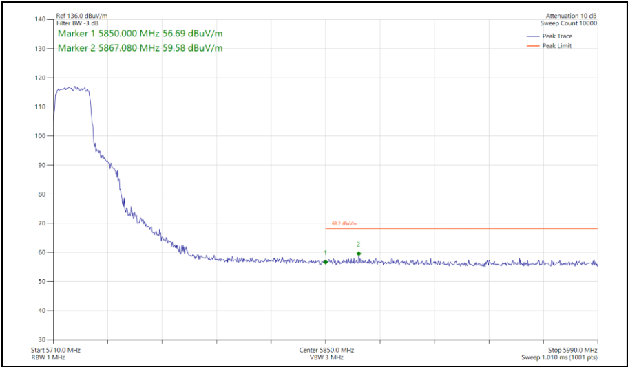
Figure 393 - 802.11n HT20, CDD, Core 0 - Core 1 - 5720 MHz Band Edge Frequency 5850 MHz
