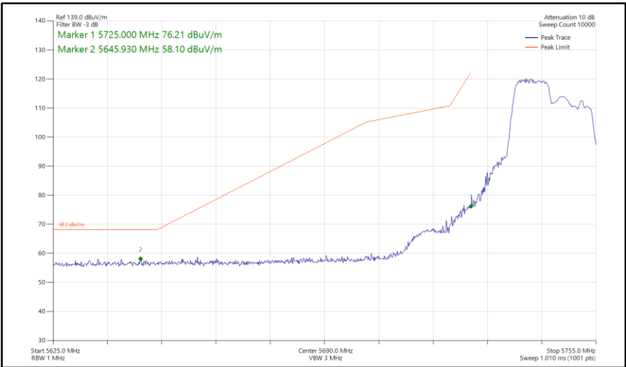
Figure 367 - 802.11ax HE20, RU 106-53, SISO, Core 1 - 5745 MHz Band Edge Frequency 5725 MHz
