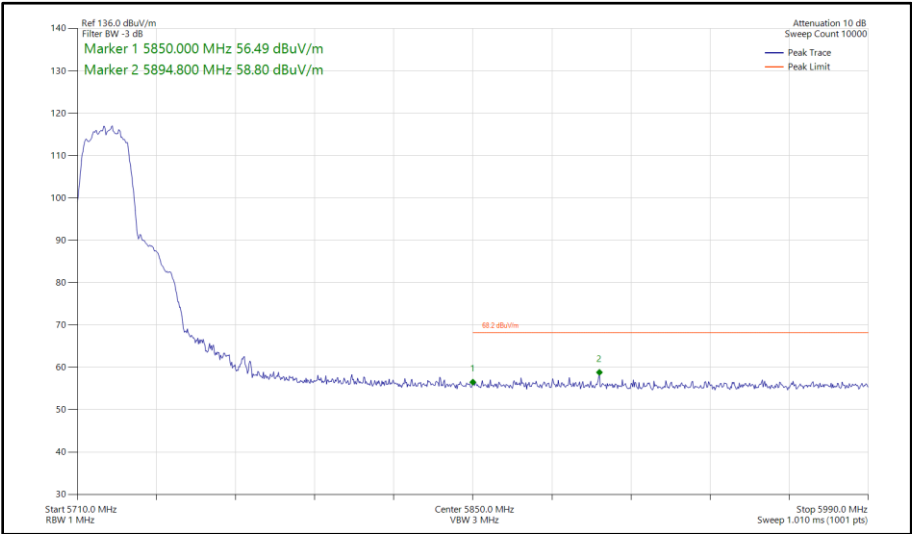
Figure 348 - 802.11a, SISO, Core 0 - 5720 MHz Band Edge Frequency 5850 MHz
