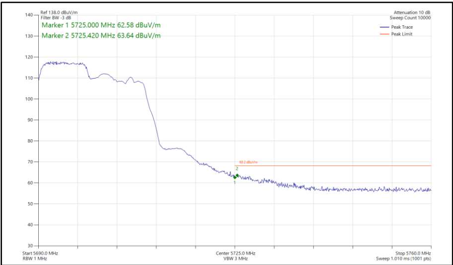
Figure 347 - 802.11ax HE20, RU 106-53, SISO, Core 0 - 5700 MHz Band Edge Frequency 5725 MHz
