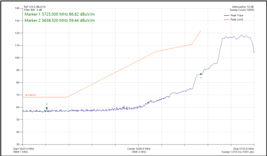
Figure 364 - 802.11a, SISO, Core 1 - 5745 MHz Band Edge Frequency 5725 MHz
