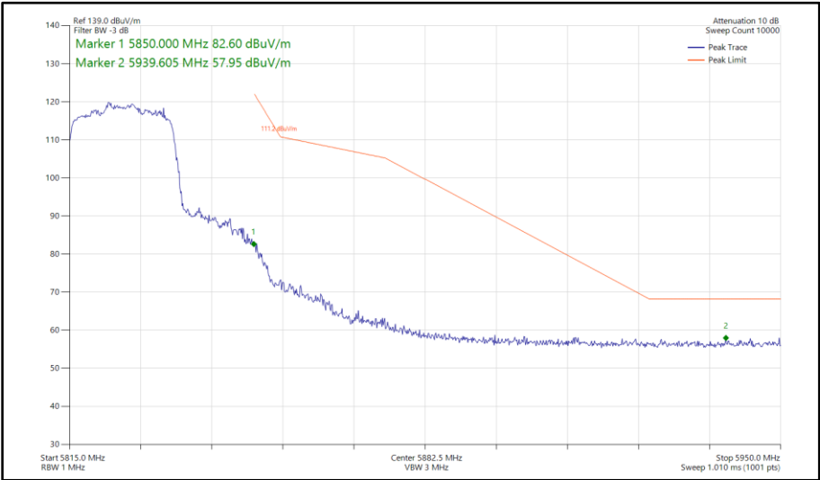
Figure 397 - 802.11ax HE20, SU, CDD, Core 0 - Core 1 - 5825 MHz Band Edge Frequency 5850 MHz
