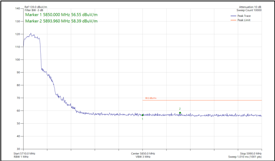
Figure 380 - 802.11ax HE20, SU, SISO, Core 1 - 5720 MHz Band Edge Frequency 5850 MHz
