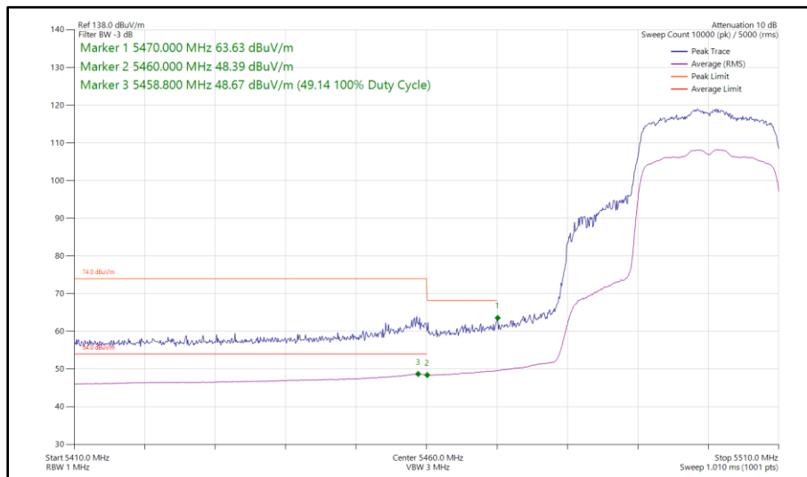
Figure 400 - 802.11ax HE20, SU, SDM, Core 0 - Core 1 - 5500 MHz Band Edge Frequency 5470 MHz
