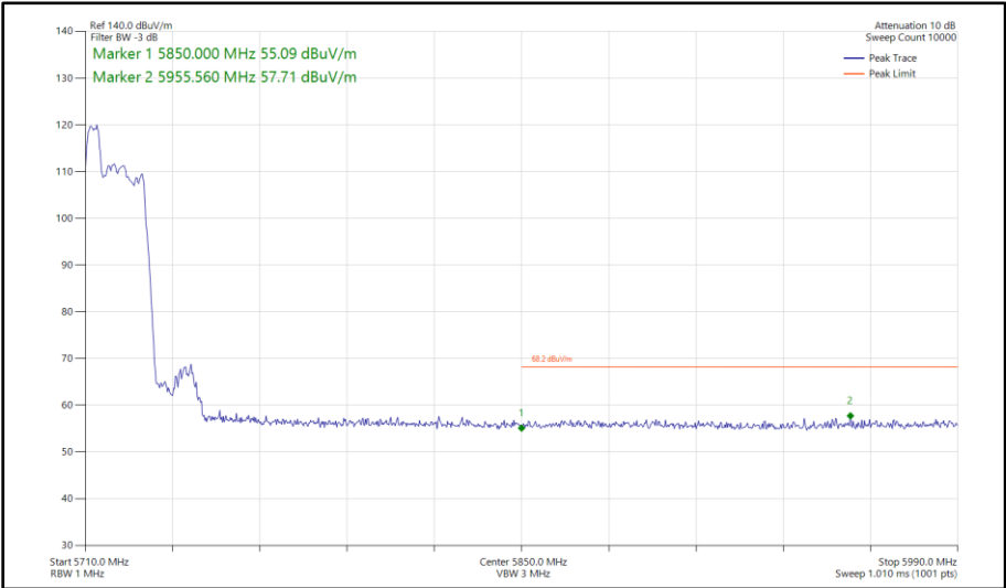
Figure 396 - 802.11ax HE20, RU 52-37, CDD, Core 0 - Core 1 - 5720 MHz Band Edge Frequency 5850 MHz
