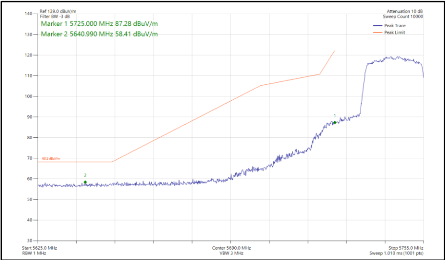
Figure 366 - 802.11ax HE20, SU, SISO, Core 1 - 5745 MHz Band Edge Frequency 5725 MHz
