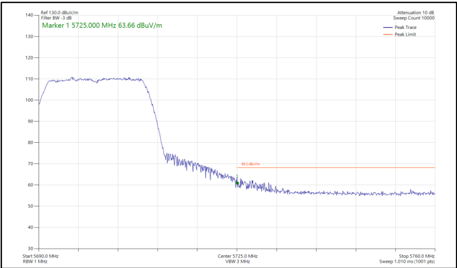
Figure 343 - 802.11n HT20, SISO, Core 0 - 5700 MHz Band Edge Frequency 5725 MHz
