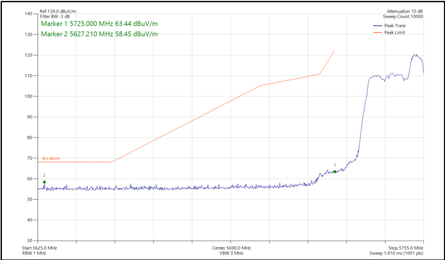
Figure 389 - 802.11ax HE20, RU 52-40, CDD, Core 0 - Core 1 - 5745 MHz Band Edge Frequency 5725 MHz
