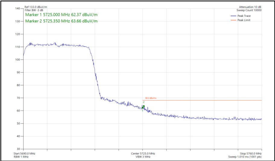
Figure 391 - 802.11ax HE20, SU, CDD, Core 0 - Core 1 - 5700 MHz Band Edge Frequency 5725 MHz
