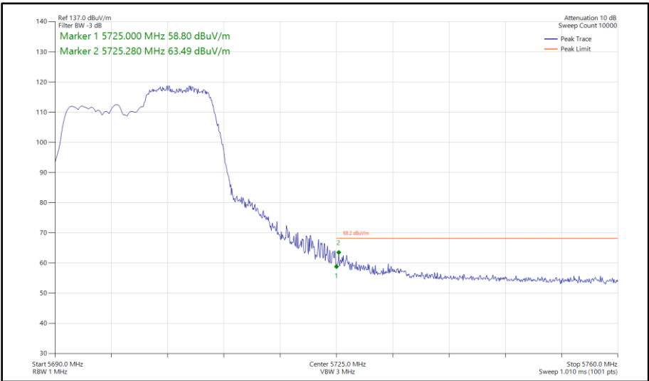
Figure 392 - 802.11ax HE20, RU 106-54, CDD, Core 0 - Core 1 - 5700 MHz Band Edge Frequency 5725 MHz
