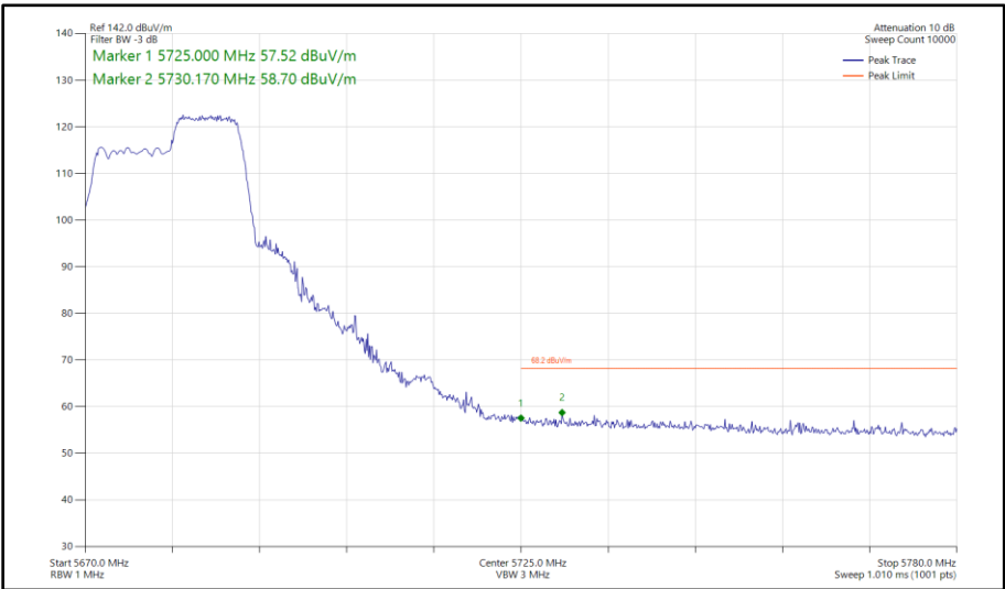
Figure 373 - 802.11ax HE20, RU 106-54, SISO, Core 1 - 5680 MHz Band Edge Frequency 5725 MHz
