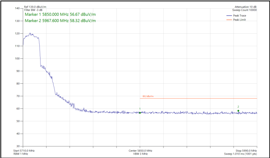
Figure 395 - 802.11ax HE20, SU, CDD, Core 0 - Core 1 - 5720 MHz Band Edge Frequency 5850 MHz
