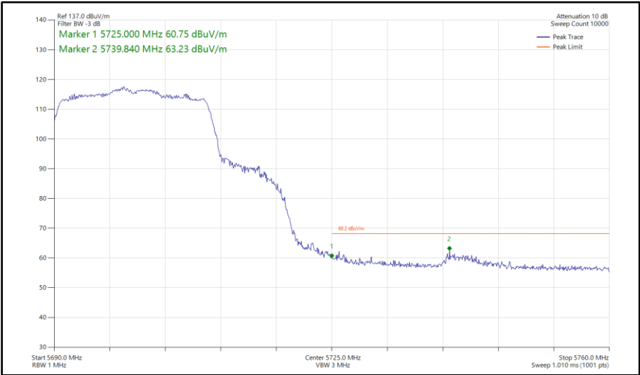
Figure 374 - 802.11ax HE20, SU, SISO, Core 1 - 5700 MHz Band Edge Frequency 5725 MHz
