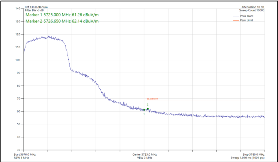
Figure 342 - 802.11n HT20, SISO, Core 0 - 5680 MHz Band Edge Frequency 5725 MHz
