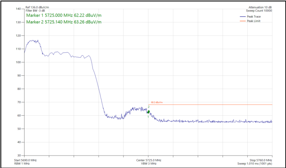
Figure 410 - 802.11ax HE20, RU 52-37, SDM, Core 0 - Core 1 - 5700 MHz Band Edge Frequency 5725 MHz
