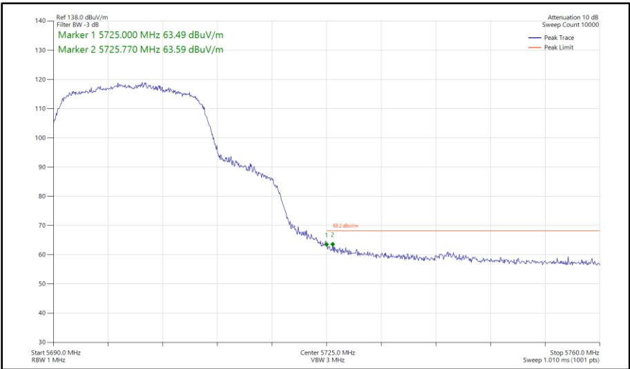
Figure 371 - 802.11n HT20, SISO, Core 1 - 5700 MHz Band Edge Frequency 5725 MHz
