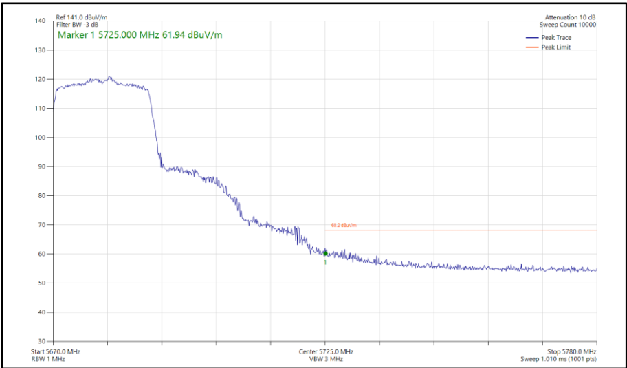
Figure 407 - 802.11ax HE20, SU, SDM, Core 0 - Core 1 - 5680 MHz Band Edge Frequency 5725 MHz
