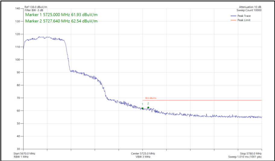
Figure 344 - 802.11ax HE20, SU, SISO, Core 0 - 5680 MHz Band Edge Frequency 5725 MHz
