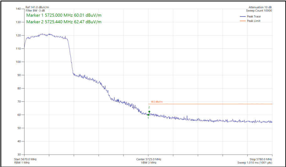
Figure 372 - 802.11ax HE20, SU, SISO, Core 1 - 5680 MHz Band Edge Frequency 5725 MHz
