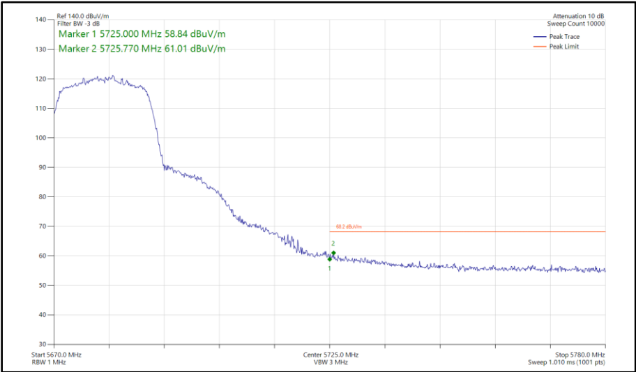
Figure 370 - 802.11n HT20, SISO, Core 1 - 5680 MHz Band Edge Frequency 5725 MHz
