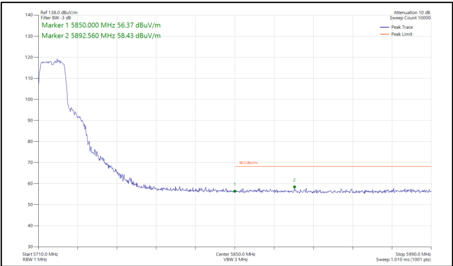
Figure 411 - 802.11n HT20, SDM, Core 0 - Core 1 - 5720 MHz Band Edge Frequency 5850 MHz
