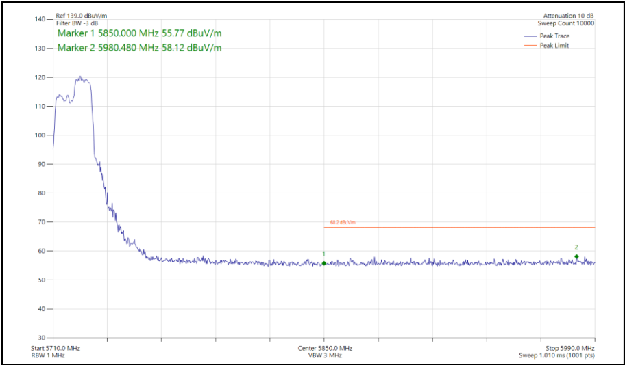
Figure 414 - 802.11ax HE20, RU 106-54, SDM, Core 0 - Core 1 - 5720 MHz Band Edge Frequency 5850 MHz
