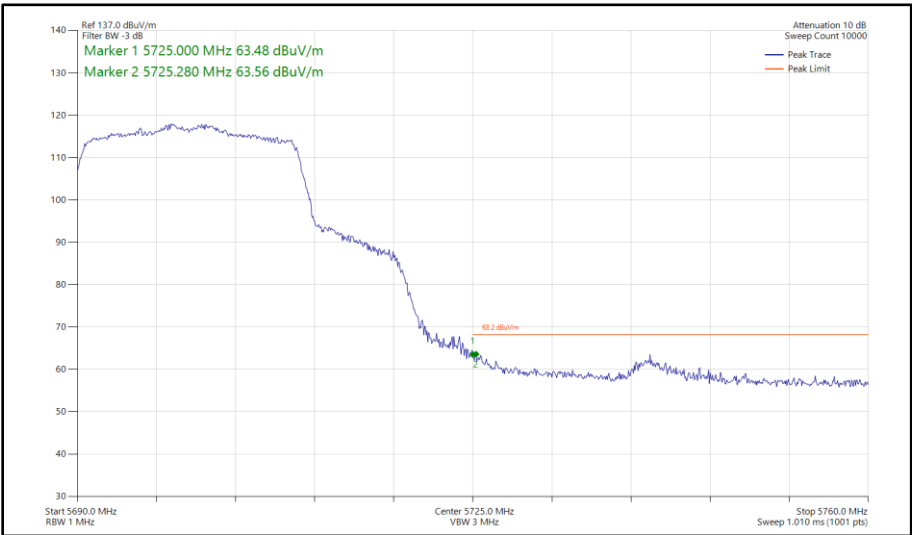
Figure 409 - 802.11ax HE20, SU, SDM, Core 0 - Core 1 - 5700 MHz Band Edge Frequency 5725 MHz
