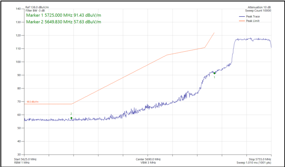
Figure 338 - 802.11ax HE20, SU, SISO, Core 0 - 5745 MHz Band Edge Frequency 5725 MHz
