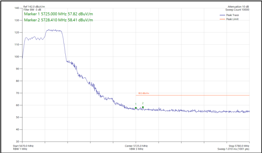
Figure 408 - 802.11ax HE20, RU 106-54, SDM, Core 0 - Core 1 - 5680 MHz Band Edge Frequency 5725 MHz
