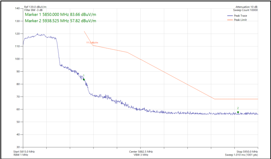
Figure 416 - 802.11ax HE20, SU, SDM, Core 0 - Core 1 - 5825 MHz Band Edge Frequency 5850 MHz
