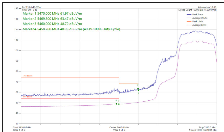
Figure 399 - 802.11n HT20, SDM, Core 0 - Core 1 - 5500 MHz Band Edge Frequency 5470 MHz
