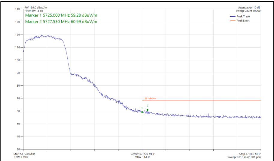
Figure 405 - 802.11n HT20, SDM, Core 0 - Core 1 - 5680 MHz Band Edge Frequency 5725 MHz
