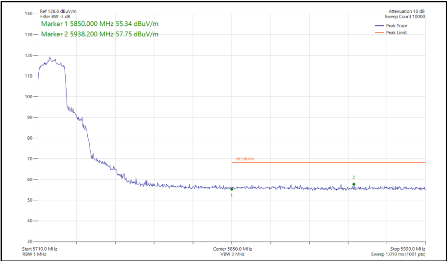
Figure 352 - 802.11ax HE20, SU, SISO, Core 0 - 5720 MHz Band Edge Frequency 5850 MHz
