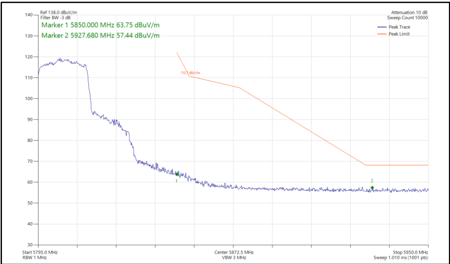
Figure 415 - 802.11ax HE20, SU, SDM, Core 0 - Core 1 - 5805 MHz Band Edge Frequency 5850 MHz
