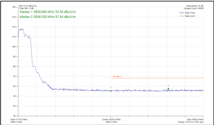
Figure 353 - 802.11ax HE20, RU 106-53, SISO, Core 0 - 5720 MHz Band Edge Frequency 5850 MHz
