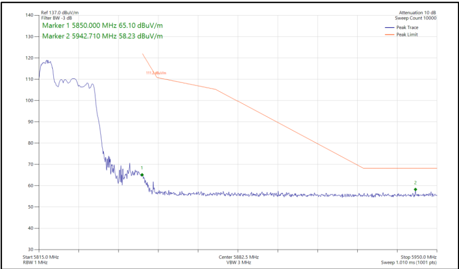
Figure 383 - 802.11ax HE20, RU 52-37, SISO, Core 1 - 5825 MHz Band Edge Frequency 5850 MHz
