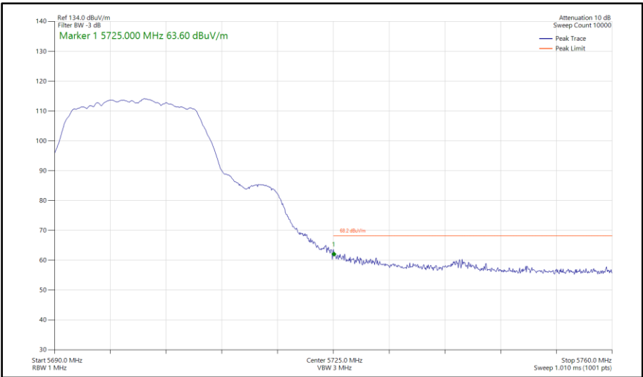
Figure 341 - 802.11a, SISO, Core 0 - 5700 MHz Band Edge Frequency 5725 MHz
