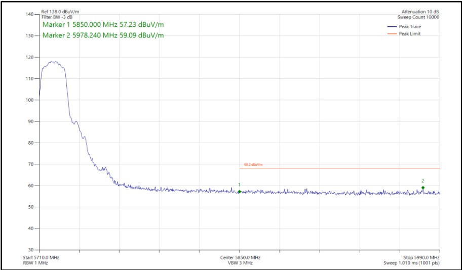
Figure 376 - 802.11a, SISO, Core 1 - 5720 MHz Band Edge Frequency 5850 MHz
