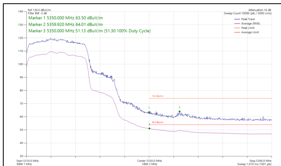
Figure 53 - 802.11ax HE20, SU, CDD, Core 0 - Core 1 - 5320 MHz Band Edge Frequency 5350 MHz
