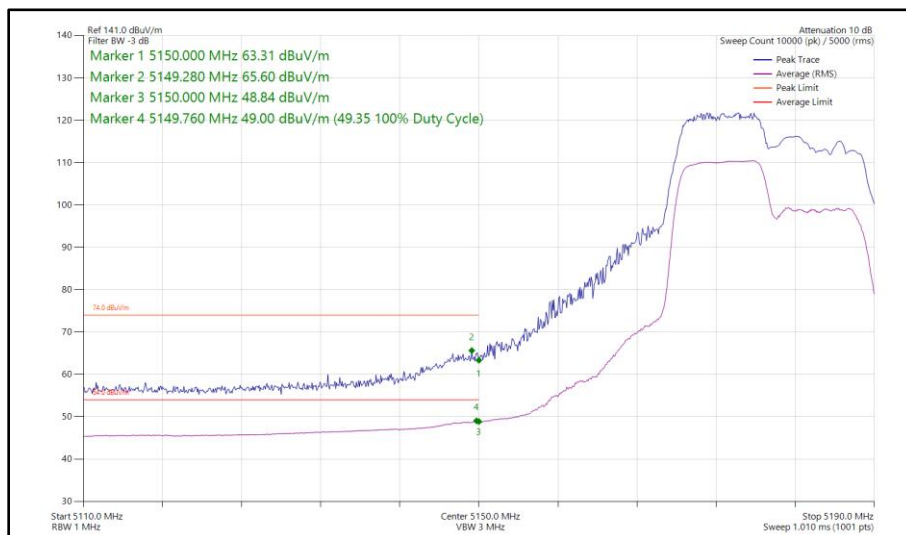
Figure 51 - 802.11ax HE20, RU 106-53, CDD, Core 0 - Core 1 - 5180 MHz Band Edge Frequency 5150 MHz
