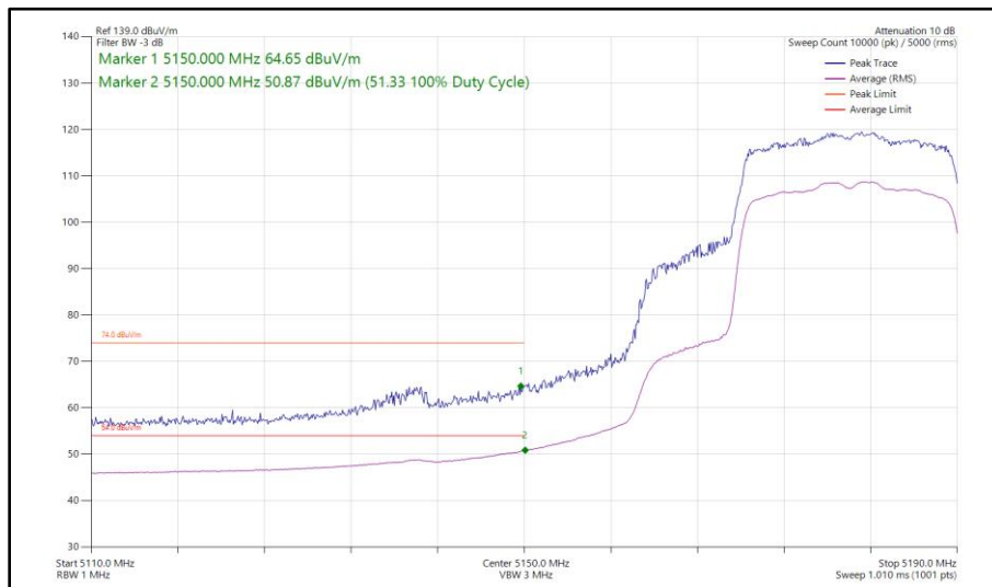
Figure 59 - 802.11ax HE20, SU, SDM, Core 0 - Core 1 - 5180 MHz Band Edge Frequency 5150 MHz
