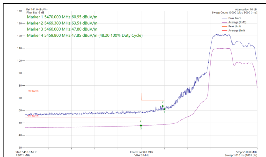
Figure 57 - 802.11ax HE20, RU 106-53, CDD, Core 0 - Core 1 - 5500 MHz Band Edge Frequency 5460 MHz
