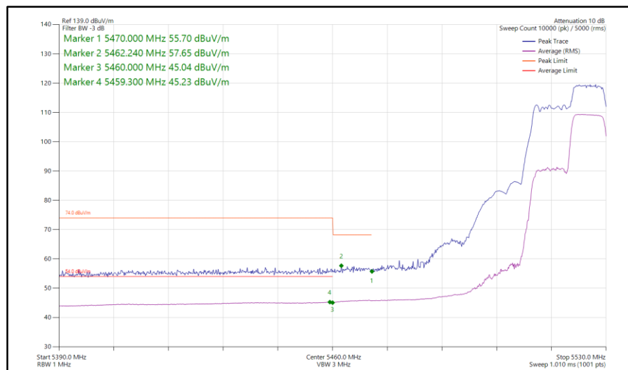
Figure 24 - 802.11ax HE20, RU 106-54, SISO, Core 0 - 5520 MHz Band Edge Frequency 5460 MHz
