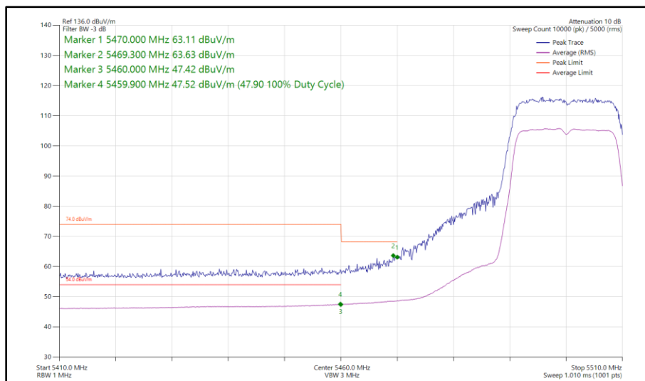
Figure 55 - 802.11n HT20, CDD, Core 0 - Core 1 - 5500 MHz Band Edge Frequency 5460 MHz
