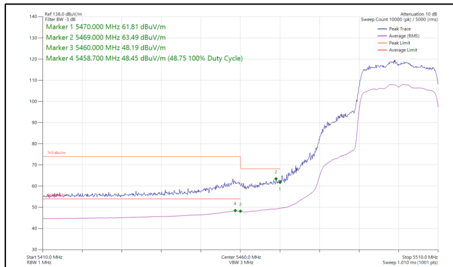
Figure 56 - 802.11ax HE20, SU, CDD, Core 0 - Core 1 - 5500 MHz Band Edge Frequency 5460 MHz
