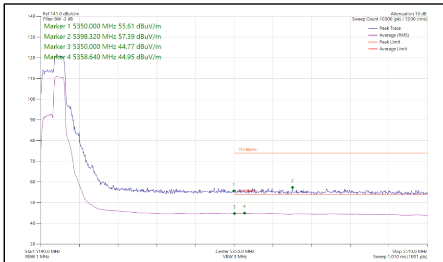
Figure 13 - 802.11ax HE20, RU 106-54, SISO, Core 0 - 5200 MHz Band Edge Frequency 5350 MHz
