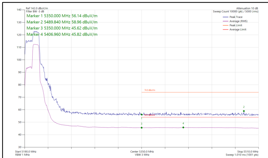
Figure 37 - 802.11ax HE20, RU 106-54, SISO, Core 1 - 5200 MHz Band Edge Frequency 5350 MHz
