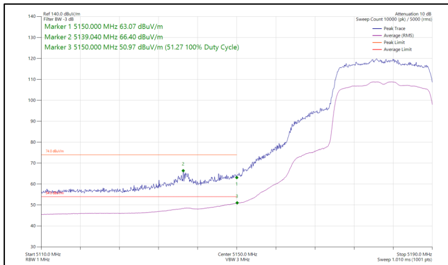
Figure 50 - 802.11ax HE20, SU, CDD, Core 0 - Core 1 - 5180 MHz Band Edge Frequency 5150 MHz
