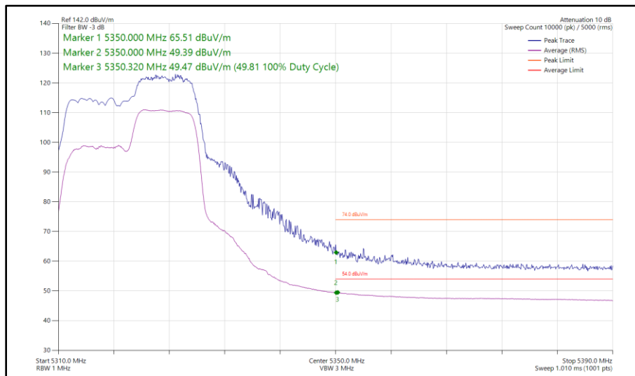
Figure 54 - 802.11ax HE20, RU 106-54, CDD, Core 0 - Core 1 - 5320 MHz Band Edge Frequency 5350 MHz
