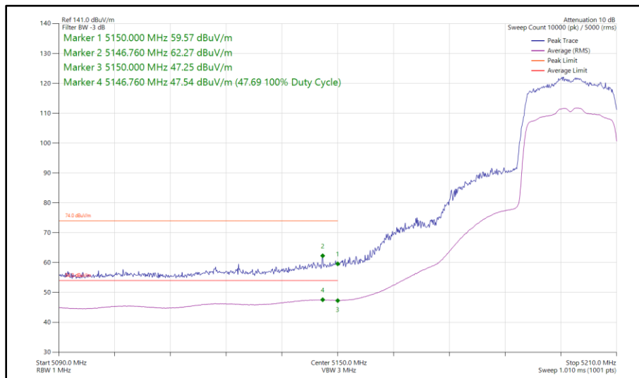
Figure 31 - 802.11ax HE20, SU, SISO, Core 1 - 5200 MHz Band Edge Frequency 5150 MHz
