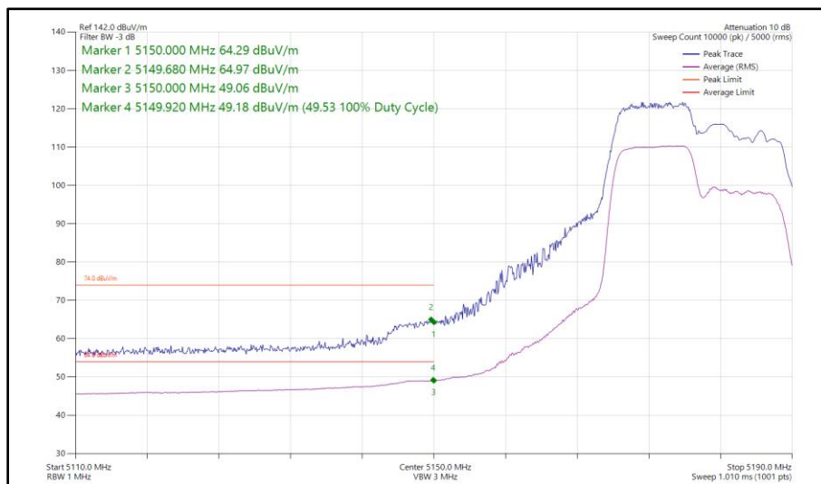
Figure 60 - 802.11ax HE20, RU 106-53, SDM, Core 0 - Core 1 - 5180 MHz Band Edge Frequency 5150 MHz
