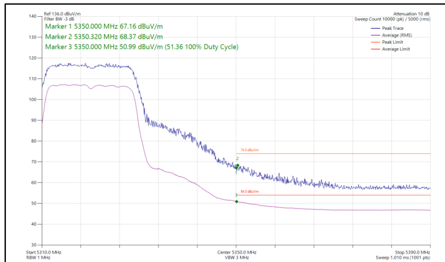
Figure 52 - 802.11n HT20, CDD, Core 0 - Core 1 - 5320 MHz Band Edge Frequency 5350 MHz
