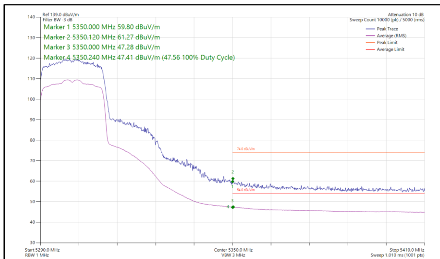
Figure 14 - 802.11ax HE20, SU, SISO, Core 0 - 5300 MHz Band Edge Frequency 5350 MHz
