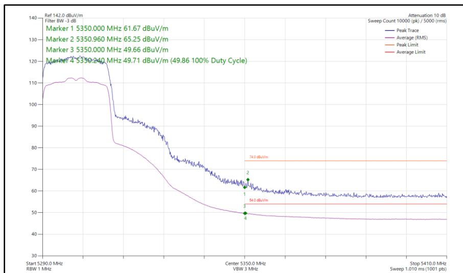
Figure 38 - 802.11ax HE20, SU, SISO, Core 1 - 5300 MHz Band Edge Frequency 5350 MHz
