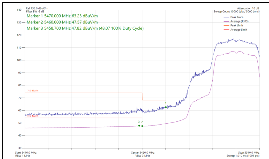
Figure 19 - 802.11n HT20, SISO, Core 0 - 5500 MHz Band Edge Frequency 5460 MHz
