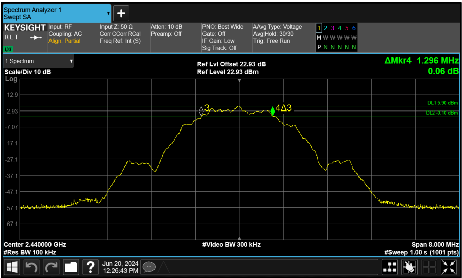
Figure 196 - Core 0 (A) 2440 MHz (CH17) 6 dB Bandwidth
