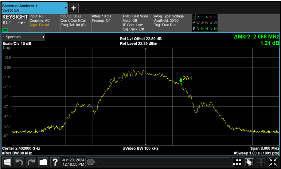
Figure 193 - Core 1 (B) 2402 MHz (CH37) 99% Bandwidth
