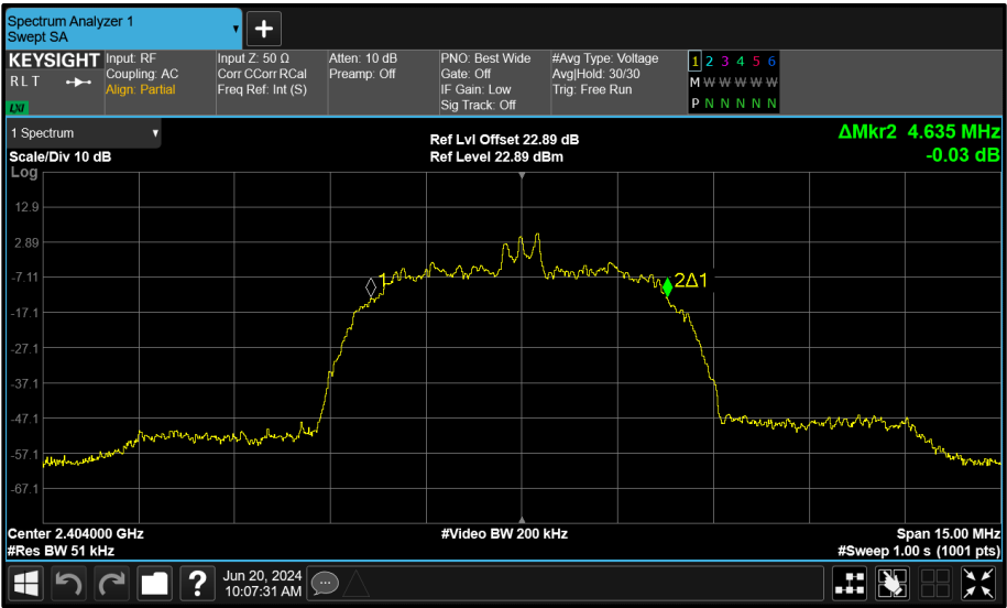
Figure 169 - Core 1 (B) 2404 MHz (CH2) 99% Bandwidth
