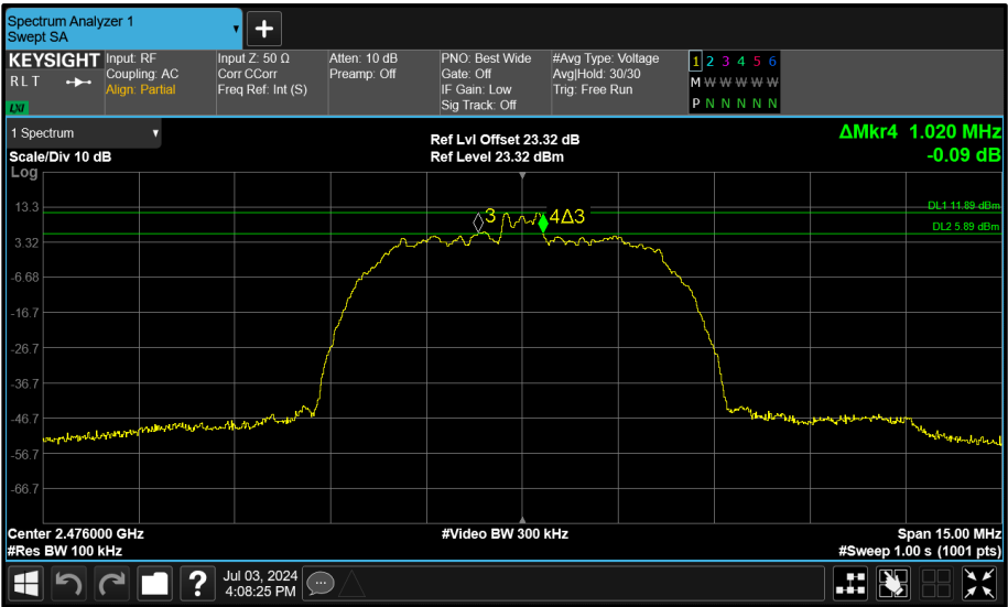
Figure 226 - Core 1 (B) 2476 MHz (CH74) 6 dB Bandwidth
