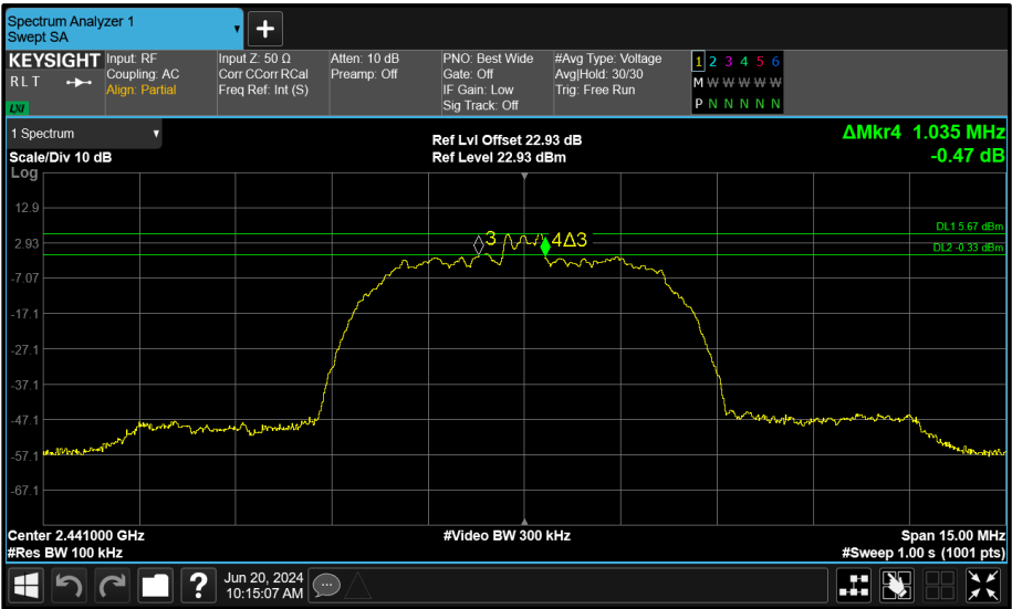
Figure 172 - Core 0 (A) 2441 MHz (CH39) 6 dB Bandwidth
