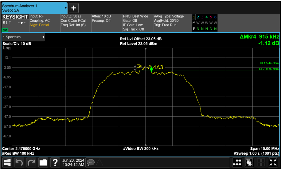
Figure 176 - Core 0 (A) 2476 MHz (CH74) 6 dB Bandwidth
