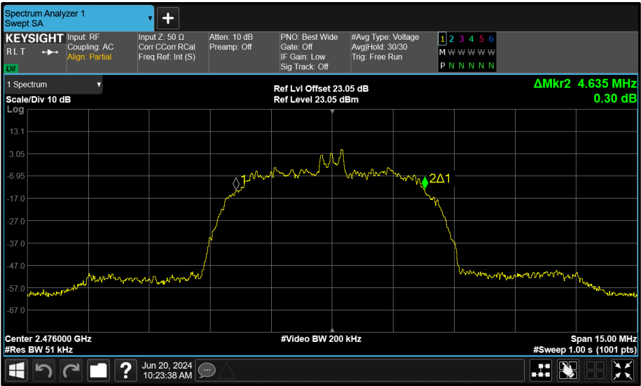
Figure 175 - Core 0 (A) 2476 MHz (CH74) 99% Bandwidth
