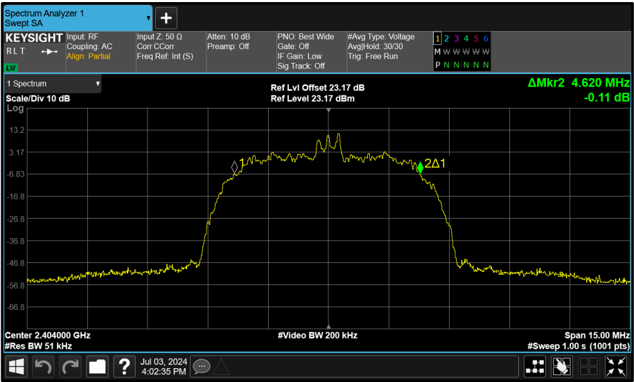
Figure 217 - Core 1 (B) 2404 MHz (CH2) 99% Bandwidth
