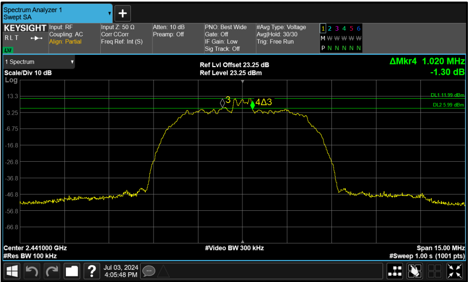
Figure 222 - Core 1 (B) 2441 MHz (CH39) 6 dB Bandwidth
