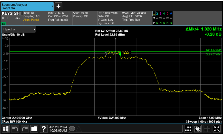
Figure 170 - Core 1 (B) 2404 MHz (CH2) 6 dB Bandwidth
