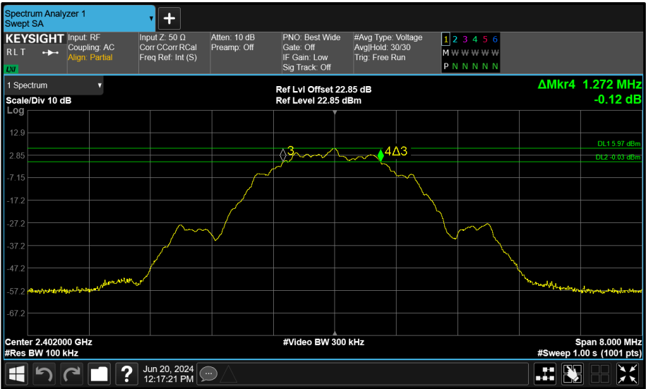
Figure 192 - Core 0 (A) 2402 MHz (CH37) 6 dB Bandwidth
