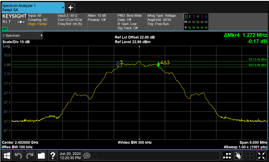
Figure 194 - Core 1 (B) 2402 MHz (CH37) 6 dB Bandwidth
