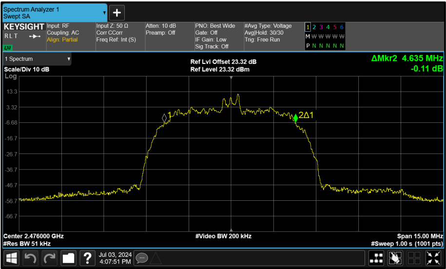
Figure 225 - Core 1 (B) 2476 MHz (CH74) 99% Bandwidth
