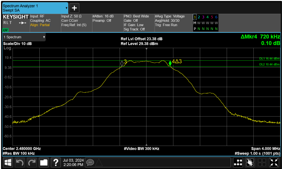
Figure 148 - Core 0 (A) 2480 MHz (CH39) 6 dB Bandwidth
