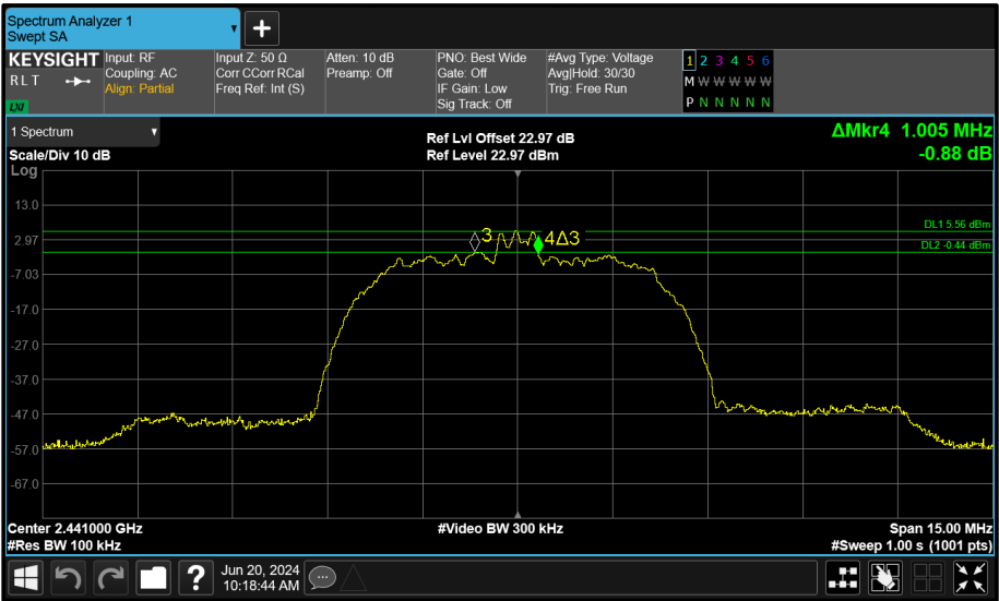
Figure 174 - Core 1 (B) 2441 MHz (CH39) 6 dB Bandwidth
