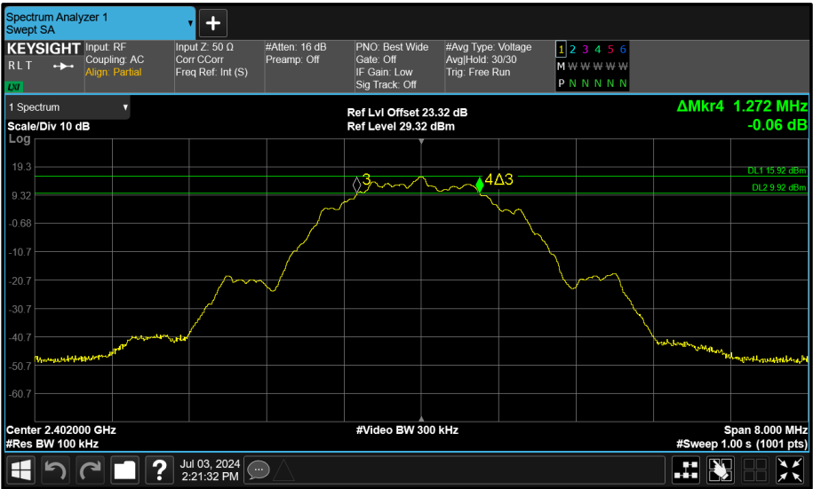
Figure 150 - Core 0 (A) 2402 MHz (CH37) 6 dB Bandwidth
