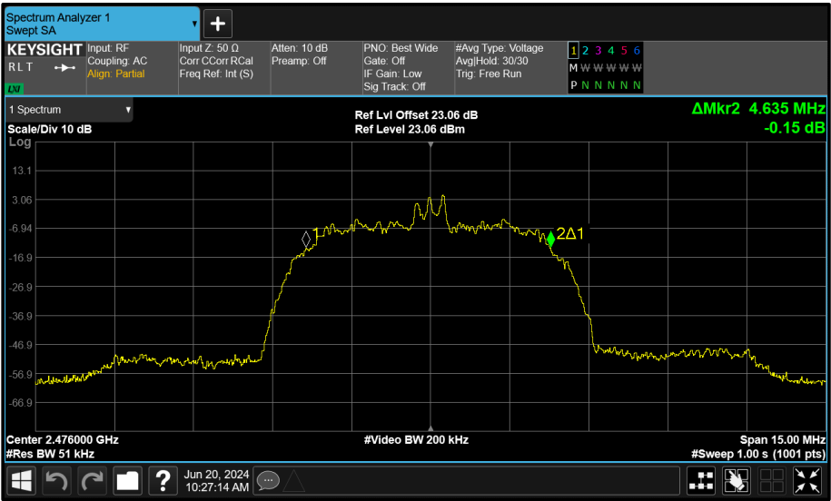
Figure 177 - Core 1 (B) 2476 MHz (CH74) 99% Bandwidth
