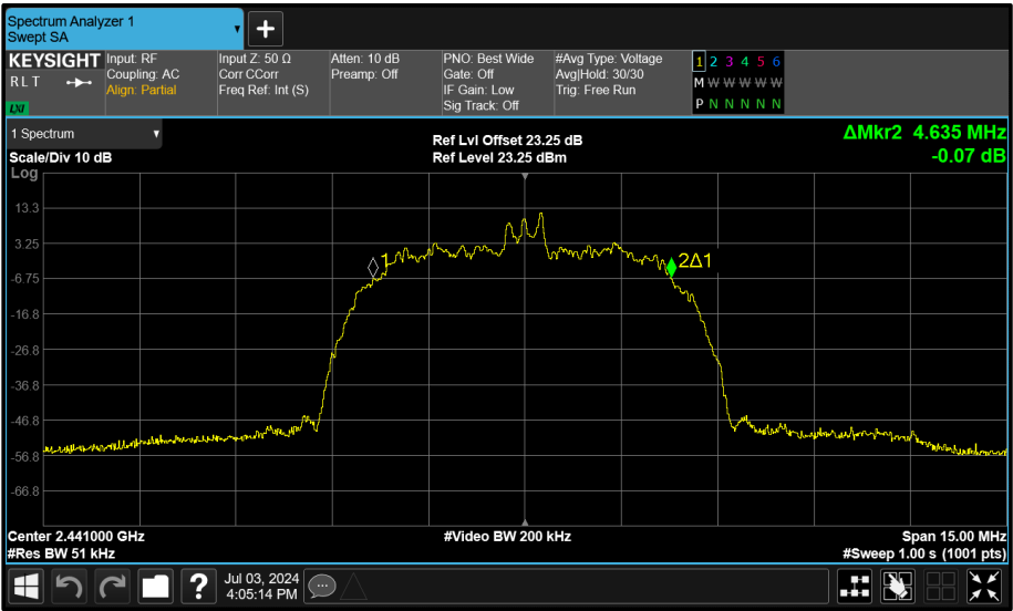
Figure 221 - Core 1 (B) 2441 MHz (CH39) 99% Bandwidth
