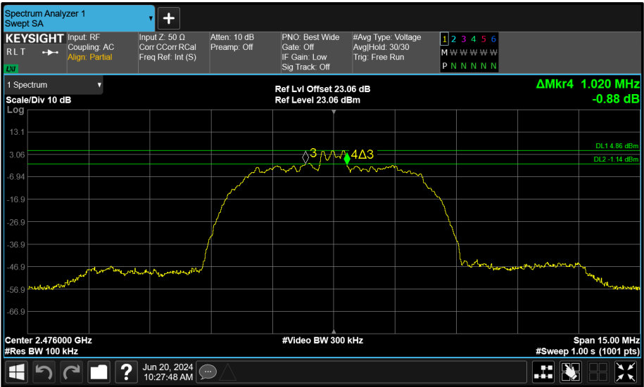
Figure 178 - Core 1 (B) 2476 MHz (CH74) 6 dB Bandwidth
