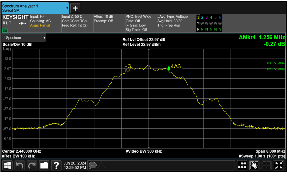
Figure 198 - Core 1 (B) 2440 MHz (CH17) 6 dB Bandwidth
