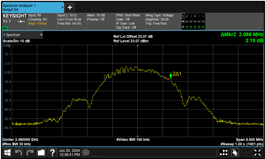
Figure 199 - Core 0 (A) 2480 MHz (CH39) 99% Bandwidth
