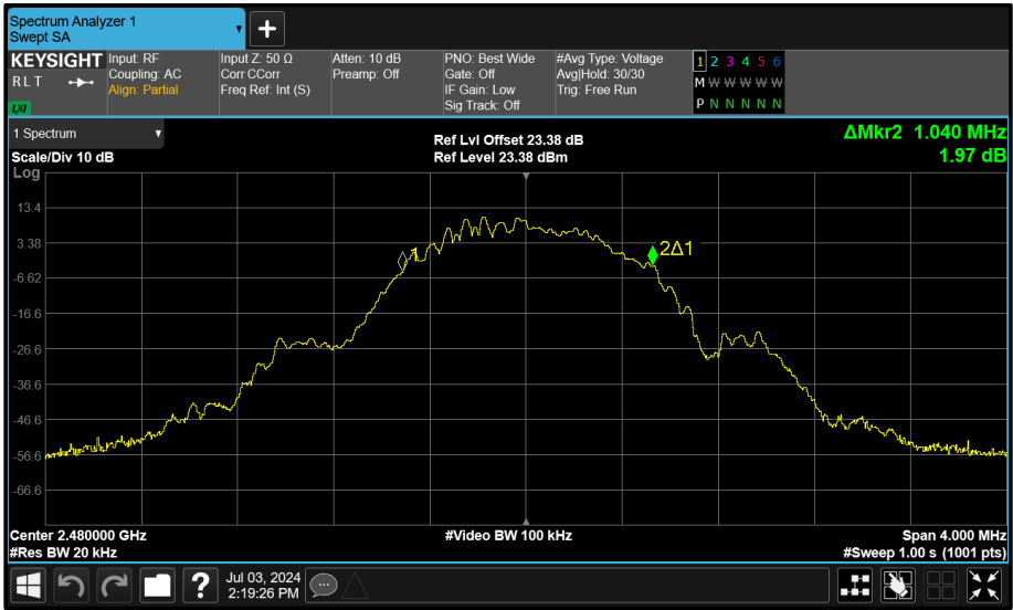
Figure 147 - Core 0 (A) 2480 MHz (CH39) 99% Bandwidth
