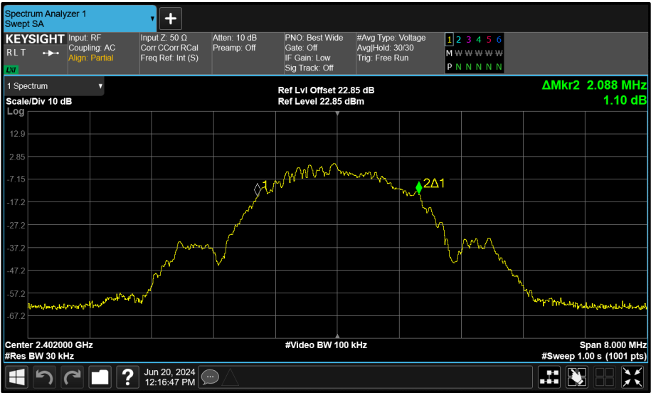
Figure 191 - Core 0 (A) 2402 MHz (CH37) 99% Bandwidth
