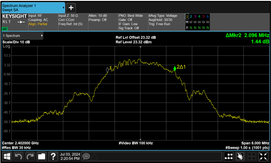
Figure 149 - Core 0 (A) 2402 MHz (CH37) 99% Bandwidth
