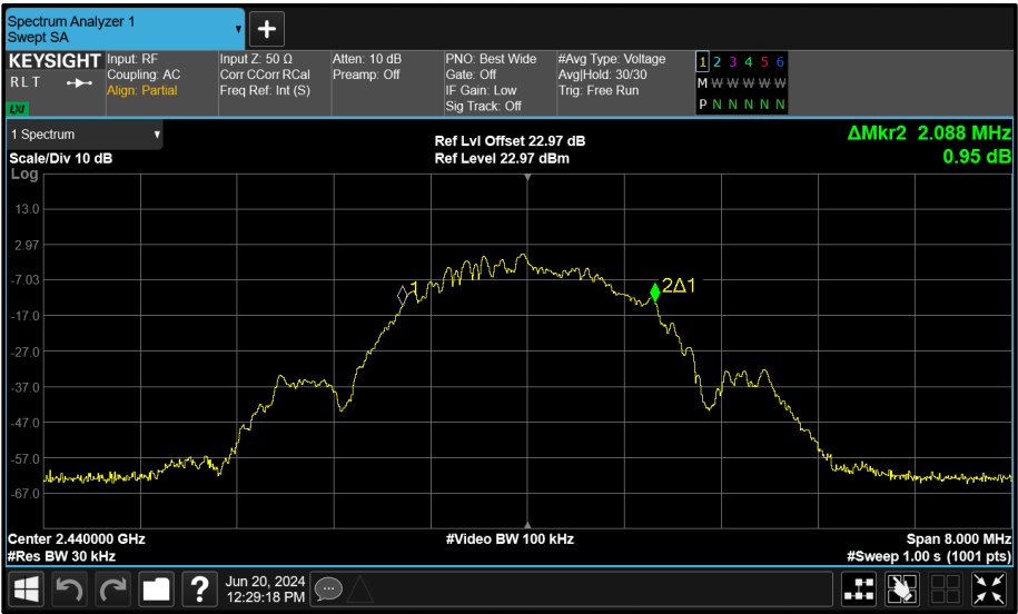
Figure 197 - Core 1 (B) 2440 MHz (CH17) 99% Bandwidth
