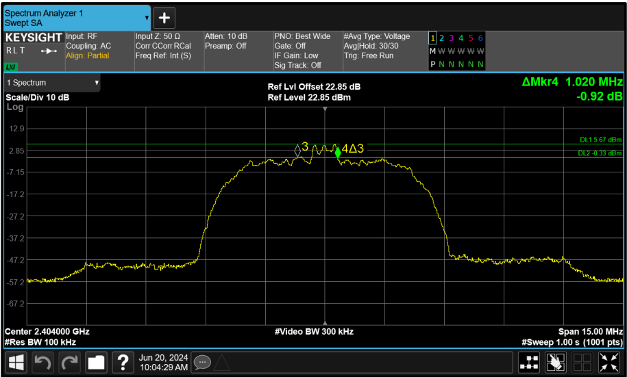
Figure 168 - Core 0 (A) 2404 MHz (CH2) 6 dB Bandwidth
