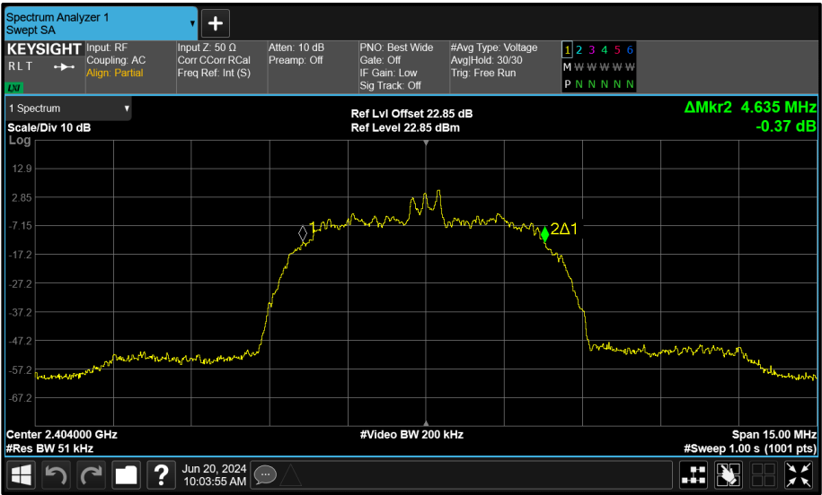
Figure 167 - Core 0 (A) 2404 MHz (CH2) 99% Bandwidth
