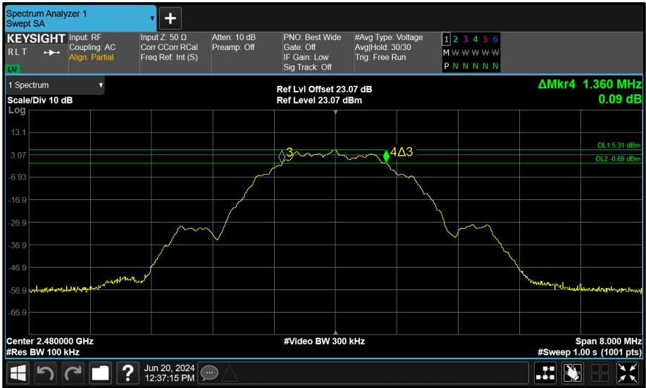
Figure 200 - Core 0 (A) 2480 MHz (CH39) 6 dB Bandwidth
