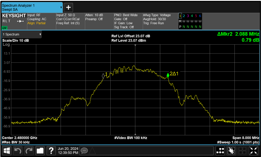
Figure 201 - Core 1 (B) 2480 MHz (CH39) 99% Bandwidth
