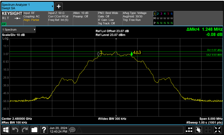
Figure 202 - Core 1 (B) 2480 MHz (CH39) 6 dB Bandwidth
