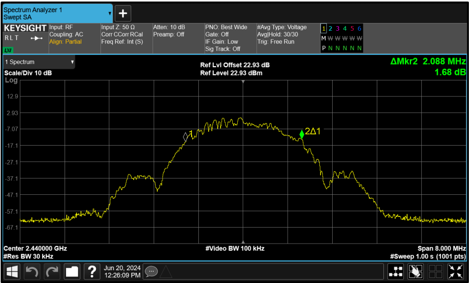
Figure 195 - Core 0 (A) 2440 MHz (CH17) 99% Bandwidth
