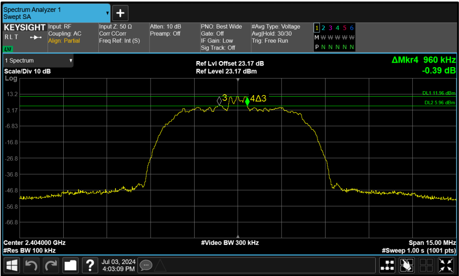
Figure 218 - Core 1 (B) 2404 MHz (CH2) 6 dB Bandwidth
