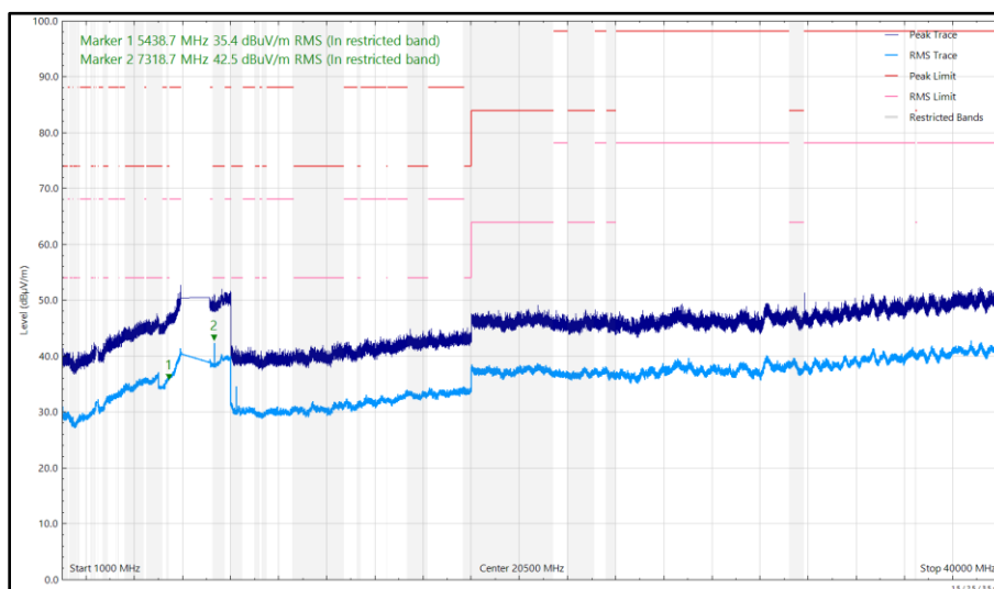
Figure 67 - U-NII-5 - 6175 MHz (CH45), HE20, SU, CDD, Core 0 + Core 1 and 2440 MHz (CH18), ePA, Core 1, 1 GHz to 40 GHz, Horizontal
