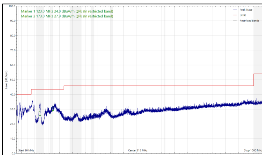
Figure 68 - U-NII-5 - 6175 MHz (CH45), HE20, SU, CDD, Core 0 + Core 1 and 2440 MHz (CH18), ePA, Core 1, 30 MHz to 1 GHz, Vertical (Peak)
