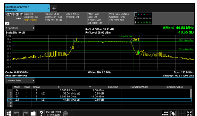
Figure 158 - 802.11ax HE20 SU SP Maximum 26 dB EBW
