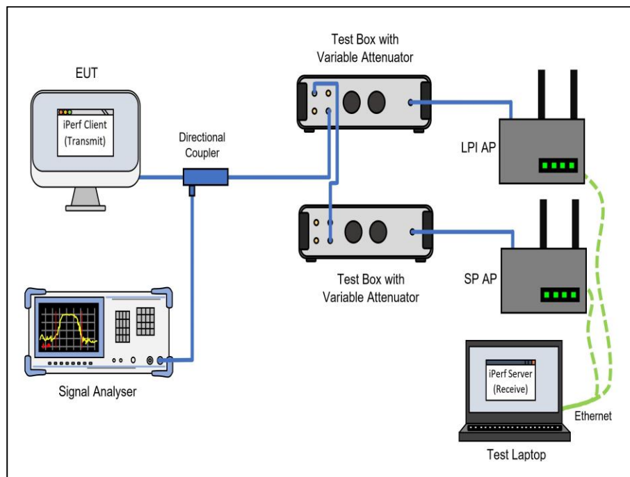
Figure 173 - Test Equipment Setup Diagram
