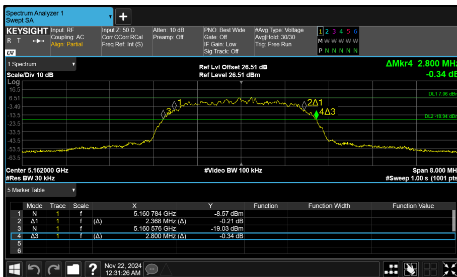
Figure 40 - Core 0 (A) 5162 MHz (CH12) 26 dB and 99% Bandwidth
