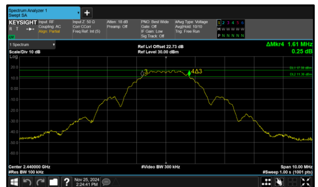
Figure 18 - Core 0 (A) 2440 MHz (CH18) 6 dB Bandwidth
