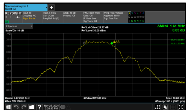
Figure 20 - Core 0 (A) 2475 MHz (CH25) 6 dB Bandwidth
