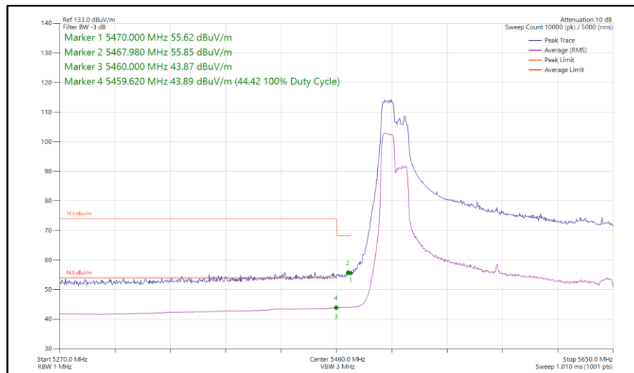
Figure 666 - 802.11ax HE160, RU 106-53P, SISO, Core 1 - 5570 MHz Band Edge Frequency 5470 MHz
