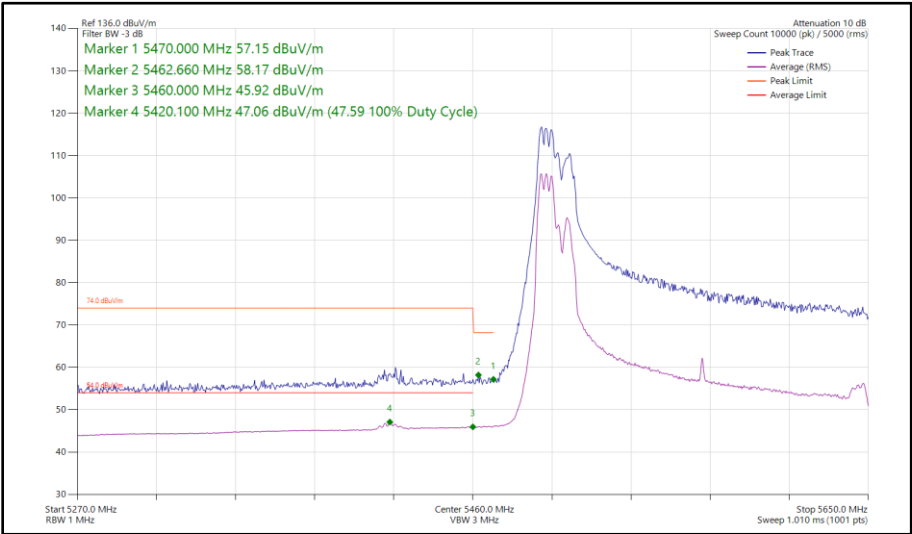
Figure 672 - 802.11ax HE160, RU 106-53P, CDD, Core 0 - Core 1 - 5570 MHz Band Edge Frequency 5470 MHz
