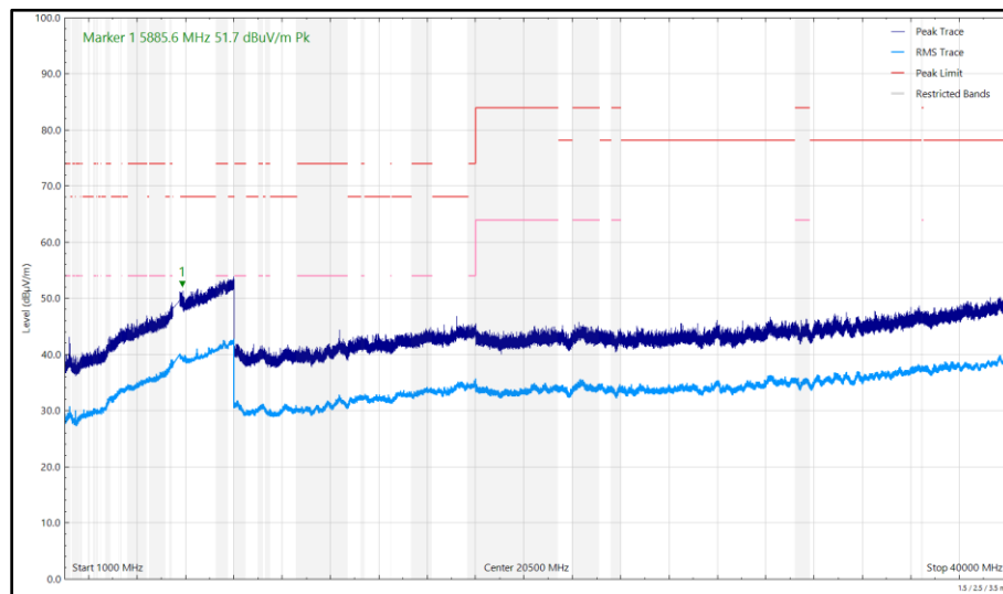
Figure 707 - U-NII-2C - 5700 MHz (CH140), 802.11a, Core 1, 1 GHz to 40 GHz, Horizontal
