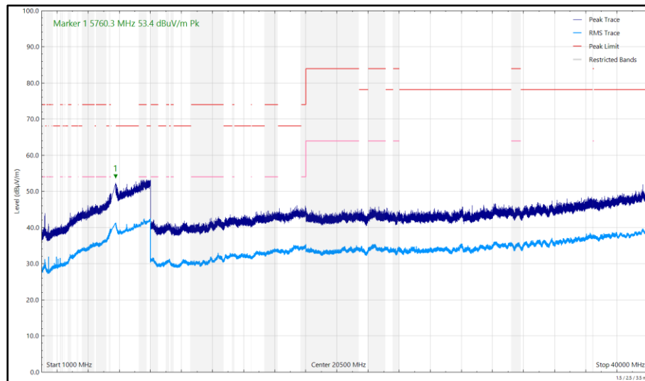
Figure 691 - U-NII-2C - 5700 MHz (CH140), 802.11a, Core 0, 1 GHz to 40 GHz, Horizontal
