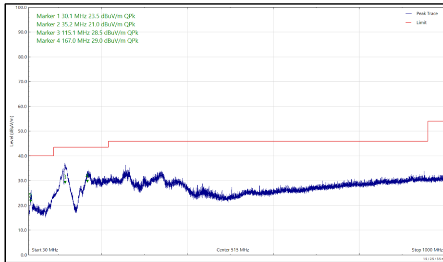
Figure 695 - U-NII-3 - 5825 MHz (CH165), 802.11a, Core 0, 30 MHz to 1 GHz, Horizontal (Peak)
