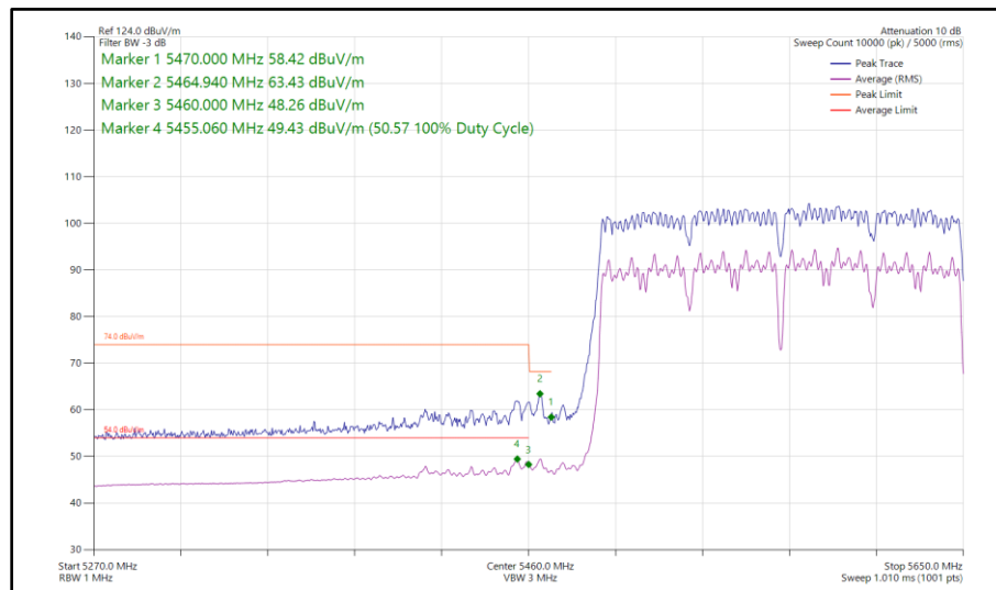
Figure 670 - 802.11ac VHT160, CDD, Core 0 - Core 1 - 5570 MHz Band Edge Frequency 5470 MHz
