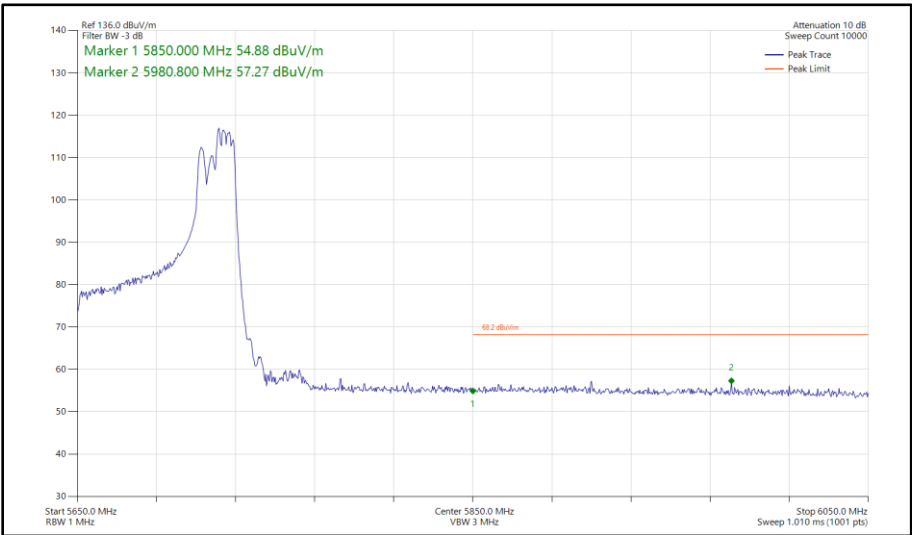
Figure 631 - 802.11ax HE80, RU 106-60, CDD, Core 0 - Core 1 - 5690 MHz Band Edge Frequency 5850 MHz
