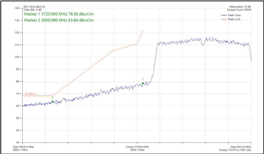
Figure 622 - 802.11ac VHT80, CDD, Core 0 - Core 1 - 5775 MHz Band Edge Frequency 5725 MHz
