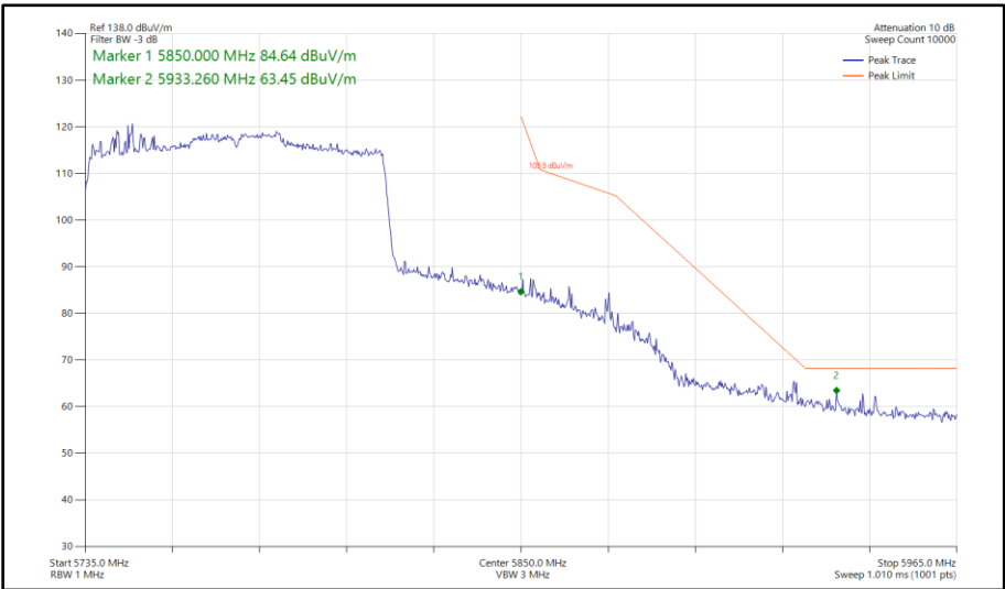
Figure 657 - 802.11ax HE80, SU, TxBF, Core 0 - Core 1 - 5775 MHz Band Edge Frequency 5850 MHz
