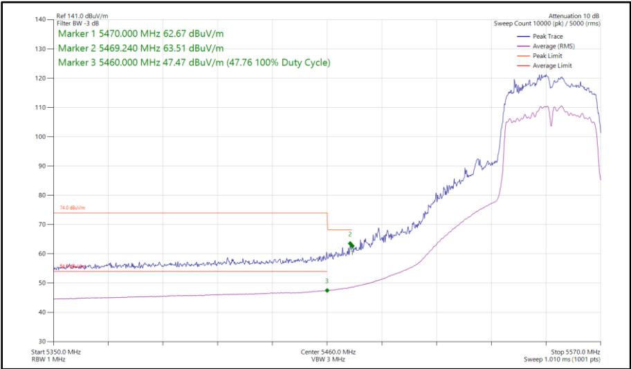
Figure 585 - 802.11ac VHT40, TxBF, Core 0 - Core 1 - 5550 MHz Band Edge Frequency 5470 MHz
