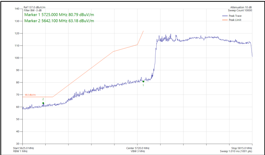
Figure 651 - 802.11ax HE80, SU, TxBF, Core 0 - Core 1 - 5775 MHz Band Edge Frequency 5725 MHz
