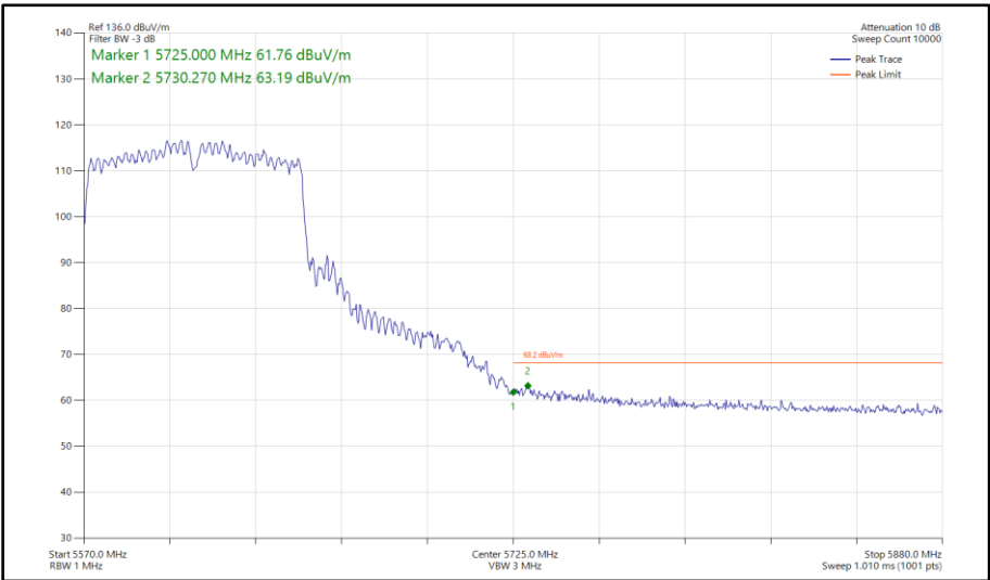
Figure 625 - 802.11ac VHT80, CDD, Core 0 - Core 1 - 5610 MHz Band Edge Frequency 5725 MHz
