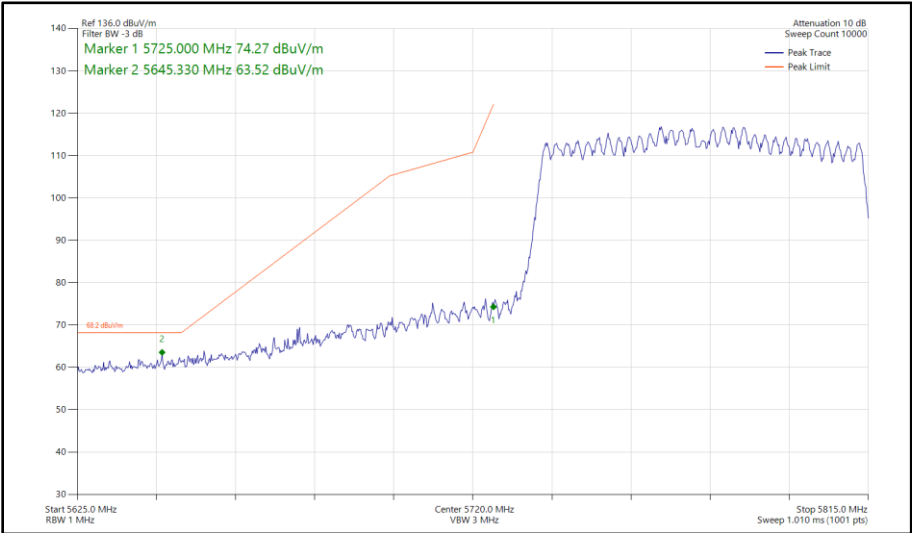
Figure 623 - 802.11ax HE80, SU, CDD, Core 0 - Core 1 - 5775 MHz Band Edge Frequency 5725 MHz
