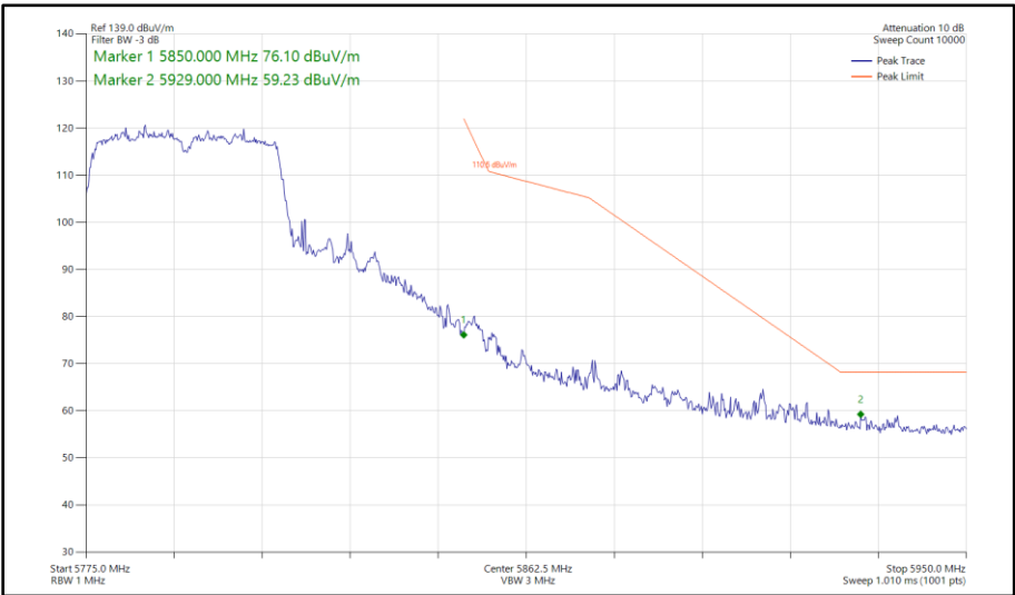
Figure 590 - 802.11ac VHT40, TxBF, Core 0 - Core 1 - 5795 MHz Band Edge Frequency 5850 MHz
