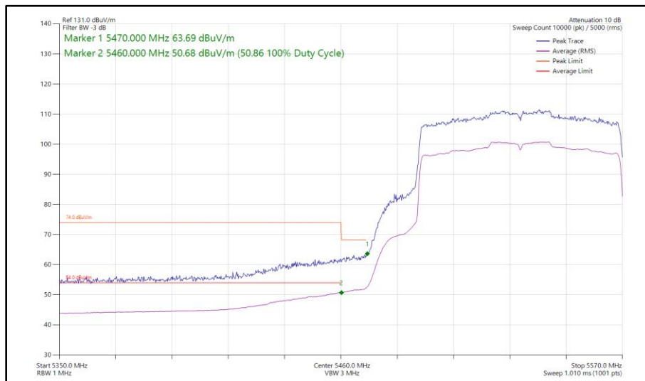
Figure 606 - 802.11ax HE80, SU, SISO, Core 1 - 5530 MHz Band Edge Frequency 5470 MHz
