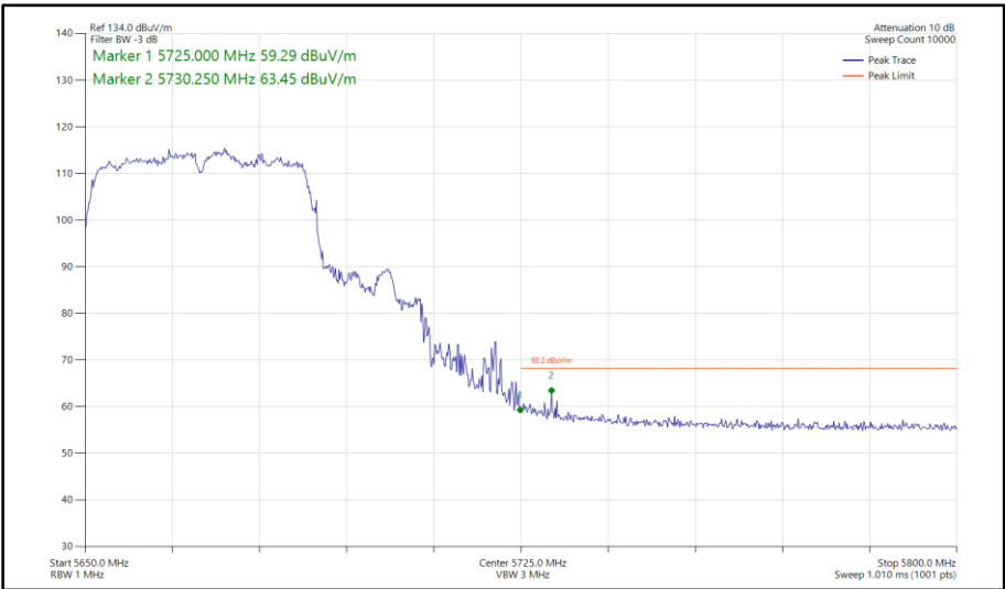
Figure 588 - 802.11ac VHT40, TxBF, Core 0 - Core 1 - 5670 MHz Band Edge Frequency 5725 MHz
