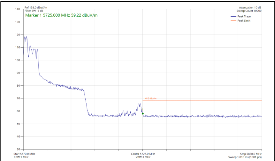
Figure 627 - 802.11ax HE80, RU 52-37, CDD, Core 0 - Core 1 - 5610 MHz Band Edge Frequency 5725 MHz
