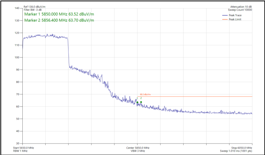
Figure 656 - 802.11ax HE80, SU, TxBF, Core 0 - Core 1 - 5690 MHz Band Edge Frequency 5850 MHz
