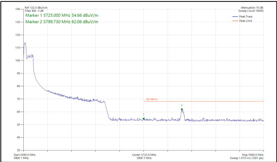
Figure 663 - 802.11ax HE160, RU 52-37P, SISO, Core 0 - 5570 MHz Band Edge Frequency 5725 MHz
