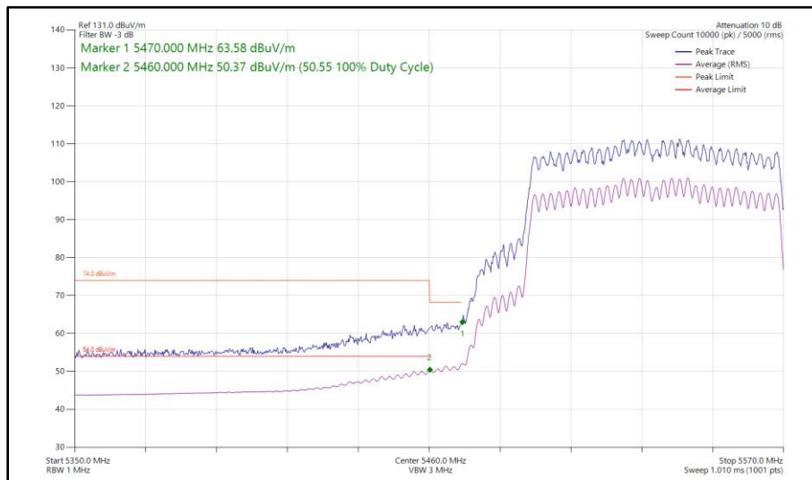
Figure 620 - 802.11ax HE80, SU, CDD, Core 0 - Core 1 - 5530 MHz Band Edge Frequency 5470 MHz
