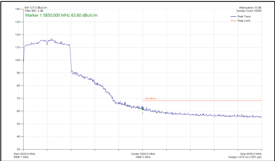
Figure 613 - 802.11ac VHT80, SISO, Core 1 - 5690 MHz Band Edge Frequency 5850 MHz
