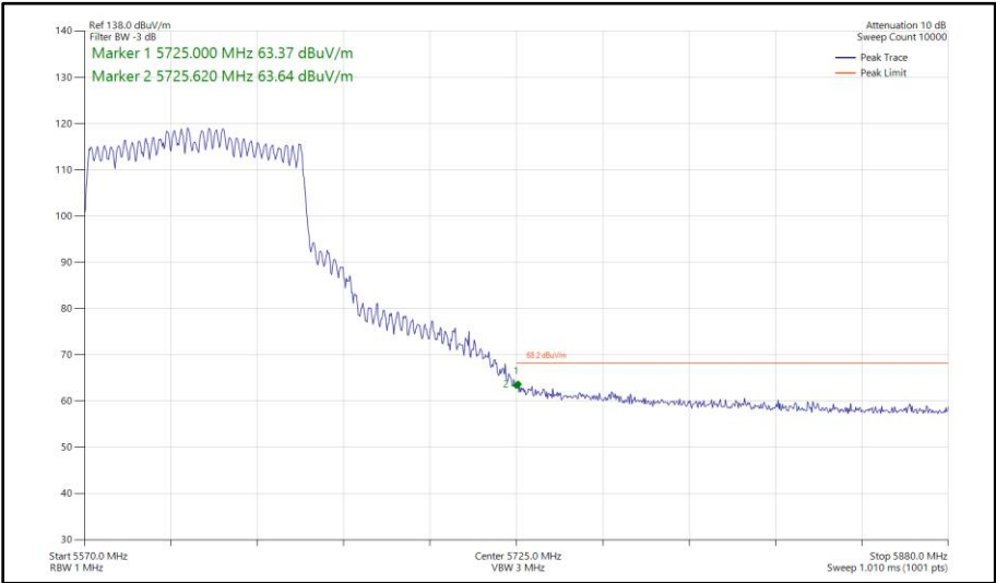
Figure 626 - 802.11ax HE80, SU, CDD, Core 0 - Core 1 - 5610 MHz Band Edge Frequency 5725 MHz
