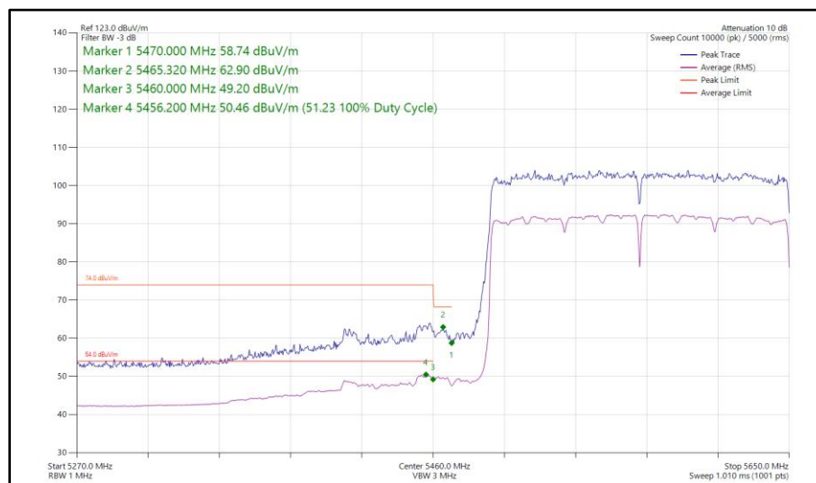
Figure 659 - 802.11ax HE160, SU, SISO, Core 0 - 5570 MHz Band Edge Frequency 5470 MHz
