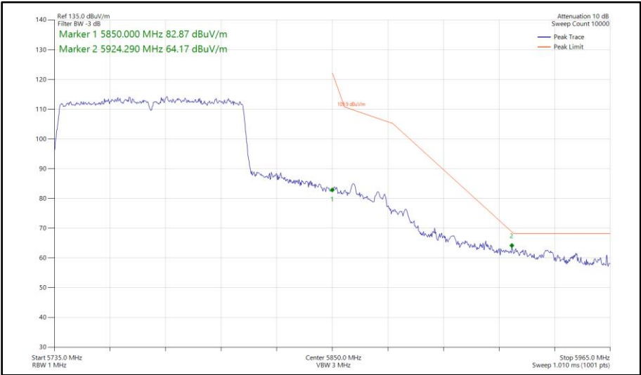
Figure 600 - 802.11ac VHT80, SISO, Core 0 - 5775 MHz Band Edge Frequency 5850 MHz
