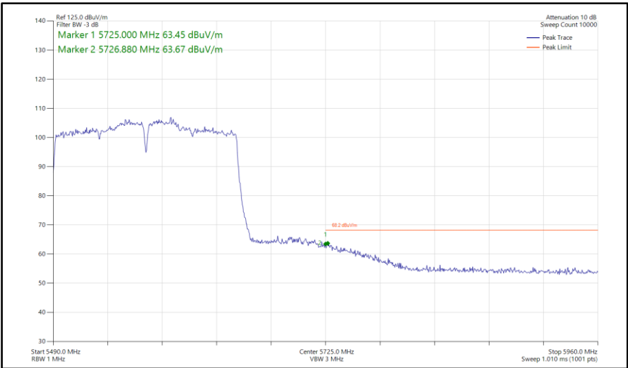
Figure 661 - 802.11ac VHT160, SISO, Core 0 - 5570 MHz Band Edge Frequency 5725 MHz
