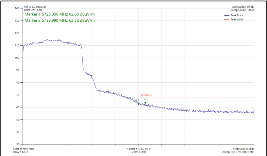
Figure 598 - 802.11ax HE80, SU, SISO, Core 0 - 5610 MHz Band Edge Frequency 5725 MHz
