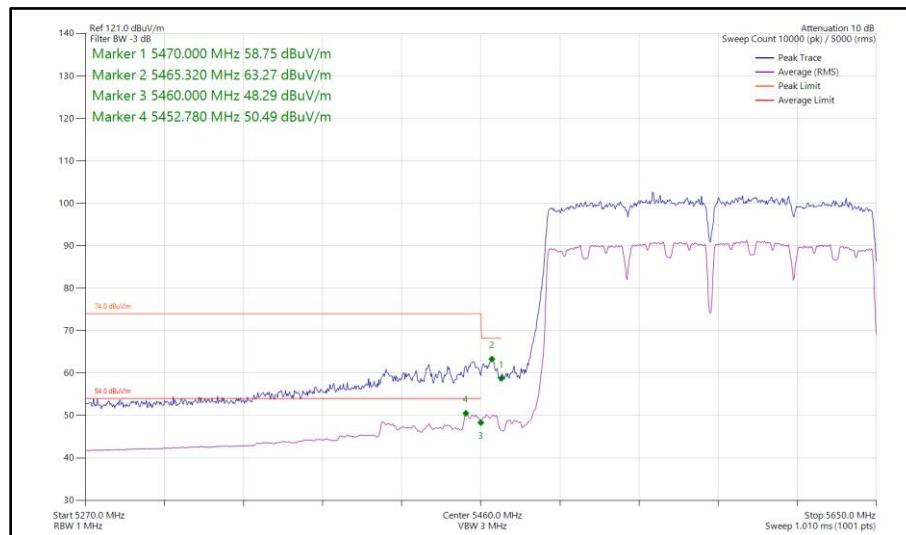
Figure 658 - 802.11ac VHT160, SISO, Core 0 - 5570 MHz Band Edge Frequency 5470 MHz
