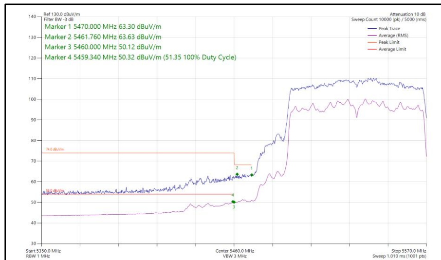
Figure 634 - 802.11ac VHT80, SDM, Core 0 - Core 1 - 5530 MHz Band Edge Frequency 5470 MHz
