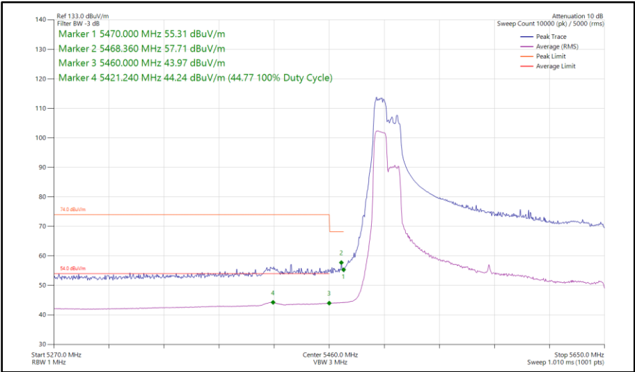
Figure 660 - 802.11ax HE160, RU 106-53P, SISO, Core 0 - 5570 MHz Band Edge Frequency 5470 MHz
