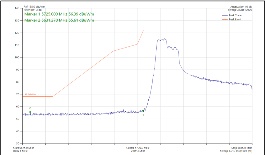
Figure 596 - 802.11ax HE80, RU 106-53, SISO, Core 0 - 5775 MHz Band Edge Frequency 5725 MHz
