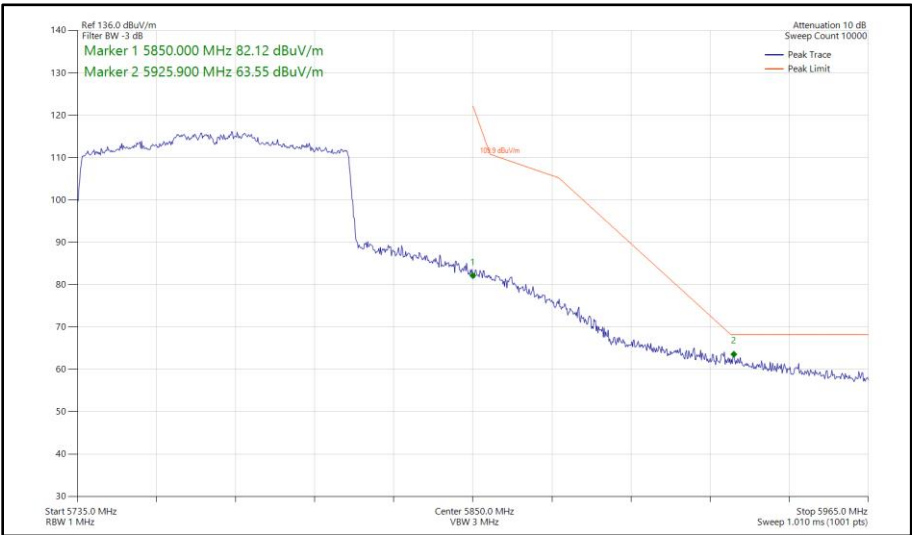
Figure 617 - 802.11ax HE80, SU, SISO, Core 1 - 5775 MHz Band Edge Frequency 5850 MHz
