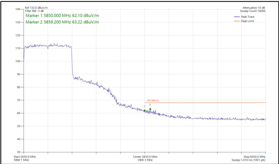
Figure 601 - 802.11ax HE80, SU, SISO, Core 0 - 5690 MHz Band Edge Frequency 5850 MHz
