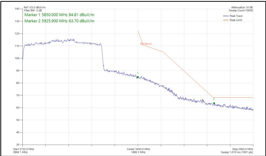
Figure 603 - 802.11ax HE80, SU, SISO, Core 0 - 5775 MHz Band Edge Frequency 5850 MHz
