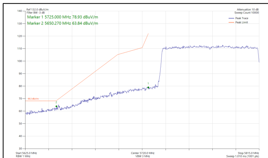
Figure 609 - 802.11ax HE80, SU, SISO, Core 1 - 5775 MHz Band Edge Frequency 5725 MHz
