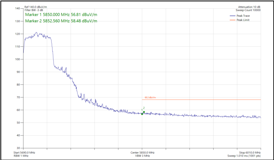
Figure 589 - 802.11ac VHT40, TxBF, Core 0 - Core 1 - 5710 MHz Band Edge Frequency 5850 MHz
