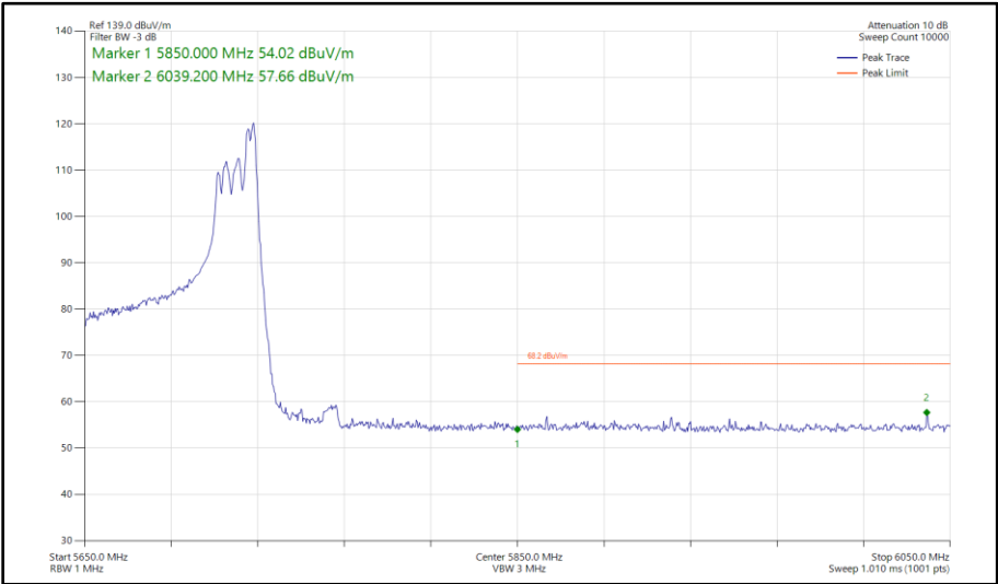
Figure 645 - 802.11ax HE80, RU 52-52, SDM, Core 0 - Core 1 - 5690 MHz Band Edge Frequency 5850 MHz
