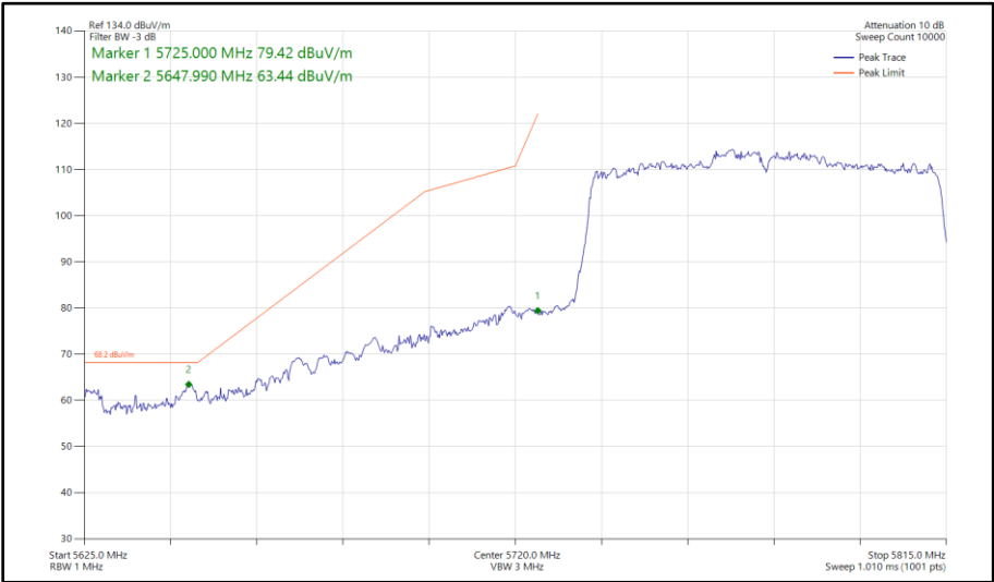
Figure 637 - 802.11ac VHT80, SDM, Core 0 - Core 1 - 5775 MHz Band Edge Frequency 5725 MHz
