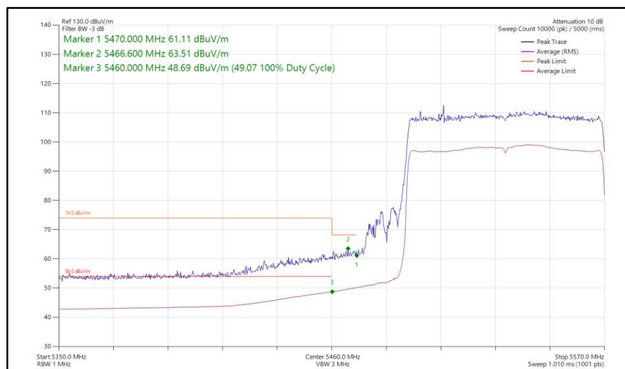
Figure 649 - 802.11ax HE80, SU, TxBF, Core 0 - Core 1 - 5530 MHz Band Edge Frequency 5470 MHz
