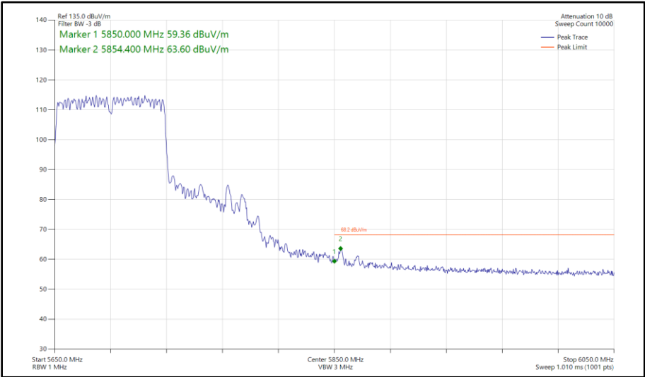
Figure 628 - 802.11ac VHT80, CDD, Core 0 - Core 1 - 5690 MHz Band Edge Frequency 5850 MHz
