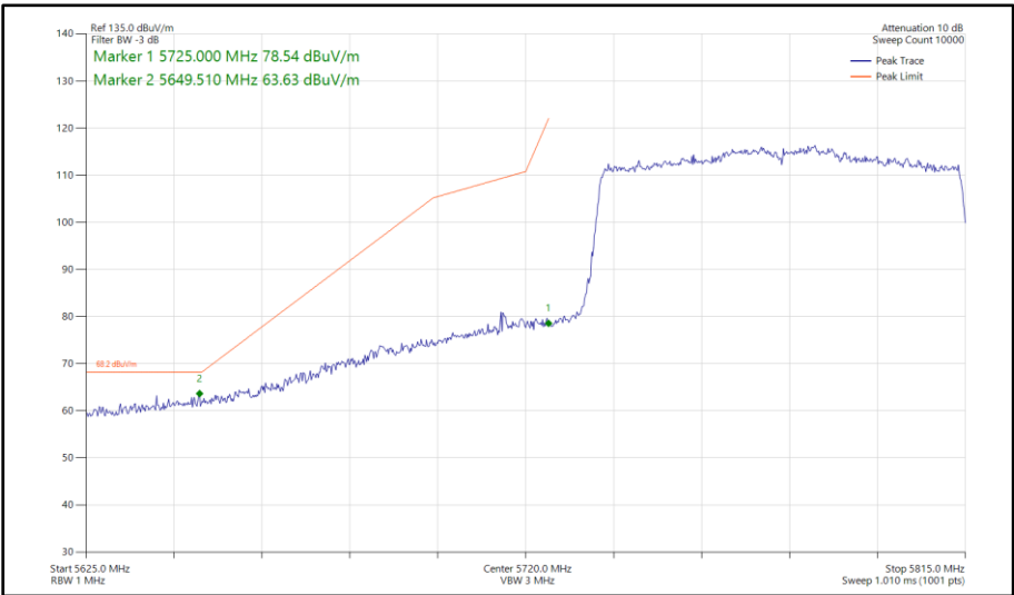
Figure 638 - 802.11ax HE80, SU, SDM, Core 0 - Core 1 - 5775 MHz Band Edge Frequency 5725 MHz
