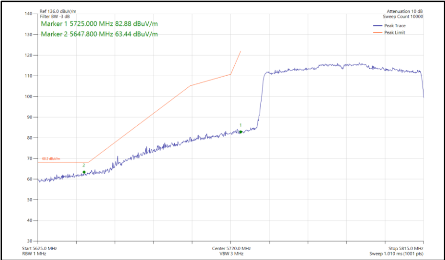
Figure 595 - 802.11ax HE80, SU, SISO, Core 0 - 5775 MHz Band Edge Frequency 5725 MHz
