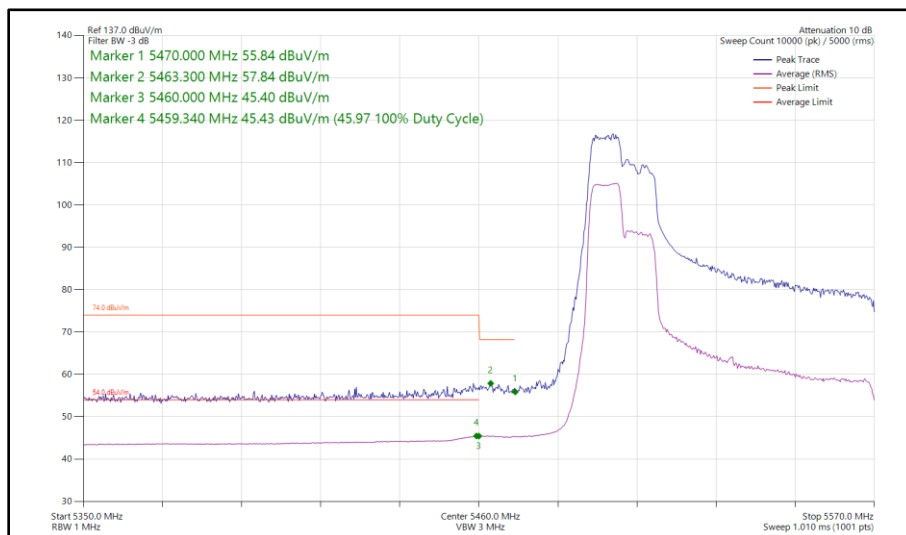
Figure 593 - 802.11ax HE80, RU 106-53, SISO, Core 0 - 5530 MHz Band Edge Frequency 5470 MHz
