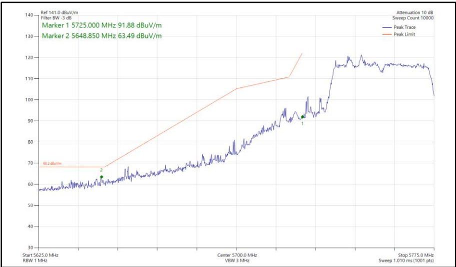
Figure 586 - 802.11ac VHT40, TxBF, Core 0 - Core 1 - 5755 MHz Band Edge Frequency 5725 MHz
