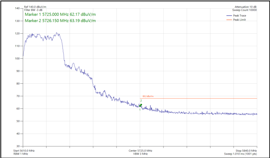
Figure 587 - 802.11ac VHT40, TxBF, Core 0 - Core 1 - 5630 MHz Band Edge Frequency 5725 MHz
