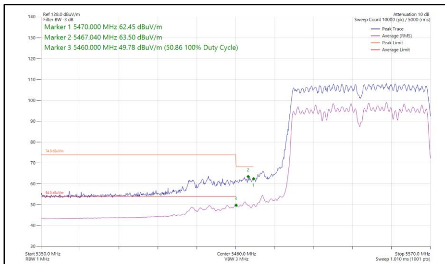
Figure 619 - 802.11ac VHT80, CDD, Core 0 - Core 1 - 5530 MHz Band Edge Frequency 5470 MHz
