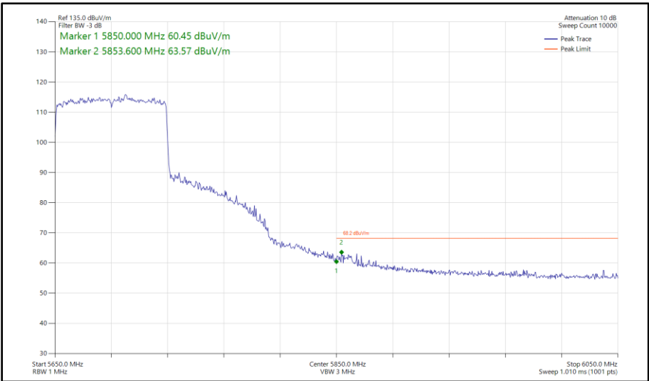
Figure 615 - 802.11ax HE80, SU, SISO, Core 1 - 5690 MHz Band Edge Frequency 5850 MHz
