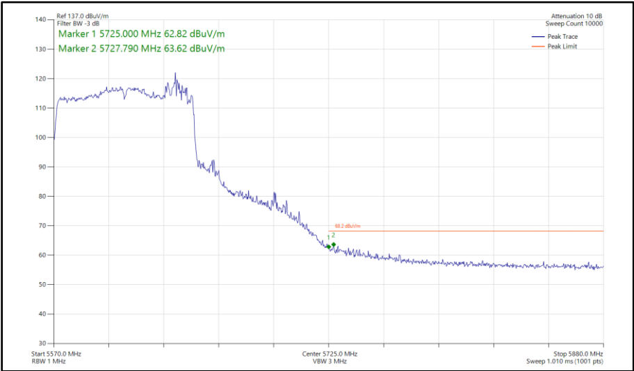
Figure 652 - 802.11ac VHT80, TxBF, Core 0 - Core 1 - 5610 MHz Band Edge Frequency 5725 MHz
