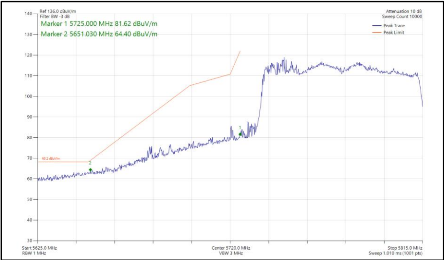
Figure 650 - 802.11ac VHT80, TxBF, Core 0 - Core 1 - 5775 MHz Band Edge Frequency 5725 MHz
