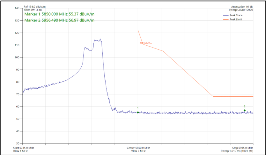
Figure 618 - 802.11ax HE80, RU 106-60, SISO, Core 1 - 5775 MHz Band Edge Frequency 5850 MHz
