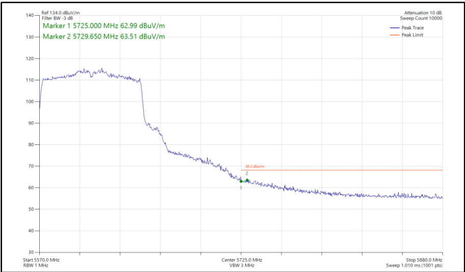
Figure 597 - 802.11ac VHT80, SISO, Core 0 - 5610 MHz Band Edge Frequency 5725 MHz
