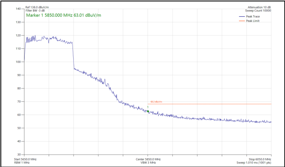
Figure 654 - 802.11ac VHT80, TxBF, Core 0 - Core 1 - 5690 MHz Band Edge Frequency 5850 MHz
