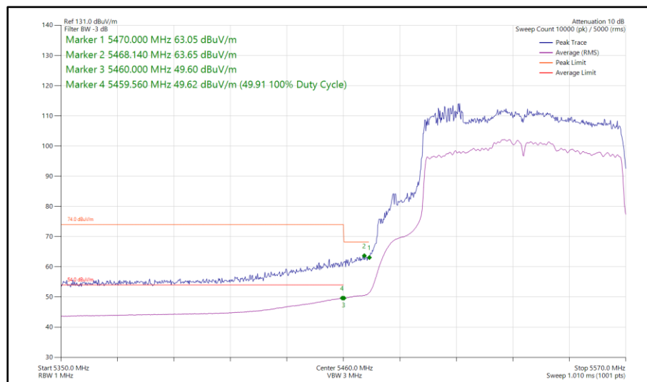
Figure 648 - 802.11ac VHT80, TxBF, Core 0 - Core 1 - 5530 MHz Band Edge Frequency 5470 MHz
