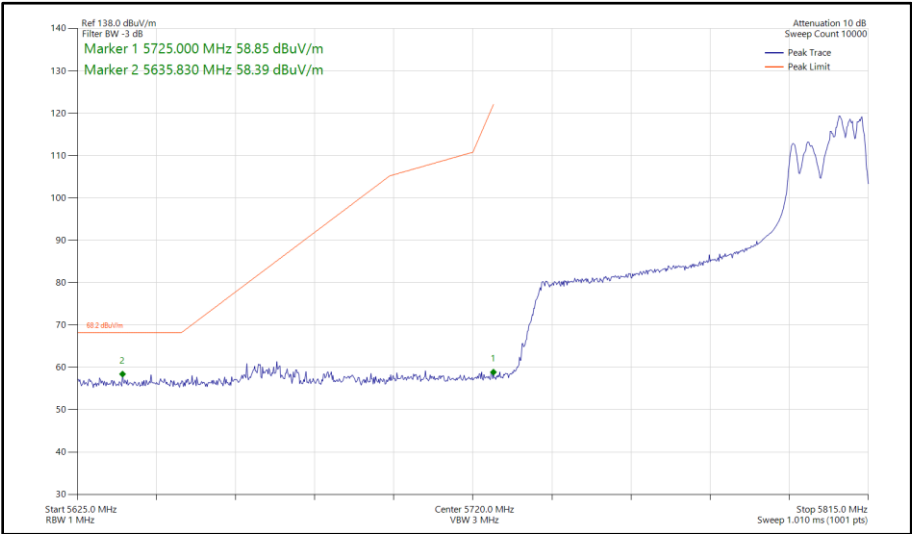
Figure 624 - 802.11ax HE80, RU 106-60, CDD, Core 0 - Core 1 - 5775 MHz Band Edge Frequency 5725 MHz
