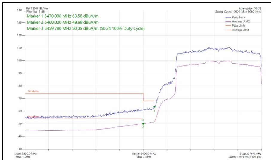
Figure 592 - 802.11ax HE80, SU, SISO, Core 0 - 5530 MHz Band Edge Frequency 5470 MHz
