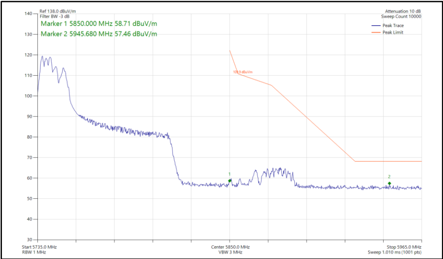
Figure 647 - 802.11ax HE80, RU 106-53, SDM, Core 0 - Core 1 - 5775 MHz Band Edge Frequency 5850 MHz
