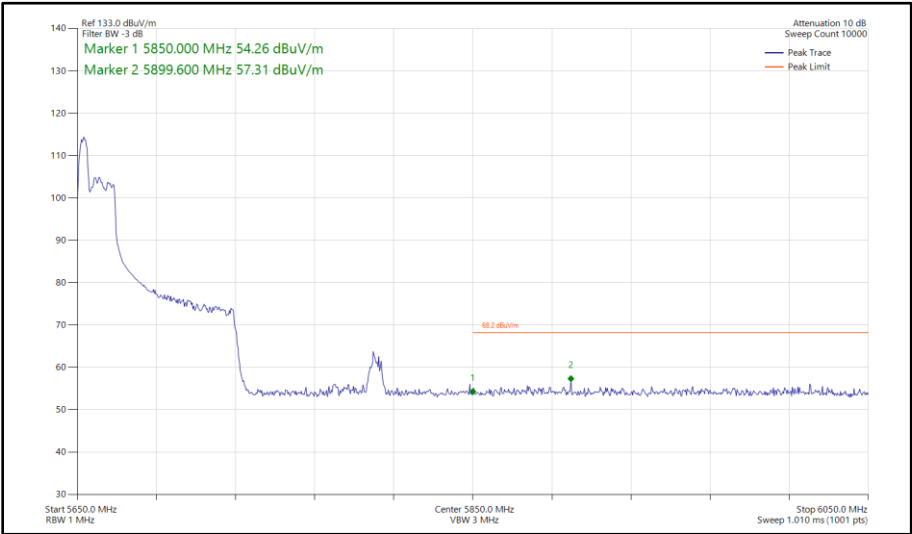
Figure 616 - 802.11ax HE80, RU 52-37, SISO, Core 1 - 5690 MHz Band Edge Frequency 5850 MHz
