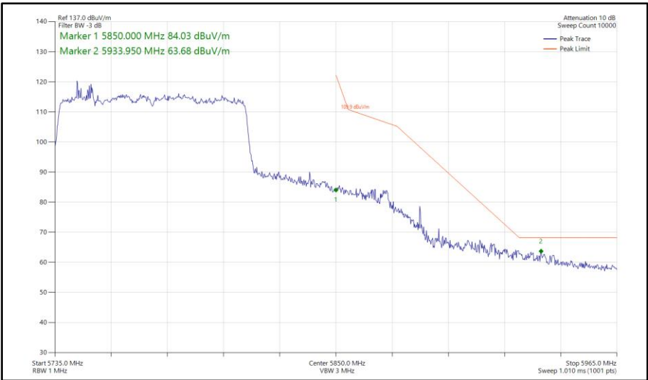
Figure 655 - 802.11ac VHT80, TxBF, Core 0 - Core 1 - 5775 MHz Band Edge Frequency 5850 MHz
