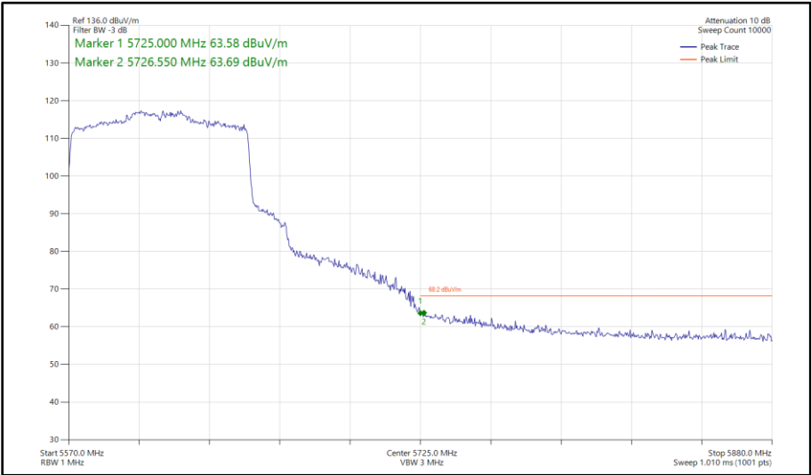
Figure 612 - 802.11ax HE80, SU, SISO, Core 1 - 5610 MHz Band Edge Frequency 5725 MHz
