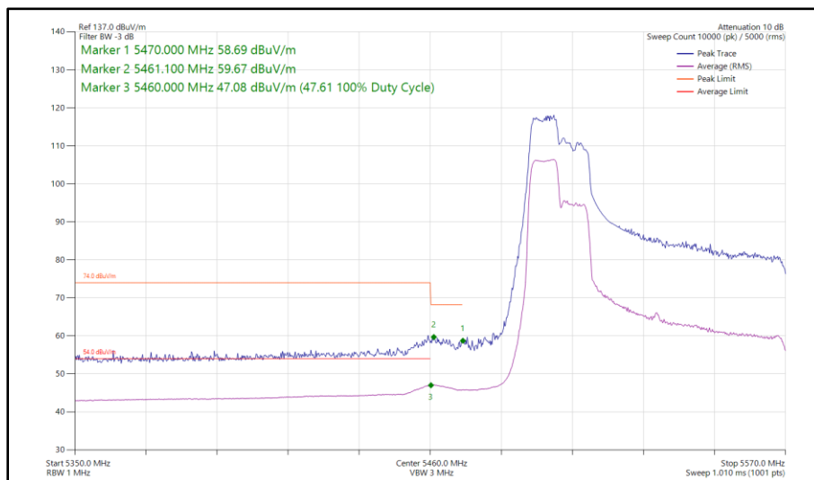
Figure 607 - 802.11ax HE80, RU 106-53, SISO, Core 1 - 5530 MHz Band Edge Frequency 5470 MHz
