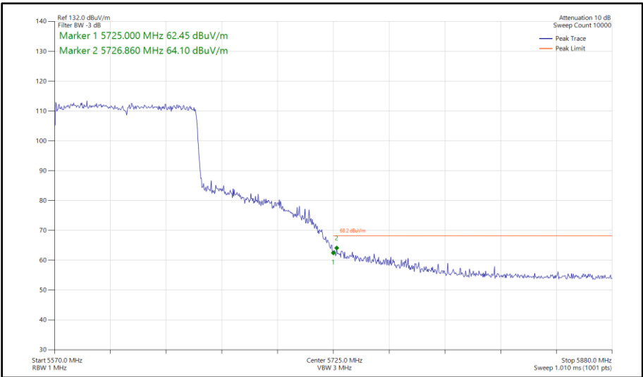
Figure 653 - 802.11ax HE80, SU, TxBF, Core 0 - Core 1 - 5610 MHz Band Edge Frequency 5725 MHz
