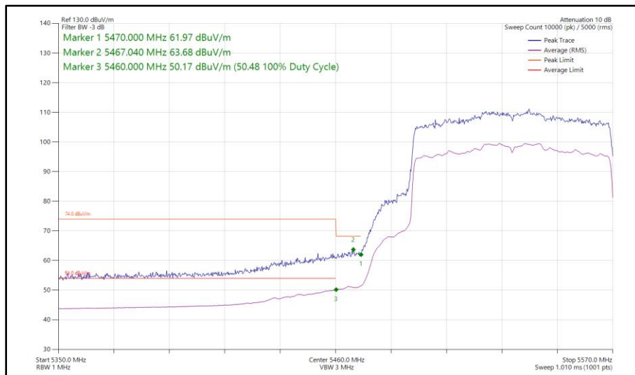
Figure 635 - 802.11ax HE80, SU, SDM, Core 0 - Core 1 - 5530 MHz Band Edge Frequency 5470 MHz
