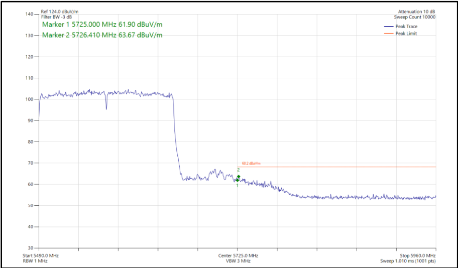
Figure 662 - 802.11ax HE160, SU, SISO, Core 0 - 5570 MHz Band Edge Frequency 5725 MHz
