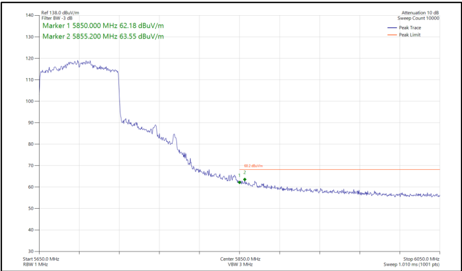
Figure 644 - 802.11ax HE80, SU, SDM, Core 0 - Core 1 - 5690 MHz Band Edge Frequency 5850 MHz
