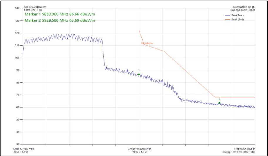
Figure 632 - 802.11ax HE80, SU, CDD, Core 0 - Core 1 - 5775 MHz Band Edge Frequency 5850 MHz
