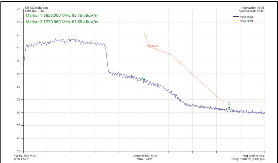
Figure 629 - 802.11ac VHT80, CDD, Core 0 - Core 1 - 5775 MHz Band Edge Frequency 5850 MHz
