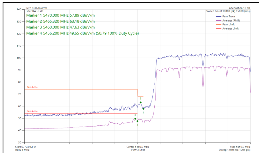
Figure 664 - 802.11ac VHT160, SISO, Core 1 - 5570 MHz Band Edge Frequency 5470 MHz
