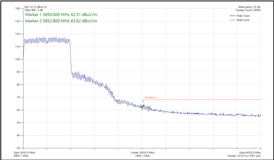
Figure 630 - 802.11ax HE80, SU, CDD, Core 0 - Core 1 - 5690 MHz Band Edge Frequency 5850 MHz
