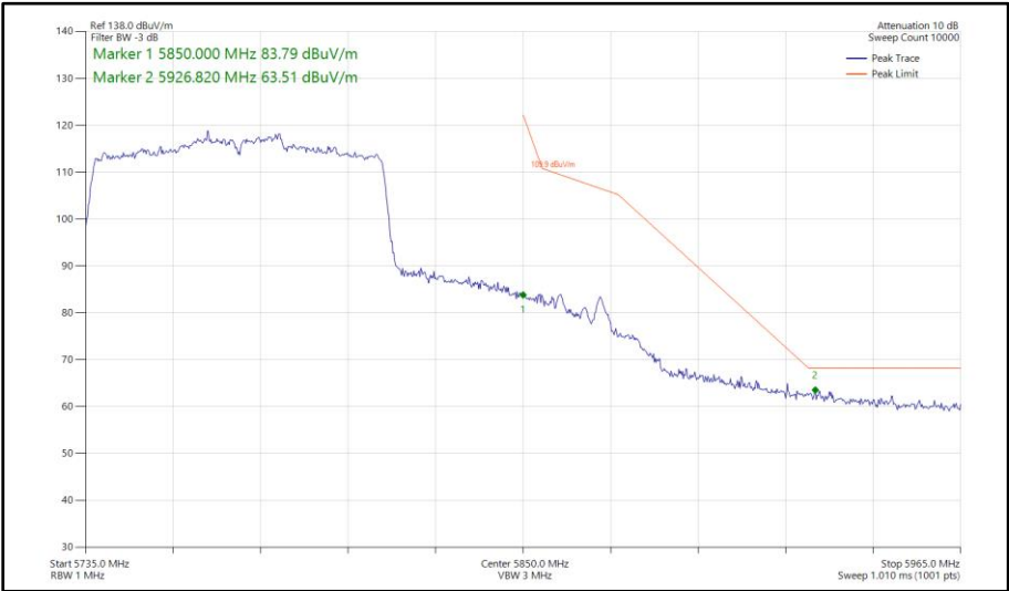
Figure 643 - 802.11ac VHT80, SDM, Core 0 - Core 1 - 5775 MHz Band Edge Frequency 5850 MHz
