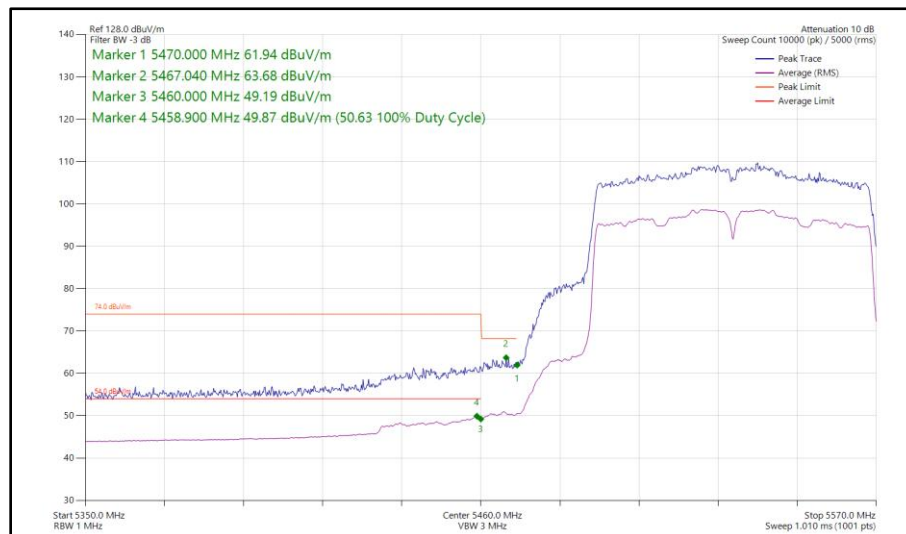
Figure 591 - 802.11ac VHT80, SISO, Core 0 - 5530 MHz Band Edge Frequency 5470 MHz
