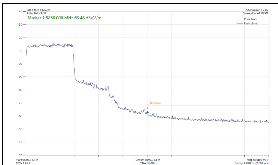
Figure 642 - 802.11ac VHT80, SDM, Core 0 - Core 1 - 5690 MHz Band Edge Frequency 5850 MHz
