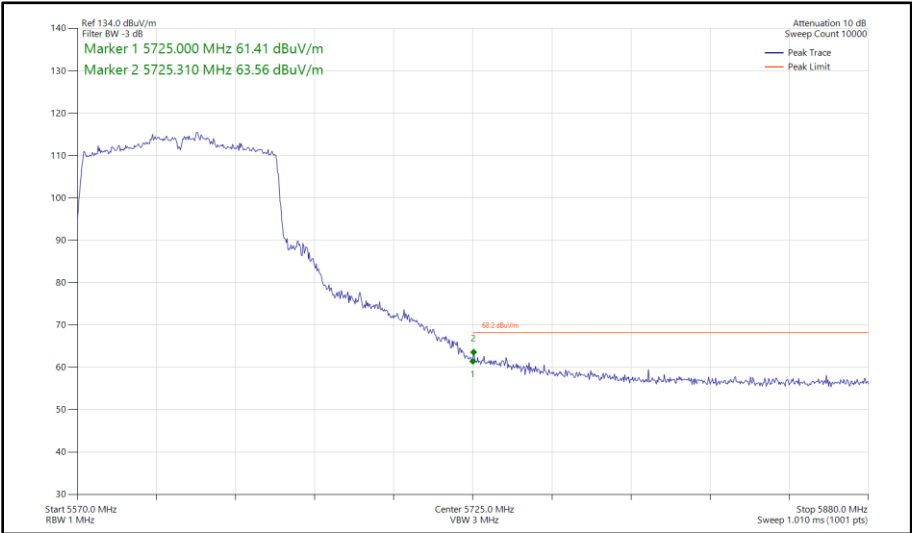
Figure 611 - 802.11ac VHT80, SISO, Core 1 - 5610 MHz Band Edge Frequency 5725 MHz
