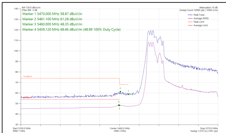
Figure 621 - 802.11ax HE80, RU 106-53, CDD, Core 0 - Core 1 - 5530 MHz Band Edge Frequency 5470 MHz
