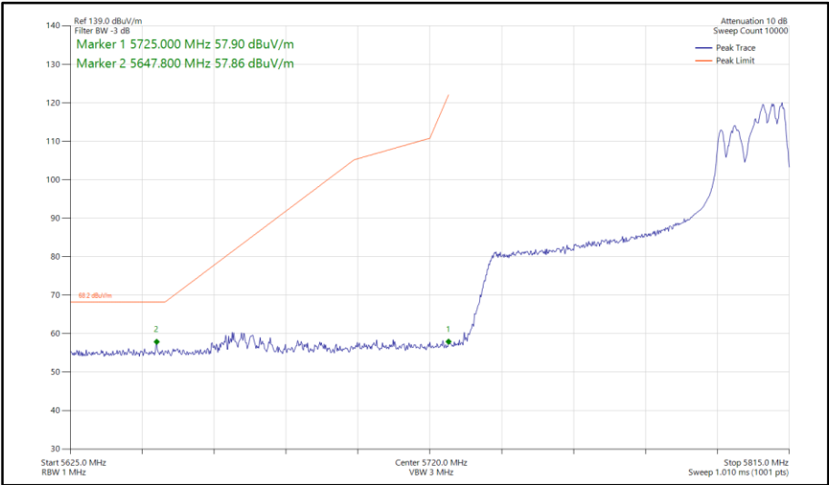
Figure 639 - 802.11ax HE80, RU 106-60, SDM, Core 0 - Core 1 - 5775 MHz Band Edge Frequency 5725 MHz
