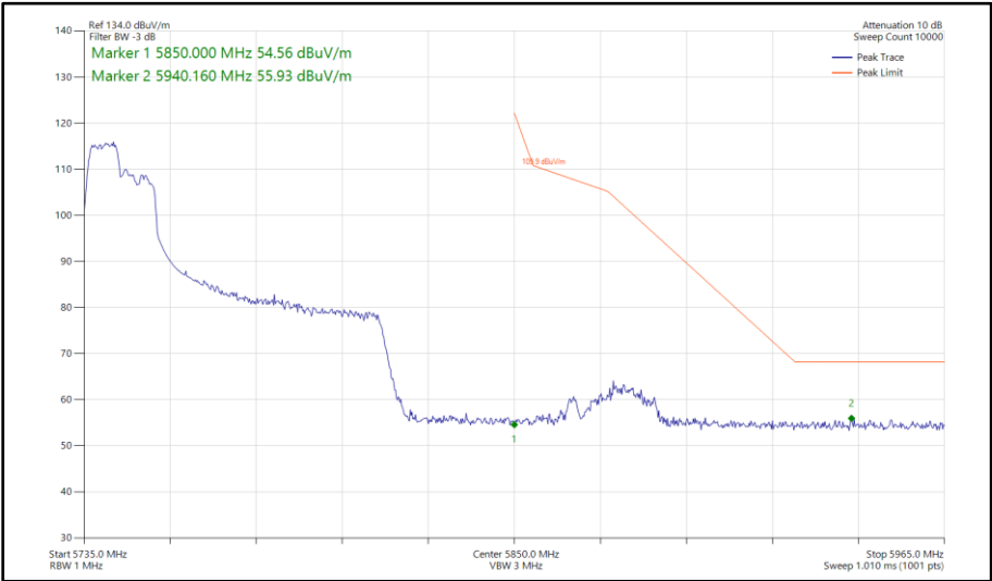
Figure 604 - 802.11ax HE80, RU 106-53, SISO, Core 0 - 5775 MHz Band Edge Frequency 5850 MHz
