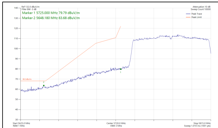
Figure 608 - 802.11ac VHT80, SISO, Core 1 - 5775 MHz Band Edge Frequency 5725 MHz
