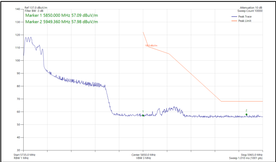
Figure 633 - 802.11ax HE80, RU 106-53, CDD, Core 0 - Core 1 - 5775 MHz Band Edge Frequency 5850 MHz
