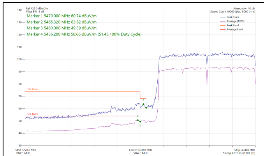
Figure 665 - 802.11ax HE160, SU, SISO, Core 1 - 5570 MHz Band Edge Frequency 5470 MHz
