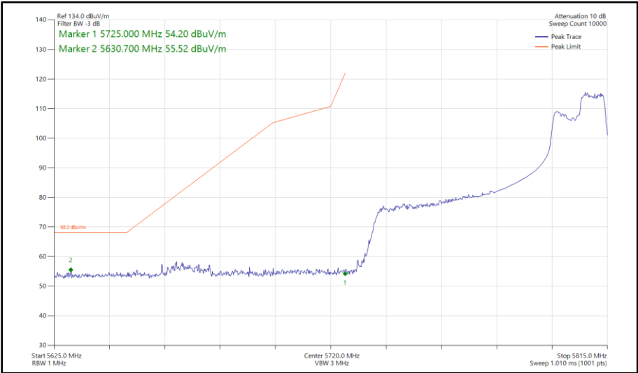
Figure 610 - 802.11ax HE80, RU 106-60, SISO, Core 1 - 5775 MHz Band Edge Frequency 5725 MHz
