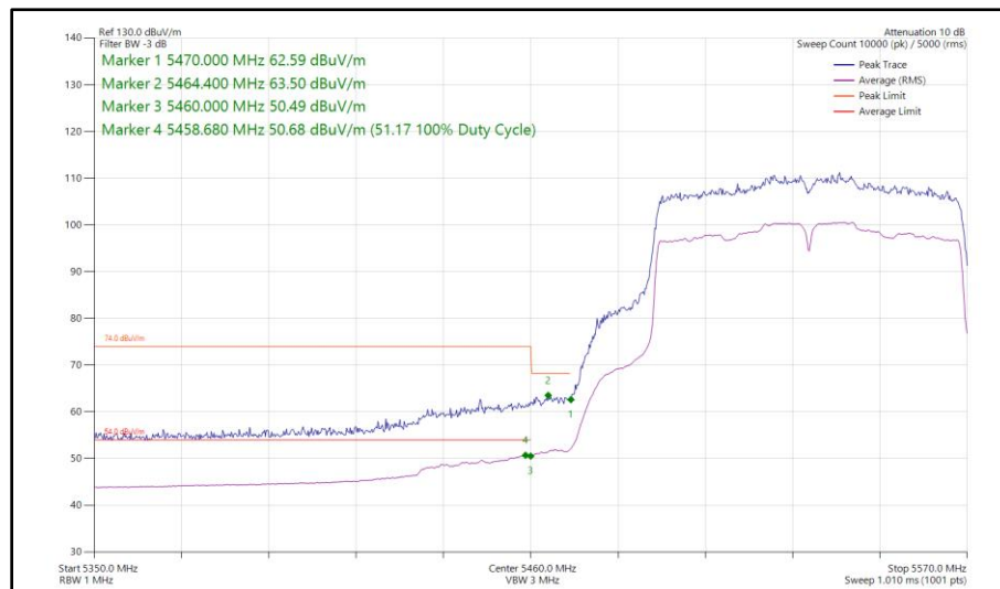
Figure 605 - 802.11ac VHT80, SISO, Core 1 - 5530 MHz Band Edge Frequency 5470 MHz
