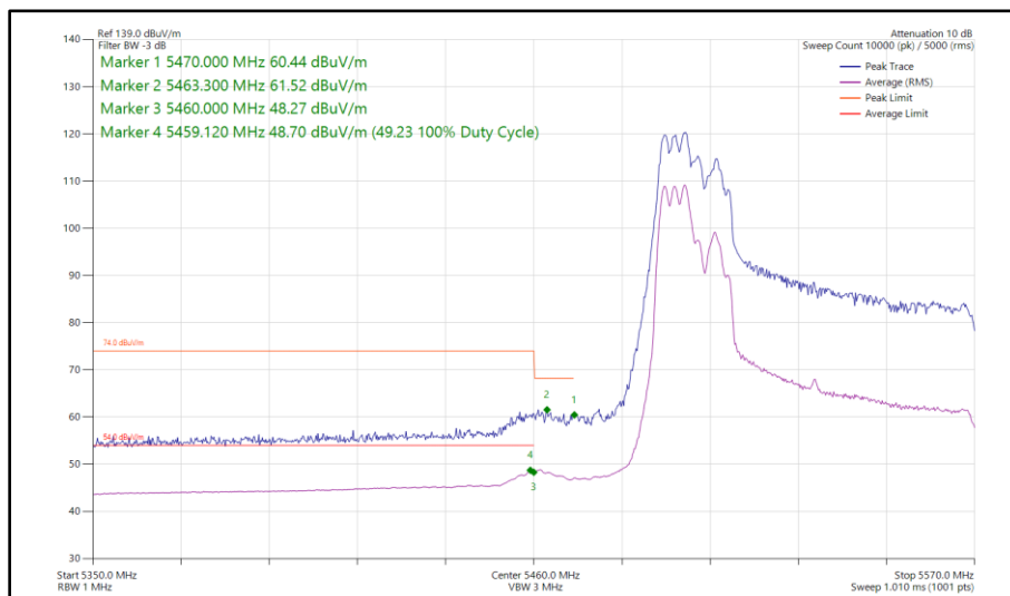
Figure 636 - 802.11ax HE80, RU 106-53, SDM, Core 0 - Core 1 - 5530 MHz Band Edge Frequency 5470 MHz
