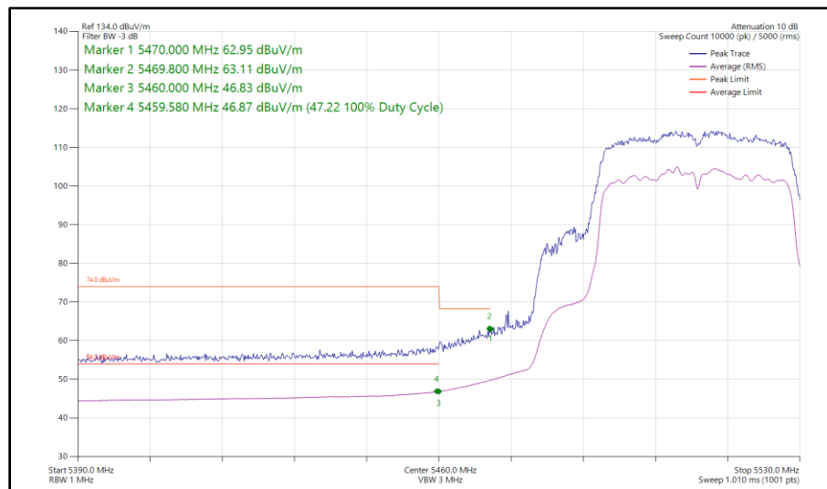
Figure 584 - 802.11ac VHT40, TxBF, Core 0 - Core 1 - 5510 MHz Band Edge Frequency 5470 MHz
