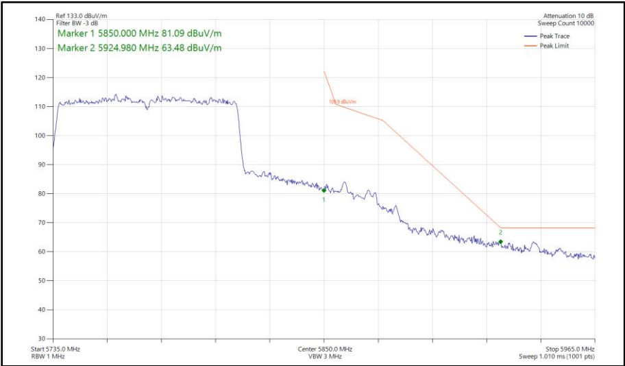
Figure 614 - 802.11ac VHT80, SISO, Core 1 - 5775 MHz Band Edge Frequency 5850 MHz
