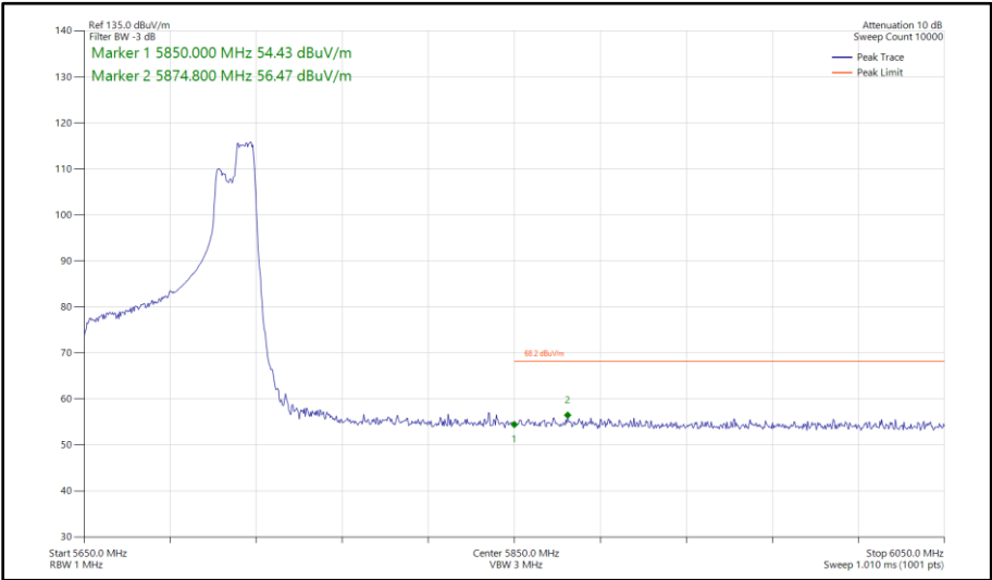
Figure 602 - 802.11ax HE80, RU 106-60, SISO, Core 0 - 5690 MHz Band Edge Frequency 5850 MHz
