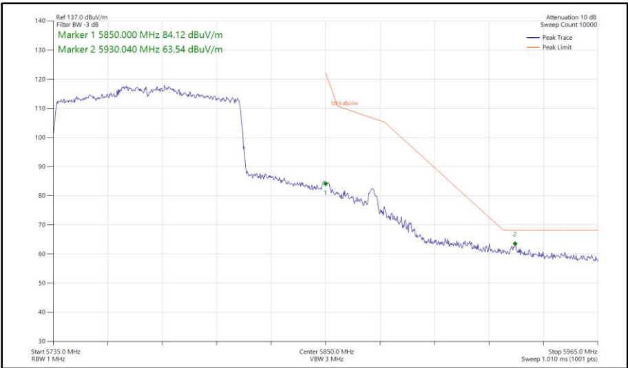
Figure 646 - 802.11ax HE80, SU, SDM, Core 0 - Core 1 - 5775 MHz Band Edge Frequency 5850 MHz
