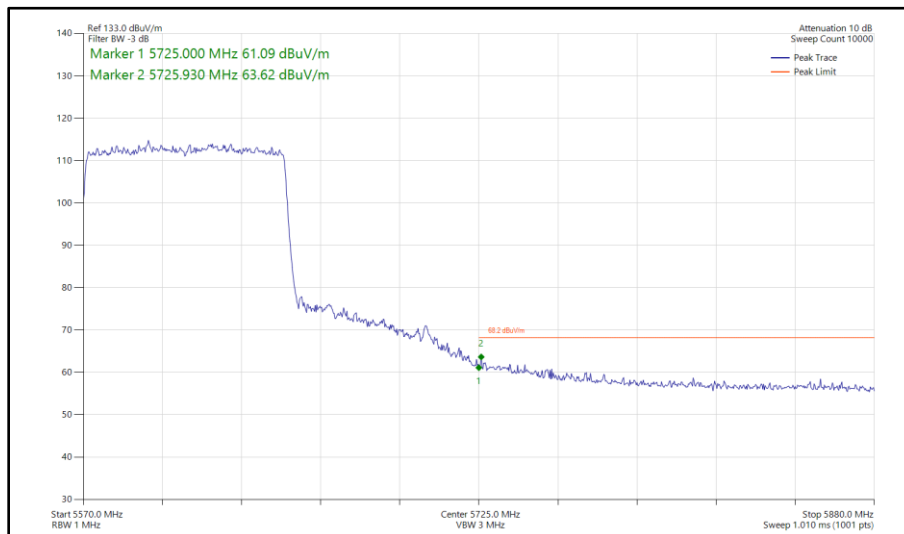
Figure 641 - 802.11ax HE80, SU, SDM, Core 0 - Core 1 - 5610 MHz Band Edge Frequency 5725 MHz
