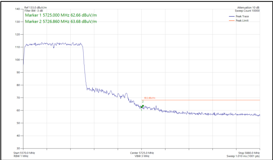
Figure 640 - 802.11ac VHT80, SDM, Core 0 - Core 1 - 5610 MHz Band Edge Frequency 5725 MHz
