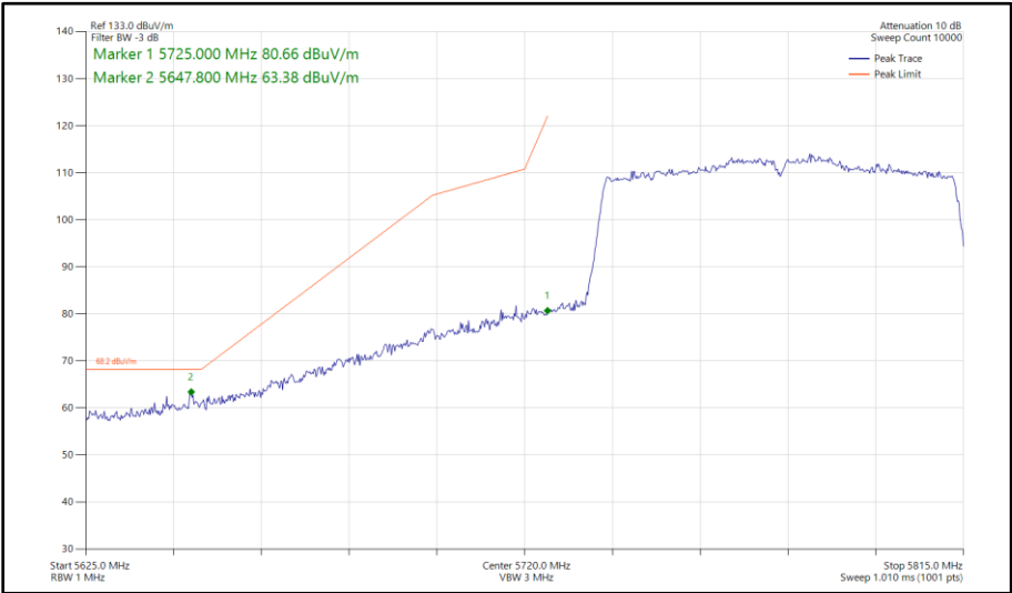
Figure 594 - 802.11ac VHT80, SISO, Core 0 - 5775 MHz Band Edge Frequency 5725 MHz
