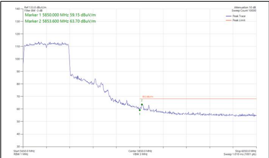
Figure 599 - 802.11ac VHT80, SISO, Core 0 - 5690 MHz Band Edge Frequency 5850 MHz
