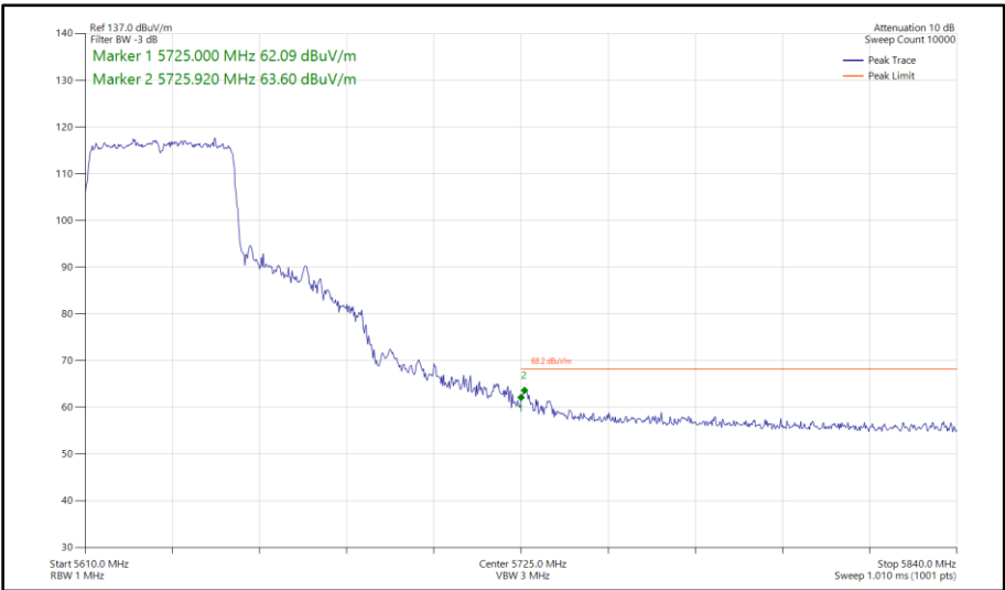
Figure 518 - 802.11ax HE40, SU, SISO, Core 0 - 5630 MHz Band Edge Frequency 5725 MHz
