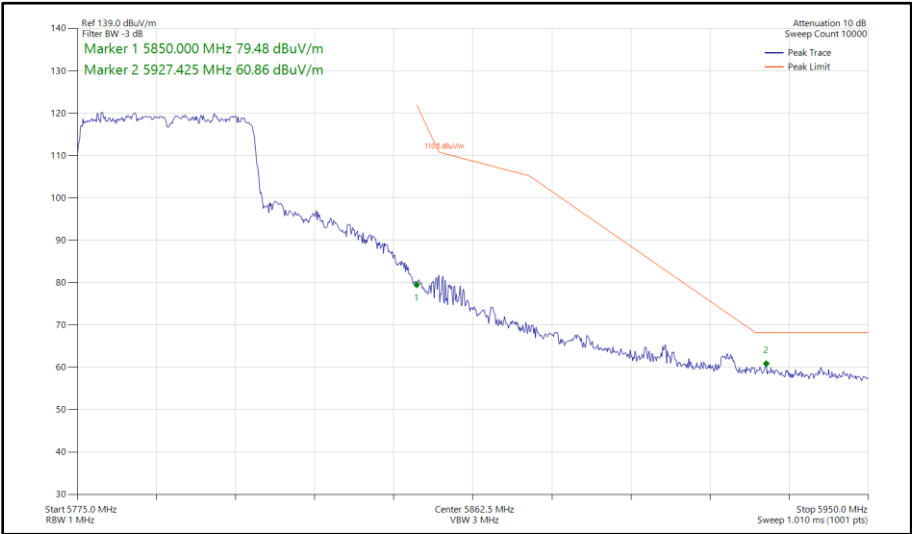
Figure 582 - 802.11ax HE40, SU, SDM, Core 0 - Core 1 - 5795 MHz Band Edge Frequency 5850 MHz
