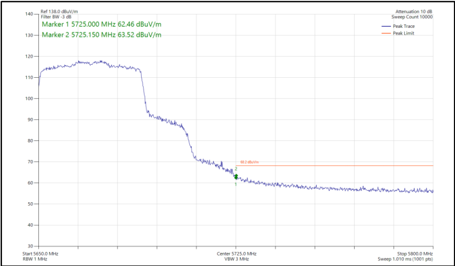
Figure 538 - 802.11ax HE40, SU, SISO, Core 1 - 5670 MHz Band Edge Frequency 5725 MHz
