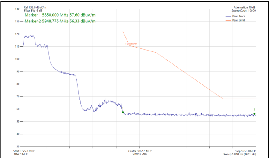
Figure 545 - 802.11ax HE40, RU 106-53, SISO, Core 1 - 5795 MHz Band Edge Frequency 5850 MHz
