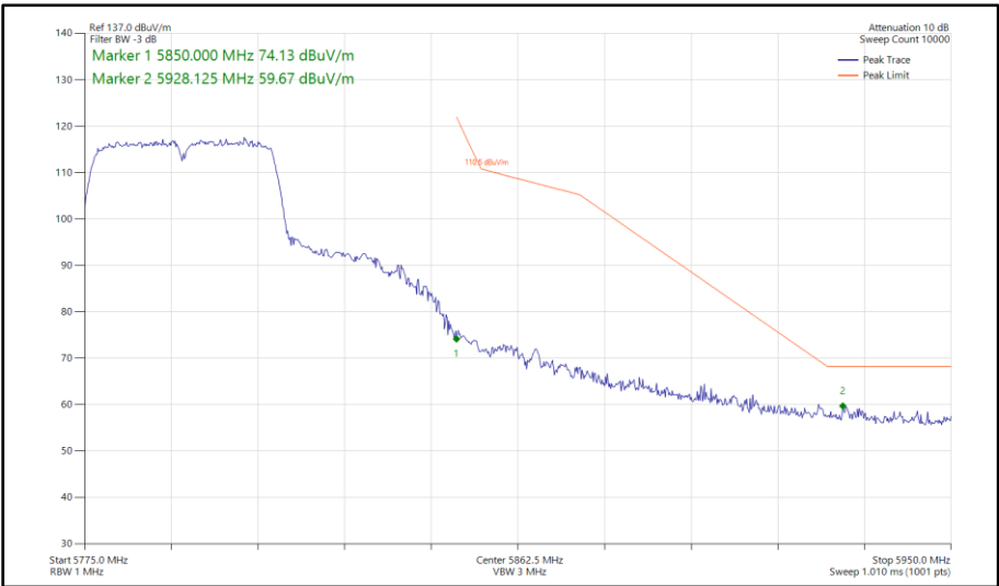
Figure 522 - 802.11n HT40, SISO, Core 0 - 5795 MHz Band Edge Frequency 5850 MHz
