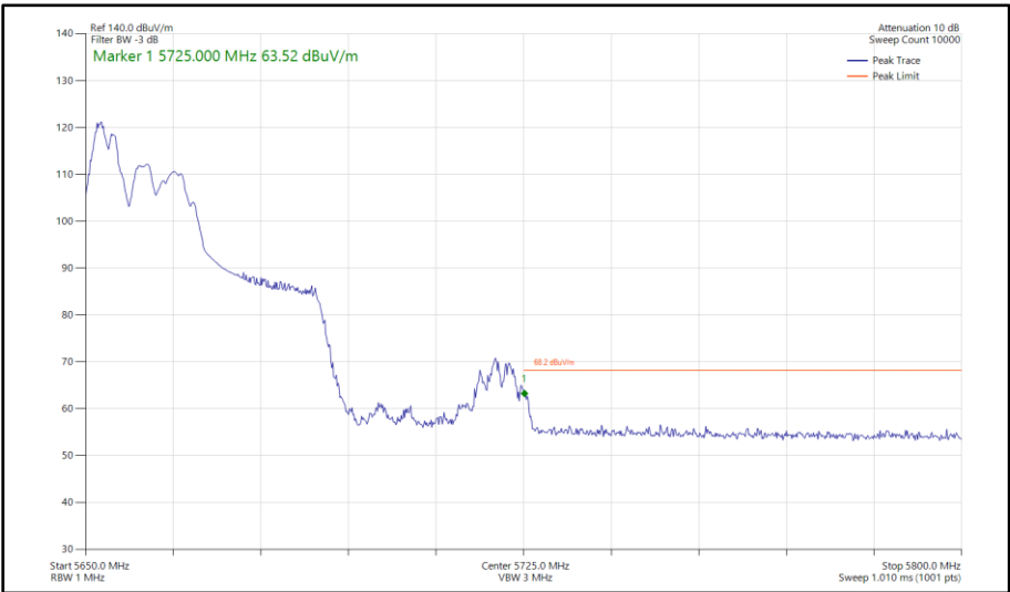
Figure 578 - 802.11ax HE40, RU 52-37, SDM, Core 0 - Core 1 - 5670 MHz Band Edge Frequency 5725 MHz
