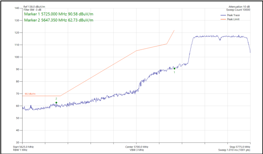
Figure 513 - 802.11n HT40, SISO, Core 0 - 5755 MHz Band Edge Frequency 5725 MHz
