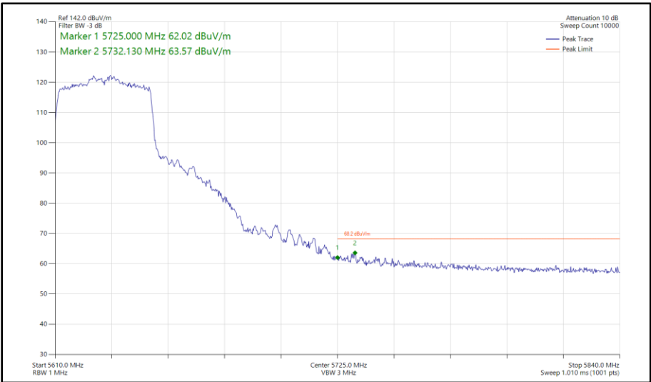
Figure 576 - 802.11ax HE40, SU, SDM, Core 0 - Core 1 - 5630 MHz Band Edge Frequency 5725 MHz
