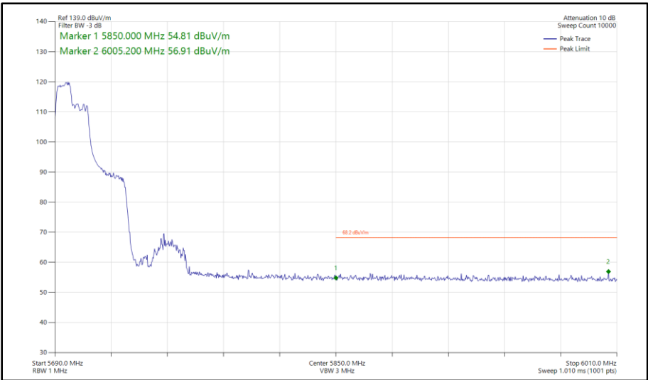
Figure 543 - 802.11ax HE40, RU 106-53, SISO, Core 1 - 5710 MHz Band Edge Frequency 5850 MHz
