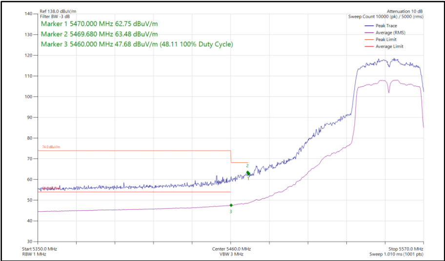
Figure 509 - 802.11n HT40, SISO, Core 0 - 5550 MHz Band Edge Frequency 5470 MHz
