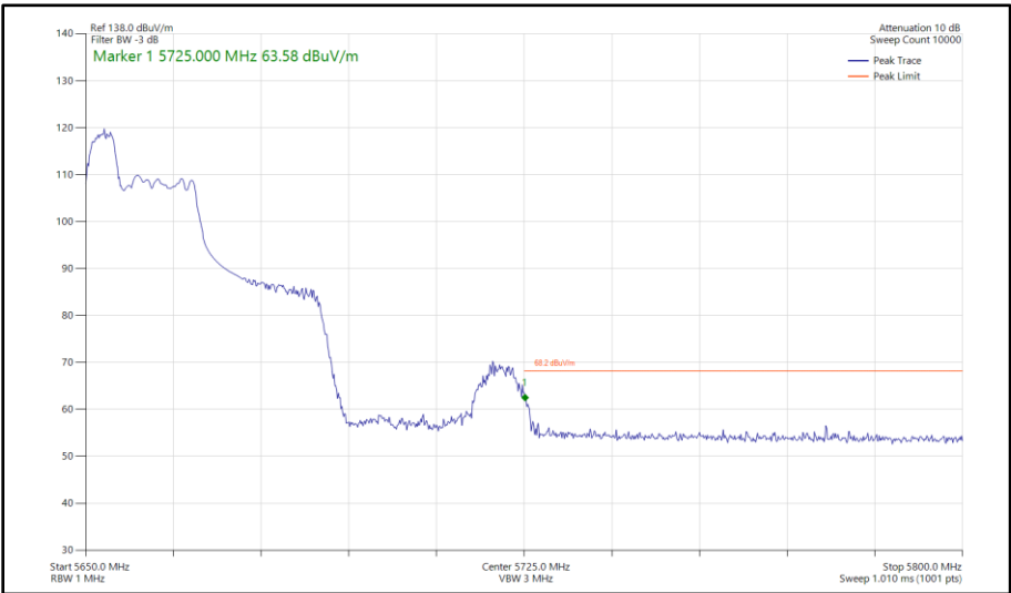
Figure 539 - 802.11ax HE40, RU 52-37, SISO, Core 1 - 5670 MHz Band Edge Frequency 5725 MHz
