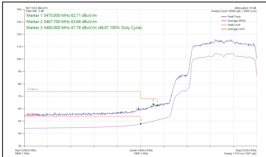
Figure 568 - 802.11ax HE40, SU, SDM, Core 0 - Core 1 - 5510 MHz Band Edge Frequency 5470 MHz
