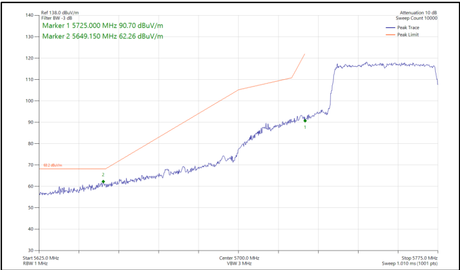
Figure 514 - 802.11ax HE40, SU, SISO, Core 0 - 5755 MHz Band Edge Frequency 5725 MHz
