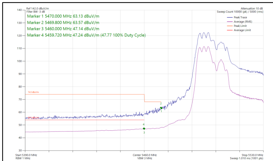
Figure 569 - 802.11ax HE40, RU 106-53, SDM, Core 0 - Core 1 - 5510 MHz Band Edge Frequency 5470 MHz
