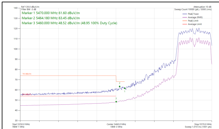
Figure 547 - 802.11n HT40, CDD, Core 0 - Core 1 - 5550 MHz Band Edge Frequency 5470 MHz
