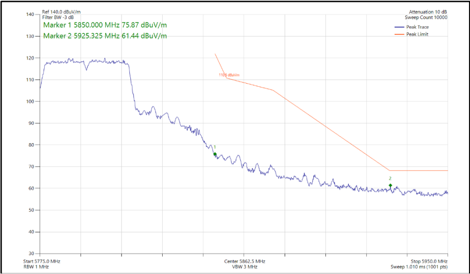
Figure 579 - 802.11n HT40, SDM, Core 0 - Core 1 - 5795 MHz Band Edge Frequency 5850 MHz
