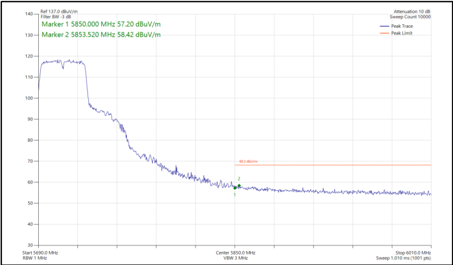
Figure 521 - 802.11n HT40, SISO, Core 0 - 5710 MHz Band Edge Frequency 5850 MHz
