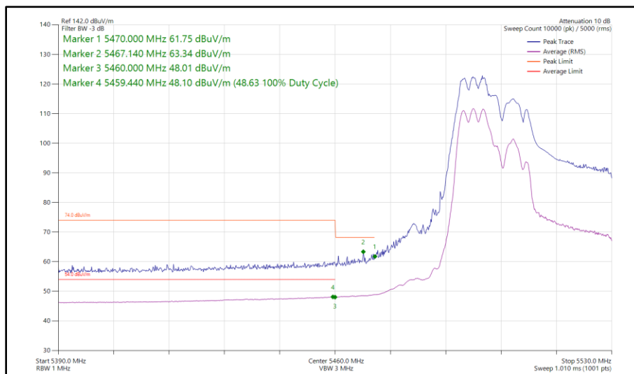
Figure 550 - 802.11ax HE40, RU 106-53, CDD, Core 0 - Core 1 - 5510 MHz Band Edge Frequency 5470 MHz
