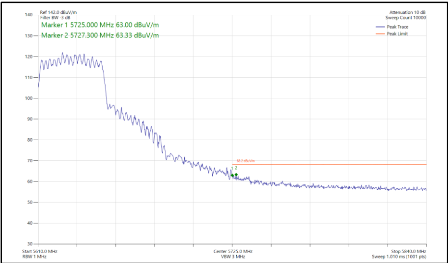
Figure 558 - 802.11ax HE40, SU, CDD, Core 0 - Core 1 - 5630 MHz Band Edge Frequency 5725 MHz
