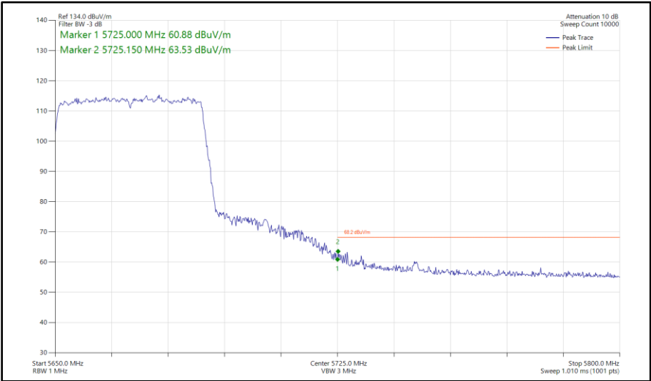
Figure 577 - 802.11ax HE40, SU, SDM, Core 0 - Core 1 - 5670 MHz Band Edge Frequency 5725 MHz
