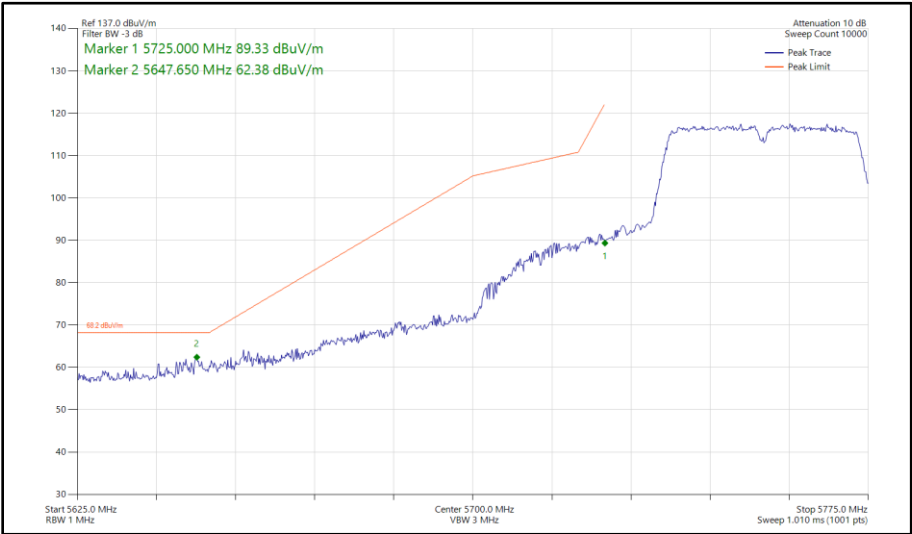
Figure 532 - 802.11n HT40, SISO, Core 1 - 5755 MHz Band Edge Frequency 5725 MHz
