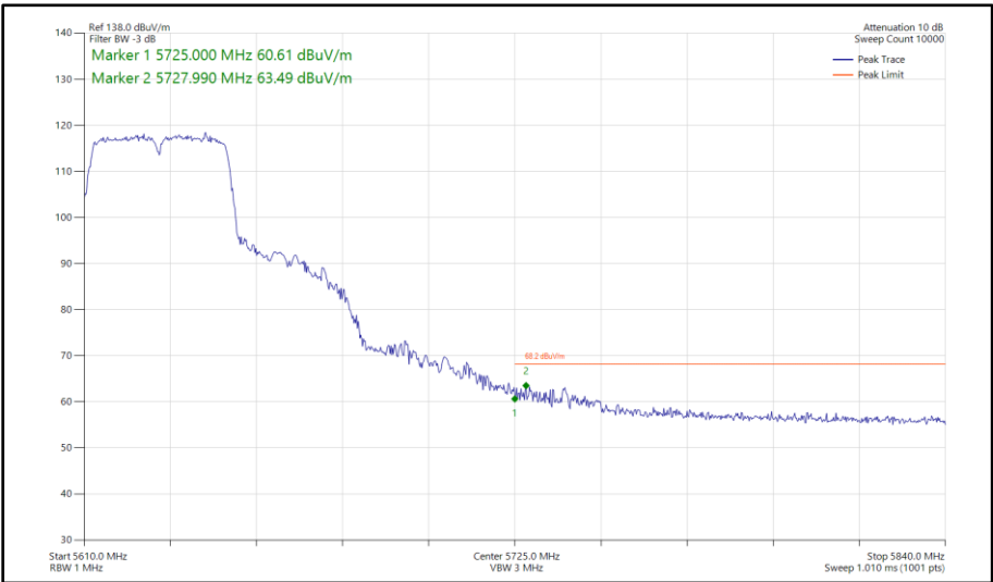
Figure 535 - 802.11n HT40, SISO, Core 1 - 5630 MHz Band Edge Frequency 5725 MHz
