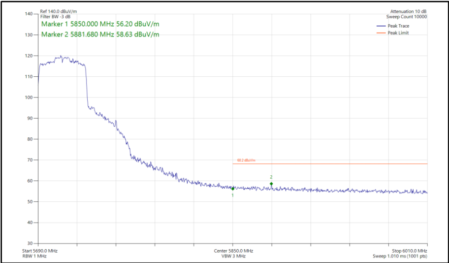
Figure 542 - 802.11ax HE40, SU, SISO, Core 1 - 5710 MHz Band Edge Frequency 5850 MHz
