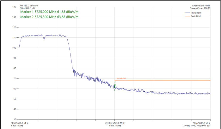
Figure 536 - 802.11n HT40, SISO, Core 1 - 5670 MHz Band Edge Frequency 5725 MHz
