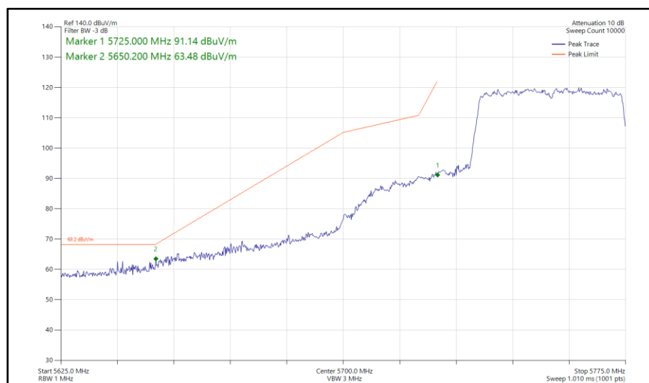
Figure 573 - 802.11ax HE40, SU, SDM, Core 0 - Core 1 - 5755 MHz Band Edge Frequency 5725 MHz
