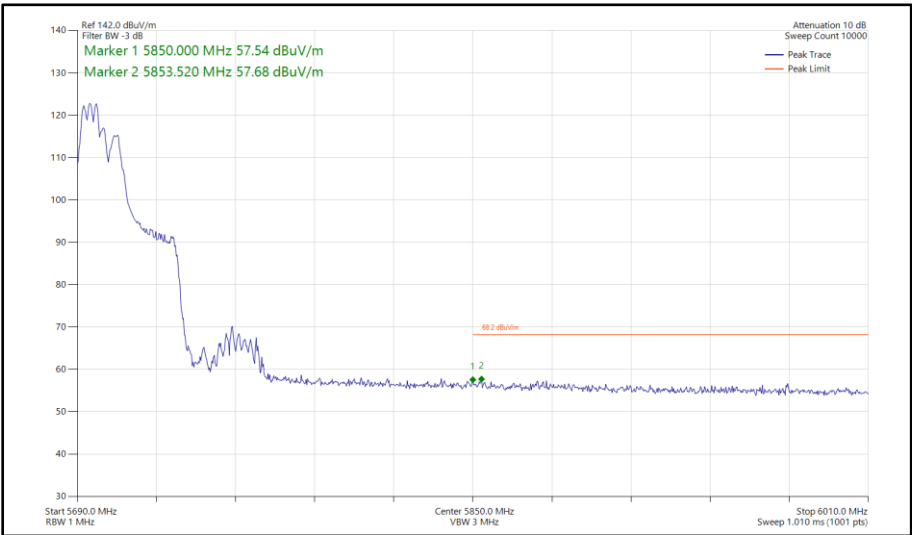
Figure 564 - 802.11ax HE40, RU 106-53, CDD, Core 0 - Core 1 - 5710 MHz Band Edge Frequency 5850 MHz
