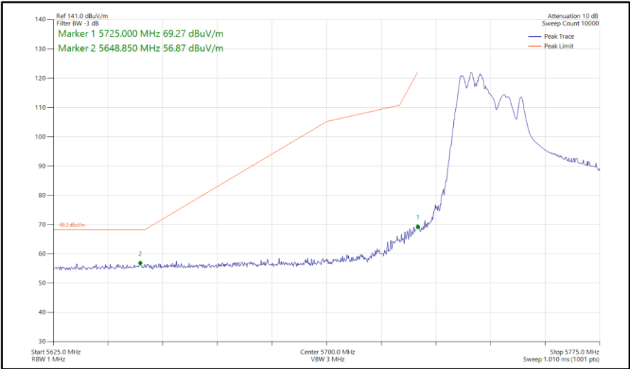
Figure 574 - 802.11ax HE40, RU 106-53, SDM, Core 0 - Core 1 - 5755 MHz Band Edge Frequency 5725 MHz
