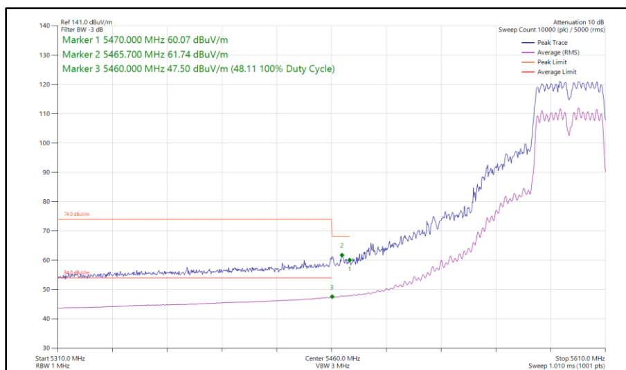
Figure 548 - 802.11n HT40, CDD, Core 0 - Core 1 - 5590 MHz Band Edge Frequency 5470 MHz
