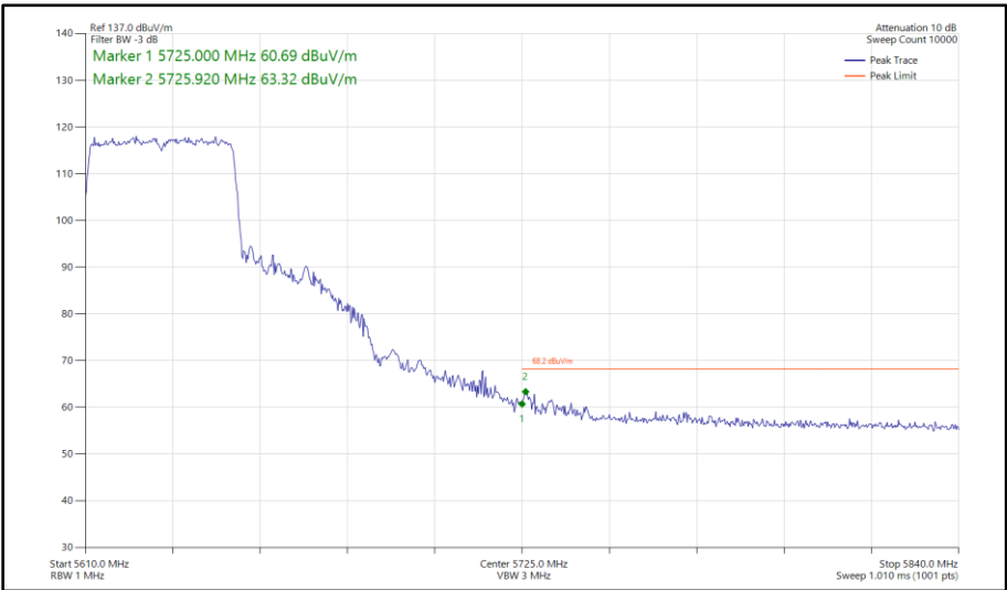
Figure 537 - 802.11ax HE40, SU, SISO, Core 1 - 5630 MHz Band Edge Frequency 5725 MHz
