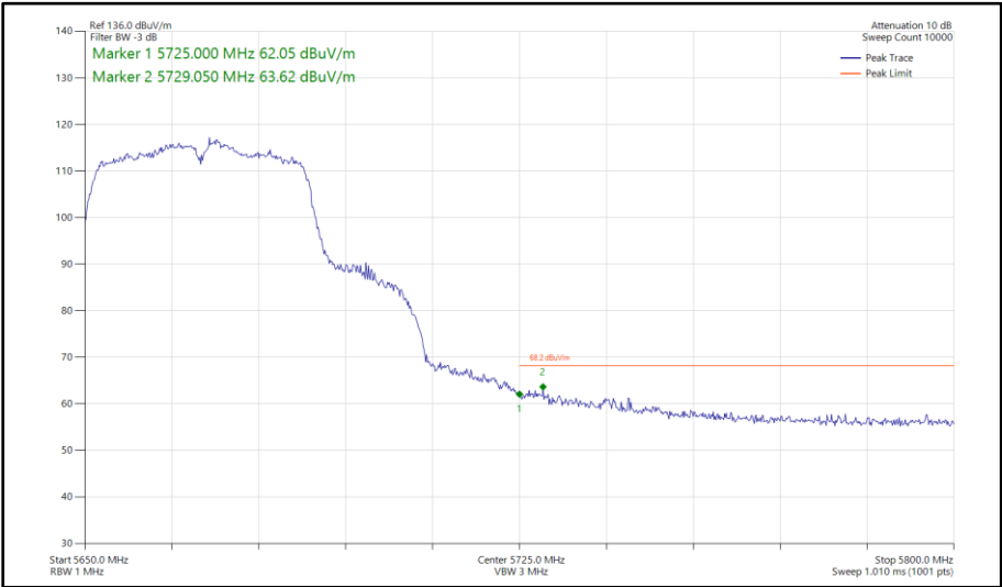
Figure 517 - 802.11n HT40, SISO, Core 0 - 5670 MHz Band Edge Frequency 5725 MHz
