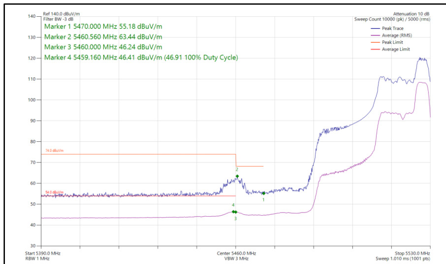
Figure 511 - 802.11ax HE40, RU 52-44, SISO, Core 0 - 5510 MHz Band Edge Frequency 5470 MHz
