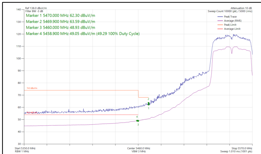
Figure 528 - 802.11n HT40, SISO, Core 1 - 5550 MHz Band Edge Frequency 5470 MHz
