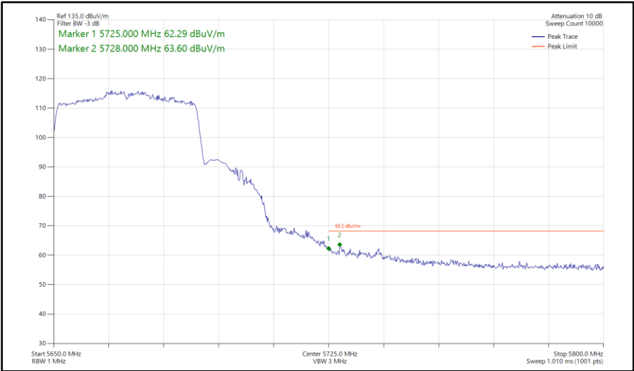
Figure 519 - 802.11ax HE40, SU, SISO, Core 0 - 5670 MHz Band Edge Frequency 5725 MHz
