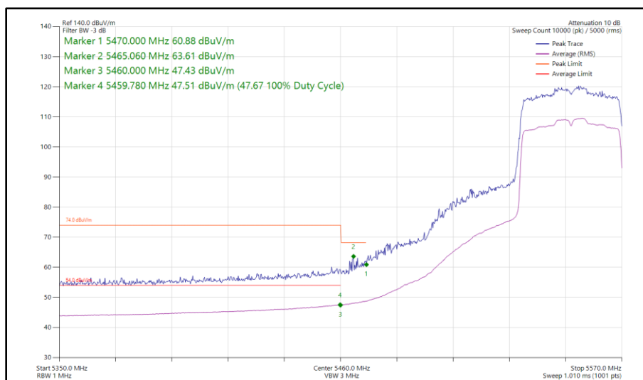
Figure 531 - 802.11ax HE40, SU, SISO, Core 1 - 5550 MHz Band Edge Frequency 5470 MHz
