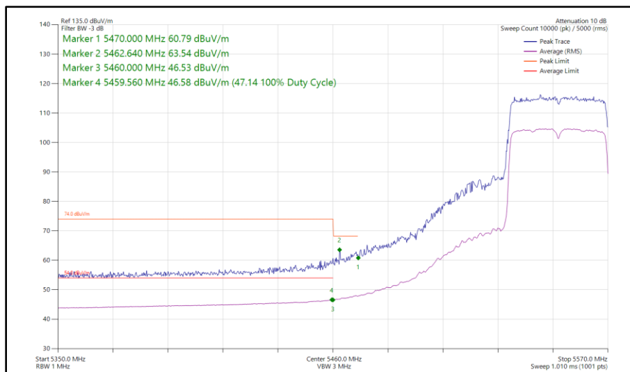
Figure 512 - 802.11ax HE40, SU, SISO, Core 0 - 5550 MHz Band Edge Frequency 5470 MHz
