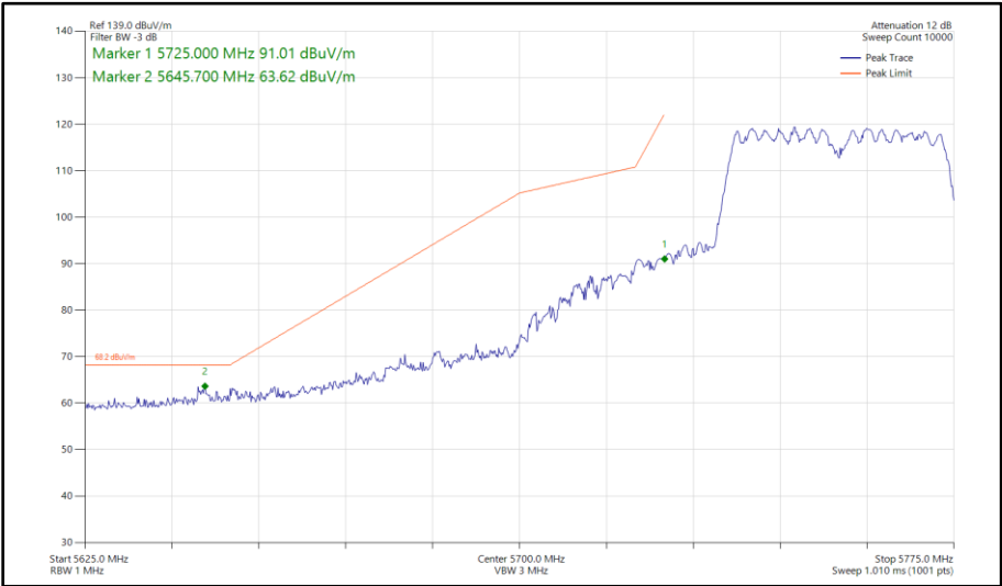
Figure 553 - 802.11n HT40, CDD, Core 0 - Core 1 - 5755 MHz Band Edge Frequency 5725 MHz
