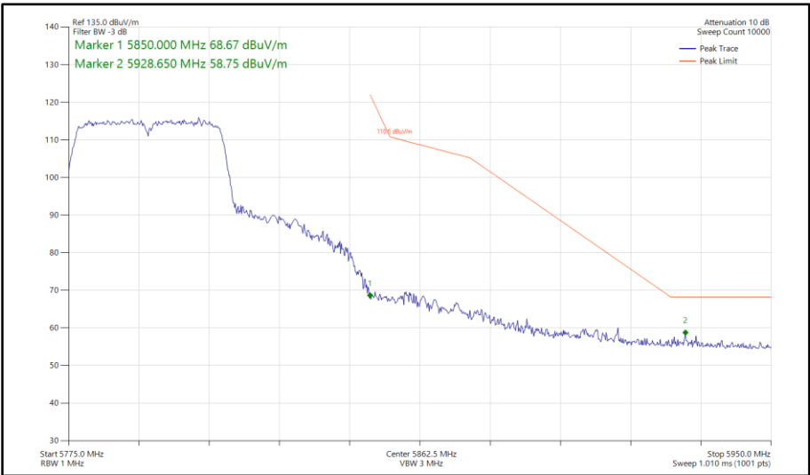
Figure 541 - 802.11n HT40, SISO, Core 1 - 5795 MHz Band Edge Frequency 5850 MHz
