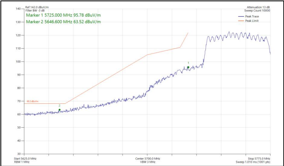
Figure 554 - 802.11ax HE40, SU, CDD, Core 0 - Core 1 - 5755 MHz Band Edge Frequency 5725 MHz
