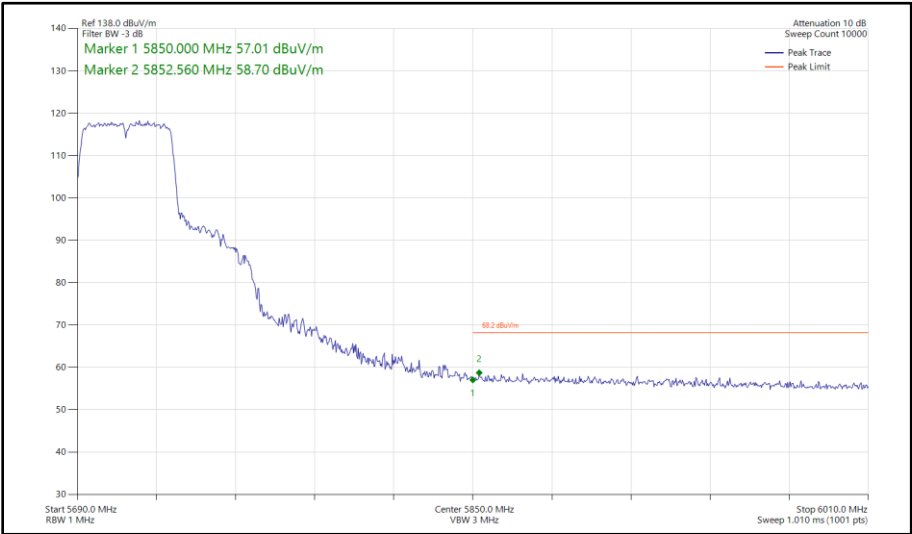
Figure 540 - 802.11n HT40, SISO, Core 1 - 5710 MHz Band Edge Frequency 5850 MHz
