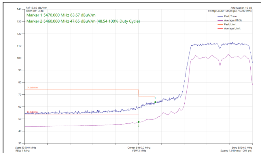
Figure 567 - 802.11n HT40, SDM, Core 0 - Core 1 - 5510 MHz Band Edge Frequency 5470 MHz
