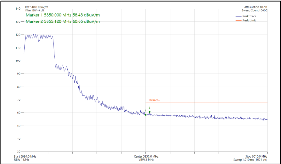
Figure 561 - 802.11n HT40, CDD, Core 0 - Core 1 - 5710 MHz Band Edge Frequency 5850 MHz
