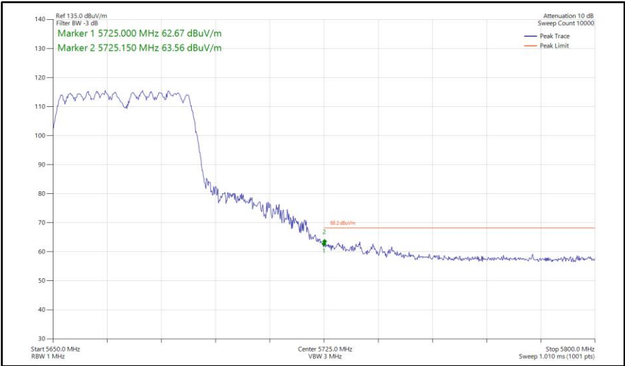
Figure 557 - 802.11n HT40, CDD, Core 0 - Core 1 - 5670 MHz Band Edge Frequency 5725 MHz
