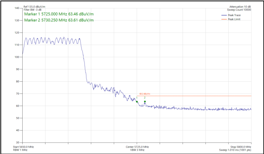
Figure 559 - 802.11ax HE40, SU, CDD, Core 0 - Core 1 - 5670 MHz Band Edge Frequency 5725 MHz
