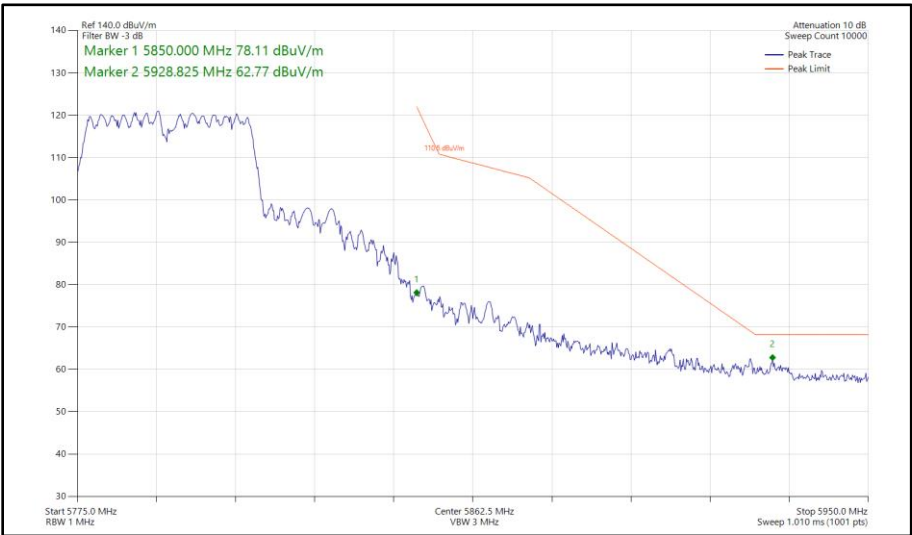
Figure 562 - 802.11n HT40, CDD, Core 0 - Core 1 - 5795 MHz Band Edge Frequency 5850 MHz
