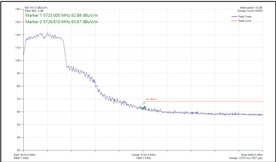
Figure 556 - 802.11n HT40, CDD, Core 0 - Core 1 - 5630 MHz Band Edge Frequency 5725 MHz
