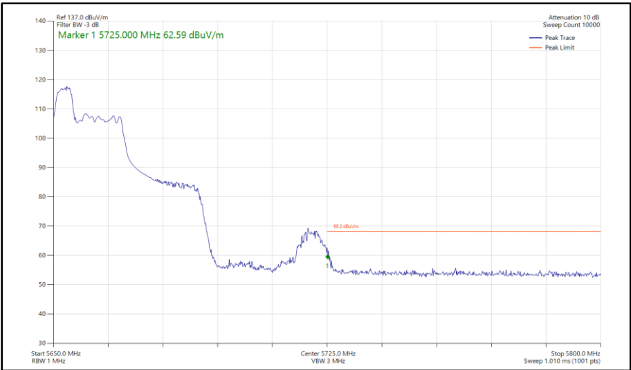
Figure 520 - 802.11ax HE40, RU 52-37, SISO, Core 0 - 5670 MHz Band Edge Frequency 5725 MHz
