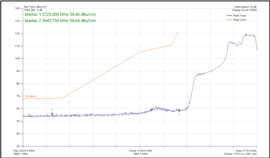
Figure 515 - 802.11ax HE40, RU 106-56, SISO, Core 0 - 5755 MHz Band Edge Frequency 5725 MHz
