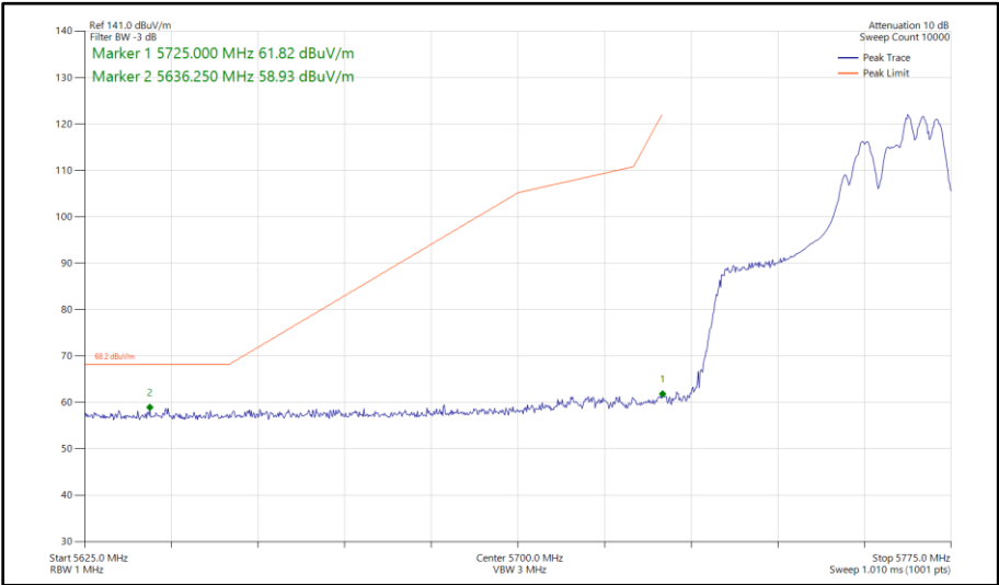
Figure 555 - 802.11ax HE40, RU 106-56, CDD, Core 0 - Core 1 - 5755 MHz Band Edge Frequency 5725 MHz
