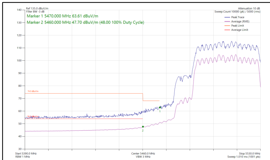
Figure 549 - 802.11ax HE40, SU, CDD, Core 0 - Core 1 - 5510 MHz Band Edge Frequency 5470 MHz
