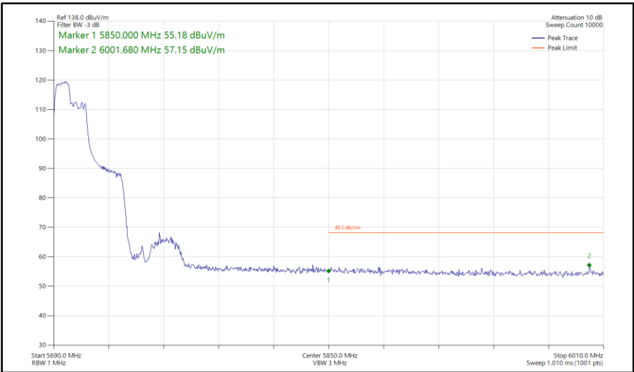
Figure 524 - 802.11ax HE40, RU 106-53, SISO, Core 0 - 5710 MHz Band Edge Frequency 5850 MHz
