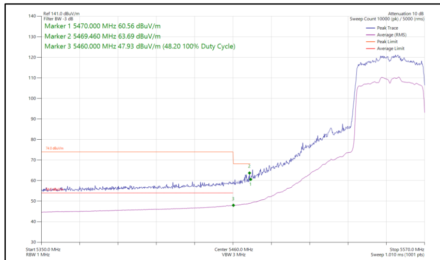
Figure 570 - 802.11ax HE40, SU, SDM, Core 0 - Core 1 - 5550 MHz Band Edge Frequency 5470 MHz
