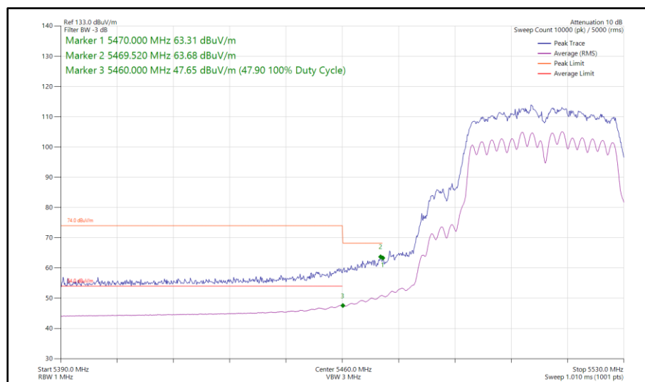
Figure 546 - 802.11n HT40, CDD, Core 0 - Core 1 - 5510 MHz Band Edge Frequency 5470 MHz
