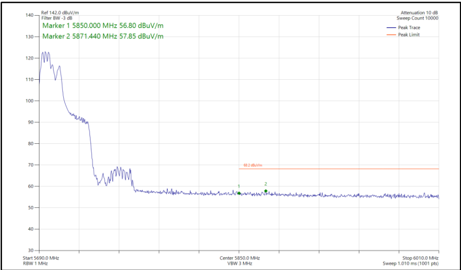
Figure 581 - 802.11ax HE40, RU 106-53, SDM, Core 0 - Core 1 - 5710 MHz Band Edge Frequency 5850 MHz
