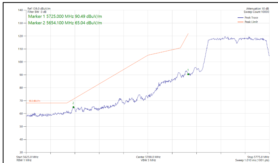
Figure 572 - 802.11n HT40, SDM, Core 0 - Core 1 - 5755 MHz Band Edge Frequency 5725 MHz
