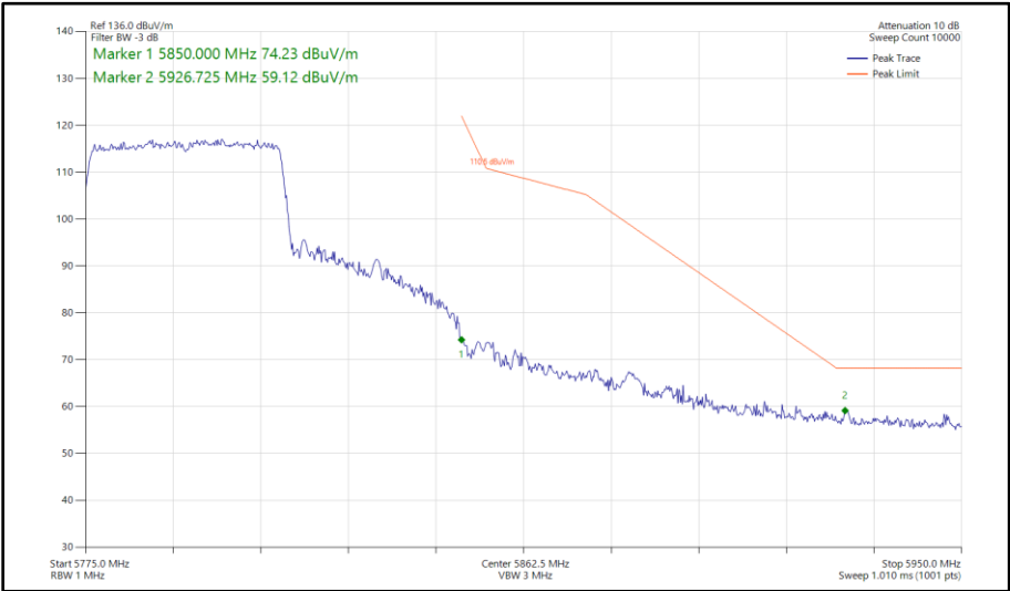
Figure 544 - 802.11ax HE40, SU, SISO, Core 1 - 5795 MHz Band Edge Frequency 5850 MHz
