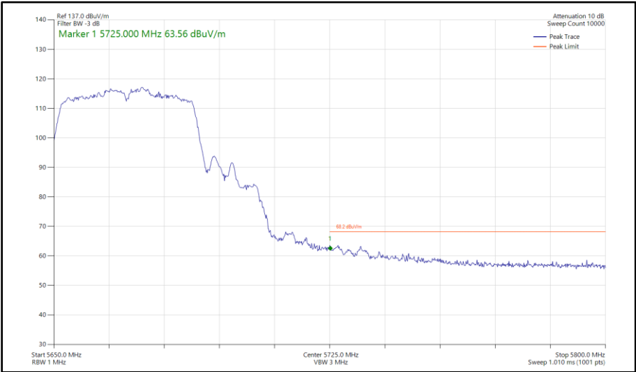
Figure 575 - 802.11n HT40, SDM, Core 0 - Core 1 - 5670 MHz Band Edge Frequency 5725 MHz
