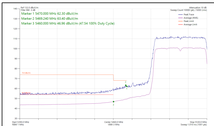
Figure 529 - 802.11ax HE40, SU, SISO, Core 1 - 5510 MHz Band Edge Frequency 5470 MHz
