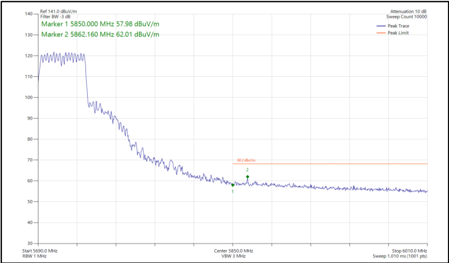
Figure 563 - 802.11ax HE40, SU, CDD, Core 0 - Core 1 - 5710 MHz Band Edge Frequency 5850 MHz
