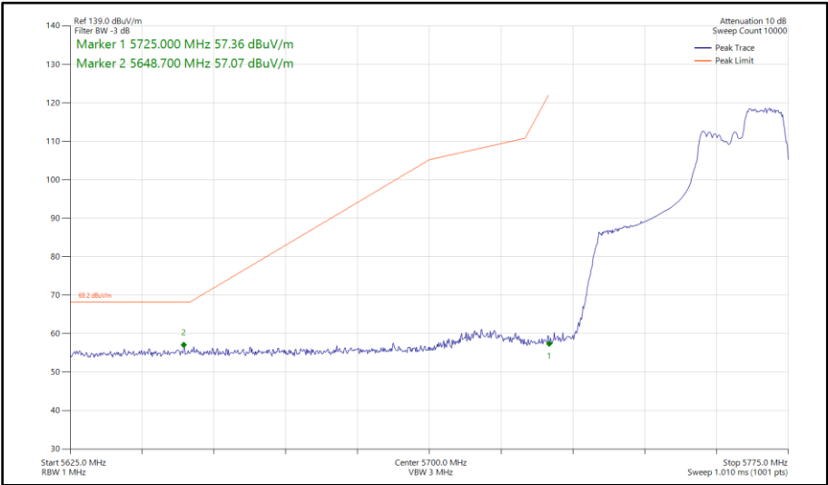
Figure 534 - 802.11ax HE40, RU 106-56, SISO, Core 1 - 5755 MHz Band Edge Frequency 5725 MHz
