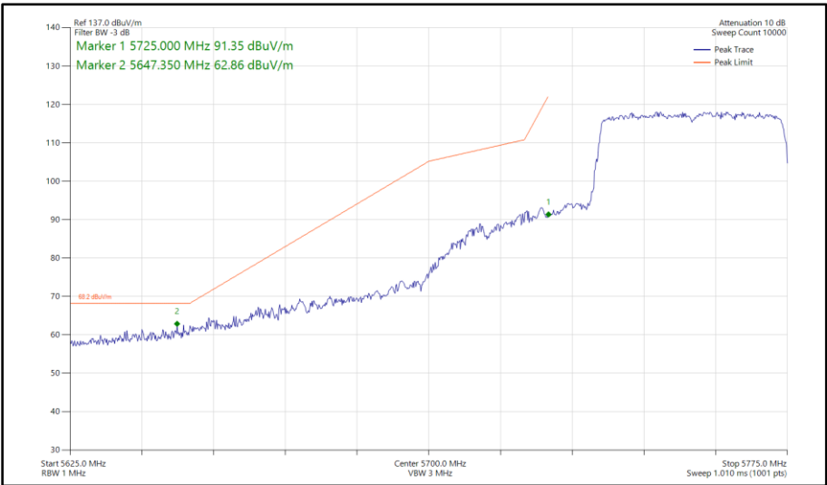
Figure 533 - 802.11ax HE40, SU, SISO, Core 1 - 5755 MHz Band Edge Frequency 5725 MHz
