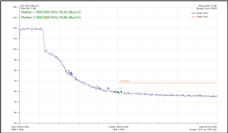
Figure 580 - 802.11ax HE40, SU, SDM, Core 0 - Core 1 - 5710 MHz Band Edge Frequency 5850 MHz
