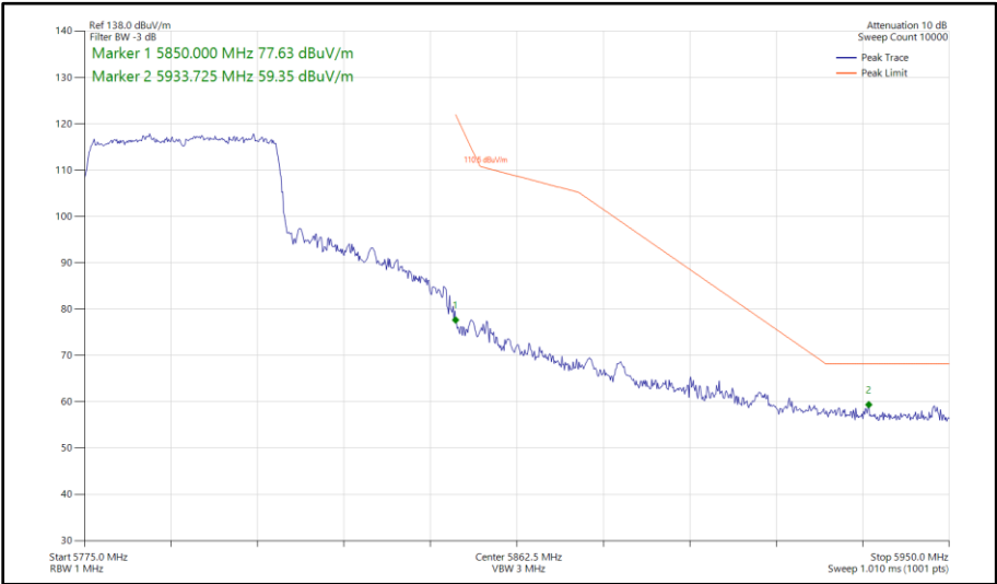
Figure 525 - 802.11ax HE40, SU, SISO, Core 0 - 5795 MHz Band Edge Frequency 5850 MHz
