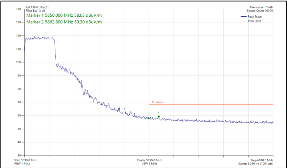
Figure 523 - 802.11ax HE40, SU, SISO, Core 0 - 5710 MHz Band Edge Frequency 5850 MHz
