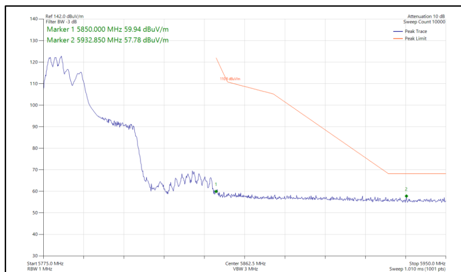
Figure 566 - 802.11ax HE40, RU 106-53, CDD, Core 0 - Core 1 - 5795 MHz Band Edge Frequency 5850 MHz
