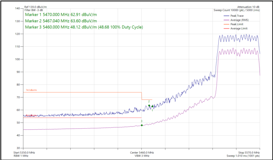
Figure 551 - 802.11ax HE40, SU, CDD, Core 0 - Core 1 - 5550 MHz Band Edge Frequency 5470 MHz
