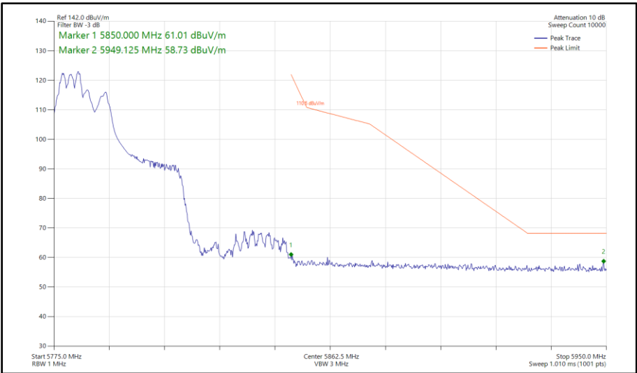
Figure 583 - 802.11ax HE40, RU 106-53, SDM, Core 0 - Core 1 - 5795 MHz Band Edge Frequency 5850 MHz
