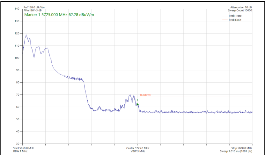
Figure 560 - 802.11ax HE40, RU 52-37, CDD, Core 0 - Core 1 - 5670 MHz Band Edge Frequency 5725 MHz
