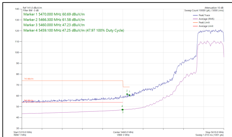
Figure 571 - 802.11ax HE40, SU, SDM, Core 0 - Core 1 - 5590 MHz Band Edge Frequency 5470 MHz
