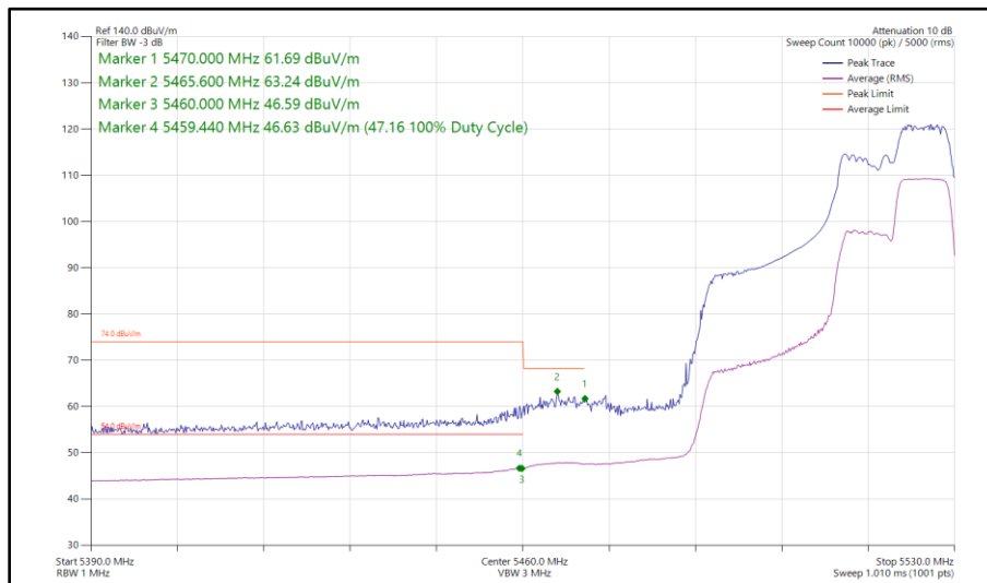
Figure 530 - 802.11ax HE40, RU 106-56, SISO, Core 1 - 5510 MHz Band Edge Frequency 5470 MHz
