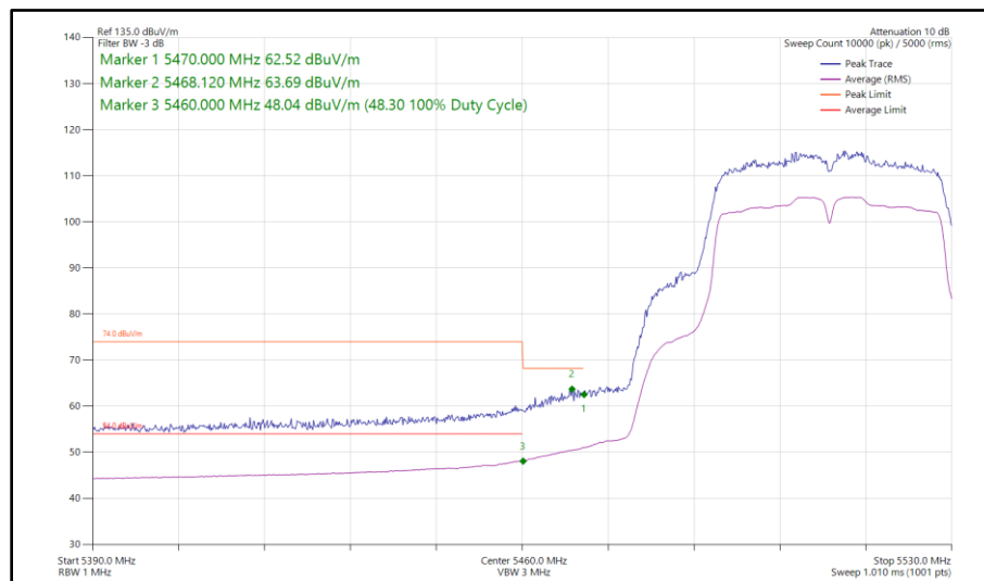
Figure 527 - 802.11n HT40, SISO, Core 1 - 5510 MHz Band Edge Frequency 5470 MHz
