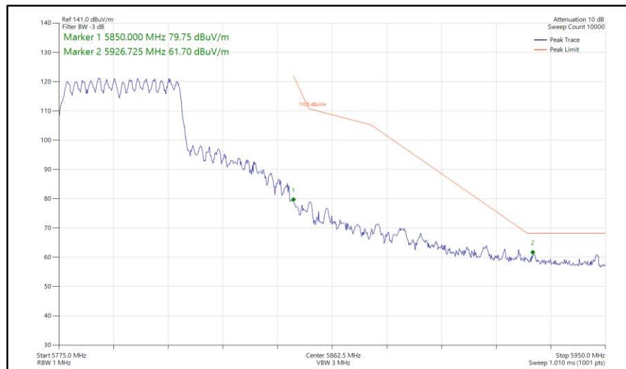
Figure 565 - 802.11ax HE40, SU, CDD, Core 0 - Core 1 - 5795 MHz Band Edge Frequency 5850 MHz
