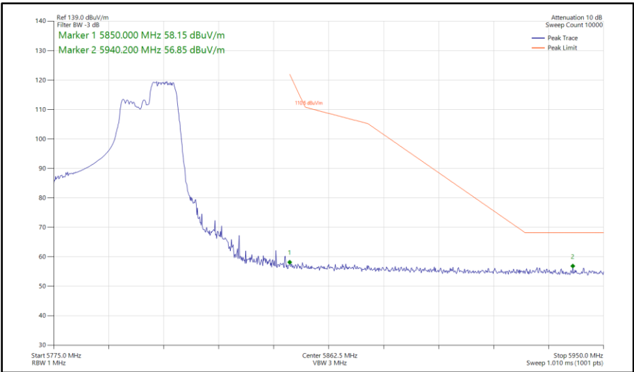
Figure 526 - 802.11ax HE40, RU 106-56, SISO, Core 0 - 5795 MHz Band Edge Frequency 5850 MHz
