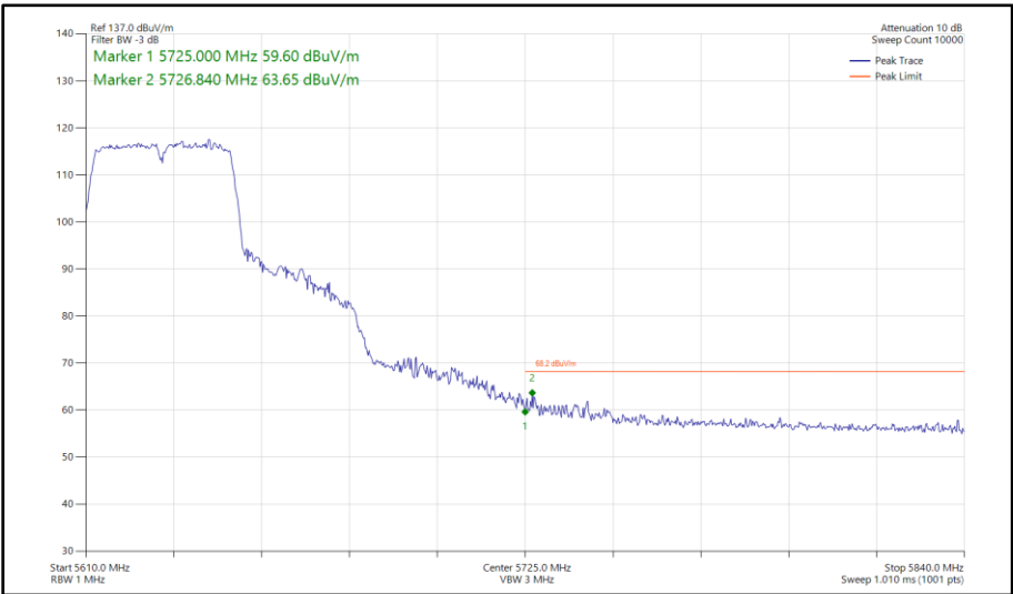
Figure 516 - 802.11n HT40, SISO, Core 0 - 5630 MHz Band Edge Frequency 5725 MHz
