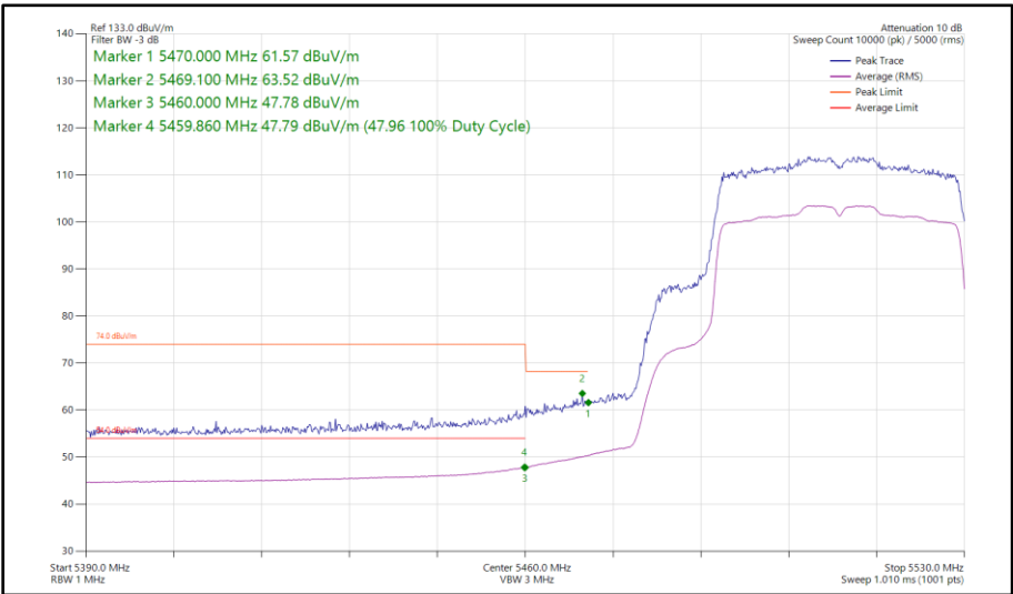
Figure 510 - 802.11ax HE40, SU, SISO, Core 0 - 5510 MHz Band Edge Frequency 5470 MHz
