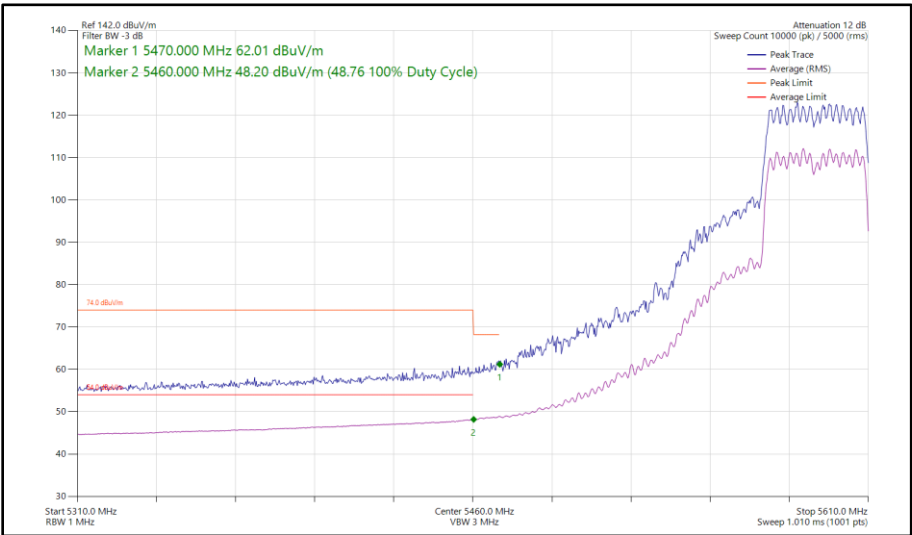
Figure 552 - 802.11ax HE40, SU, CDD, Core 0 - Core 1 - 5590 MHz Band Edge Frequency 5470 MHz
