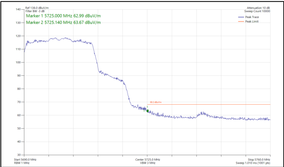
Figure 491 - 802.11ax HE20, SU, SDM, Core 0 - Core 1 - 5700 MHz Band Edge Frequency 5725 MHz
