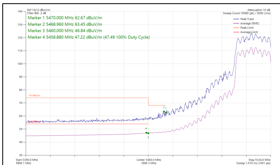
Figure 457 - 802.11ax HE20, SU, CDD, Core 0 - Core 1 - 5520 MHz Band Edge Frequency 5470 MHz
