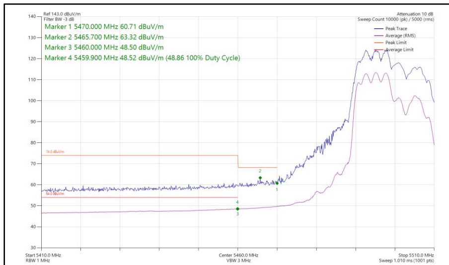
Figure 456 - 802.11ax HE20, RU 106-53, CDD, Core 0 - Core 1 - 5500 MHz Band Edge Frequency 5470 MHz
