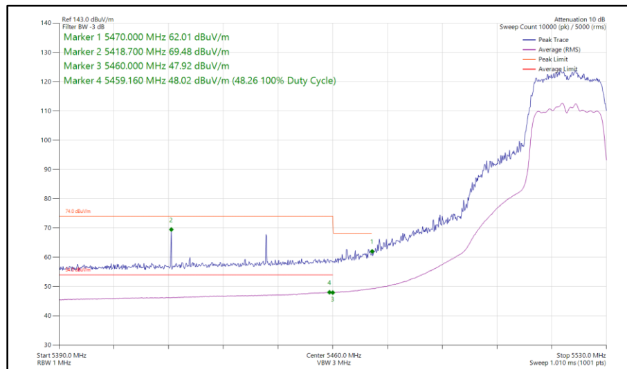
Figure 500 - 802.11ac VHT20, TxBF, Core 0 - Core 1 - 5520 MHz Band Edge Frequency 5470 MHz
