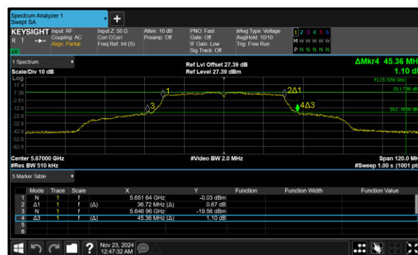
Figure 321 - 802.11n HT40 Maximum 26 dB EBW
