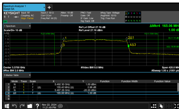
Figure 288 - 802.11ax HE160 SU Minimum 26 dB EBW
