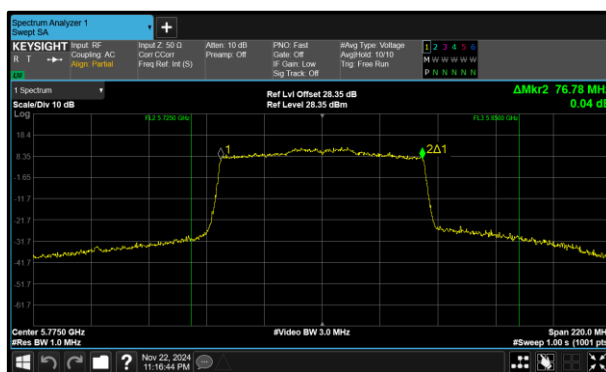
Figure 302 - 802.11ax HE80 SU Minimum 99% OBW
