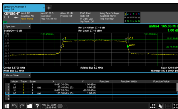
Figure 304 - 802.11ax HE160 SU Minimum 99% OBW
