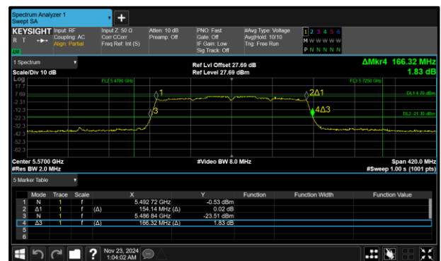
Figure 325 - 802.11ac VHT160 Maximum 26 dB EBW
