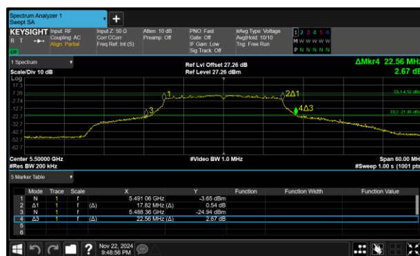
Figure 275 - 802.11n HT20 Maximum 26 dB EBW
