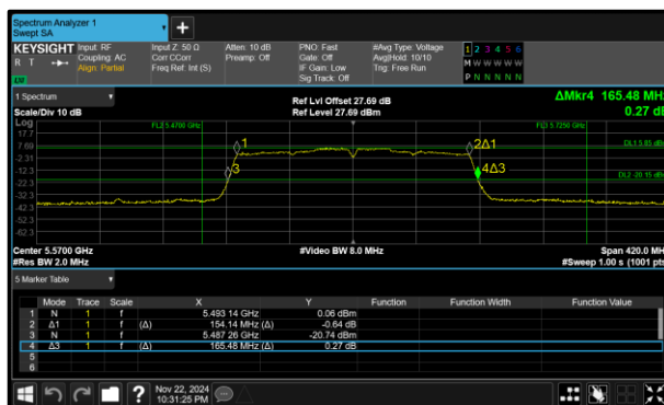
Figure 296 - 802.11ac VHT160 Minimum 99% OBW
