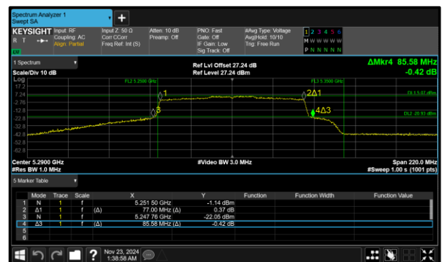
Figure 331 - 802.11ax HE80 SU Maximum 26 dB EBW
