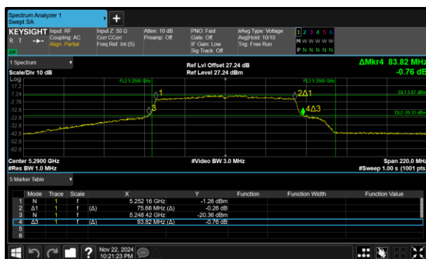
Figure 278 - 802.11ac VHT80 Minimum 26 dB EBW
