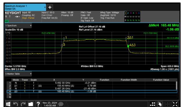
Figure 333 - 802.11ax HE160 SU Maximum 26 dB EBW
