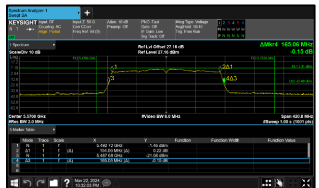
Figure 297 - 802.11ac VHT160 Maximum 99% OBW
