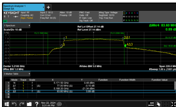
Figure 330 - 802.11ax HE80 SU Minimum 26 dB EBW
