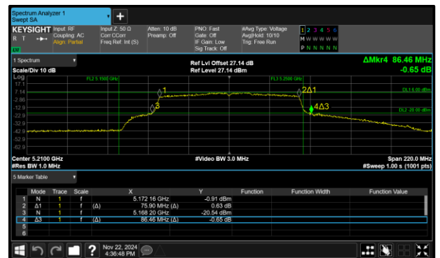
Figure 295 - 802.11ac VHT80 Maximum 99% OBW
