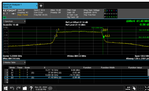
Figure 328 - 802.11ax HE40 SU Minimum 26 dB EBW
