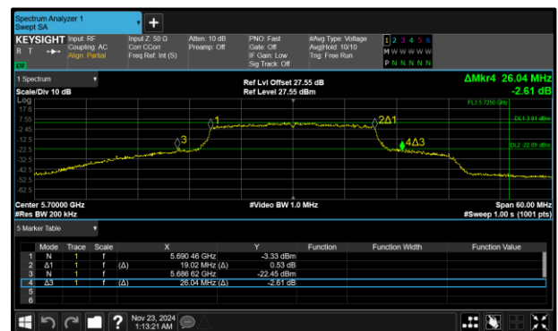
Figure 327 - 802.11ax HE20 SU Maximum 26 dB EBW
