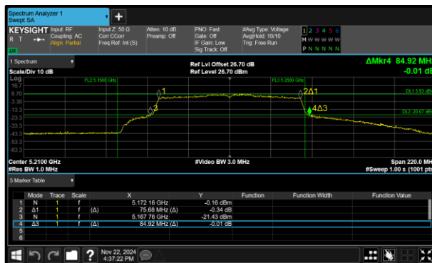
Figure 294 - 802.11ac VHT80 Minimum 99% OBW
