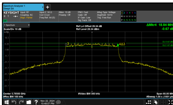
Figure 312 - 802.11ax HE20 SU Minimum 6 dB EBW
