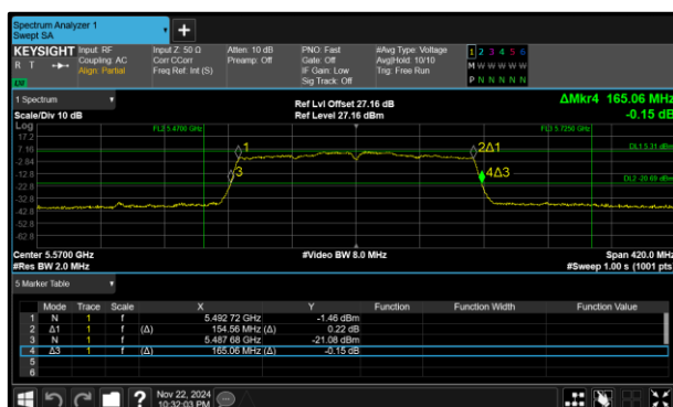
Figure 280 - 802.11ac VHT160 Minimum 26 dB EBW
