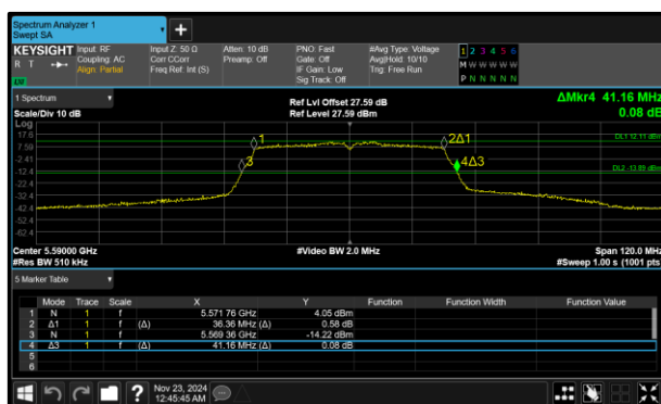
Figure 320 - 802.11n HT40 Minimum 26 dB EBW
