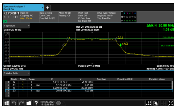
Figure 318 - 802.11n HT20 Minimum 26 dB EBW
