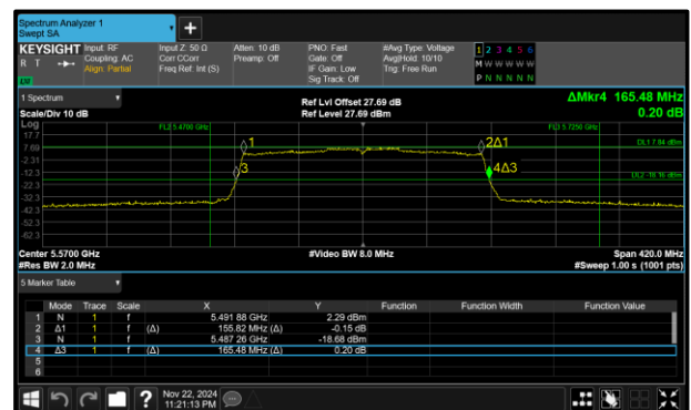
Figure 289 - 802.11ax HE160 SU Maximum 26 dB EBW
