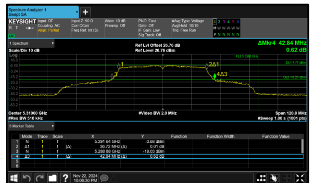
Figure 293 - 802.11n HT40 Maximum 99% OBW
