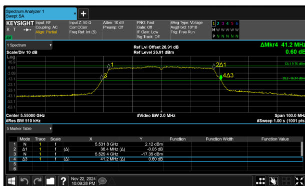
Figure 276 - 802.11n HT40 Minimum 26 dB EBW
