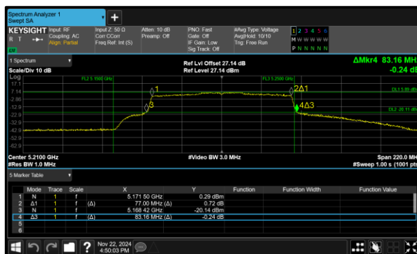
Figure 286 - 802.11ax HE80 SU Minimum 26 dB EBW
