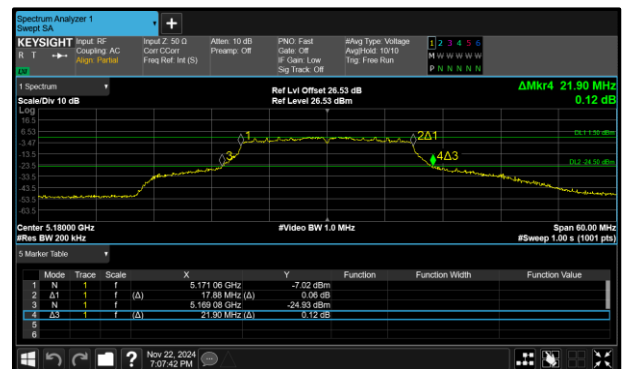
Figure 335 - 802.11n HT20 Maximum 99% OBW
