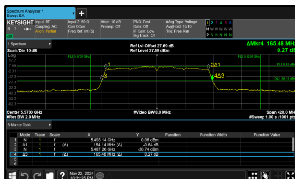
Figure 281 - 802.11ac VHT160 Maximum 26 dB EBW
