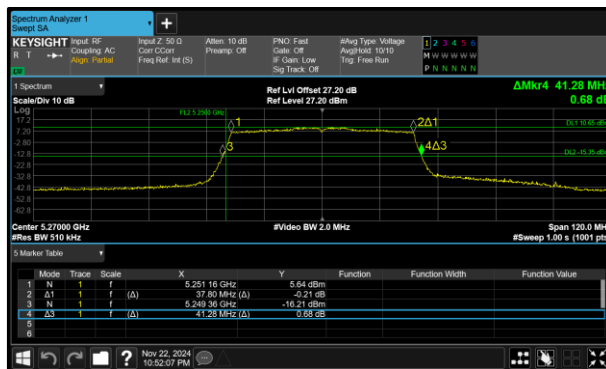
Figure 284 - 802.11ax HE40 SU Minimum 26 dB EBW
