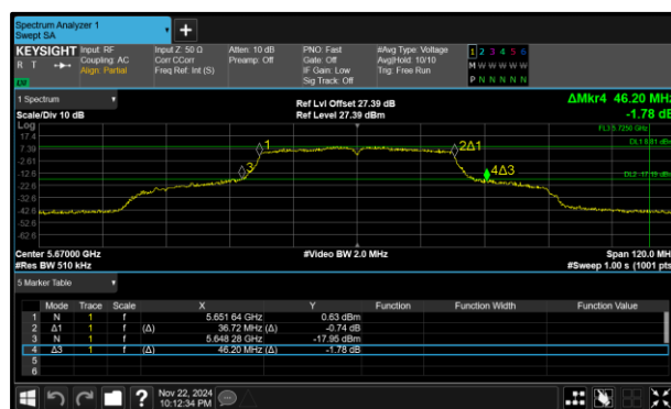
Figure 277 - 802.11n HT40 Maximum 26 dB EBW
