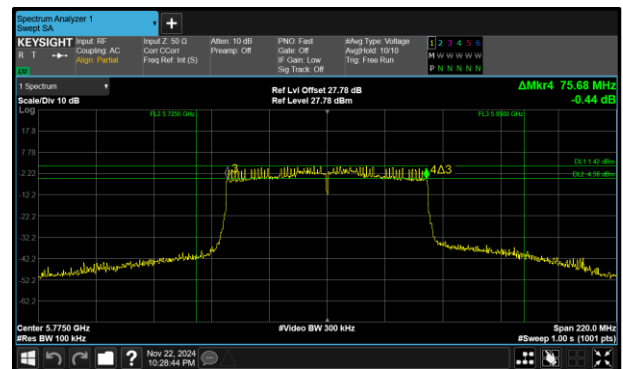
Figure 311 - 802.11ac VHT80 Maximum 6 dB EBW
