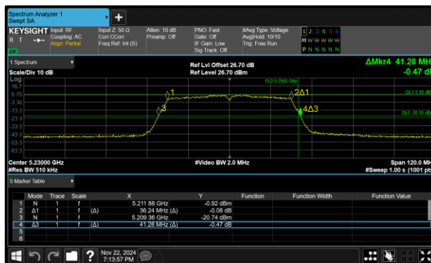
Figure 336 - 802.11n HT40 Minimum 99% OBW
