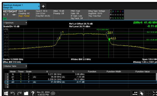
Figure 292 - 802.11n HT40 Minimum 99% OBW
