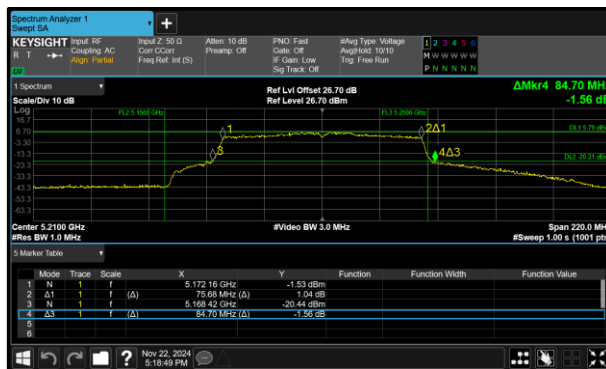
Figure 322 - 802.11ac VHT80 Minimum 26 dB EBW
