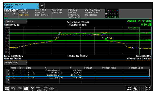
Figure 291 - 802.11n HT20 Maximum 99% OBW
