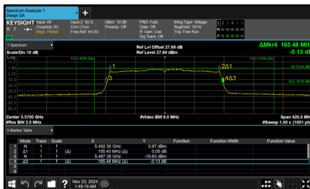
Figure 332 - 802.11ax HE160 SU Minimum 26 dB EBW
