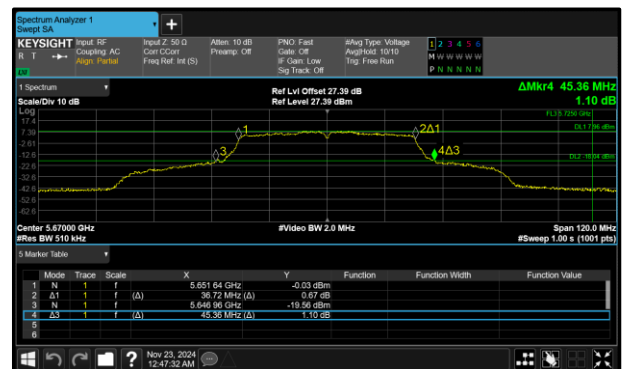
Figure 337 - 802.11n HT40 Maximum 99% OBW
