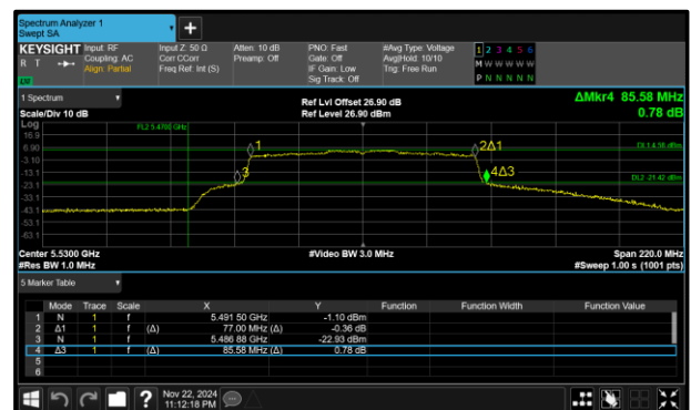
Figure 287 - 802.11ax HE80 SU Maximum 26 dB EBW
