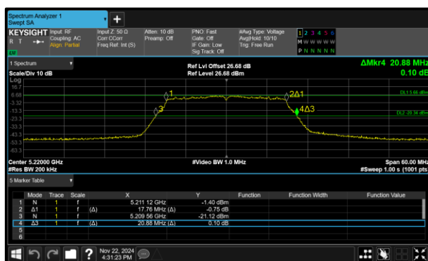
Figure 274 - 802.11n HT20 Minimum 26 dB EBW
