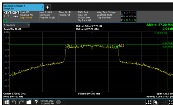
Figure 314 - 802.11ax HE40 SU Minimum 6 dB EBW
