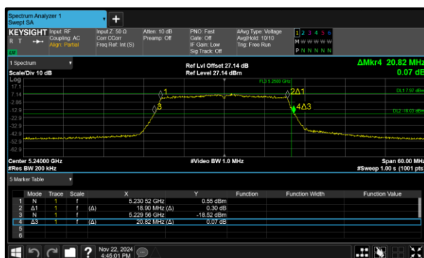
Figure 282 - 802.11ax HE20 SU Minimum 26 dB EBW
