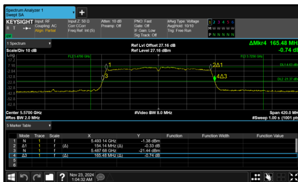
Figure 324 - 802.11ac VHT160 Minimum 26 dB EBW
