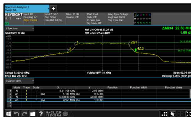
Figure 319 - 802.11n HT20 Maximum 26 dB EBW
