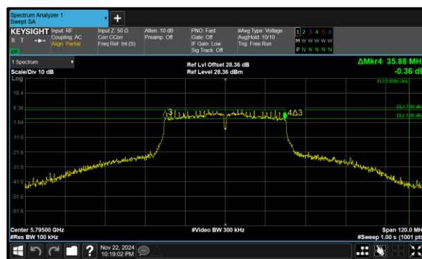
Figure 309 - 802.11n HT40 Maximum 6 dB EBW
