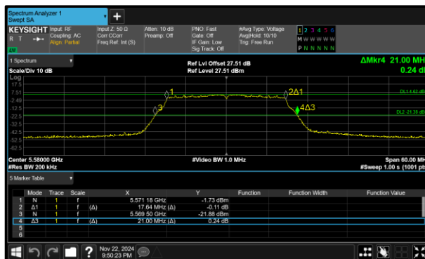
Figure 290 - 802.11n HT20 Minimum 99% OBW
