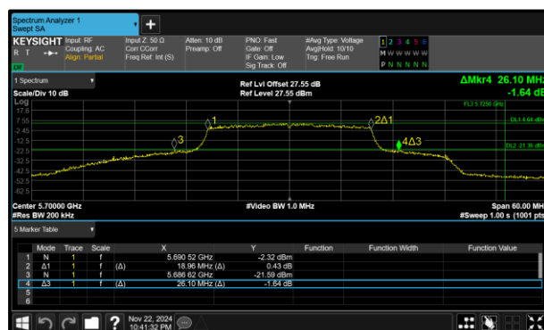
Figure 283 - 802.11ax HE20 SU Maximum 26 dB EBW
