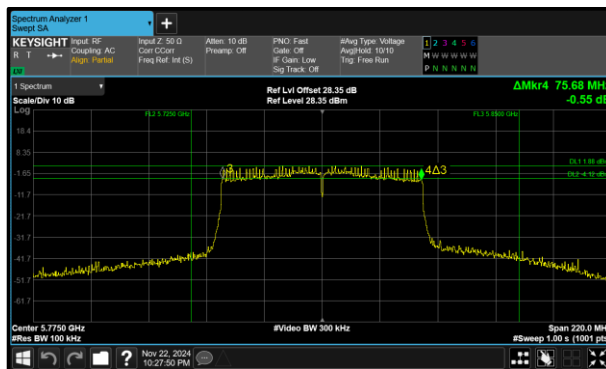
Figure 310 - 802.11ac VHT80 Minimum 6 dB EBW
