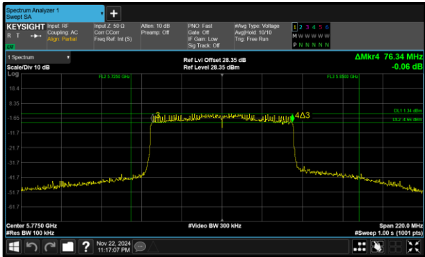
Figure 316 - 802.11ax HE80 SU Minimum 6 dB EBW
