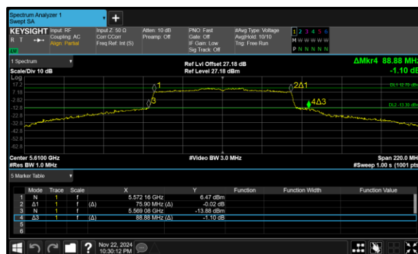
Figure 279 - 802.11ac VHT80 Maximum 26 dB EBW
