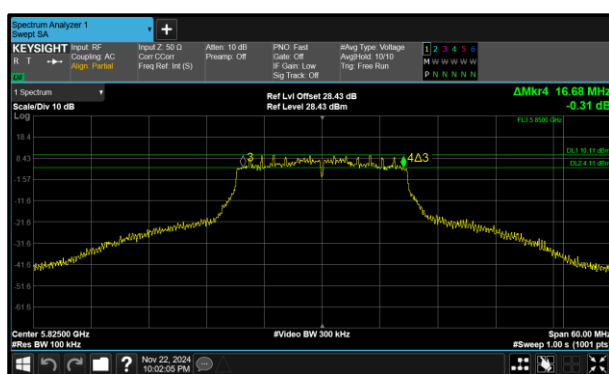
Figure 306 - 802.11n HT20 Minimum 6 dB EBW
