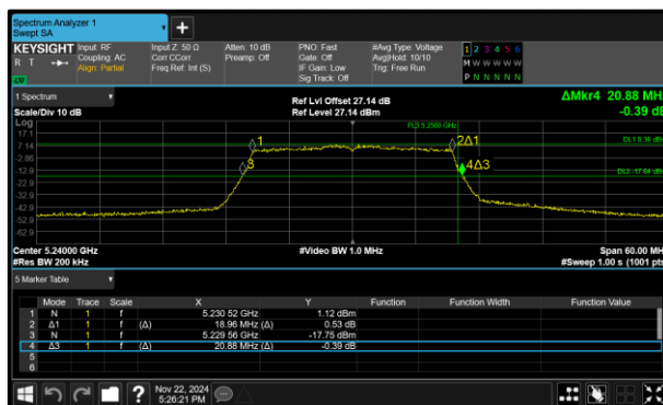
Figure 326 - 802.11ax HE20 SU Minimum 26 dB EBW
