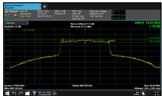
Figure 313 - 802.11ax HE20 SU Maximum 6 dB EBW
