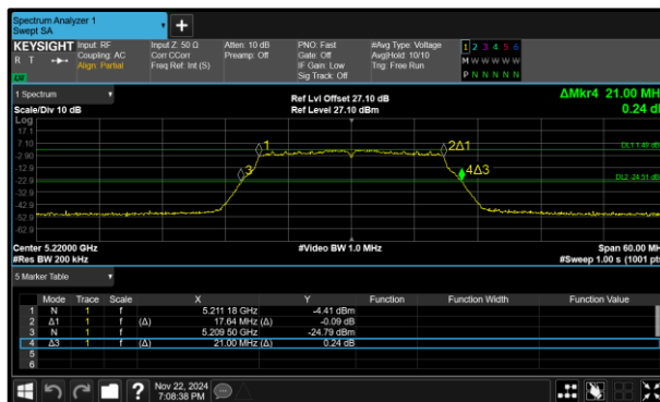
Figure 334 - 802.11n HT20 Minimum 99% OBW
