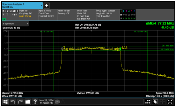
Figure 317 - 802.11ax HE80 SU Maximum 6 dB EBW
