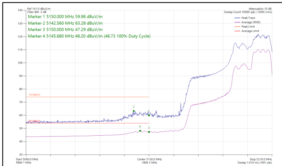
Figure 132 - 802.11ax HE40, RU 106-56, SDM, Core 0 - Core 1 - 5190 MHz Band Edge Frequency 5150 MHz
