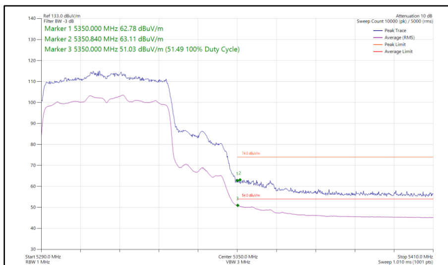
Figure 136 - 802.11ax HE40, SU, SDM, Core 0 - Core 1 - 5310 MHz Band Edge Frequency 5350 MHz
