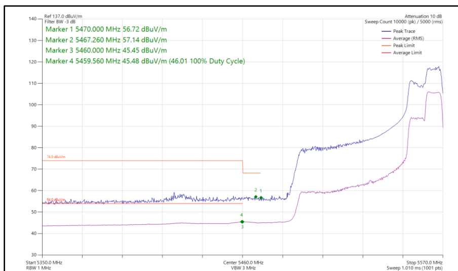
Figure 157 - 802.11ax HE80, RU 106-60, SISO, Core 0 - 5530 MHz Band Edge Frequency 5460 MHz
