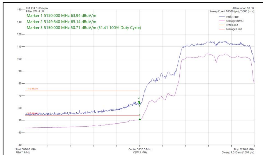
Figure 130 - 802.11n HT40, SDM, Core 0 - Core 1 - 5190 MHz Band Edge Frequency 5150 MHz
