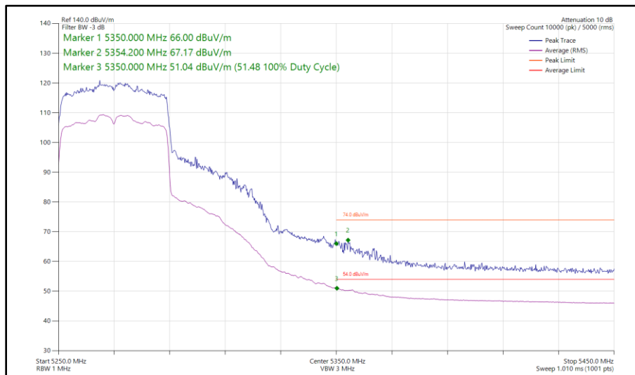
Figure 135 - 802.11ax HE40, SU, SDM, Core 0 - Core 1 - 5270 MHz Band Edge Frequency 5350 MHz
