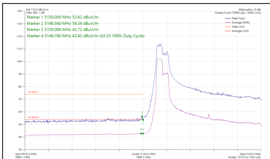
Figure 190 - 802.11ax HE160, RU 106-53P, SISO, Core 0 - 5250 MHz Band Edge Frequency 5150 MHz
