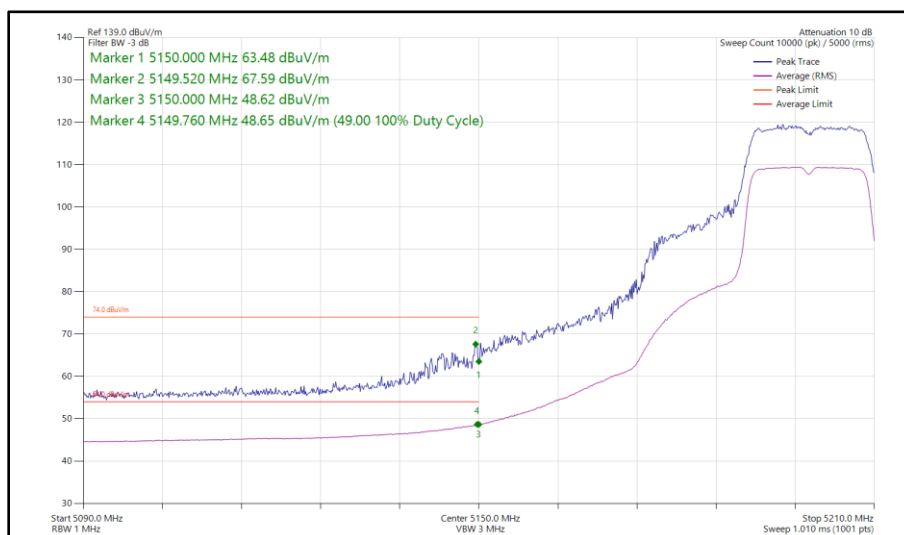
Figure 27 - 802.11n HT20, SISO, Core 1 - 5200 MHz Band Edge Frequency 5150 MHz
