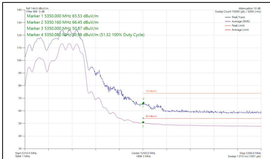
Figure 56 - 802.11ax HE20, RU 106-54, CDD, Core 0 - Core 1 - 5320 MHz Band Edge Frequency 5350 MHz
