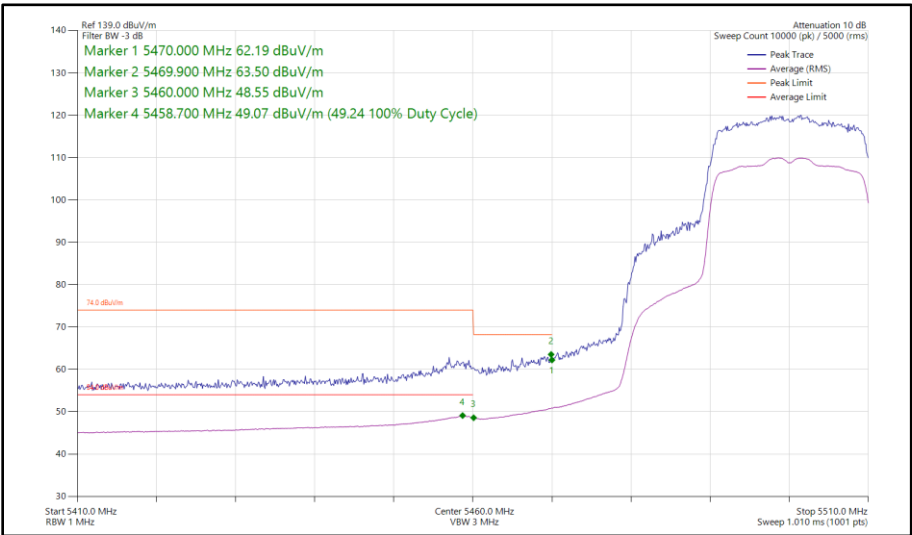
Figure 43 - 802.11ax HE20, SU, SISO, Core 1 - 5500 MHz Band Edge Frequency 5460 MHz
