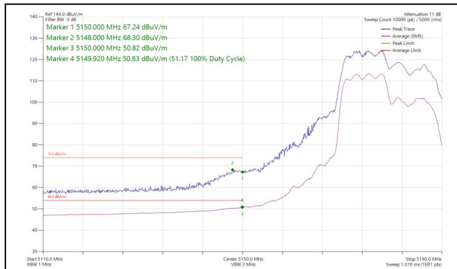
Figure 50 - 802.11ax HE20, RU 106-53, CDD, Core 0 - Core 1 - 5180 MHz Band Edge Frequency 5150 MHz
