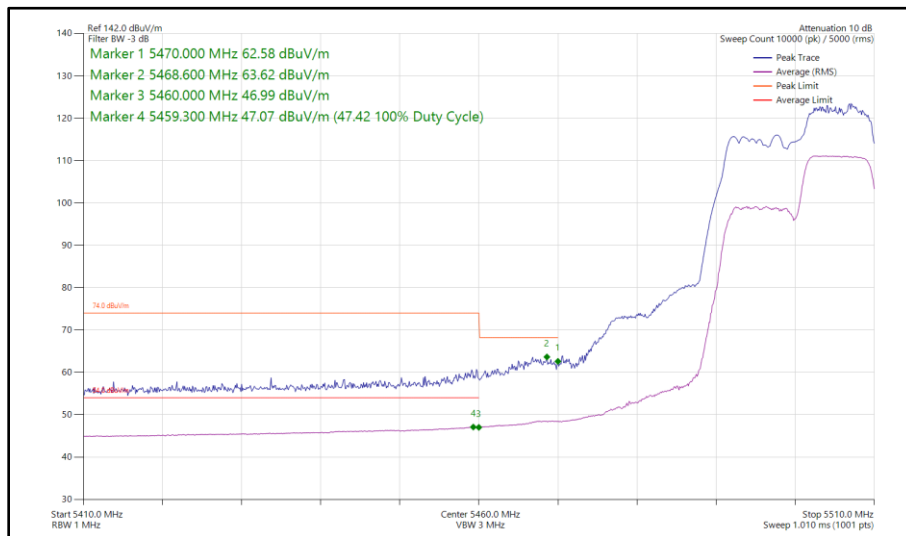
Figure 44 - 802.11ax HE20, RU 106-54, SISO, Core 1 - 5500 MHz Band Edge Frequency 5460 MHz
