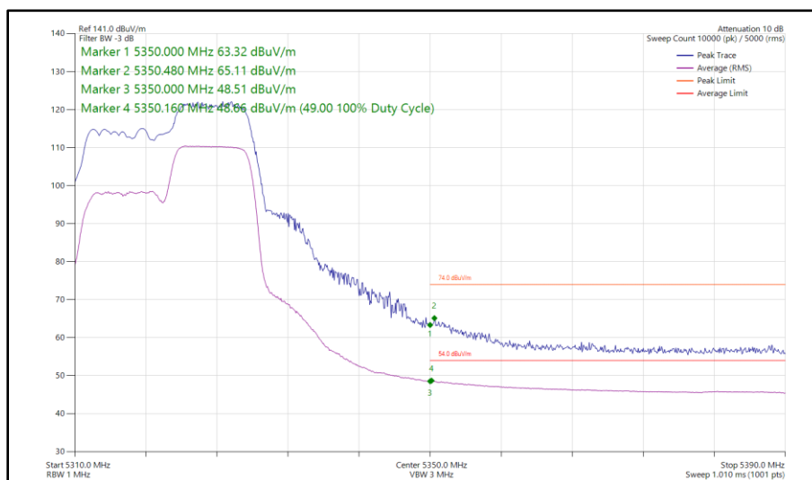
Figure 37 - 802.11ax HE20, RU 106-54, SISO, Core 1 - 5320 MHz Band Edge Frequency 5350 MHz
