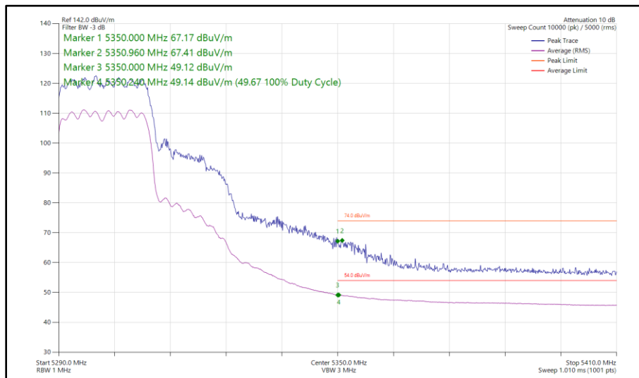
Figure 54 - 802.11ax HE20, SU, CDD, Core 0 - Core 1 - 5300 MHz Band Edge Frequency 5350 MHz
