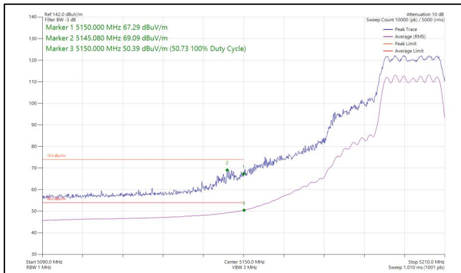
Figure 48 - 802.11n HT20, CDD, Core 0 - Core 1 - 5200 MHz Band Edge Frequency 5150 MHz
