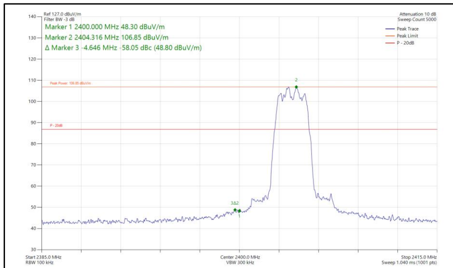
Figure 233 - Bluetooth HDR4, SISO, Core 1 - 2404 MHz Band Edge Frequency 2400 MHz
