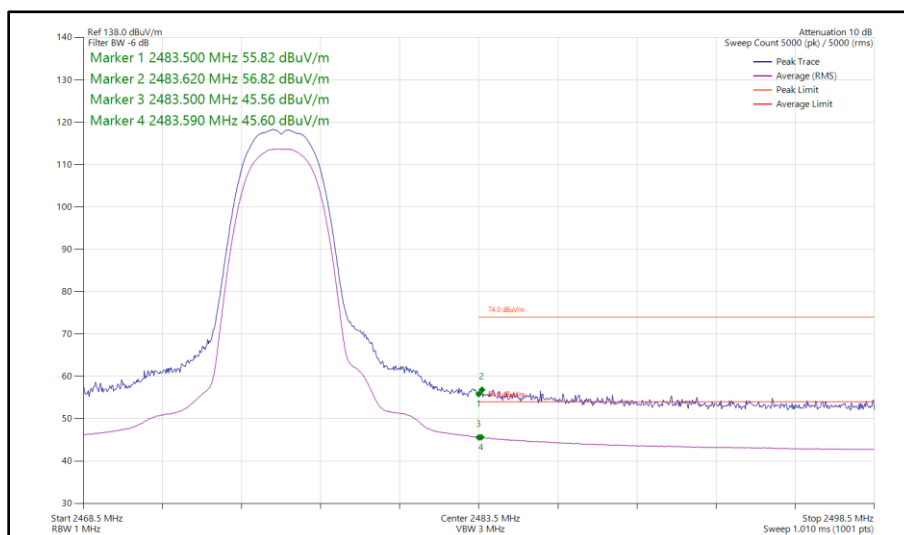
Figure 55 - Bluetooth HDR4, MIMO, Core 0 - Core 1 - 2476 MHz Band Edge Frequency 2483.5 MHz
