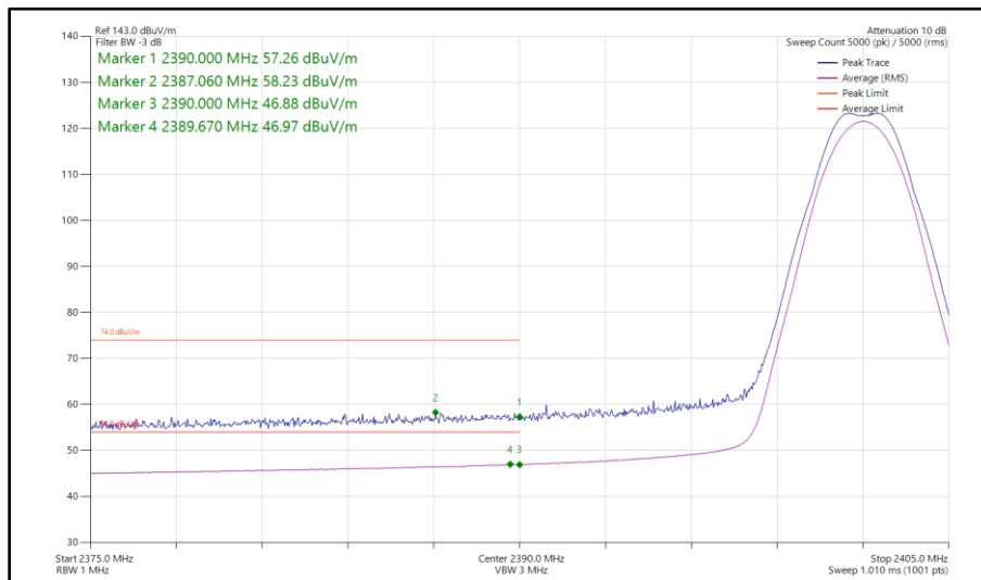
Figure 54 - Bluetooth LE2M, MIMO, Core 0 - Core 1 - 2402 MHz Band Edge Frequency 2390 MHz
