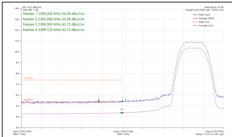
Figure 22 - Bluetooth HDR8, MIMO, Core 0 - Core 1 - 2404 MHz Band Edge Frequency 2390 MHz
