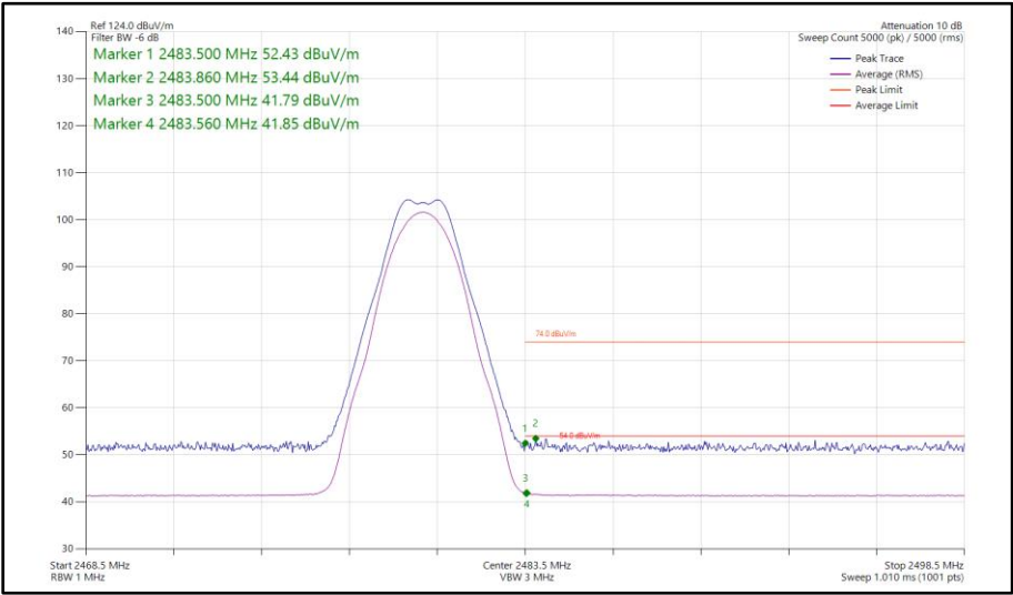
Figure 30 - Bluetooth LE2M, MIMO, Core 0-1 - 2480 MHz Band Edge Frequency 2483.5 MHz
