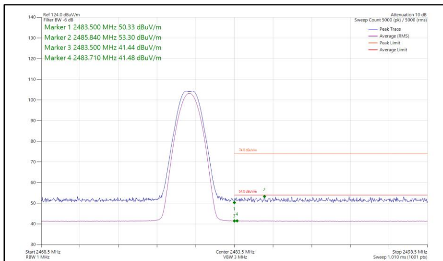
Figure 29 - Bluetooth LE1M, MIMO, Core 0-1 - 2480 MHz Band Edge Frequency 2483.5 MHz
