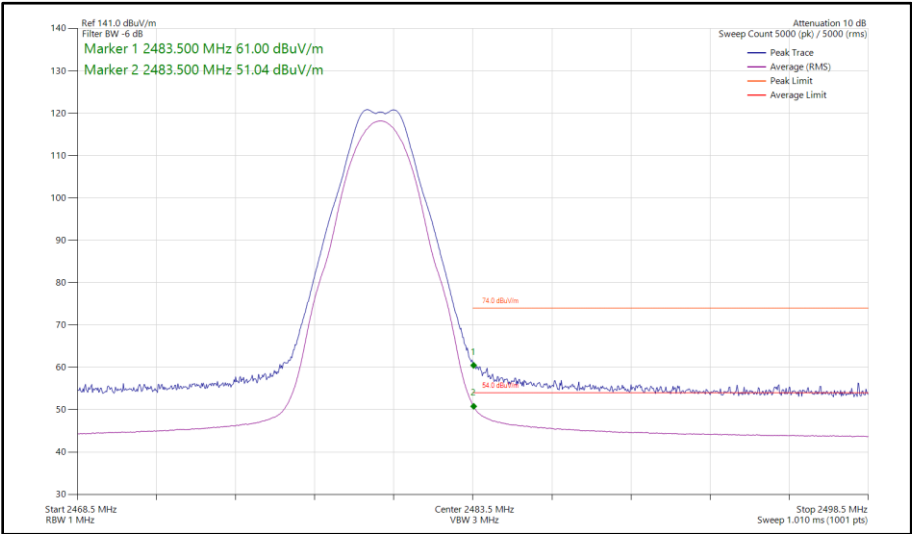
Figure 60 - Bluetooth LE2M, MIMO, Core 0-1 - 2480 MHz Band Edge Frequency 2483.5 MHz
