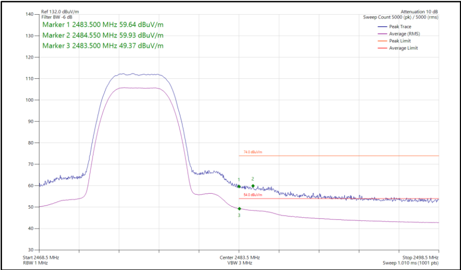
Figure 36 - Bluetooth HDR8, SISO, Core 0 - 2476 MHz Band Edge Frequency 2483.5 MHz
