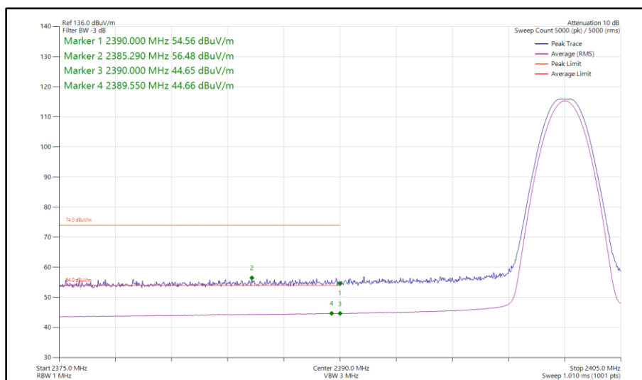
Figure 43 - Bluetooth LE1M, SISO, Core 1 - 2402 MHz Band Edge Frequency 2390 MHz
