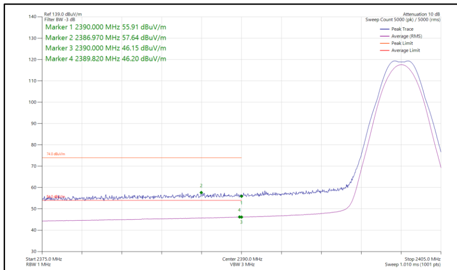
Figure 34 - Bluetooth LE2M, SISO, Core 0 - 2402 MHz Band Edge Frequency 2390 MHz
