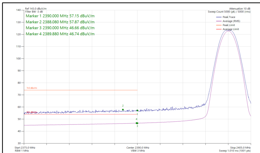
Figure 53 - Bluetooth LE1M, MIMO, Core 0 - Core 1 - 2402 MHz Band Edge Frequency 2390 MHz
