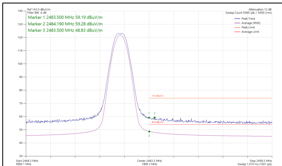
Figure 59 - Bluetooth LE1M, MIMO, Core 0-1 - 2480 MHz Band Edge Frequency 2483.5 MHz
