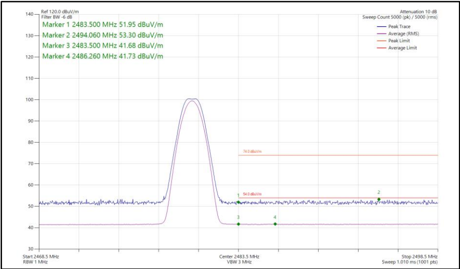
Figure 9 - Bluetooth LE1M, SISO, Core 0 - 2480 MHz Band Edge Frequency 2483.5 MHz
