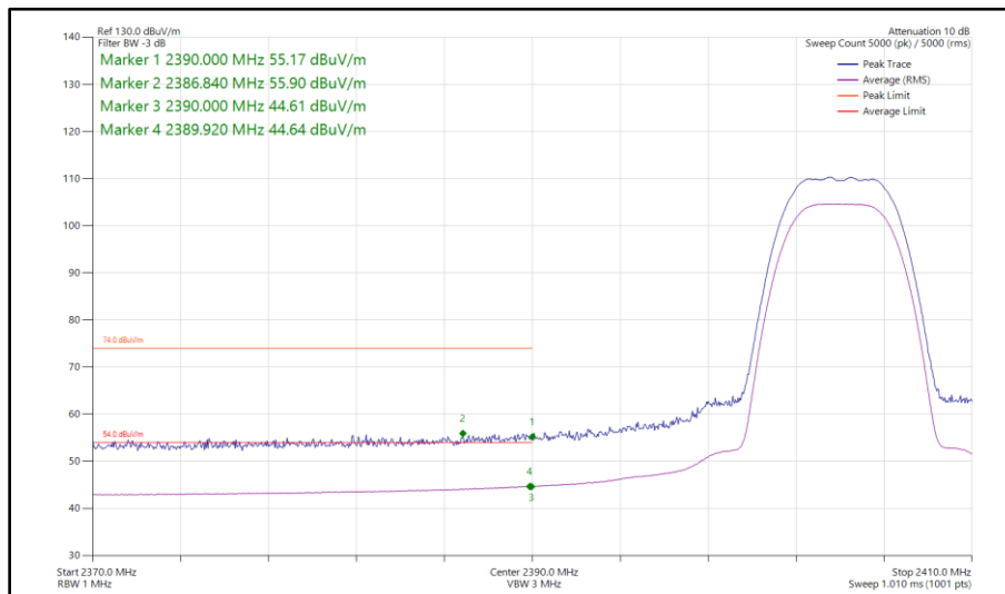
Figure 42 - Bluetooth HDR8, SISO, Core 1 - 2404 MHz Band Edge Frequency 2390 MHz
