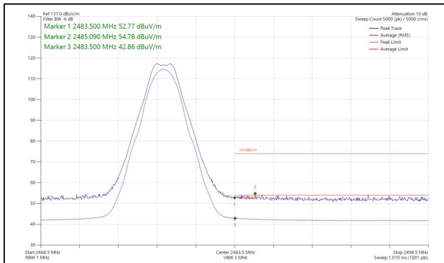
Figure 28 - Bluetooth LE2M, MIMO, Core 0 - Core 1 - 2478 MHz Band Edge Frequency 2483.5 MHz
