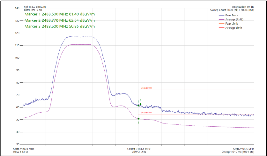
Figure 56 - Bluetooth HDR8, MIMO, Core 0 - Core 1 - 2476 MHz Band Edge Frequency 2483.5 MHz
