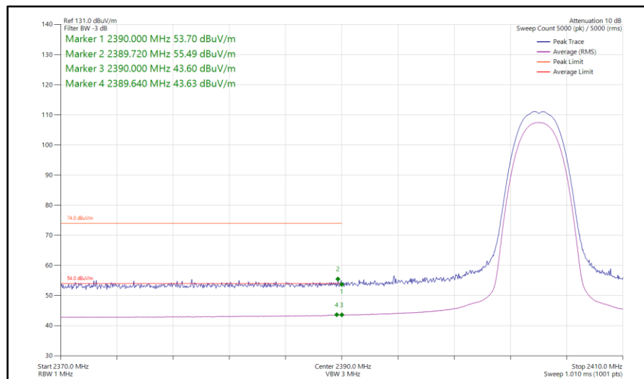
Figure 41 - Bluetooth HDR4, SISO, Core 1 - 2404 MHz Band Edge Frequency 2390 MHz
