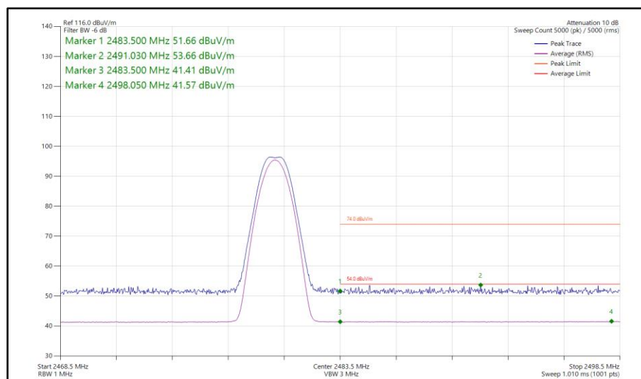
Figure 19 - Bluetooth LE1M, SISO, Core 1 - 2480 MHz Band Edge Frequency 2483.5 MHz
