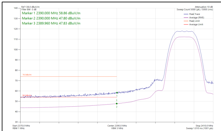
Figure 52 - Bluetooth HDR8, MIMO, Core 0 - Core 1 - 2404 MHz Band Edge Frequency 2390 MHz
