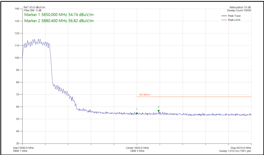
Figure 387 - 802.11ax HE40, SU, CDD, Core 0-1 - 5710 MHz Band Edge Frequency 5850 MHz
