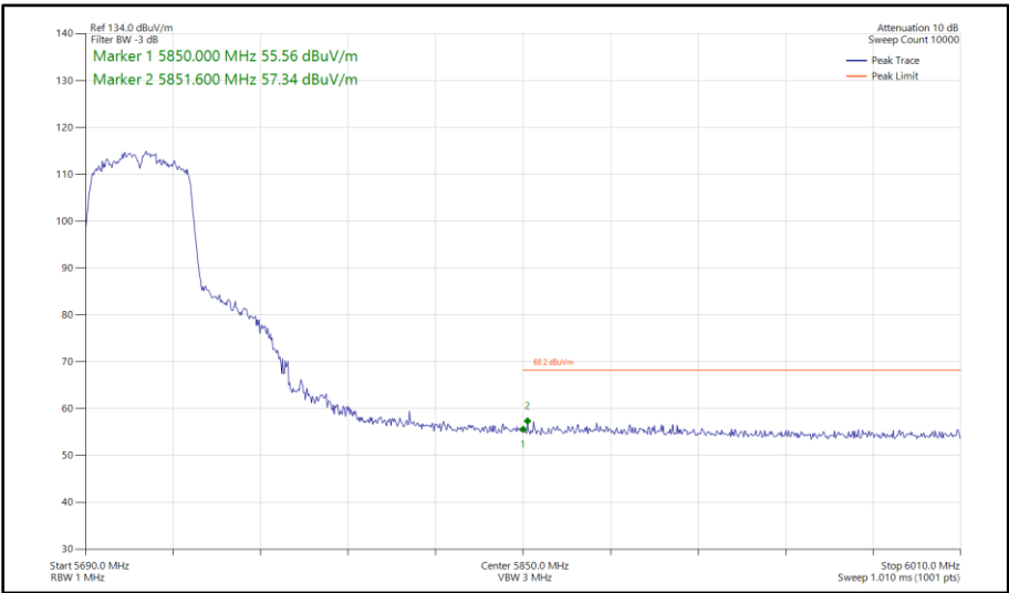
Figure 370 - 802.11n HT40, SISO, Core 1 - 5710 MHz Band Edge Frequency 5850 MHz
