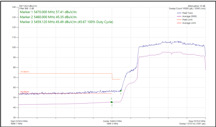
Figure 414 - 802.11ax HE80, SU, SISO, Core 0 - 5530 MHz Band Edge Frequency 5470 MHz
