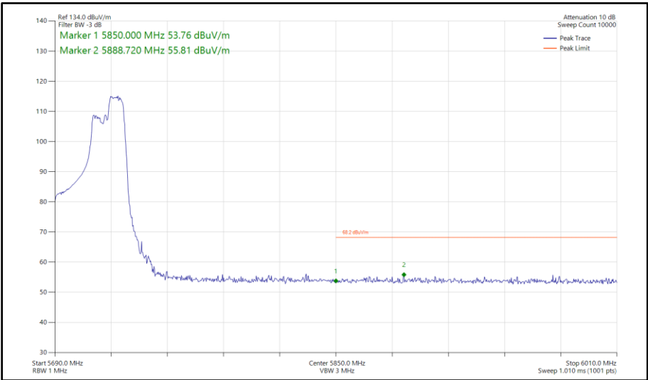
Figure 373 - 802.11ax HE40, RU 106-56, SISO, Core 1 - 5710 MHz Band Edge Frequency 5850 MHz
