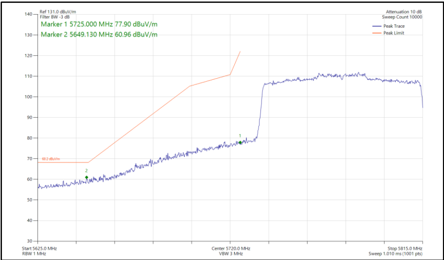
Figure 432 - 802.11ax HE80, SU, SISO, Core 1 - 5775 MHz Band Edge Frequency 5725 MHz
