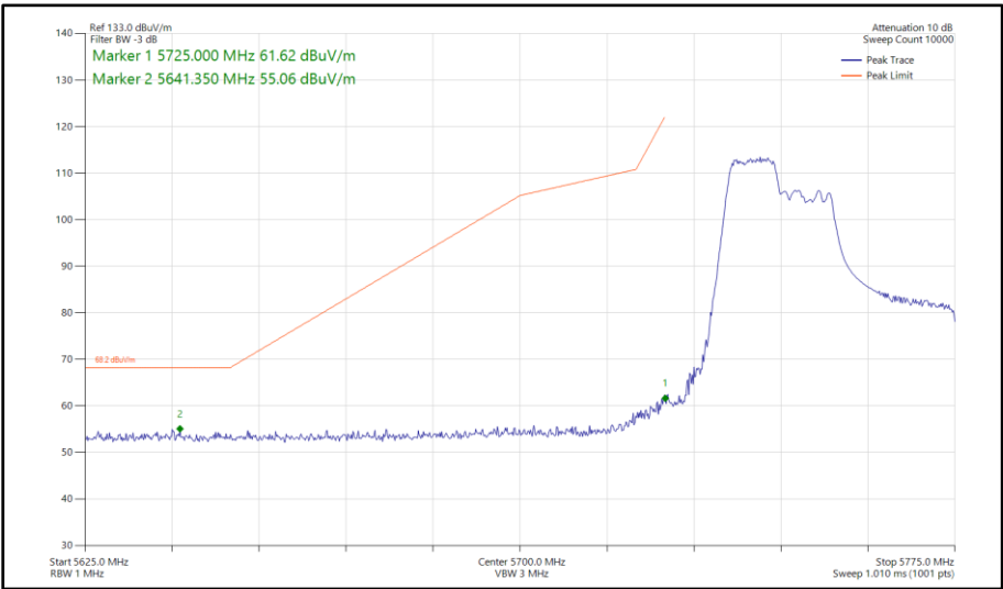
Figure 366 - 802.11ax HE40, RU 106-53, SISO, Core 1 - 5755 MHz Band Edge Frequency 5725 MHz
