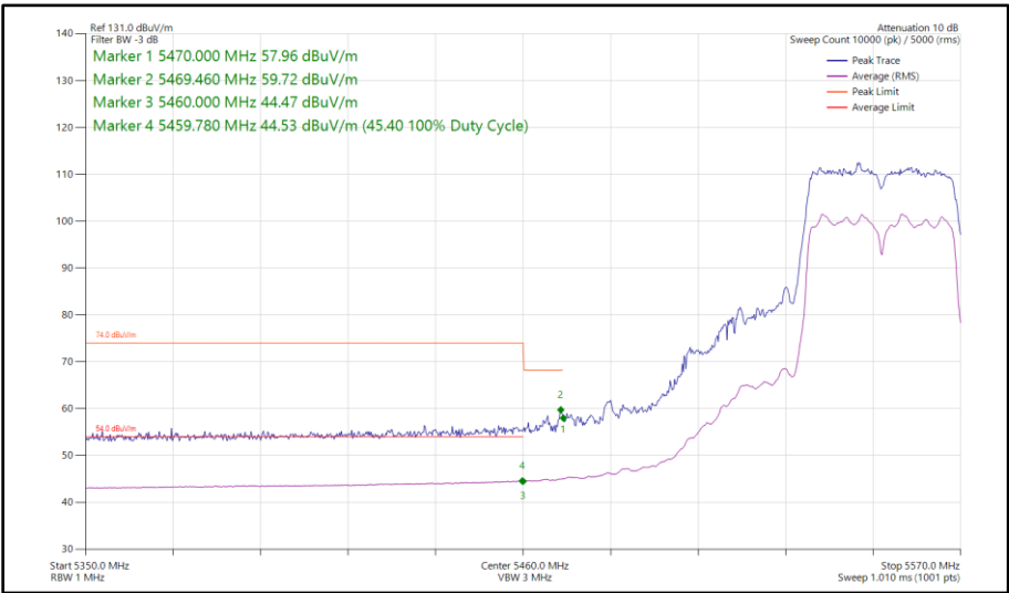
Figure 392 - 802.11n HT40, SDM, Core 0-1 - 5550 MHz Band Edge Frequency 5470 MHz
