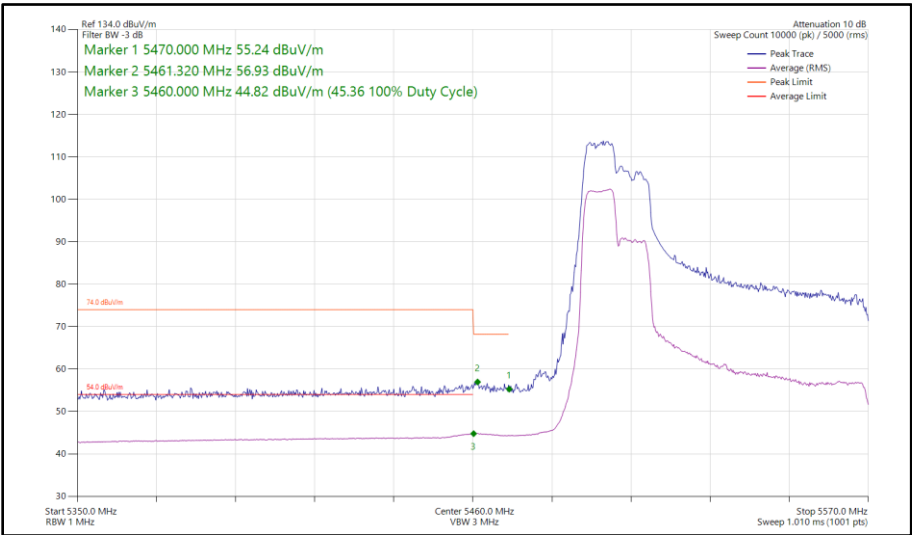
Figure 430 - 802.11ax HE80, RU 106-53, SISO, Core 1 - 5530 MHz Band Edge Frequency 5470 MHz
