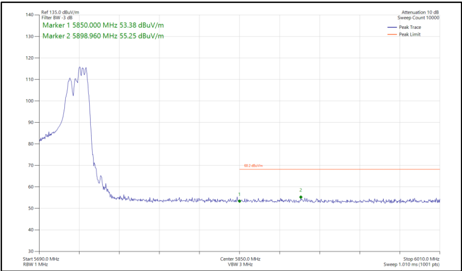
Figure 405 - 802.11ax HE40, RU 106-56, SDM, Core 0-1 - 5710 MHz Band Edge Frequency 5850 MHz
