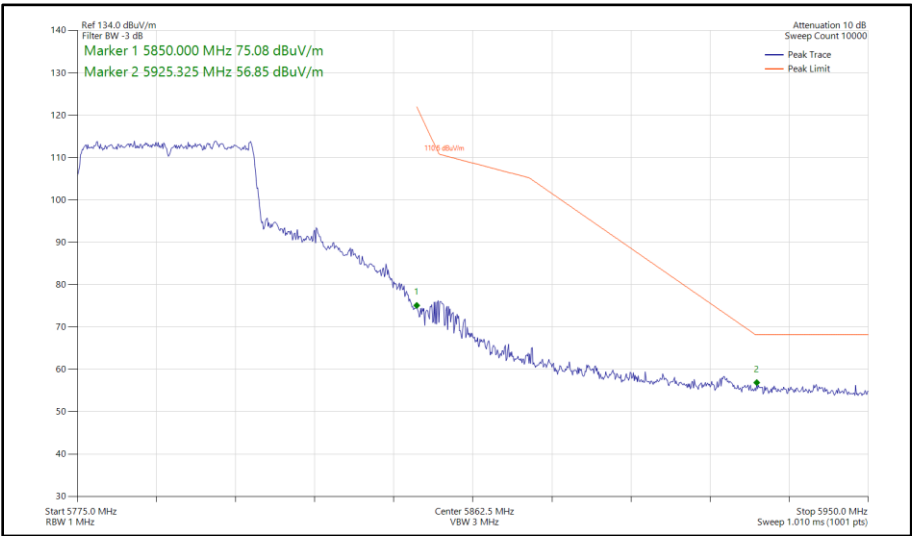
Figure 406 - 802.11ax HE40, SU, SDM, Core 0-1 - 5795 MHz Band Edge Frequency 5850 MHz
