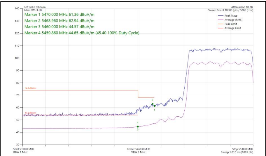
Figure 393 - 802.11ax HE40, SU, SDM, Core 0-1 - 5510 MHz Band Edge Frequency 5470 MHz
