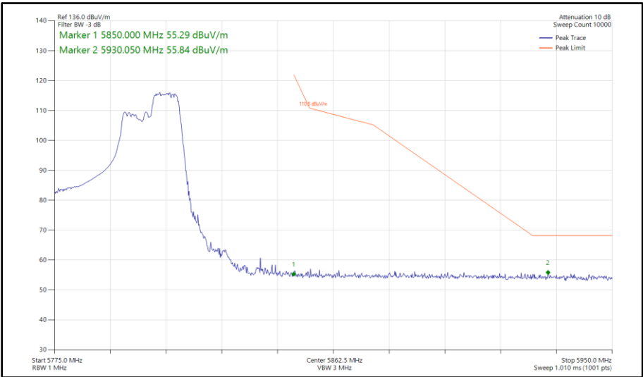
Figure 375 - 802.11ax HE40, RU 106-56, SISO, Core 1 - 5795 MHz Band Edge Frequency 5850 MHz
