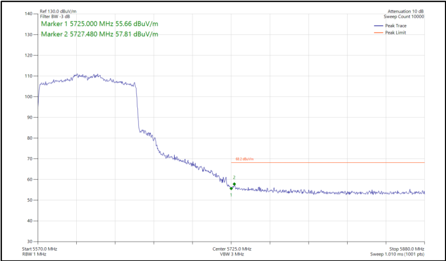
Figure 420 - 802.11ax HE80, SU, SISO, Core 0 - 5610 MHz Band Edge Frequency 5725 MHz
