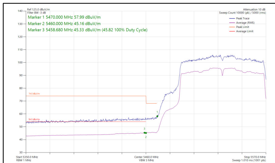
Figure 413 - 802.11ac VHT80, SISO, Core 0 - 5530 MHz Band Edge Frequency 5470 MHz
