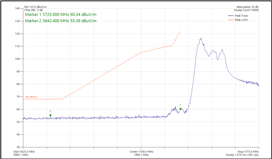
Figure 381 - 802.11ax HE40, RU 52-37, CDD, Core 0-1 - 5755 MHz Band Edge Frequency 5725 MHz
