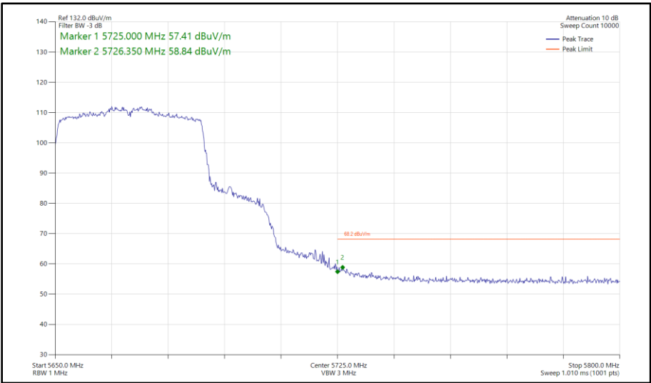
Figure 400 - 802.11ax HE40, SU, SDM, Core 0-1 - 5670 MHz Band Edge Frequency 5725 MHz
