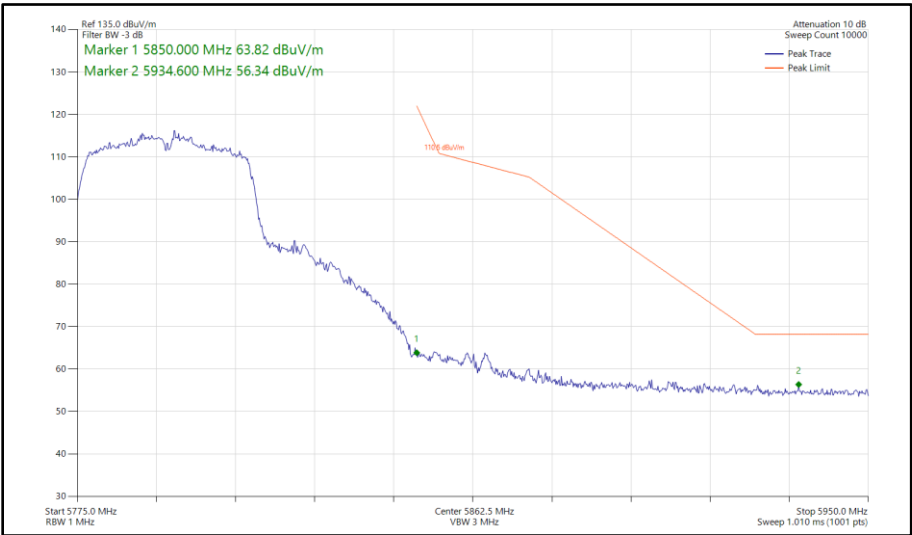
Figure 356 - 802.11n HT40, SISO, Core 0 - 5795 MHz Band Edge Frequency 5850 MHz
