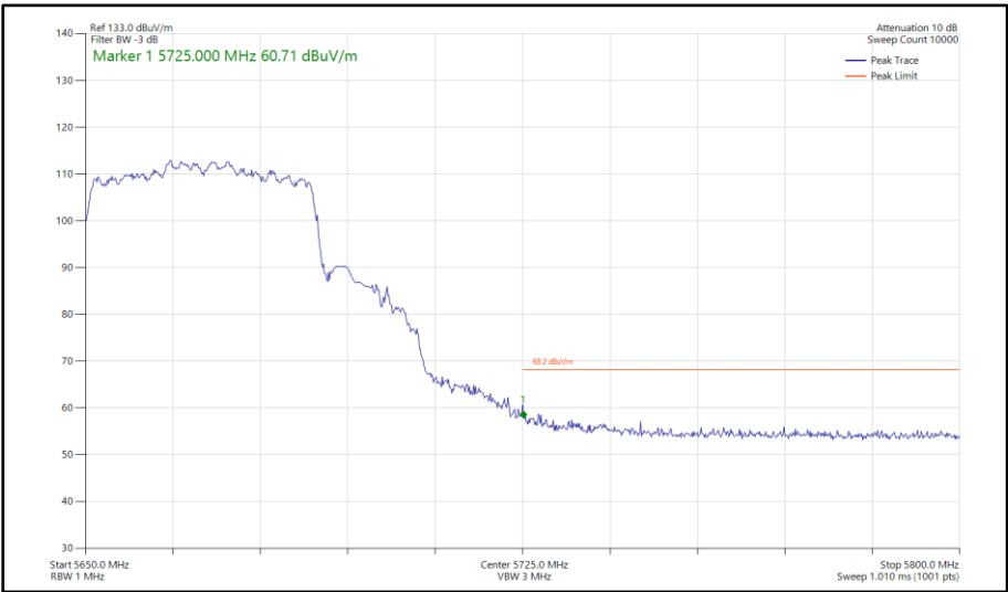
Figure 383 - 802.11ax HE40, SU, CDD, Core 0-1 - 5670 MHz Band Edge Frequency 5725 MHz
