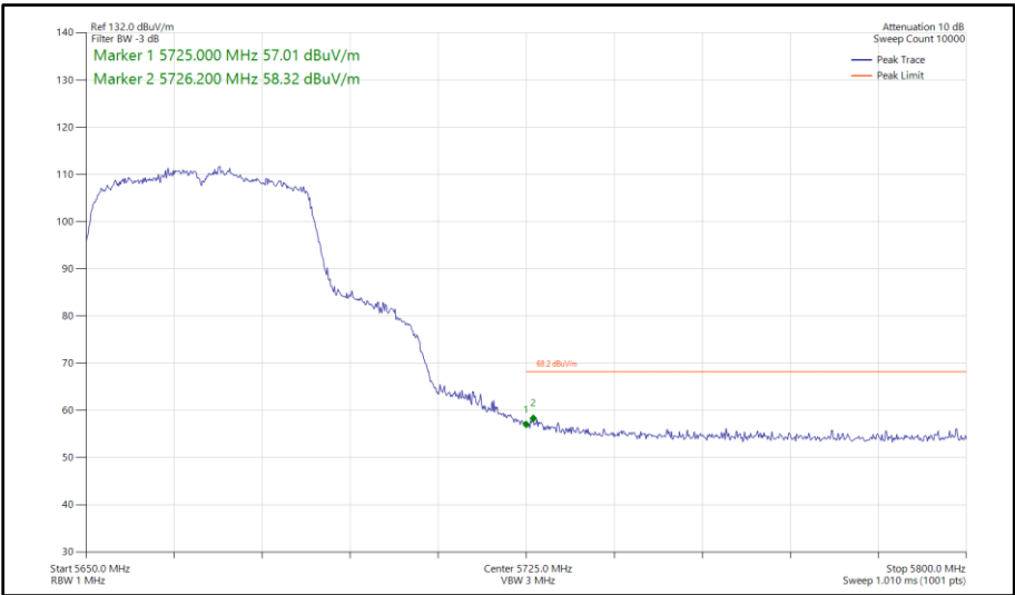
Figure 367 - 802.11n HT40, SISO, Core 1 - 5670 MHz Band Edge Frequency 5725 MHz
