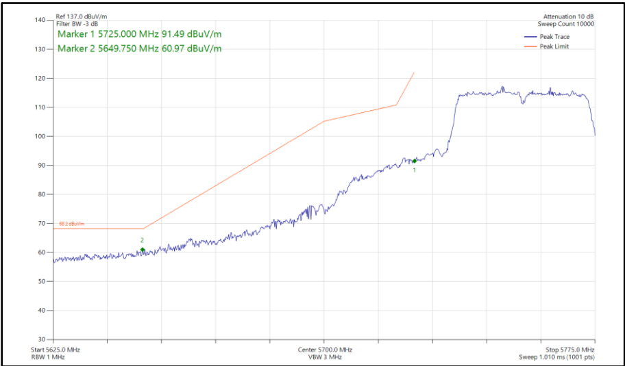
Figure 395 - 802.11n HT40, SDM, Core 0-1 - 5755 MHz Band Edge Frequency 5725 MHz
