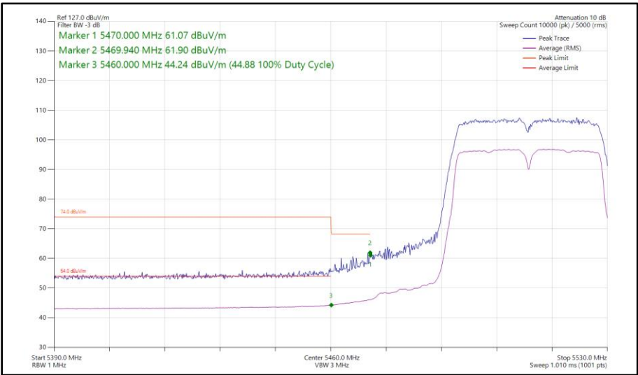
Figure 361 - 802.11n HT40, SISO, Core 1 - 5510 MHz Band Edge Frequency 5470 MHz
