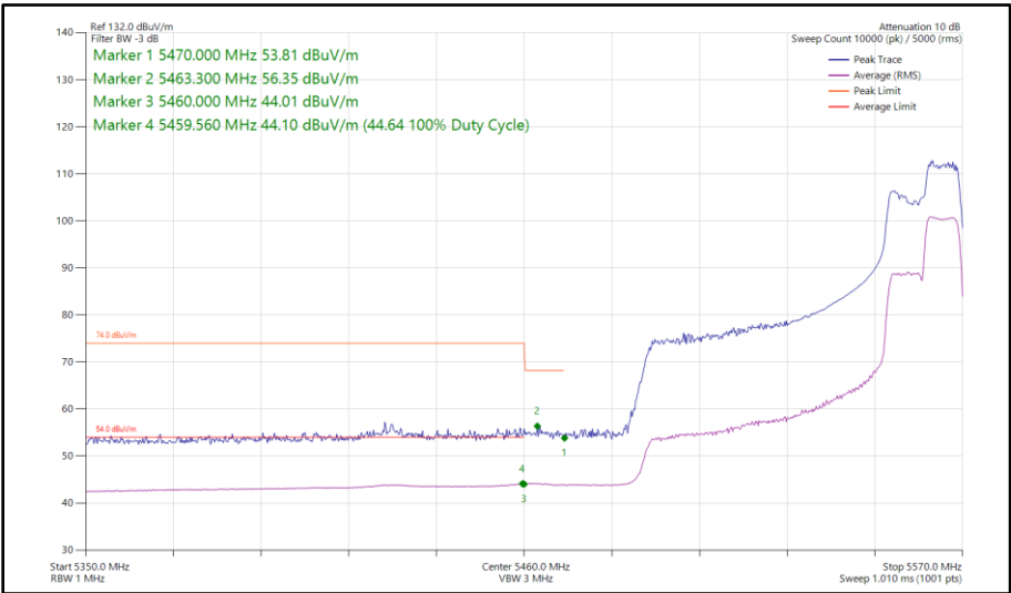
Figure 415 - 802.11ax HE80, RU 106-60, SISO, Core 0 - 5530 MHz Band Edge Frequency 5470 MHz
