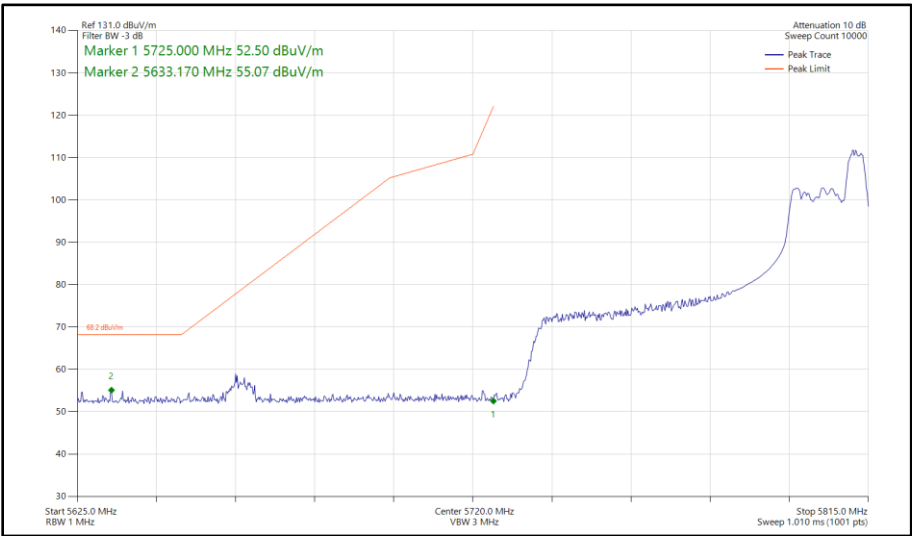
Figure 418 - 802.11ax HE80, RU 52-52, SISO, Core 0 - 5775 MHz Band Edge Frequency 5725 MHz
