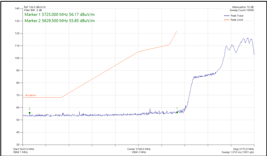
Figure 397 - 802.11ax HE40, RU 106-56, SDM, Core 0-1 - 5755 MHz Band Edge Frequency 5725 MHz
