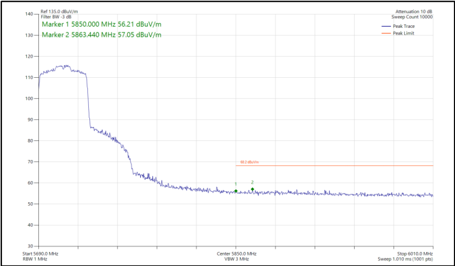
Figure 372 - 802.11ax HE40, SU, SISO, Core 1 - 5710 MHz Band Edge Frequency 5850 MHz
