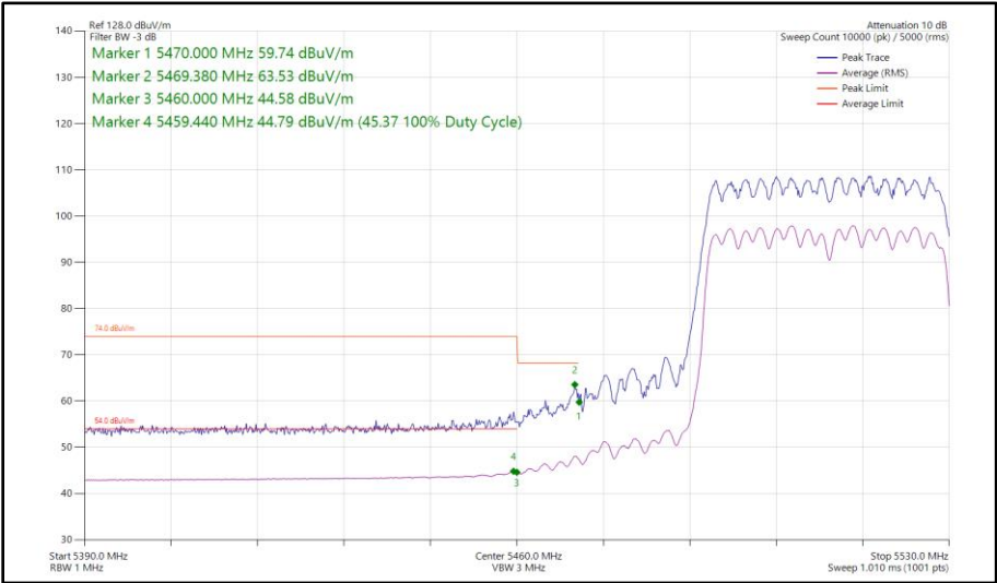
Figure 377 - 802.11ax HE40, SU, CDD, Core 0-1 - 5510 MHz Band Edge Frequency 5470 MHz
