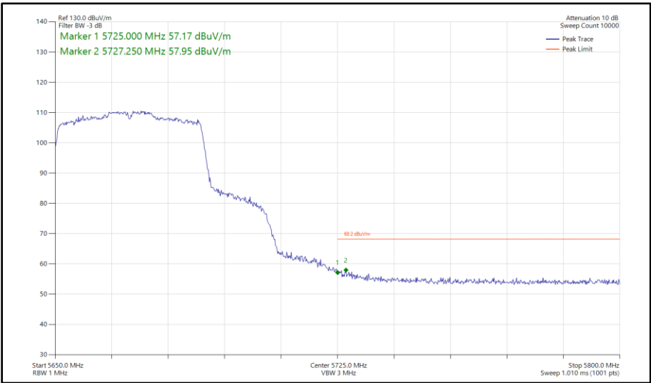
Figure 368 - 802.11ax HE40, SU, SISO, Core 1 - 5670 MHz Band Edge Frequency 5725 MHz
