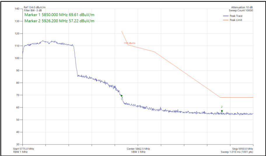
Figure 374 - 802.11ax HE40, SU, SISO, Core 1 - 5795 MHz Band Edge Frequency 5850 MHz
