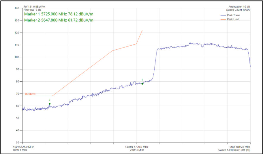
Figure 431 - 802.11ac VHT80, SISO, Core 1 - 5775 MHz Band Edge Frequency 5725 MHz
