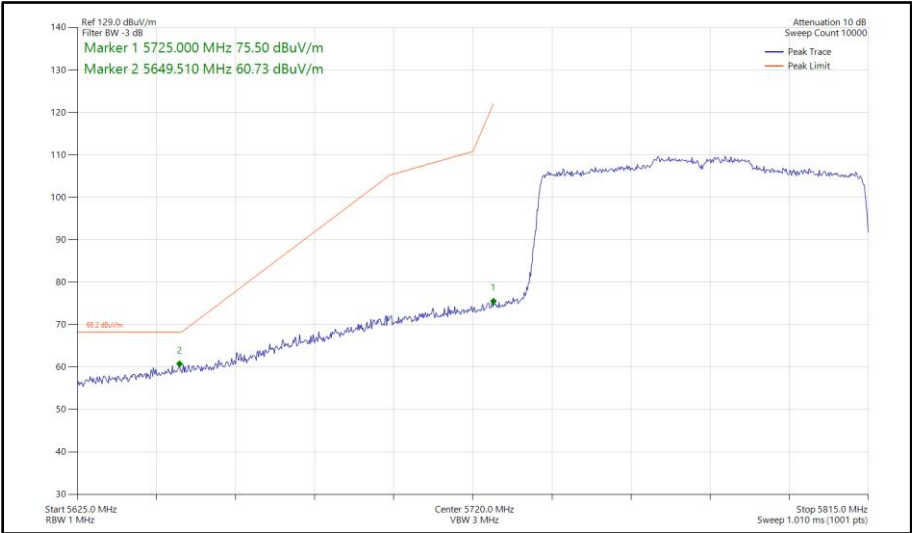
Figure 417 - 802.11ax HE80, SU, SISO, Core 0 - 5775 MHz Band Edge Frequency 5725 MHz
