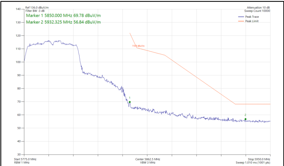
Figure 403 - 802.11n HT40, SDM, Core 0-1 - 5795 MHz Band Edge Frequency 5850 MHz
