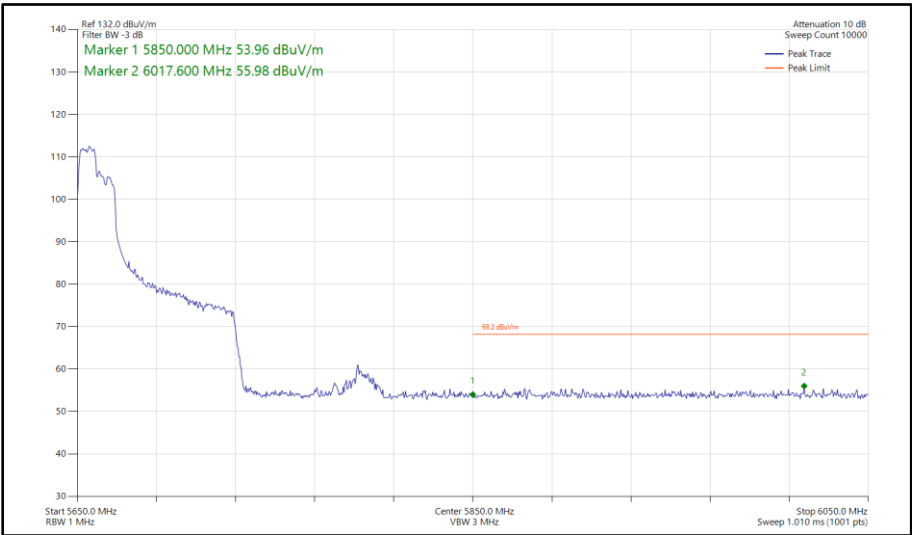
Figure 425 - 802.11ax HE80, RU 106-53, SISO, Core 0 - 5690 MHz Band Edge Frequency 5850 MHz
