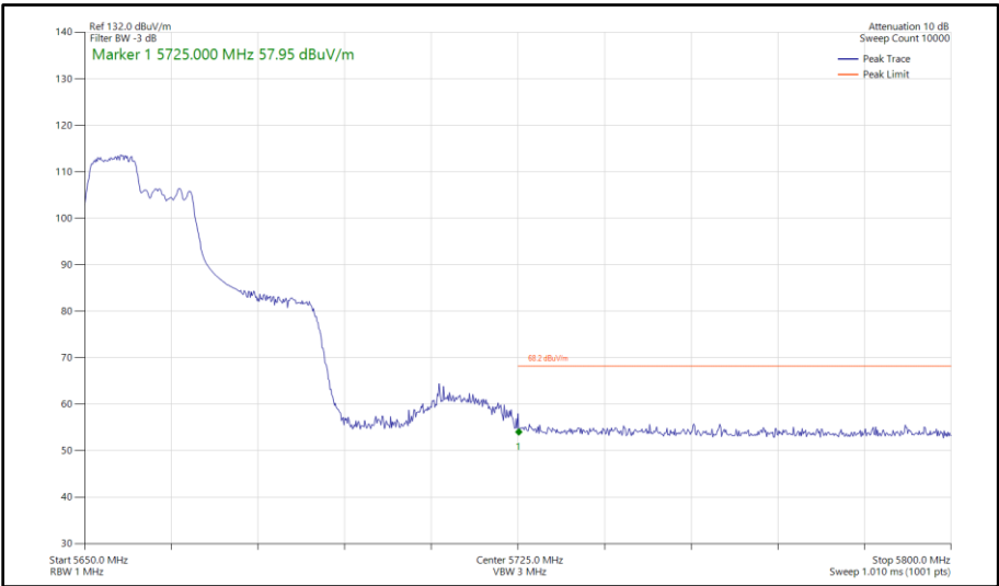
Figure 369 - 802.11ax HE40, RU 106-53, SISO, Core 1 - 5670 MHz Band Edge Frequency 5725 MHz
