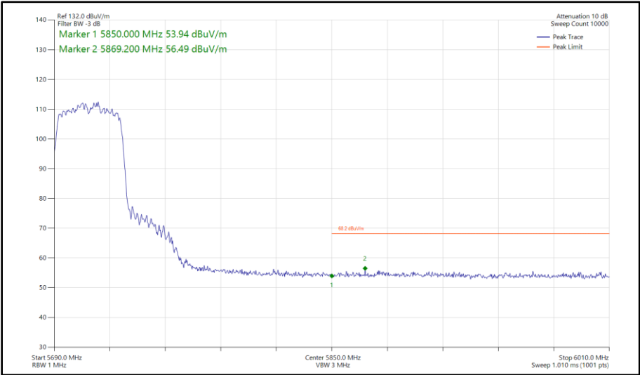
Figure 385 - 802.11n HT40, CDD, Core 0-1 - 5710 MHz Band Edge Frequency 5850 MHz
