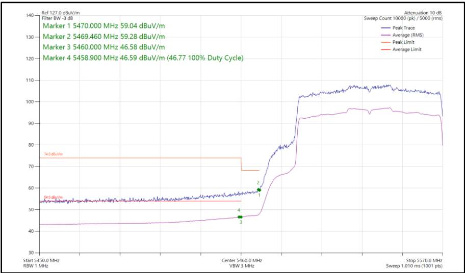
Figure 429 - 802.11ax HE80, SU, SISO, Core 1 - 5530 MHz Band Edge Frequency 5470 MHz
