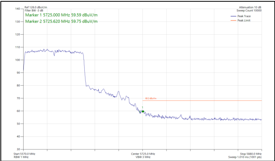
Figure 419 - 802.11ac VHT80, SISO, Core 0 - 5610 MHz Band Edge Frequency 5725 MHz
