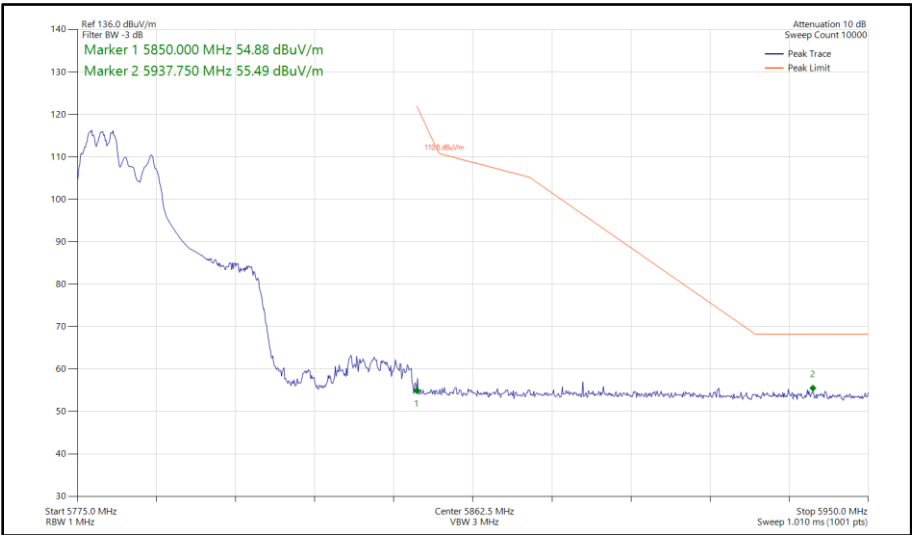
Figure 390 - 802.11ax HE40, RU 106-53, CDD, Core 0-1 - 5795 MHz Band Edge Frequency 5850 MHz
