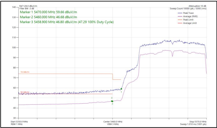
Figure 428 - 802.11ac VHT80, SISO, Core 1 - 5530 MHz Band Edge Frequency 5470 MHz
