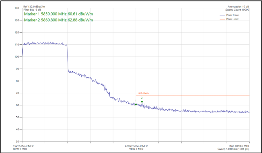
Figure 424 - 802.11ax HE80, SU, SISO, Core 0 - 5690 MHz Band Edge Frequency 5850 MHz
