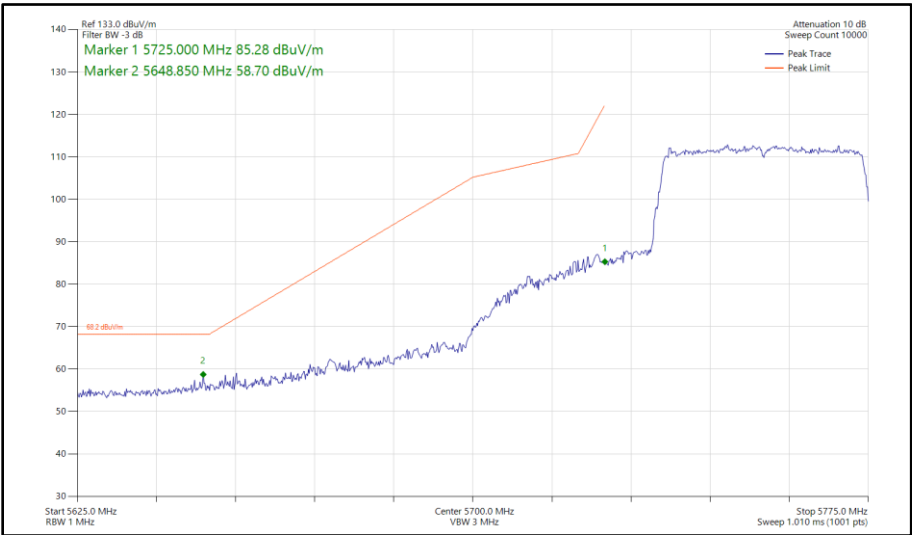
Figure 365 - 802.11ax HE40, SU, SISO, Core 1 - 5755 MHz Band Edge Frequency 5725 MHz
