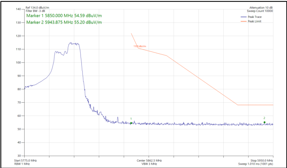
Figure 360 - 802.11ax HE40, RU 106-56, SISO, Core 0 - 5795 MHz Band Edge Frequency 5850 MHz
