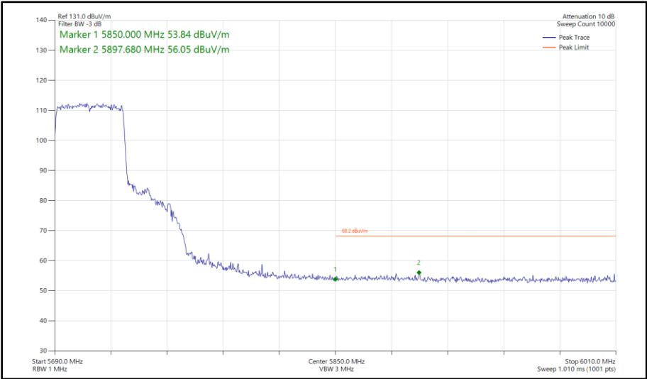
Figure 404 - 802.11ax HE40, SU, SDM, Core 0-1 - 5710 MHz Band Edge Frequency 5850 MHz
