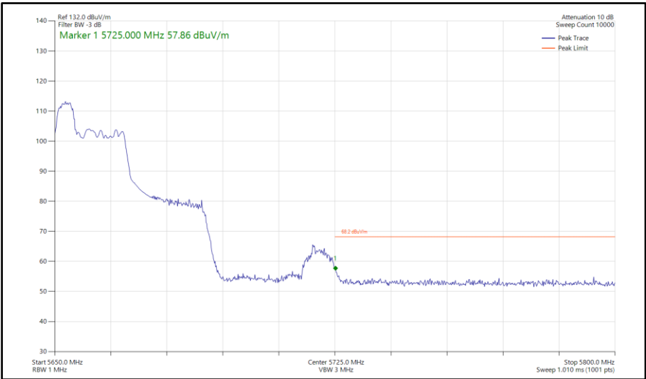
Figure 384 - 802.11ax HE40, RU 52-37, CDD, Core 0-1 - 5670 MHz Band Edge Frequency 5725 MHz
