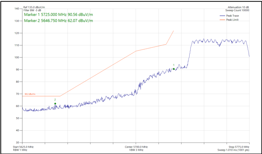
Figure 379 - 802.11n HT40, CDD, Core 0-1 - 5755 MHz Band Edge Frequency 5725 MHz
