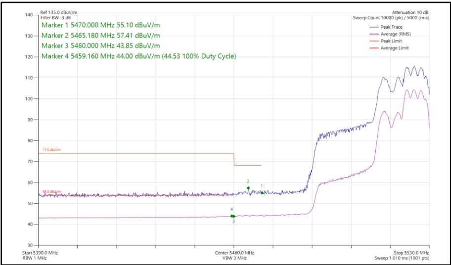
Figure 394 - 802.11ax HE40, RU 106-56, SDM, Core 0-1 - 5510 MHz Band Edge Frequency 5470 MHz
