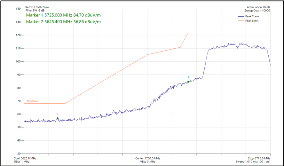
Figure 364 - 802.11n HT40, SISO, Core 1 - 5755 MHz Band Edge Frequency 5725 MHz
