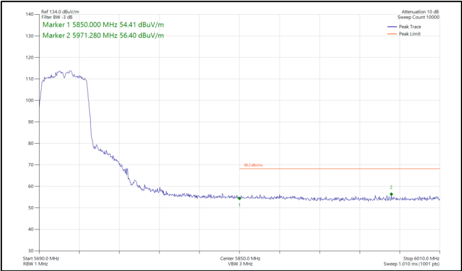
Figure 402 - 802.11n HT40, SDM, Core 0-1 - 5710 MHz Band Edge Frequency 5850 MHz
