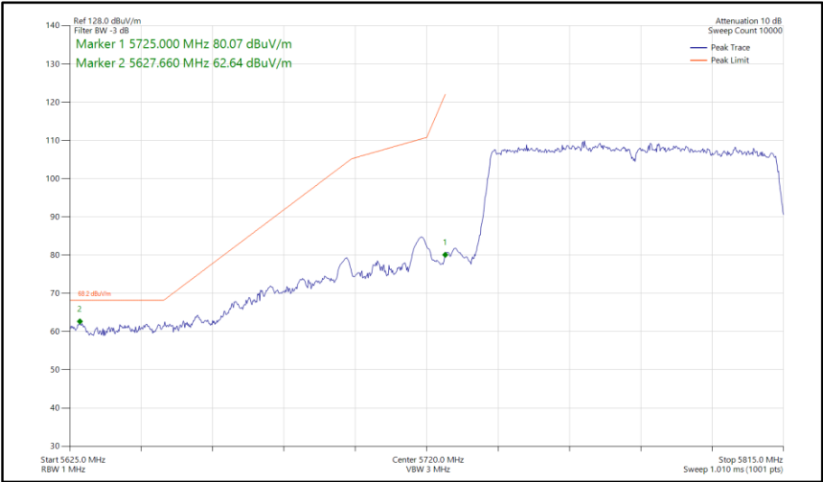
Figure 416 - 802.11ac VHT80, SISO, Core 0 - 5775 MHz Band Edge Frequency 5725 MHz
