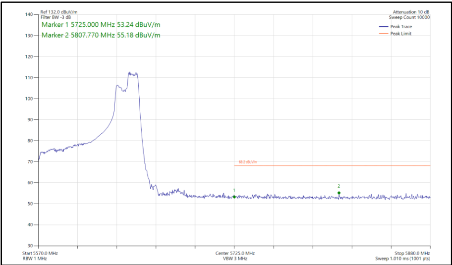
Figure 436 - 802.11ax HE80, RU 106-60, SISO, Core 1 - 5610 MHz Band Edge Frequency 5725 MHz
