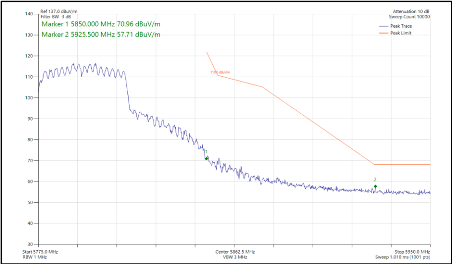
Figure 389 - 802.11ax HE40, SU, CDD, Core 0-1 - 5795 MHz Band Edge Frequency 5850 MHz
