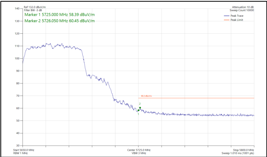
Figure 382 - 802.11n HT40, CDD, Core 0-1 - 5670 MHz Band Edge Frequency 5725 MHz
