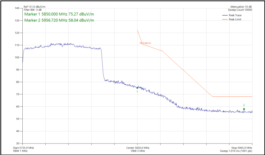
Figure 426 - 802.11ax HE80, SU, SISO, Core 0 - 5775 MHz Band Edge Frequency 5850 MHz
