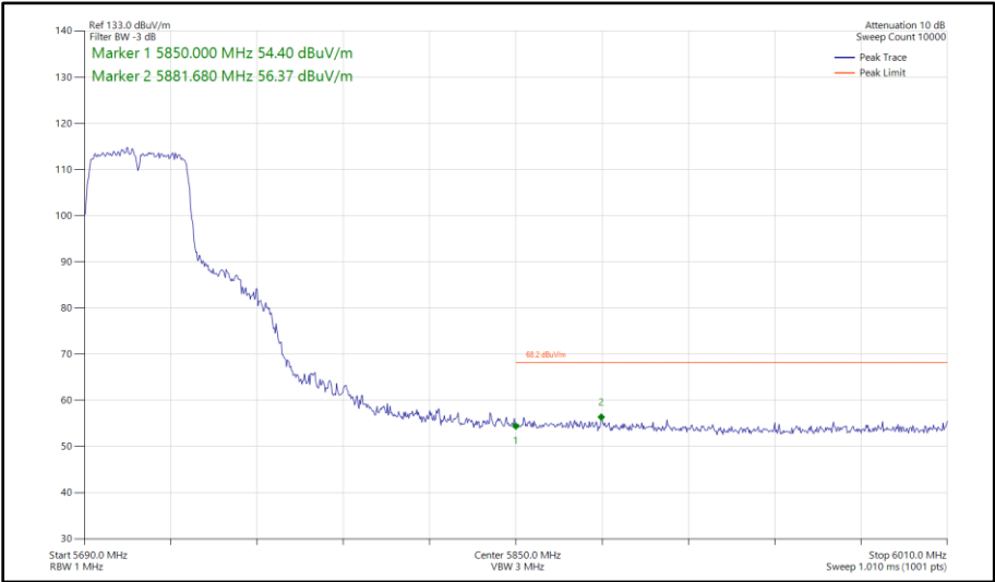
Figure 355 - 802.11n HT40, SISO, Core 0 - 5710 MHz Band Edge Frequency 5850 MHz
