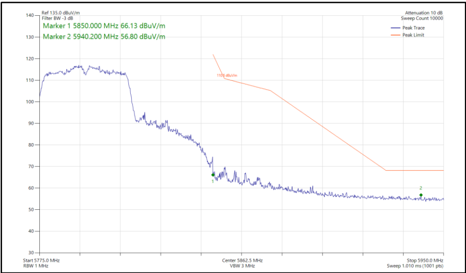
Figure 412 - 802.11ac VHT40, TxBF, Core 0-1 - 5795 MHz Band Edge Frequency 5850 MHz
