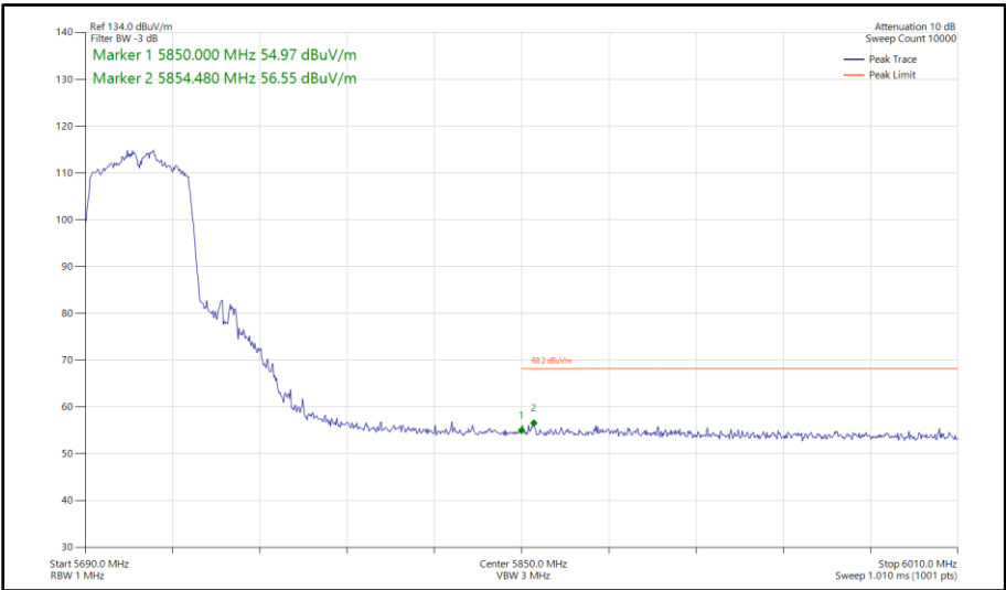
Figure 411 - 802.11ac VHT40, TxBF, Core 0-1 - 5710 MHz Band Edge Frequency 5850 MHz
