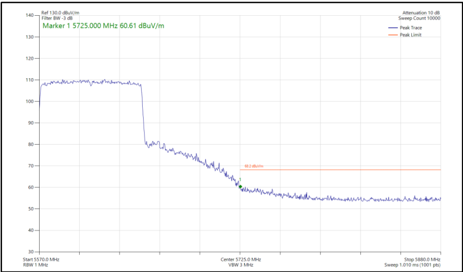
Figure 435 - 802.11ax HE80, SU, SISO, Core 1 - 5610 MHz Band Edge Frequency 5725 MHz
