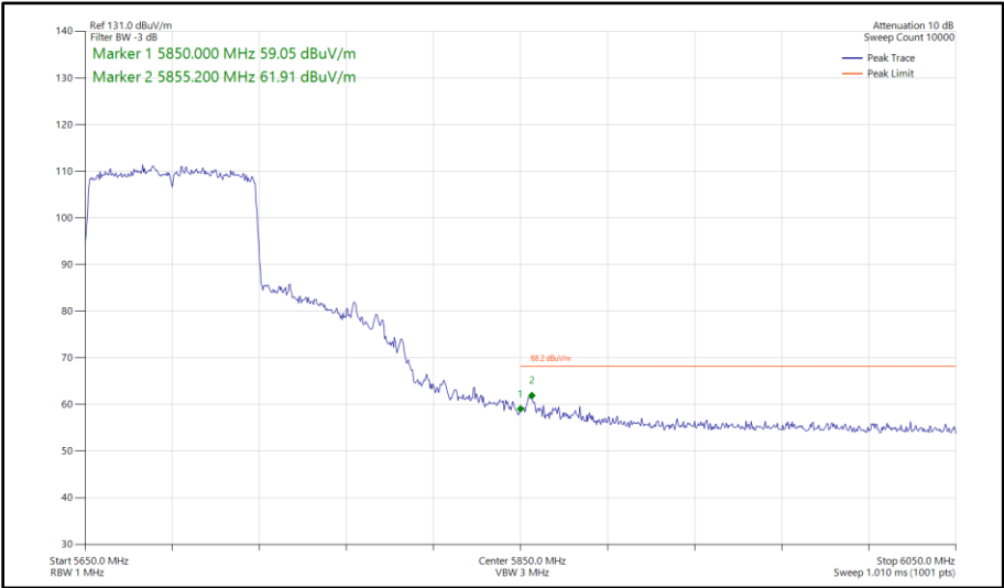
Figure 422 - 802.11ac VHT80, SISO, Core 0 - 5690 MHz Band Edge Frequency 5850 MHz
