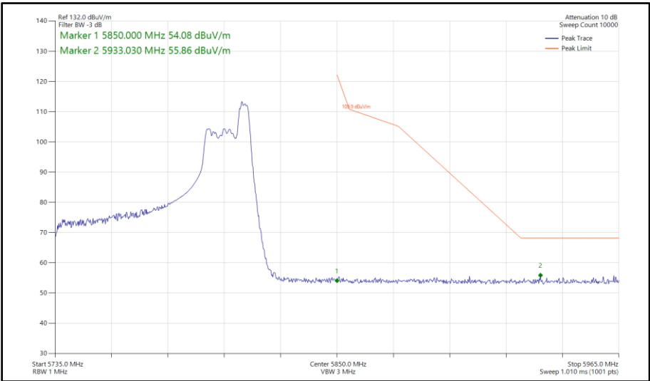
Figure 427 - 802.11ax HE80, RU 52-52, SISO, Core 0 - 5775 MHz Band Edge Frequency 5850 MHz
