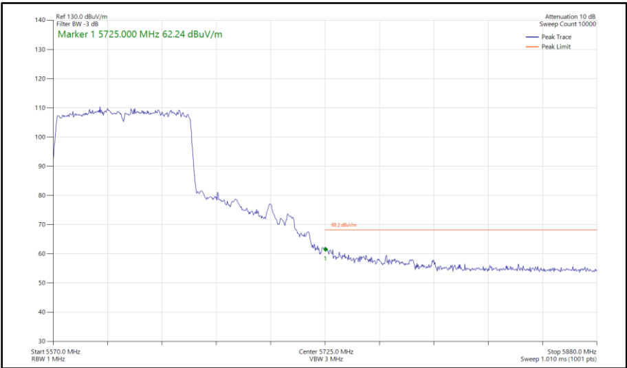
Figure 434 - 802.11ac VHT80, SISO, Core 1 - 5610 MHz Band Edge Frequency 5725 MHz
