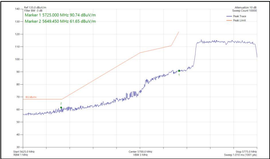
Figure 396 - 802.11ax HE40, SU, SDM, Core 0-1 - 5755 MHz Band Edge Frequency 5725 MHz
