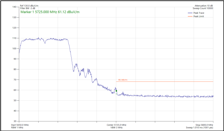
Figure 410 - 802.11ac VHT40, TxBF, Core 0-1 - 5670 MHz Band Edge Frequency 5725 MHz
