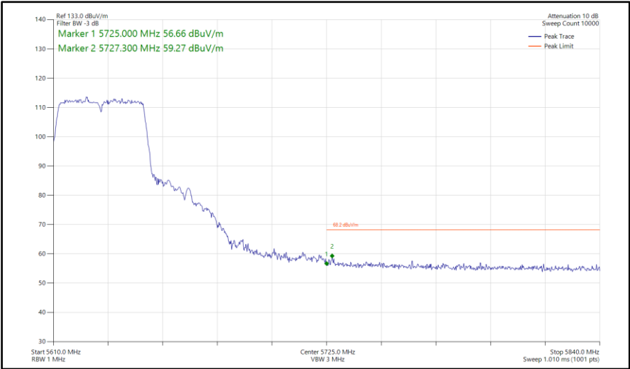
Figure 398 - 802.11n HT40, SDM, Core 0-1 - 5630 MHz Band Edge Frequency 5725 MHz
