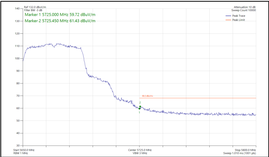
Figure 399 - 802.11n HT40, SDM, Core 0-1 - 5670 MHz Band Edge Frequency 5725 MHz
