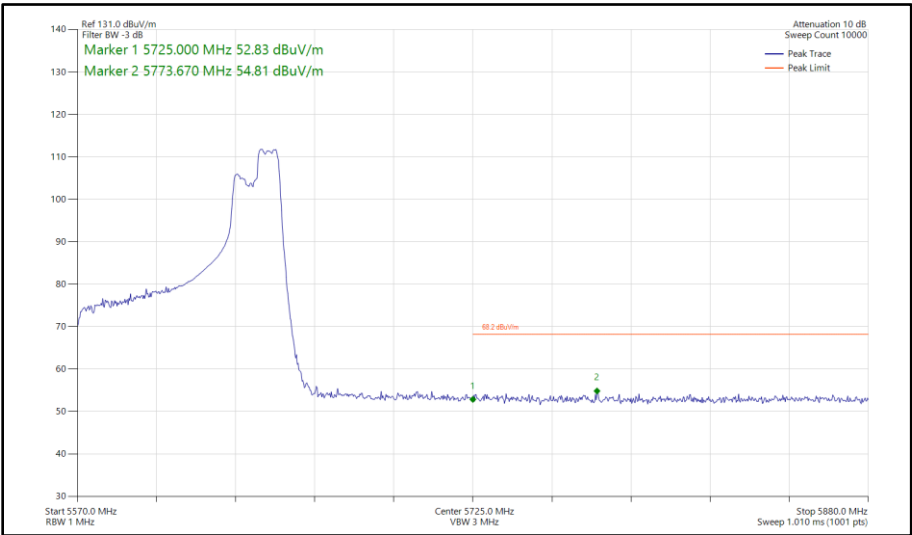
Figure 421 - 802.11ax HE80, RU 106-60, SISO, Core 0 - 5610 MHz Band Edge Frequency 5725 MHz
