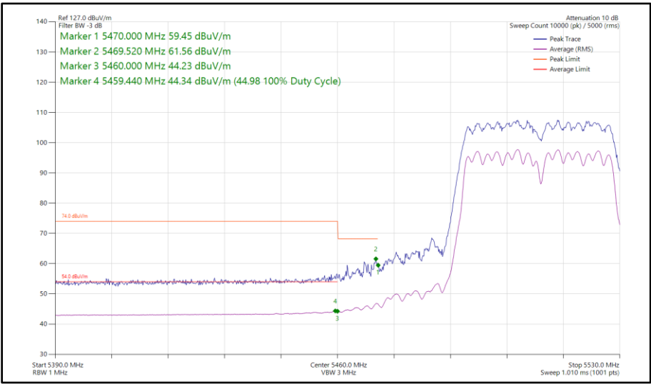
Figure 376 - 802.11n HT40, CDD, Core 0-1 - 5510 MHz Band Edge Frequency 5470 MHz
