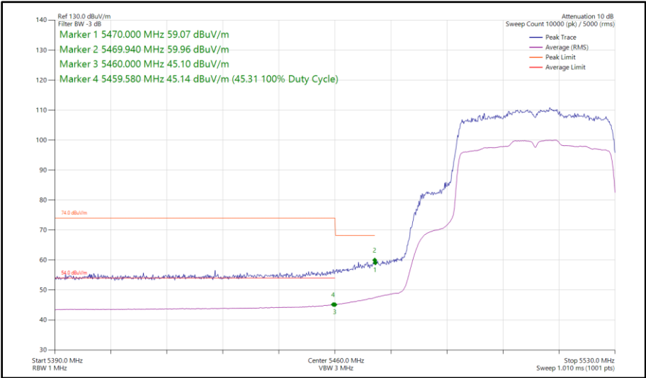
Figure 362 - 802.11ax HE40, SU, SISO, Core 1 - 5510 MHz Band Edge Frequency 5470 MHz
