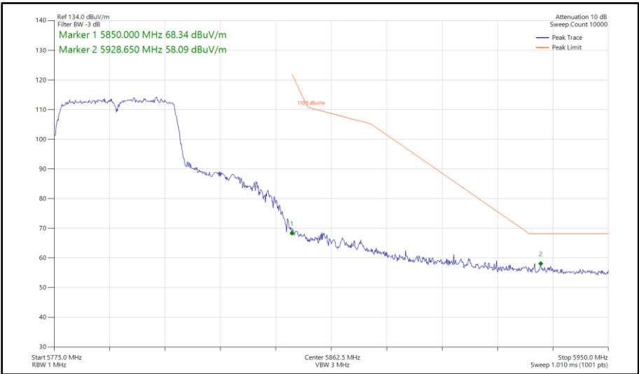
Figure 371 - 802.11n HT40, SISO, Core 1 - 5795 MHz Band Edge Frequency 5850 MHz
