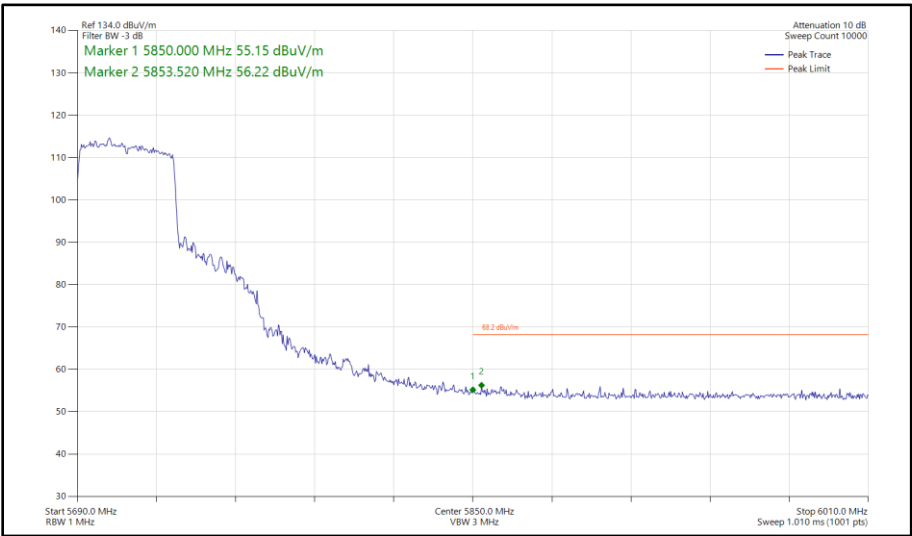
Figure 357 - 802.11ax HE40, SU, SISO, Core 0 - 5710 MHz Band Edge Frequency 5850 MHz
