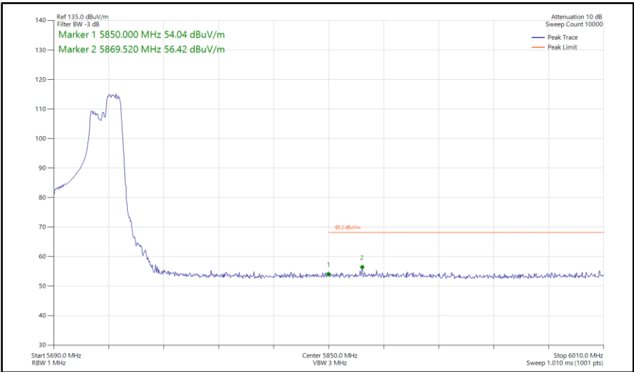
Figure 358 - 802.11ax HE40, RU 106-56, SISO, Core 0 - 5710 MHz Band Edge Frequency 5850 MHz
