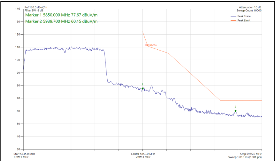
Figure 423 - 802.11ac VHT80, SISO, Core 0 - 5775 MHz Band Edge Frequency 5850 MHz
