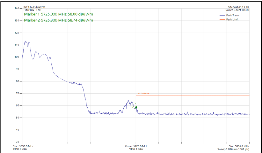
Figure 401 - 802.11ax HE40, RU 52-37, SDM, Core 0-1 - 5670 MHz Band Edge Frequency 5725 MHz
