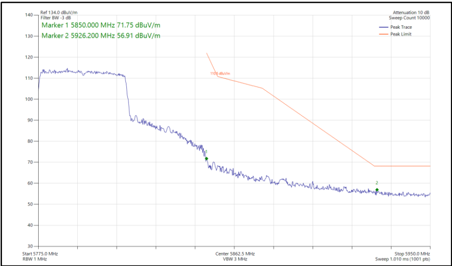
Figure 359 - 802.11ax HE40, SU, SISO, Core 0 - 5795 MHz Band Edge Frequency 5850 MHz
