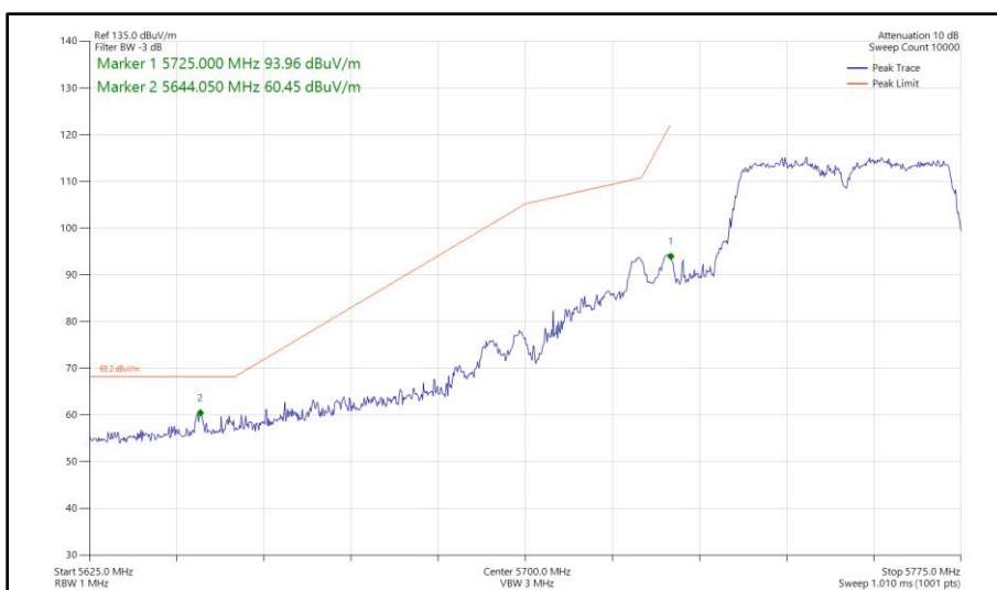
Figure 409 - 802.11ac VHT40, TxBF, Core 0-1 - 5755 MHz Band Edge Frequency 5725 MHz
