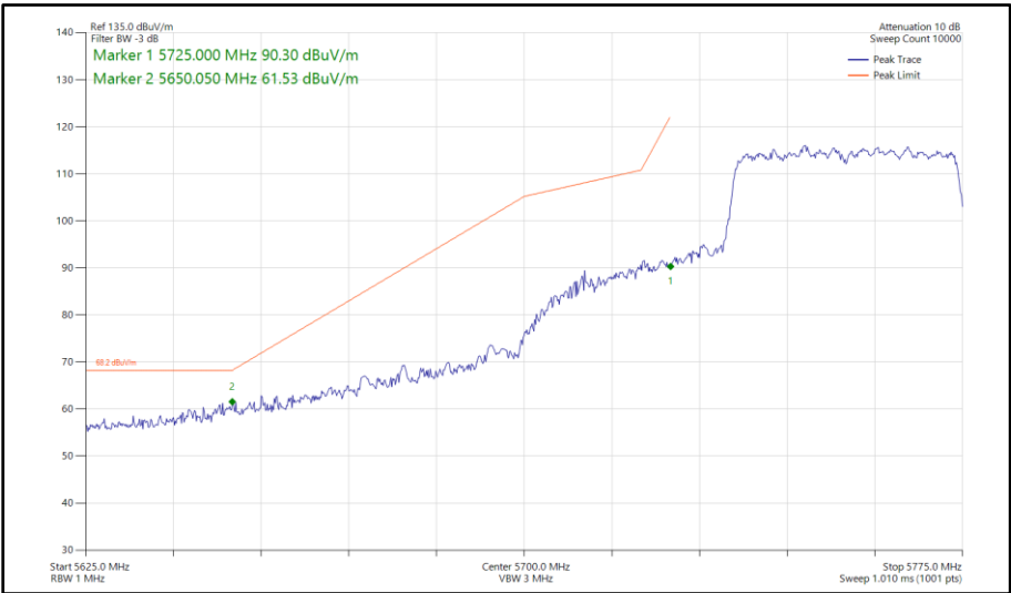
Figure 380 - 802.11ax HE40, SU, CDD, Core 0-1 - 5755 MHz Band Edge Frequency 5725 MHz
