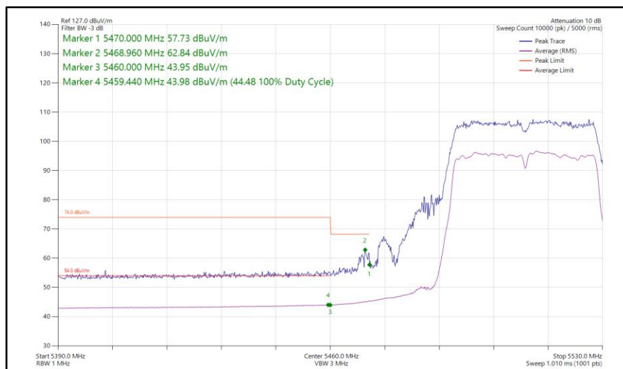
Figure 408 - 802.11ac VHT40, TxBF, Core 0-1 - 5510 MHz Band Edge Frequency 5470 MHz
