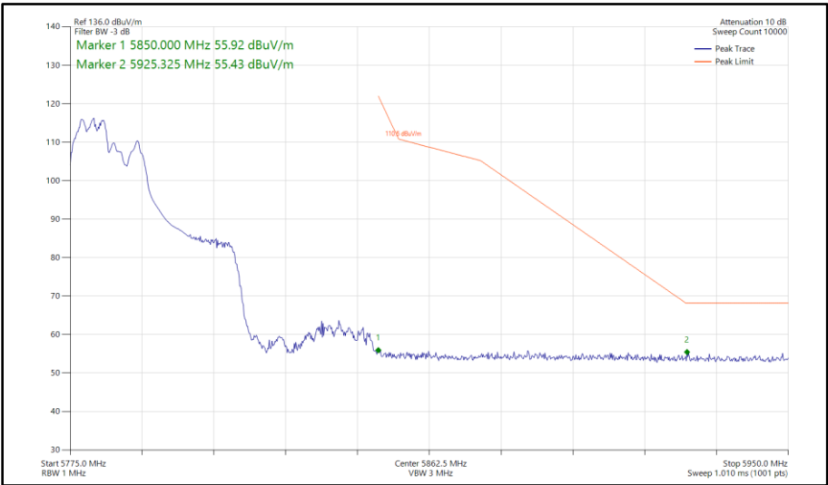
Figure 407 - 802.11ax HE40, RU 106-53, SDM, Core 0-1 - 5795 MHz Band Edge Frequency 5850 MHz
