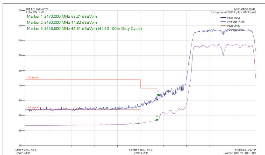
Figure 391 - 802.11n HT40, SDM, Core 0-1 - 5510 MHz Band Edge Frequency 5470 MHz
