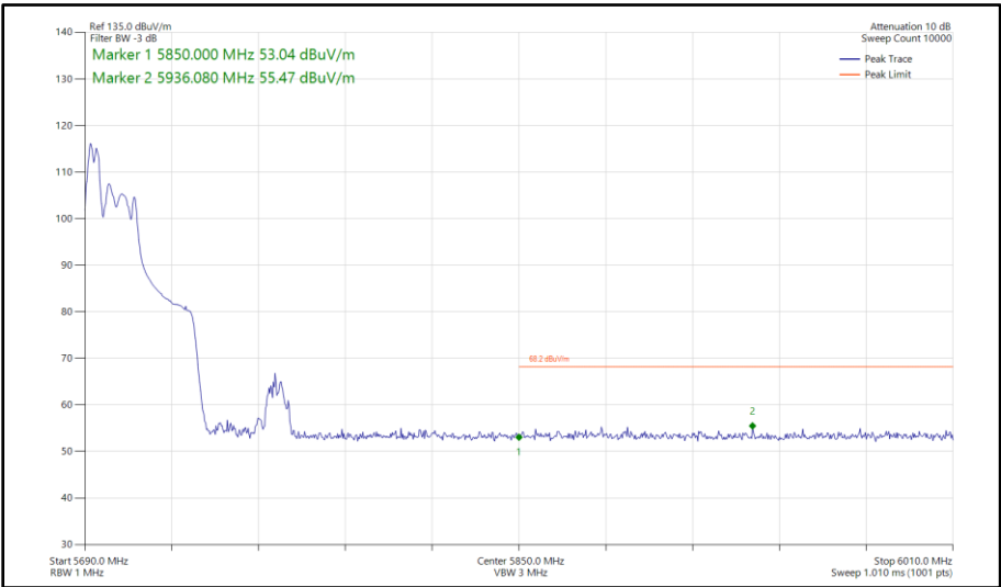
Figure 388 - 802.11ax HE40, RU 52-37, CDD, Core 0-1 - 5710 MHz Band Edge Frequency 5850 MHz
