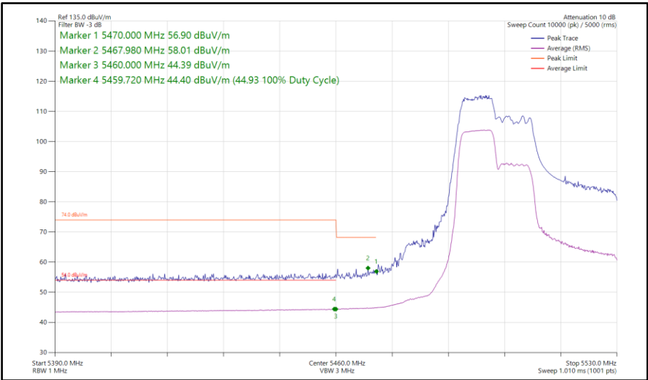
Figure 363 - 802.11ax HE40, RU 106-53, SISO, Core 1 - 5510 MHz Band Edge Frequency 5470 MHz
