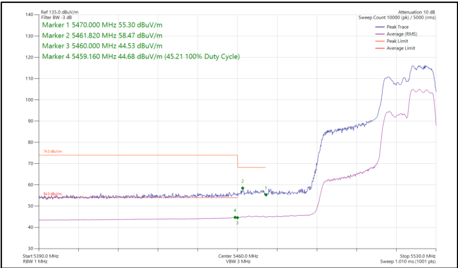
Figure 378 - 802.11ax HE40, RU 106-56, CDD, Core 0-1 - 5510 MHz Band Edge Frequency 5470 MHz
