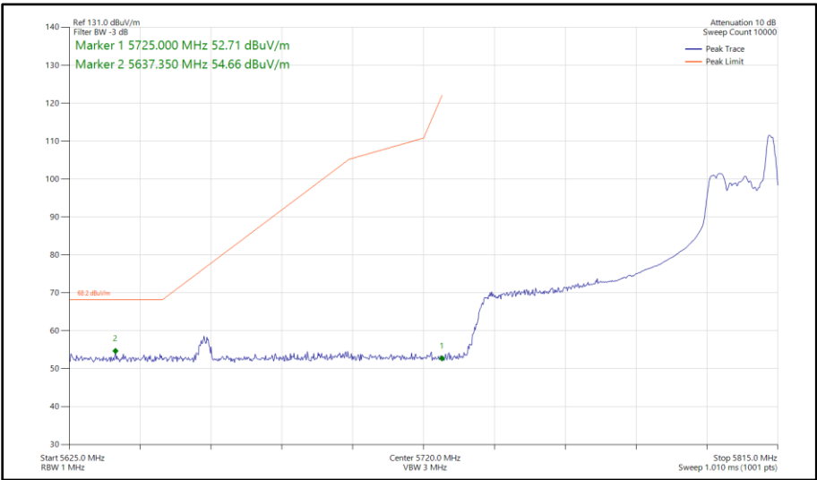
Figure 433 - 802.11ax HE80, RU 26-36, SISO, Core 1 - 5775 MHz Band Edge Frequency 5725 MHz
