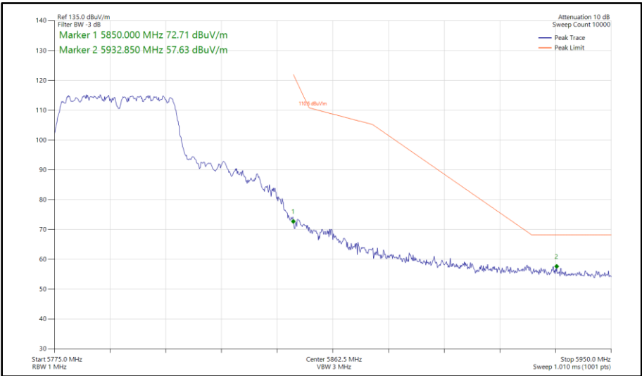
Figure 386 - 802.11n HT40, CDD, Core 0-1 - 5795 MHz Band Edge Frequency 5850 MHz
