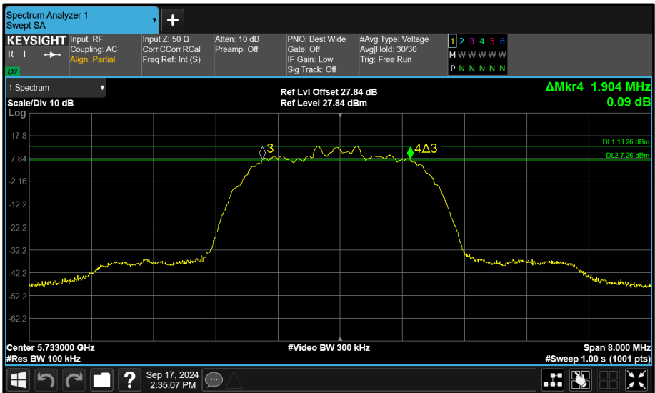
Figure 167 - Core 0 (A) 5733 MHz (CH8) 6 dB Bandwidth
