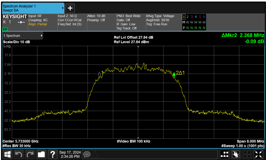
Figure 166 - Core 0 (A) 5733 MHz (CH8) 99% Bandwidth
