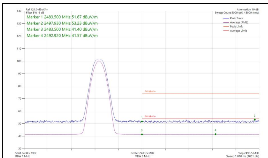
Figure 7 - Bluetooth LE1M, SISO, Core 0 - 2478 MHz Band Edge Frequency 2483.5 MHz
