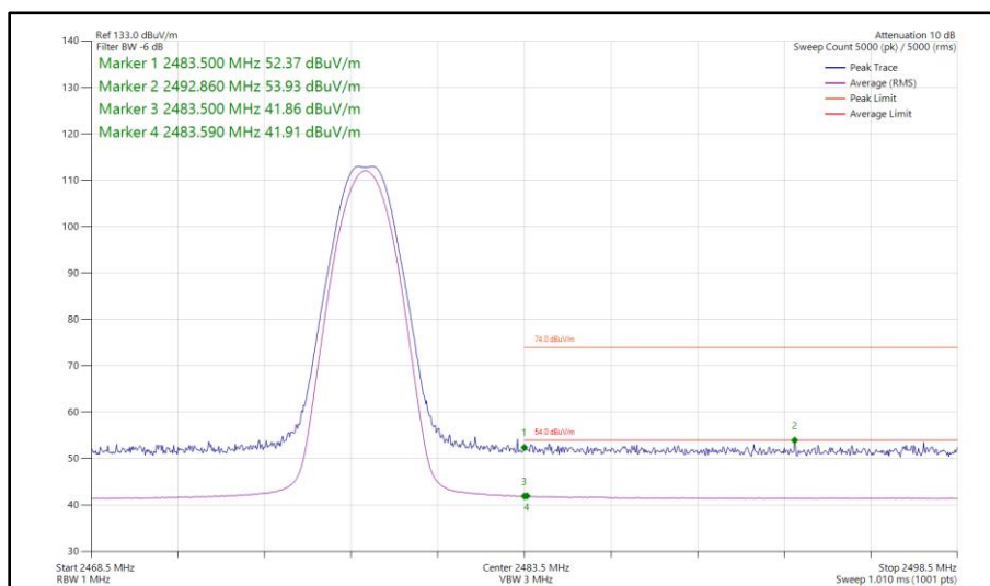
Figure 37 - Bluetooth LE1M, MIMO, Core 0-1 - 2478 MHz Band Edge Frequency 2483.5 MHz
