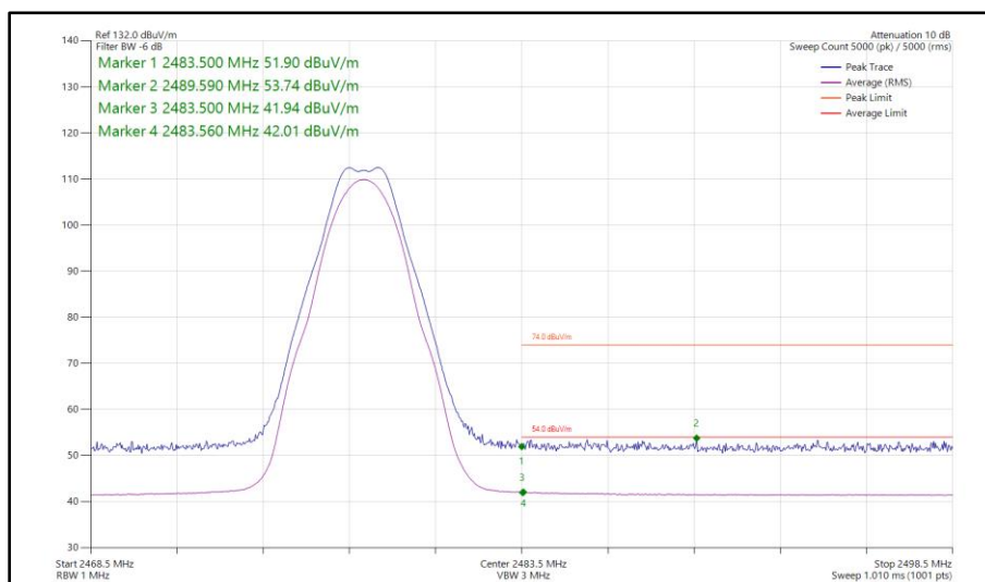
Figure 39 - Bluetooth LE2M, MIMO, Core 0-1 - 2478 MHz Band Edge Frequency 2483.5 MHz
