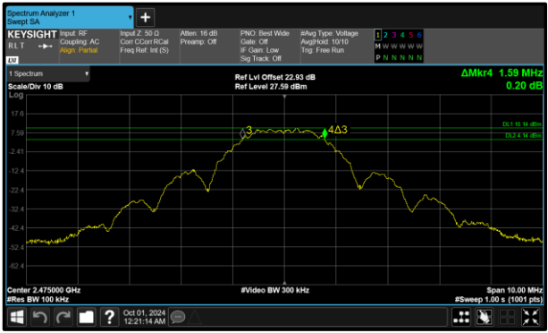
Figure 28 - Core 2 (C) 2475 MHz (CH25) 6 dB Bandwidth
