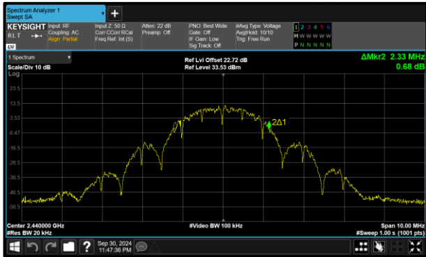
Figure 37 - Core 1 (B) 2440 MHz (CH18) 99% Bandwidth
