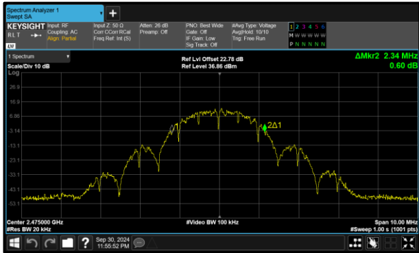
Figure 39 - Core 1 (B) 2475 MHz (CH25) 99% Bandwidth
