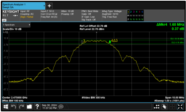
Figure 22 - Core 1 (B) 2475 MHz (CH25) 6 dB Bandwidth
