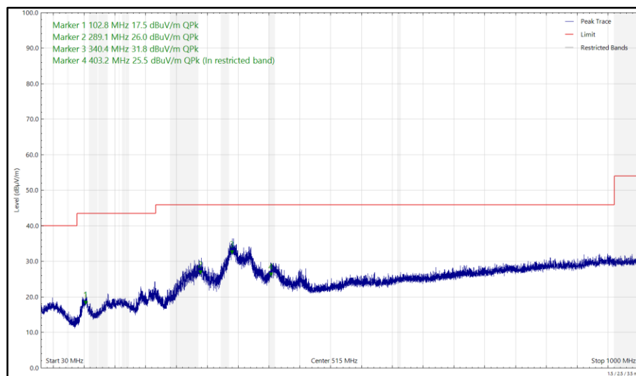
Figure 708 - U-NII-1 - 5180 MHz (CH36), HE20, RU26-0, CDD, Core 0 + Core 1 30 MHz to 1 GHz, Horizontal (Peak)
