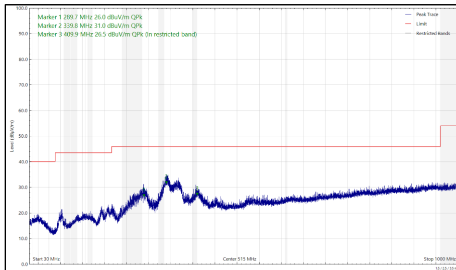
Figure 704 - U-NII-3 - 5825 MHz (CH165), HT20, CDD, Core 0 + Core 1 30 MHz to 1 GHz, Horizontal (Peak)
