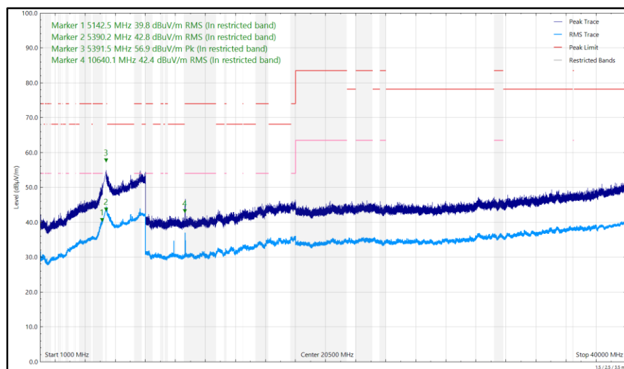
Figure 697 - U-NII-2A - 5320 MHz (CH64), HT20, CDD, Core 0 + Core 1 1 GHz to 40 GHz, Vertical
