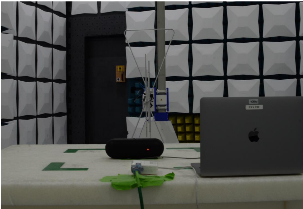
Figure 20: 30MHz-1GHz Test Setup (Rear View)
