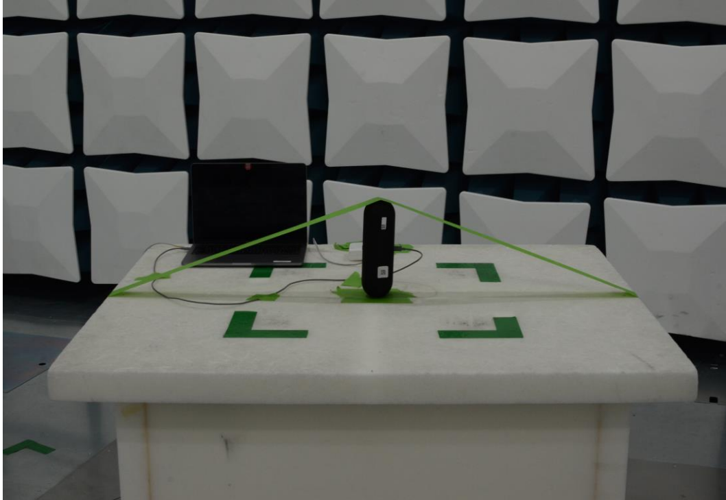
Figure 21: 30MHz-1GHz Test Setup (Front View)
