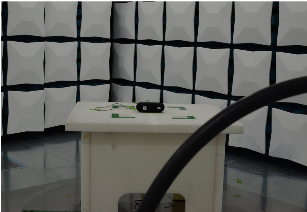
Figure 24: 9kHz-30MHz Test Setup (Front View)
