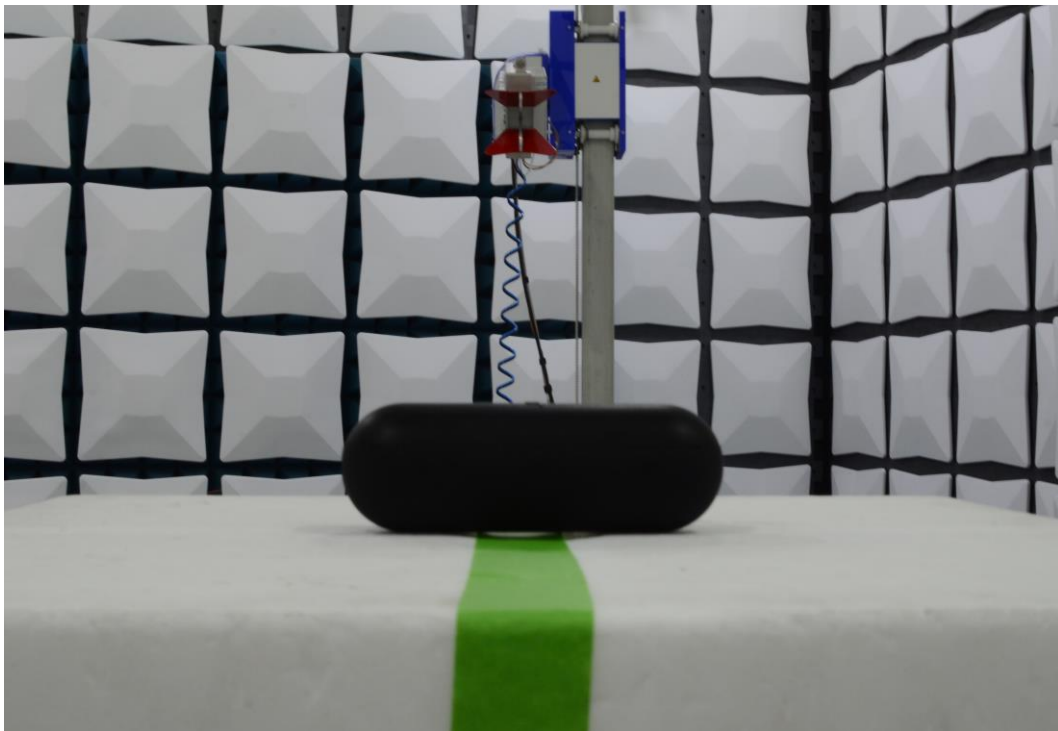
Figure 8: 1-18GHz Test Setup (Rear View)
