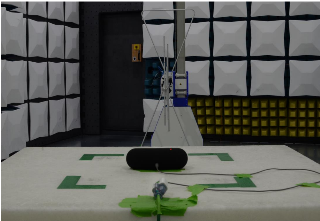
Figure 12: 30MHz-1GHz Test Setup (Rear View)
