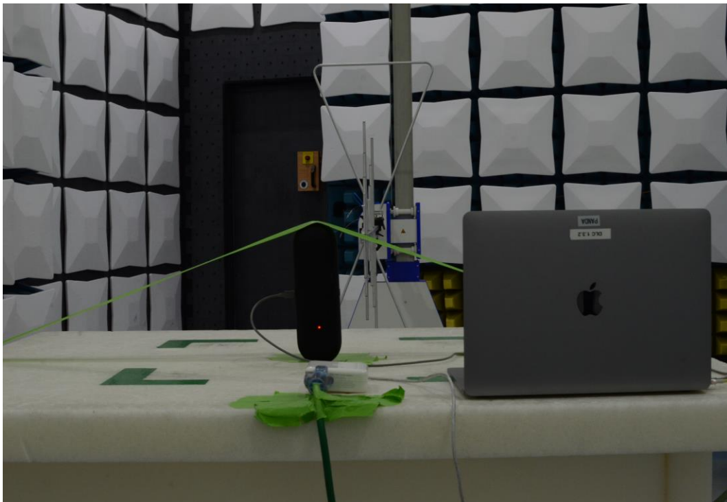
Figure 22: 30MHz-1GHz Test Setup (Rear View)
