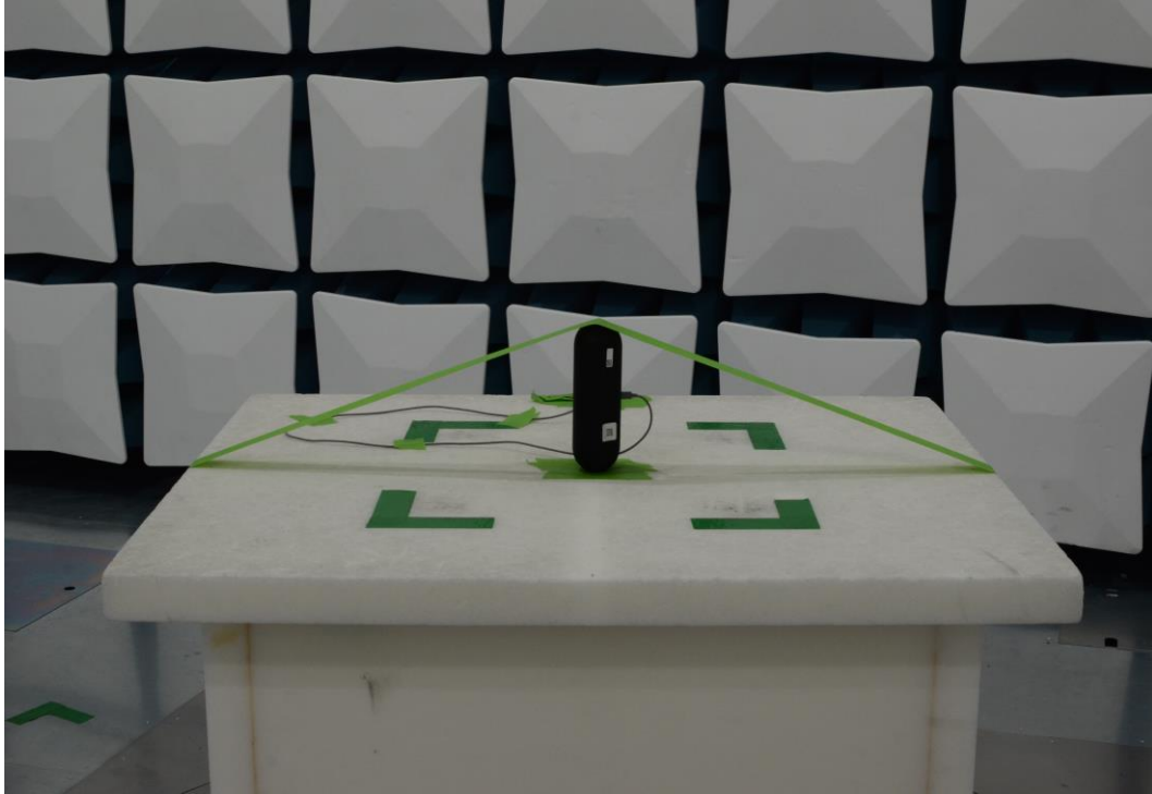
Figure 15: 30MHz-1GHz Test Setup (Front View)
