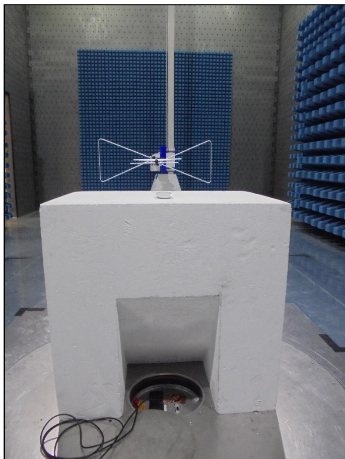
Figure 2 - Radiated Disturbance - Below 1 GHz
