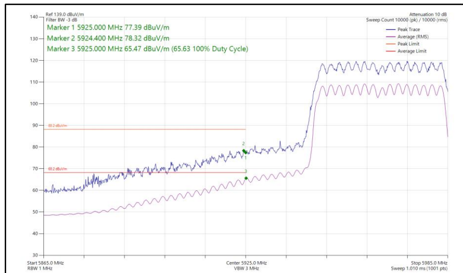
Figure 232 - 802.11ax HE40, SU, CDD, Core 0 - Core 1 - 5965 MHz Band Edge Frequency 5925 MHz
