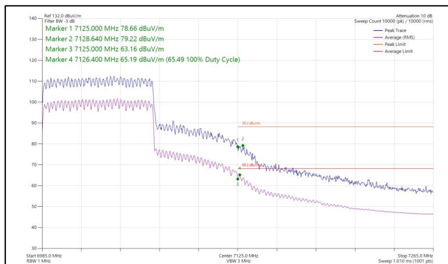
Figure 274 - 802.11ax HE80, SU, CDD, Core 0 - Core 1 - 7025 MHz Band Edge Frequency 7125 MHz
