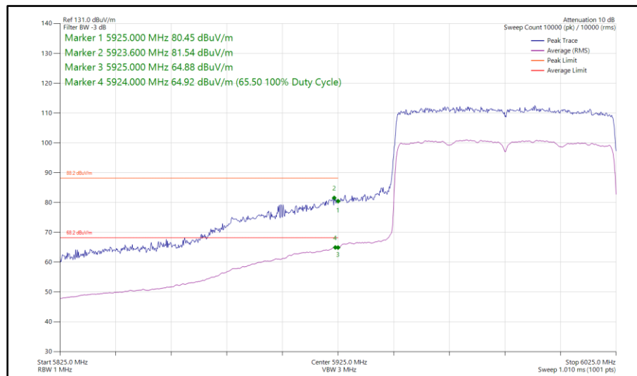
Figure 260 - 802.11ax HE80, SU, SISO, Core 1 - 5985 MHz Band Edge Frequency 5925 MHz
