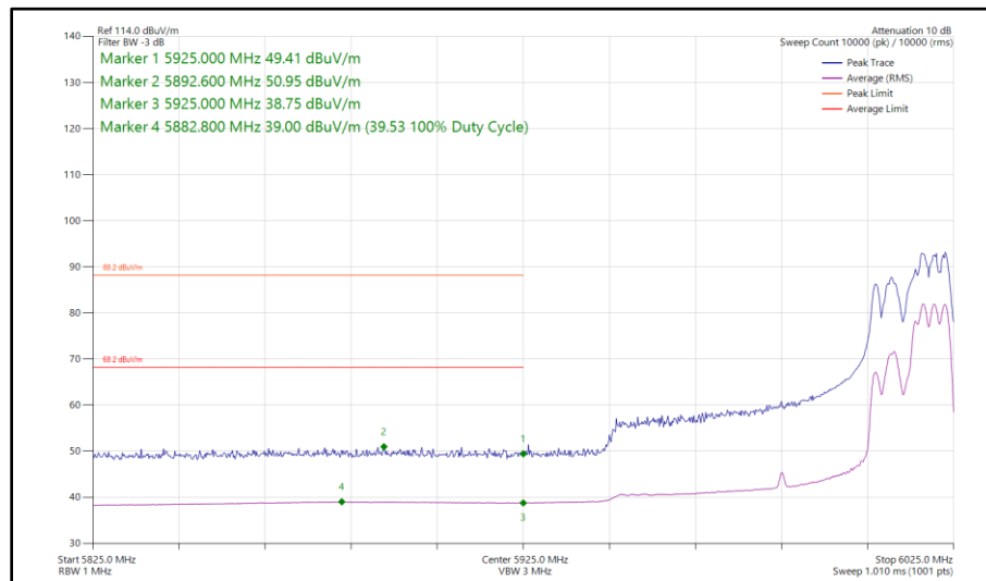
Figure 277 - 802.11ax HE80, RU 106-60, SDM, Core 0 - Core 1 - 5985 MHz Band Edge Frequency 5925 MHz
