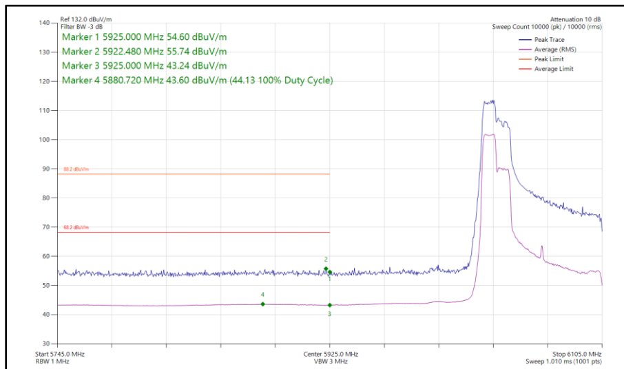
Figure 263 - 802.11ax HE80, RU 106-53, SISO, Core 1 - 6065 MHz Band Edge Frequency 5925 MHz
