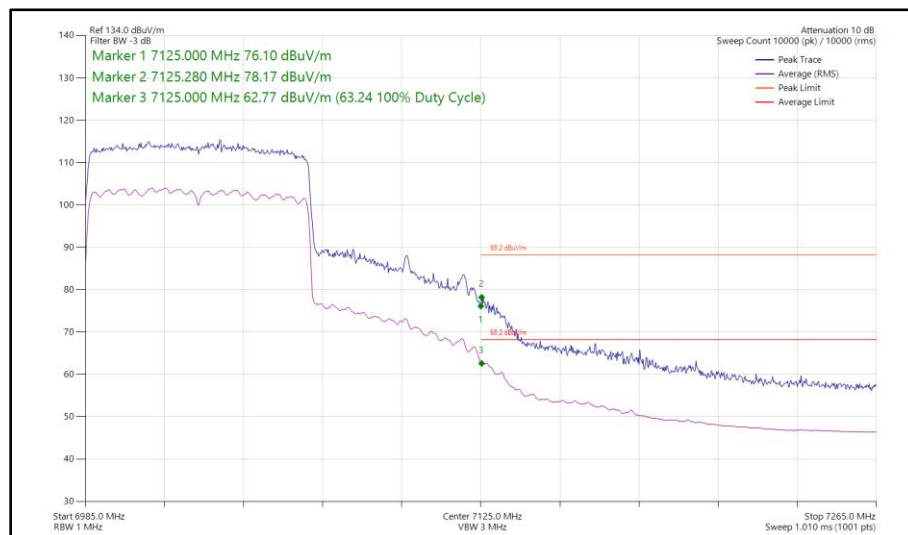
Figure 282 - 802.11ax HE80, SU, SDM, Core 0 - Core 1 - 7025 MHz Band Edge Frequency 7125 MHz
