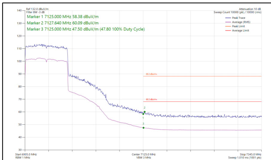
Figure 256 - 802.11ax HE80, SU, SISO, Core 0 - 6945 MHz Band Edge Frequency 7125 MHz
