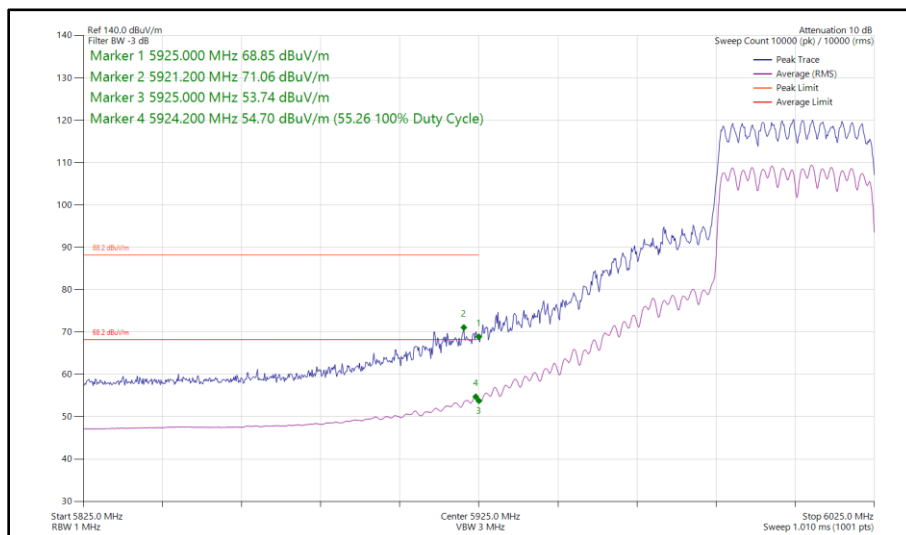
Figure 234 - 802.11ax HE40, SU, CDD, Core 0 - Core 1 - 6005 MHz Band Edge Frequency 5925 MHz
