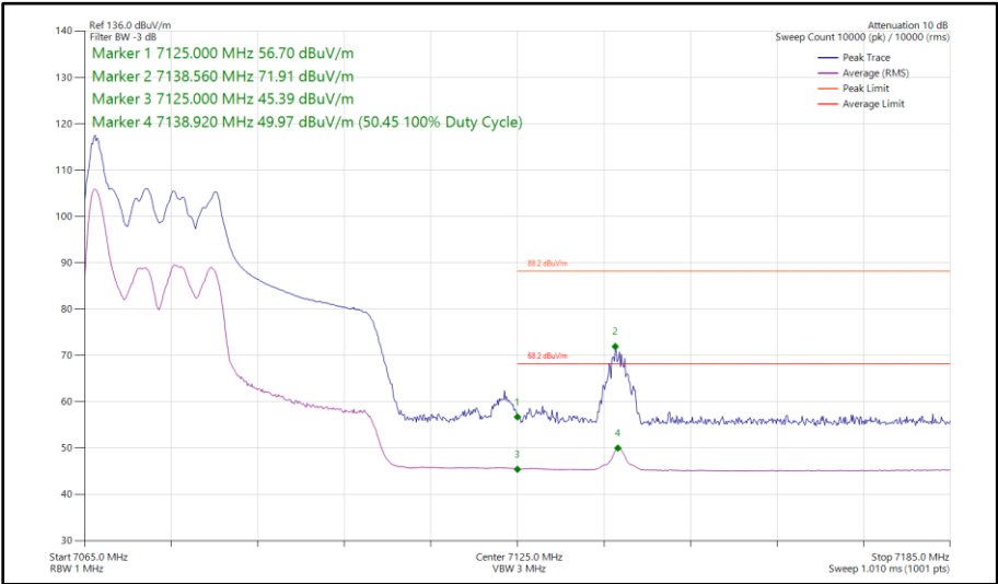
Figure 247 - 802.11ax HE40, RU 26-0, SDM, Core 0 - Core 1 - 7085 MHz Band Edge Frequency 7125 MHz
