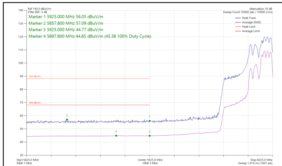
Figure 243 - 802.11ax HE40, RU 106-56, SDM, Core 0 - Core 1 - 6005 MHz Band Edge Frequency 5925 MHz
