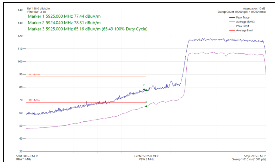
Figure 240 - 802.11ax HE40, SU, SDM, Core 0 - Core 1 - 5965 MHz Band Edge Frequency 5925 MHz
