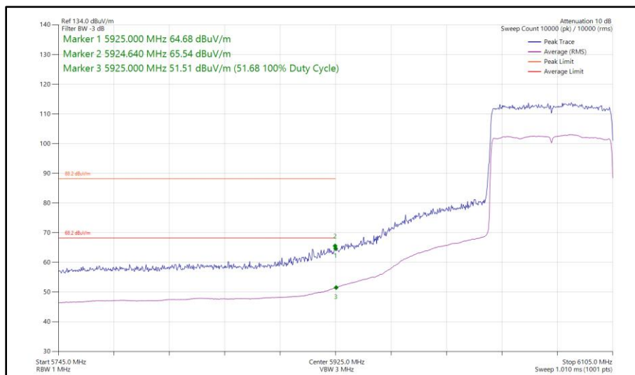
Figure 254 - 802.11ax HE80, SU, SISO, Core 0 - 6065 MHz Band Edge Frequency 5925 MHz
