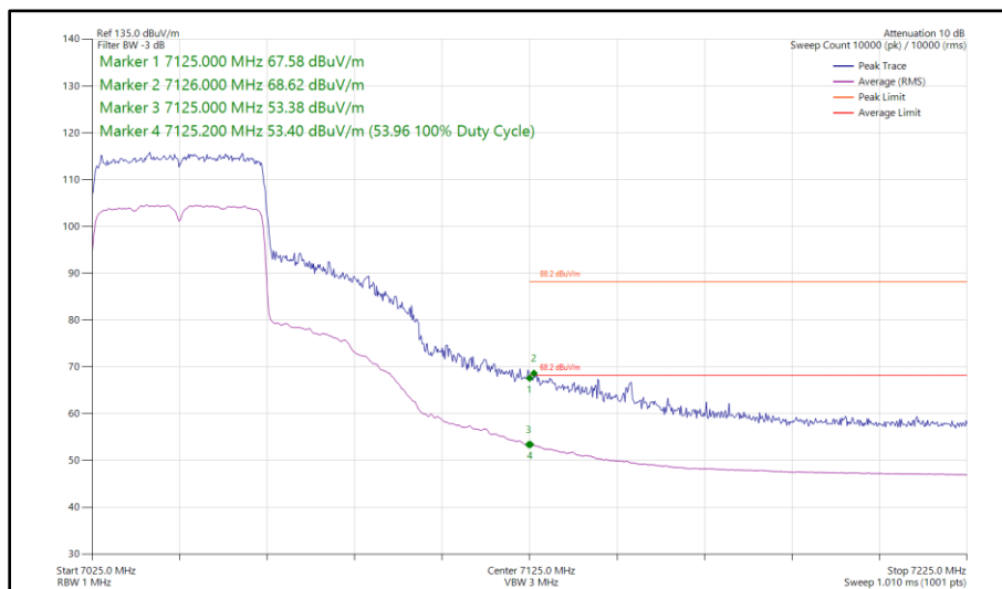
Figure 228 - 802.11ax HE40, SU, SISO, Core 1 - 7045 MHz Band Edge Frequency 7125 MHz
