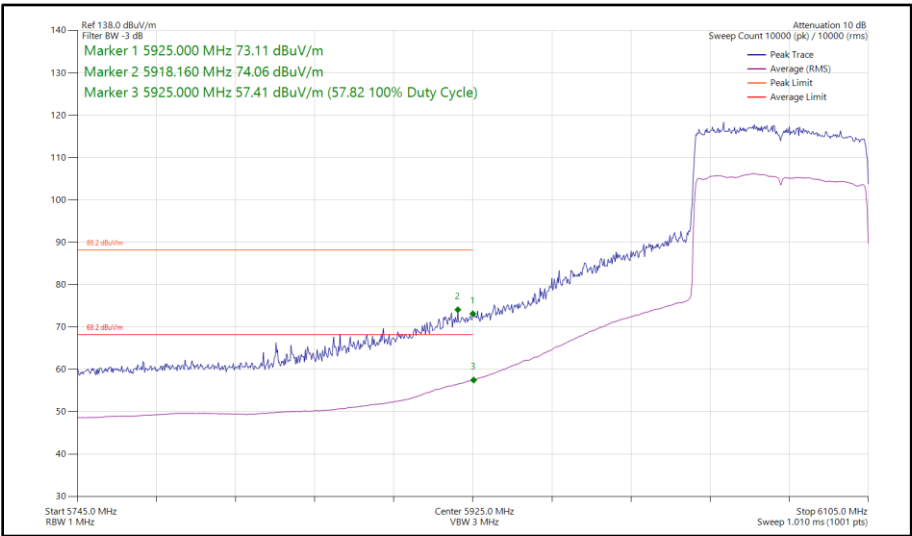
Figure 285 - 802.11ax HE80, SU, TxBF, Core 0 - Core 1 - 6065 MHz Band Edge Frequency 5925 MHz
