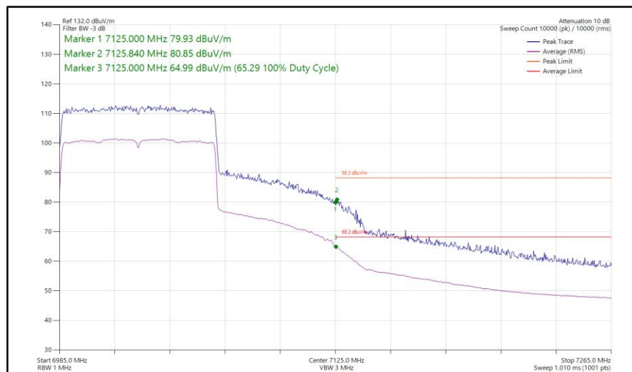
Figure 266 - 802.11ax HE80, SU, SISO, Core 1 - 7025 MHz Band Edge Frequency 7125 MHz
