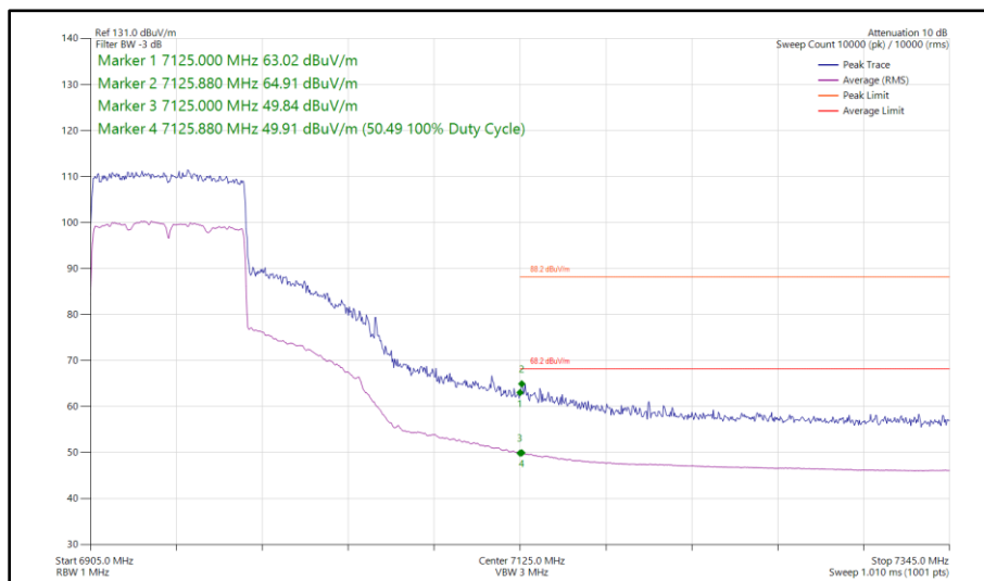
Figure 264 - 802.11ax HE80, SU, SISO, Core 1 - 6945 MHz Band Edge Frequency 7125 MHz
