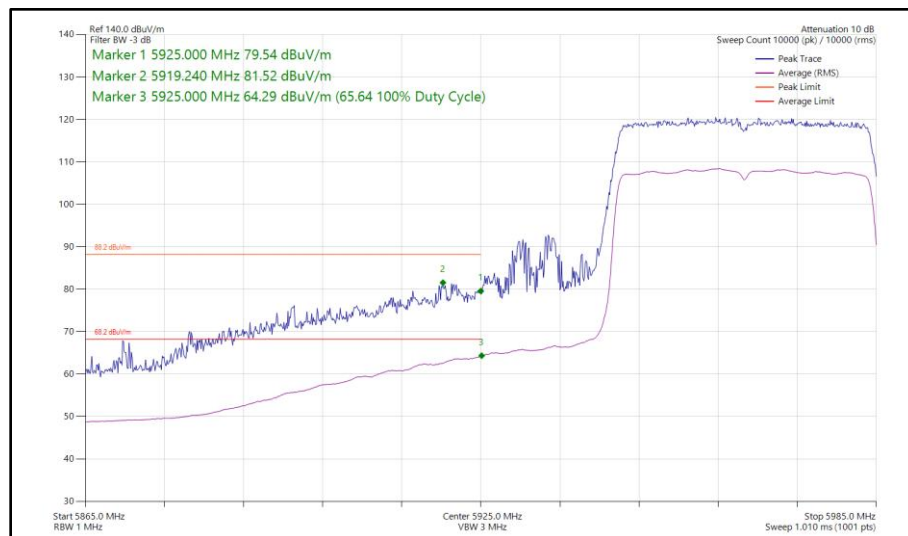
Figure 248 - 802.11ax HE40, SU, TxBF, Core 0 - Core 1 - 5965 MHz Band Edge Frequency 5925 MHz
