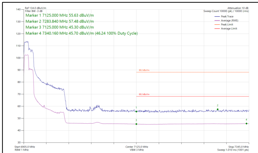
Figure 257 - 802.11ax HE80, RU 106-53, SISO, Core 0 - 6945 MHz Band Edge Frequency 7125 MHz
