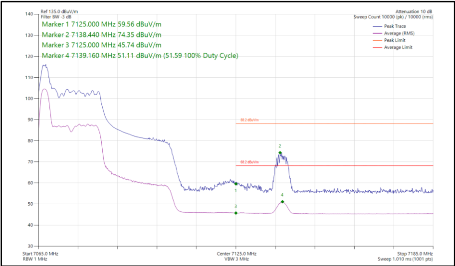
Figure 231 - 802.11ax HE40, RU 26-0, SISO, Core 1 - 7085 MHz Band Edge Frequency 7125 MHz
