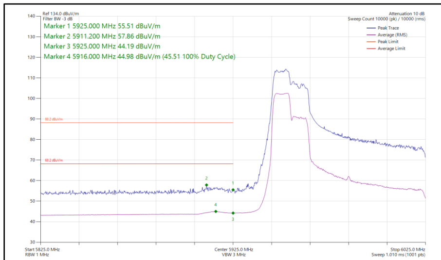
Figure 253 - 802.11ax HE80, RU 106-53, SISO, Core 0 - 5985 MHz Band Edge Frequency 5925 MHz
