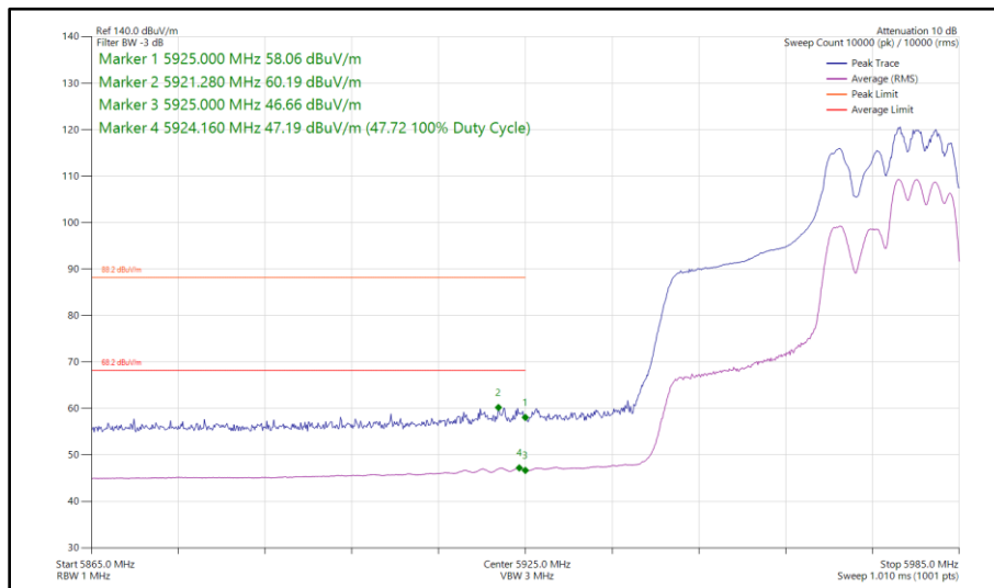
Figure 241 - 802.11ax HE40, RU 106-56, SDM, Core 0 - Core 1 - 5965 MHz Band Edge Frequency 5925 MHz
