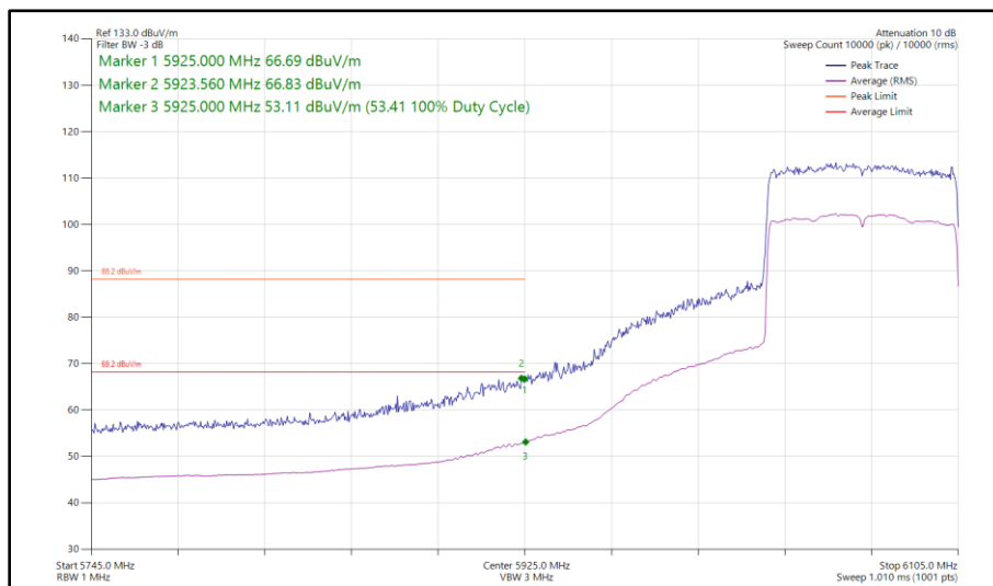
Figure 262 - 802.11ax HE80, SU, SISO, Core 1 - 6065 MHz Band Edge Frequency 5925 MHz
