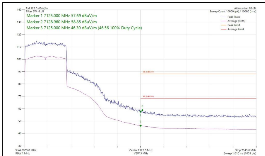
Figure 286 - 802.11ax HE80, SU, TxBF, Core 0 - Core 1 - 6945 MHz Band Edge Frequency 7125 MHz
