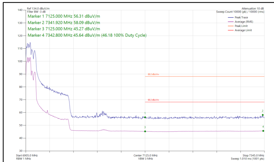
Figure 281 - 802.11ax HE80, RU 106-53, SDM, Core 0 - Core 1 - 6945 MHz Band Edge Frequency 7125 MHz
