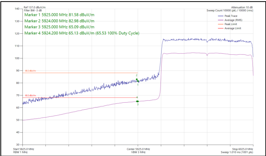
Figure 284 - 802.11ax HE80, SU, TxBF, Core 0 - Core 1 - 5985 MHz Band Edge Frequency 5925 MHz
