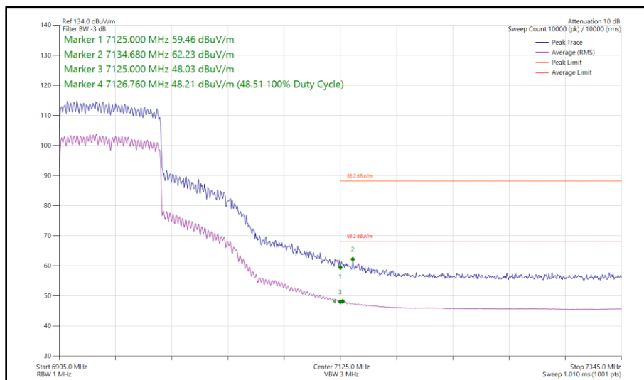
Figure 272 - 802.11ax HE80, SU, CDD, Core 0 - Core 1 - 6945 MHz Band Edge Frequency 7125 MHz
