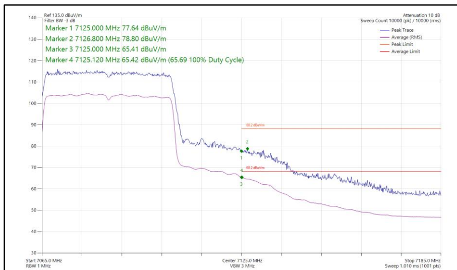
Figure 246 - 802.11ax HE40, SU, SDM, Core 0 - Core 1 - 7085 MHz Band Edge Frequency 7125 MHz
