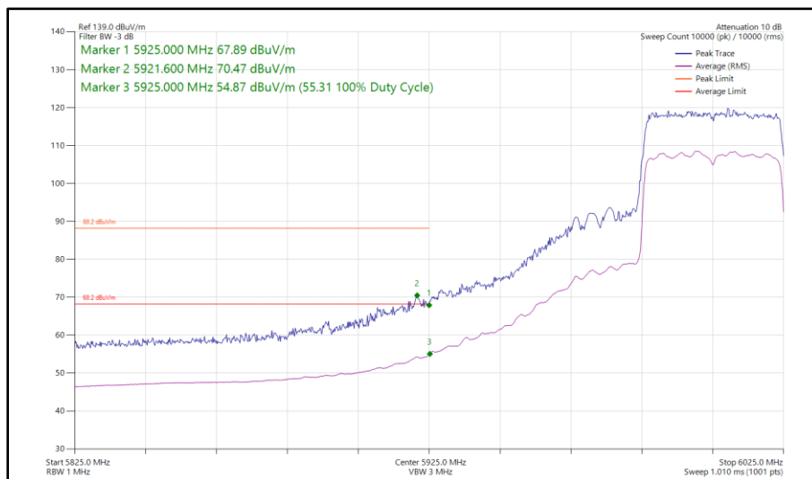
Figure 242 - 802.11ax HE40, SU, SDM, Core 0 - Core 1 - 6005 MHz Band Edge Frequency 5925 MHz
