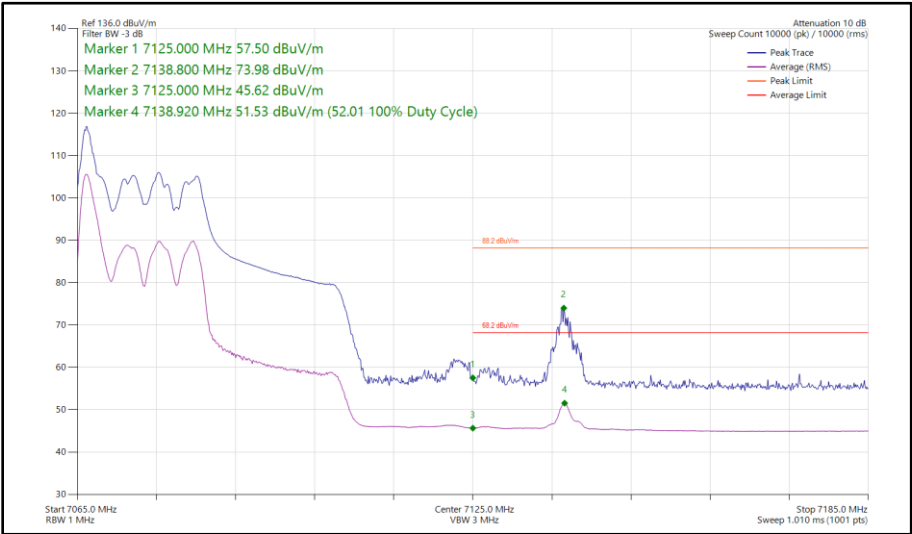
Figure 239 - 802.11ax HE40, RU 26-0, CDD, Core 0 - Core 1 - 7085 MHz Band Edge Frequency 7125 MHz
