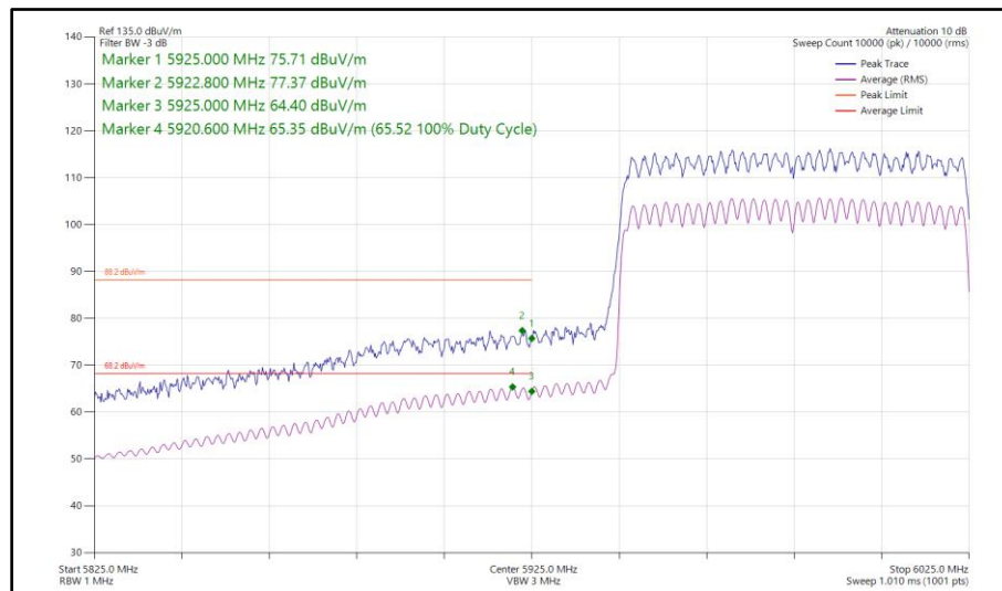
Figure 268 - 802.11ax HE80, SU, CDD, Core 0 - Core 1 - 5985 MHz Band Edge Frequency 5925 MHz
