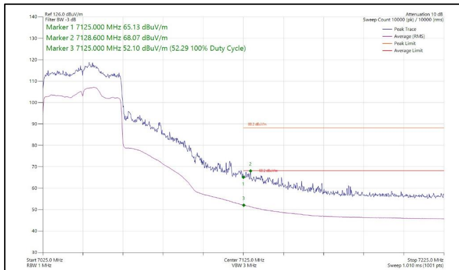
Figure 250 - 802.11ax HE40, SU, TxBF, Core 0 - Core 1 - 7045 MHz Band Edge Frequency 7125 MHz
