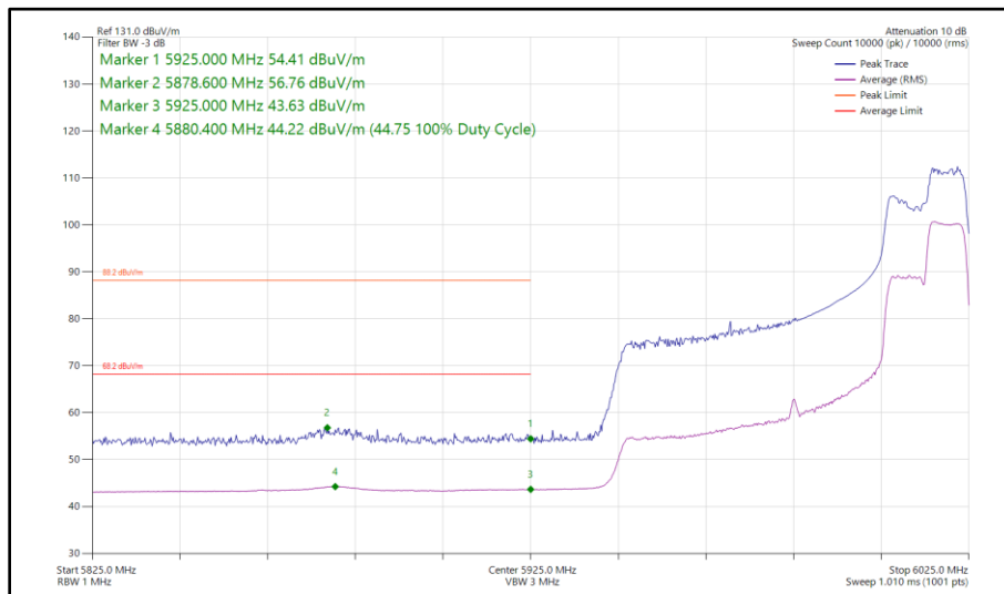
Figure 261 - 802.11ax HE80, RU 106-60, SISO, Core 1 - 5985 MHz Band Edge Frequency 5925 MHz
