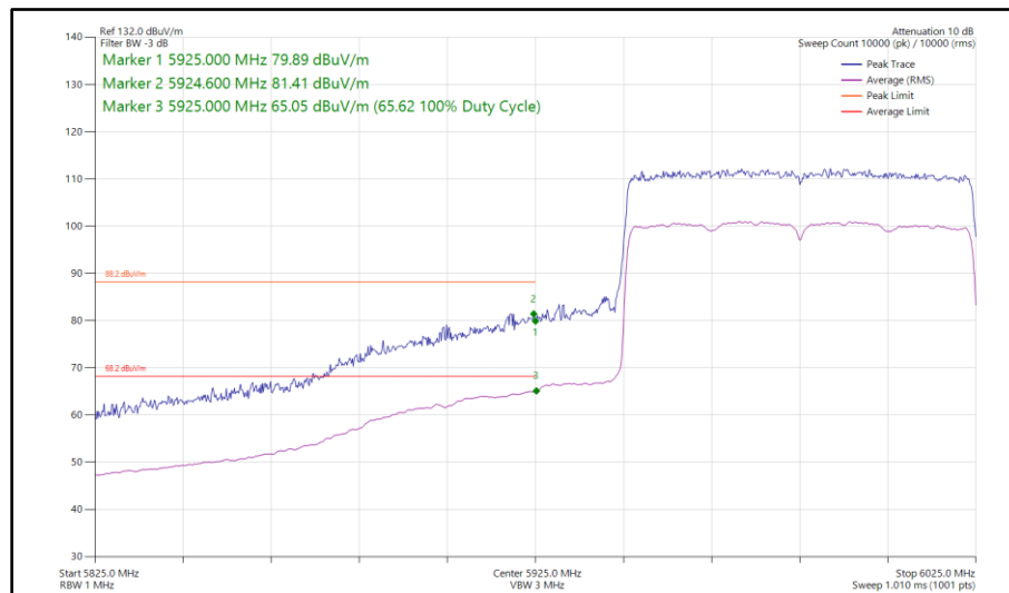
Figure 252 - 802.11ax HE80, SU, SISO, Core 0 - 5985 MHz Band Edge Frequency 5925 MHz
