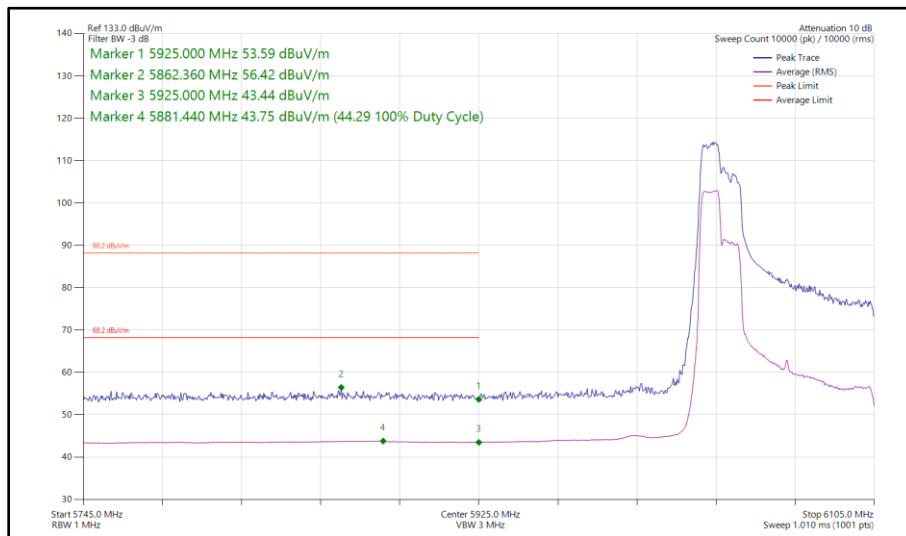
Figure 255 - 802.11ax HE80, RU 106-53, SISO, Core 0 - 6065 MHz Band Edge Frequency 5925 MHz
