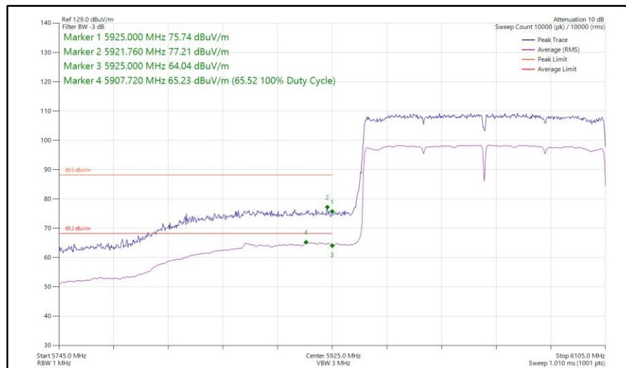
Figure 288 - 802.11ax HE160, SU, SISO, Core 0 - 6025 MHz Band Edge Frequency 5925 MHz
