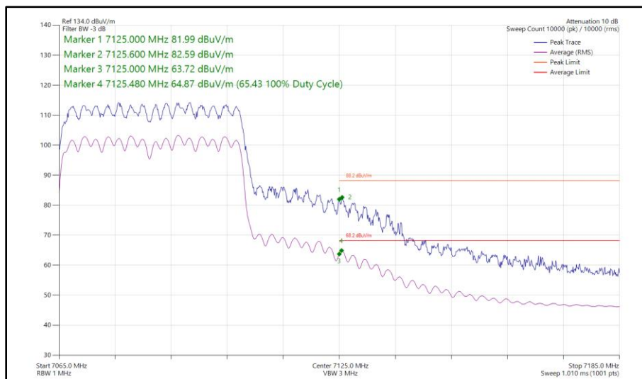
Figure 238 - 802.11ax HE40, SU, CDD, Core 0 - Core 1 - 7085 MHz Band Edge Frequency 7125 MHz
