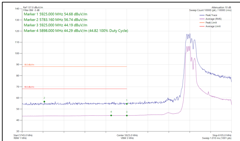
Figure 279 - 802.11ax HE80, RU 106-53, SDM, Core 0 - Core 1 - 6065 MHz Band Edge Frequency 5925 MHz
