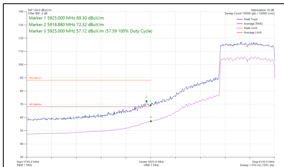
Figure 278 - 802.11ax HE80, SU, SDM, Core 0 - Core 1 - 6065 MHz Band Edge Frequency 5925 MHz
