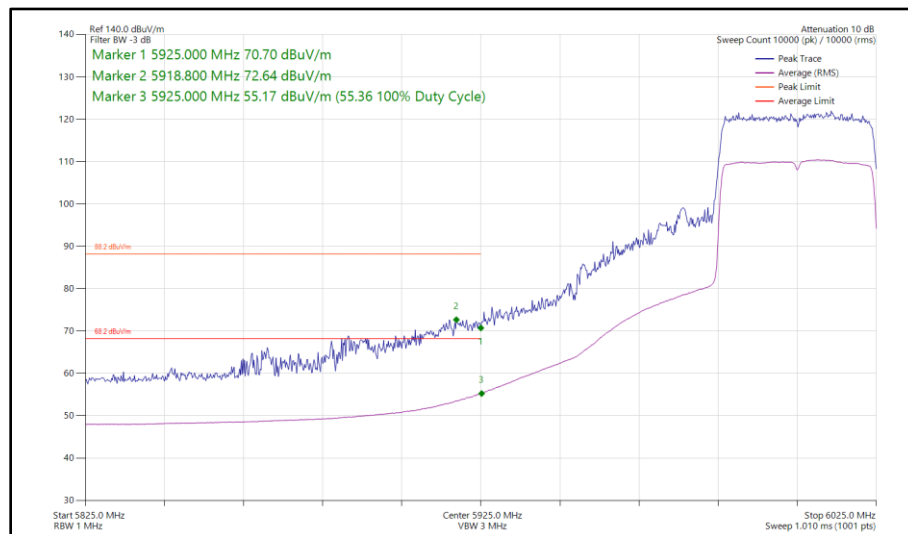
Figure 249 - 802.11ax HE40, SU, TxBF, Core 0 - Core 1 - 6005 MHz Band Edge Frequency 5925 MHz
