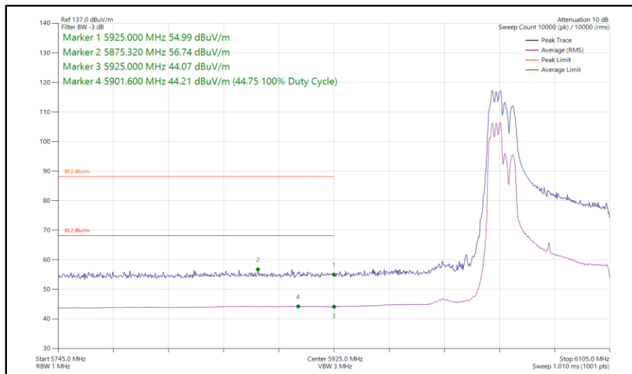
Figure 271 - 802.11ax HE80, RU 106-53, CDD, Core 0 - Core 1 - 6065 MHz Band Edge Frequency 5925 MHz
