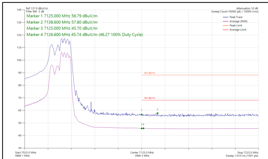
Figure 237 - 802.11ax HE40, RU 106-56, CDD, Core 0 - Core 1 - 7045 MHz Band Edge Frequency 7125 MHz
