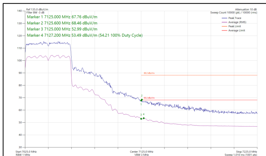
Figure 244 - 802.11ax HE40, SU, SDM, Core 0 - Core 1 - 7045 MHz Band Edge Frequency 7125 MHz
