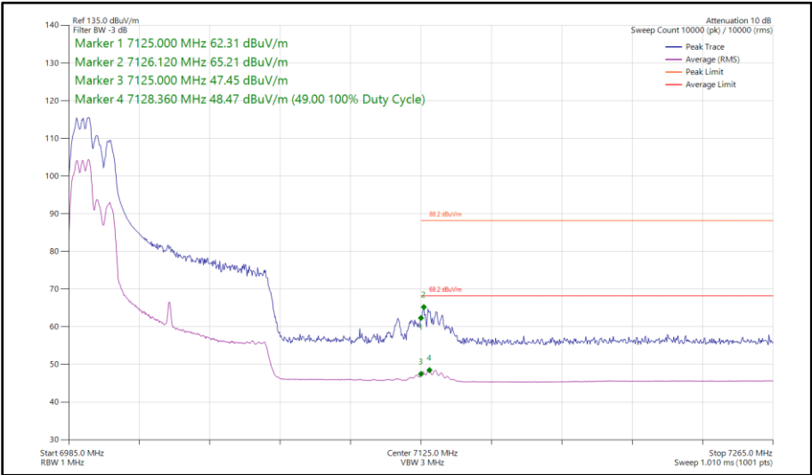
Figure 283 - 802.11ax HE80, RU 106-53, SDM, Core 0 - Core 1 - 7025 MHz Band Edge Frequency 7125 MHz
