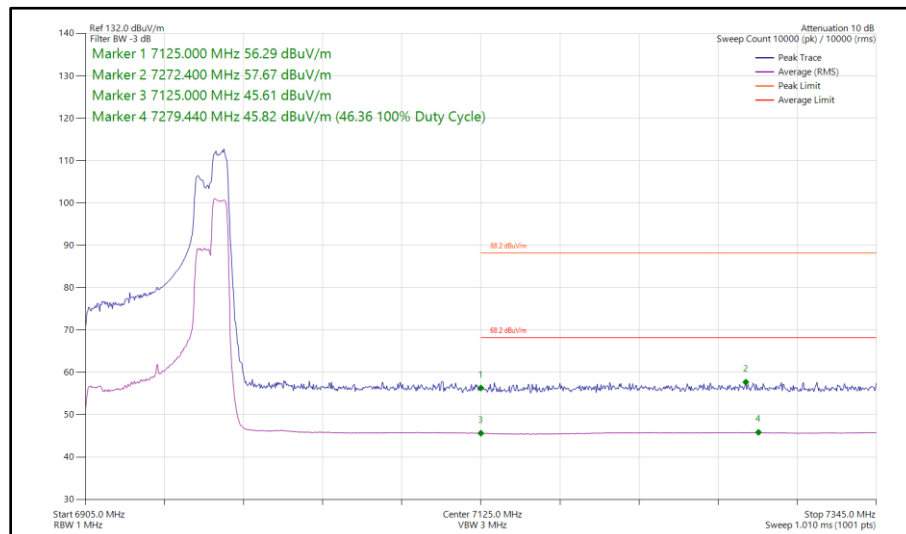
Figure 265 - 802.11ax HE80, RU 106-60, SISO, Core 1 - 6945 MHz Band Edge Frequency 7125 MHz
