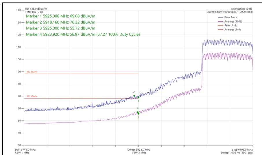
Figure 270 - 802.11ax HE80, SU, CDD, Core 0 - Core 1 - 6065 MHz Band Edge Frequency 5925 MHz
