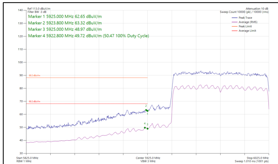
Figure 276 - 802.11ax HE80, SU, SDM, Core 0 - Core 1 - 5985 MHz Band Edge Frequency 5925 MHz
