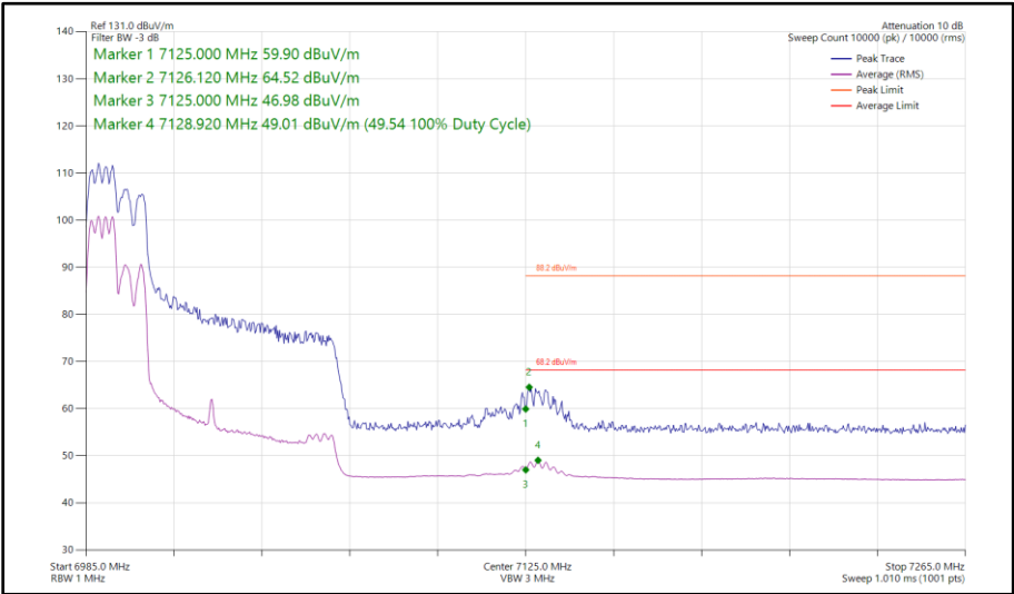
Figure 275 - 802.11ax HE80, RU 106-53, CDD, Core 0 - Core 1 - 7025 MHz Band Edge Frequency 7125 MHz
