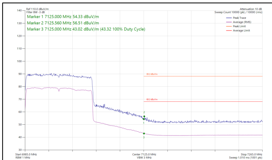
Figure 258 - 802.11ax HE80, SU, SISO, Core 0 - 7025 MHz Band Edge Frequency 7125 MHz
