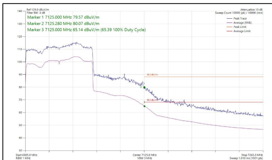
Figure 287 - 802.11ax HE80, SU, TxBF, Core 0 - Core 1 - 7025 MHz Band Edge Frequency 7125 MHz
