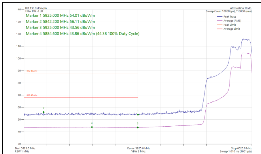
Figure 227 - 802.11ax HE40, RU 106-56, SISO, Core 1 - 6005 MHz Band Edge Frequency 5925 MHz
