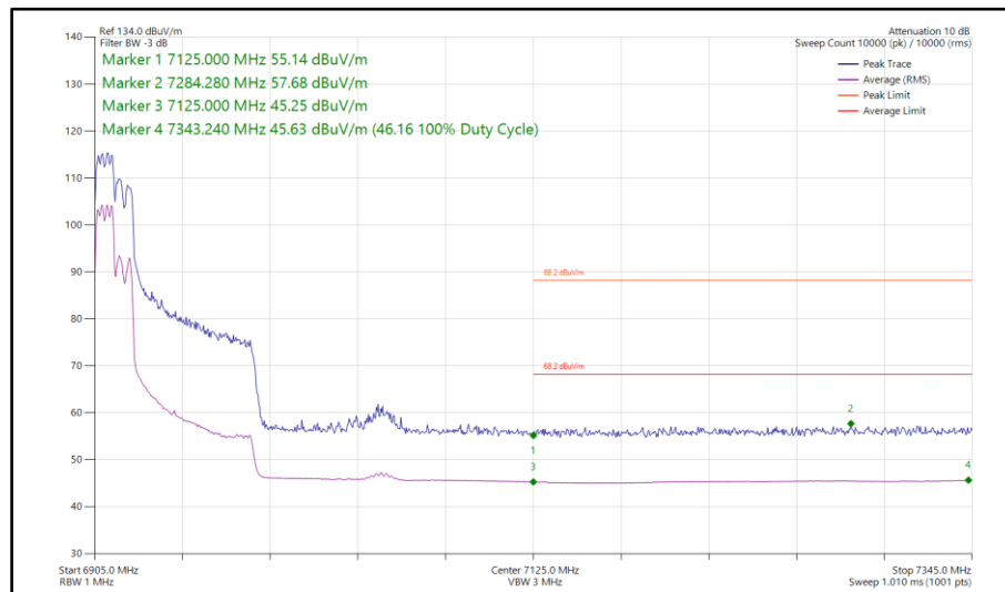
Figure 273 - 802.11ax HE80, RU 106-53, CDD, Core 0 - Core 1 - 6945 MHz Band Edge Frequency 7125 MHz
