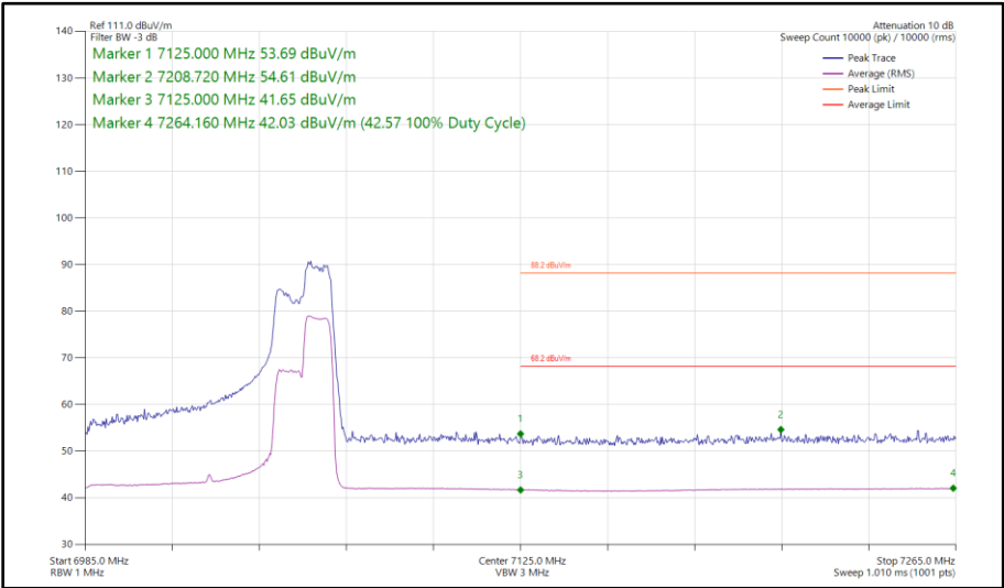
Figure 259 - 802.11ax HE80, RU 106-60, SISO, Core 0 - 7025 MHz Band Edge Frequency 7125 MHz
