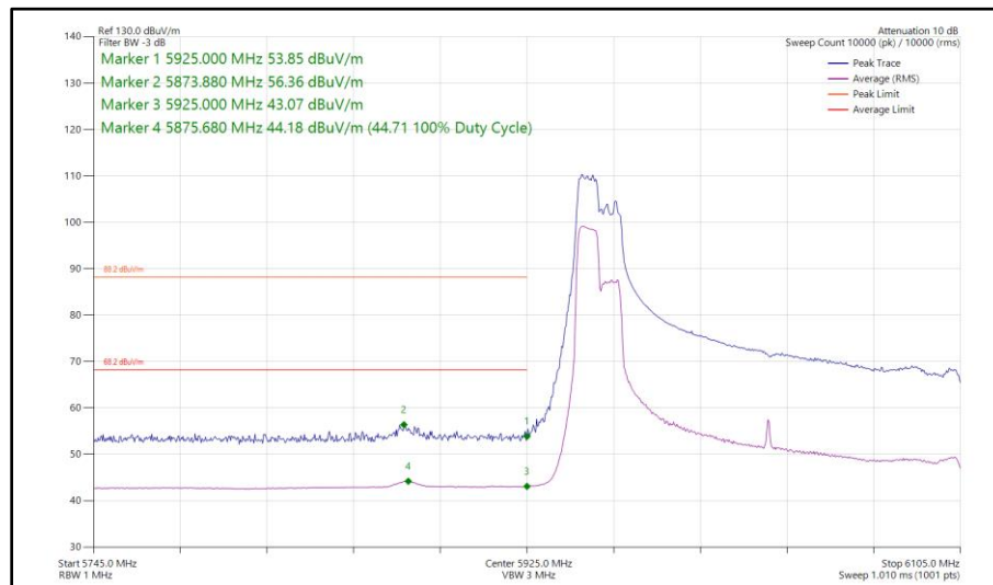
Figure 289 - 802.11ax HE160, RU 106-53P, SISO, Core 0 - 6025 MHz Band Edge Frequency 5925 MHz
