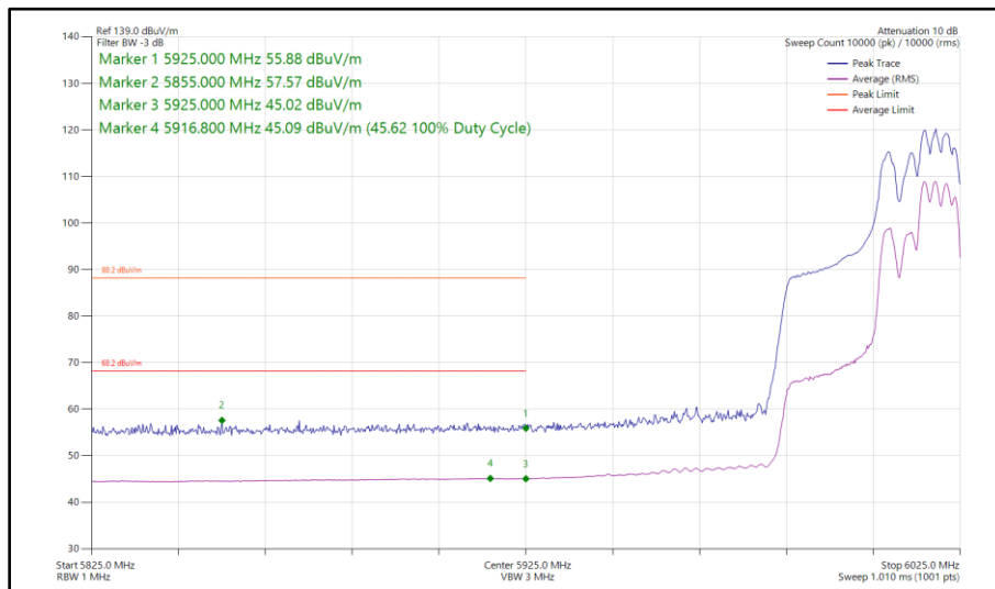
Figure 235 - 802.11ax HE40, RU 106-56, CDD, Core 0 - Core 1 - 6005 MHz Band Edge Frequency 5925 MHz
