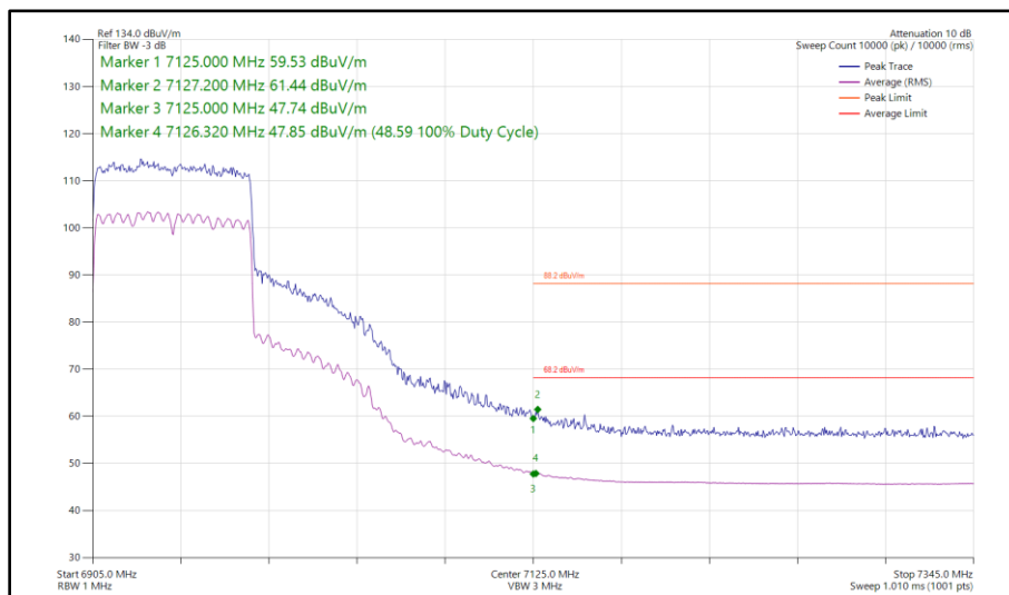
Figure 280 - 802.11ax HE80, SU, SDM, Core 0 - Core 1 - 6945 MHz Band Edge Frequency 7125 MHz
