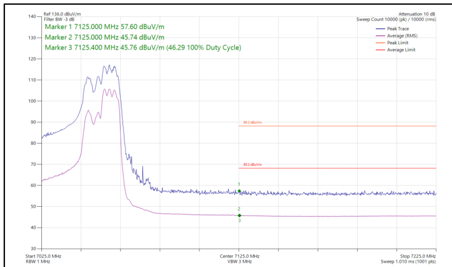
Figure 245 - 802.11ax HE40, RU 106-56, SDM, Core 0 - Core 1 - 7045 MHz Band Edge Frequency 7125 MHz
