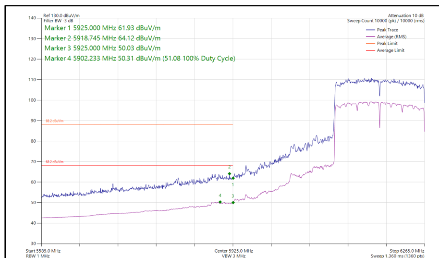
Figure 290 - 802.11ax HE160, SU, SISO, Core 0 - 6185 MHz Band Edge Frequency 5925 MHz
