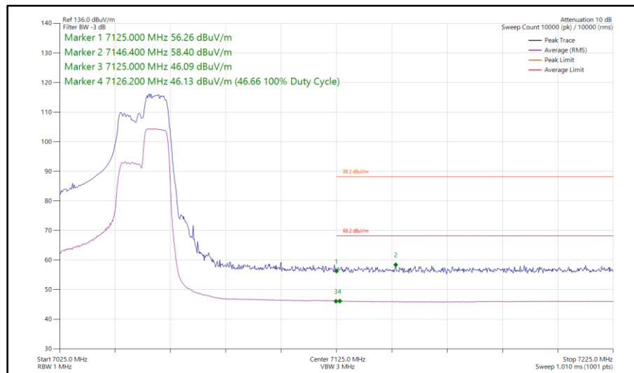
Figure 229 - 802.11ax HE40, RU 106-56, SISO, Core 1 - 7045 MHz Band Edge Frequency 7125 MHz
