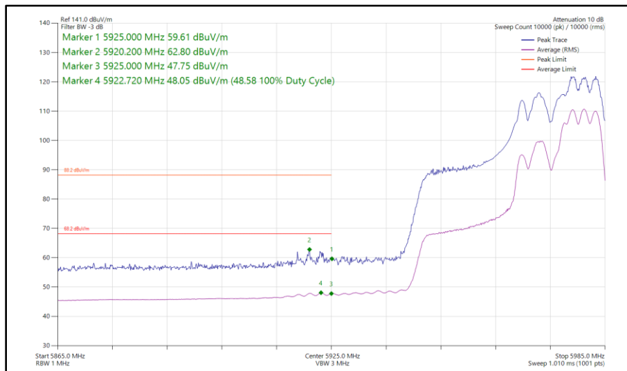
Figure 233 - 802.11ax HE40, RU 106-56, CDD, Core 0 - Core 1 - 5965 MHz Band Edge Frequency 5925 MHz
