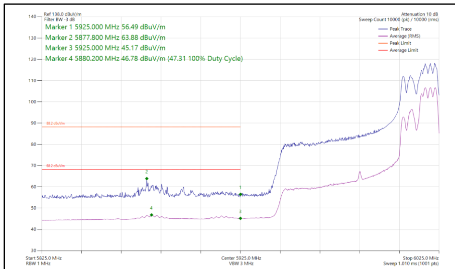
Figure 269 - 802.11ax HE80, RU 106-60, CDD, Core 0 - Core 1 - 5985 MHz Band Edge Frequency 5925 MHz
