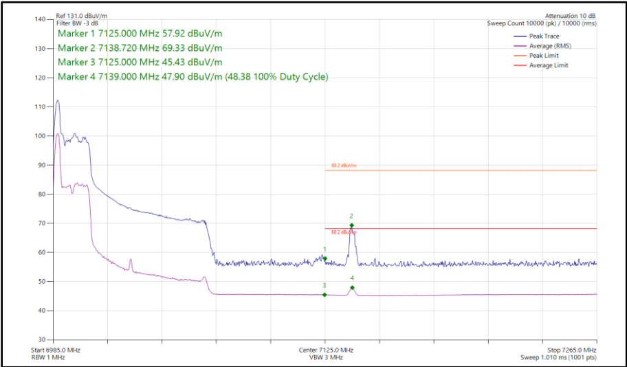
Figure 267 - 802.11ax HE80, RU 26-0, SISO, Core 1 - 7025 MHz Band Edge Frequency 7125 MHz
