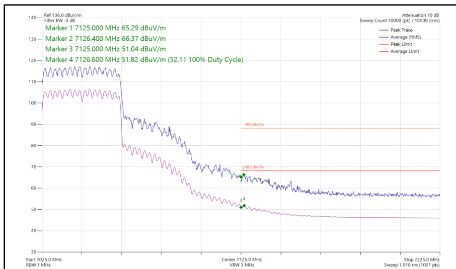
Figure 236 - 802.11ax HE40, SU, CDD, Core 0 - Core 1 - 7045 MHz Band Edge Frequency 7125 MHz
