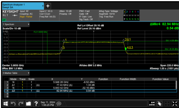
Figure 156 - 802.11ax HE80 SU LPI Maximum 26 dB EBW
