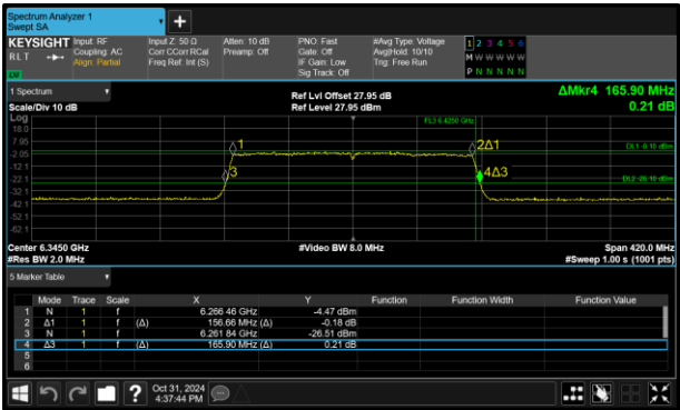
Figure 127 - 802.11ax HE160 SU VLP Minimum 26 dB EBW
