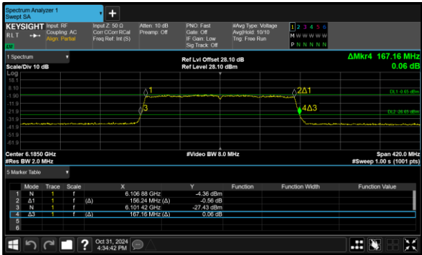
Figure 128 - 802.11ax HE160 SU VLP Maximum 26 dB EBW
