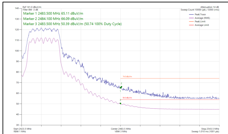
Figure 108 - 802.11n HT20, CDD, Core 0 - Core 1 - 2437 MHz Band Edge Frequency 2483.5 MHz
