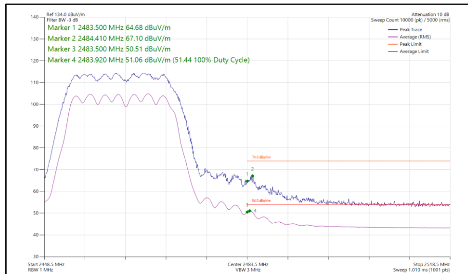
Figure 112 - 802.11n HT20, CDD, Core 0 - Core 1 - 2462 MHz Band Edge Frequency 2483.5 MHz
