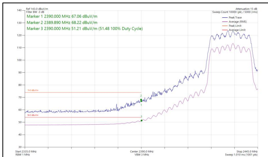
Figure 107 - 802.11ax HE20, SU, CDD, Core 0 - Core 1 - 2432 MHz Band Edge Frequency 2390 MHz
