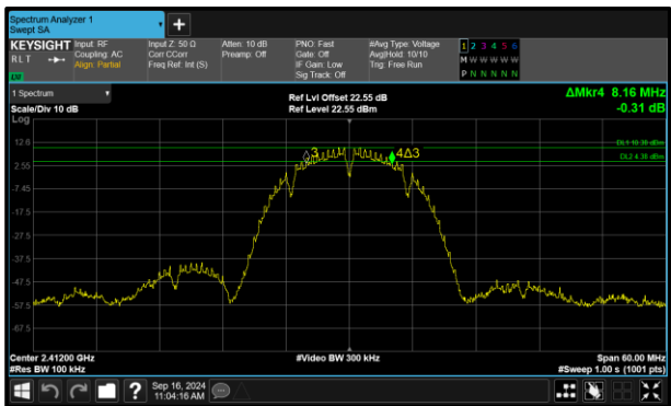
Figure 126 - 802.11b Minimum 6 dB EBW
