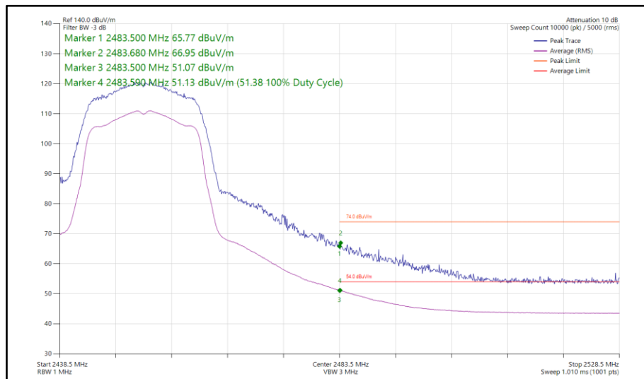
Figure 79 - 802.11n HT20, SISO, Core 1 - 2452 MHz Band Edge Frequency 2483.5 MHz
