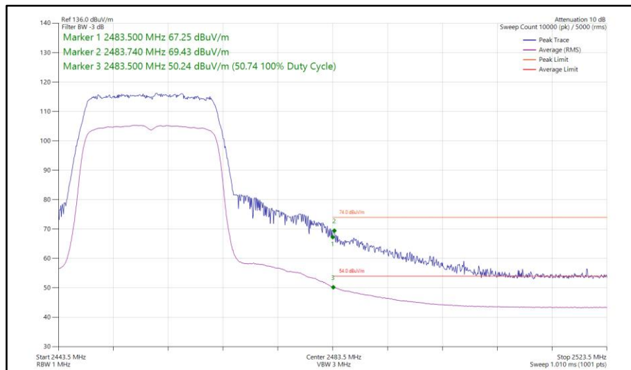
Figure 87 - 802.11ax HE20, SU, SISO, Core 1 - 2457 MHz Band Edge Frequency 2483.5 MHz
