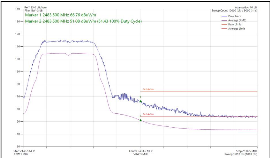
Figure 74 - 802.11g, SISO, Core 1 - 2462 MHz Band Edge Frequency 2483.5 MHz
