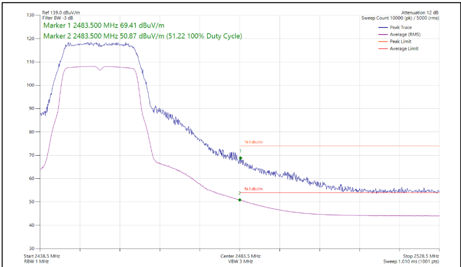
Figure 72 - 802.11g, SISO, Core 1 - 2452 MHz Band Edge Frequency 2483.5 MHz
