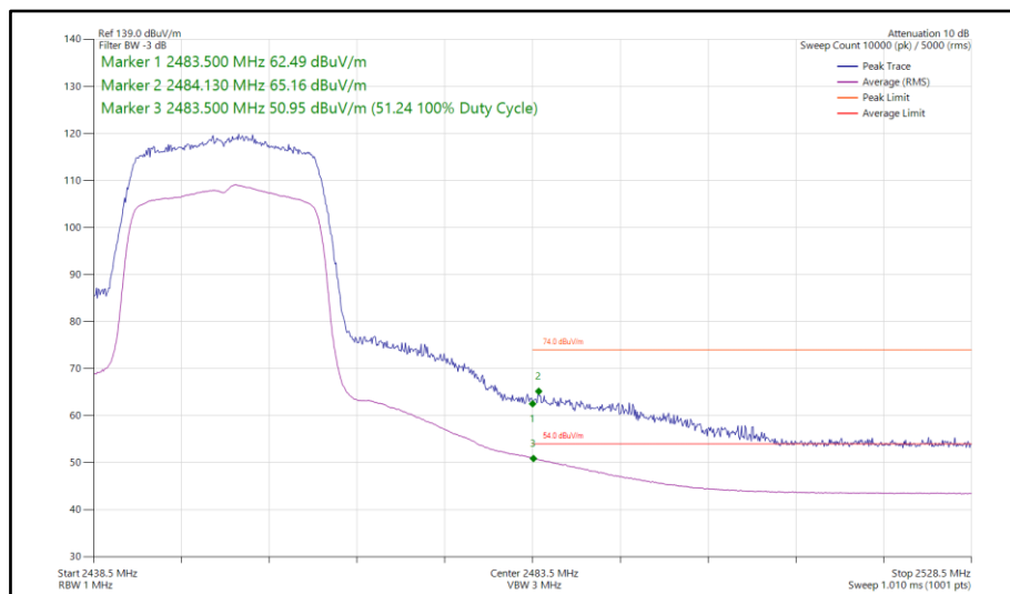
Figure 86 - 802.11ax HE20, SU, SISO, Core 1 - 2452 MHz Band Edge Frequency 2483.5 MHz
