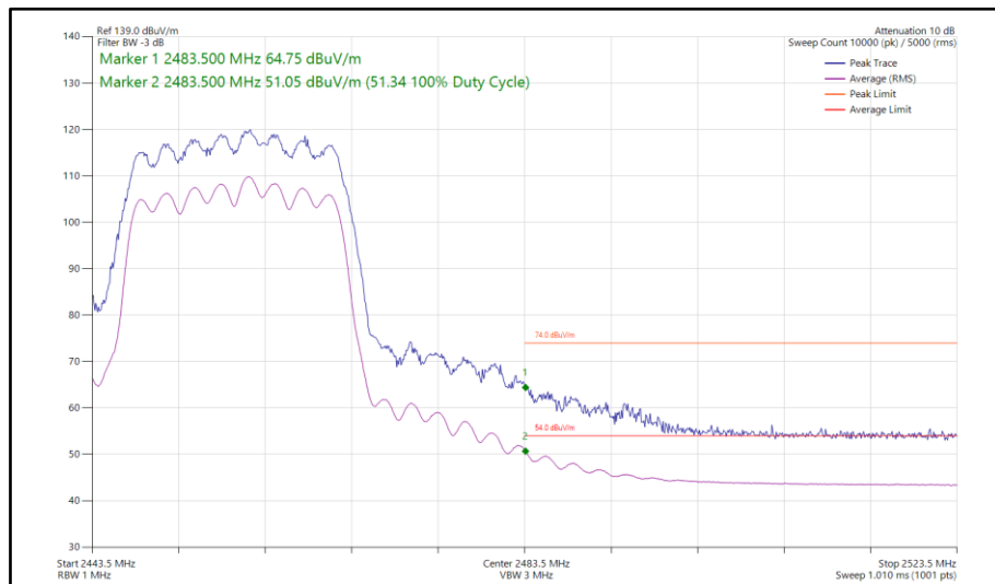
Figure 118 - 802.11ax HE20, SU, CDD, Core 0 - Core 1 - 2457 MHz Band Edge Frequency 2483.5 MHz
