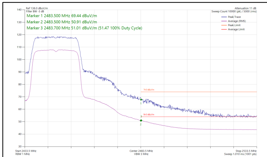
Figure 85 - 802.11ax HE20, SU, SISO, Core 1 - 2447 MHz Band Edge Frequency 2483.5 MHz
