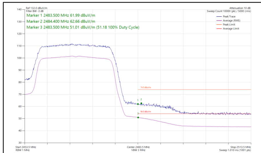
Figure 91 - 802.11ax HE20, SU, SISO, Core 1 - 2467 MHz Band Edge Frequency 2483.5 MHz
