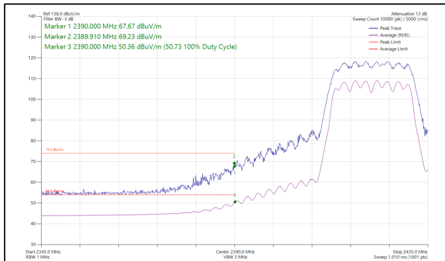
Figure 97 - 802.11n HT20, CDD, Core 0 - Core 1 - 2422 MHz Band Edge Frequency 2390 MHz
