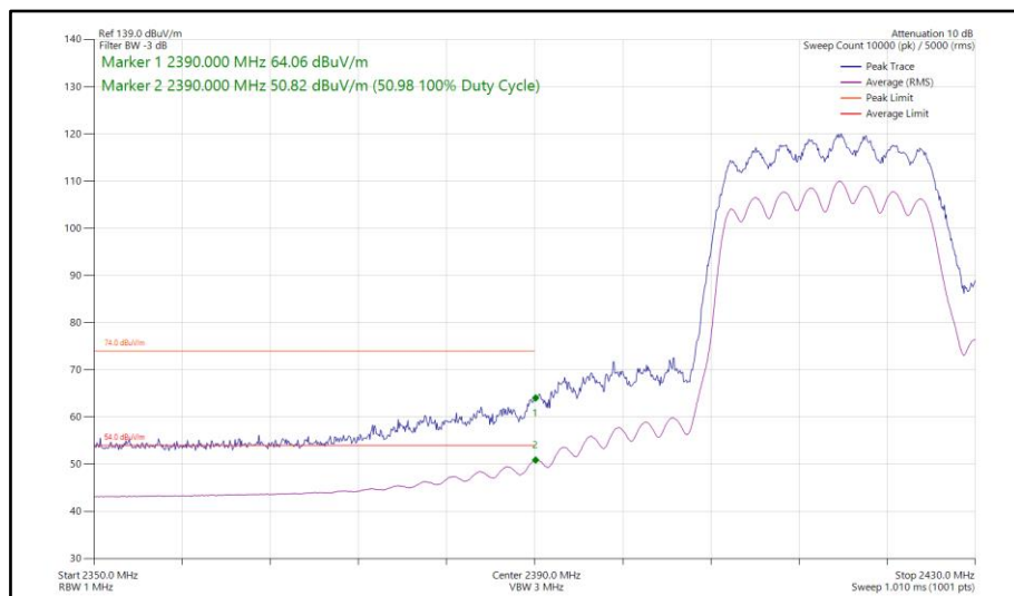
Figure 102 - 802.11ax HE20, SU, CDD, Core 0 - Core 1 - 2417 MHz Band Edge Frequency 2390 MHz
