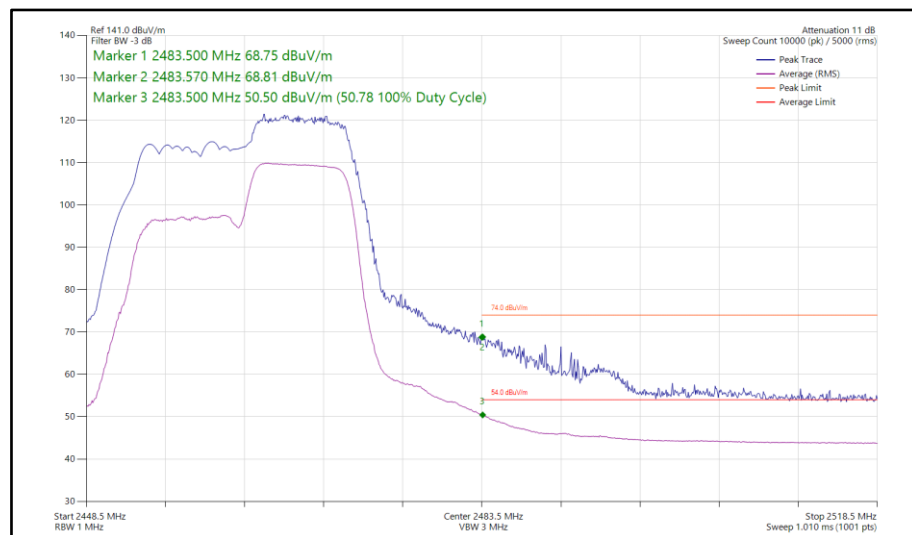
Figure 90 - 802.11ax HE20, RU 106-54, SISO, Core 1 - 2462 MHz Band Edge Frequency 2483.5 MHz
