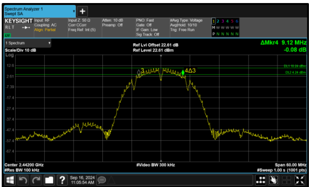
Figure 127 - 802.11b Maximum 6 dB EBW
