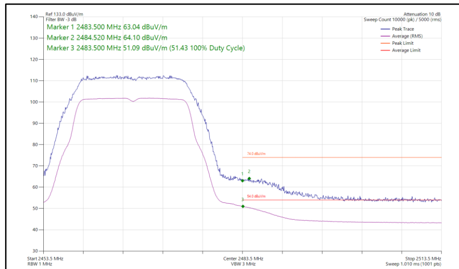
Figure 75 - 802.11g, SISO, Core 1 - 2467 MHz Band Edge Frequency 2483.5 MHz
