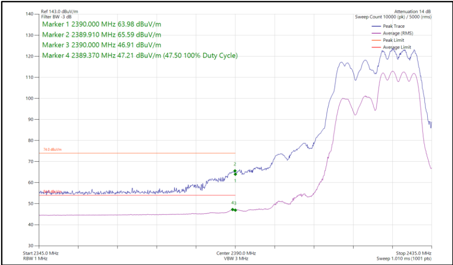
Figure 105 - 802.11ax HE20, RU 106-54, CDD, Core 0 - Core 1 - 2422 MHz Band Edge Frequency 2390 MHz
