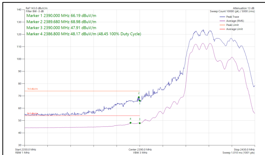
Figure 103 - 802.11ax HE20, RU 106-53, CDD, Core 0 - Core 1 - 2417 MHz Band Edge Frequency 2390 MHz
