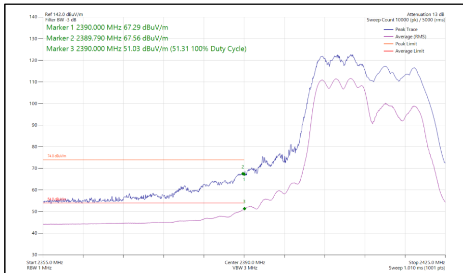
Figure 101 - 802.11ax HE20, RU 106-53, CDD, Core 0 - Core 1 - 2412 MHz Band Edge Frequency 2390 MHz
