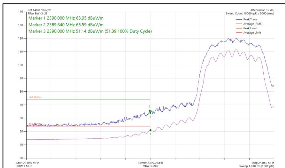
Figure 96 - 802.11n HT20, CDD, Core 0 - Core 1 - 2417 MHz Band Edge Frequency 2390 MHz
