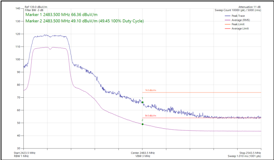
Figure 77 - 802.11n HT20, SISO, Core 1 - 2437 MHz Band Edge Frequency 2483.5 MHz
