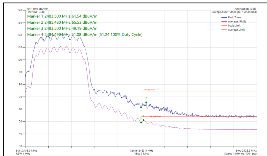
Figure 117 - 802.11ax HE20, SU, CDD, Core 0 - Core 1 - 2452 MHz Band Edge Frequency 2483.5 MHz
