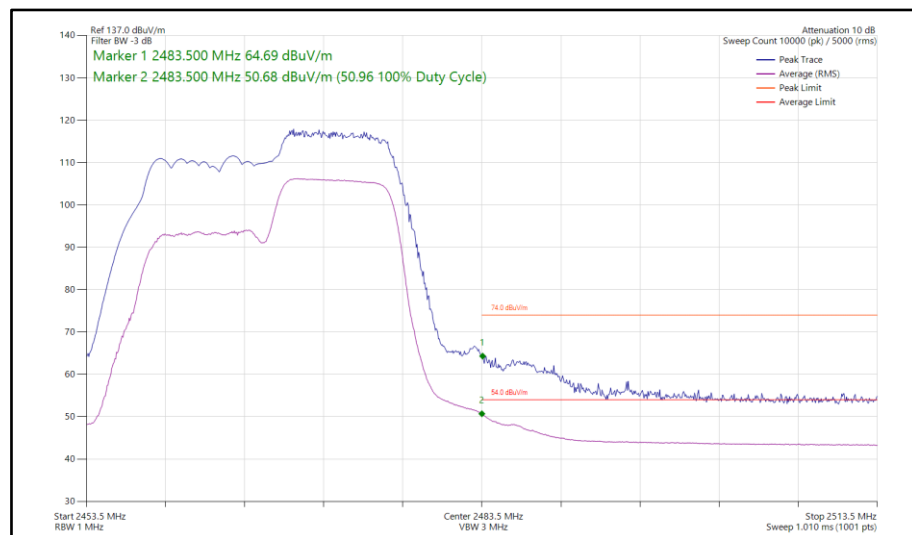
Figure 92 - 802.11ax HE20, RU 106-54, SISO, Core 1 - 2467 MHz Band Edge Frequency 2483.5 MHz
