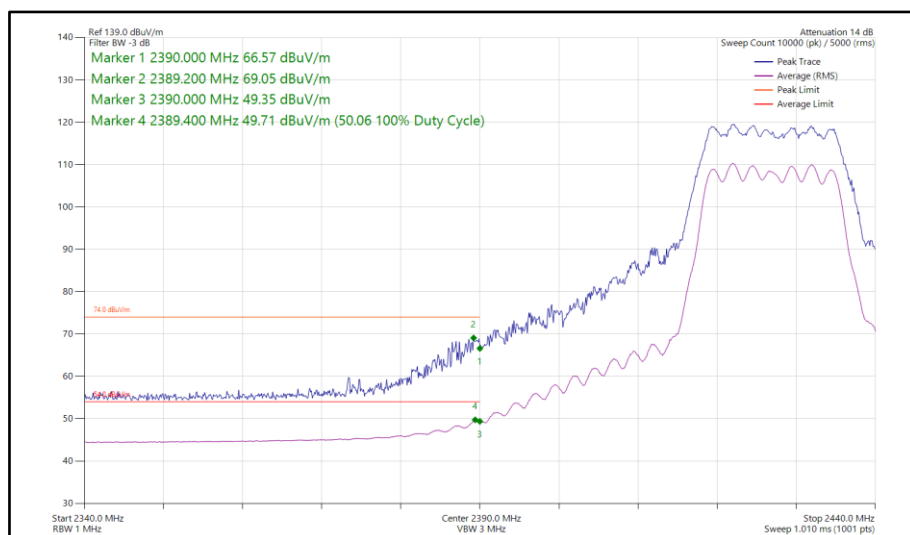
Figure 98 - 802.11n HT20, CDD, Core 0 - Core 1 - 2427 MHz Band Edge Frequency 2390 MHz
