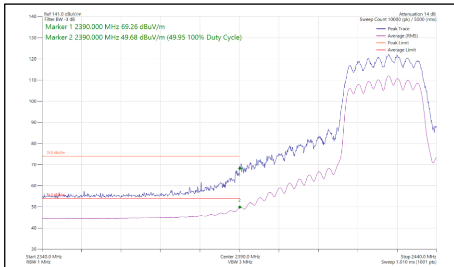
Figure 106 - 802.11ax HE20, SU, CDD, Core 0 - Core 1 - 2427 MHz Band Edge Frequency 2390 MHz
