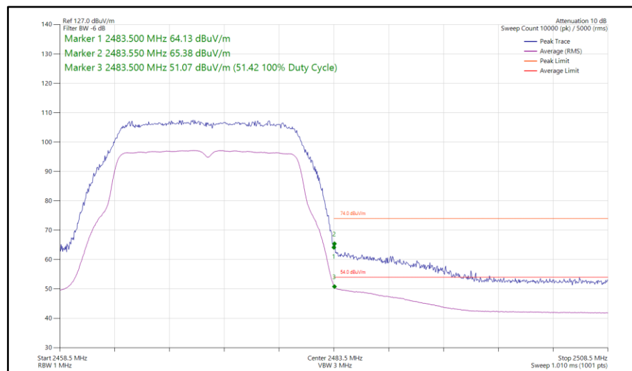
Figure 76 - 802.11g, SISO, Core 1 - 2472 MHz Band Edge Frequency 2483.5 MHz
