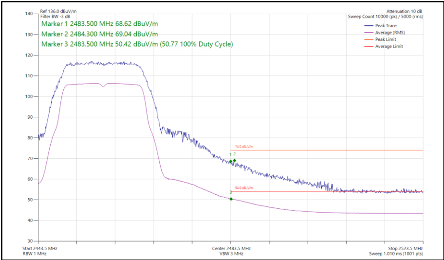
Figure 73 - 802.11g, SISO, Core 1 - 2457 MHz Band Edge Frequency 2483.5 MHz
