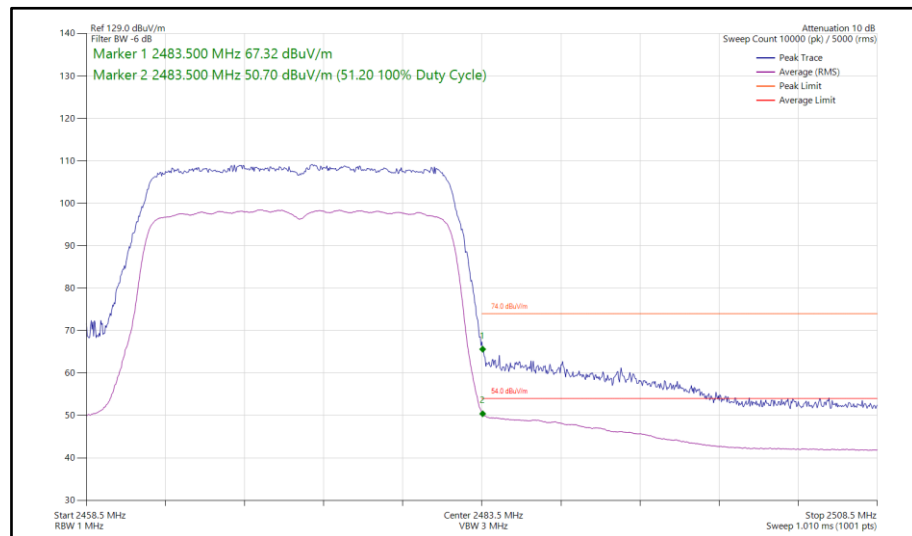
Figure 93 - 802.11ax HE20, SU, SISO, Core 1 - 2472 MHz Band Edge Frequency 2483.5 MHz
