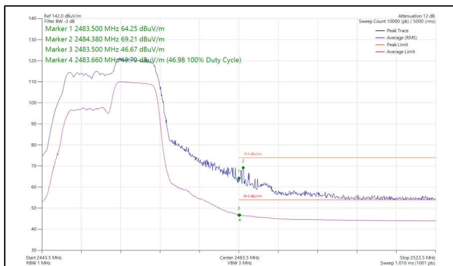
Figure 88 - 802.11ax HE20, RU 106-54, SISO, Core 1 - 2457 MHz Band Edge Frequency 2483.5 MHz
