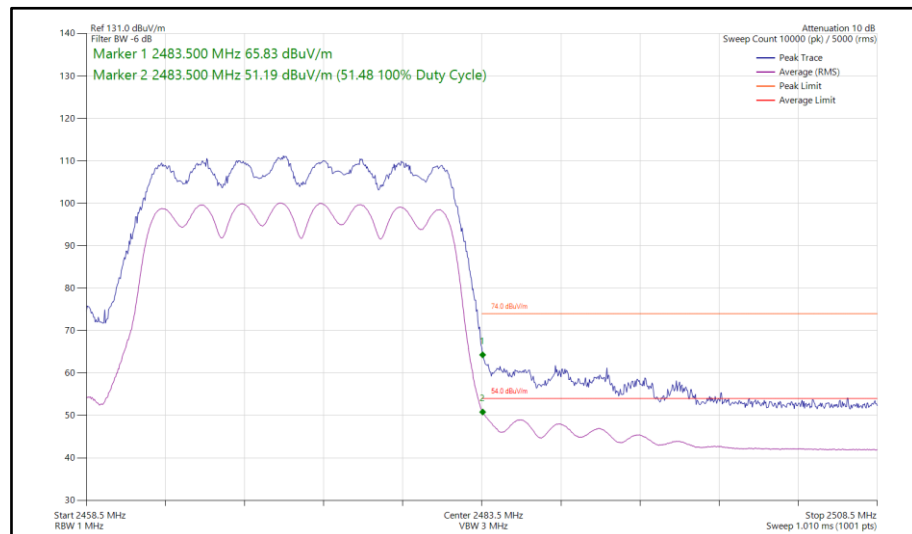
Figure 124 - 802.11ax HE20, SU, CDD, Core 0 - Core 1 - 2472 MHz Band Edge Frequency 2483.5 MHz
