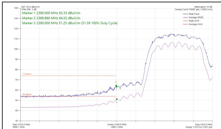
Figure 95 - 802.11n HT20, CDD, Core 0 - Core 1 - 2412 MHz Band Edge Frequency 2390 MHz
