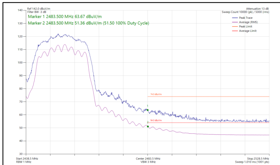
Figure 110 - 802.11n HT20, CDD, Core 0 - Core 1 - 2452 MHz Band Edge Frequency 2483.5 MHz
