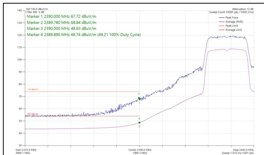
Figure 66 - 802.11ax HE20, SU, SISO, Core 1 - 2432 MHz Band Edge Frequency 2390 MHz
