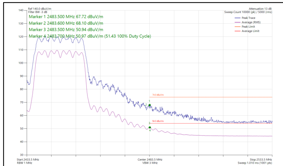
Figure 116 - 802.11ax HE20, SU, CDD, Core 0 - Core 1 - 2447 MHz Band Edge Frequency 2483.5 MHz
