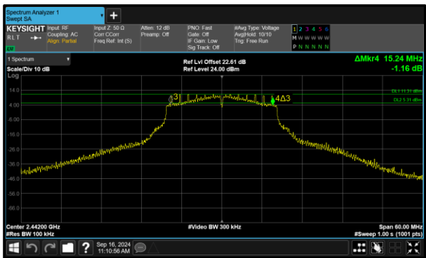
Figure 128 - 802.11g Minimum 6 dB EBW
