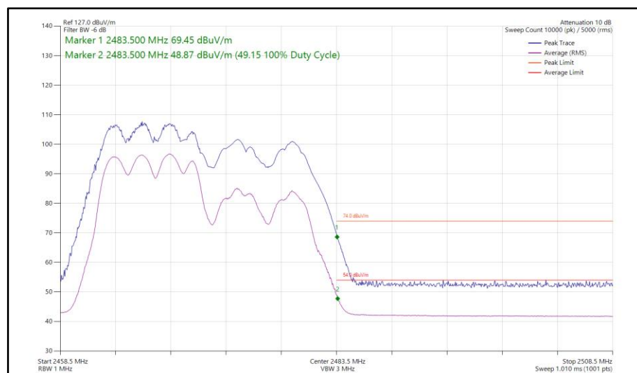
Figure 125 - 802.11ax HE20, RU 106-53, CDD, Core 0 - Core 1 - 2472 MHz Band Edge Frequency 2483.5 MHz
