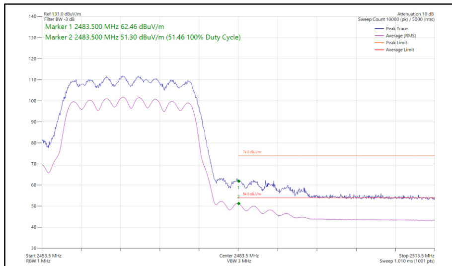
Figure 122 - 802.11ax HE20, SU, CDD, Core 0 - Core 1 - 2467 MHz Band Edge Frequency 2483.5 MHz
