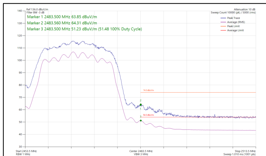
Figure 113 - 802.11n HT20, CDD, Core 0 - Core 1 - 2467 MHz Band Edge Frequency 2483.5 MHz
