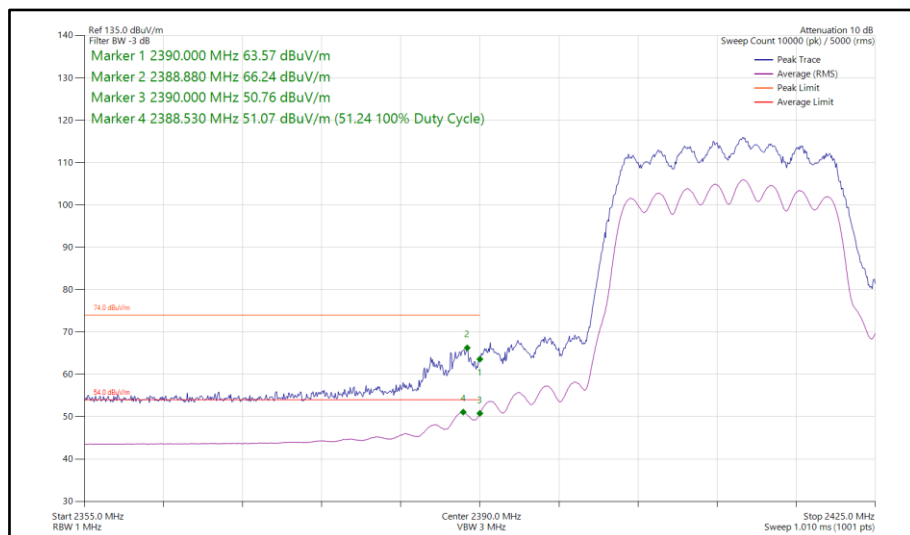
Figure 100 - 802.11ax HE20, SU, CDD, Core 0 - Core 1 - 2412 MHz Band Edge Frequency 2390 MHz
