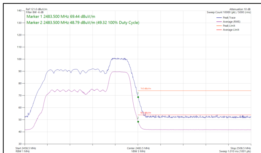
Figure 94 - 802.11ax HE20, RU 52-40, SISO, Core 1 - 2472 MHz Band Edge Frequency 2483.5 MHz
