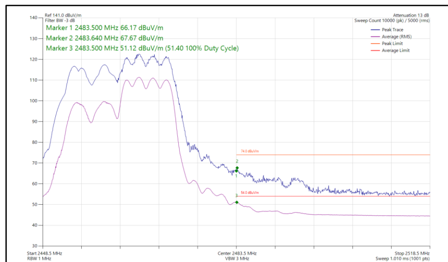
Figure 121 - 802.11ax HE20, RU 106-54, CDD, Core 0 - Core 1 - 2462 MHz Band Edge Frequency 2483.5 MHz
