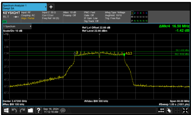
Figure 129 - 802.11g Maximum 6 dB EBW
