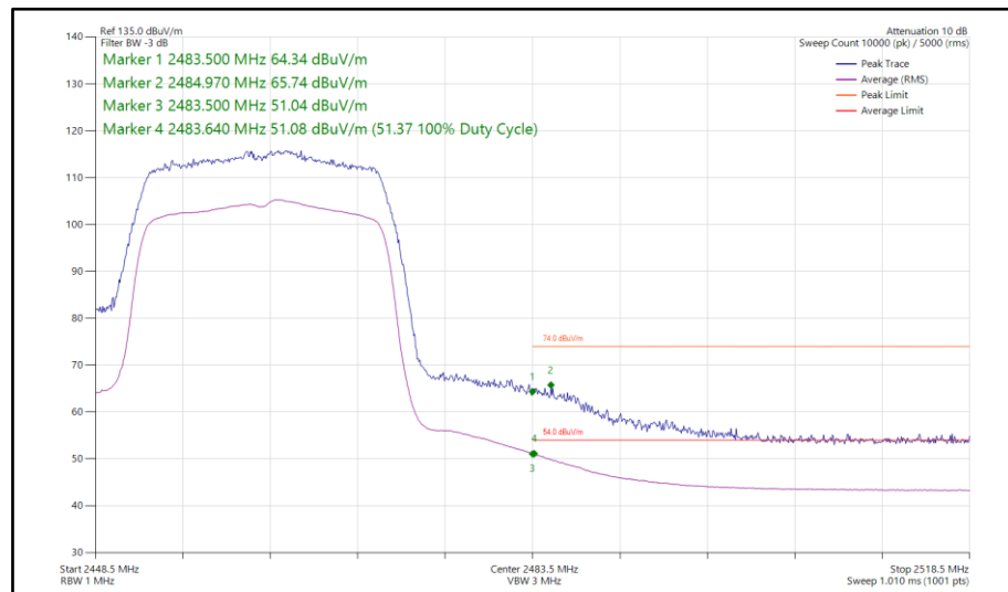
Figure 89 - 802.11ax HE20, SU, SISO, Core 1 - 2462 MHz Band Edge Frequency 2483.5 MHz
