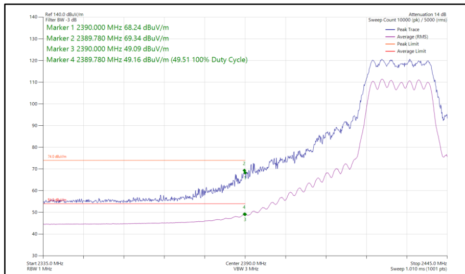
Figure 99 - 802.11n HT20, CDD, Core 0 - Core 1 - 2432 MHz Band Edge Frequency 2390 MHz
