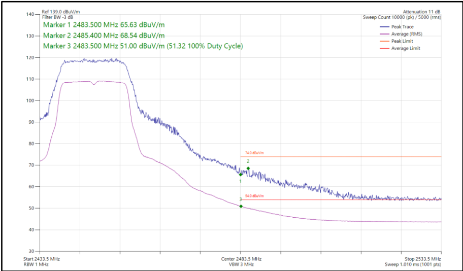
Figure 71 - 802.11g, SISO, Core 1 - 2447 MHz Band Edge Frequency 2483.5 MHz
