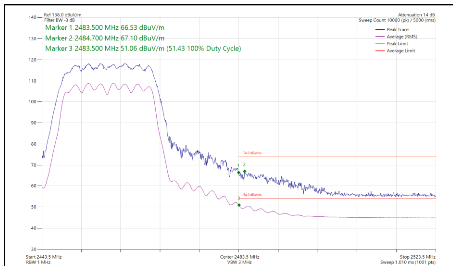
Figure 111 - 802.11n HT20, CDD, Core 0 - Core 1 - 2457 MHz Band Edge Frequency 2483.5 MHz
