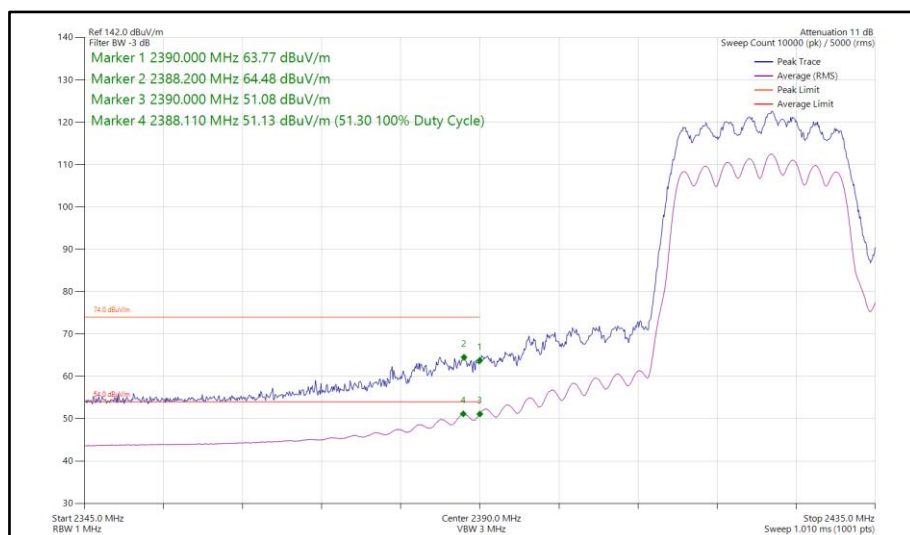
Figure 104 - 802.11ax HE20, SU, CDD, Core 0 - Core 1 - 2422 MHz Band Edge Frequency 2390 MHz
