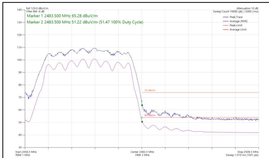
Figure 114 - 802.11n HT20, CDD, Core 0 - Core 1 - 2472 MHz Band Edge Frequency 2483.5 MHz
