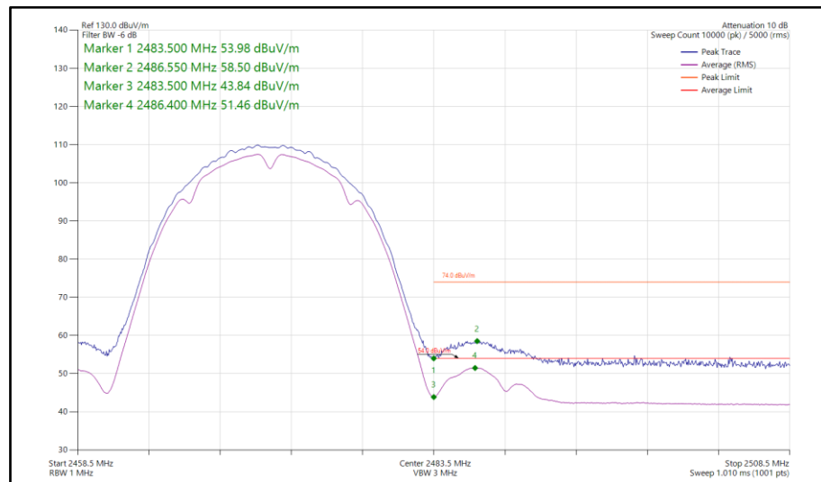
Figure 69 - 802.11b, SISO, Core 1 - 2472 MHz Band Edge Frequency 2483.5 MHz
