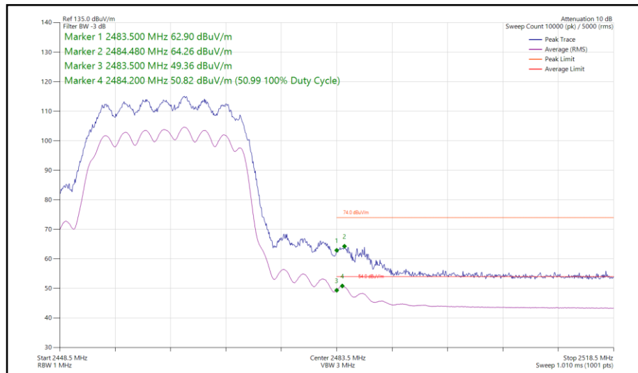
Figure 120 - 802.11ax HE20, SU, CDD, Core 0 - Core 1 - 2462 MHz Band Edge Frequency 2483.5 MHz
