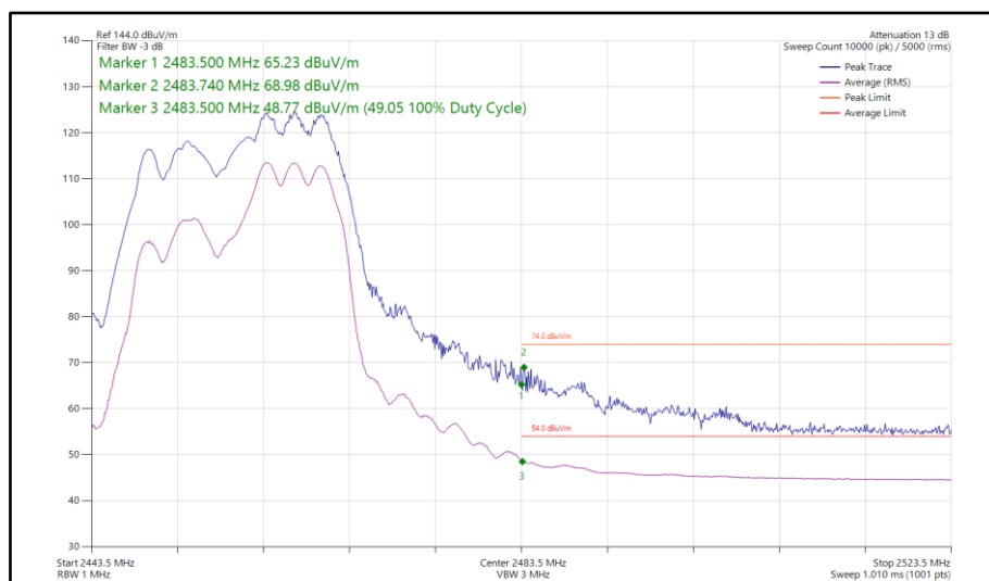
Figure 119 - 802.11ax HE20, RU 106-54, CDD, Core 0 - Core 1 - 2457 MHz Band Edge Frequency 2483.5 MHz
