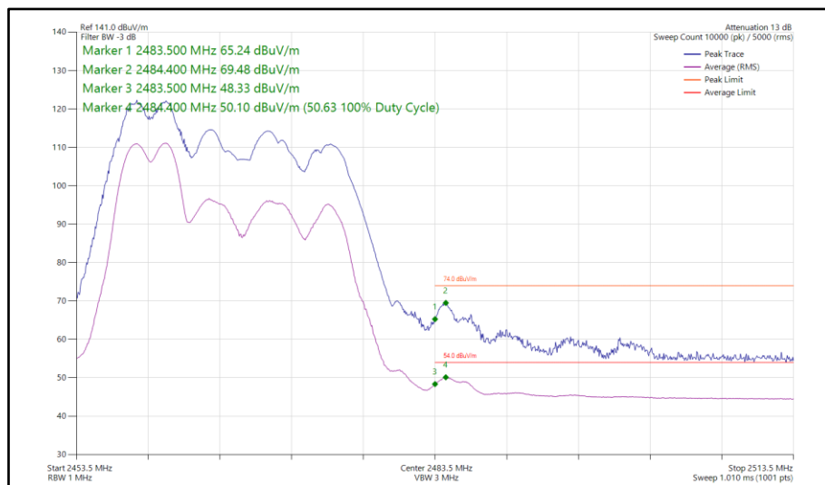
Figure 123 - 802.11ax HE20, RU 52-37, CDD, Core 0 - Core 1 - 2467 MHz Band Edge Frequency 2483.5 MHz
