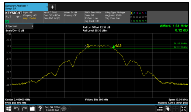
Figure 18 - Core 0 (A) 2405 MHz (CH11) 6 dB Bandwidth
