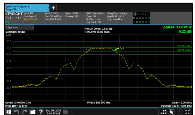
Figure 20 - Core 0 (A) 2440 MHz (CH18) 6 dB Bandwidth
