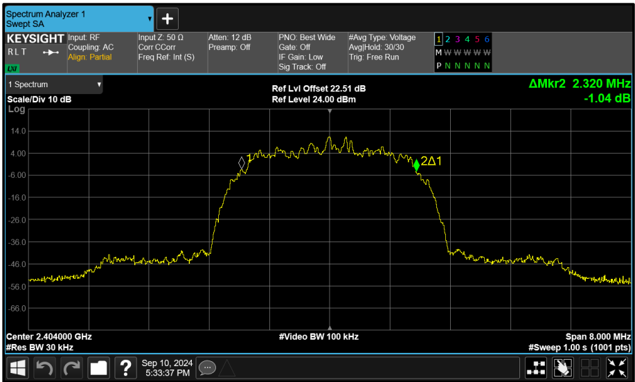
Figure 112 - Core 1 (B) 2404 MHz (CH2) 99% Bandwidth
