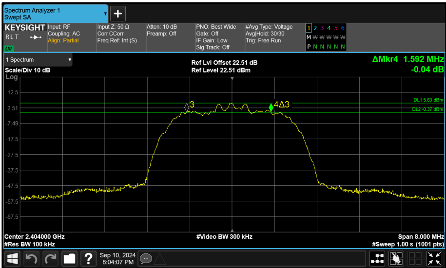
Figure 139 - Core 1 (B) 2404 MHz (CH2) 6 dB Bandwidth
