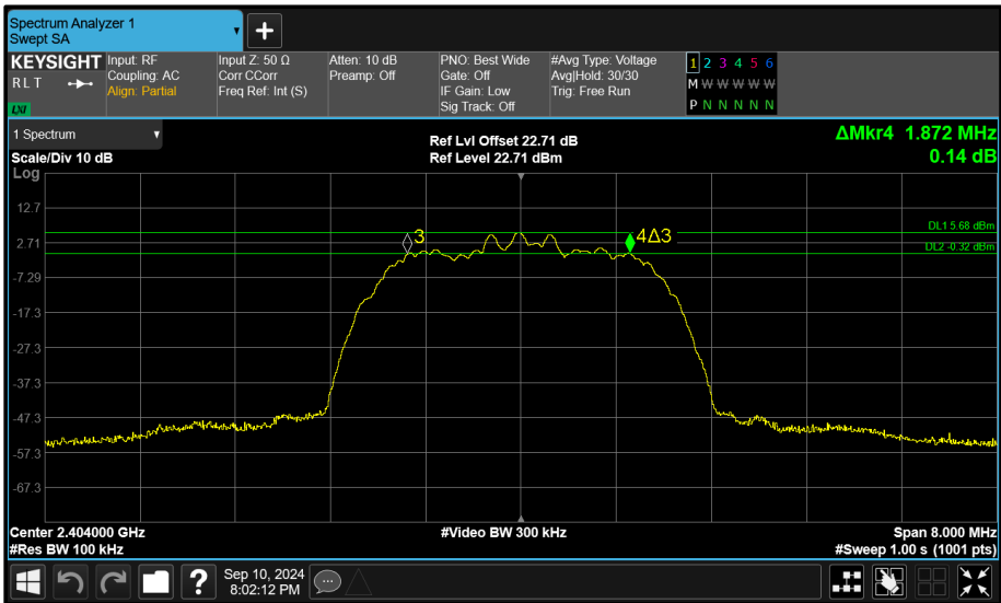
Figure 137 - Core 0 (A) 2404 MHz (CH2) 6 dB Bandwidth
