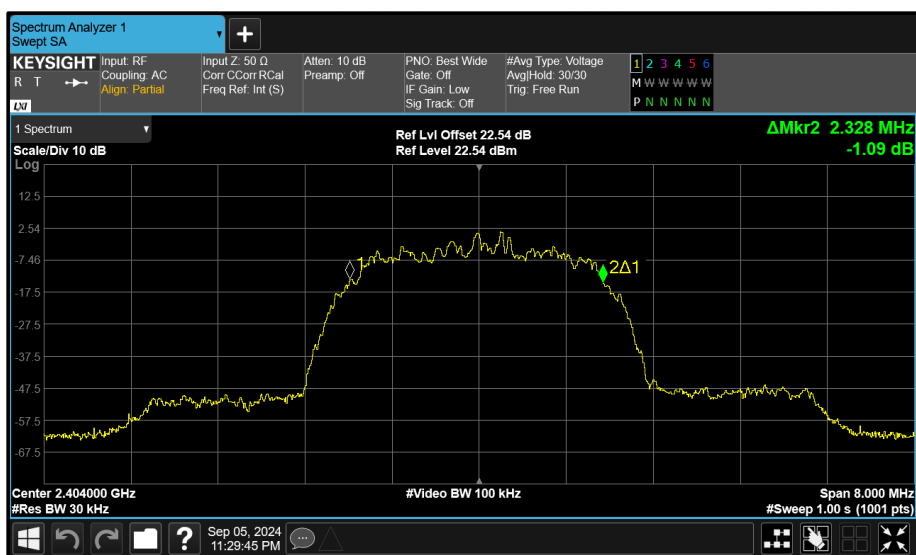
Figure 88 - Core 2 (C) 2404 MHz (CH2) 99% Bandwidth
