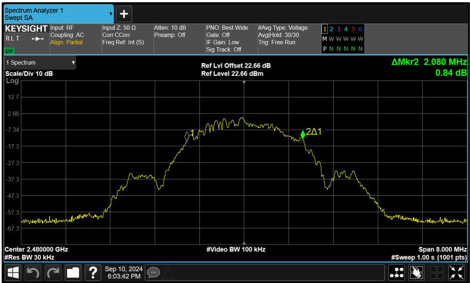
Figure 86 - Core 1 (B) 2480 MHz (CH39) 99% Bandwidth
