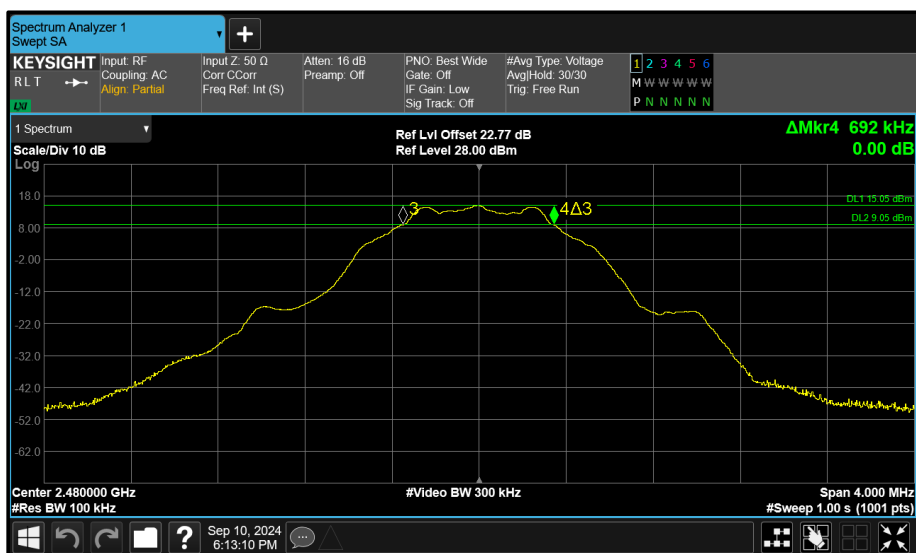
Figure 129 - Core 0 (A) 2480 MHz (CH39) 6 dB Bandwidth
