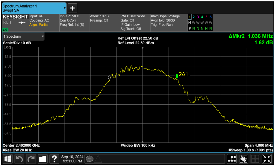
Figure 76 - Core 1 (B) 2402 MHz (CH37) 99% Bandwidth
