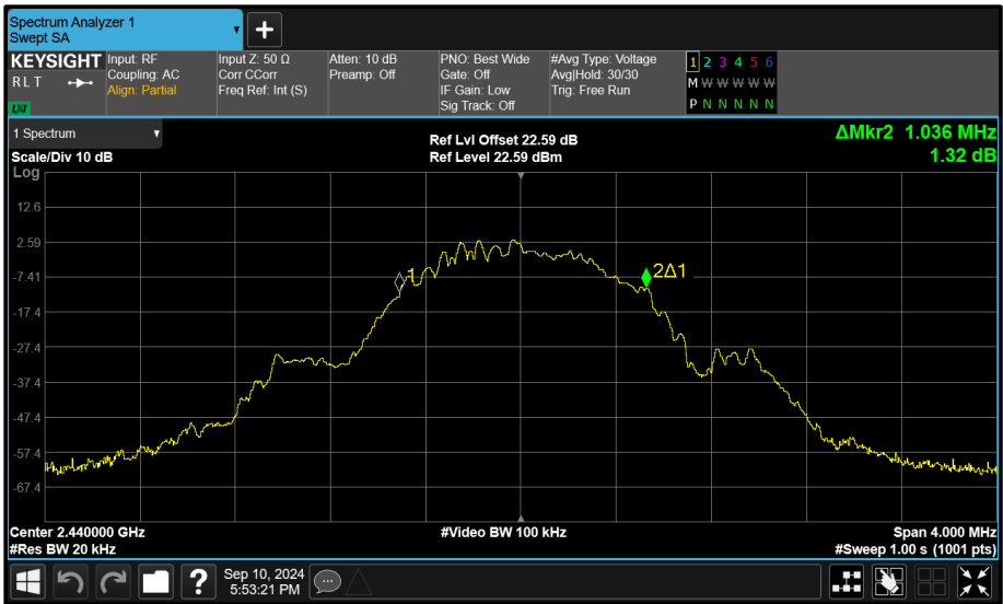
Figure 78 - Core 1 (B) 2440 MHz (CH17) 99% Bandwidth
