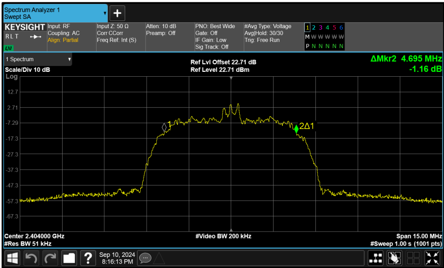
Figure 148 - Core 0 (A) 2404 MHz (CH2) 99% Bandwidth
