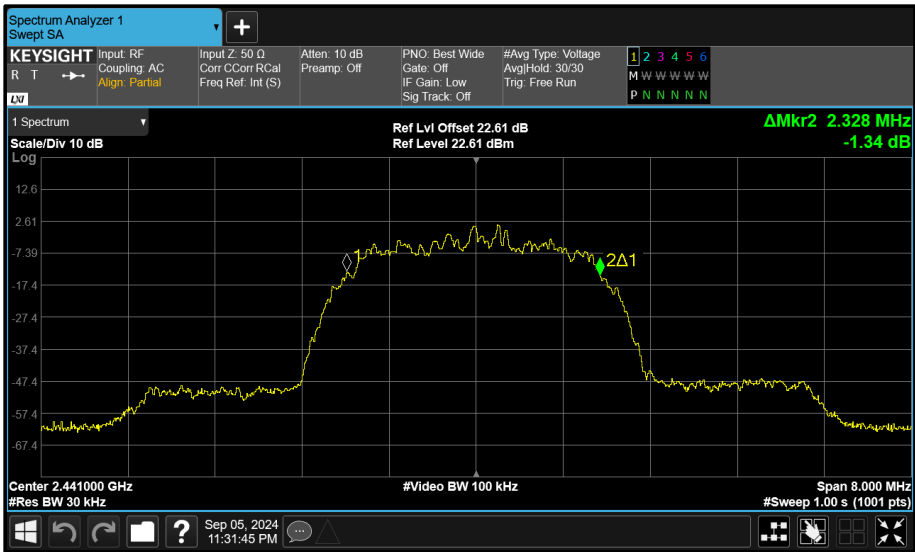
Figure 90 - Core 2 (C) 2441 MHz (CH39) 99% Bandwidth
