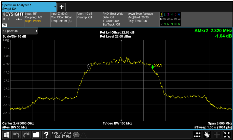
Figure 92 - Core 2 (C) 2476 MHz (CH74) 99% Bandwidth
