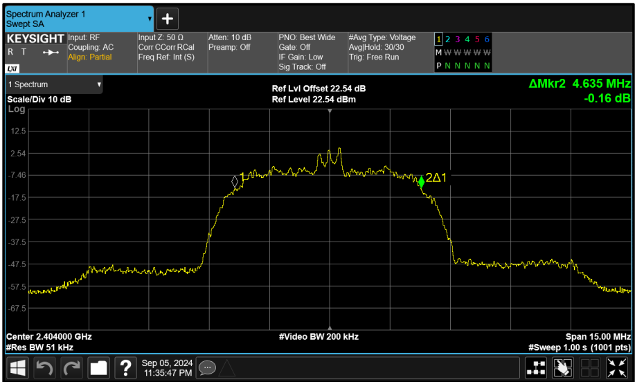
Figure 94 - Core 2 (C) 2404 MHz (CH2) 99% Bandwidth
