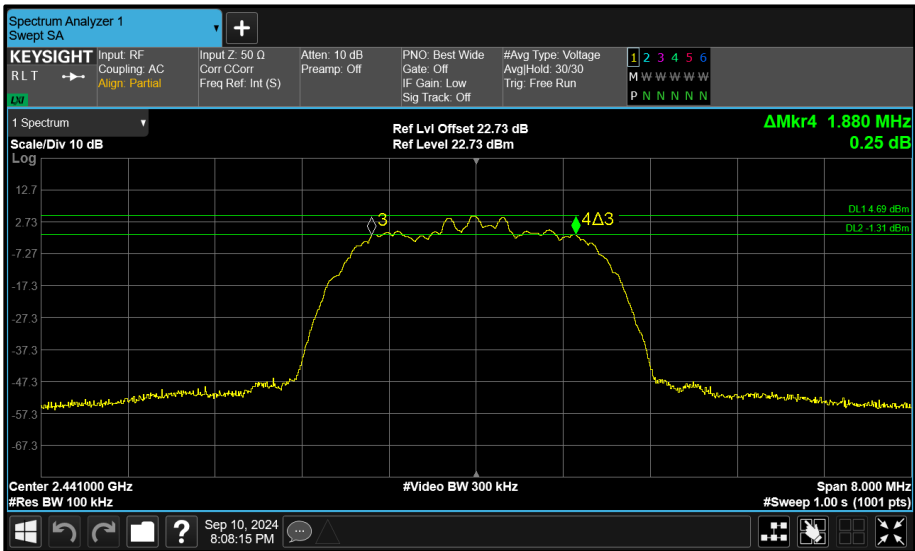
Figure 141 - Core 0 (A) 2441 MHz (CH39) 6 dB Bandwidth
