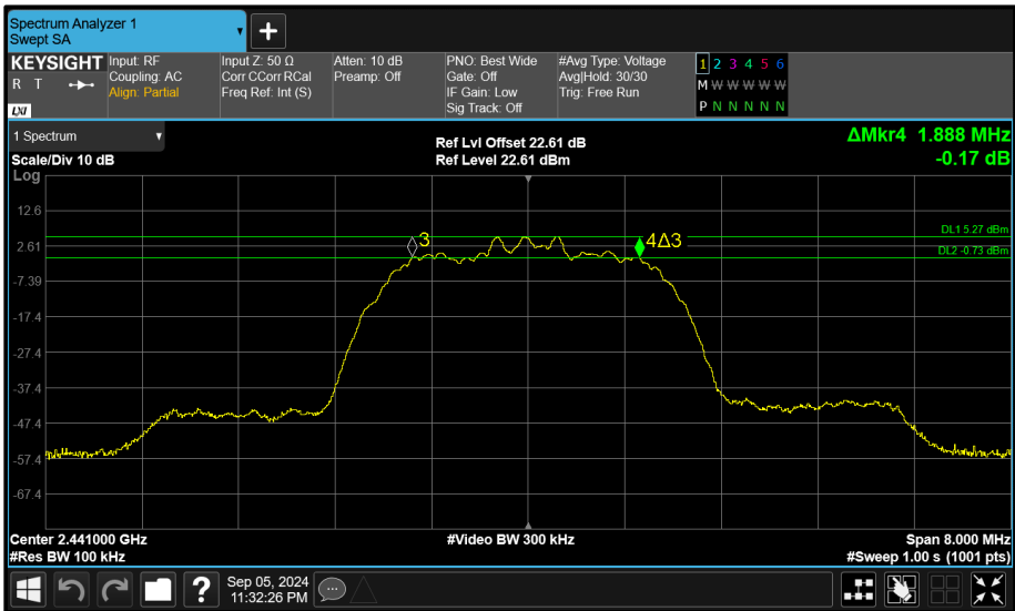
Figure 91 - Core 2 (C) 2441 MHz (CH39) 6 dB Bandwidth
