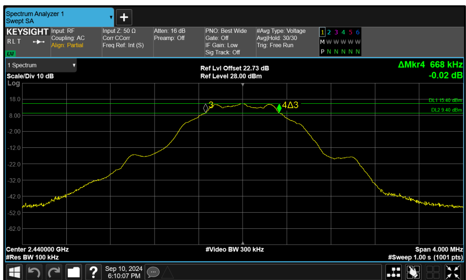
Figure 127 - Core 0 (A) 2440 MHz (CH17) 6 dB Bandwidth
