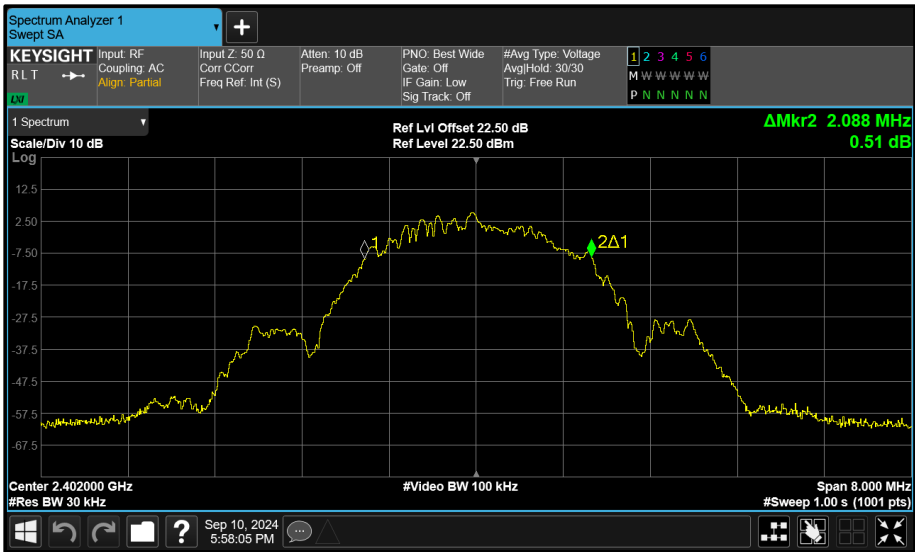
Figure 82 - Core 1 (B) 2402 MHz (CH37) 99% Bandwidth
