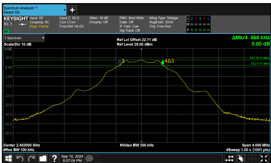
Figure 125 - Core 0 (A) 2402 MHz (CH37) 6 dB Bandwidth
