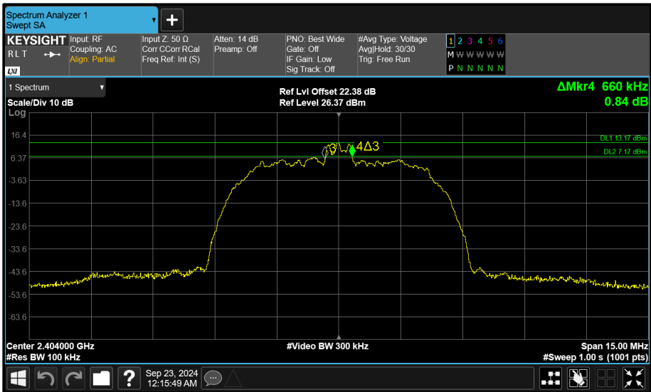
Figure 119 - Core 1 (B) 2404 MHz (CH2) 6 dB Bandwidth
