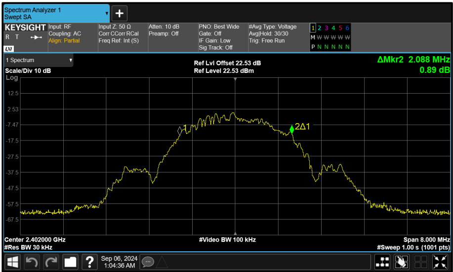
Figure 106 - Core 2 (C) 2402 MHz (CH37) 99% Bandwidth
