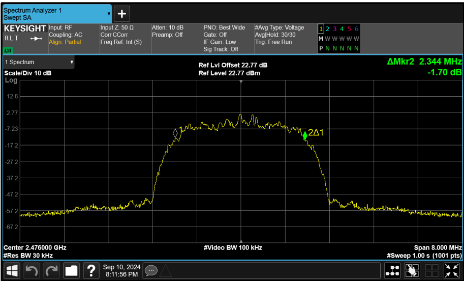
Figure 144 - Core 0 (A) 2476 MHz (CH74) 99% Bandwidth
