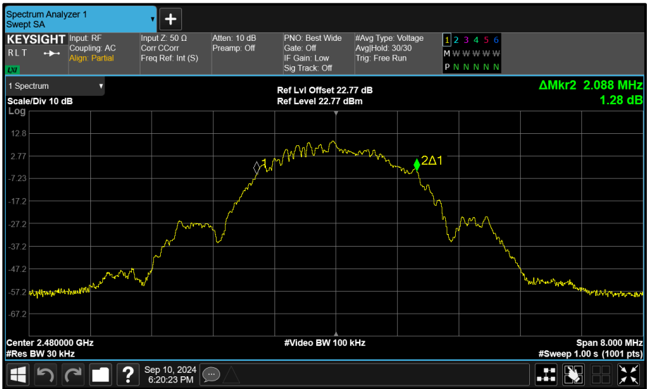
Figure 134 - Core 0 (A) 2480 MHz (CH39) 99% Bandwidth
