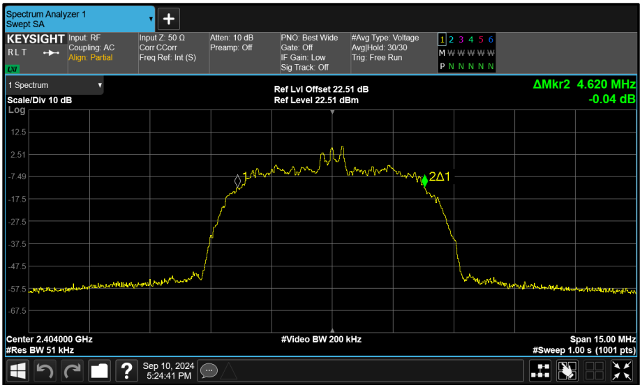
Figure 70 - Core 1 (B) 2404 MHz (CH2) 99% Bandwidth
