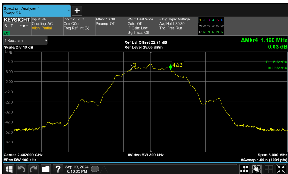
Figure 131 - Core 0 (A) 2402 MHz (CH37) 6 dB Bandwidth
