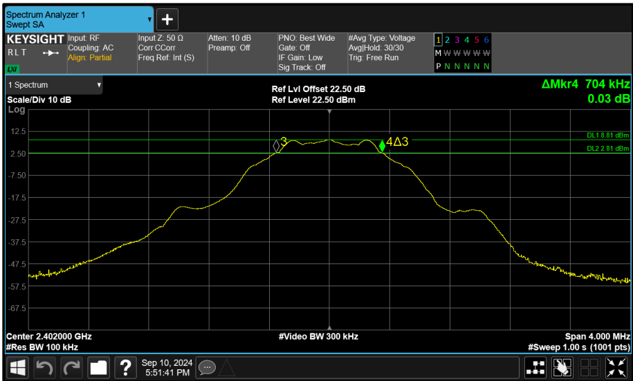
Figure 77 - Core 1 (B) 2402 MHz (CH37) 6 dB Bandwidth
