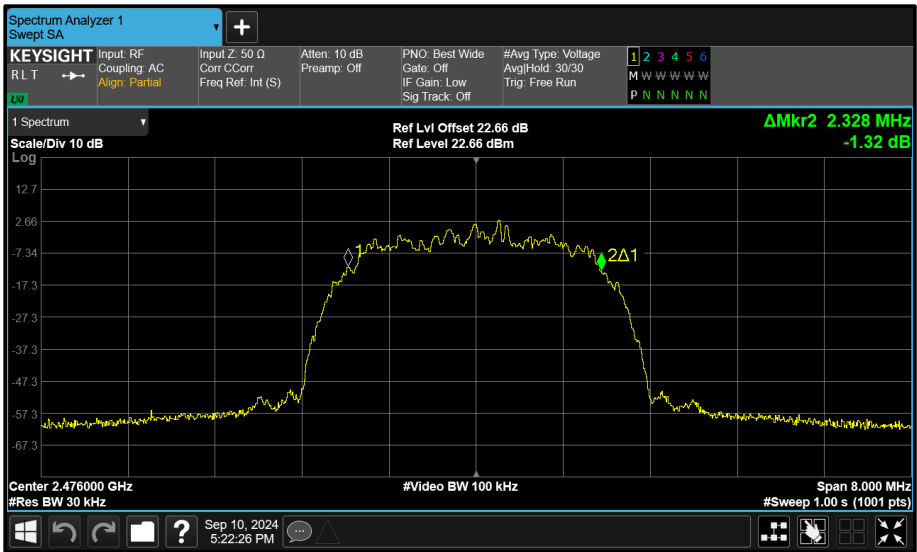
Figure 68 - Core 1 (B) 2476 MHz (CH74) 99% Bandwidth
