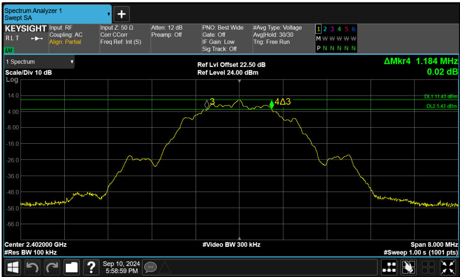
Figure 83 - Core 1 (B) 2402 MHz (CH37) 6 dB Bandwidth
