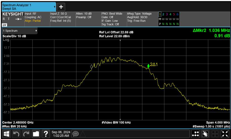
Figure 104 - Core 2 (C) 2480 MHz (CH39) 99% Bandwidth
