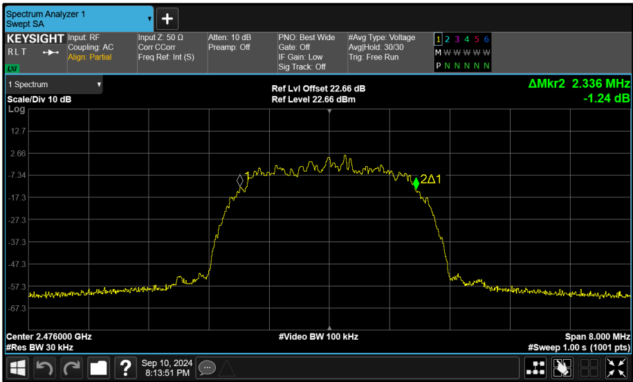
Figure 146 - Core 1 (B) 2476 MHz (CH74) 99% Bandwidth
