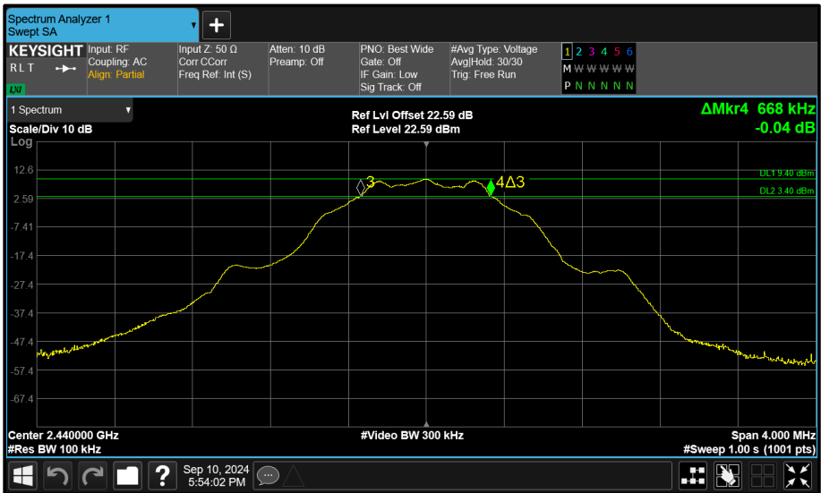
Figure 79 - Core 1 (B) 2440 MHz (CH17) 6 dB Bandwidth
