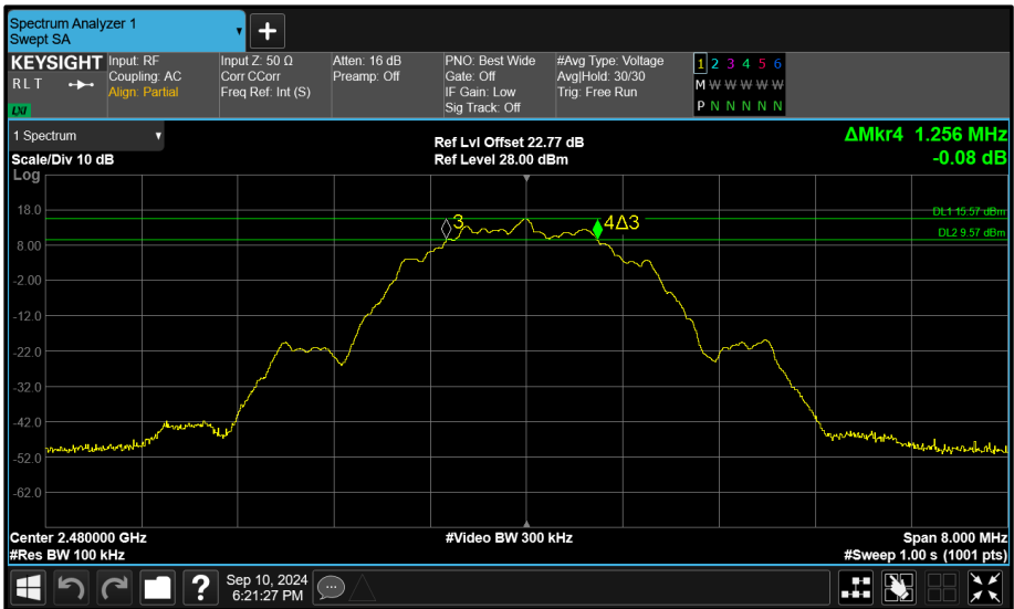
Figure 135 - Core 0 (A) 2480 MHz (CH39) 6 dB Bandwidth
