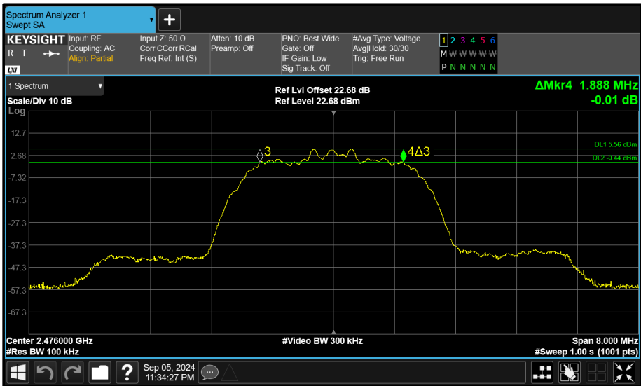
Figure 93 - Core 2 (C) 2476 MHz (CH74) 6 dB Bandwidth
