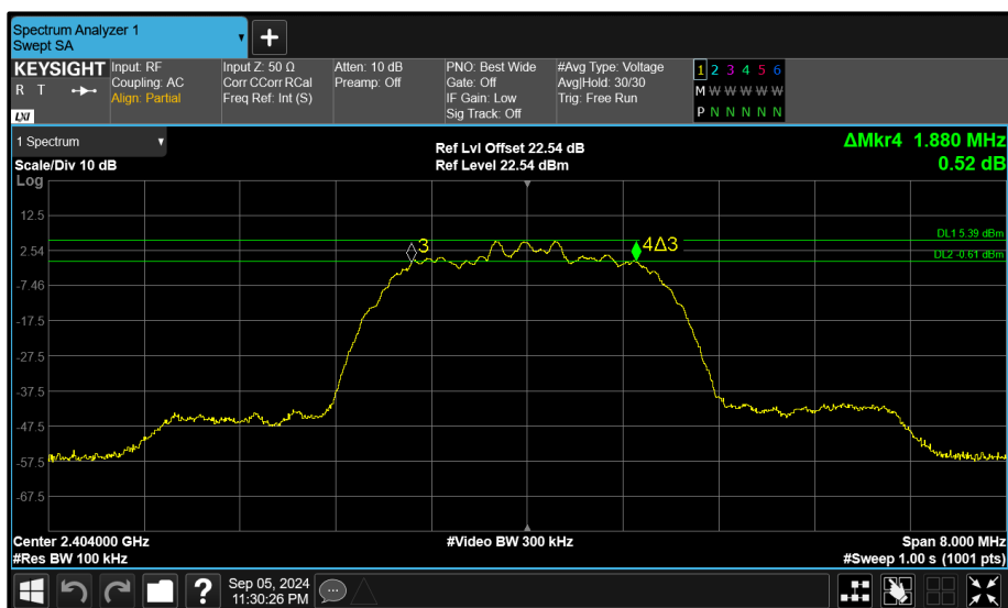
Figure 89 - Core 2 (C) 2404 MHz (CH2) 6 dB Bandwidth
