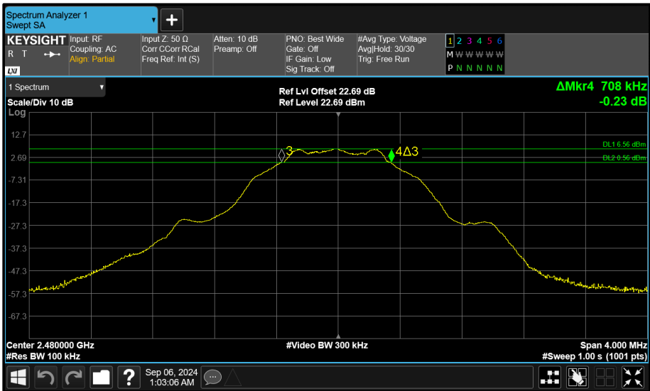
Figure 105 - Core 2 (C) 2480 MHz (CH39) 6 dB Bandwidth
