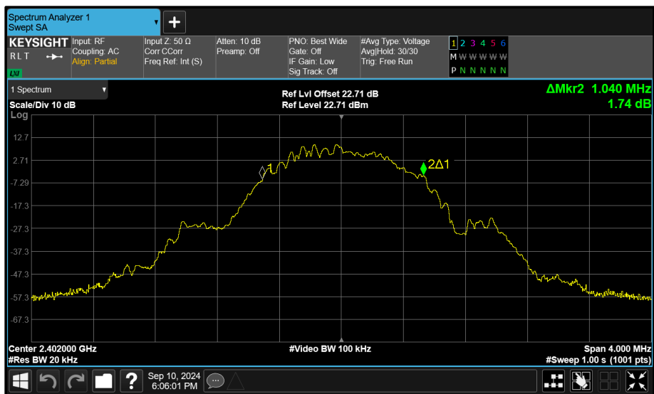
Figure 124 - Core 0 (A) 2402 MHz (CH37) 99% Bandwidth
