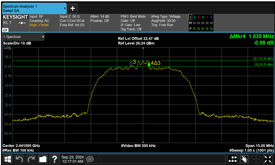
Figure 121 - Core 1 (B) 2441 MHz (CH39) 6 dB Bandwidth
