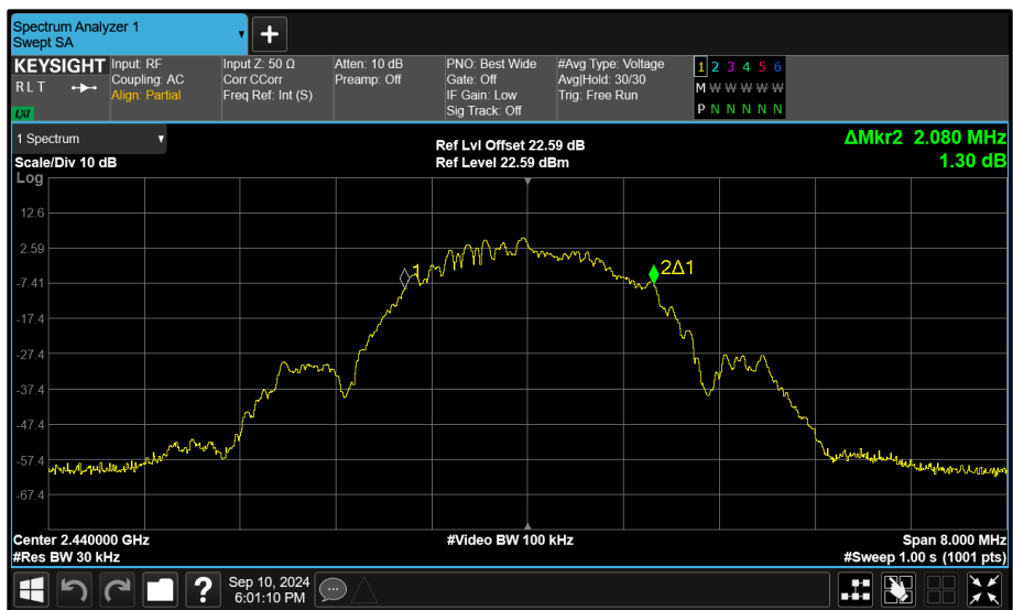
Figure 84 - Core 1 (B) 2440 MHz (CH17) 99% Bandwidth
