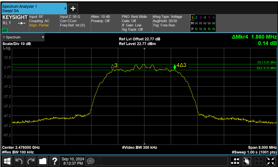
Figure 145 - Core 0 (A) 2476 MHz (CH74) 6 dB Bandwidth
