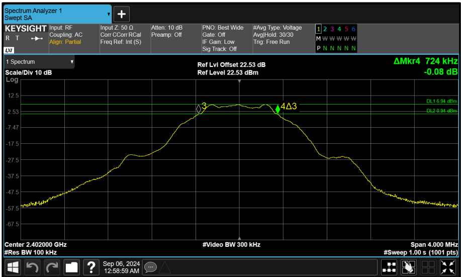
Figure 101 - Core 2 (C) 2402 MHz (CH37) 6 dB Bandwidth
