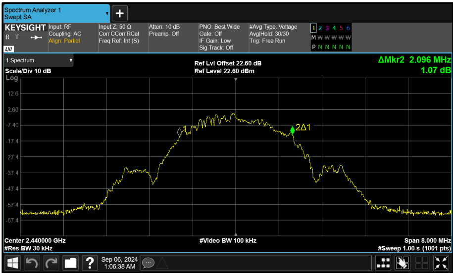
Figure 108 - Core 2 (C) 2440 MHz (CH17) 99% Bandwidth
