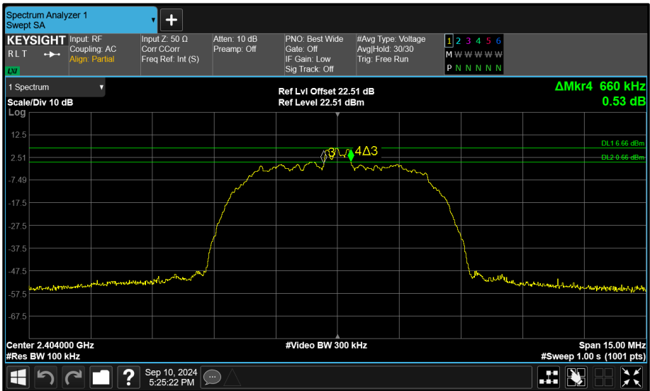
Figure 71 - Core 1 (B) 2404 MHz (CH2) 6 dB Bandwidth
