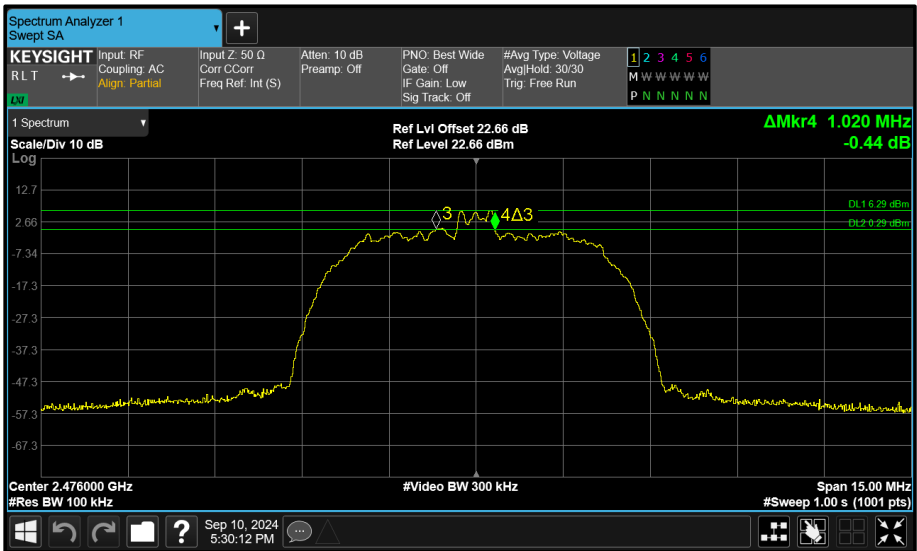
Figure 75 - Core 1 (B) 2476 MHz (CH74) 6 dB Bandwidth
