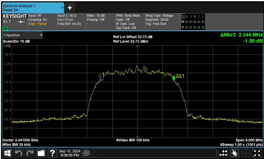
Figure 140 - Core 0 (A) 2441 MHz (CH39) 99% Bandwidth
