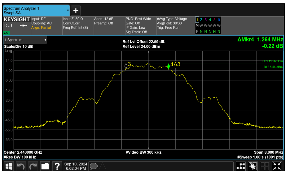
Figure 85 - Core 1 (B) 2440 MHz (CH17) 6 dB Bandwidth
