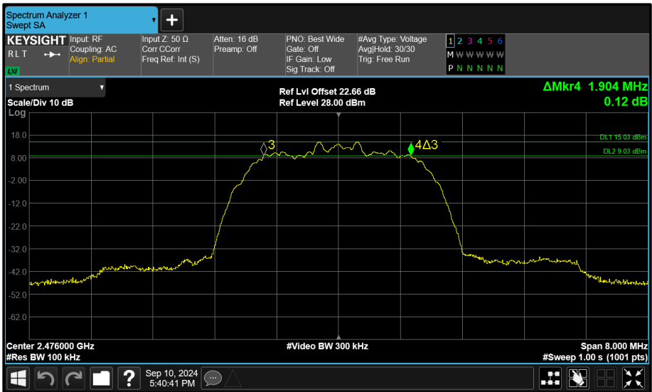
Figure 117 - Core 1 (B) 2476 MHz (CH74) 6 dB Bandwidth
