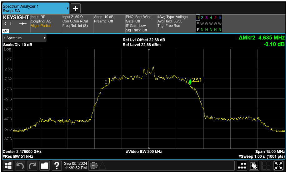
Figure 98 - Core 2 (C) 2476 MHz (CH74) 99% Bandwidth
