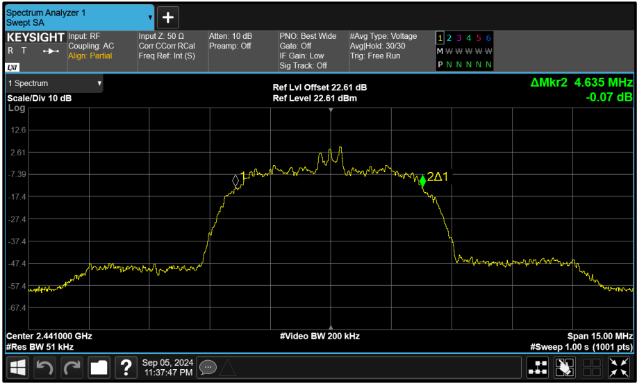
Figure 96 - Core 2 (C) 2441 MHz (CH39) 99% Bandwidth
