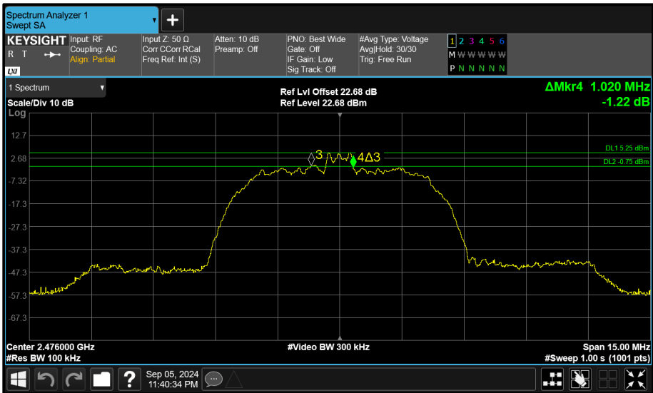
Figure 99 - Core 2 (C) 2476 MHz (CH74) 6 dB Bandwidth
