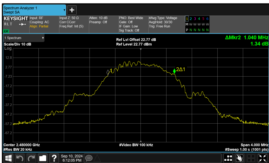
Figure 128 - Core 0 (A) 2480 MHz (CH39) 99% Bandwidth
