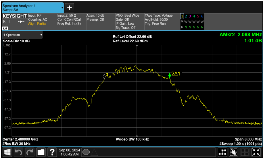
Figure 110 - Core 2 (C) 2480 MHz (CH39) 99% Bandwidth
