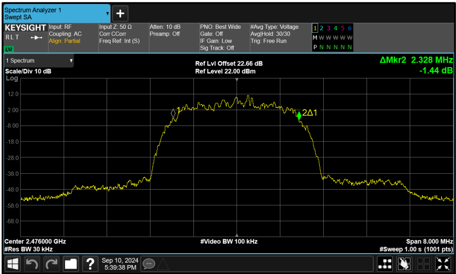
Figure 116 - Core 1 (B) 2476 MHz (CH74) 99% Bandwidth
