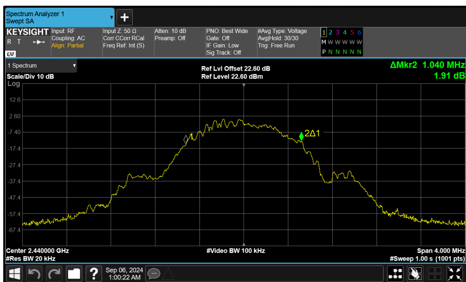
Figure 102 - Core 2 (C) 2440 MHz (CH17) 99% Bandwidth
