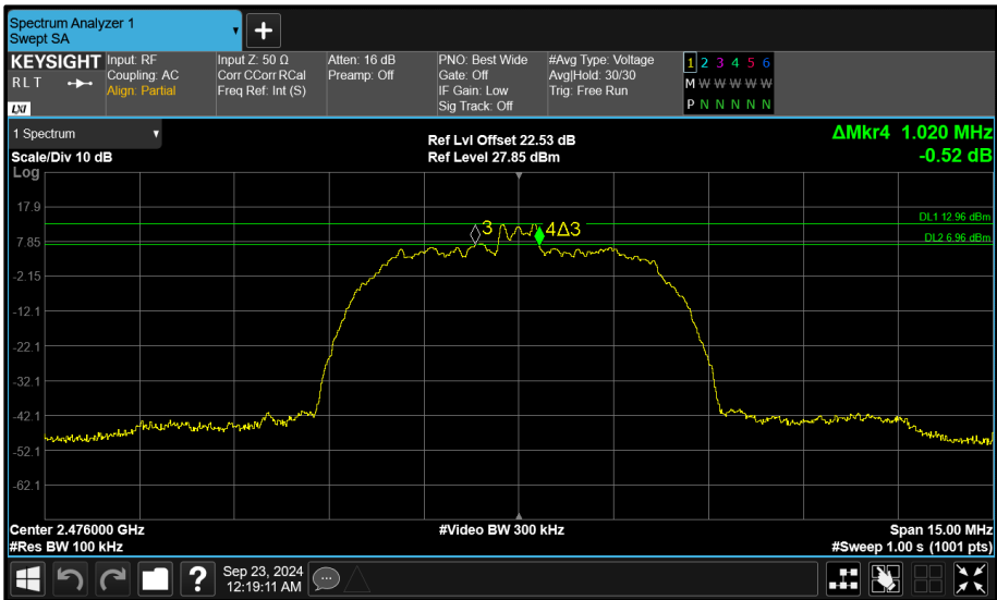
Figure 123 - Core 1 (B) 2476 MHz (CH74) 6 dB Bandwidth
