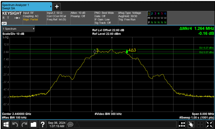
Figure 109 - Core 2 (C) 2440 MHz (CH17) 6 dB Bandwidth
