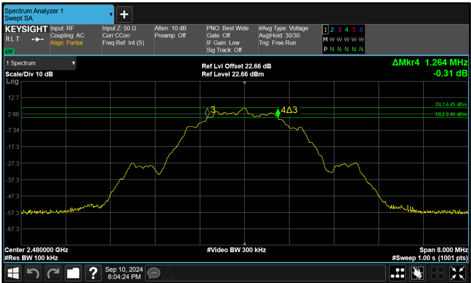
Figure 87 - Core 1 (B) 2480 MHz (CH39) 6 dB Bandwidth
