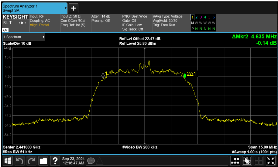
Figure 120 - Core 1 (B) 2441 MHz (CH39) 99% Bandwidth
