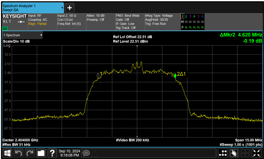
Figure 150 - Core 1 (B) 2404 MHz (CH2) 99% Bandwidth
