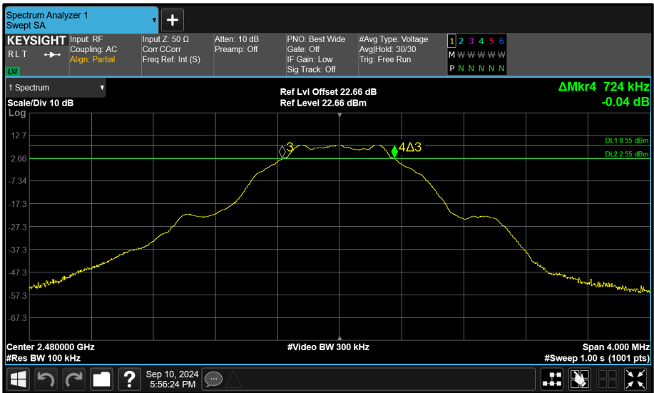
Figure 81 - Core 1 (B) 2480 MHz (CH39) 6 dB Bandwidth
