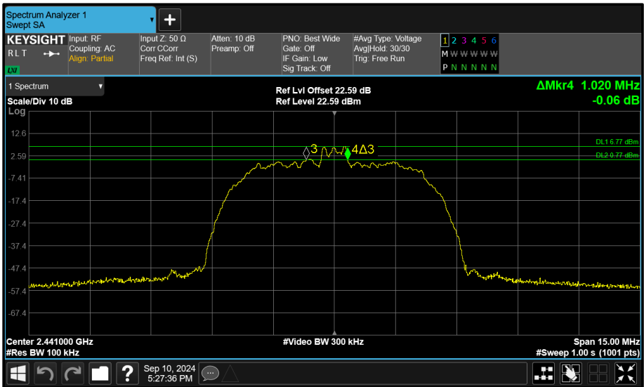
Figure 73 - Core 1 (B) 2441 MHz (CH39) 6 dB Bandwidth
