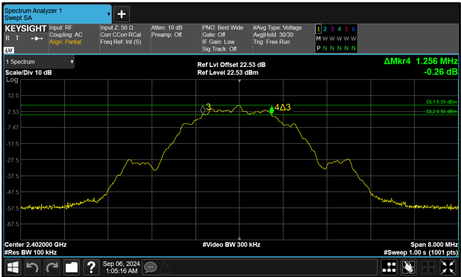
Figure 107 - Core 2 (C) 2402 MHz (CH37) 6 dB Bandwidth
