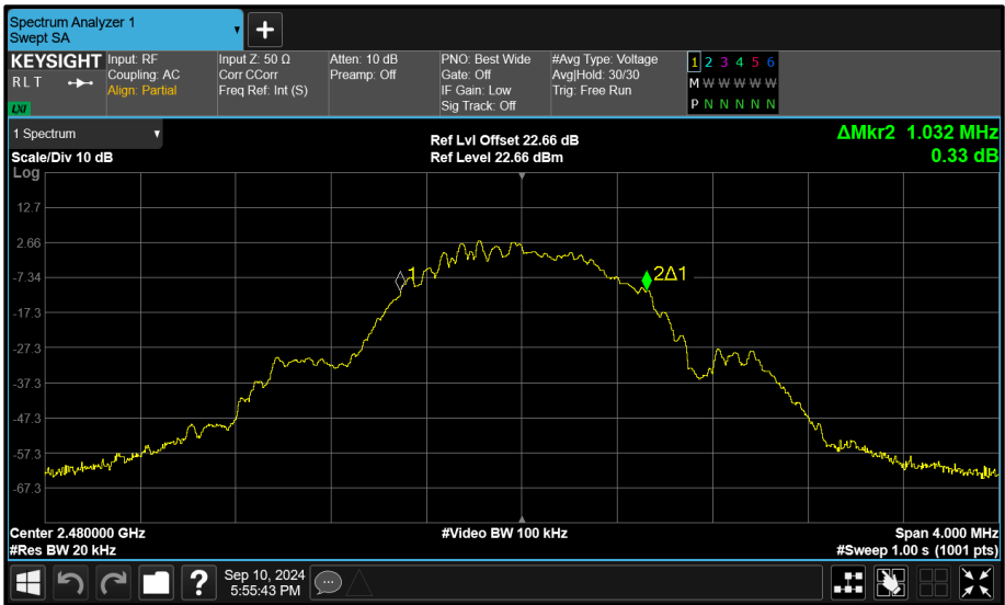
Figure 80 - Core 1 (B) 2480 MHz (CH39) 99% Bandwidth
