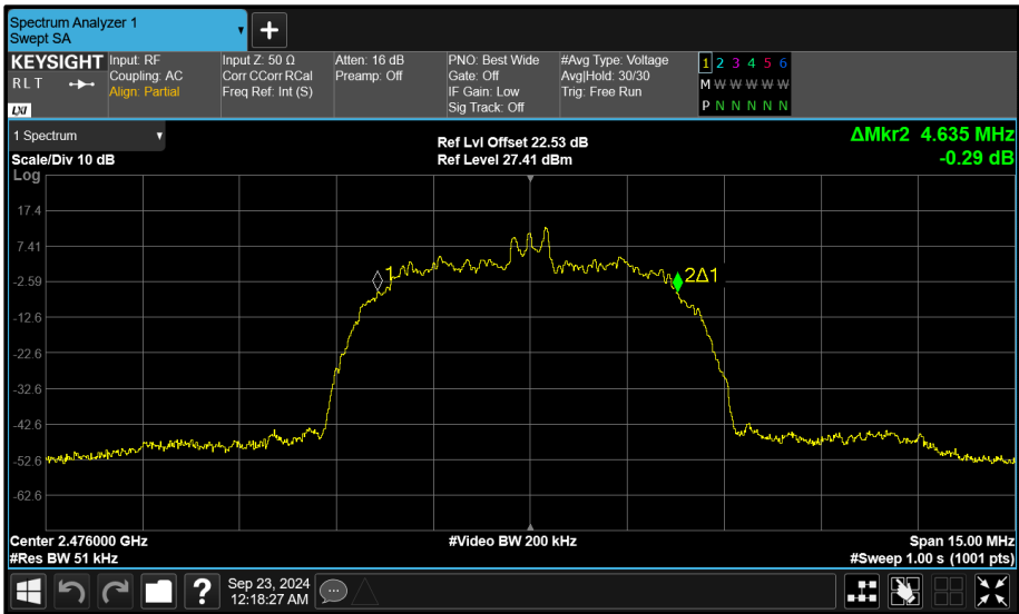
Figure 122 - Core 1 (B) 2476 MHz (CH74) 99% Bandwidth
