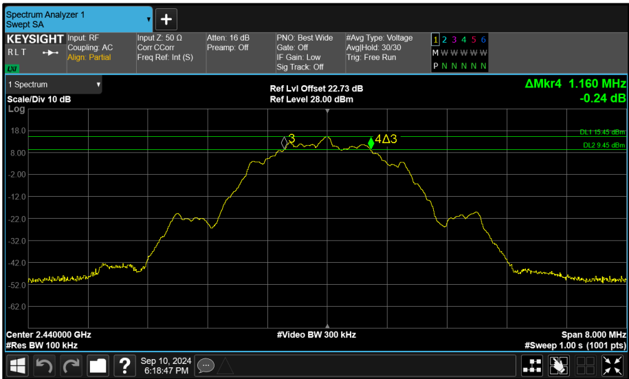
Figure 133 - Core 0 (A) 2440 MHz (CH17) 6 dB Bandwidth
