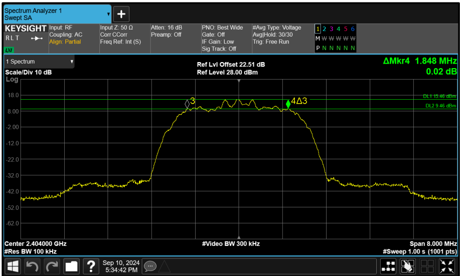
Figure 113 - Core 1 (B) 2404 MHz (CH2) 6 dB Bandwidth
