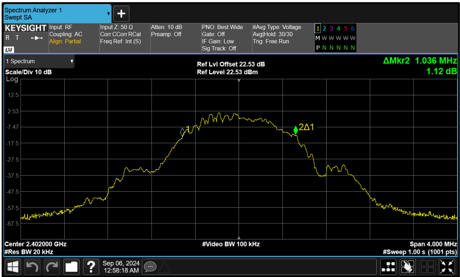
Figure 100 - Core 2 (C) 2402 MHz (CH37) 99% Bandwidth
