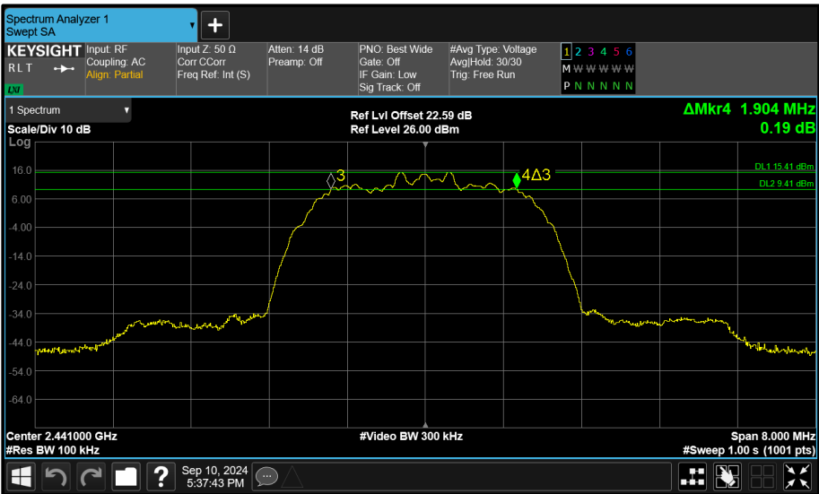
Figure 115 - Core 1 (B) 2441 MHz (CH39) 6 dB Bandwidth
