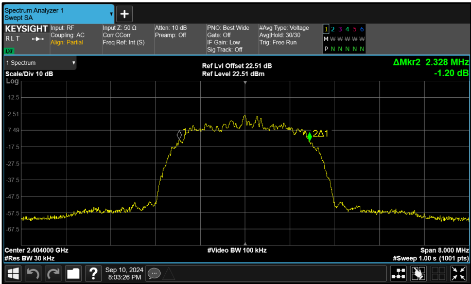
Figure 138 - Core 1 (B) 2404 MHz (CH2) 99% Bandwidth
