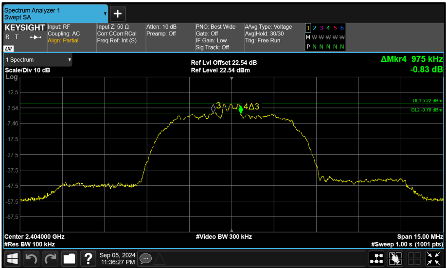
Figure 95 - Core 2 (C) 2404 MHz (CH2) 6 dB Bandwidth
