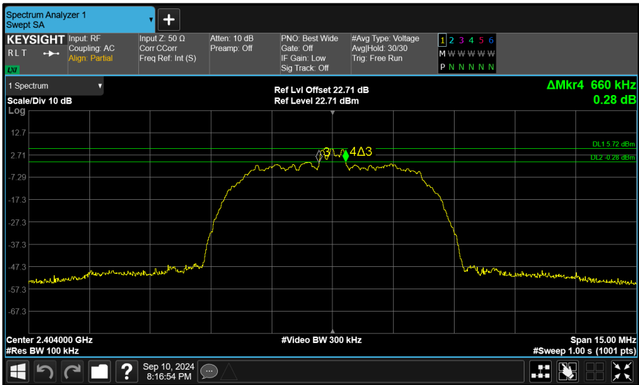
Figure 149 - Core 0 (A) 2404 MHz (CH2) 6 dB Bandwidth
