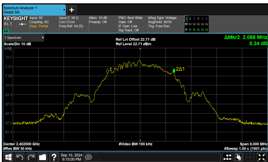
Figure 130 - Core 0 (A) 2402 MHz (CH37) 99% Bandwidth
