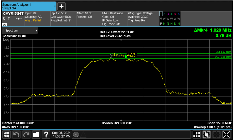
Figure 97 - Core 2 (C) 2441 MHz (CH39) 6 dB Bandwidth
