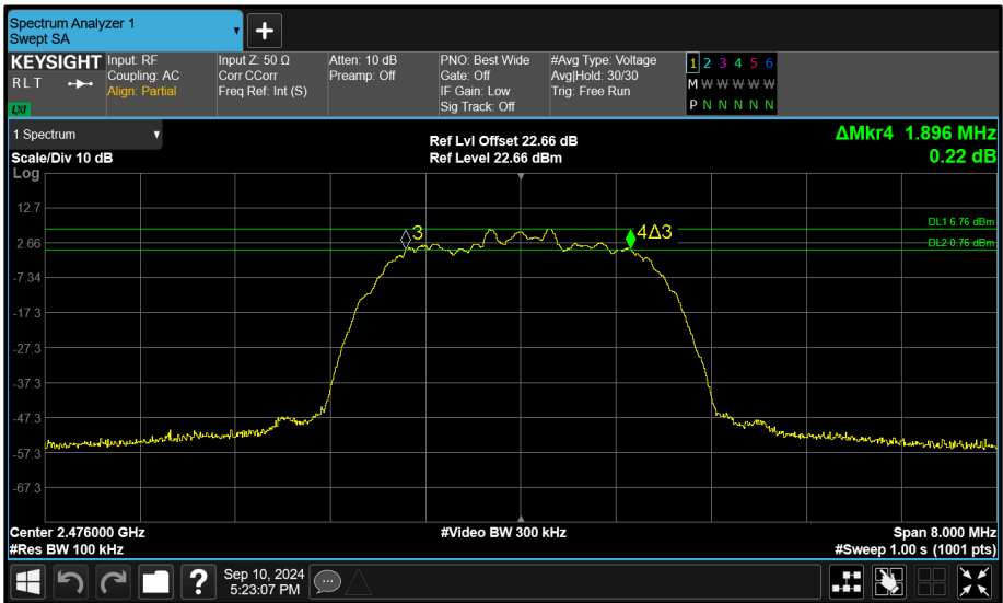
Figure 69 - Core 1 (B) 2476 MHz (CH74) 6 dB Bandwidth
