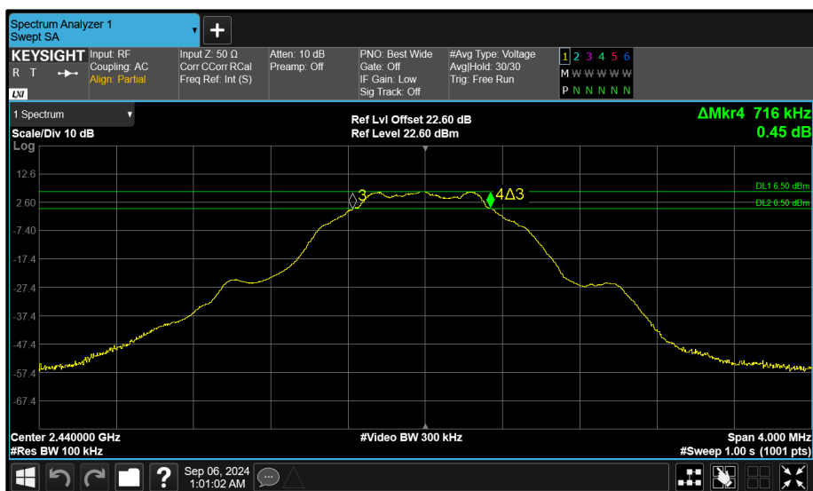
Figure 103 - Core 2 (C) 2440 MHz (CH17) 6 dB Bandwidth
