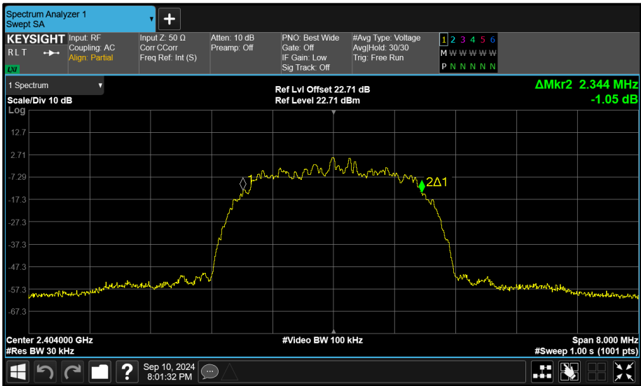
Figure 136 - Core 0 (A) 2404 MHz (CH2) 99% Bandwidth
