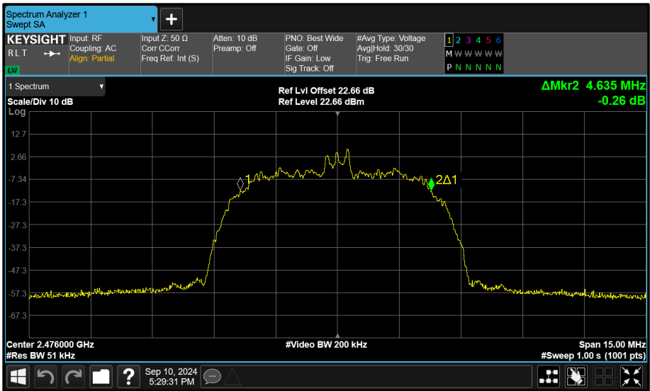
Figure 74 - Core 1 (B) 2476 MHz (CH74) 99% Bandwidth
