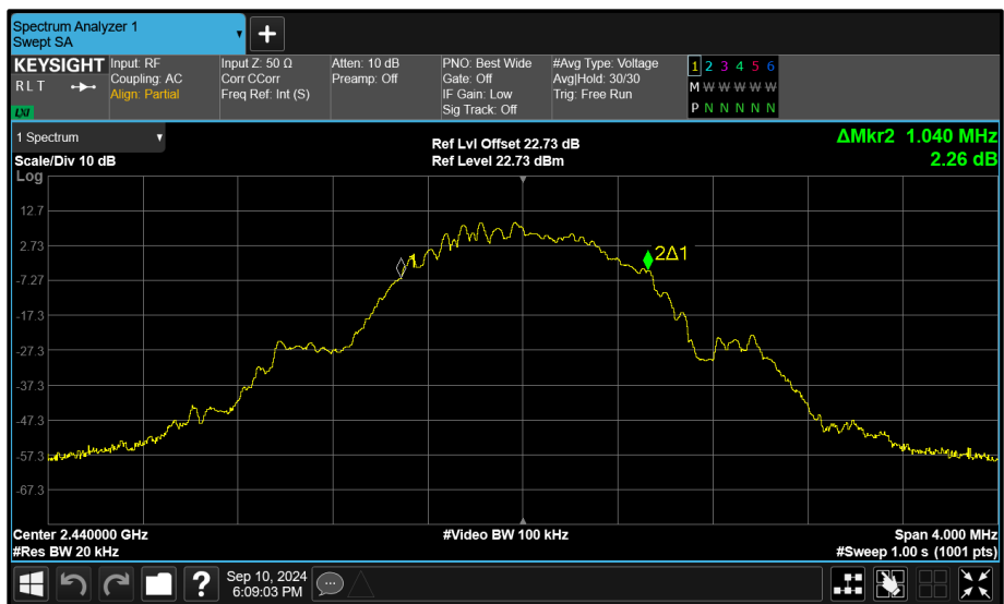
Figure 126 - Core 0 (A) 2440 MHz (CH17) 99% Bandwidth
